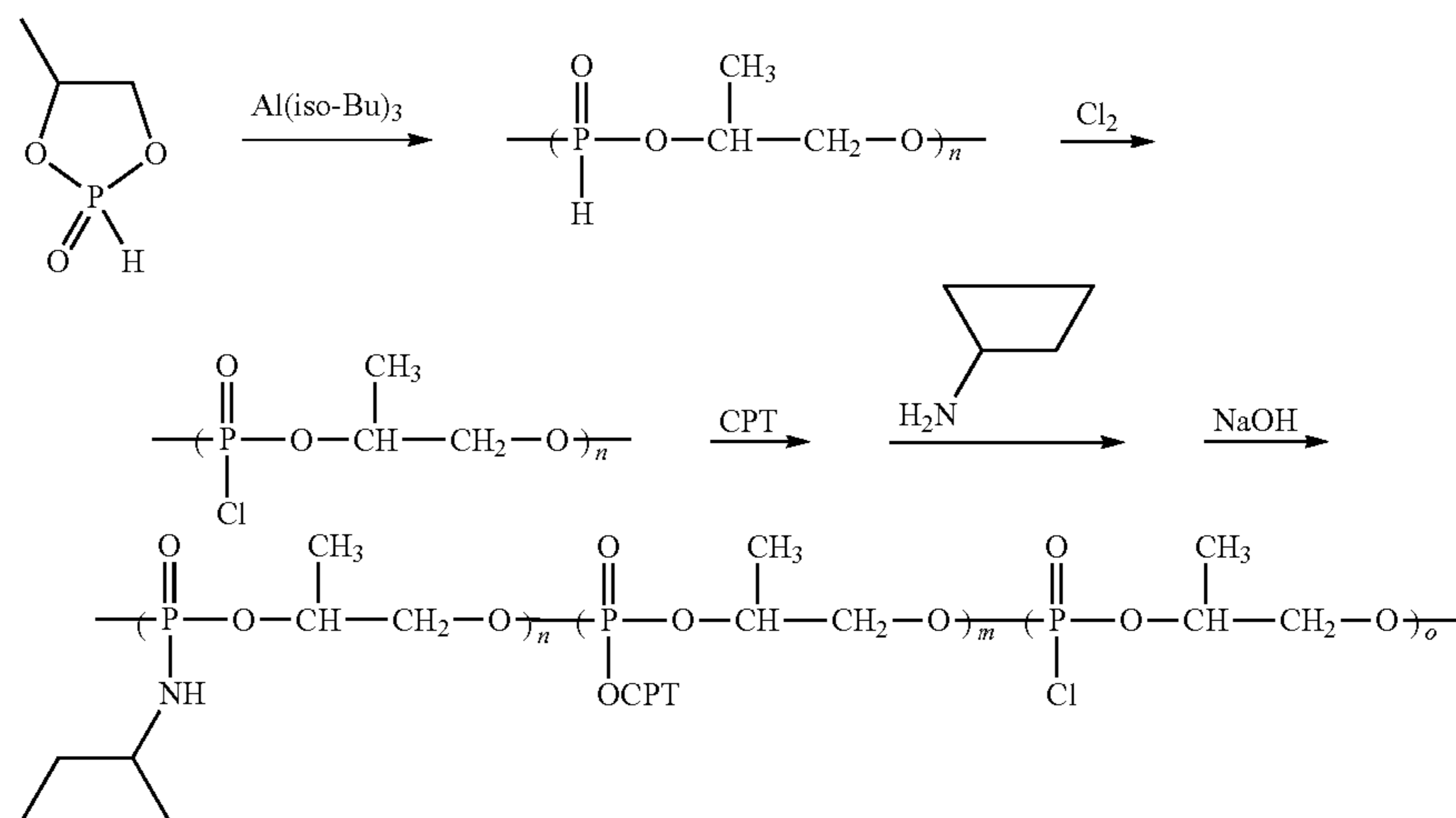
Scheme IX
