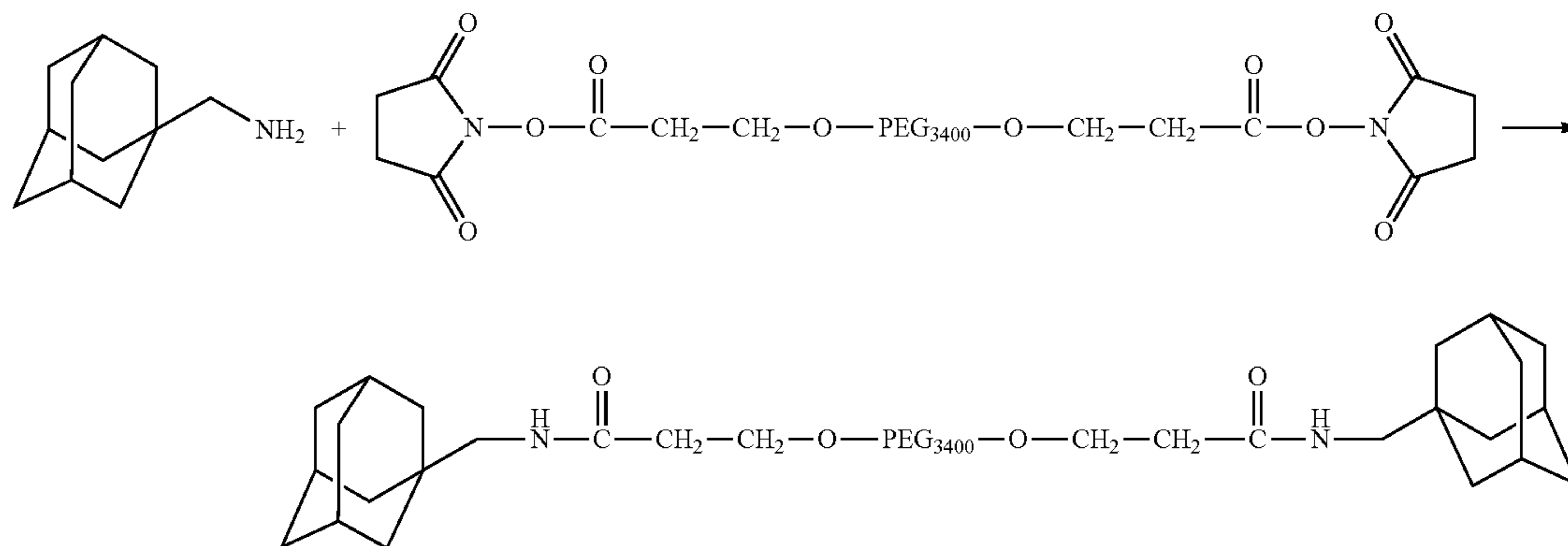
Scheme XXXXVI
