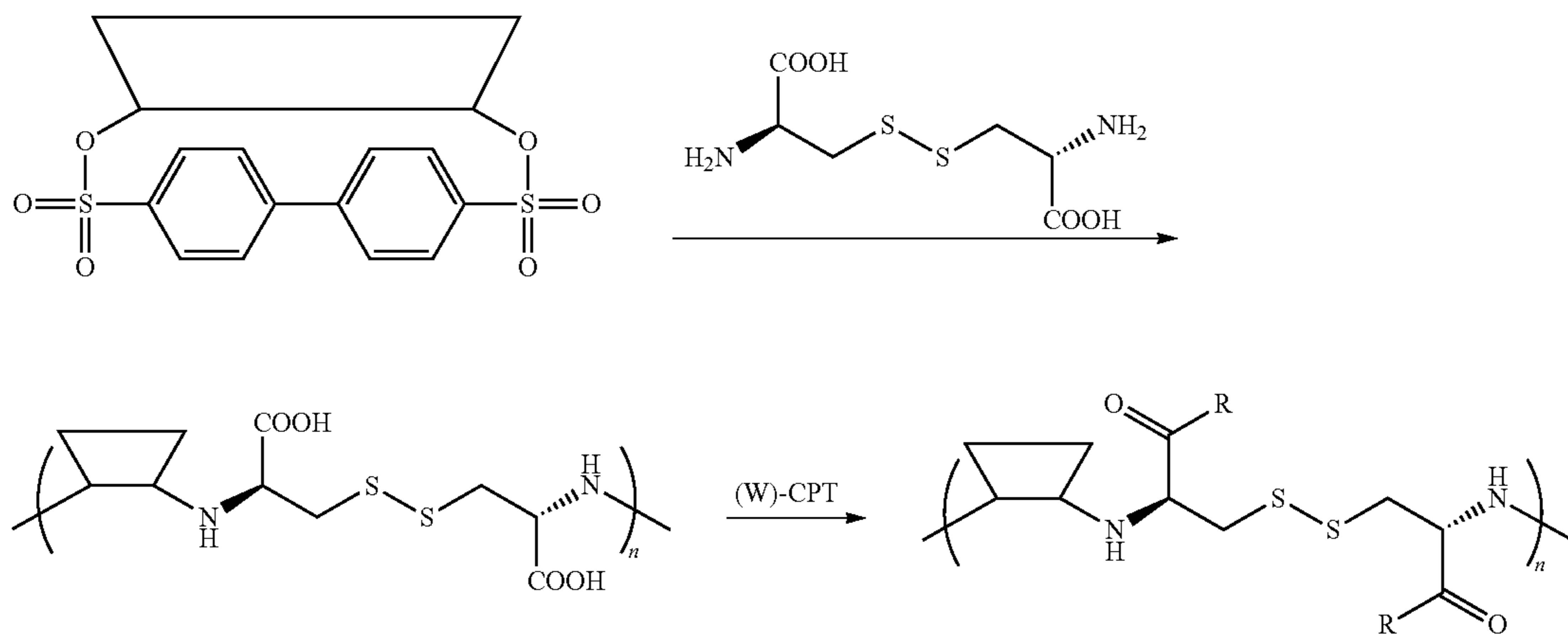
Scheme III
