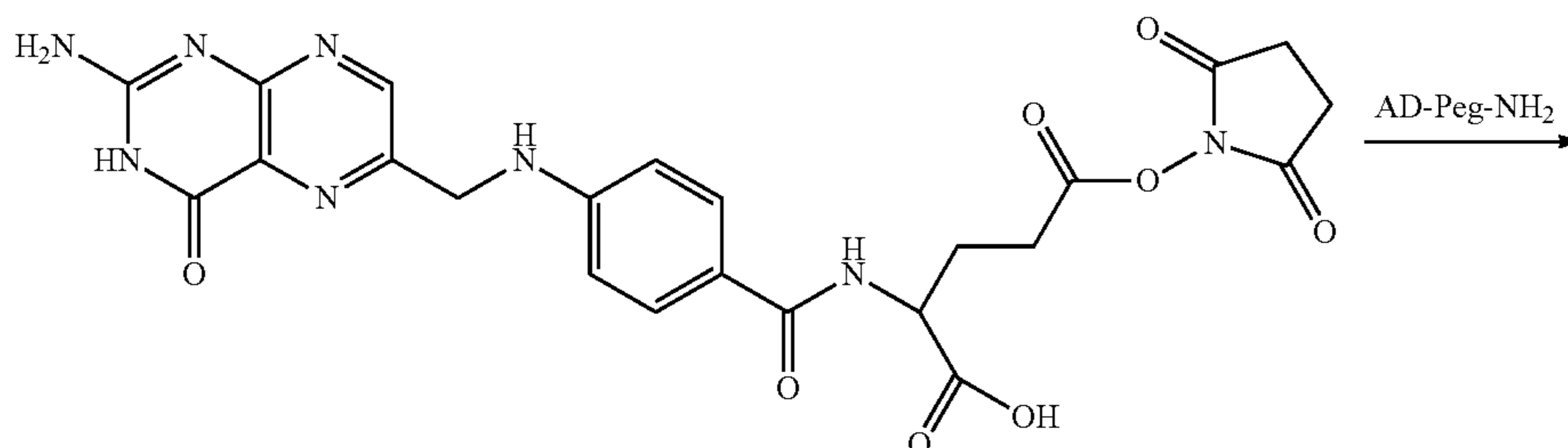
Scheme L
