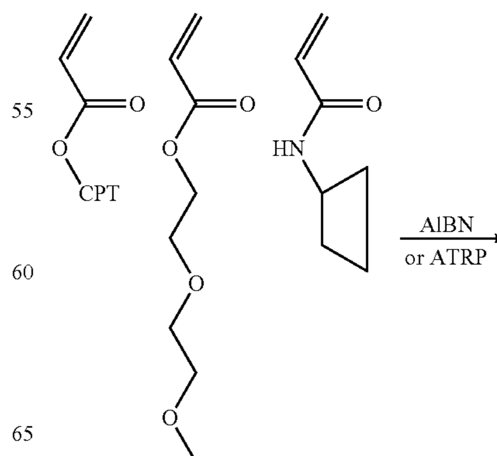
Scheme XXXV
