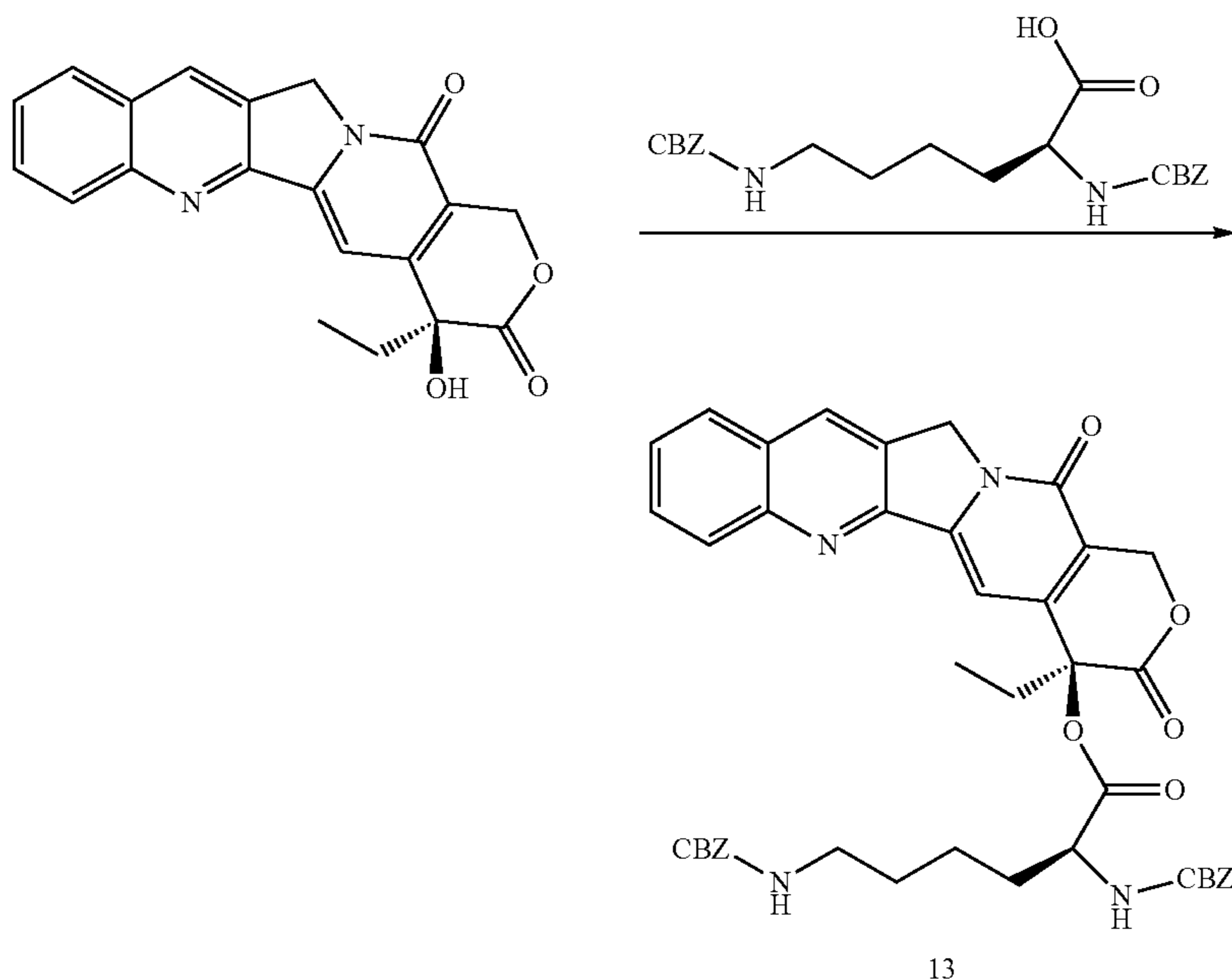
Scheme XXVII
