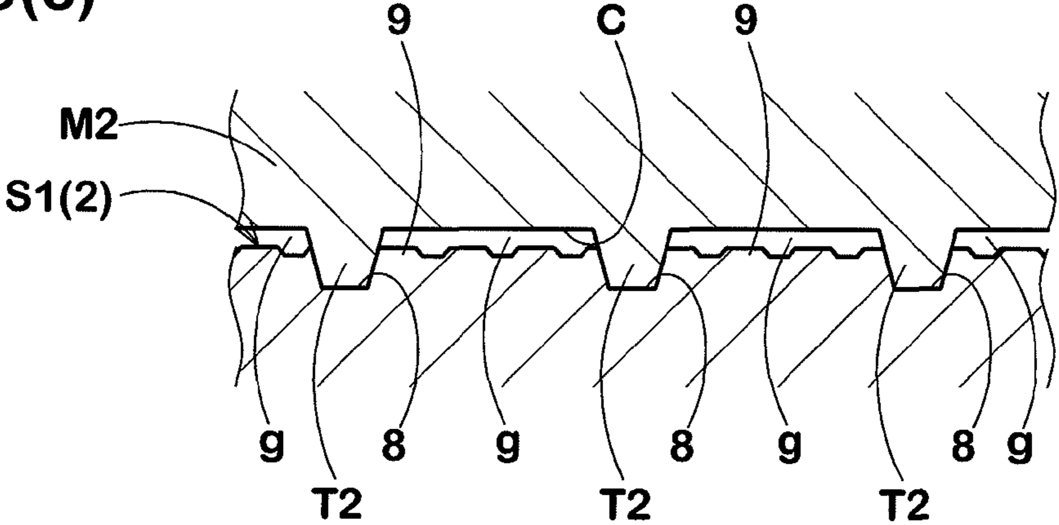
FIG.9(c)
