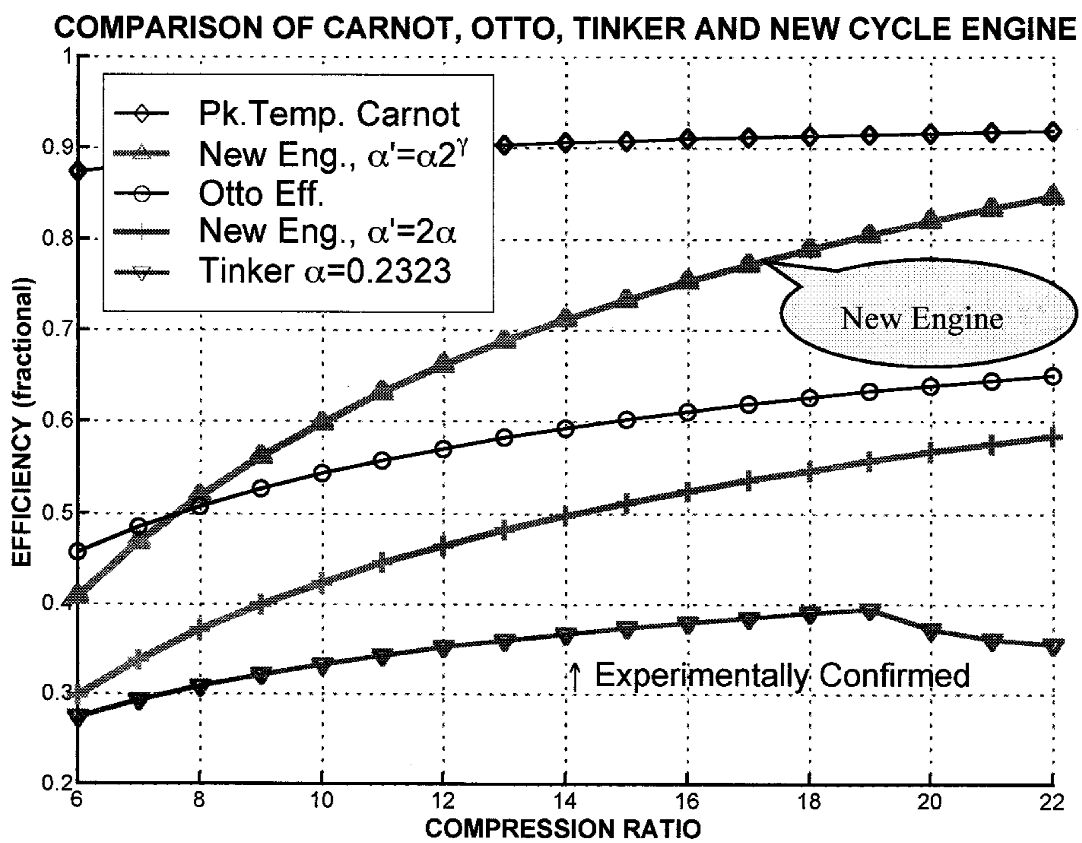
Thermal to Mechanical Conversion Efficiency of New Engine.
