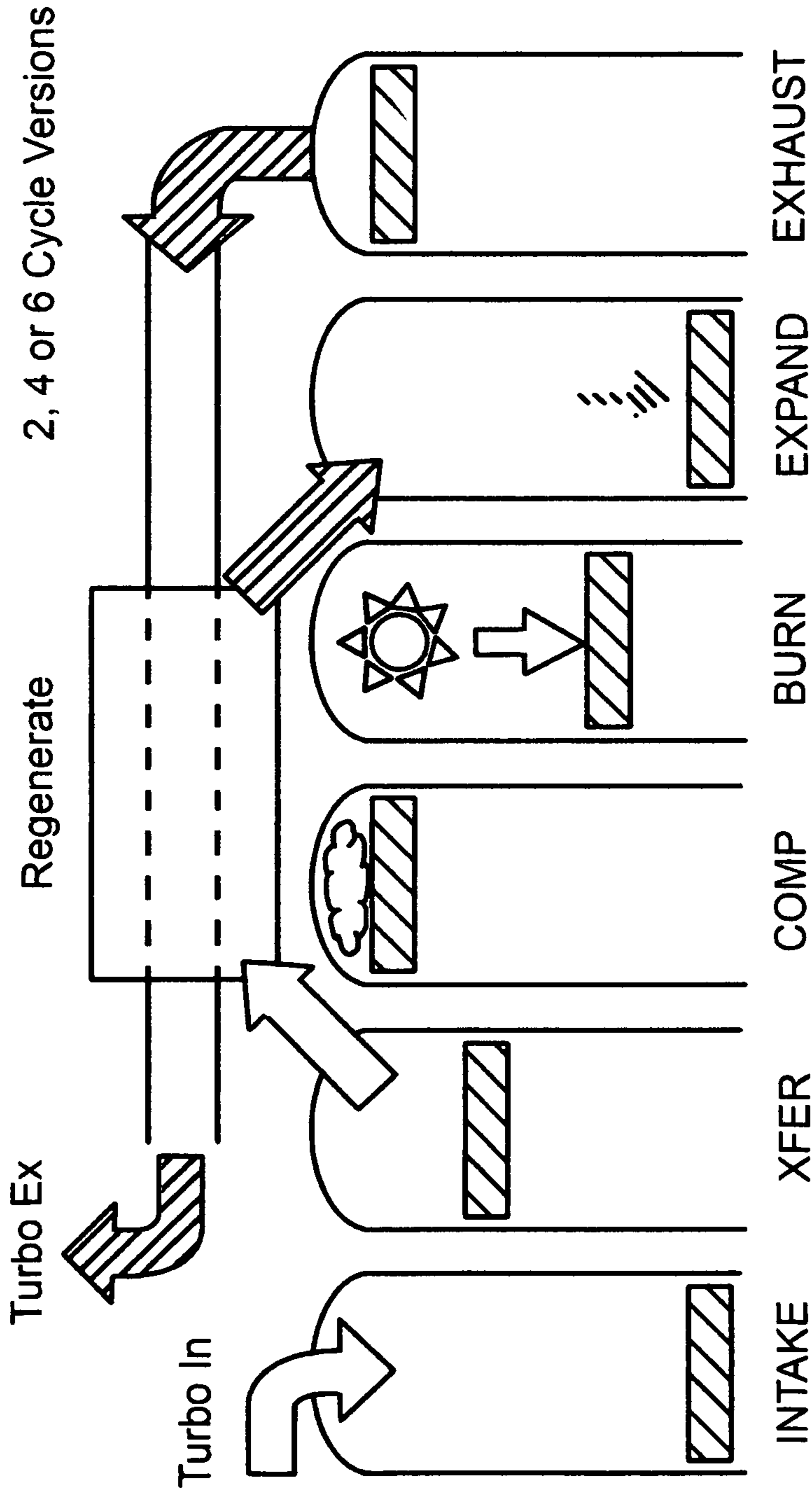
Extremely High Efficiency 4-Cycle, 7-Phase Engine
