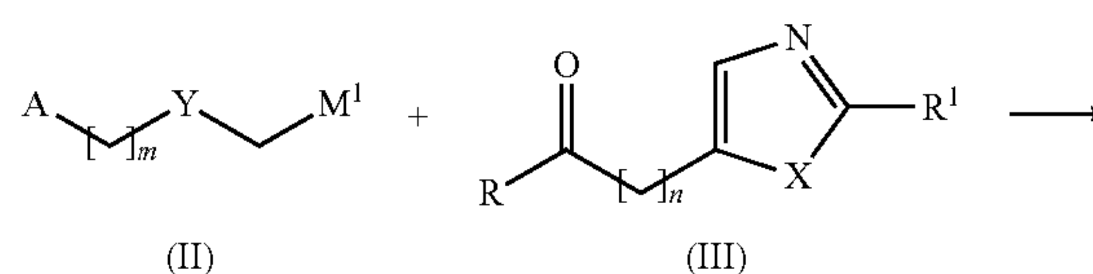
Scheme 1: Process A
