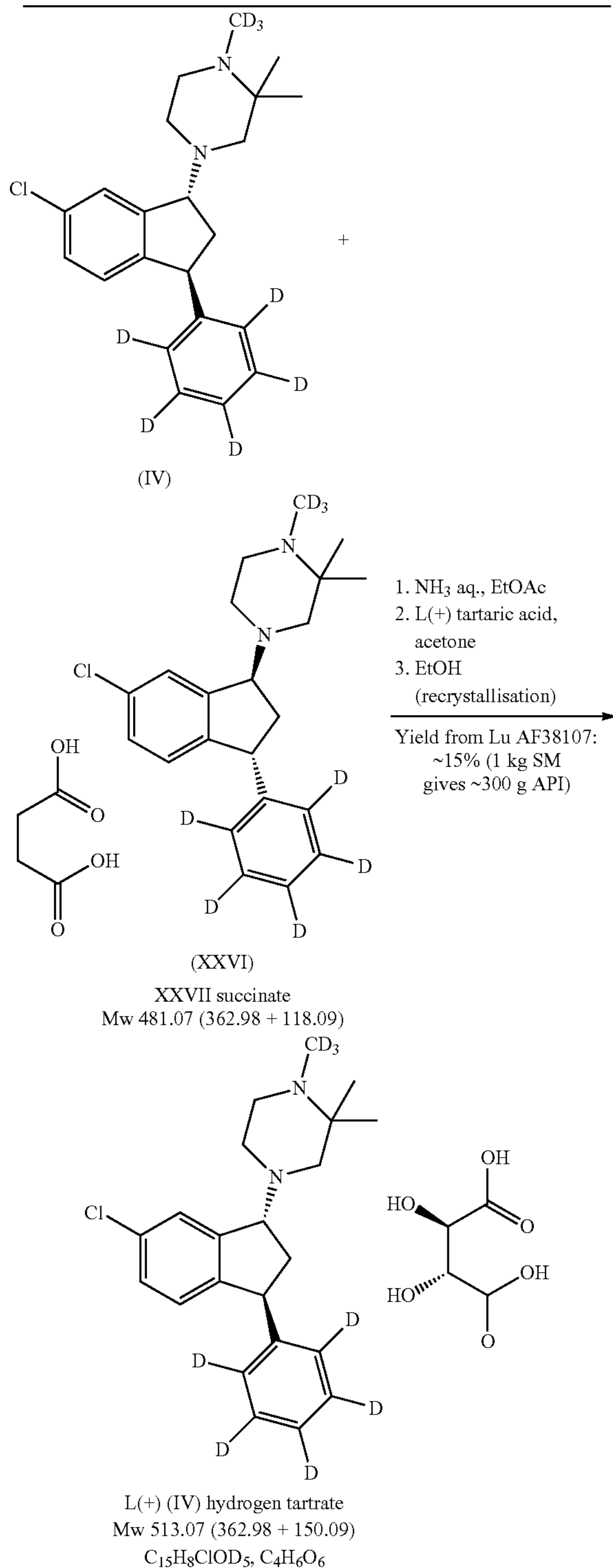
Scheme 18. Synthesis of 4-((1R,3S)-6-chloro-3-phenyl( d_5 )-indan-1-yl)-1( d_3 ), 2,2-trimethyl-piperazine L(+)-hydrogen tartrate.
