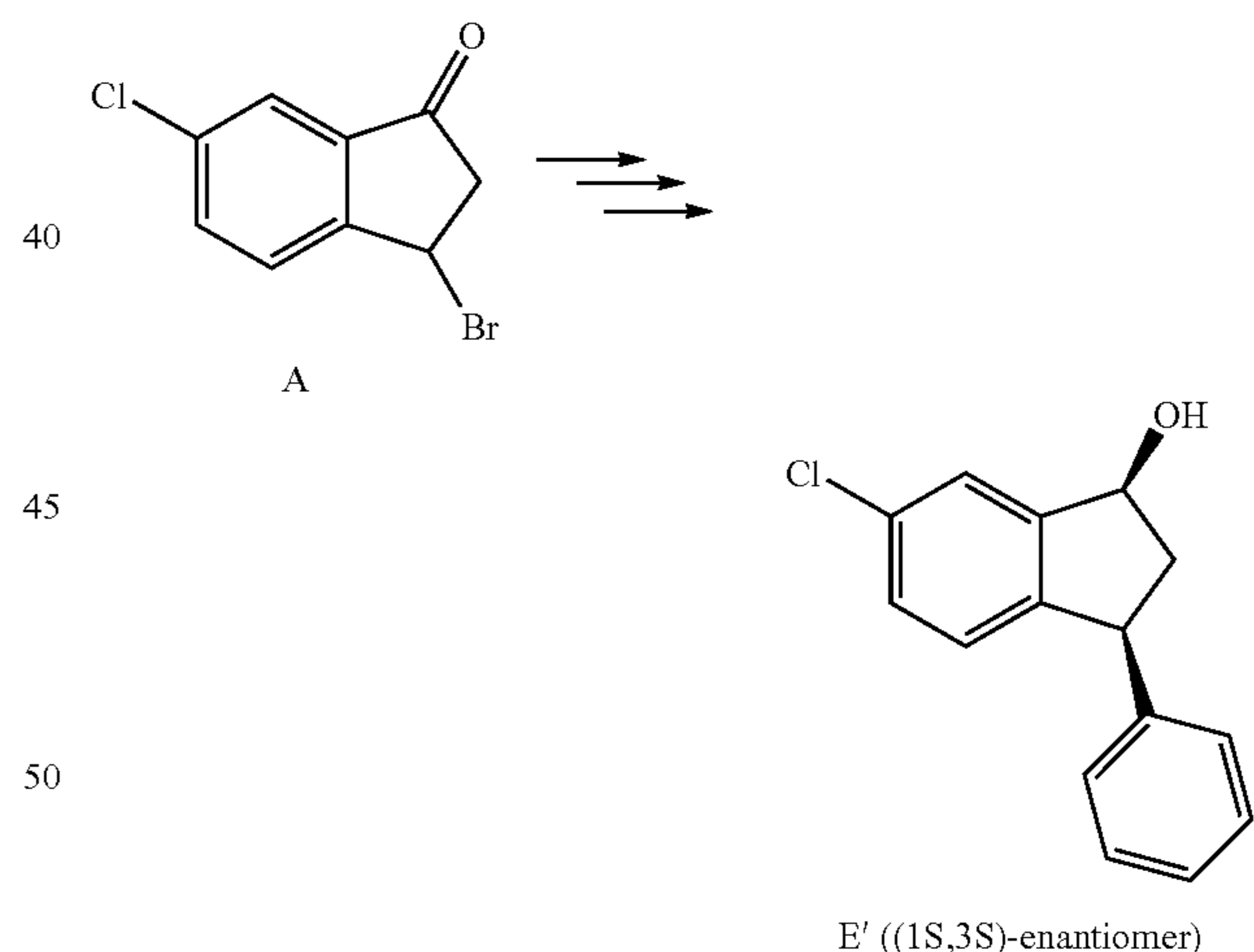
Scheme 3. Exemplary synthesis of intermediate E'.
