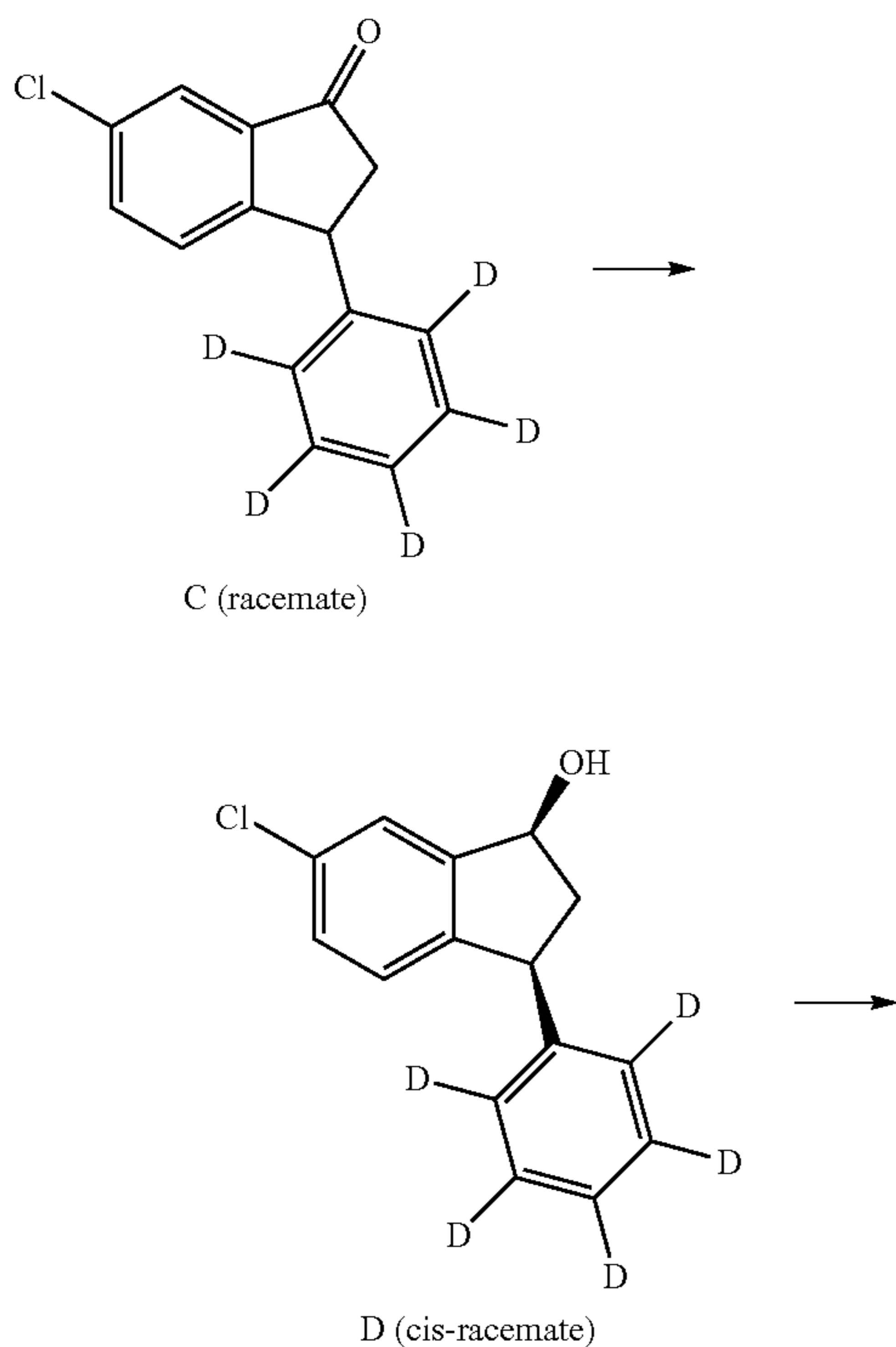
Scheme 10. Synthesis and resolution of Compound E.
