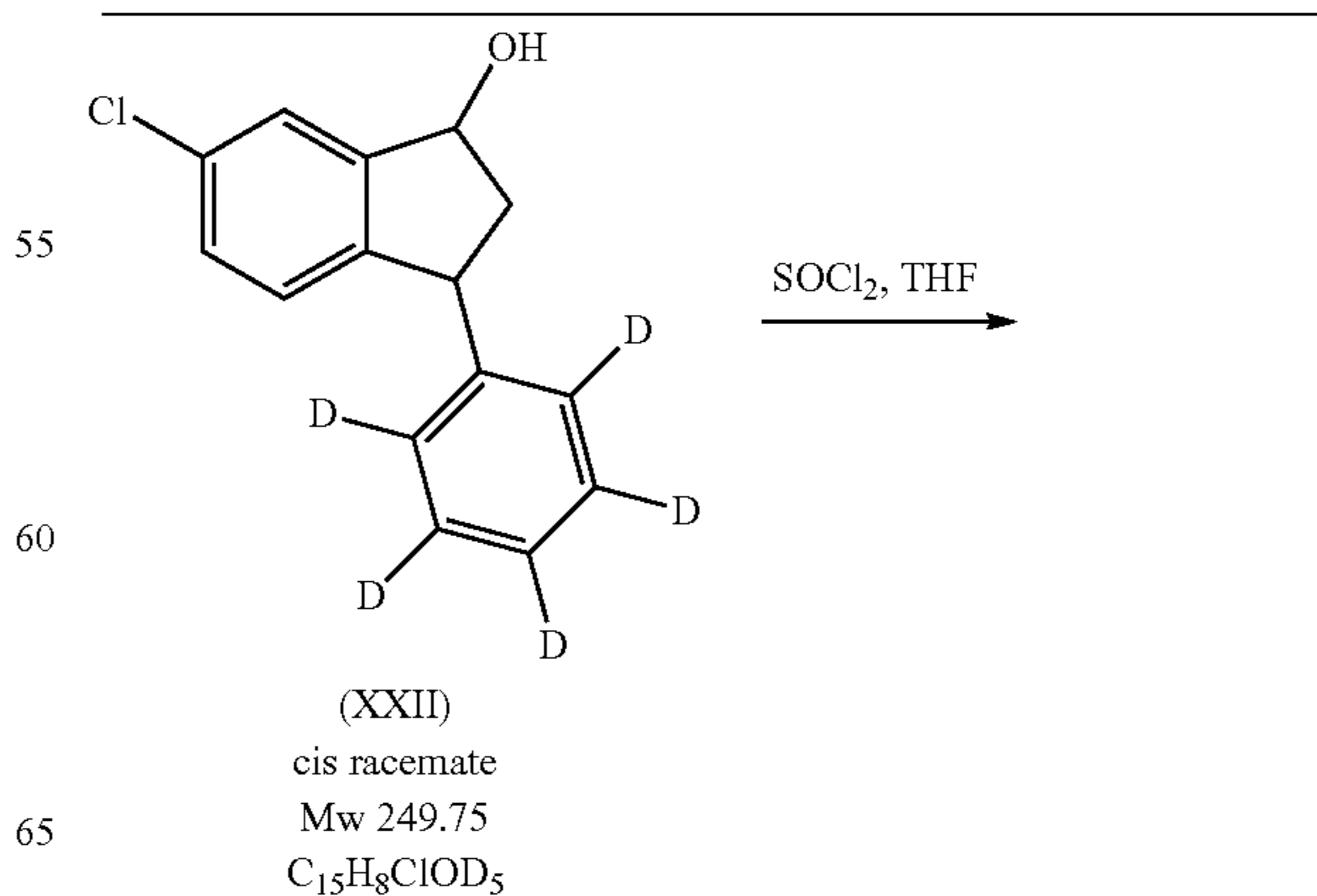
Scheme 16. Synthesis of rac-trans-1-(6-Chloro-3-phenyl(d 5 )-indan-1-yl)-3,3-dimethyl-piperazine maleate
