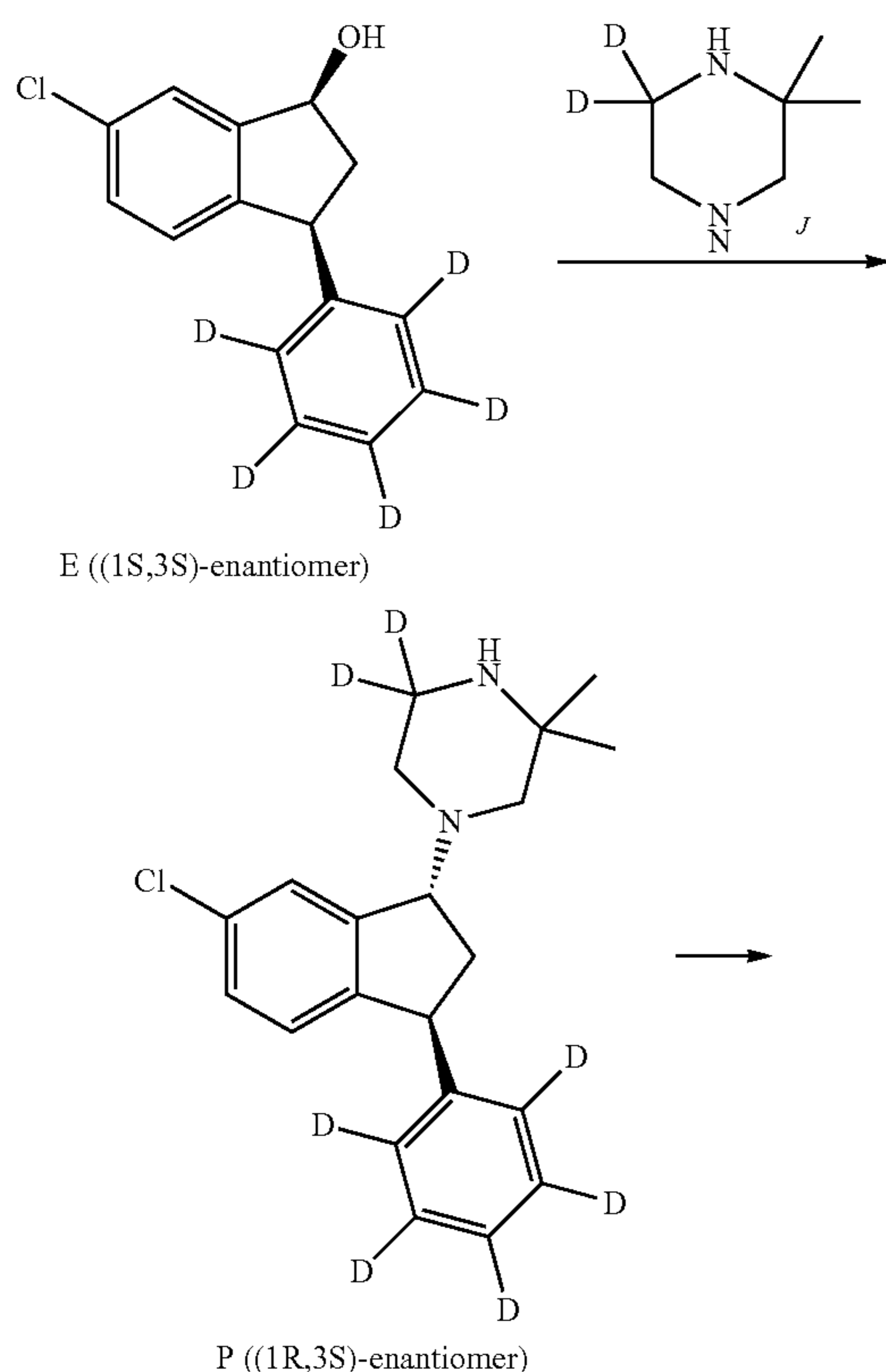
Scheme 13. Synthesis of Compound (VI) and Compound (VII).
