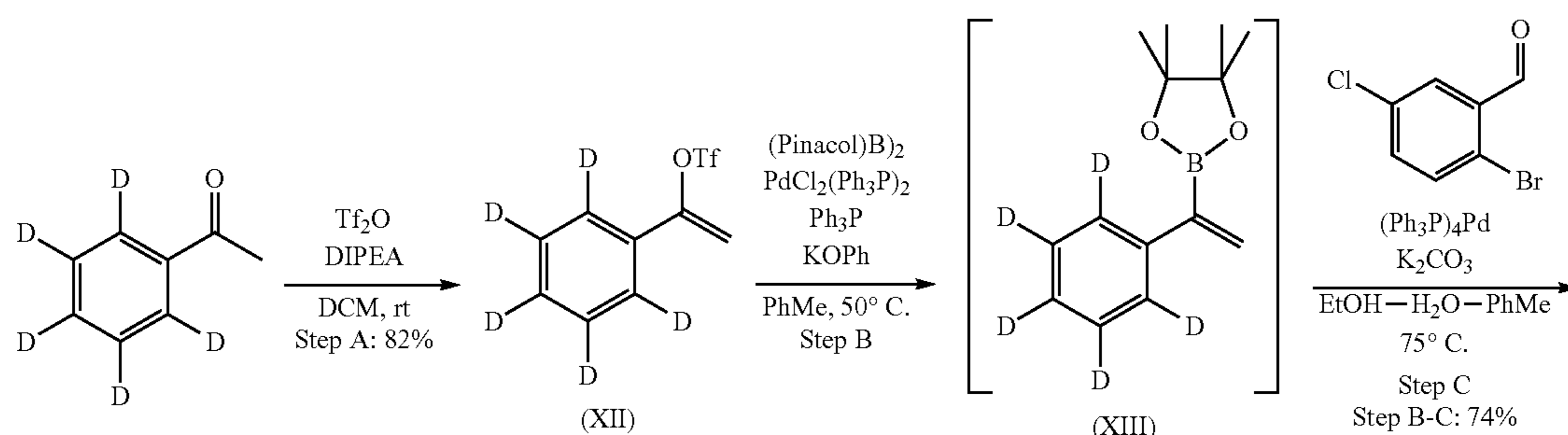
Scheme 14. Synthesis of Compound (XV)
