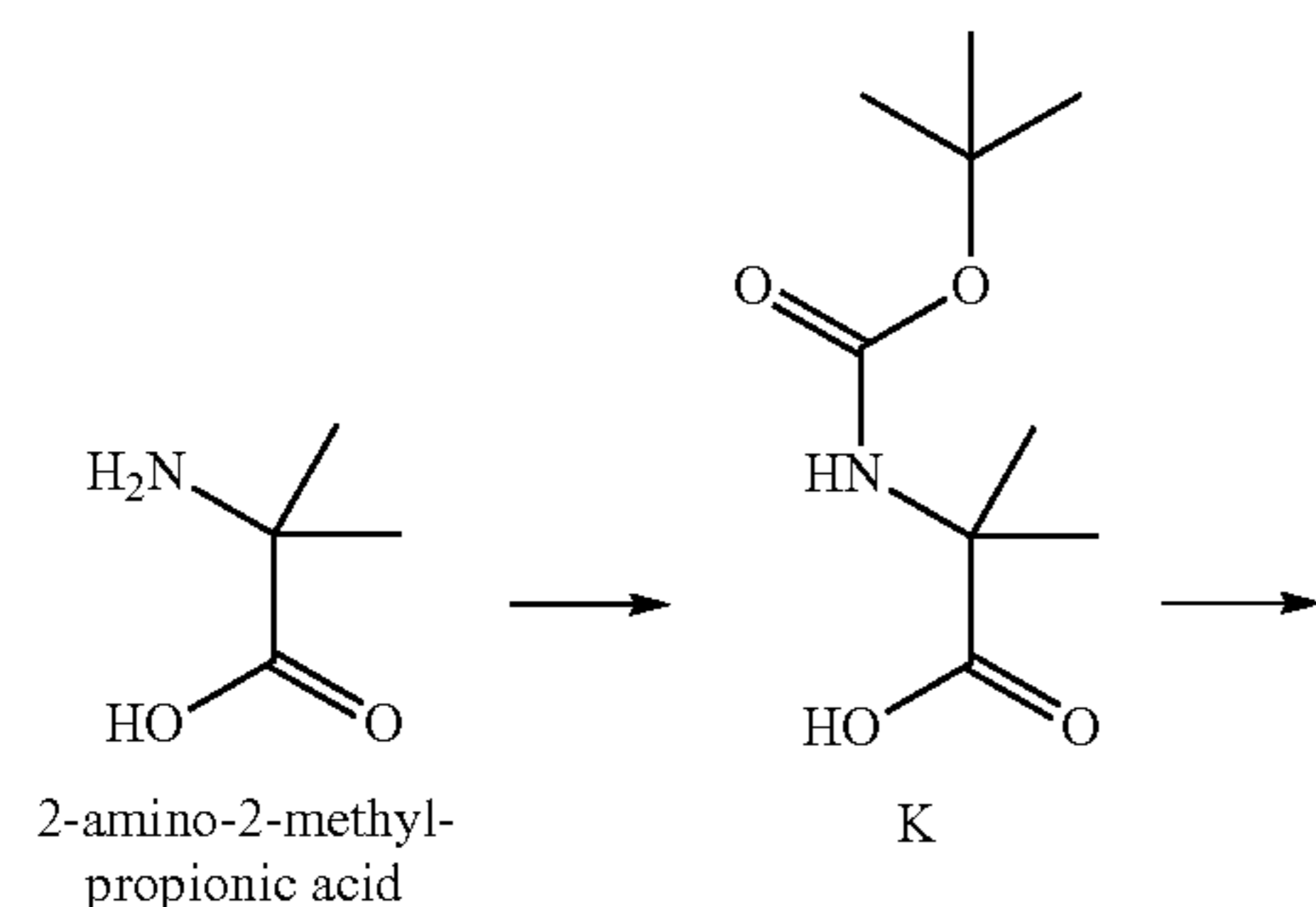
Scheme 7. Alternative exemplary synthesis of intermediate J.
