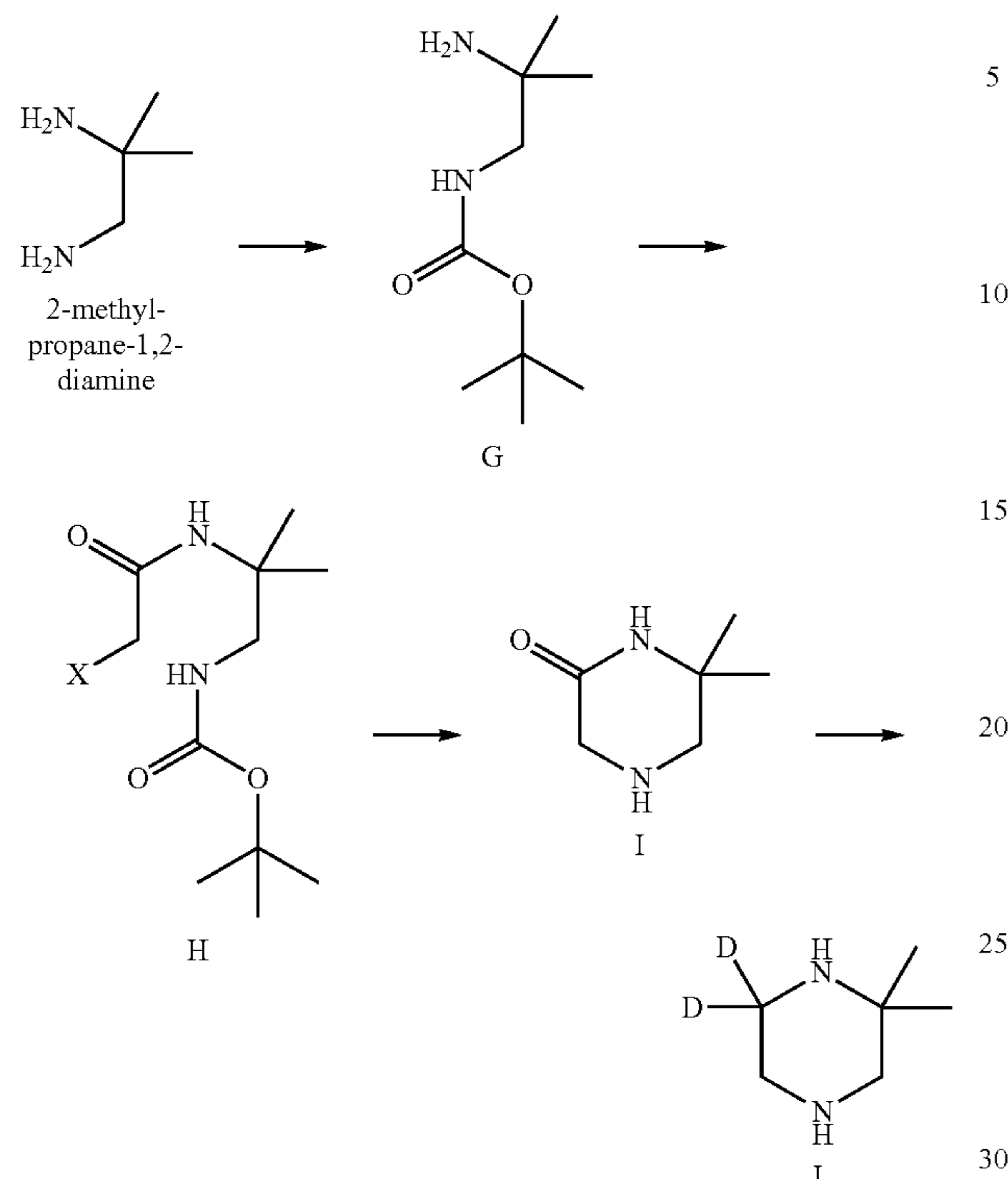
Scheme 6. Exemplary synthesis of intermediate J.
