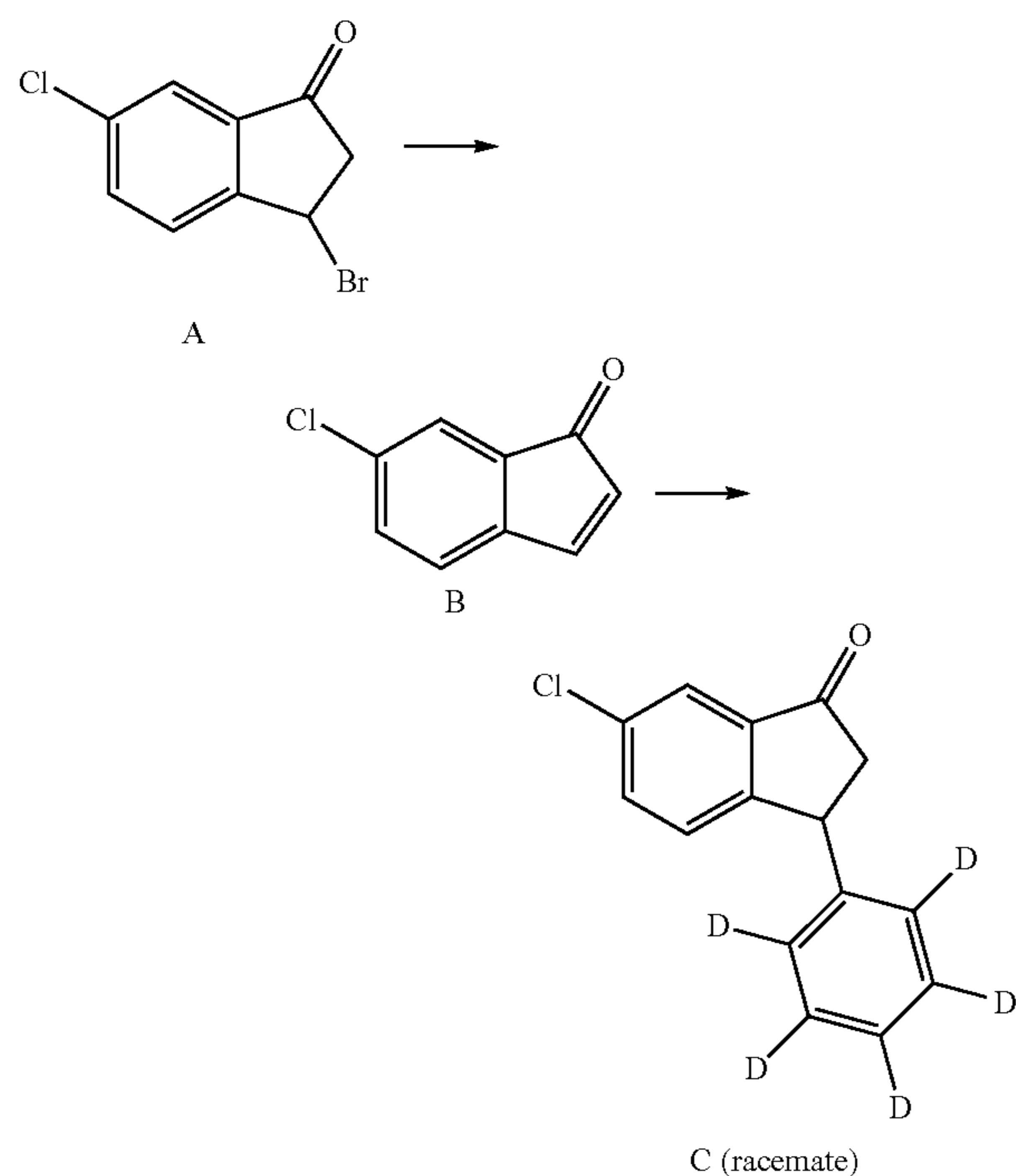
Scheme 1. Exemplary synthesis of intermediate C.
