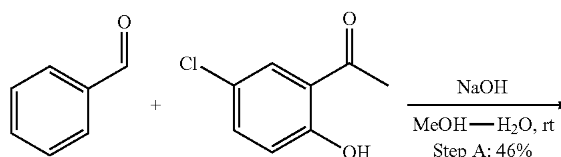
Scheme 15. Synthesis of Compound (XVIII)
