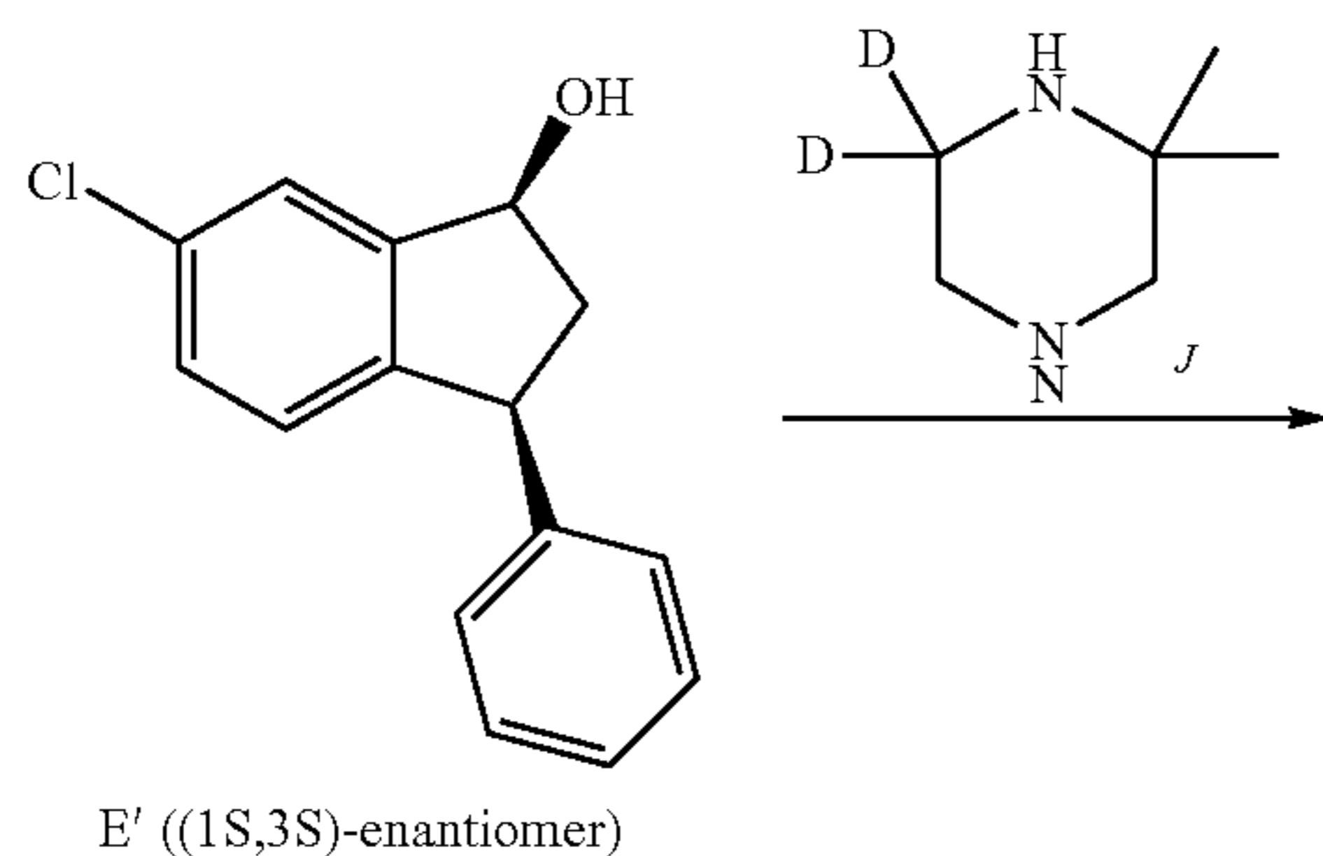
Scheme 12. Synthesis of Compound (III) and Compound (V).
