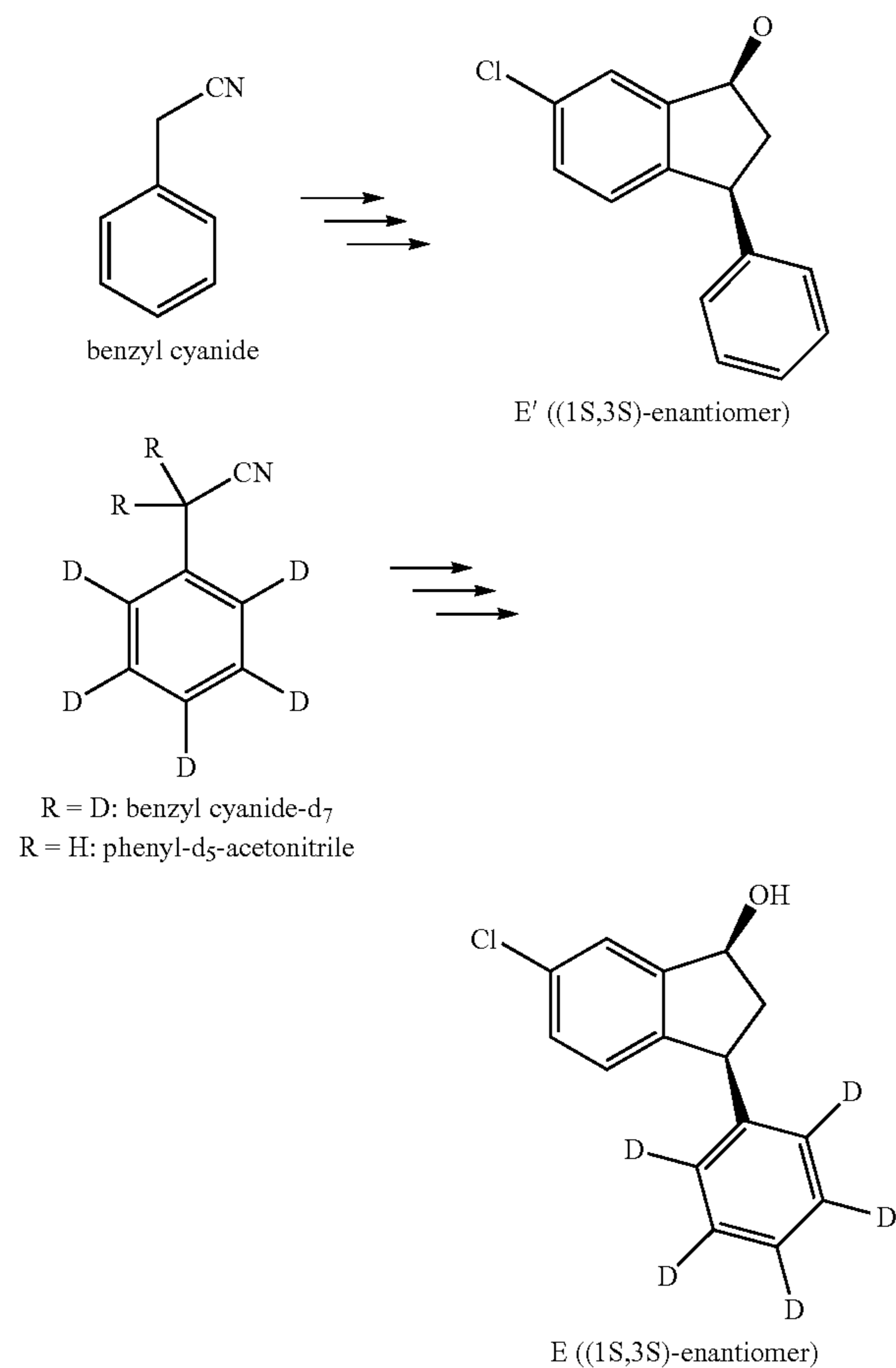
Scheme 4. Exemplary synthesis of intermediates E and E'.
