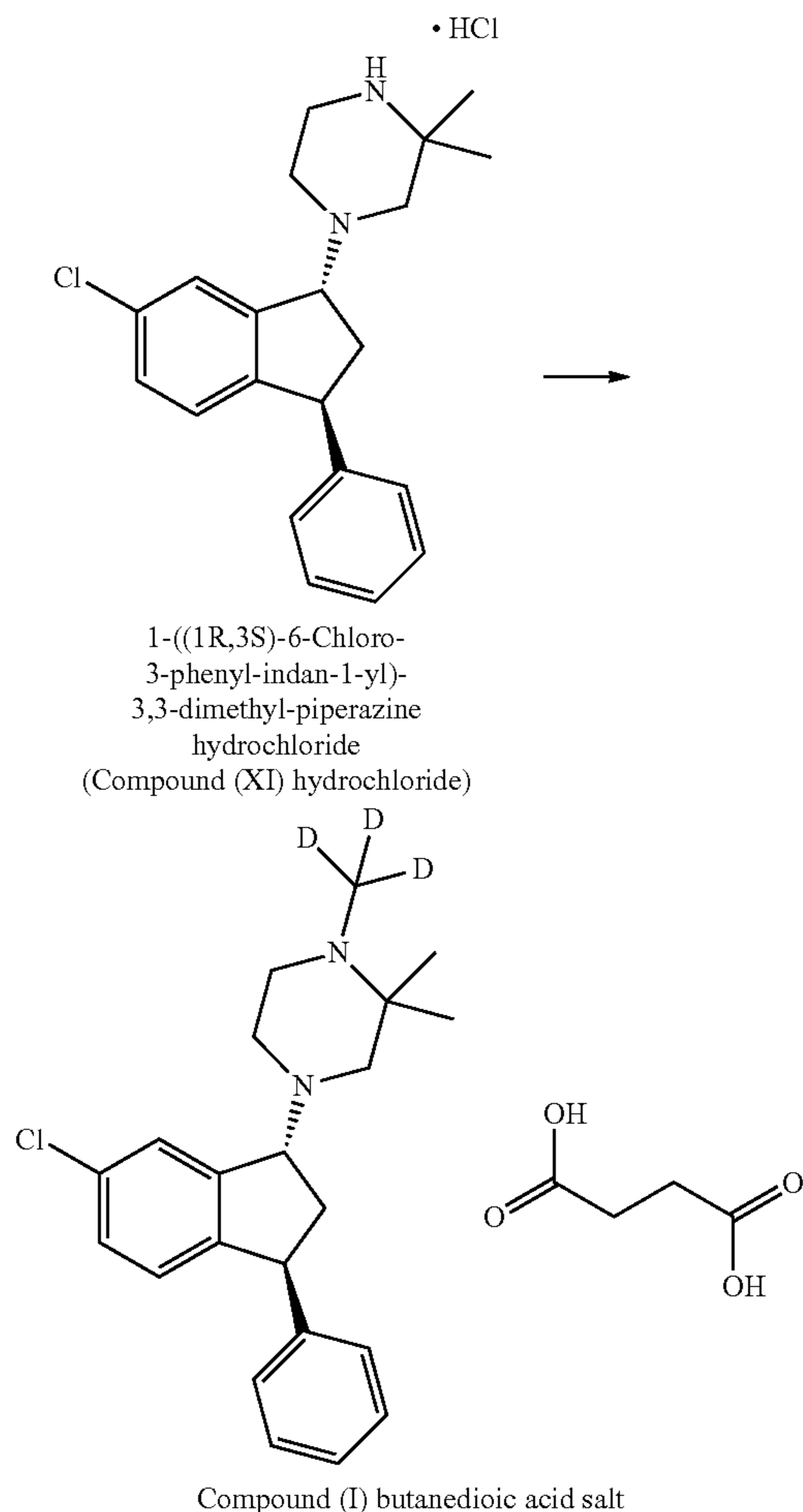
Scheme 8. Synthesis of Compound (I).
