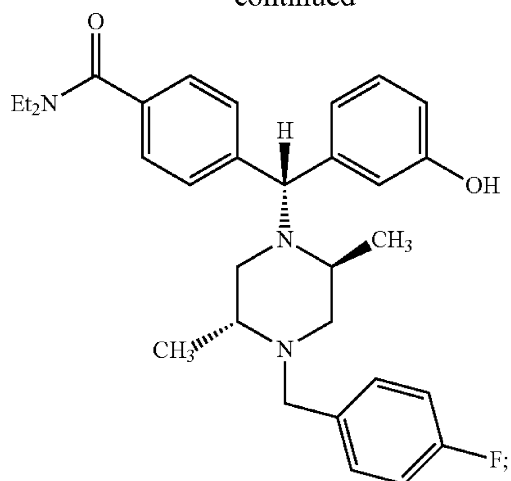
4-((alpha-R)-alpha-((2S,5R)-2,5-Dimethyl-4-(4-fluorobenzyl)-1-piperazinyl)-3-hydroxybenzyl)-N,N-diethylbenzamide
