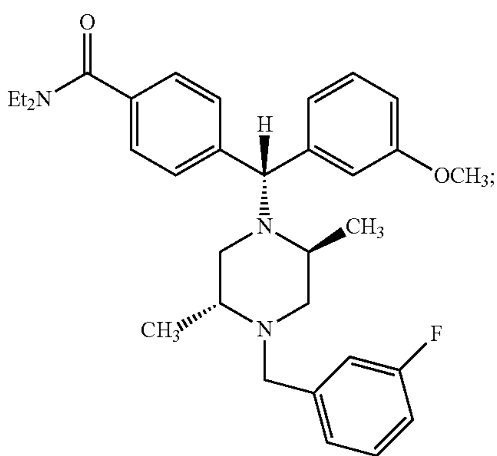
4-((alpha-S)-alpha-((2R,5S)-2,5-Dimethyl-4-(3-fluorobenzyl)-1-piperazinyl)benzyl)-N,N-diethylbenzamide
