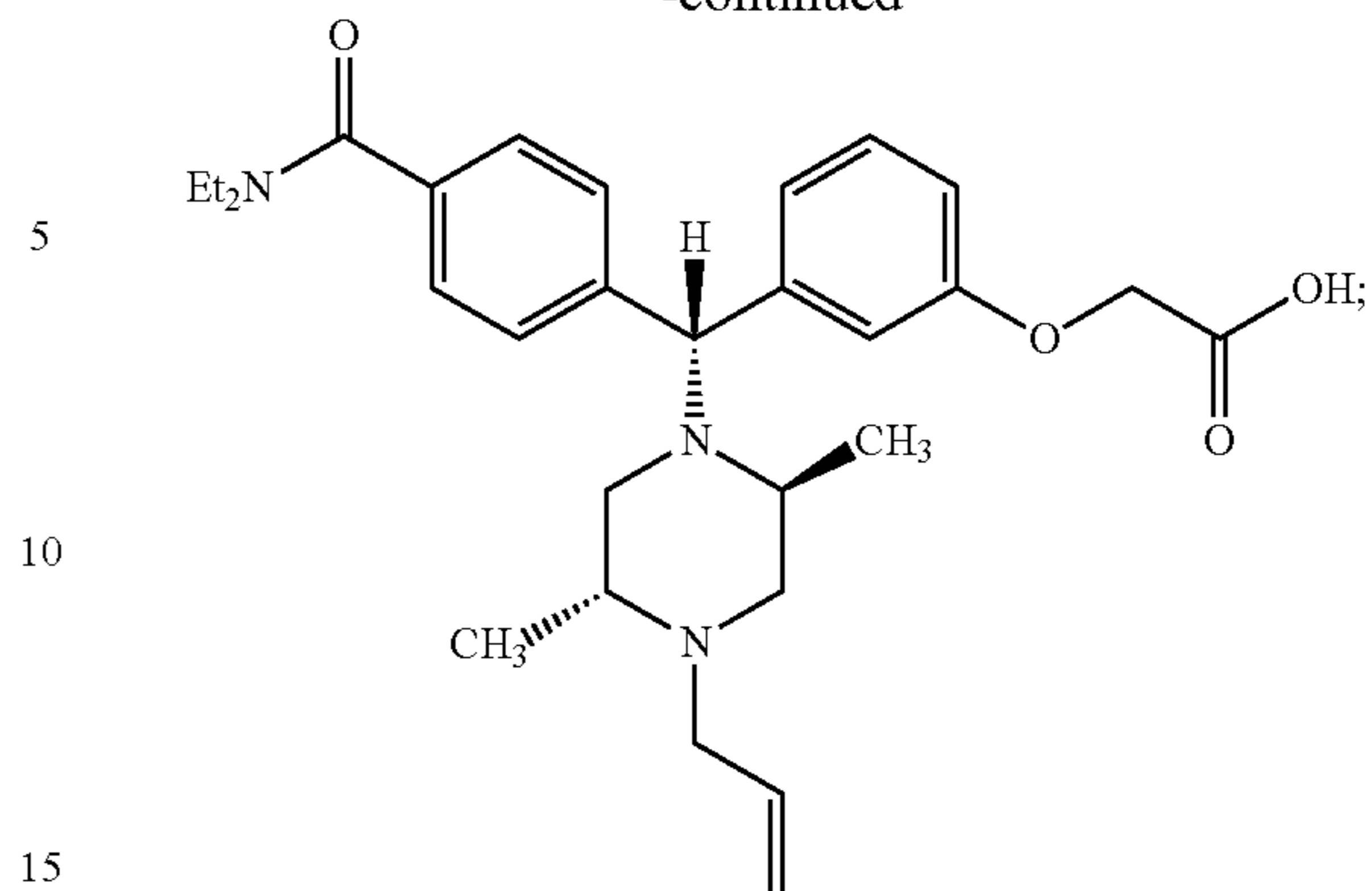
3-((alpha-R)-alpha-((2S,5R)-4-Allyl-2,5-dimethyl-1-piperazinyl)-4-(diethylaminocarbonyl)benzyl)phenoyacetic acid
