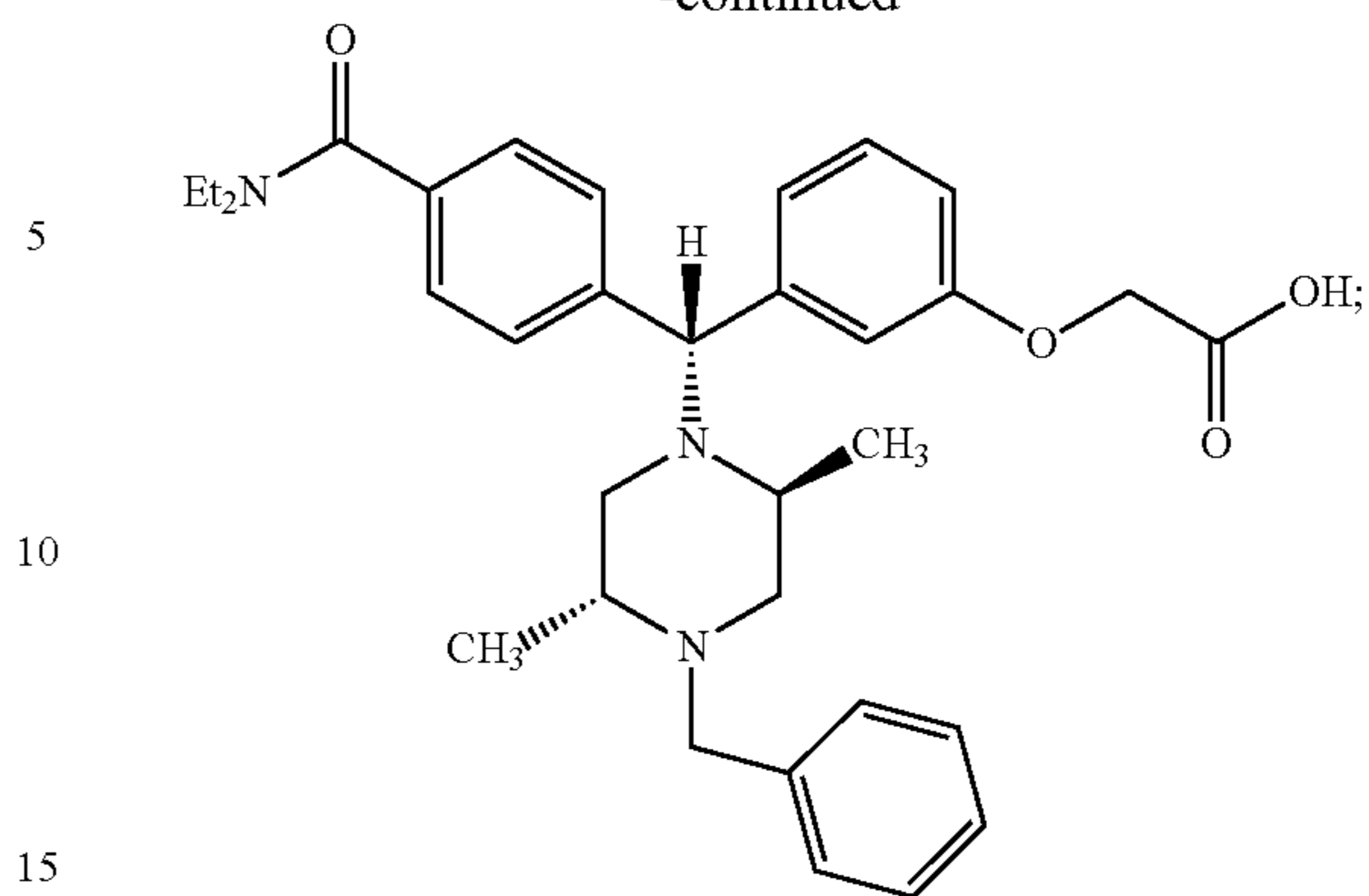
3-((alpha-R)-alpha-((2S,5R)-4-Benzyl-2,5-dimethyl-1-piperazinyl)-4-(diethylaminocarbonyl)benzyl)phenoxyacetic acid
