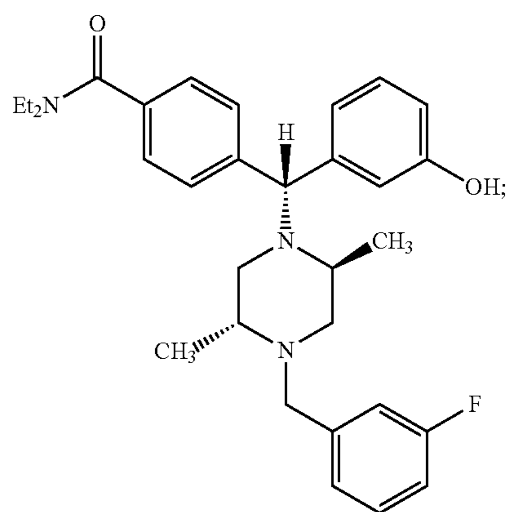
4-((alpha-R)-alpha-((2S,5R)-2,5-Dimethyl-4-(3-fluorobenzyl)-1-piperazinyl)-3-hydroxybenzyl)-N,N-diethylbenzamide
