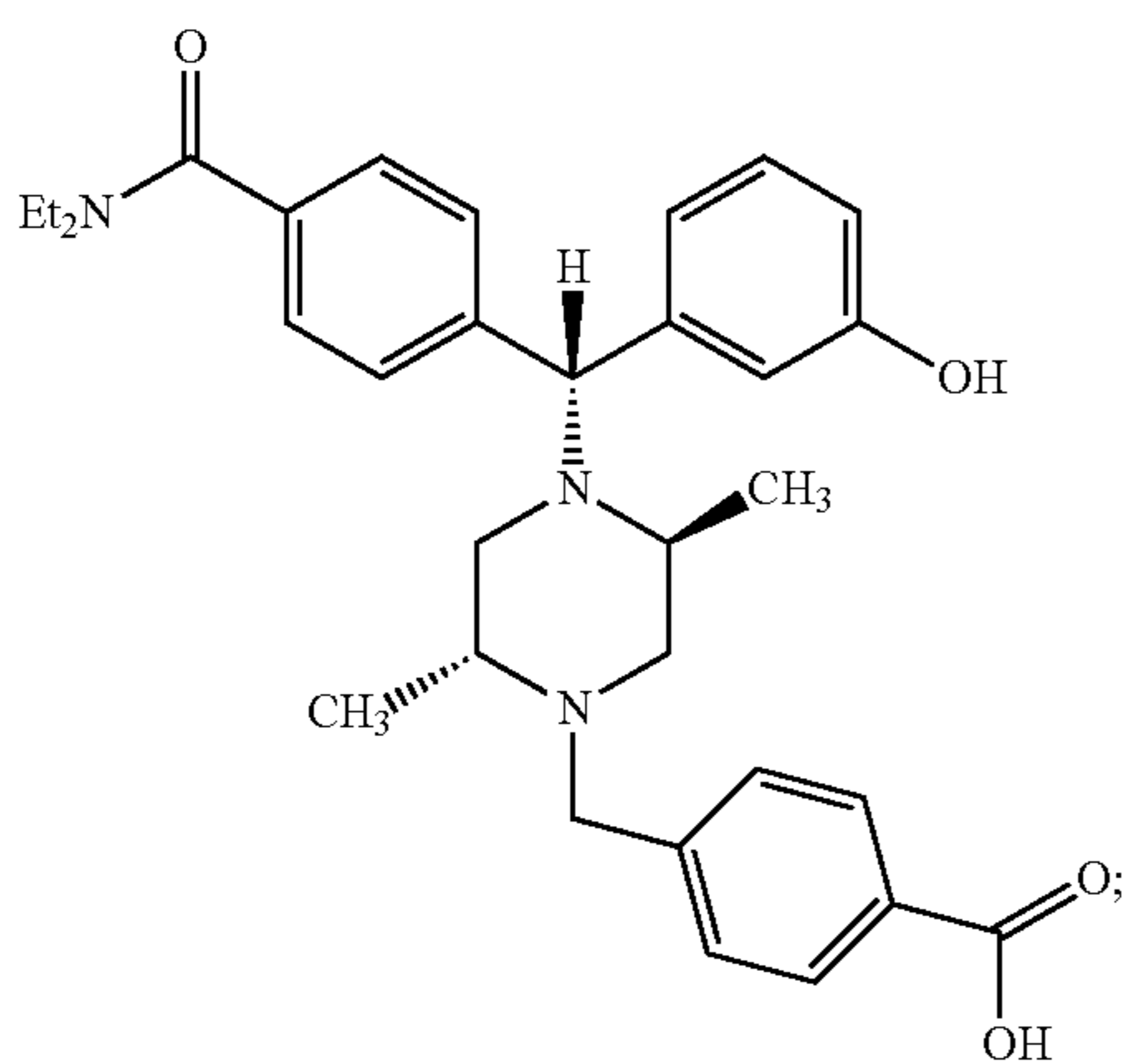
4-((2R,5S)-4-[(R)-(4-Diethylcarbamoylphenyl)(3-hydroxyphenyl)methyl]-2,5-dimethylpiperazin-1-ylmethyl)benzoic acid
