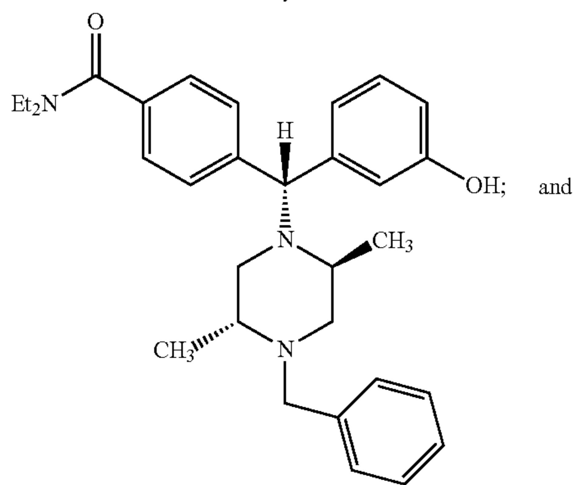
4-((alpha-R)-alpha-((2S,5R)-4-Benzyl-2,5-dimethyl-1-piperazinyl)-3-hydroxybenzyl)-N,N-diethylbenzamide
