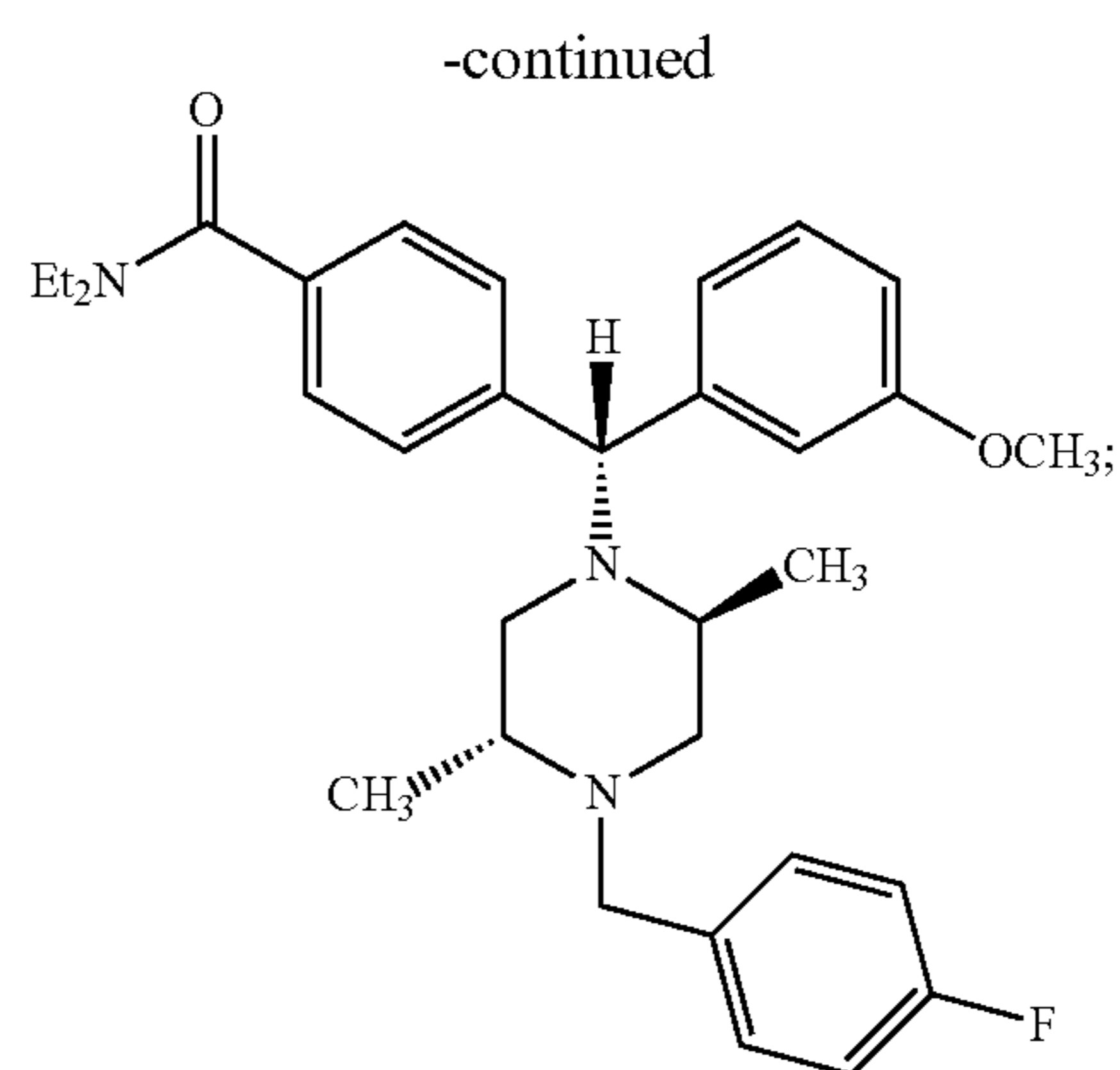
4-((alpha-R)-alpha-((2S,5R)-2,5-Dimethyl-4-(4-fluorobenzyl)-1-piperazinyl)-3-methoxybenzyl-N,N-diethylbenzamide
