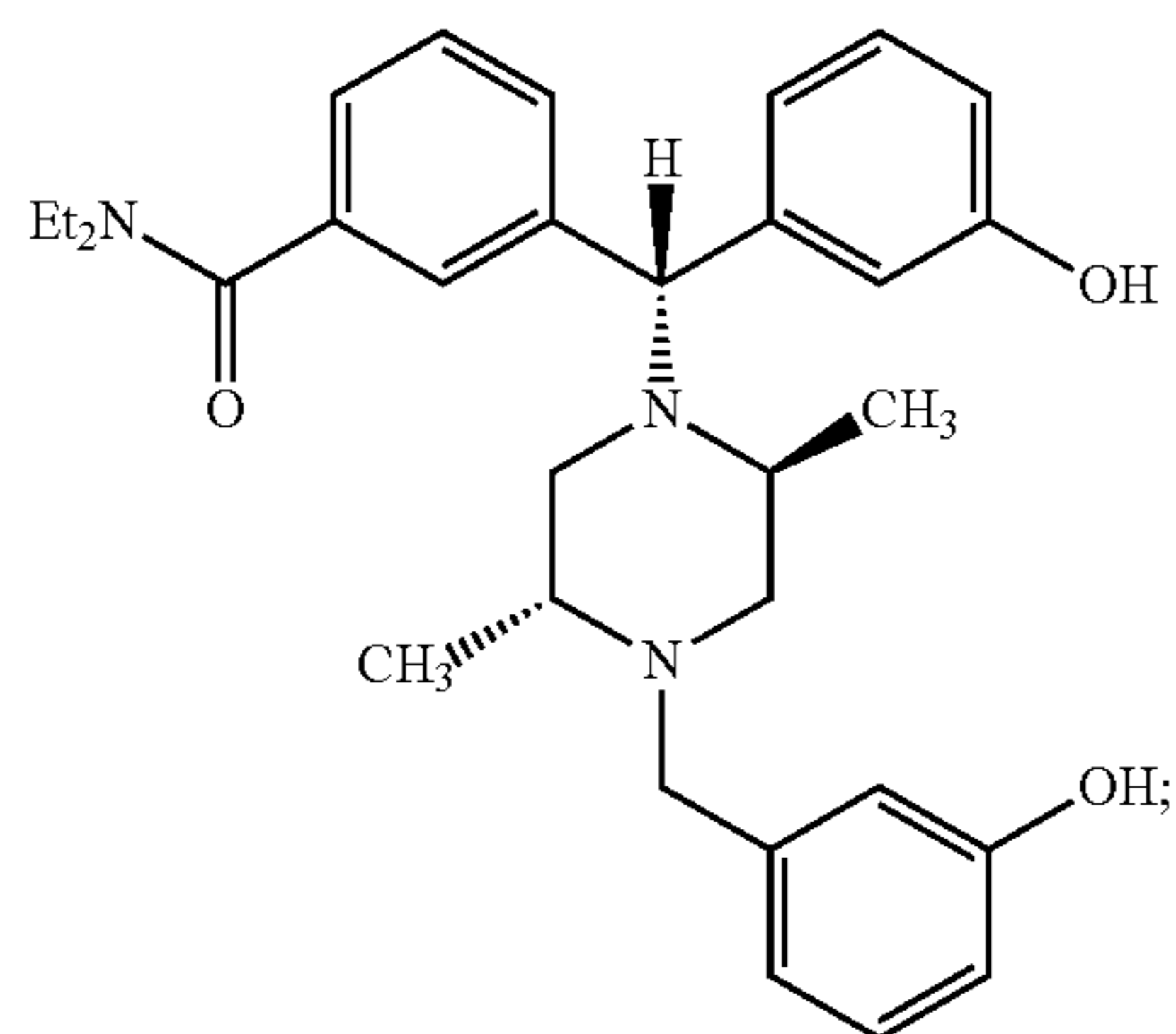
N,N-Diethyl-3-((R)-((2S,5R)-2,5-dimethyl-4-(3-hydroxybenzyl)piperazin-1-yl)(3-hydroxyphenyl)methyl)benzamide
