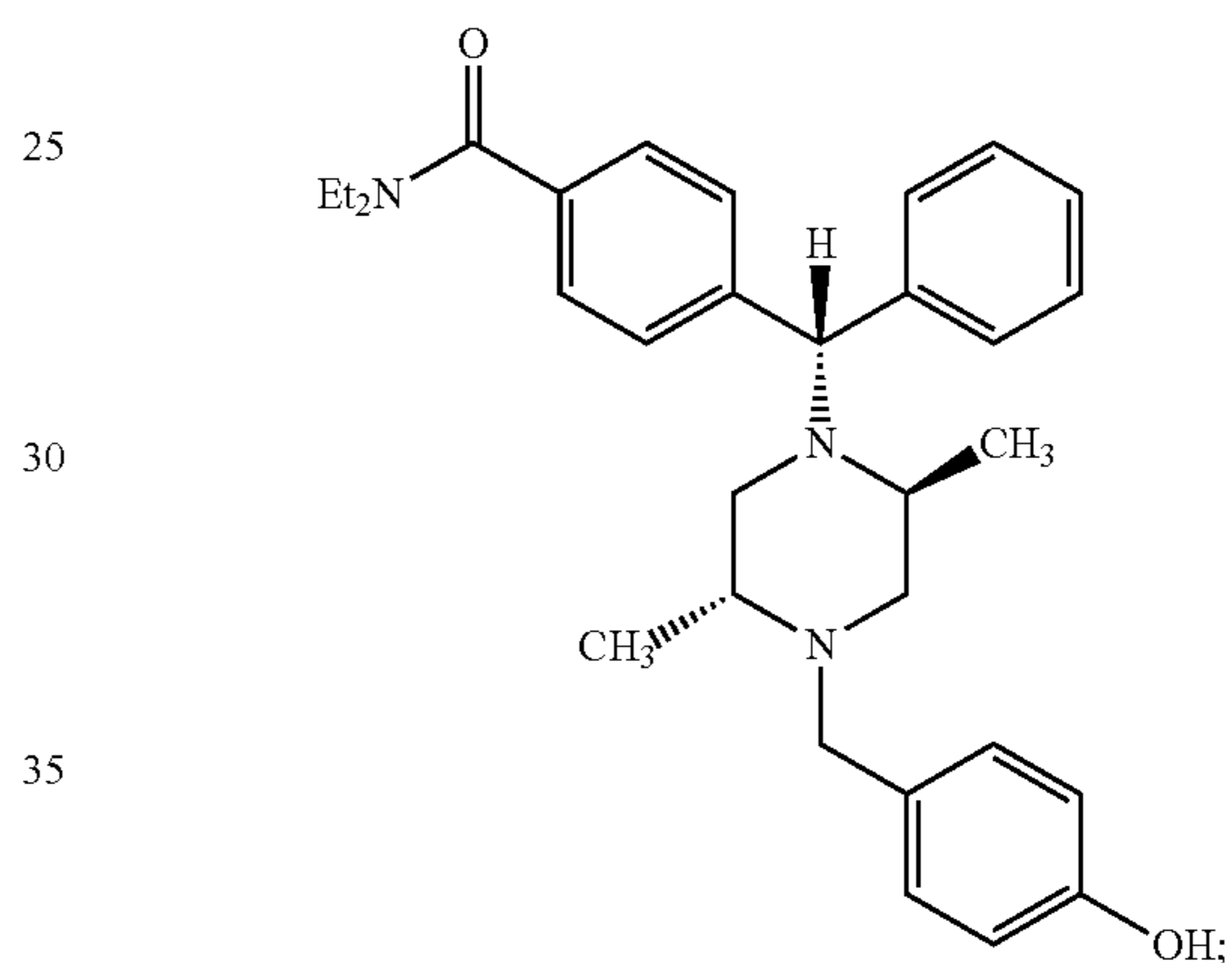
4-((alpha-S)-alpha-((2S,5R)-2,5-Dimethyl-4-(4-hydroxybenzyl)-1-piperazinyl)-benzyl)-N,N-diethylbenzamide
