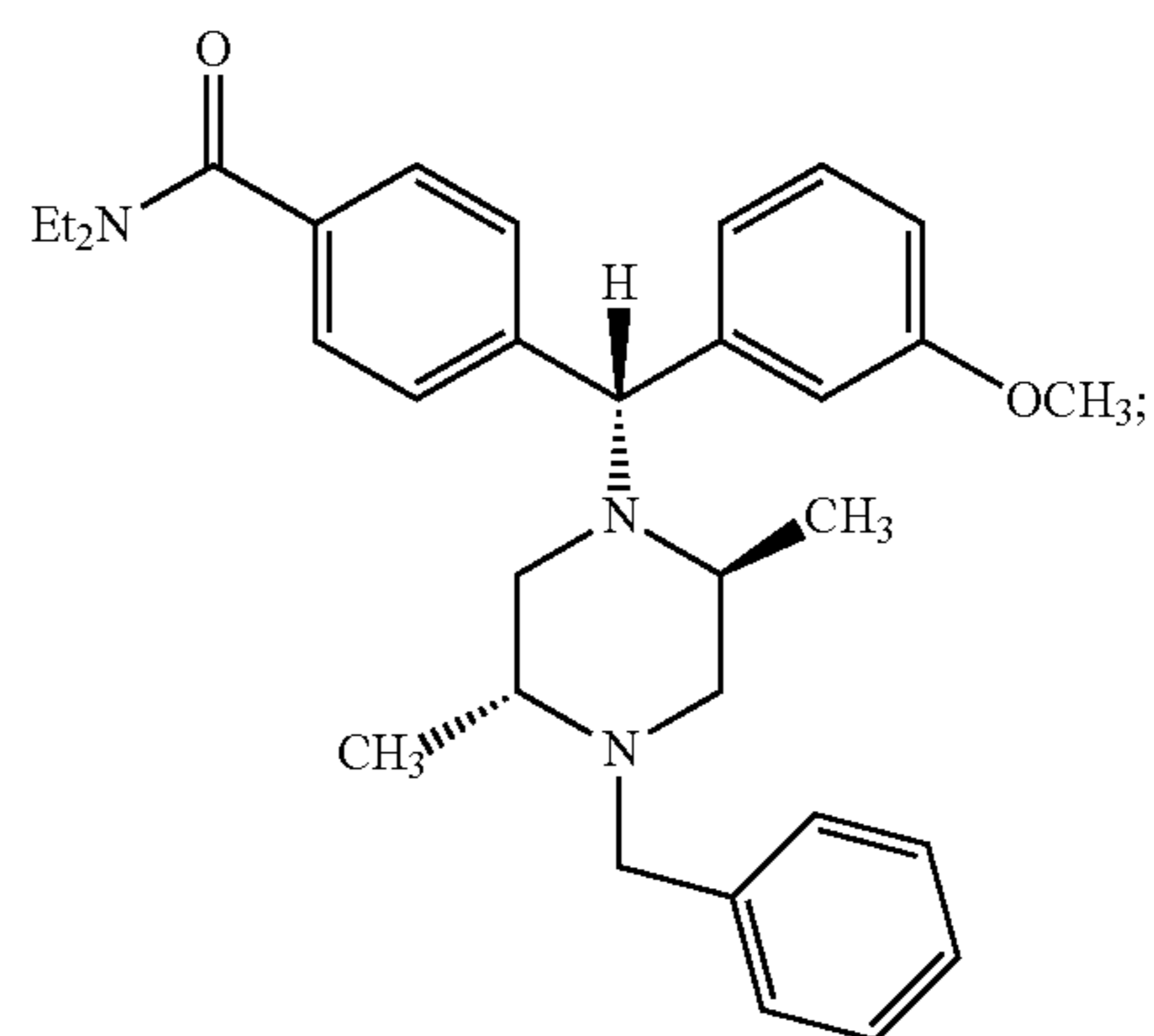
4-(alpha-R)-alpha-((2S,5R)-4-Benzyl-2,5-dimethyl-1-piperazinyl)-3-methoxybenzyl-N,N-diethylbenzamide
