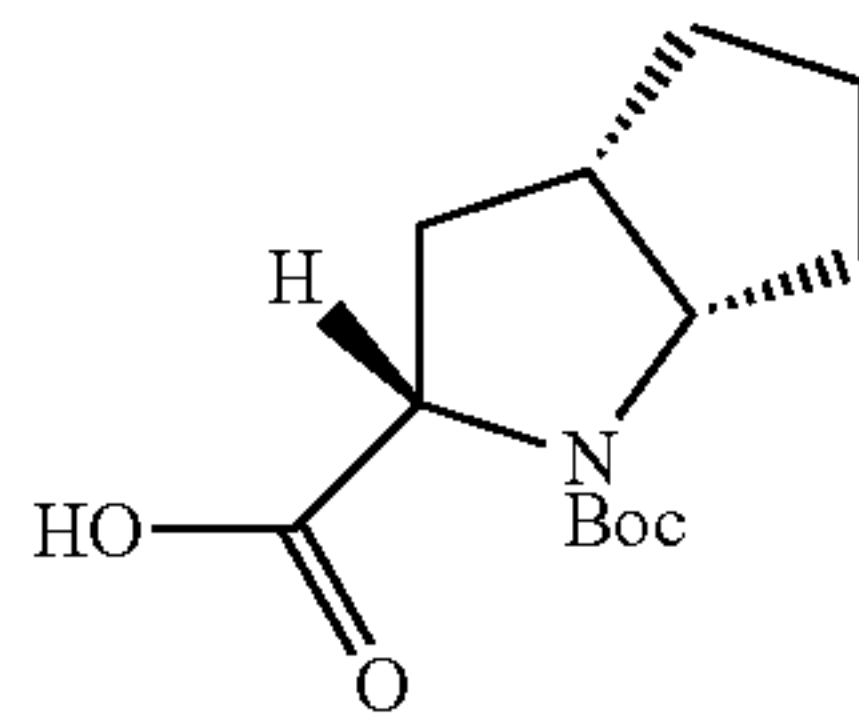
(2S,3aS,6aS)-1-(tert-butoxycarbonyl)octahydrocyclopenta[b]pyrrole-2-carboxylic acid
