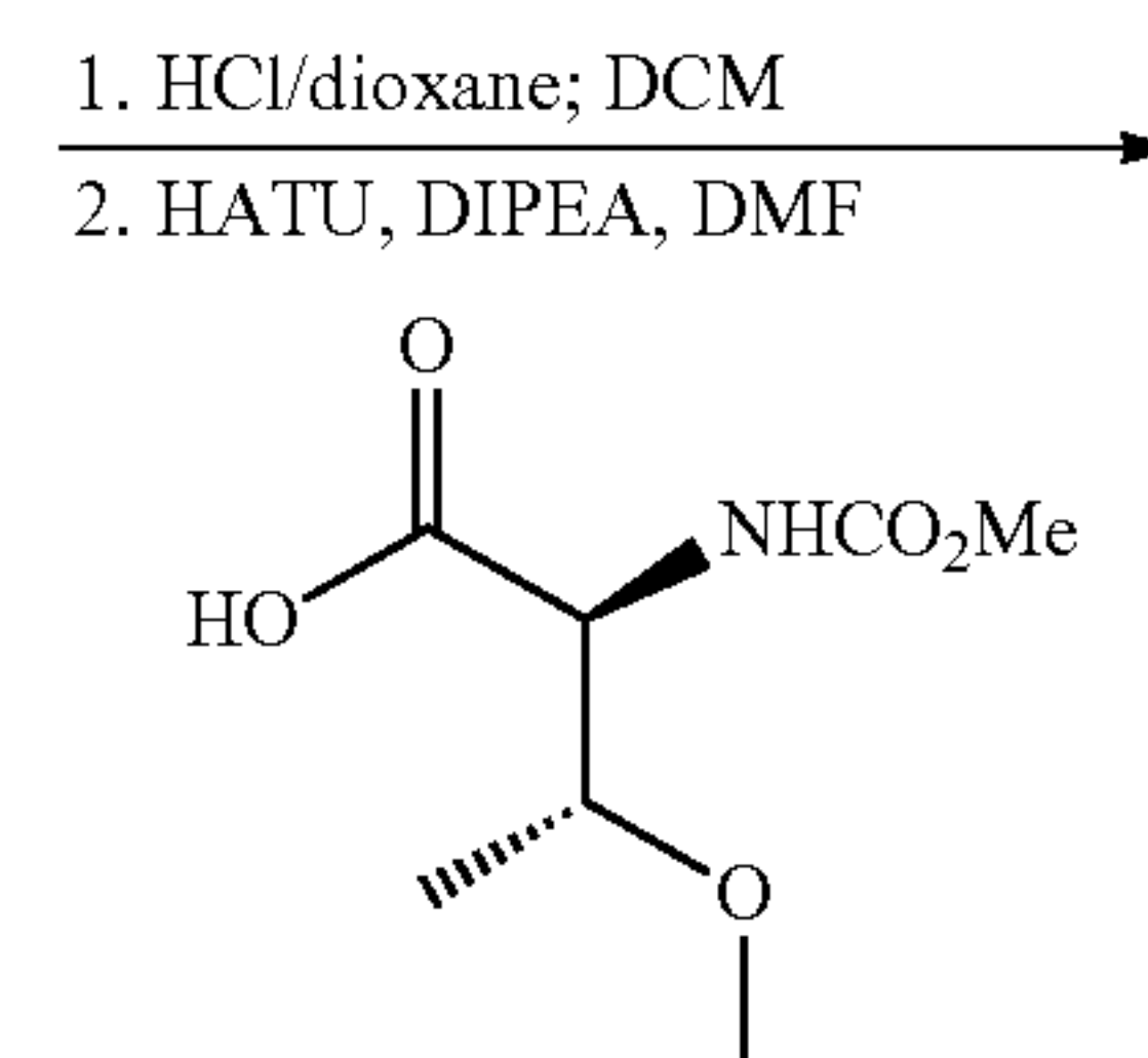
(2S,3R)-3-methoxy-2-(methoxycarbonylamino)butanoic acid
