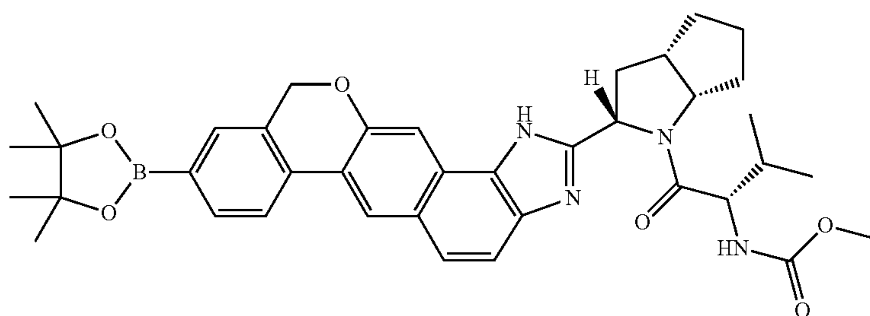
methyl {(2S)-3-methyl-1-oxo-1-[(2S,3aS,6aS)-2-[9-(4,4,5,5-tetramethyl-1,3,2-dioxaborolan-2-yl)-1,11-dihydroisochromeno[4',3':6,7]naphtho[1,2-d]imidazol-2-yl]hexahydrocyclopenta[b]pyrrol-1(2H)-yl]butan-2-yl} carbamate
