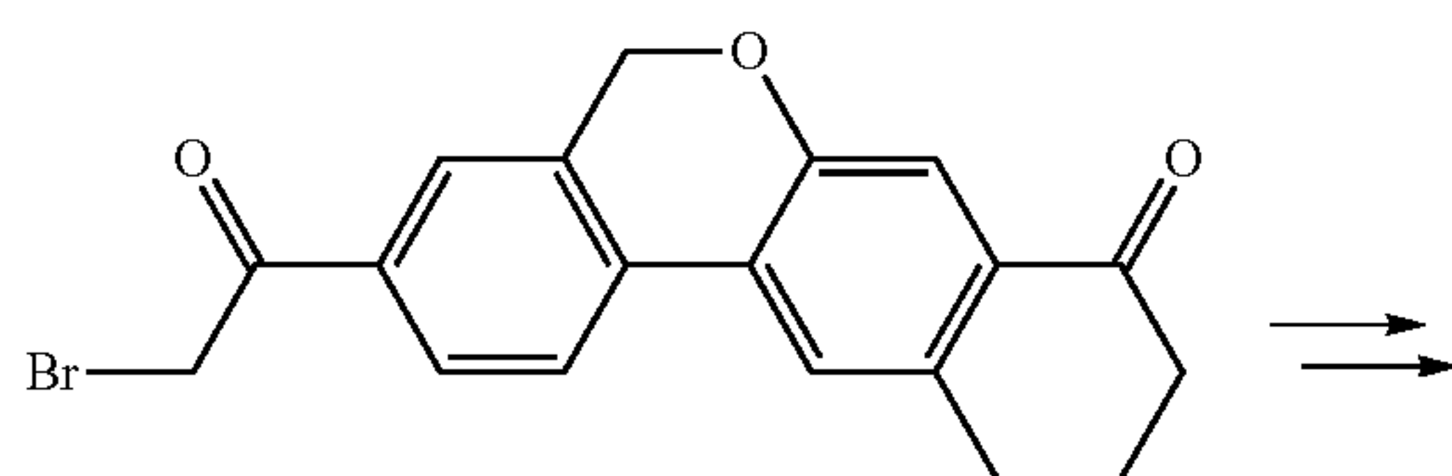
3-(2-bromoacetyl)-10,11-dihydro-5H-dibenzo[c,g]chromen-8(9H)-one
