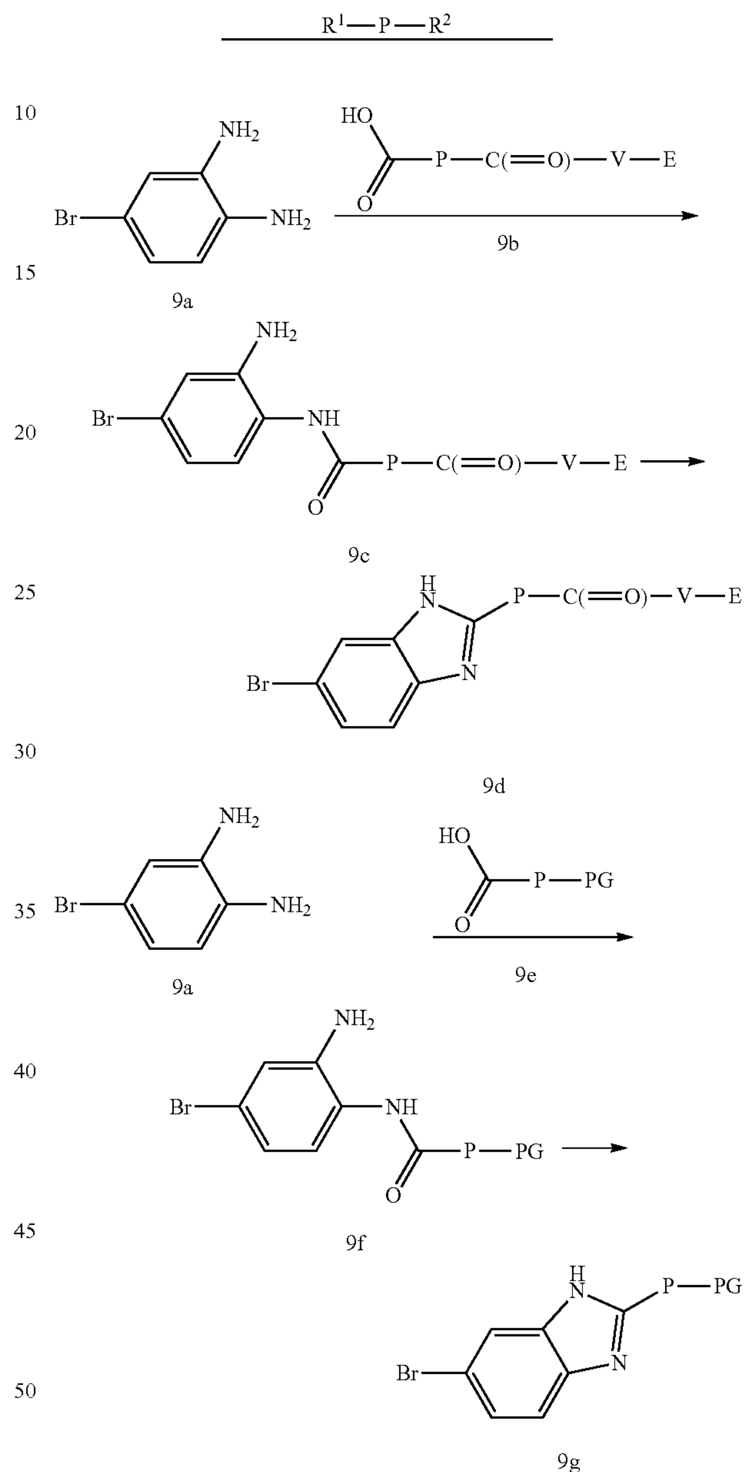
Scheme 9. Representative synthesis
