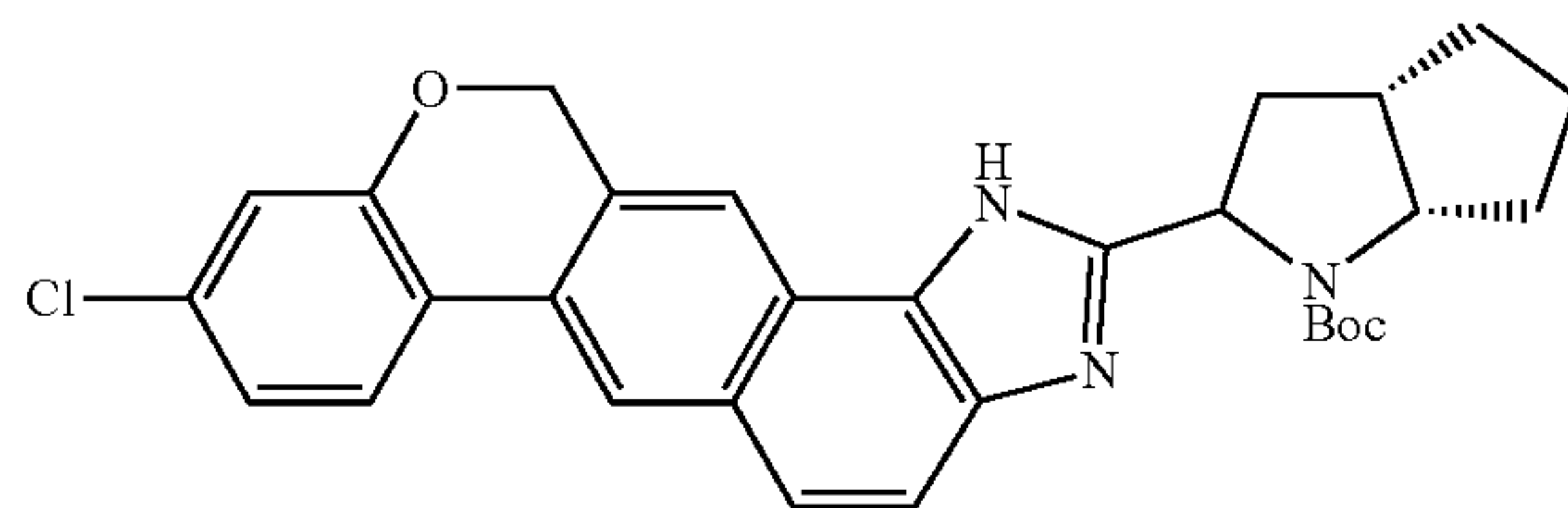
tert-butyl (3aS,6aS)-2-(9-chloro-1,12-dihydrochromeno[4',3':6,7]naphtho[1,2-d]imidazol-2-yl)hexahydrocyclopenta[b]pyrrole-1(2H)-carboxylate
