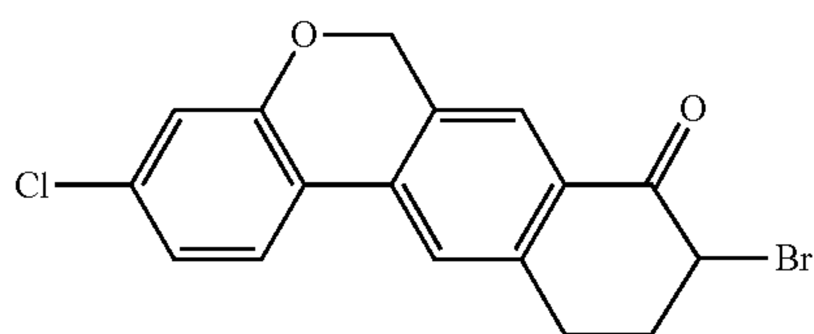
9-bromo-3-chloro-10,11-dihydro-6H-naphtho[2,3-c]chromen-8(9H)-one
