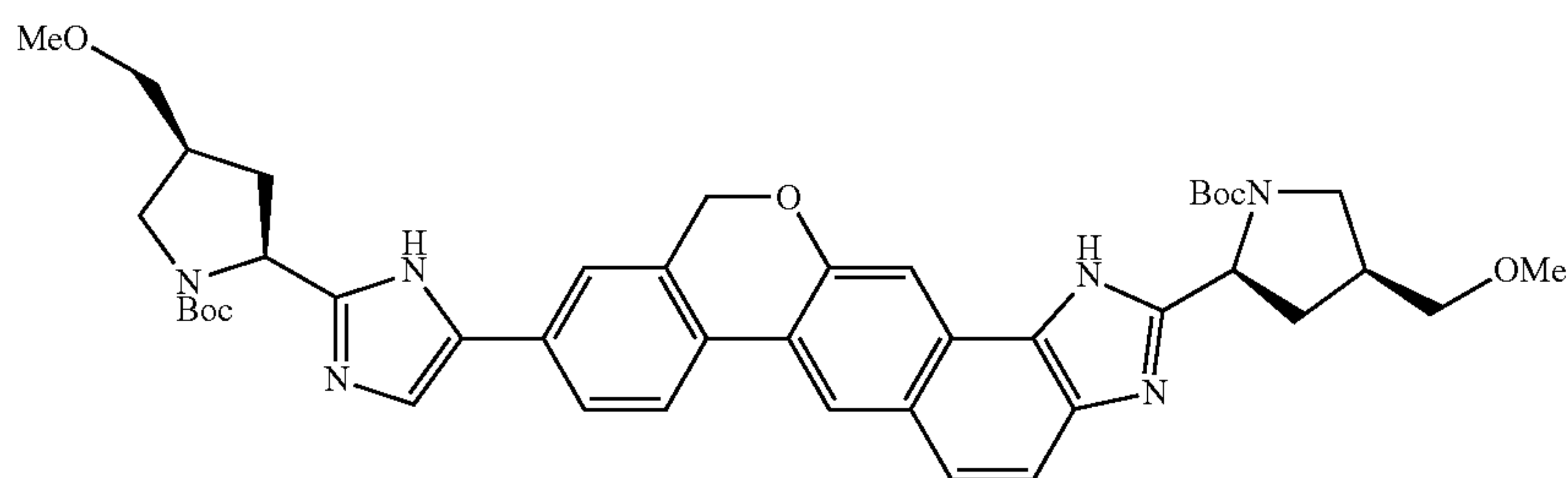
tert-butyl (2S,4S)-2-(5-{2-[(2S,4S)-1-(tert-butoxycarbonyl)-4-(methoxymethyl)pyrrolidin-2-yl]-1,11-dihydroisochromeno[4',3':6,7]naphtho[1,2-d]imidazol-9-yl}-1H-imidazol-2-yl)-4-(methoxymethyl)pyrrolidine-1-carboxylate
