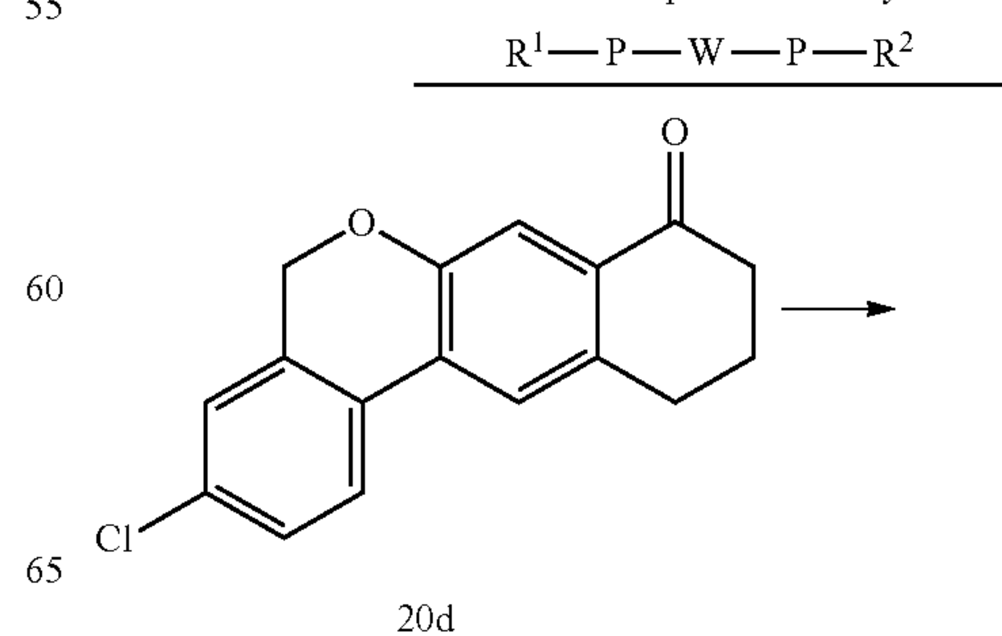
Scheme 21. Representative synthesis
