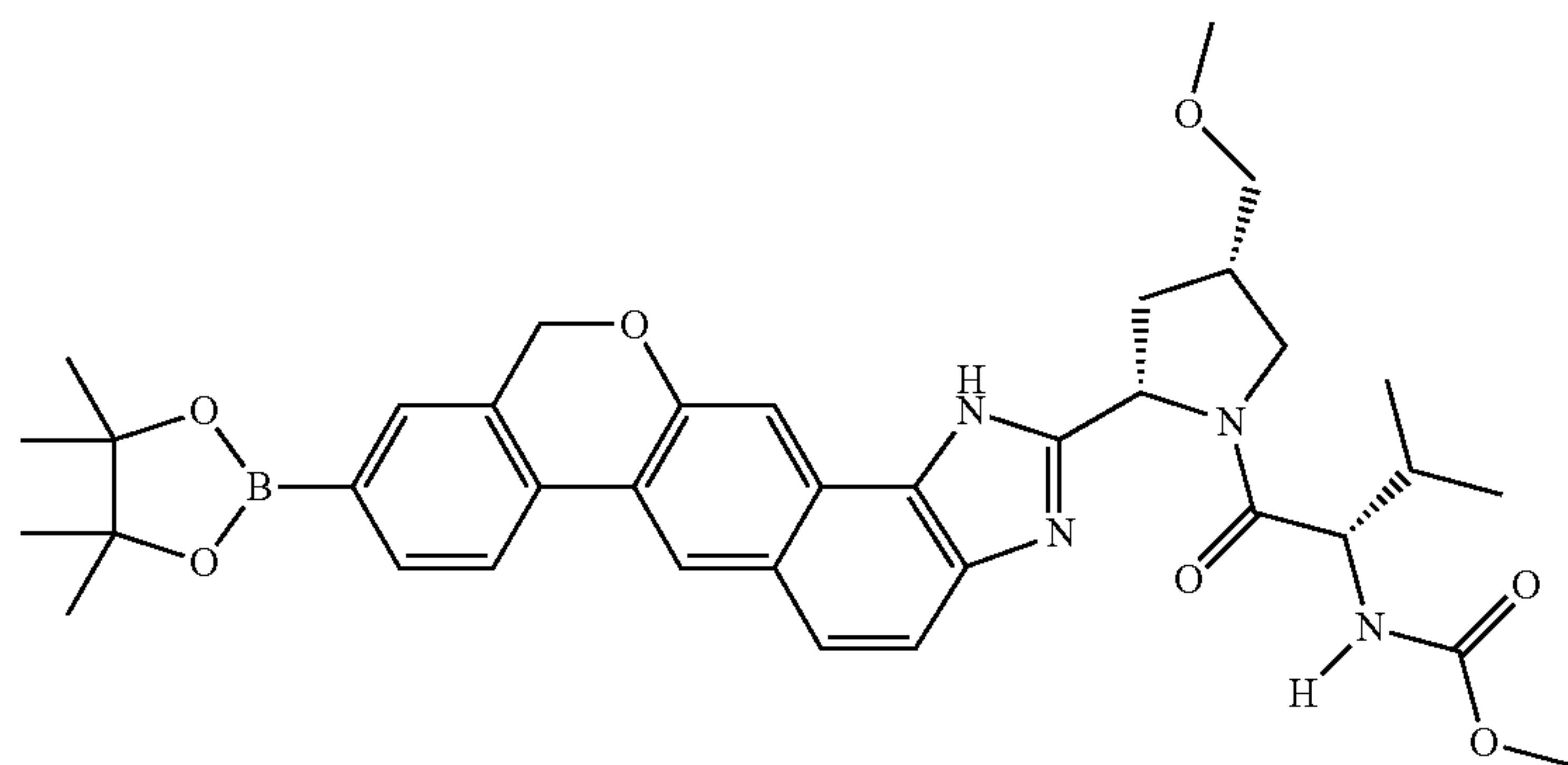
methyl [(2S)-3-methyl-1-((2S,4S)-4-methyl-2-[9-(4,4,5,5-tetramethyl-1,3,2-dioxaborolan-2-yl)-1,11-dihydroisochromeno[4',3':6,7]naphtho[1,2-d]imidazole-2-yl]pyrrolidin-1-yl)-3-methyl-1-oxobutan-2-yl]carbamate
