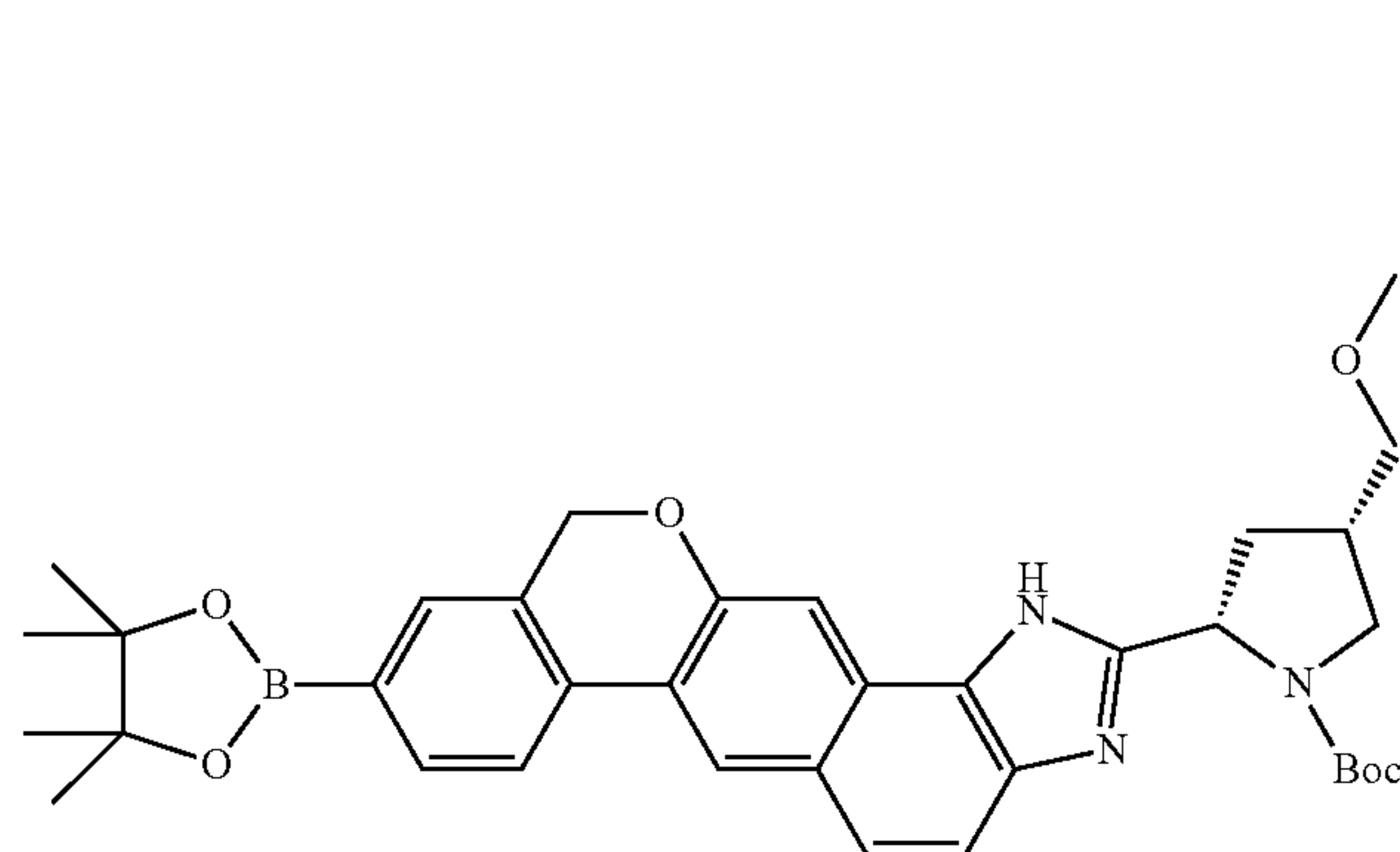
(2S,4S)-tert-butyl 4-(methoxymethyl)-2-(9-(4,4,5,5-tetramethyl-1,3,2-dioxaborolan-2-yl)-1,11-dihydroisochromeno[4',3':6,7]naphtho[1,2-d]imidazol-2-yl)pyrrolidine-1-carboxylate
