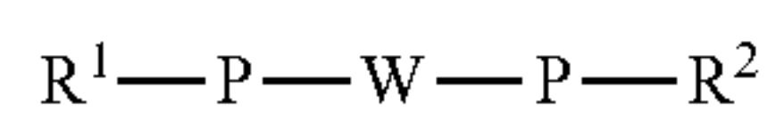
Scheme 27. Representative synthesis of
