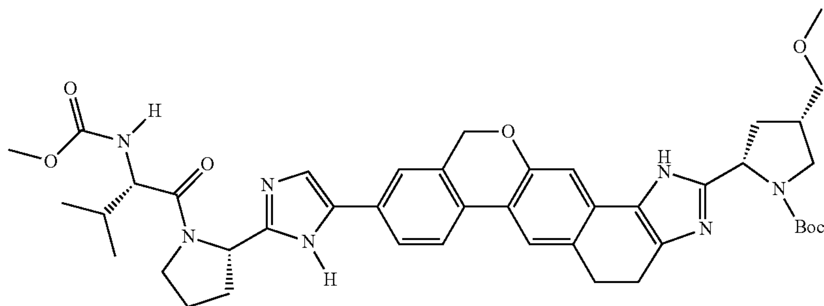
(2S,4S)-tert-butyl 2-(9-(2-((S)-1-((S)-2-(methoxycarbonylamino)-3-methylbutanoyl)pyrrolidin-2-yl)-1H-imidazol-5-yl)-4,5-dihydro-1,11-dihydroisochromeno[4',3':6,7]naphtho[1,2-d]imidazol-2-yl)-4-(methoxymethyl)pyrrolidine-1-carboxylate
