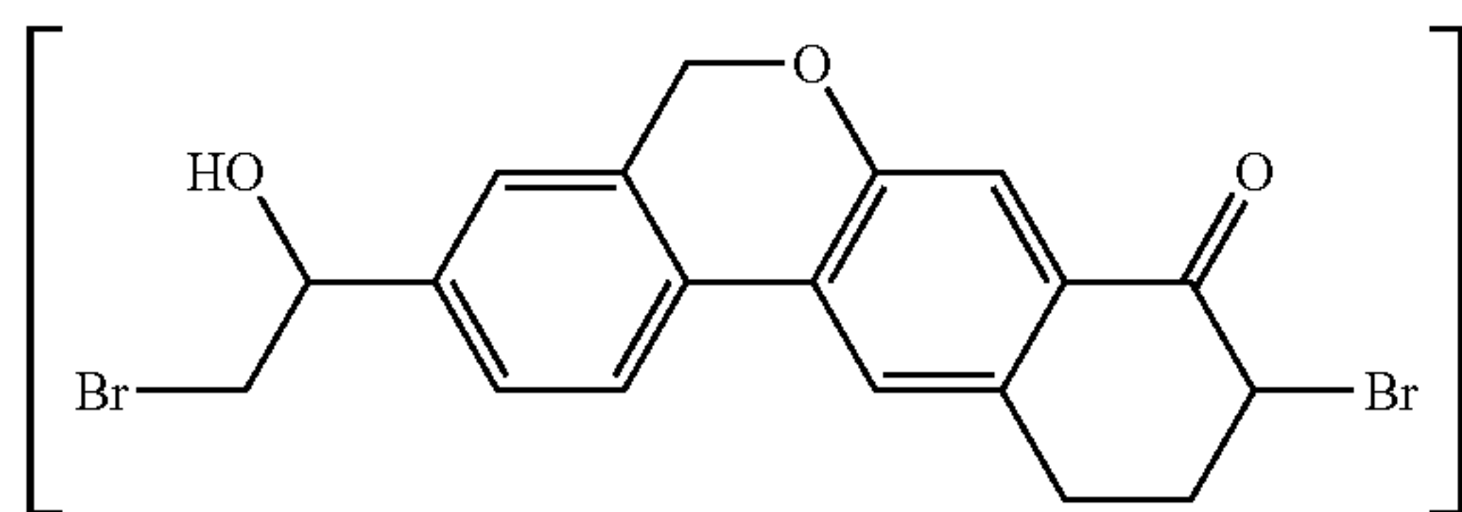
9-bromo-3-(2-bromo-1-hydroxyethyl)-10,11-dihydro-5H-dibenzo[c,g]chromen-8(9H)-one
