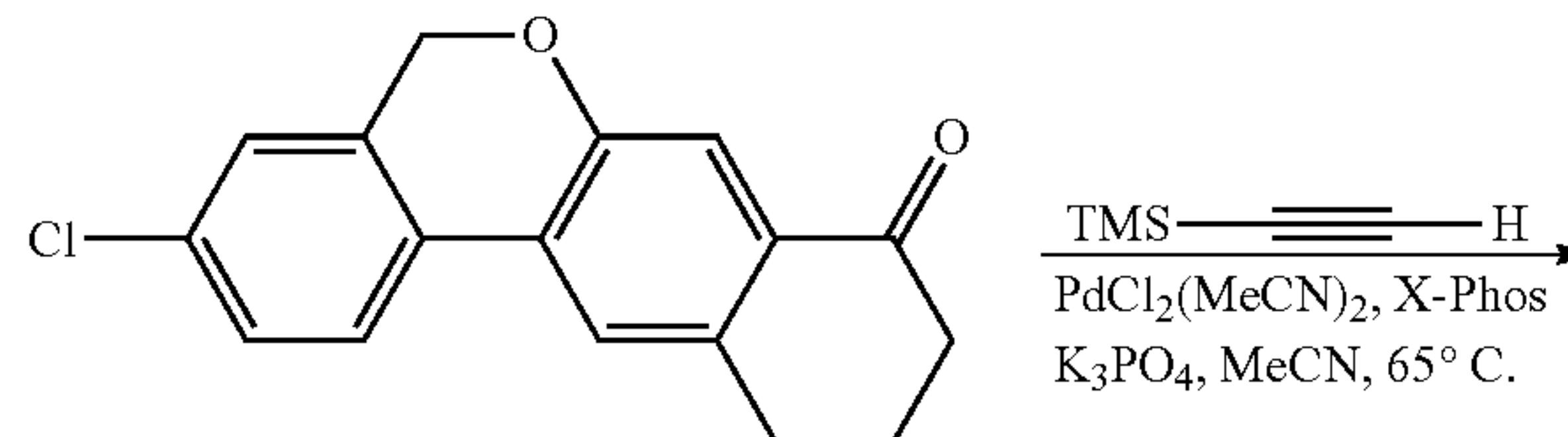
3-chloro-10,11-dihydro-5H-dibenzo[c,g]chromen-8(9H)-one
