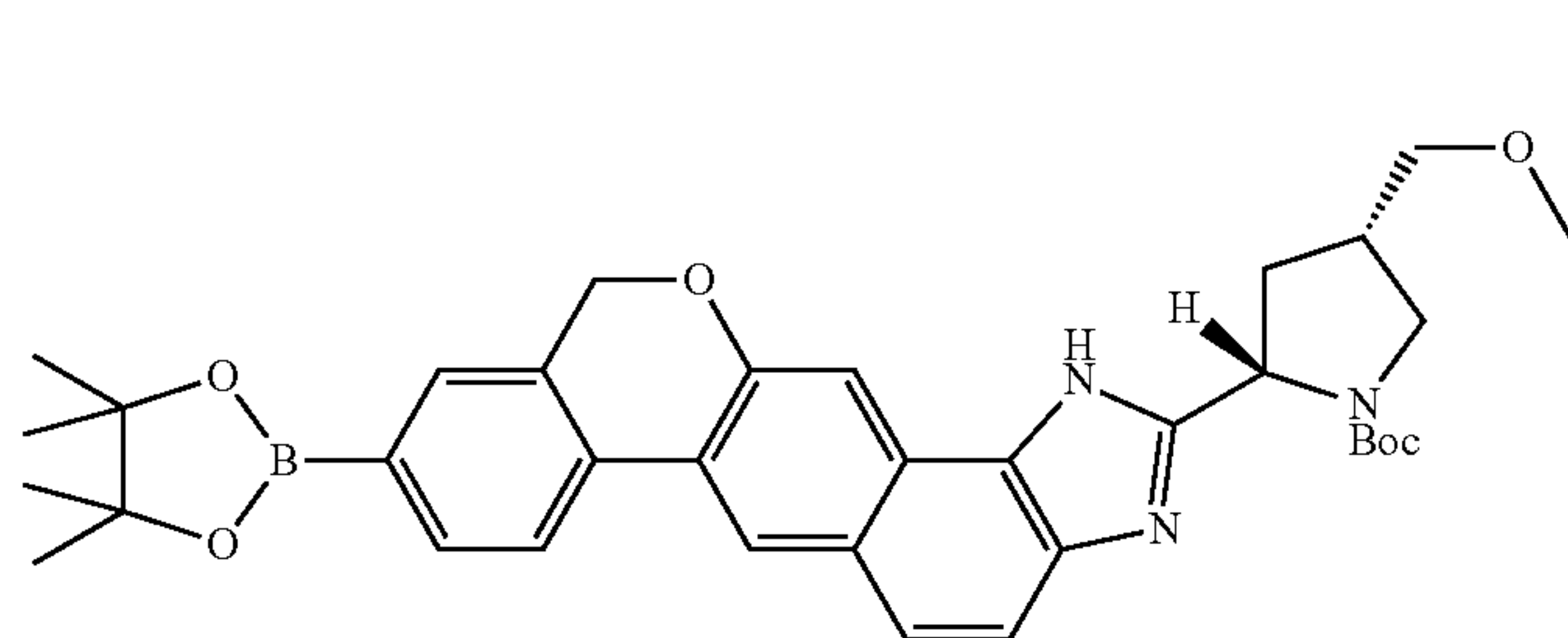
methyl (1-{4-(methoxymethyl)-2-[9-(4,4,5,5-tetramethyl-1,3,2-dioxaborolan-2-yl)-1,11-dihydroisochromeno[4',3':6,7]naphtho[1,2-d]imidazol-2-yl]pyrrolidin-1-yl}-3-methyl-1-oxobutan-2-yl)carbamate
