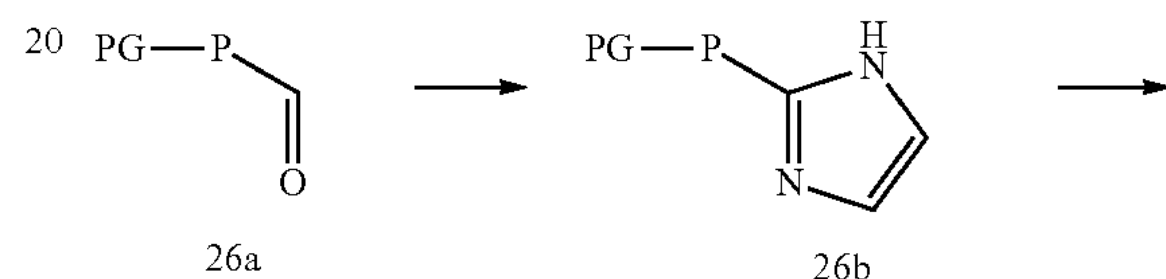
Scheme 26. Representative syntheses of E—V—C(=O)—P—R and R 1 —P—R
