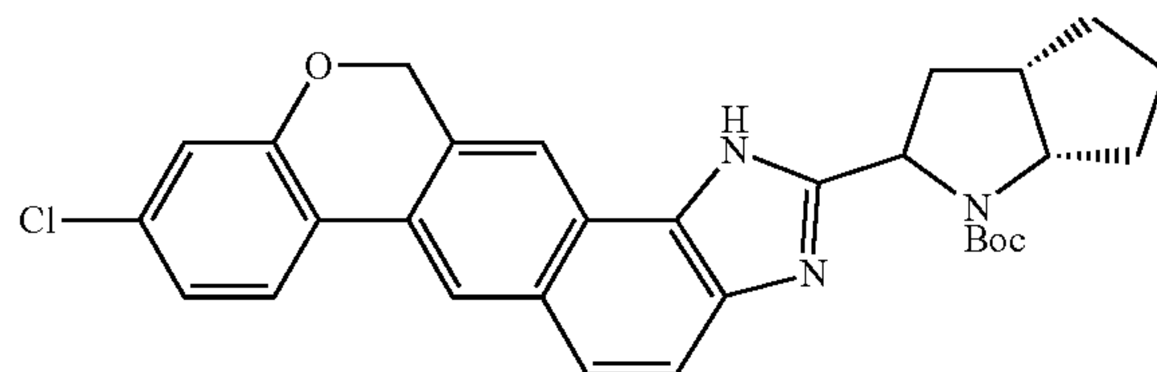
tert-butyl (3aS,6aS)-2-(9-chloro-1,12-dihydrochromeno[4',3':6,7]naphtho[1,2-d]imidazol-2-yl)hexahydrocyclopenta[b]pyrrole-1(2H)-carboxylate
