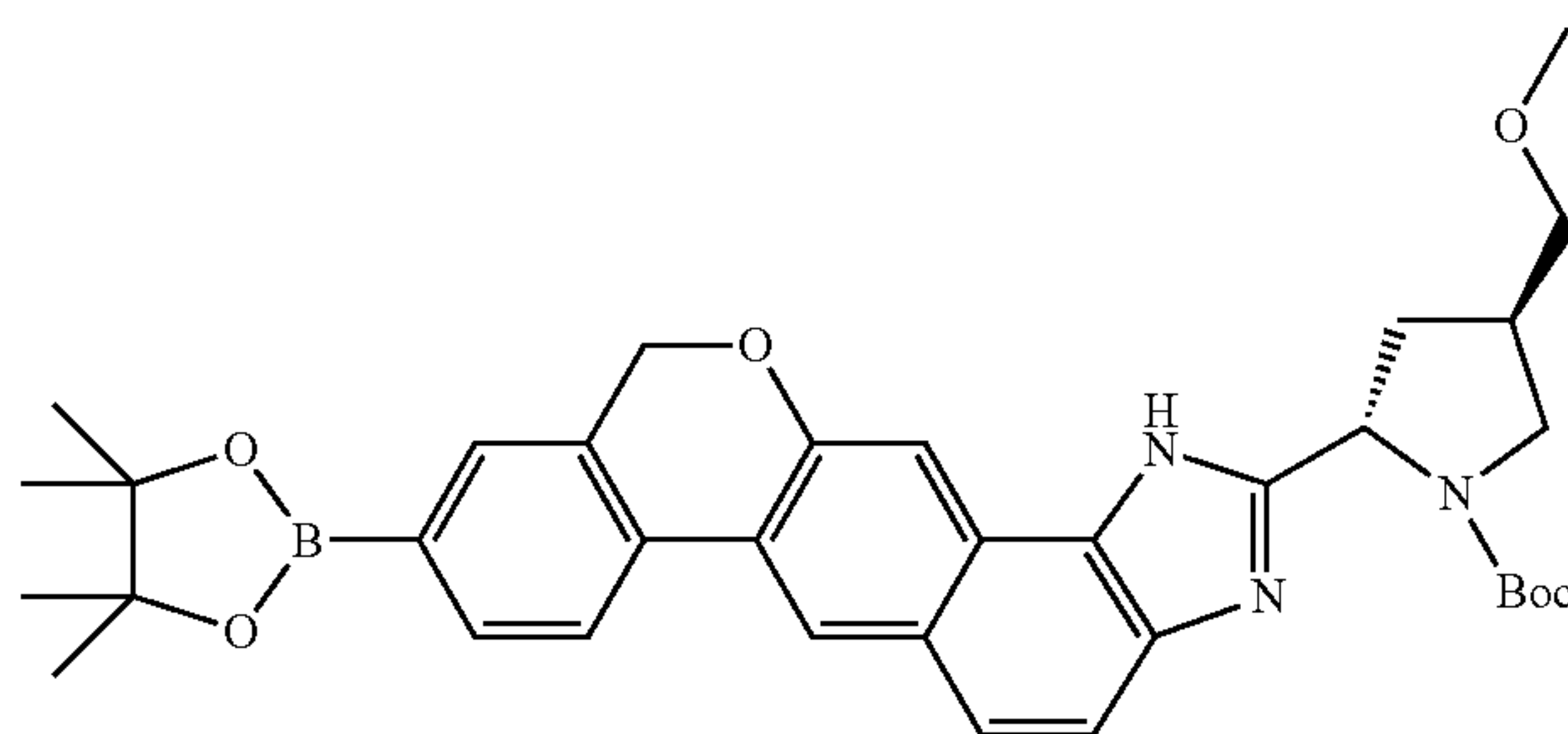
(2S,4R)-tert-butyl 4-(methoxymethyl)-2-(9-(4,4,5,5-tetramethyl-1,3,2-dioxaborolan-2-yl)-1,11-dihydroisochromeno[4',3':6,7]naphtho[1,2-d]imidazol-2-yl)pyrrolidine-1-carboxylate
