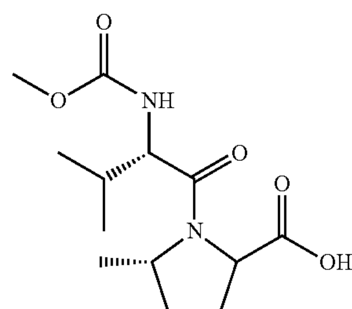
(2S,5S)-1-((S)-2-(methoxycarbonylamino)-3-methylbutanoyl)-5-methylpyrrolidine-2-carboxylic acid
