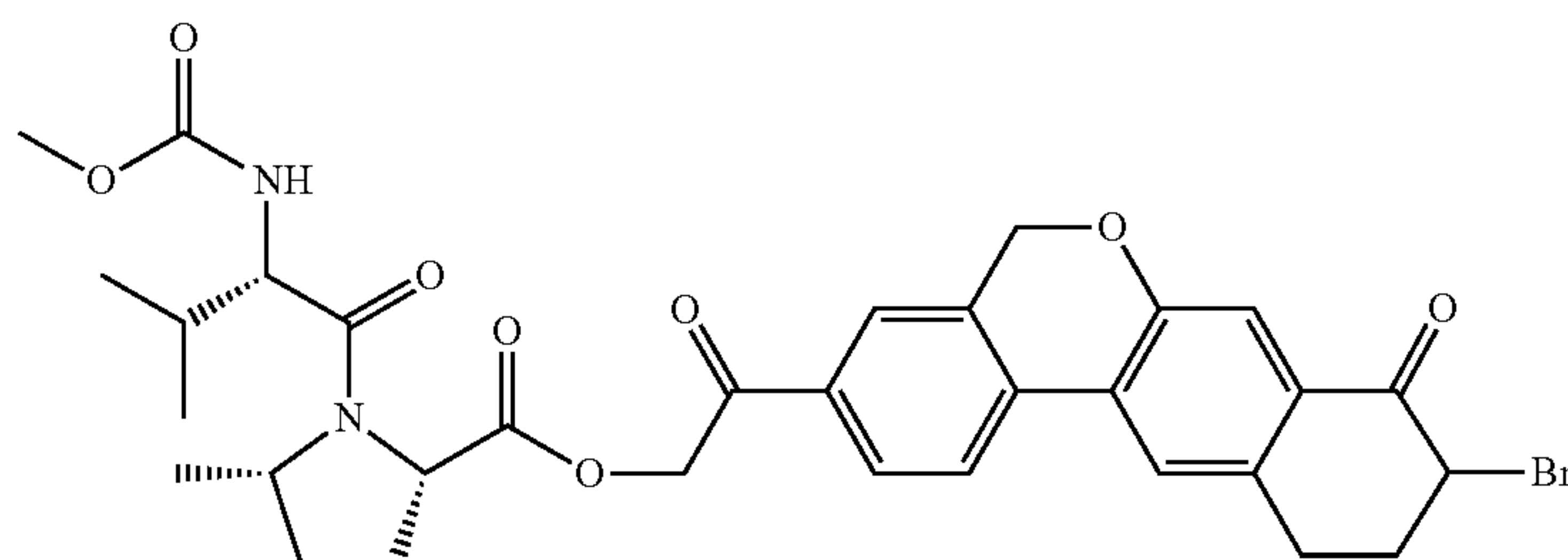
(2S,5S)-2-(9-bromo-8-oxo-8,9,10,11-tetrahydro-5H-dibenzo[c,g]chromen-3-yl)-2-oxoethyl 1-((S)-2-(methoxycarbonylamino)-3-methylbutanoyl)-5-methylpyrrolidine-2-carboxylate
