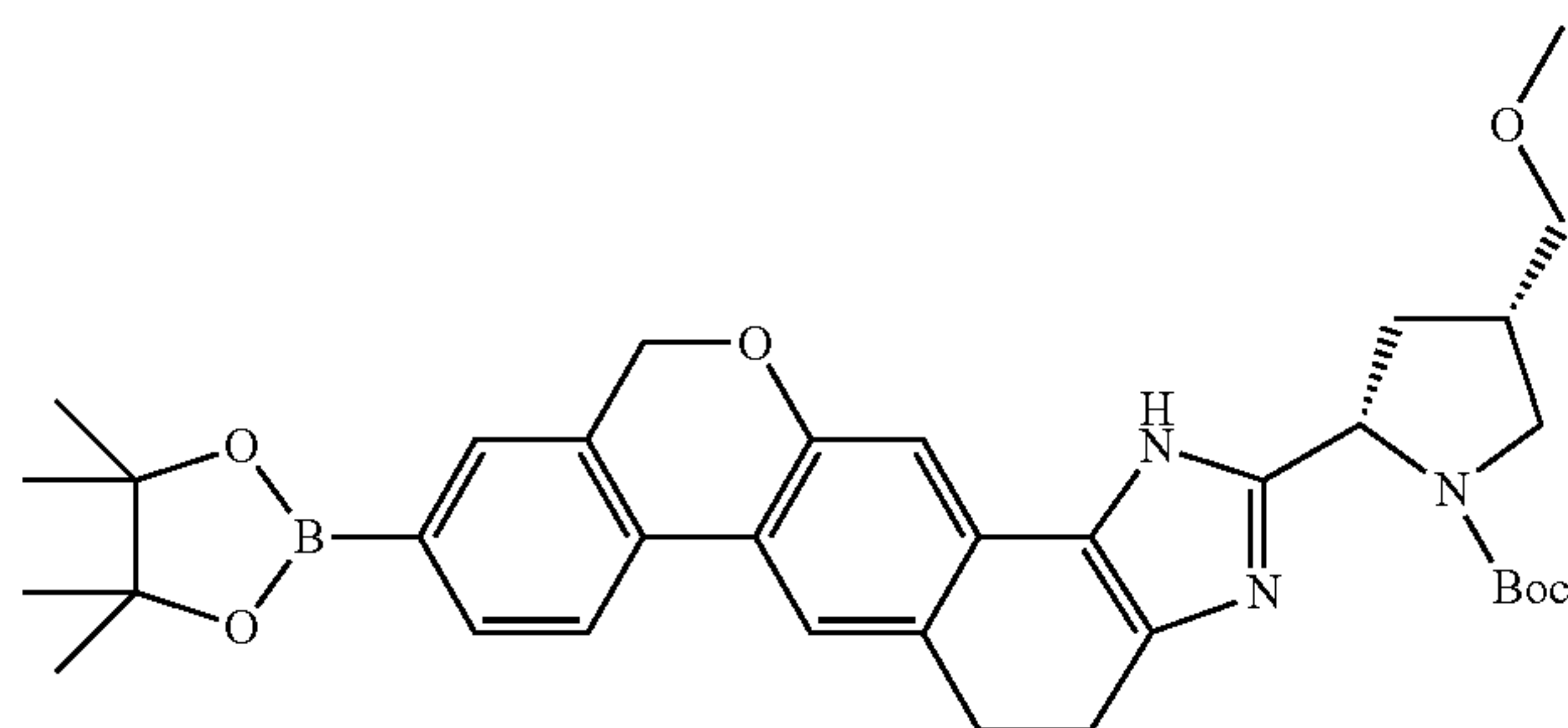
(2S,4S)-tert-butyl 4-(methoxymethyl)-2-(9-(4,4,5,5-tetramethyl-1,3,2-dioxaborolan-2-yl)-4,5-dihydro-1,11-dihydroisochromeno[4',3':6,7]naphtho[1,2-d]imidazol-2-yl)pyrrolidine-1-carboxylate
