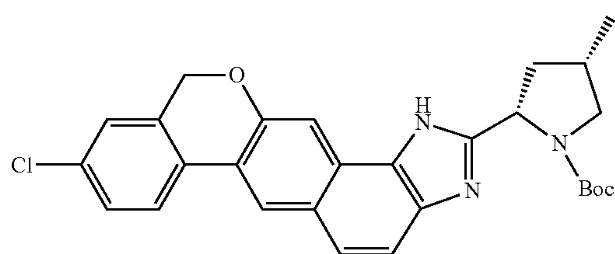
(2S,4S)-tert-butyl 2-(9-chloro-5H-naphtho[c,g]chromeno[8,9-d]imidazol-2-yl)-4-methylpyrrolidine-1-carboxylate
