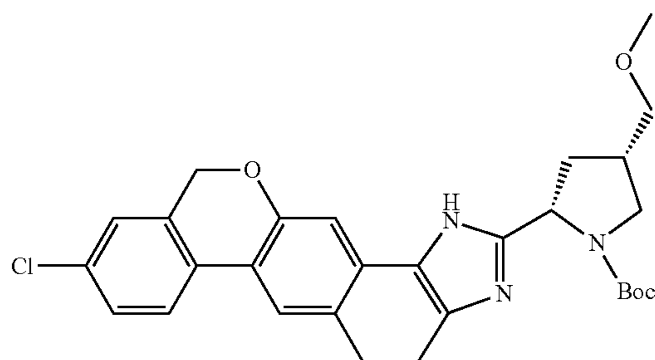
(2S,4S)-tert-butyl 2-(9-chloro-4,5-dihydro-1,11-dihydroisochromeno[4',3':6,7]naphtho[1,2-d]imidazol-2-yl)-4-(methoxymethyl)pyrrolidine-1-carboxylate
