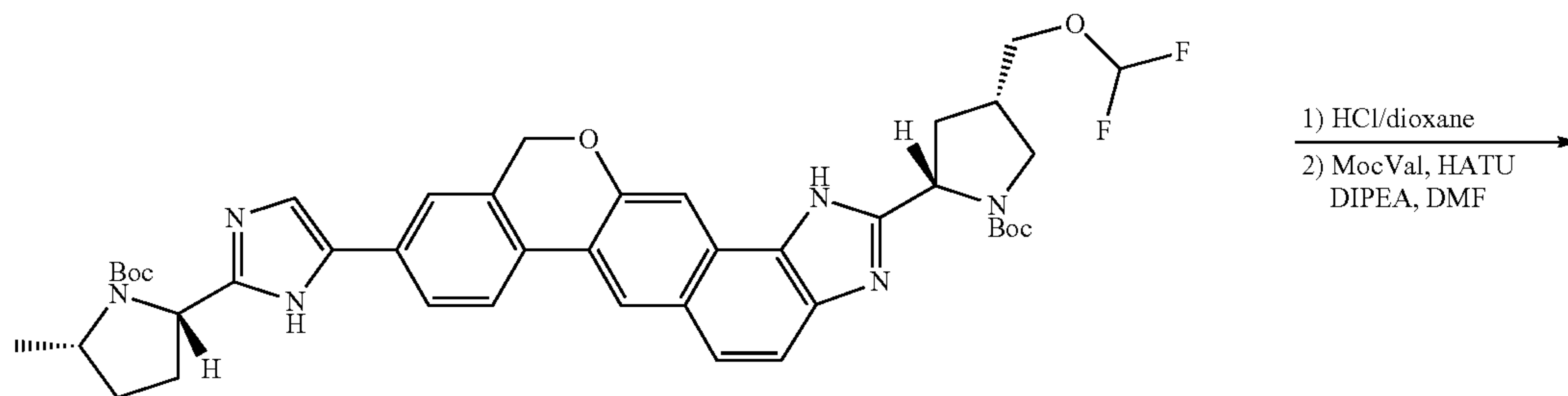
tert-butyl (2S,4S)-2-(9-{2-[(2S,5S)-1-(tert-butoxycarbonyl)-5-methylpyrrolidin-2-yl]-1H-imidazol-5-yl}-1,11-dihydroisochromeno[4',3':6,7]naphtho[1,2-d]imidazol-2-yl)-4-[(difluoromethoxy)methyl]pyrrolidine-1-carboxylate
