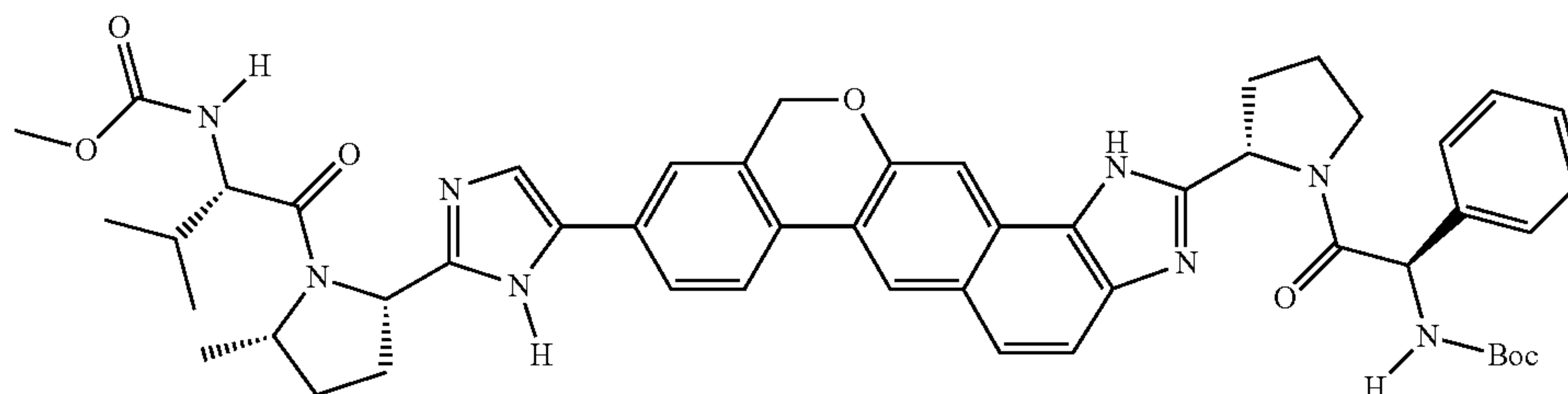
methyl {(2S)-1-[(2S,5S)-2-(5-{2-[(2S)-1-[(2R)-2-[(tert-butoxycarbonyl)amino]-2-phenylacetyl]pyrrolidin-2-yl]-1,11-dihydroisochromeno[4',3':6,7]naphtho[1,2-d]imidazol-9-yl}-1H-imidazol-2-yl)-5-methylpyrrolidin-1-yl]-3-methyl-1-oxobutan-2-yl} carbamate
