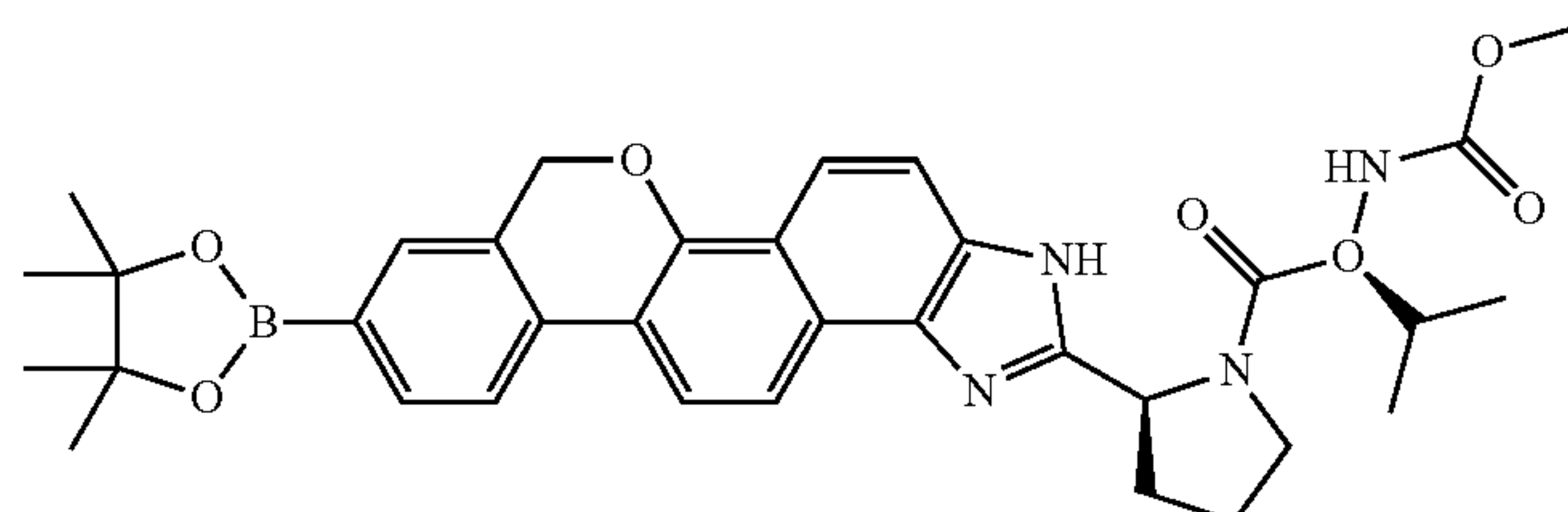
methyl[(2S)-3-methyl-1-oxo-1-[(2S)-2-[9-(4,4,5,5-tetramethyl-1,3,2-dioxaborolan-2-yl)-3,11-dihydroisochromeno[4',3':6,7]naphtho[1,2-d]imidazol-2-yl]pyrrolidin-1-yl]butan-2-yl]carbamate
