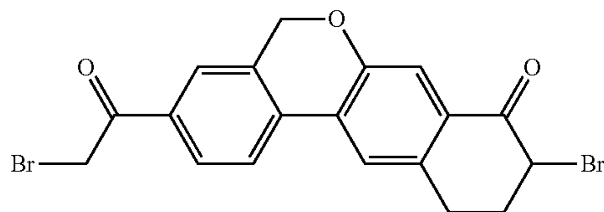
9-bromo-3-(2-bromoacetyl)-10,11-dihydro-5H-dibenzo[c,g]chromen-8(9H)-one
