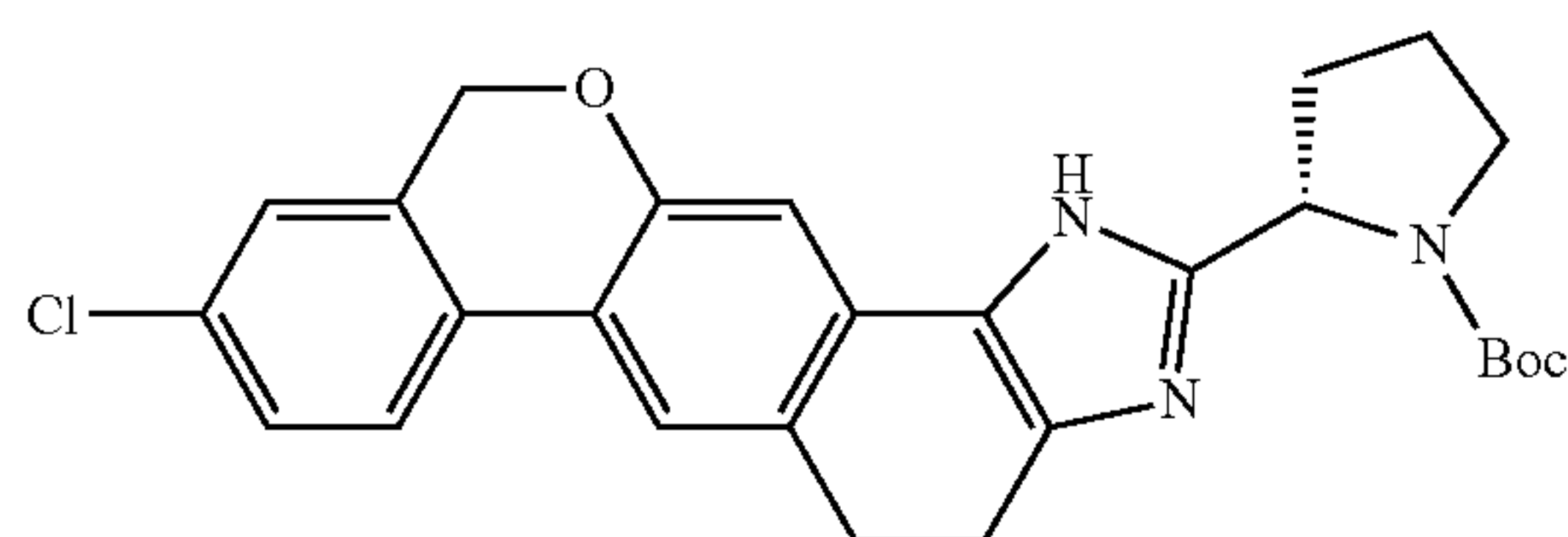
tert-butyl 2-(9-chloro-1,4,5,11-tetrahydroisochromeno[4',3':6,7]naphtho[1,2-d]imidazol-2-yl)pyrrolidine-1-carboxylate
