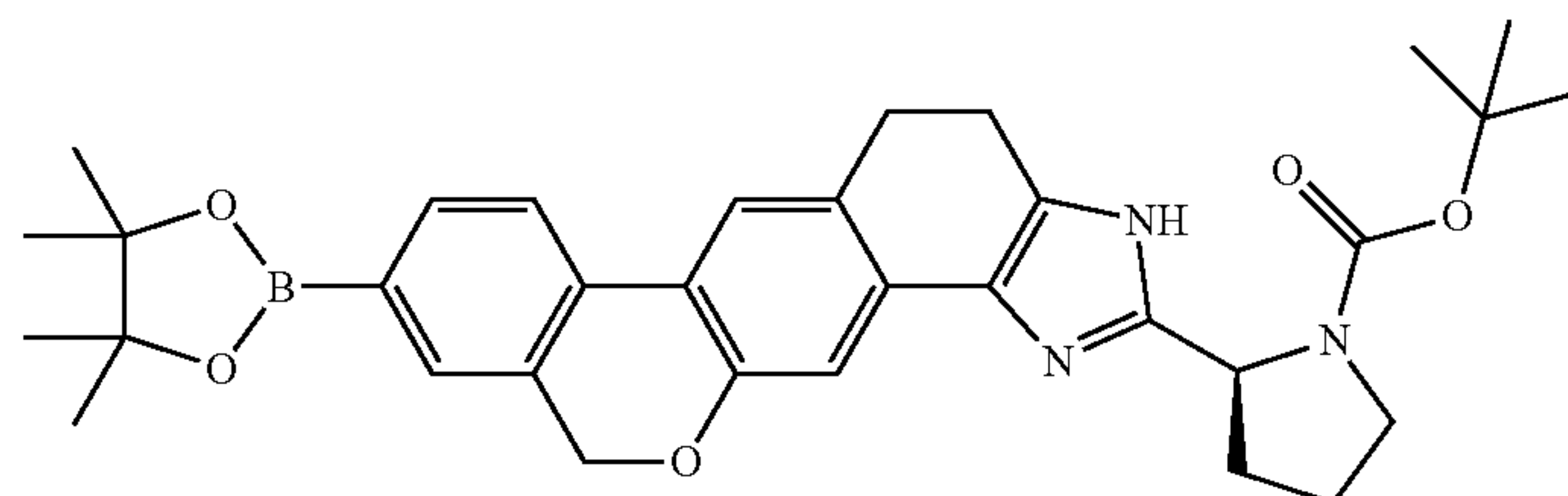
tert-butyl (2S)-2-[9-(4,4,5,5-tetramethyl-1,3,2-dioxaborolan-2-yl)-3,4,5,11-tetrahydroisochromeno[4',3':6,7]naphtho[1,2-d]imidazol-2-yl]pyrrolidine-1-carboxylate
