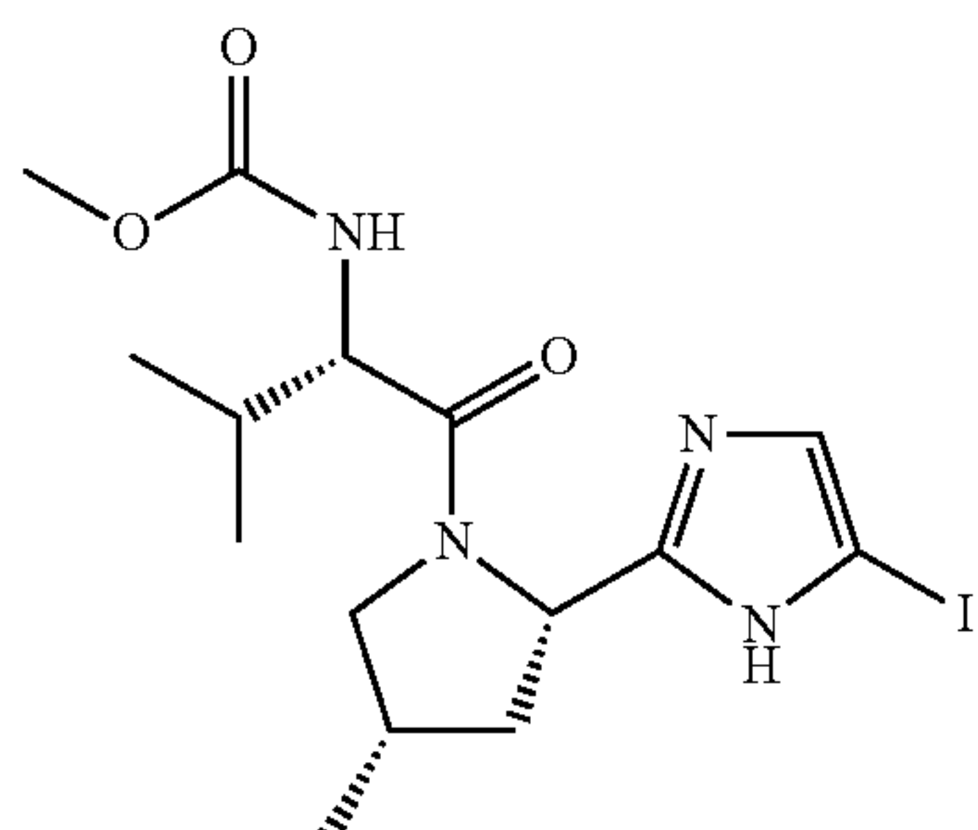
methyl (S)-1-((2S,4S)-2-(5-iodo-1H-imidazol-2-yl)-4-methylpyrrolidin-1-yl)-3-methyl-1-oxobutan-2-ylcarbamate
