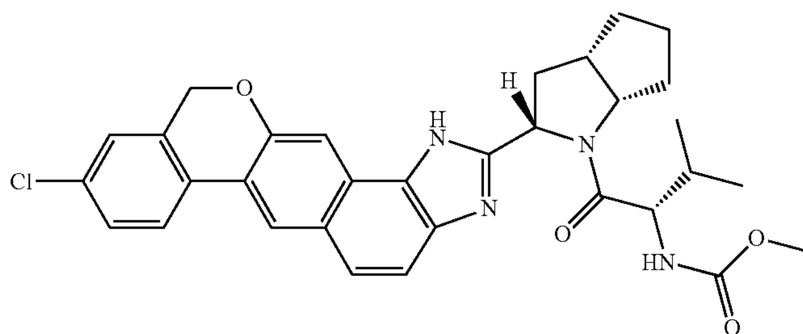
methyl {(2S)-1-[(2S,3aS,6aS)-2-9-chloro-1,11-dihydroisochromeno[4'3':6,7]naphtho[1,2-d]imidazol-2-yl]hexahydrocyclopenta[b]pyrrol-1(2H)-yl]-3-methyl-1-oxobutan-2-yl}carbamate
