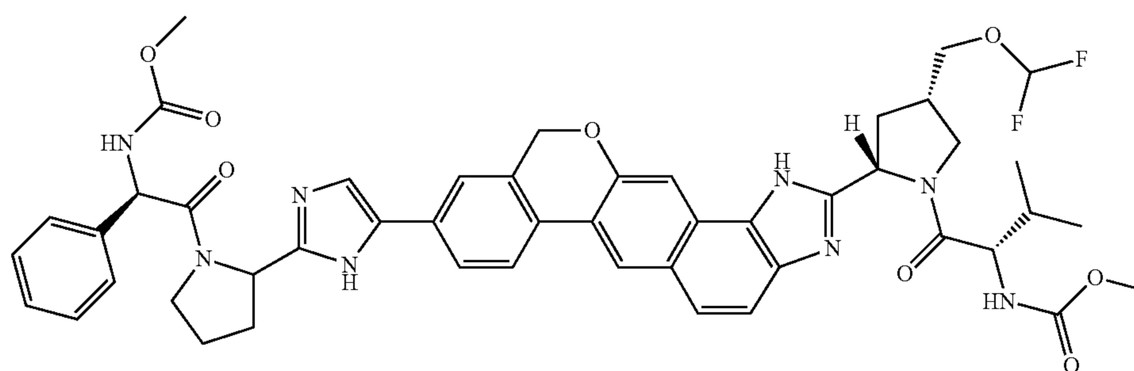
methyl ((1R)-2-[2-(5-(2-((2S,4S)-4-((difluoromethoxy)methyl)-1-[N-(methoxycarbonyl)-L-valyl]pyrrolidin-2-yl)-1,11-dihydroisochromeno[4',3':6,7]naphtho[1,2-d]imidazol-9-yl)-1H-imidazol-2-yl]pyrrolidine-1-carboxylate
