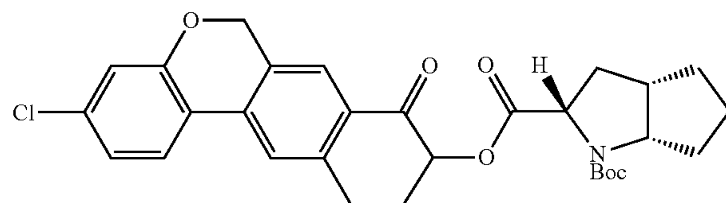
(2S,3aS,6aS)-1-tert-butyl 2-(3-chloro-8-oxo-8,9,10,11-tetrahydro-6H-naphtho[2,3-c]chromen-9-yl)hexahydrocyclopenta[b]pyrrole-1,2(2H)-dicarboxylate
