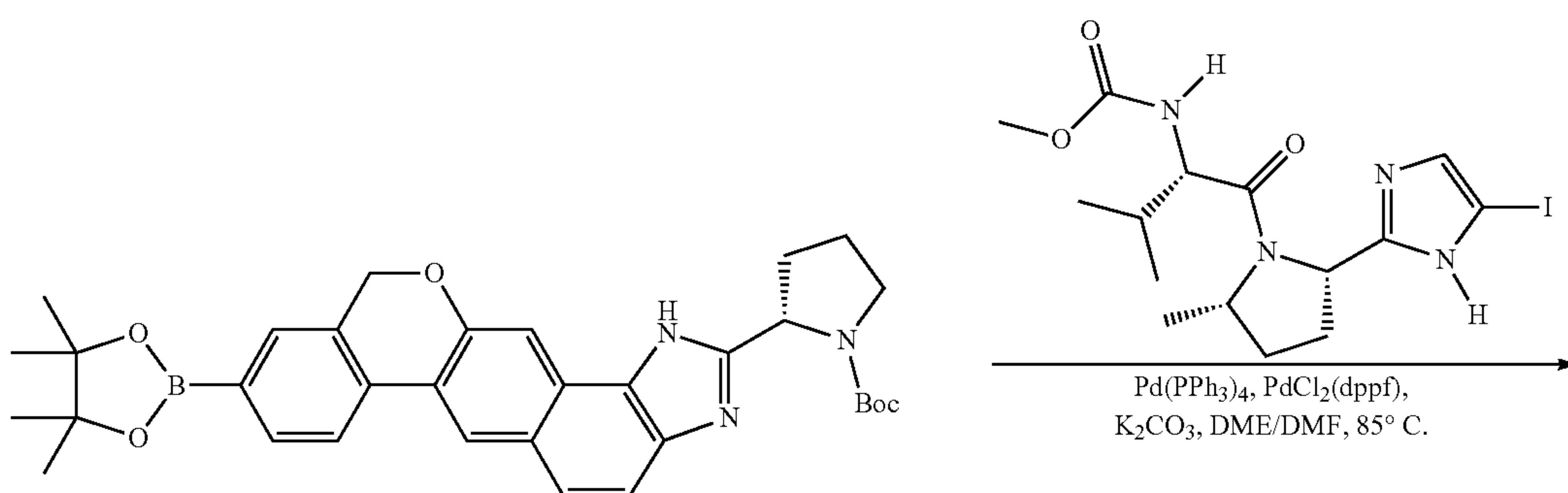
tert-butyl 2-[9-(4,4,5,5-tetramethyl-1,3,2-dioxaborolan-2-yl)-1,11-dihydroisochromeno[4',3':6,7]naphtho[1,2-d]imidazol-2-yl]pyrrolidine-1-carboxylate
