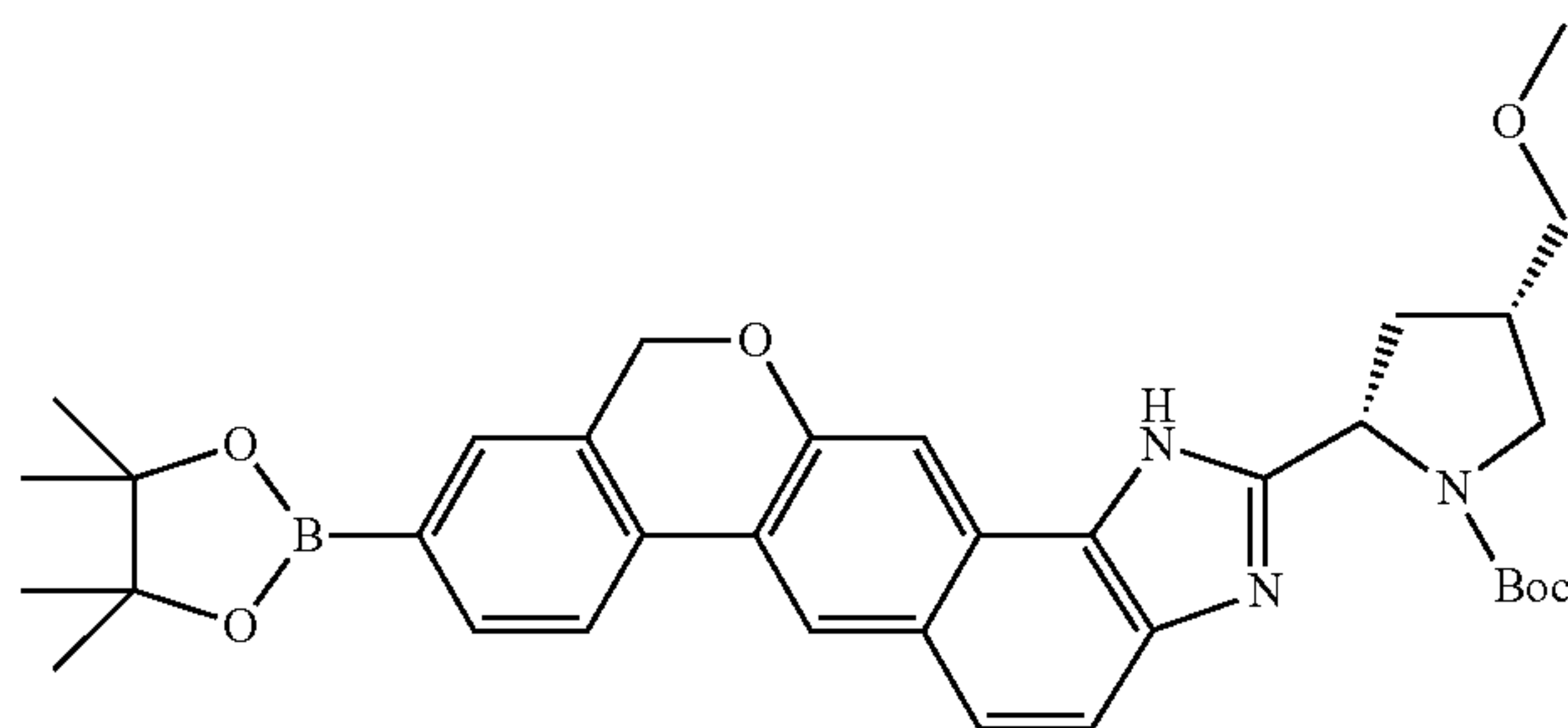
(2S,4S)-tert-butyl 4-(methoxymethyl)-2-(9-(4,4,5,5-tetramethyl-1,3,2-dioxaborolan-2-yl)-1,11-dihydroisochromeno[4',3':6,7]naphtho[1,2-d]imidazol-2-yl)pyrrolidine-1-carboxylate
