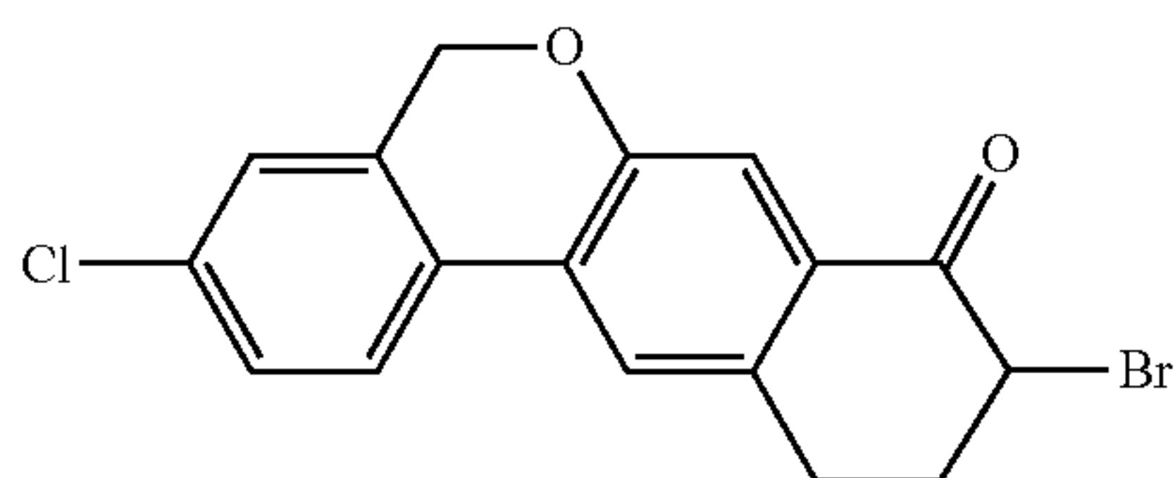
9-bromo-3-chloro-10,11-dihydro-5H-dibenzo[c,g]chromen-8(9H)-one
