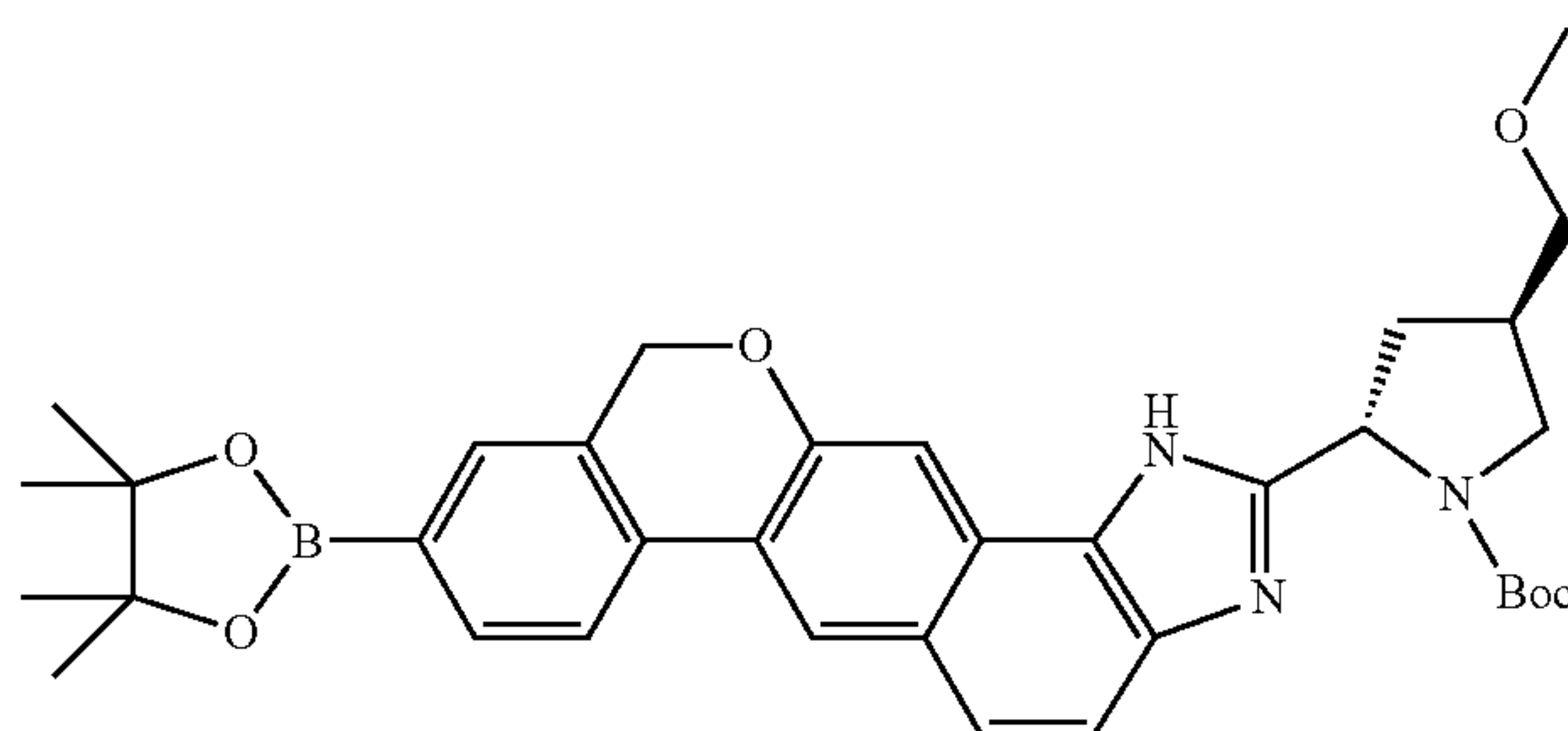
(2S,4R)-tert-butyl 4-(methoxymethyl)-2-(9-(4,4,5,5-tetramethyl-1,3,2-dioxaborolan-2-yl)-1,11-dihydroisochromeno[4',3':6,7]naphtho[1,2-d]imidazol-2-yl)pyrrolidine-1-carboxylate
