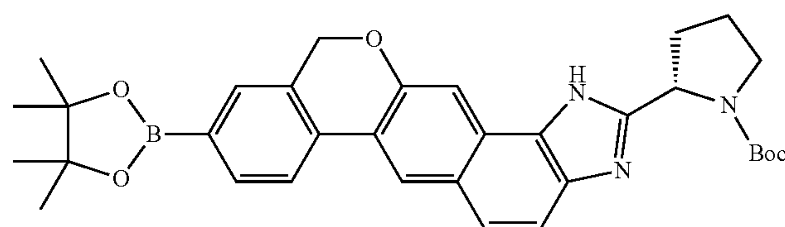
tert-butyl 2-[9-(4,4,5,5-tetramethyl-1,3,2-dioxaborolan-2-yl)-1,11-dihydroisochromeno[4',3':6,7]naphtho[1,2-d]imidazol-2-yl]pyrrolidine-1-carboxylate
