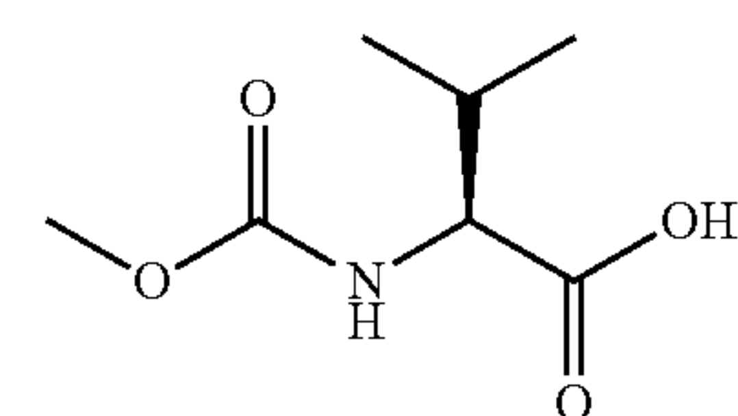
(S)-2-(methoxycarbonylamino)-3-methylbutanoic acid
