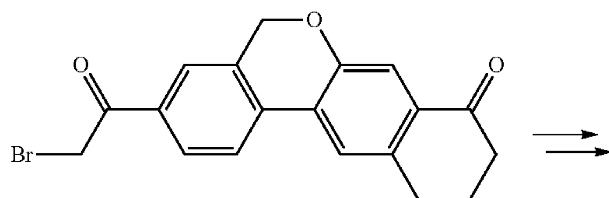
3-(2-bromoacetyl)-10,11-dihydro-5H-dibenzo[c,g]chromen-8(9H)-one
