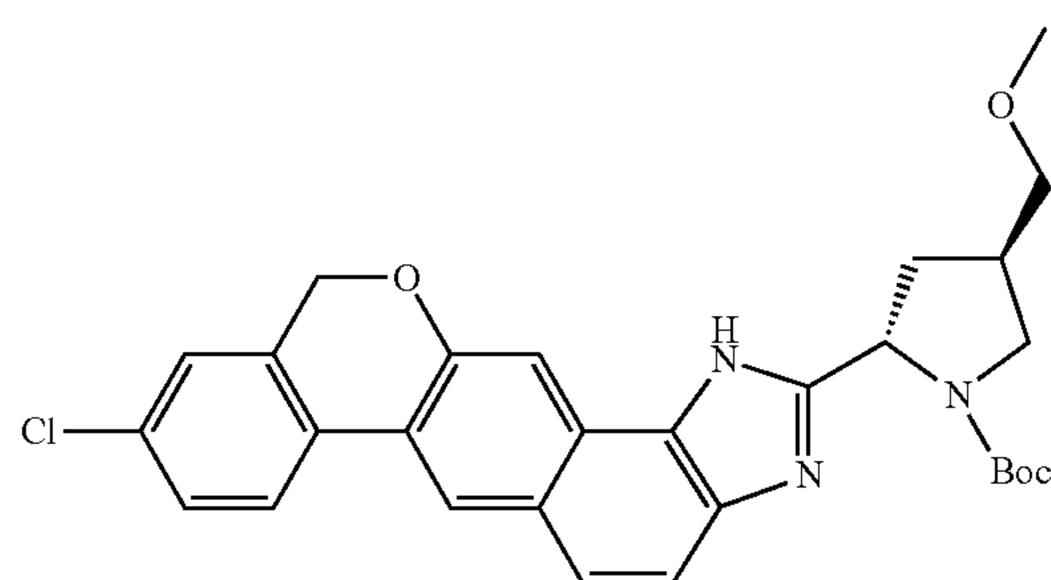
(2S,4R)-tert-butyl 2-(9-chloro-1,11-dihydroisochromeno[4',3':6,7]naphtho[1,2-d]imidazol-2-yl)-4-(methoxymethyl)pyrrolidine-1-carboxylate
