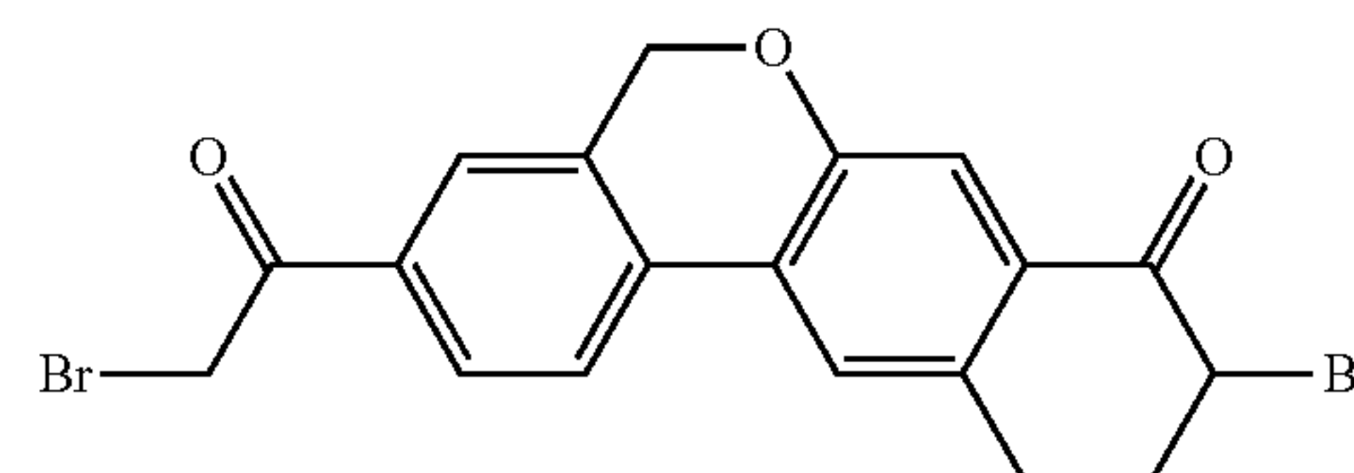
9-bromo-3-(2-bromoacetyl)-10,11-dihydro-5H-dibenzo[c,g]chromen-8(9H)-one
