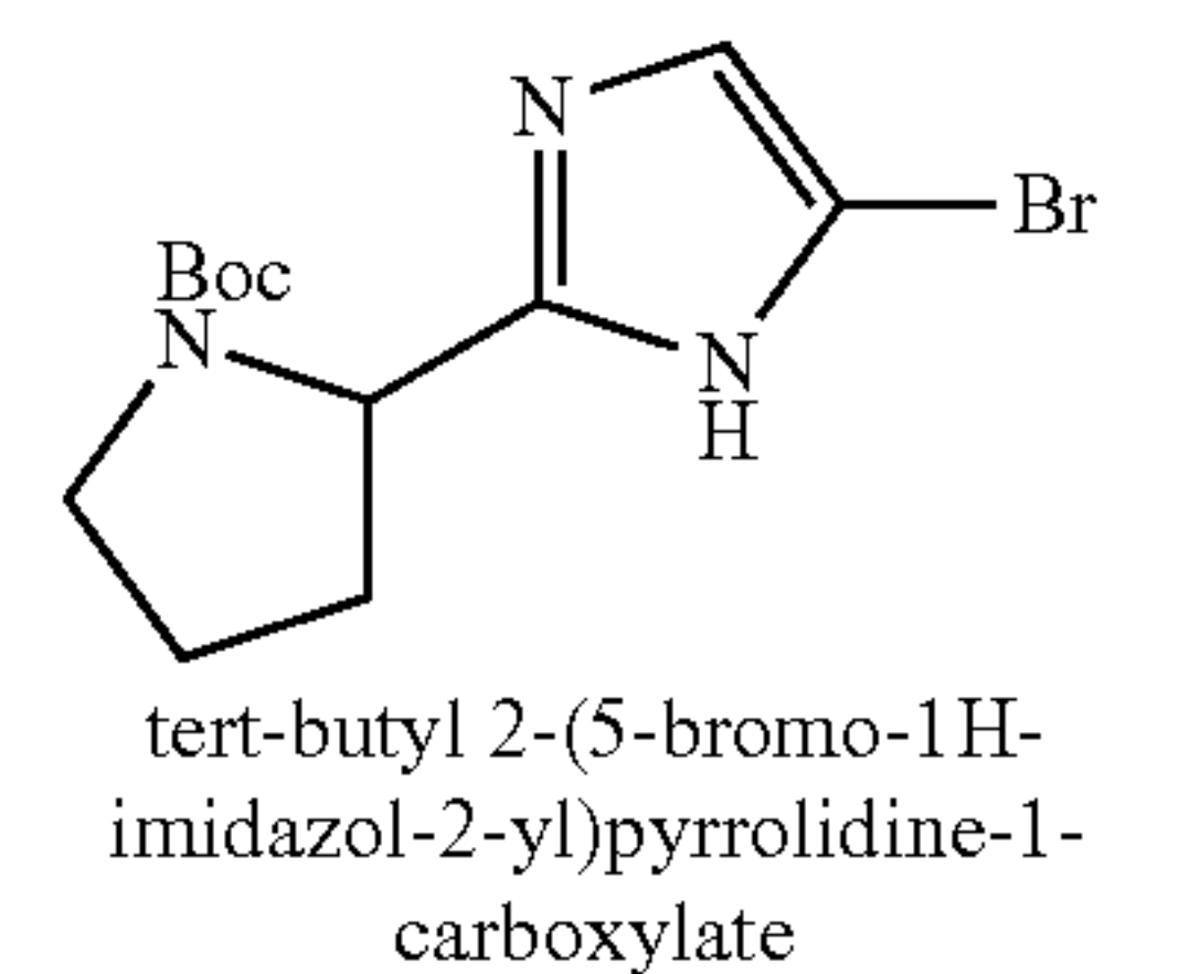
tert-butyl 2-(5-bromo-1H-imidazol-2-yl)pyrrolidine-1-carboxylate
