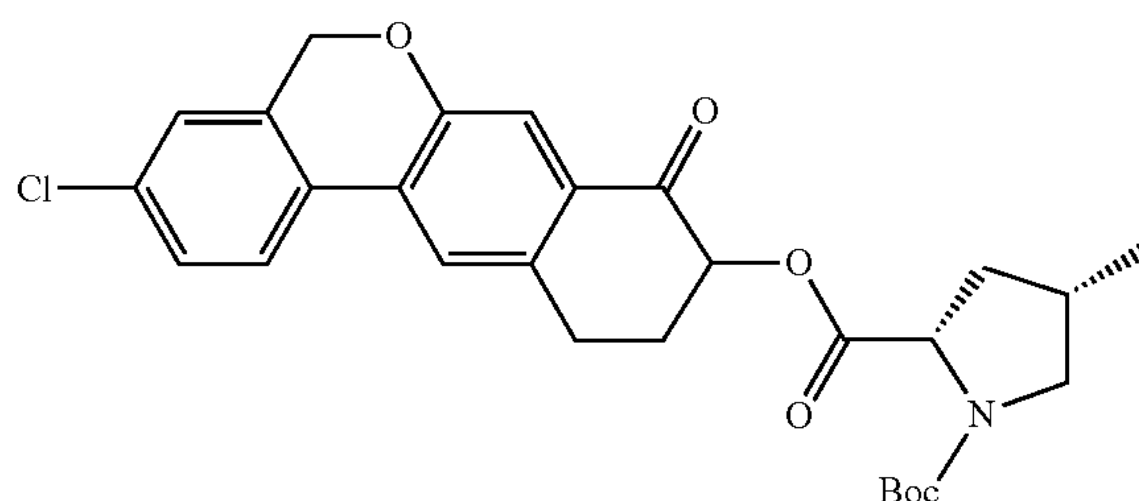
(2S,4S)-1-tert-butyl 2-(3-chloro-8-oxo-8,9,10,11-tetrahydro-5H-dibenzo[c,g]chromen-9-yl)-4-methylpyrrolidine-1,2-dicarboxylate
