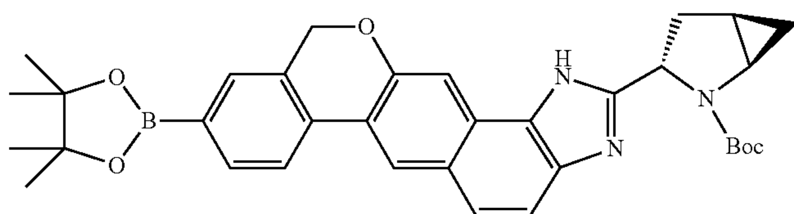
(1R,3S,5R)-tert-butyl 3-(9-(4,4,5,5-tetramethyl-1,3,2-dioxaborolan-2-yl)-1,11-dihydroisochromeno[4',3':6,7]naphtho[1,2-d]imidazol-2-yl)-2-azabicyclo[3.1.0]hexane-2-carboxylate
