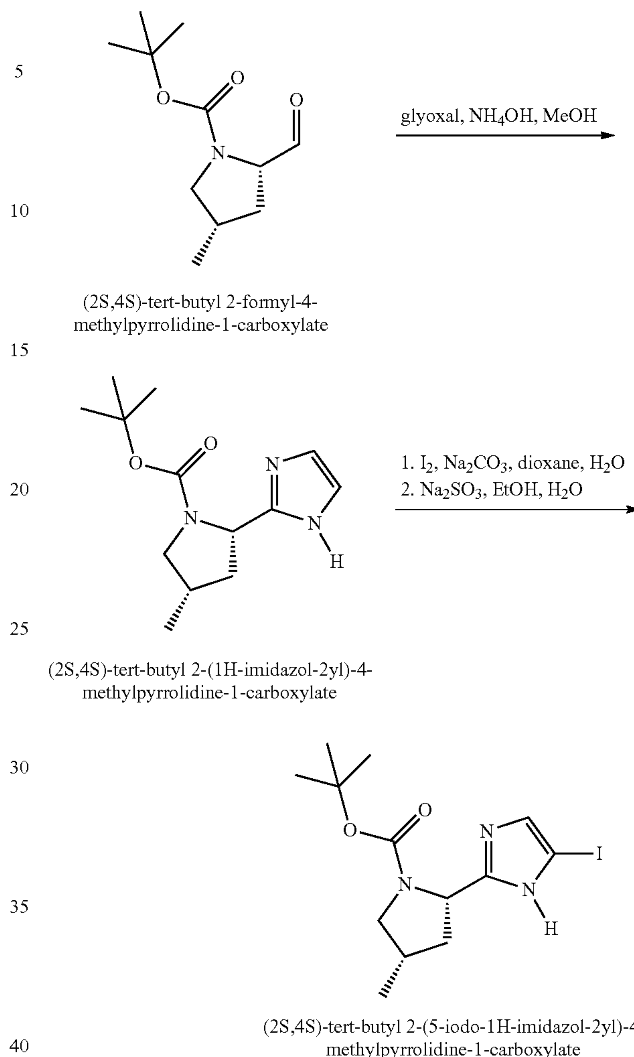
(2S,4S)-tert-butyl 2-formyl-4-methylpyrrolidine-1-carboxylate
