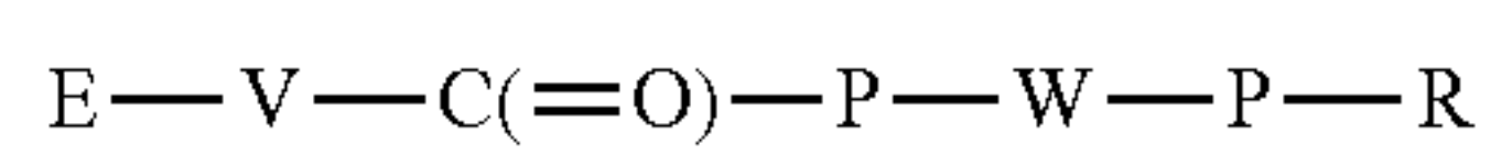
Scheme 28. Representative synthesis of
