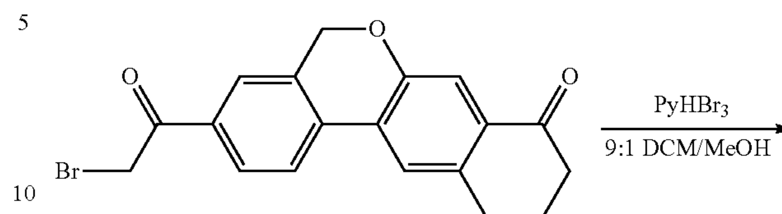
3-(2-bromoacetyl)-10,11-dihydro-5H-dibenzo[c,g]chromen-8(9H)-one
