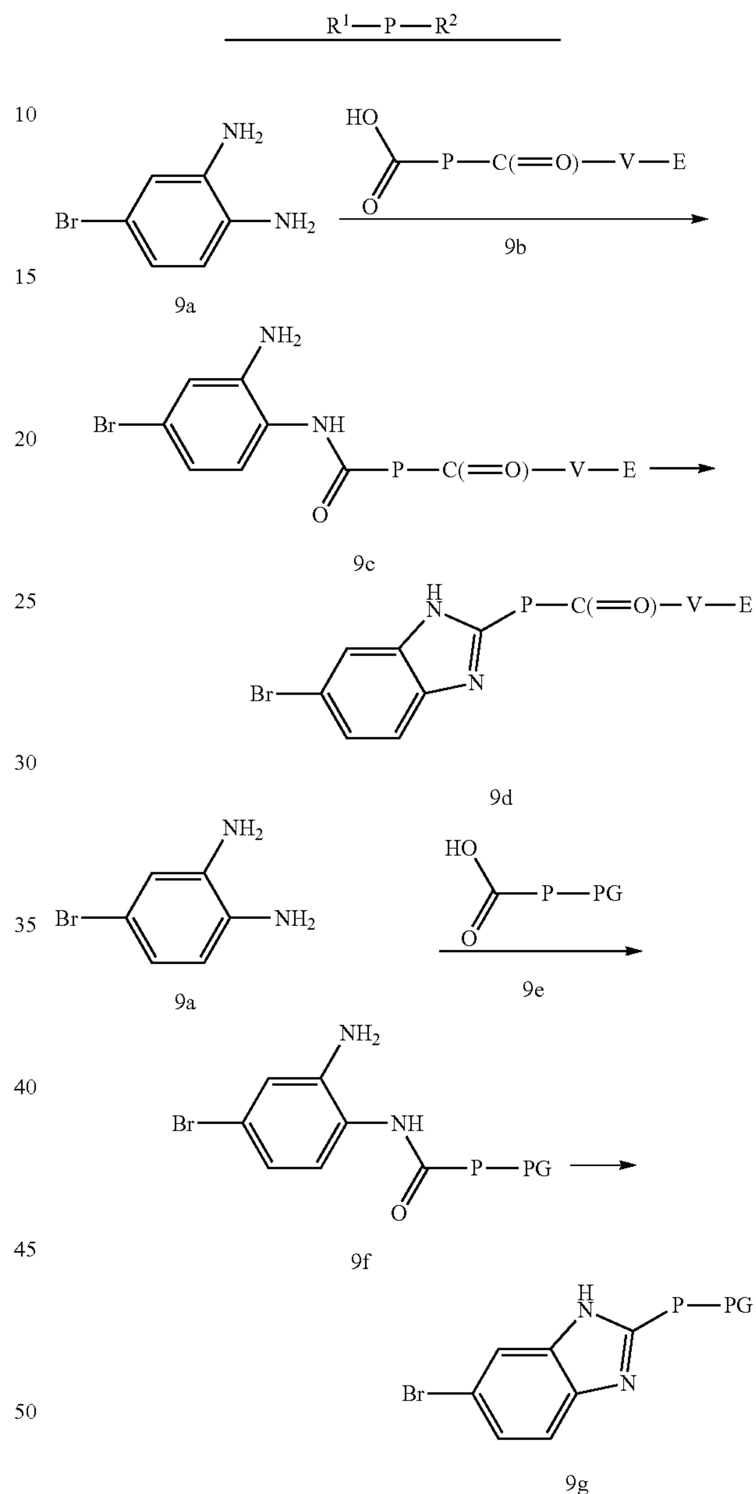
Scheme 9. Representative synthesis
