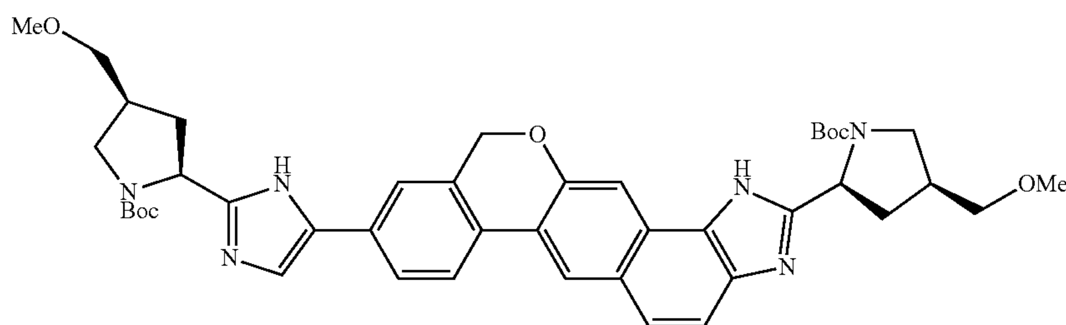
tert-butyl (2S,4S)-2-(5-{2-[(2S,4S)-1-(tert-butoxycarbonyl)-4-(methoxymethyl)pyrrolidin-2-yl]-1,11-dihydroisochromeno[4',3':6,7]naphtho[1,2-d]imidazol-9-yl}-1H-imidazol-2-yl)-4-(methoxymethyl)pyrrolidine-1-carboxylate
