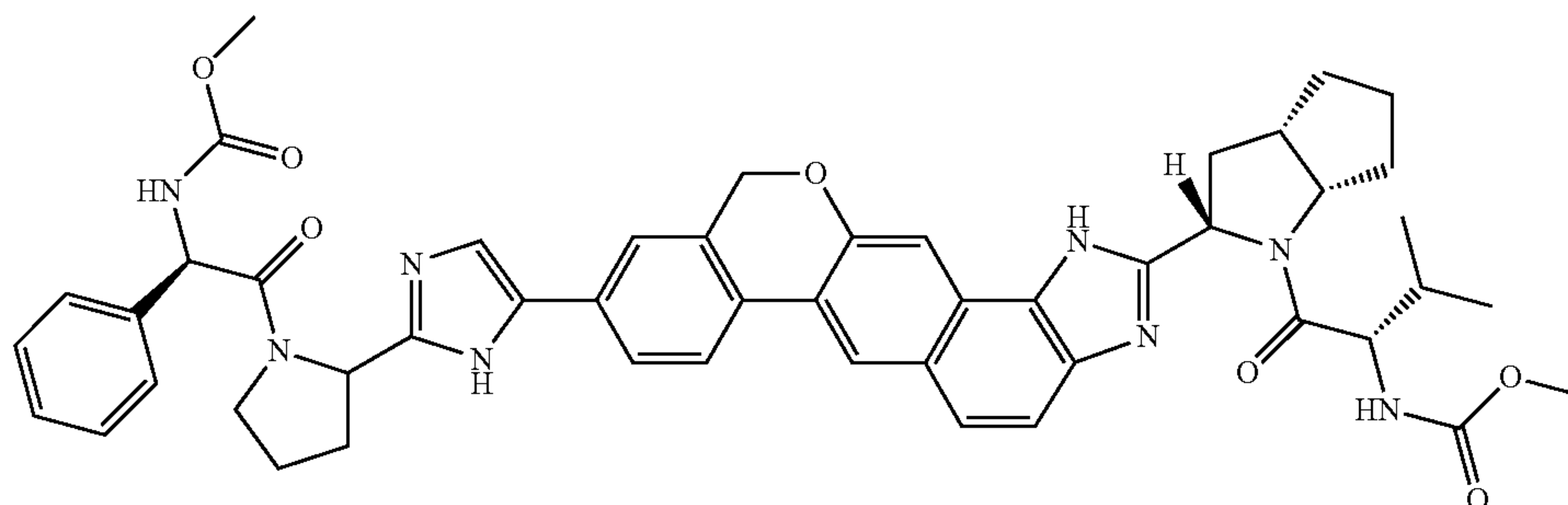
methyl ((1R)-2-[2-(5-{2-[(2S,3aS,6aS)-1-{(2S)-2-[(methoxycarbonyl)amino]-3-methylbutanoyl}octahydrocyclopenta[b]pyrrol-2-yl]-1,11-dihydroisochromeno[4',3':6,7]naphtho[1,2-d]imidazol-9-yl}-1H-imidazol-2-yl)pyrrolidin-1-yl]-2-oxo-1-phenylethyl}carbamate
