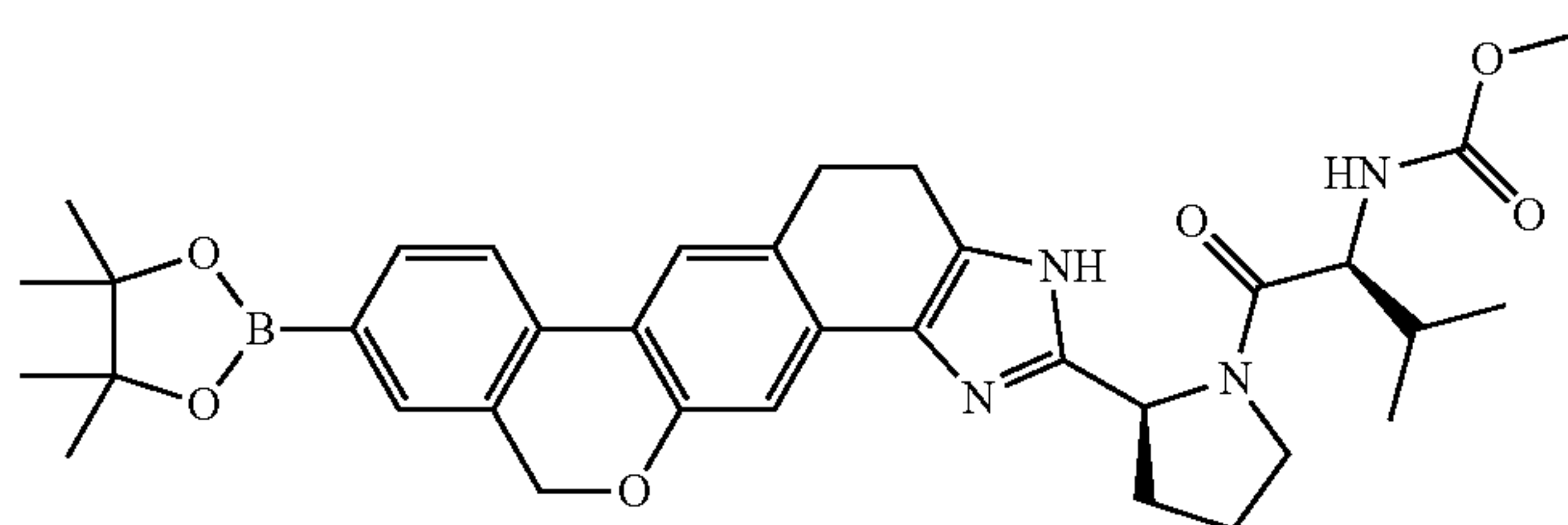
methyl[(2S)-3-methyl-1-oxo-1-{(2S)-2-[9-(4,4,5,5-tetramethyl-1,3,2-dioxaborolan-2-yl)-3,4,5,11-tetrahydroisochromeno[4',3':6,7]naphtho[1,2-d]imidazol-2-yl]pyrrolidin-1-yl}butan-2-yl]carbamate
