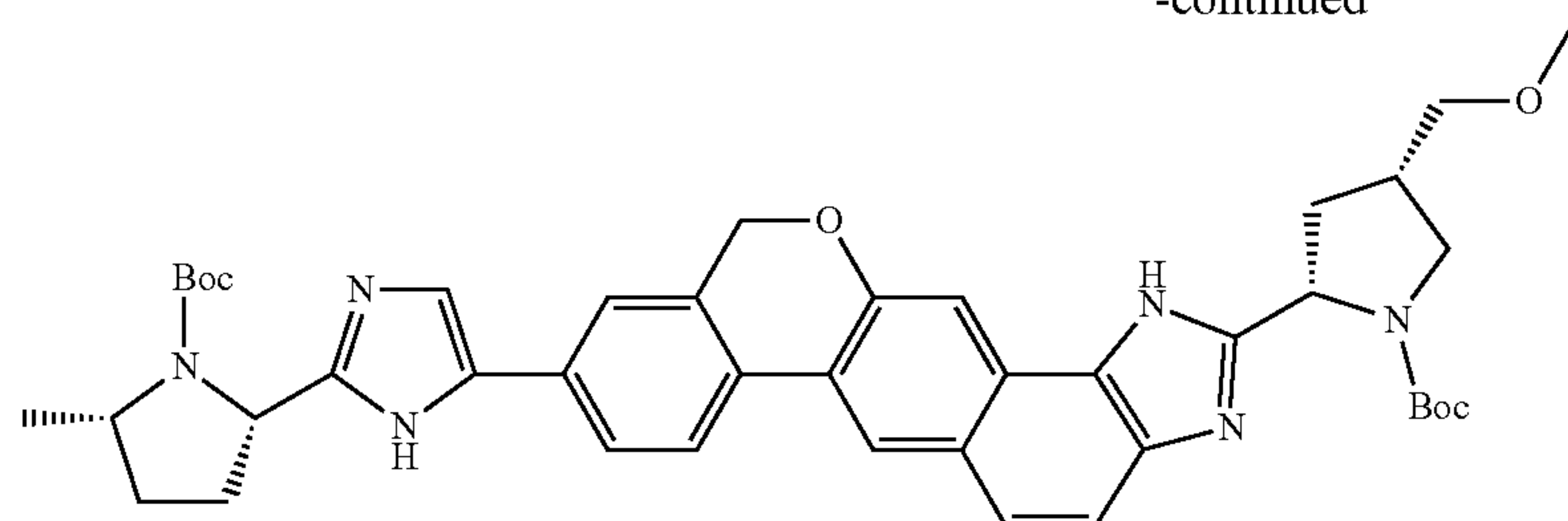
tert-butyl (2S,4S)-2-(5-{2-[(2S,4S)-1-(tert-butoxycarbonyl)-4-(methoxymethyl)pyrrolidin-2-yl]-1,11-dihydroisochromeno[4',3':6,7]naphtho[1,2-d]imidazol-9-yl}-1H-imidazol-2-yl)-5-methylpyrrolidine-1-carboxylate
