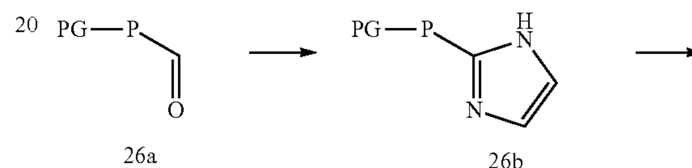
Scheme 26. Representative syntheses of E-V-C(=O)-P-R and R 1 -P-R
