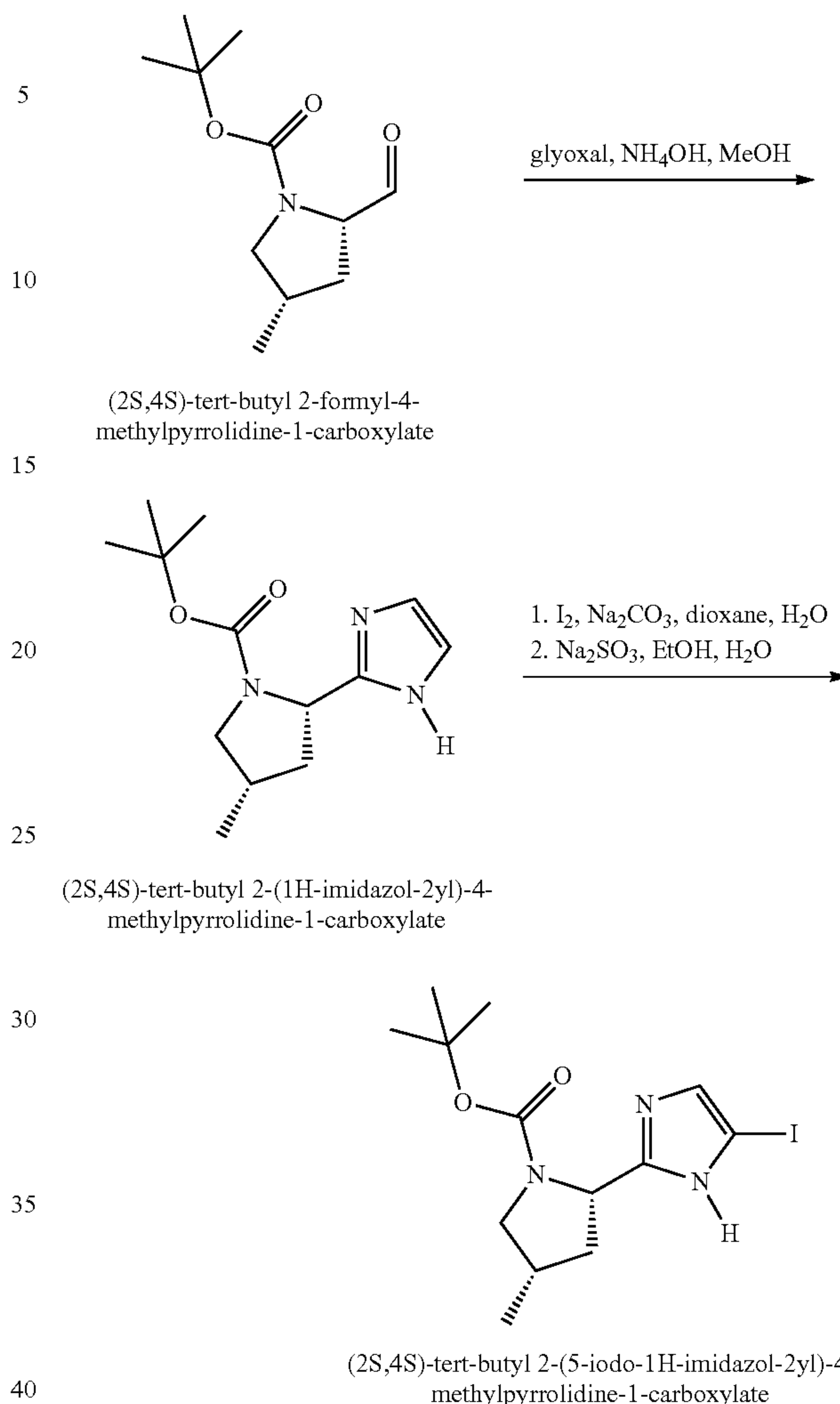
(2S,4S)-tert-butyl 2-formyl-4-methylpyrrolidine-1-carboxylate
