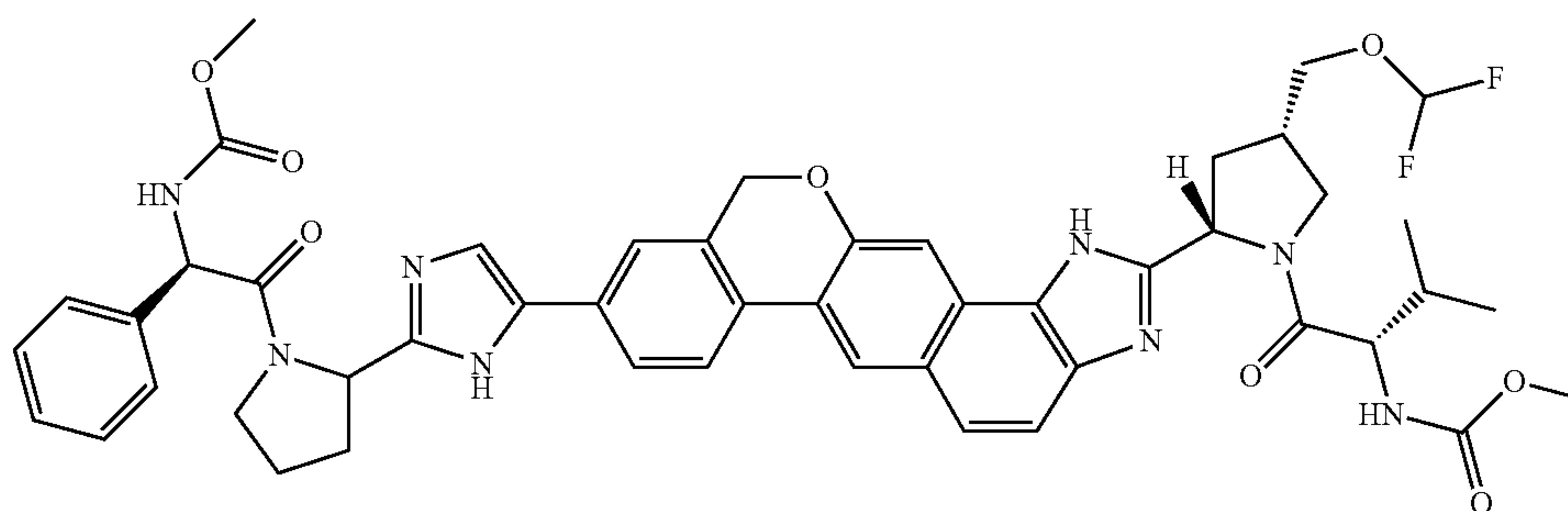
methyl ((1R)-2-[2-(5-(2-((2S,4S)-4-[(difluoromethoxy)methyl]-1-[N-(methoxycarbonyl)amino]-3-methylbutanoyl]pyrrolidin-2-yl)-1,11-dihydroisochromeno[4',3':6,7]naphtho[1,2-d]imidazol-9-yl)-1H-imidazol-2-yl]pyrrolidin-1-yl]-2-oxo-1-phenylethyl]carbamate
