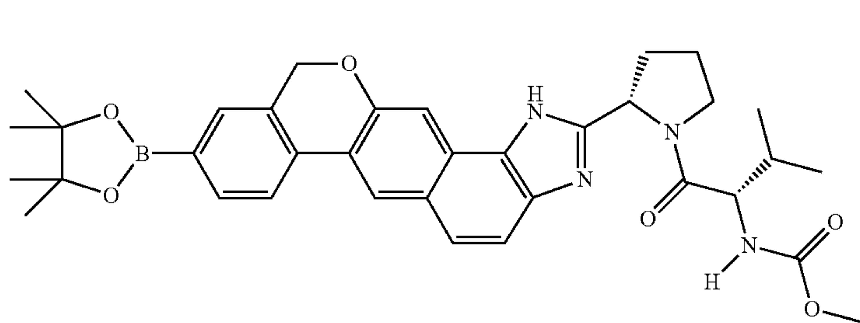
(2S)-methyl {2-[(9-(4,4,5,5-tetramethyl-1,3,2-dioxaborolan-2-yl)-1,11-dihydroisochromeno[4',3':6,7]naphtho[1,2-d]imidazol-2-yl)pyrrolidin-1-yl]-3-methyl-1-oxobutan-2-yl}carbamate
