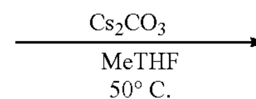
(2S,4S)-1-(tert-butoxycarbonyl)-4-methylpyrrolidine-2-carboxylic acid
