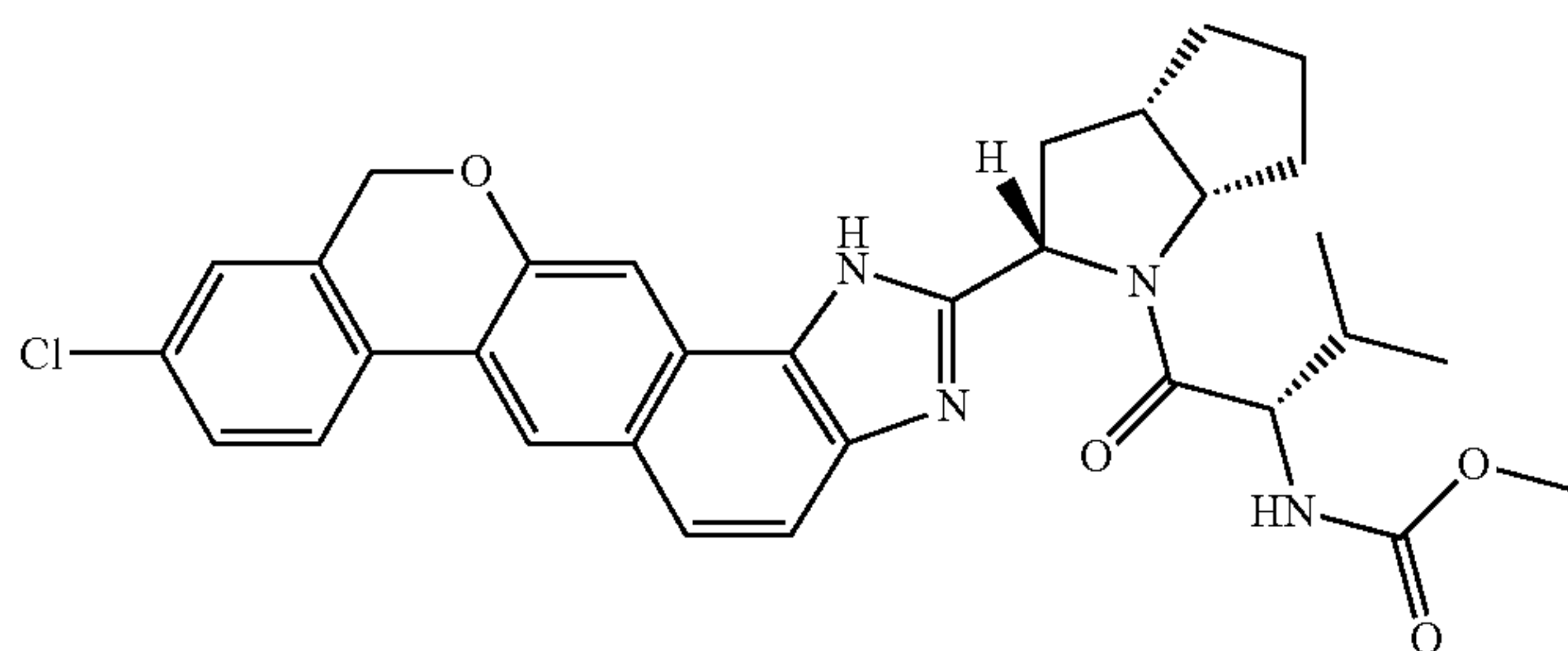
methyl {(2S)-1-[(2S,3aS,6aS)-2-9-chloro-1,11-dihydroisochromeno[4'3':6,7]naphtho[1,2-d]imidazol-2-yl]hexahydrocyclopenta[b]pyrrol-1(2H)-yl]-3-methyl-1-oxobutan-2-yl}carbamate
