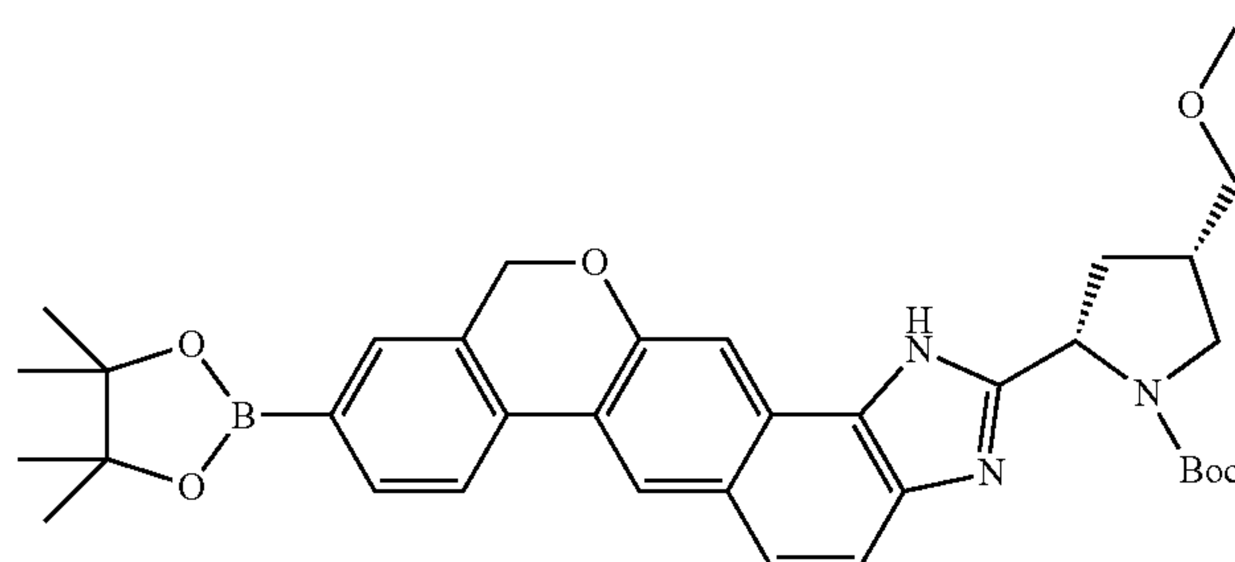
(2S,4S)-tert-butyl 4-(methoxymethyl)-2-(9-(4,4,5,5-tetramethyl-1,3,2-dioxaborolan-2-yl)-1,11-dihydroisochromeno[4',3':6,7]naphtho[1,2-d]imidazol-2-yl)pyrrolidine-1-carboxylate
