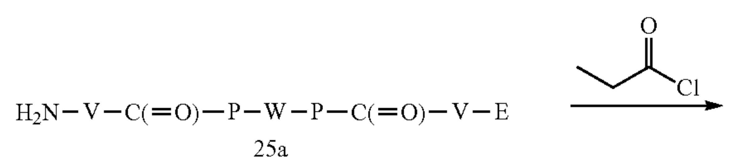
Scheme 25. Representative synthesis of E-V-C(=O)-P-W-P-C(=O)-V-E
