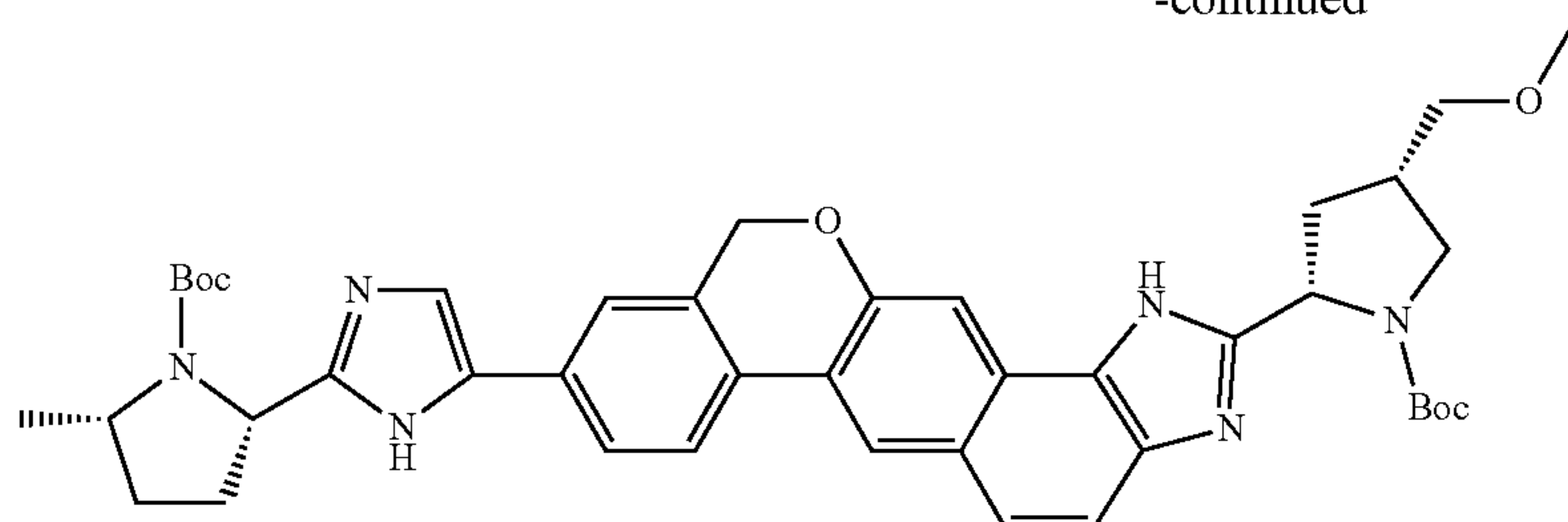
tert-butyl (2S,4S)-2-(5-{2-[(2S,4S)-1-(tert-butoxycarbonyl)-4-(methoxymethyl)pyrrolidin-2-yl]-1,11-dihydroisochromeno[4',3':6,7]naphtho[1,2-d]imidazol-9-yl}-1H-imidazol-2-yl)-5-methylpyrrolidine-1-carboxylate
