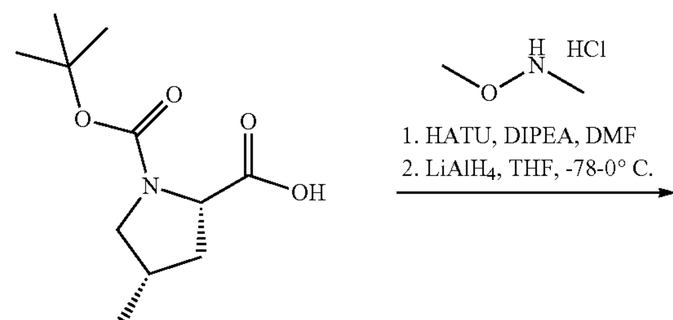
(2S,4S)-1-tert-butoxycarbonyl-4-methylpyrrolidine-2-carboxylic acid
