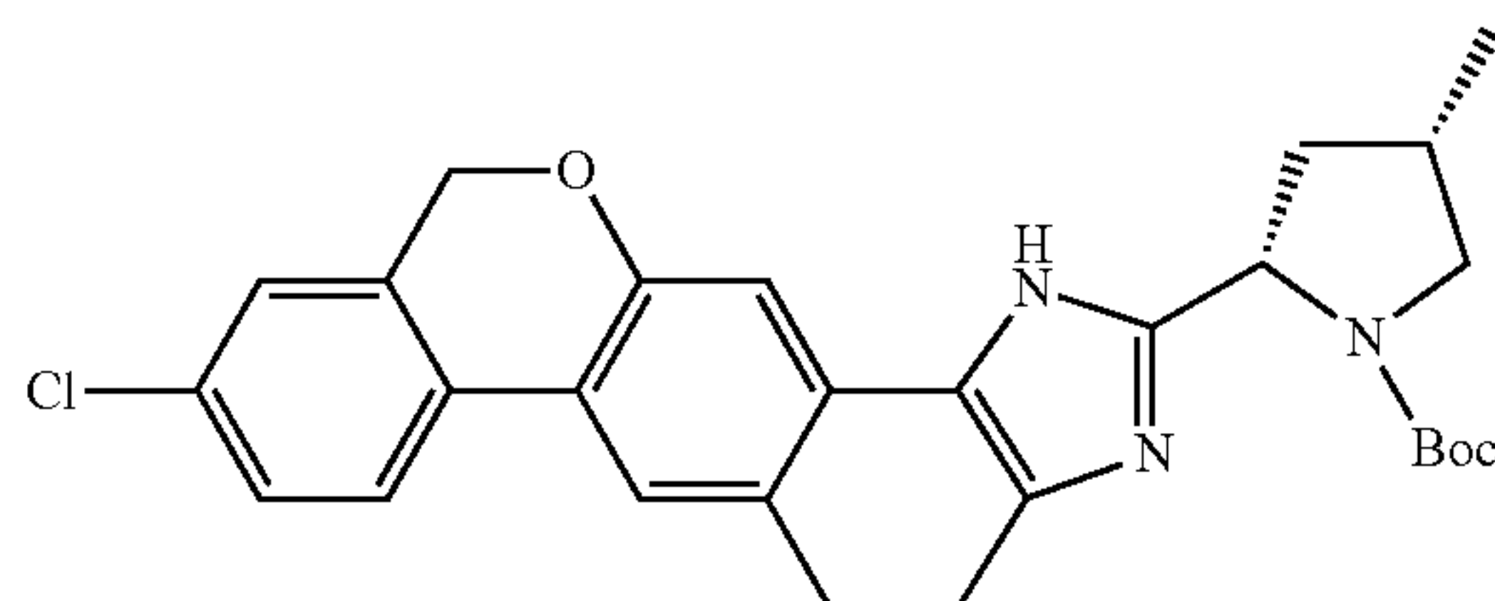
(2S,4S)-1-tert-butyl 2-(9-chloro-4,5-dihydro-5H-naphtho[c,g]chromeno[8,9-d]imidazol-2-yl)-4-methylpyrrolidine-1-carboxylate
