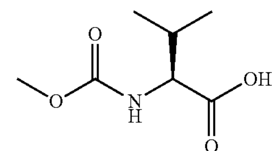
(S)-2-(methoxycarbonylamino)-3-methylbutanoic acid
