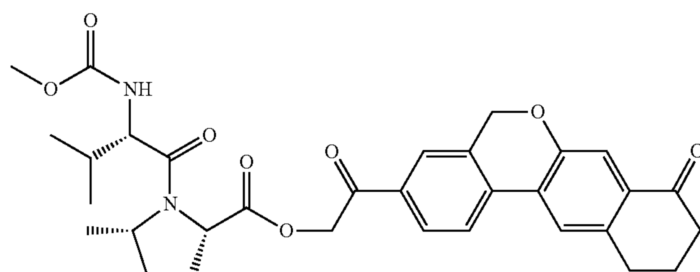
(2S,5S)-2-oxo-2-(8-oxo-8,9,10,11-tetrahydro-5H-dibenzo[c,g]chromen-3-yl)ethyl 1-((S)-2-(methoxycarbonylamino)-3-methylbutanoyl)-5-methylpyrrolidine-2-carboxylate
