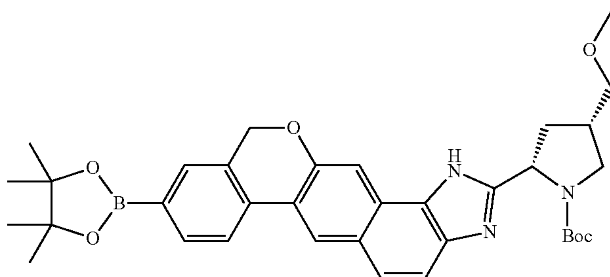
(2S,4S)-tert-butyl 4-(methoxymethyl)-2-(9-(4,4,5,5-tetramethyl-1,3,2-dioxaborolan-2-yl)-5H-naphtho[c,g]chromeno[8,9-d]imidazol-2-yl)pyrrolidine-2-carboxylate
