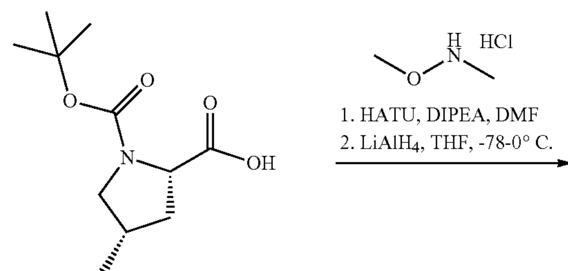
(2S,4S)-1-tert-butoxycarbonyl-4-methylpyrrolidine-2-carboxylic acid
