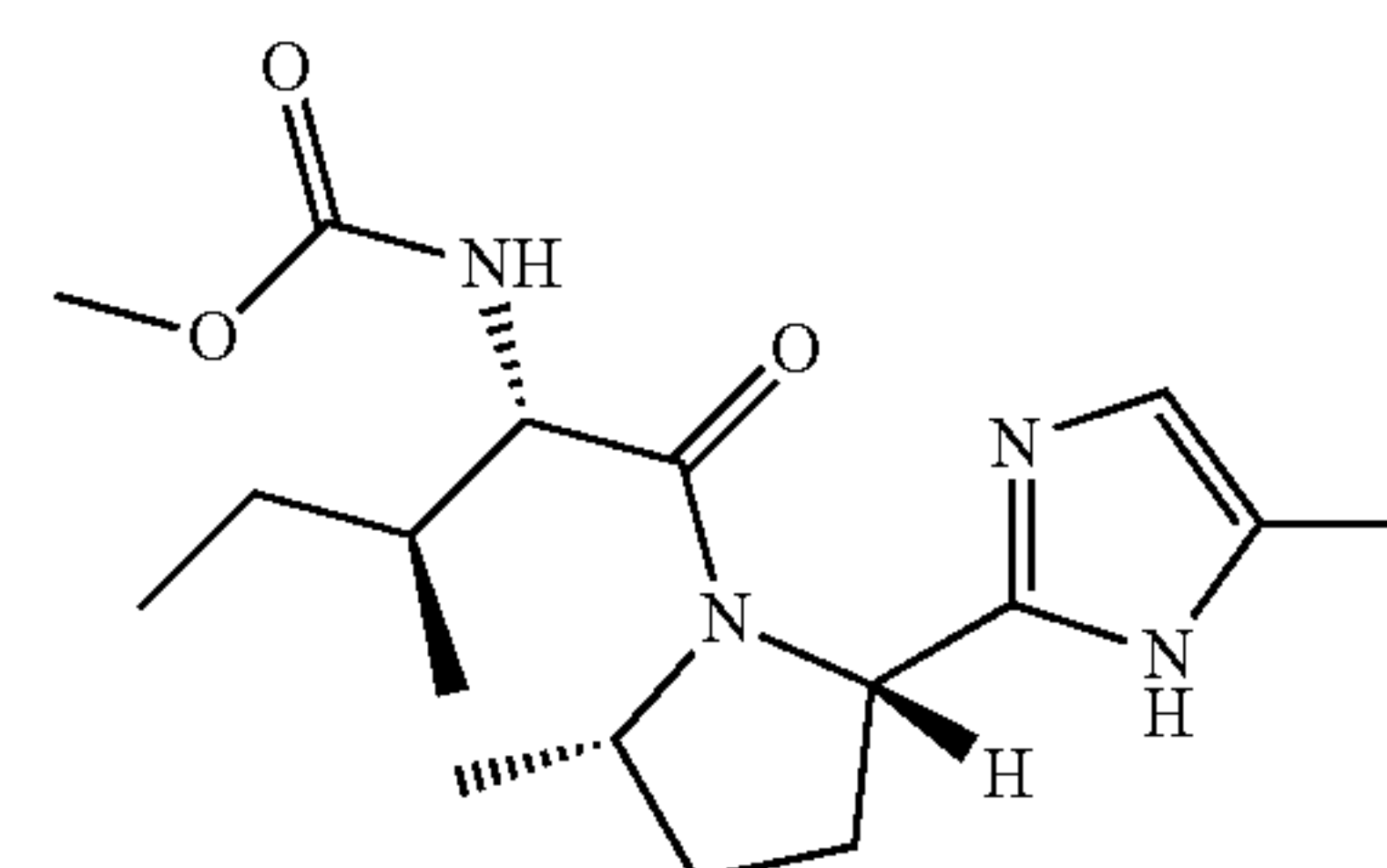
methyl (2S,3S)-1-((2S,5S)-2-(5-iodo-1H-imidazol-2-yl)-5-methylpyrrolidin-1-yl)-3-methyl-1-oxopentan-2-ylcarbamate
