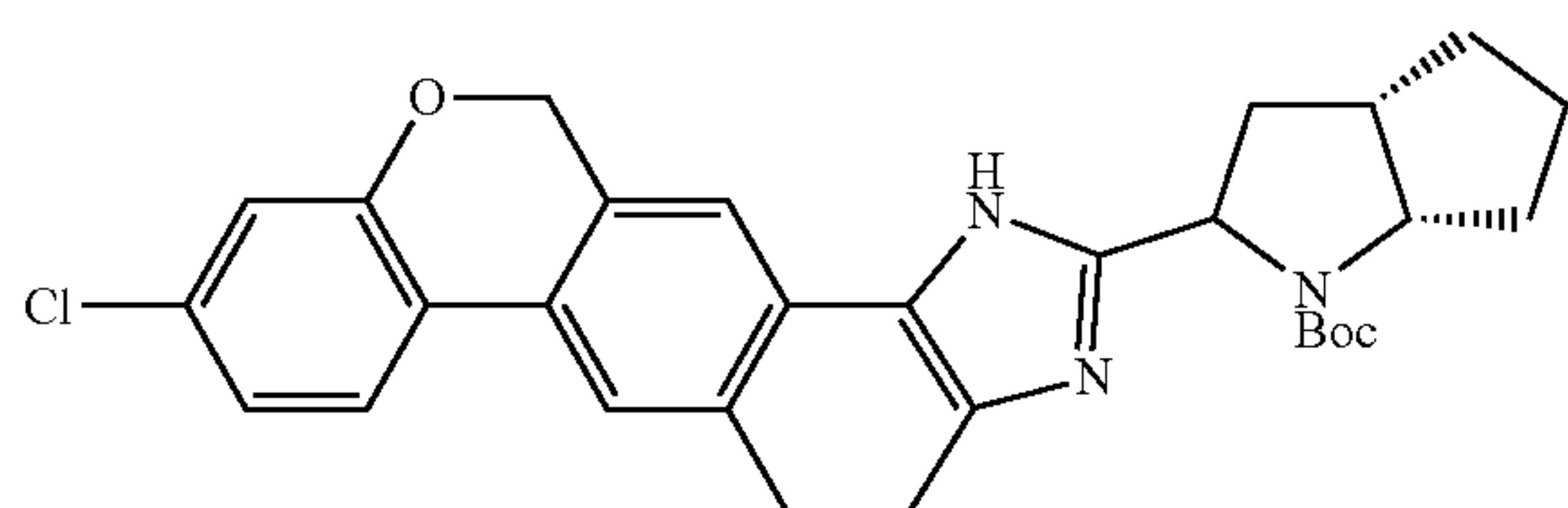
tert-butyl (3aS,6aS)-2-(9-chloro-1,4,5,12-tetrahydrochromeno[4',3':6,7]naphtho[1,2-d]imidazol-2-yl)hexahydrocyclopenta[b]pyrrole-1(2H)-carboxylate
