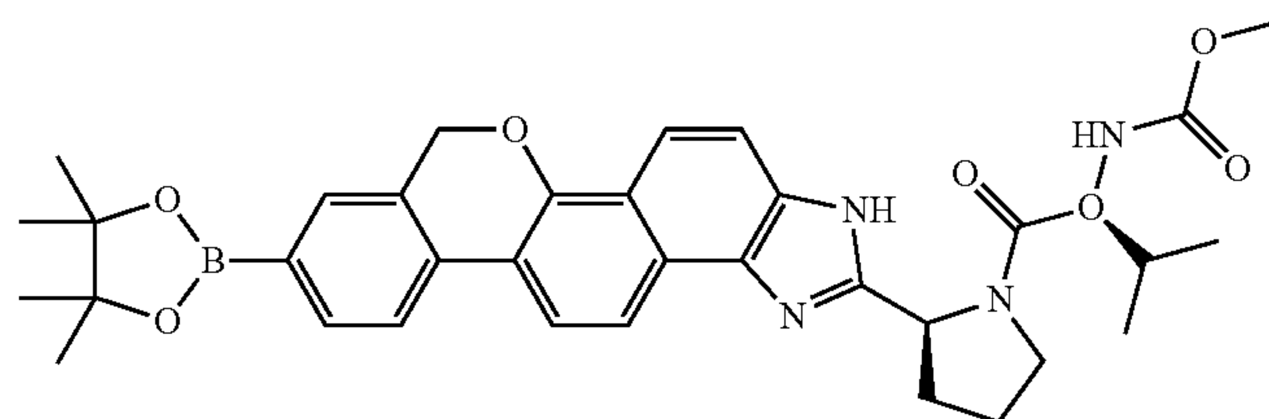
methyl[(2S)-3-methyl-1-oxo-1-((2S)-2-[9-(4,4,5,5-tetramethyl-1,3,2-dioxaborolan-2-yl)-3,11-dihydroisochromeno[4',3':6,7]naphtho[1,2-d]imidazol-2-yl]pyrrolidin-1-yl)butan-2-yl]carbamate
