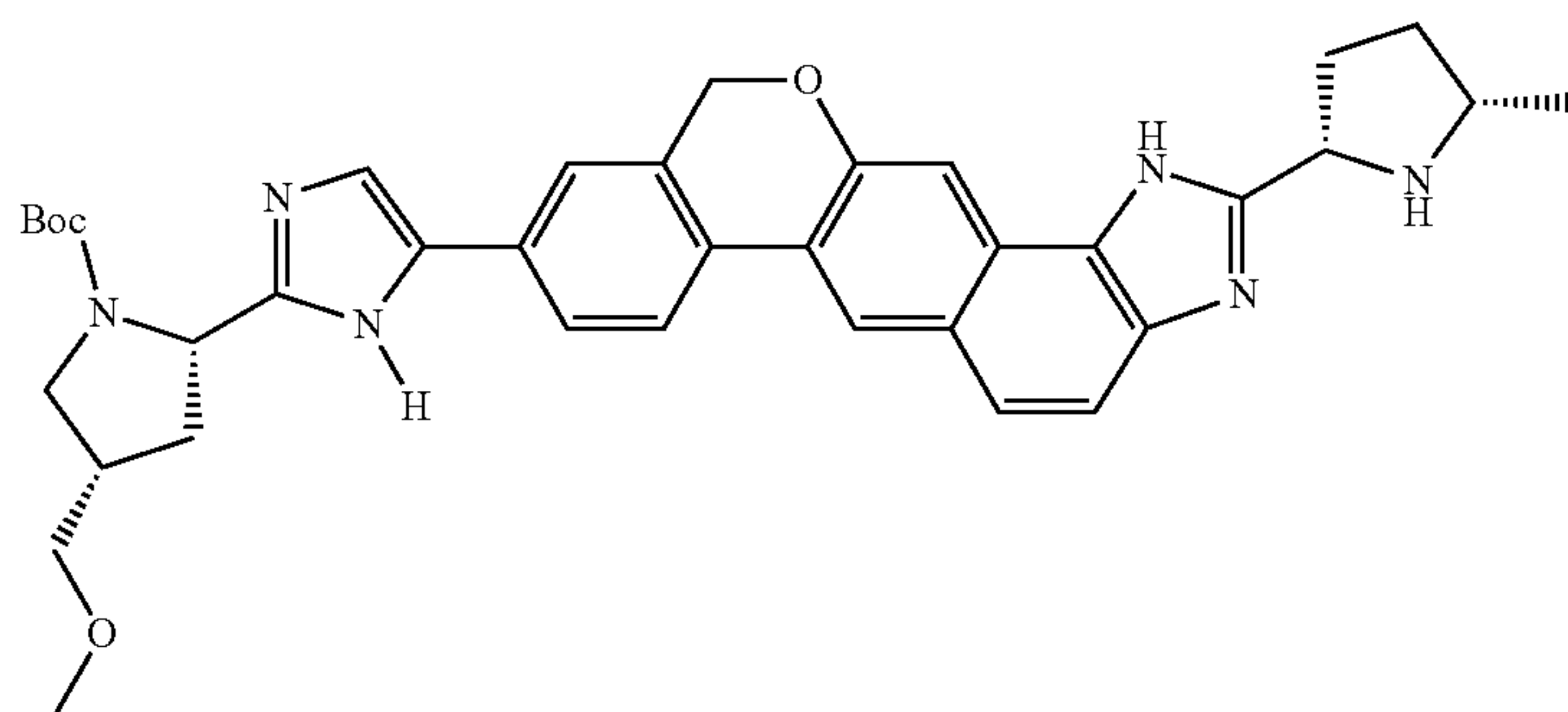
tert-butyl (2S,4S)-4-(methoxymethyl)-2-(5-{2-[(2S,5S)-5-methylpyrrolidin-2-yl]-1,11-dihydroisochromeno[4',3':6,7]naphtho[1,2-d]imidazol-9-yl}-1H-imidazol-2-yl)pyrrolidine-1-carboxylate
