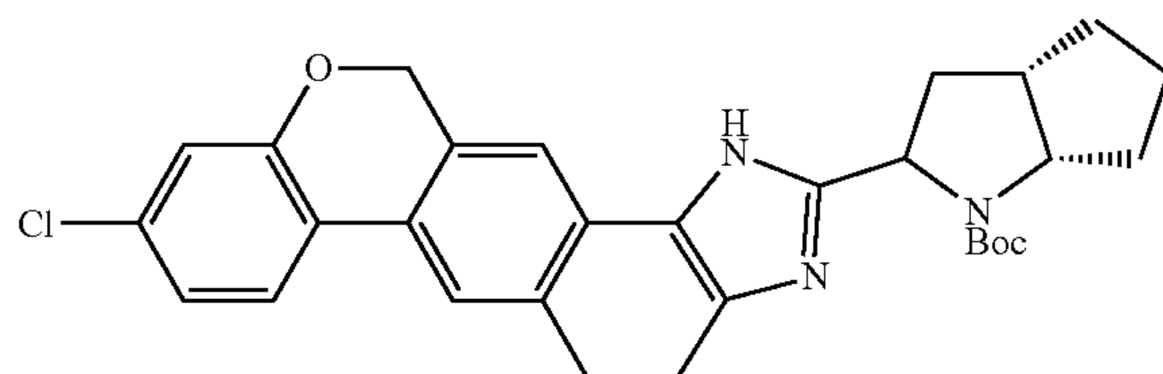
tert-butyl (3aS,6aS)-2-(9-chloro-1,4,5,12-tetrahydrochromeno[4',3':6,7]naphtho[1,2-d]imidazol-2-yl)hexahydrocyclopenta[b]pyrrole-1(2H)-carboxylate
