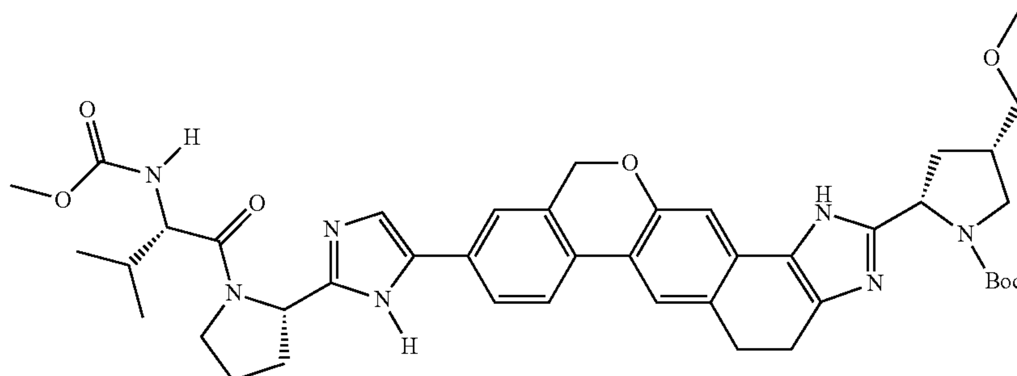
(2S,4S)-tert-butyl 2-(9-(2-((S)-1-((S)-2-(methoxycarbonylamino)-3-methylbutanoyl)pyrrolidin-2-yl)-1H-imidazol-5-yl)-4,5-dihydro-1,11-dihydroisochromeno[4',3':6,7]naphtho[1,2-d]imidazol-2-yl)-4-(methoxymethyl)pyrrolidine-1-carboxylate
