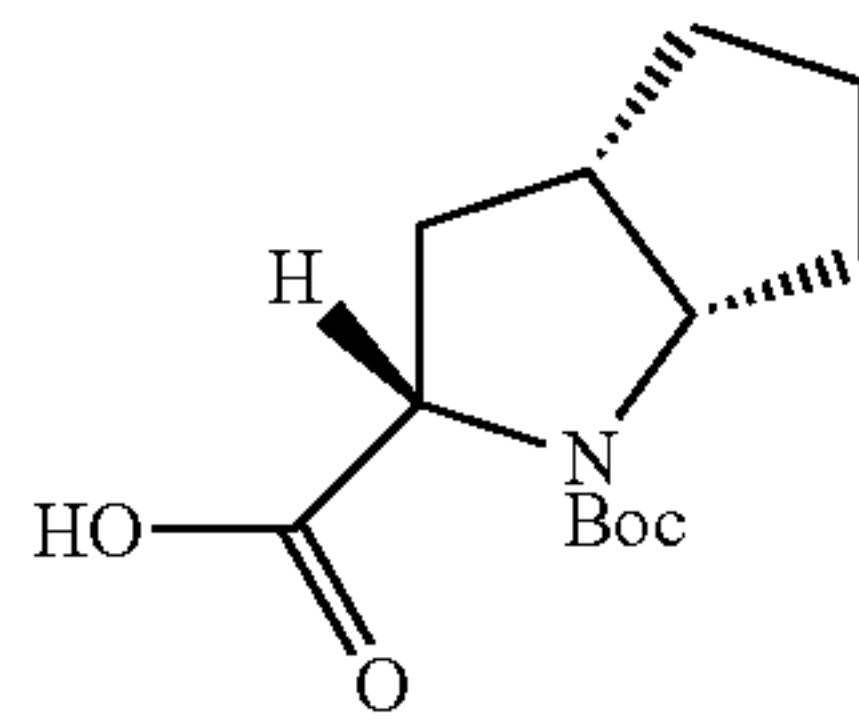
(2S,3aS,6aS)-1-(tert-butoxycarbonyl)octahydrocyclopenta[b]pyrrole-2-carboxylic acid
