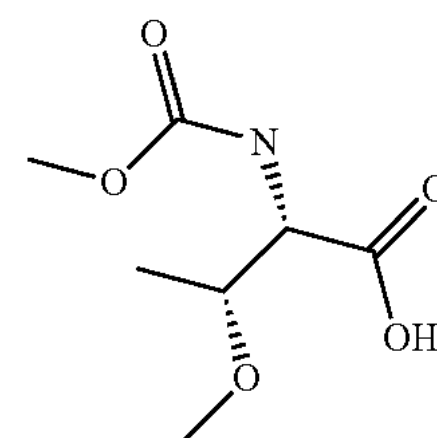
(2S,3R)-3-methoxy-2-(methoxycarbonylamino)butanoic acid
