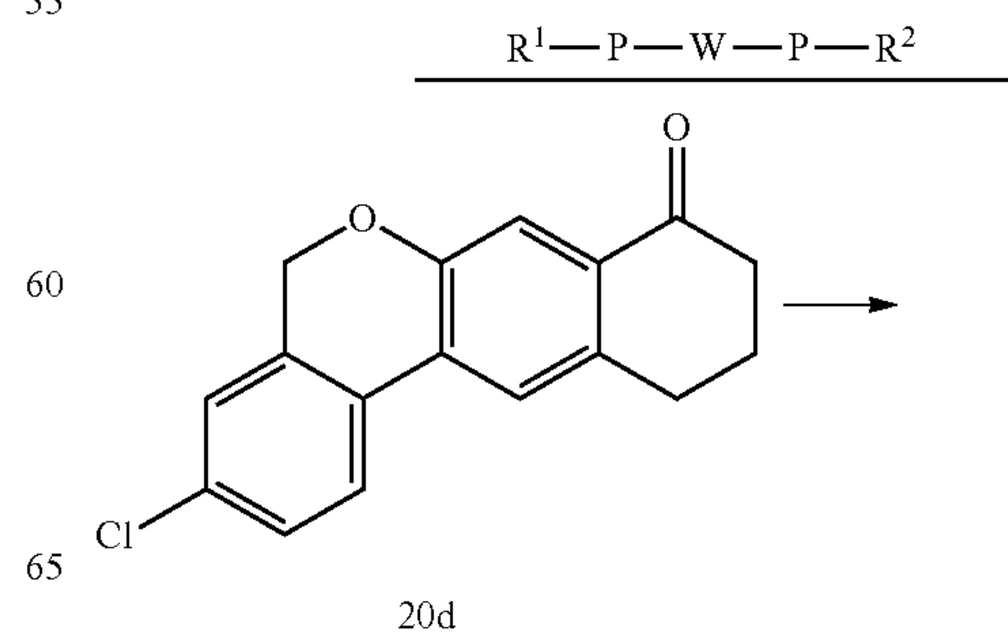
Scheme 21. Representative synthesis
