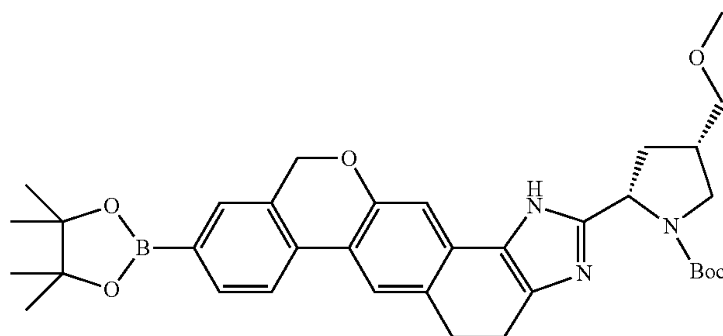
(2S,4S)-tert-butyl 4-(methoxymethyl)-2-(9-(4,4,5,5-tetramethyl-1,3,2-dioxaborolan-2-yl)-4,5-dihydro-1,11-dihydroisochromeno[4',3':6,7]naphtho[1,2-d]imidazol-2-yl)pyrrolidine-1-carboxylate
