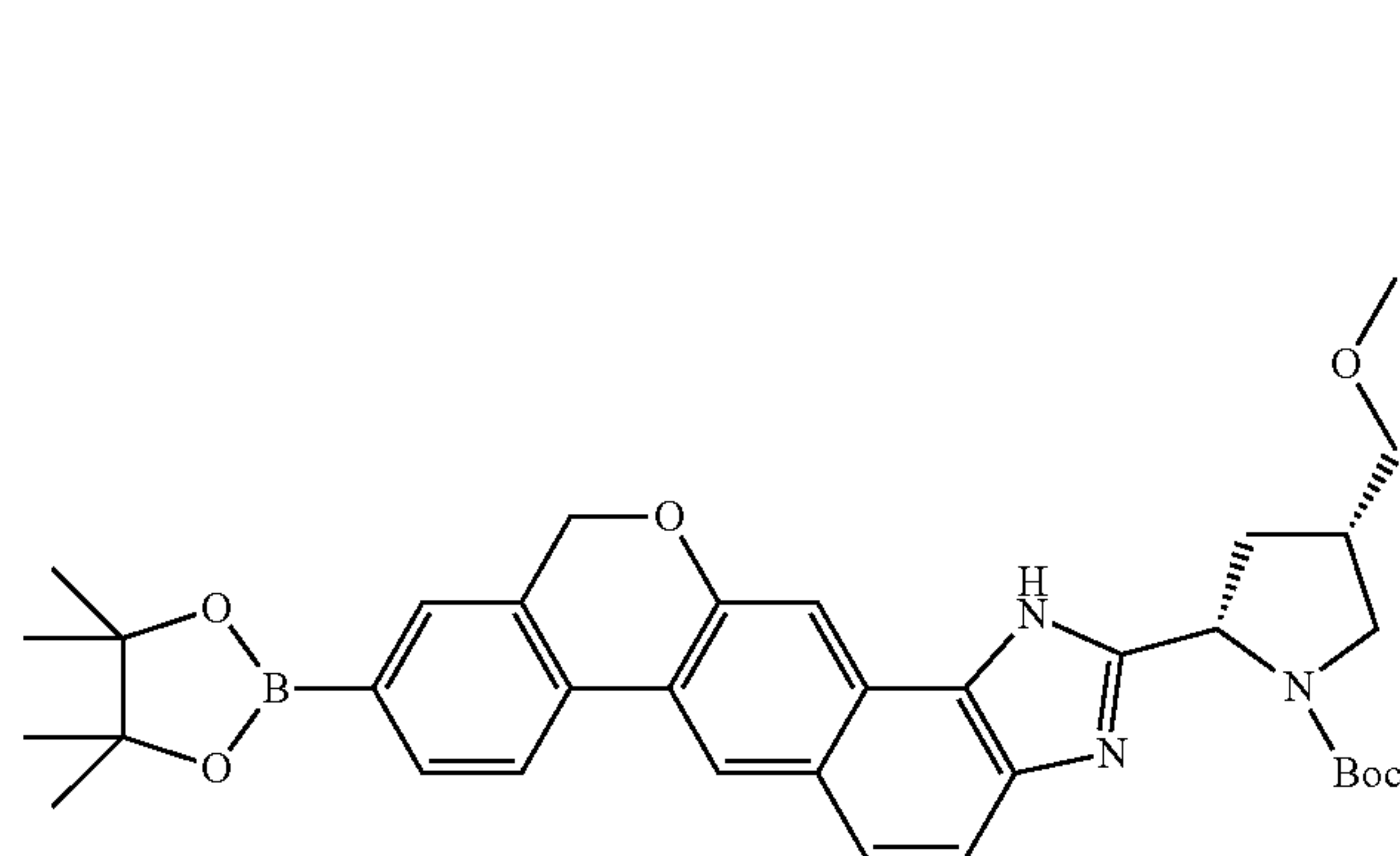
(2S,4S)-tert-butyl 4-(methoxymethyl)-2-(9-(4,4,5,5-tetramethyl-1,3,2-dioxaborolan-2-yl)-1,11-dihydroisochromeno[4',3':6,7]naphtho[1,2-d]imidazol-2-yl)pyrrolidine-1-carboxylate
