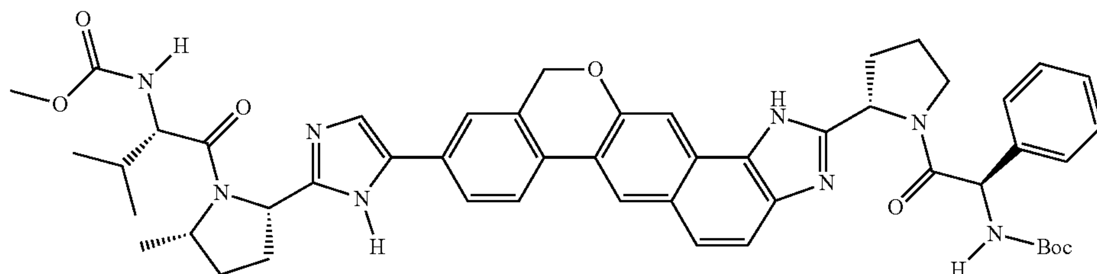
methyl {(2S)-1-[(2S,5S)-2-(5-{2-[(2S)-1-[(2R)-2-[(tert-butoxycarbonyl)amino]-2-phenylacetyl]pyrrolidin-2-yl]-3,11-dihydroisochromeno[4',3':6,7]naphtho[1,2-d]imidazol-9-yl}-1H-imidazol-2-yl)-5-methylpyrrolidin-1-yl]-3-methyl-1-oxobutan-2-yl}carbamate
