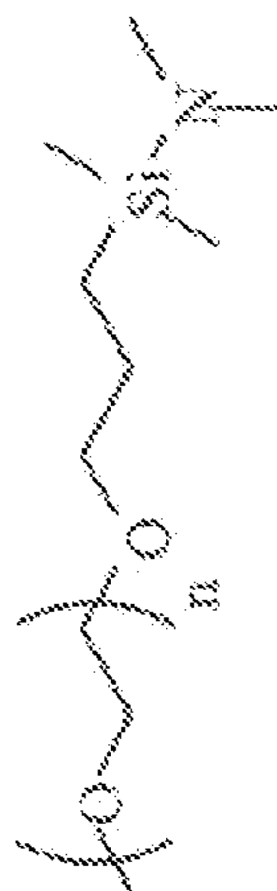
2-[Methoxy(polyethyleneoxy)propyl] dimethylaminodimethylsilane
