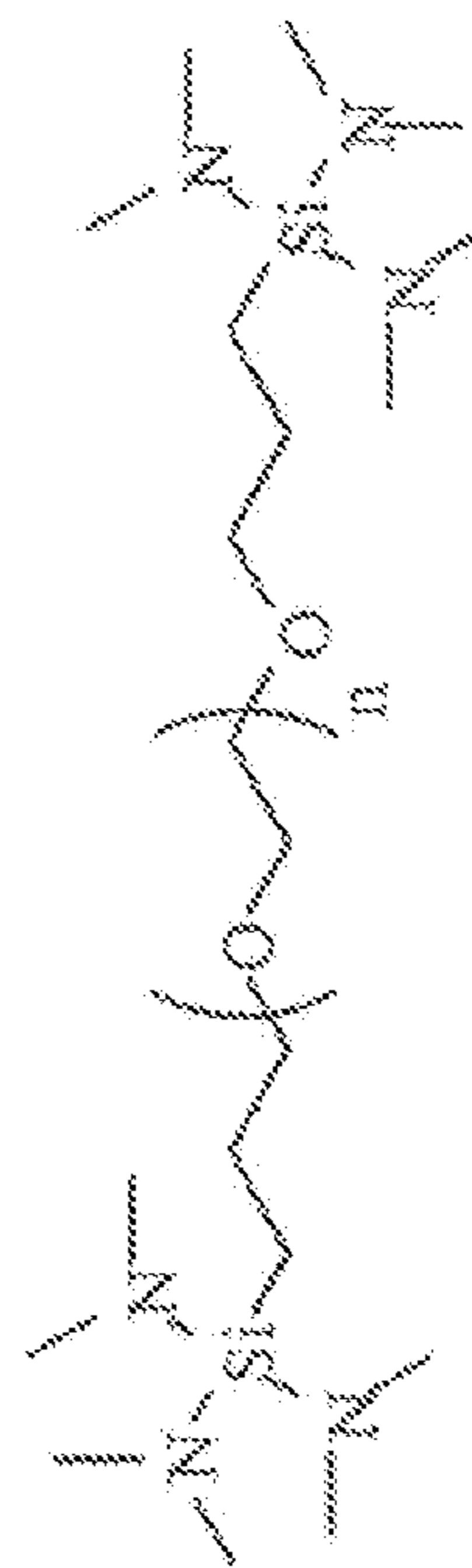
Bis[3-tris(dimethylamino)silylpropyl]polyethyleneoxide
