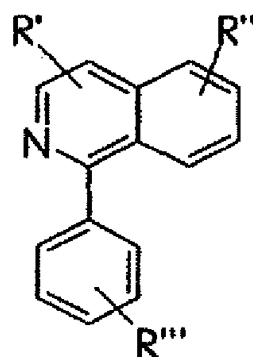
arylquinolines
