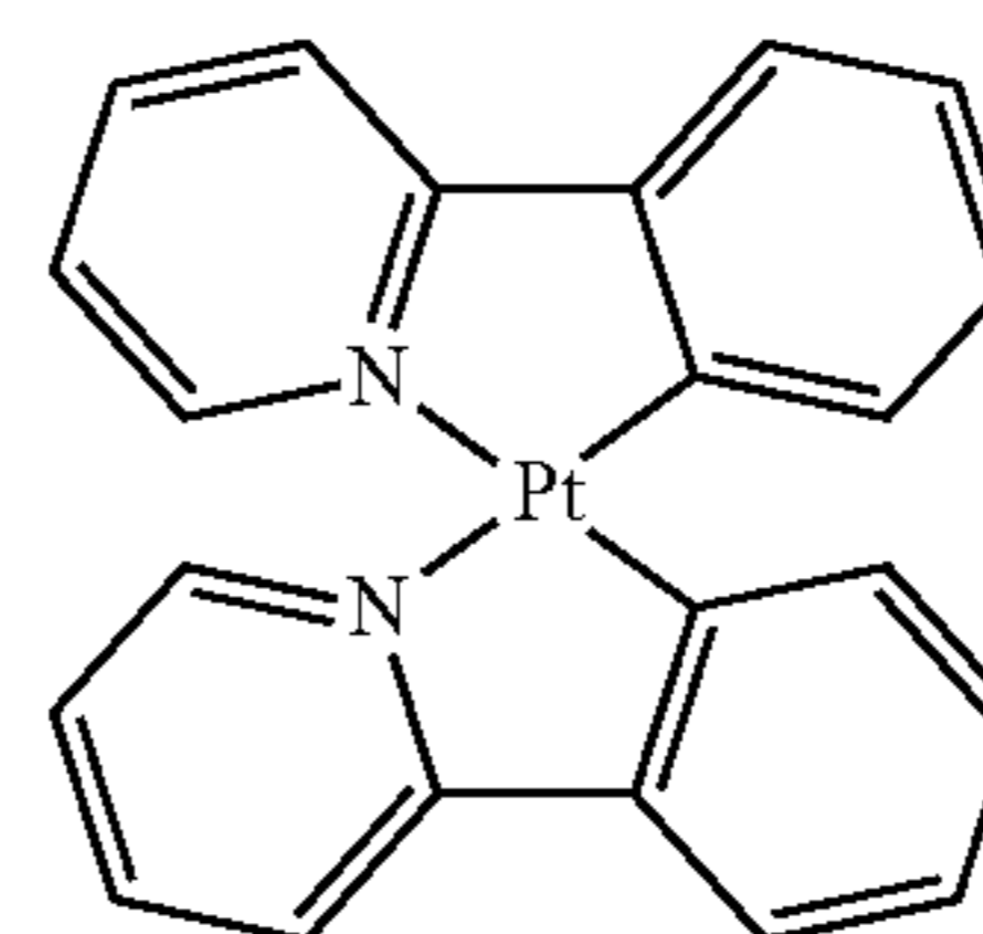
cis-Bis[2-(2-phenyl)pyridinato-N,C 2 ]Pt (II) Pt(Phpy) 2 (1)
