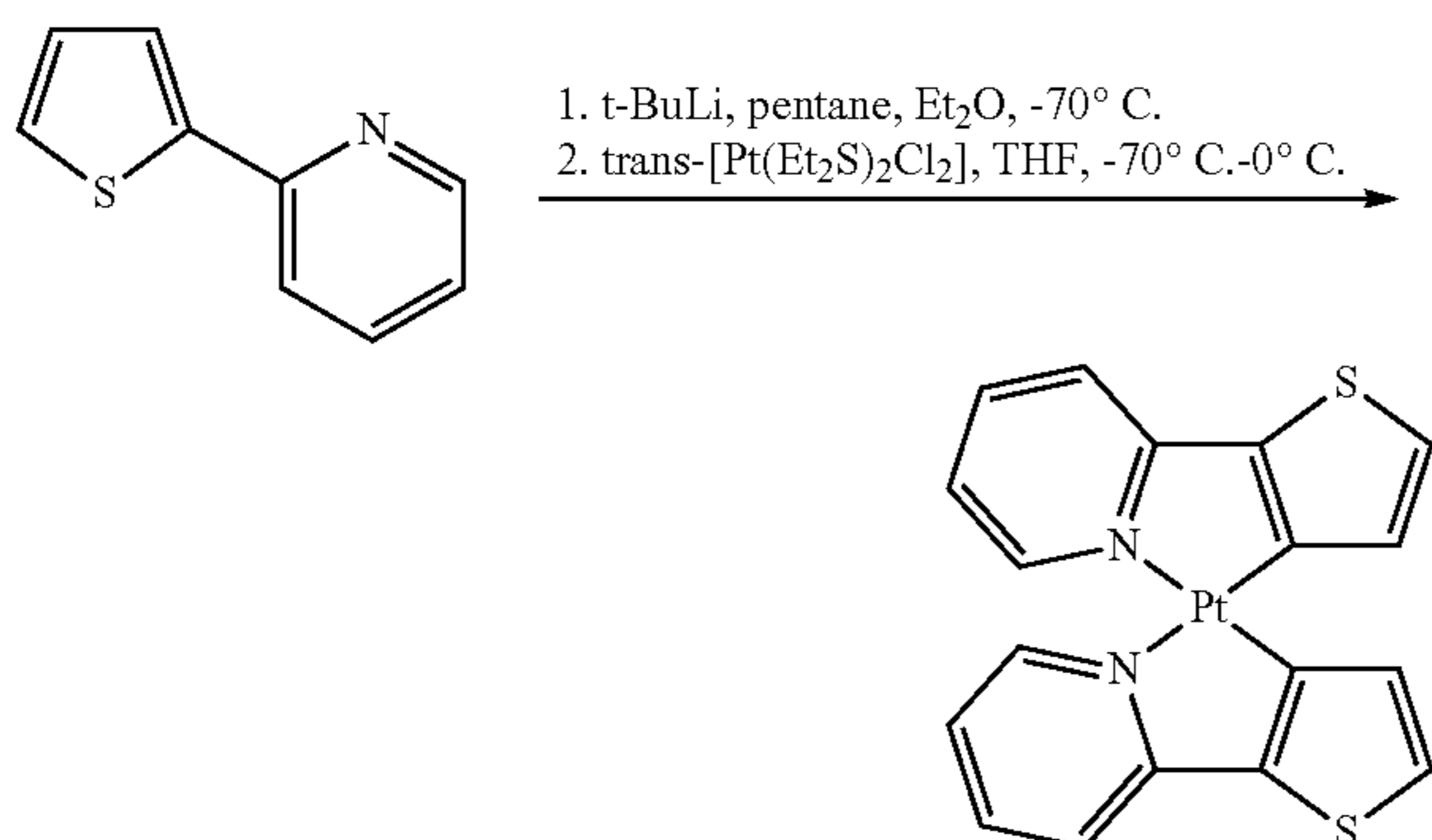
Scheme 9: Synthesis of cis-bis[2-(2'-thienyl)pyridinato-N,C 3 ] platinum (II).
