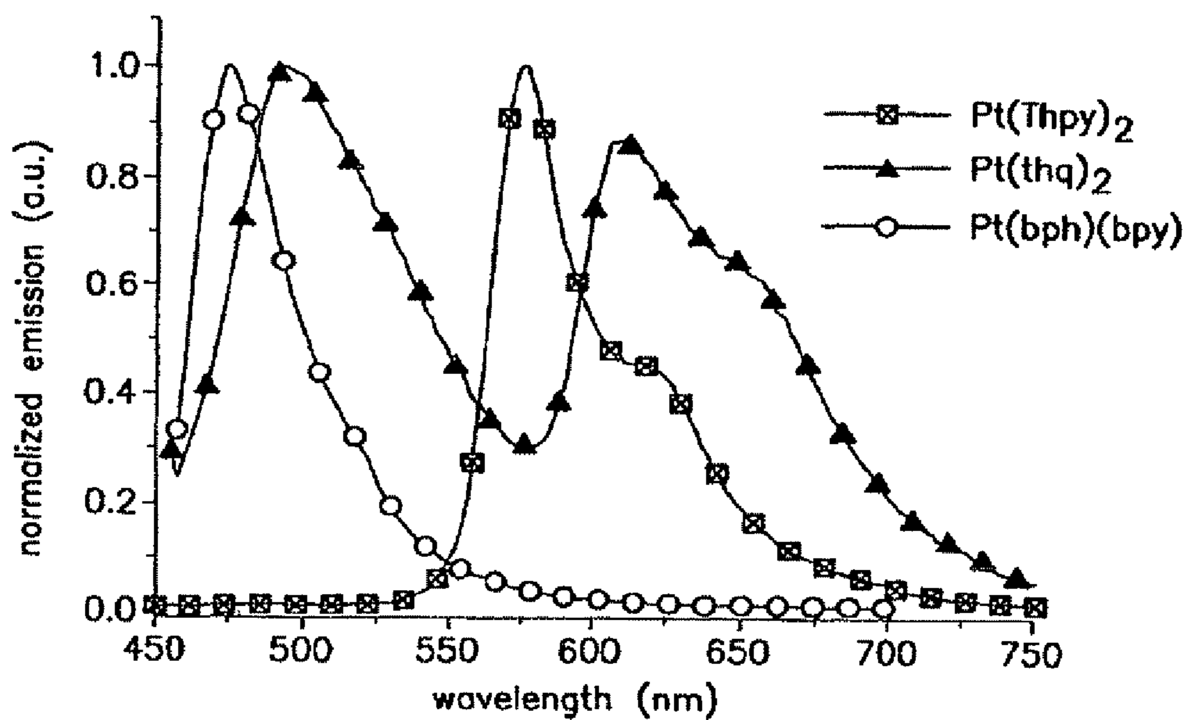
Emission spectra of the complexes.
