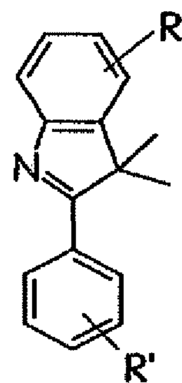
phenylindoles
