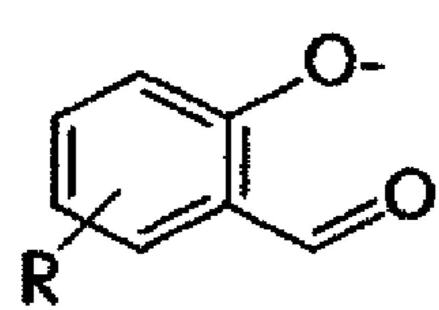
salicylaldehydes
