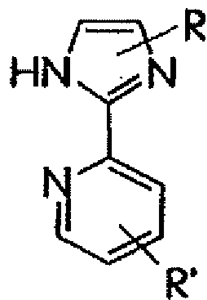
pyridylimidazoles
