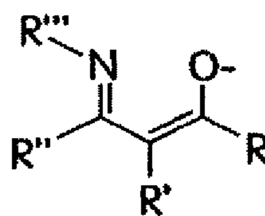
iminoacetates
