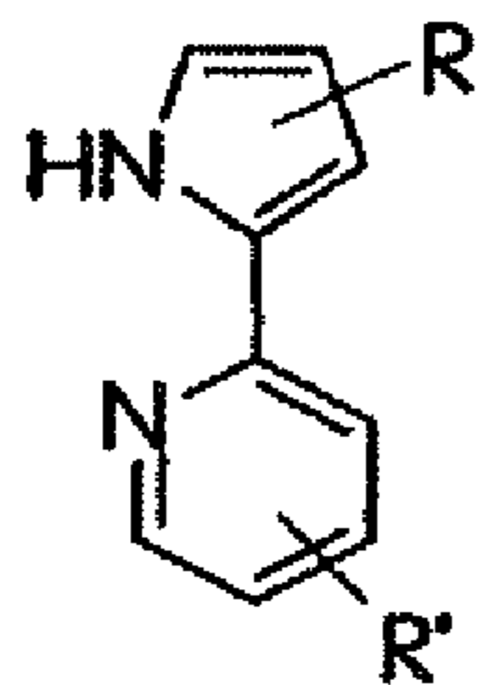
pyridylpyroles
