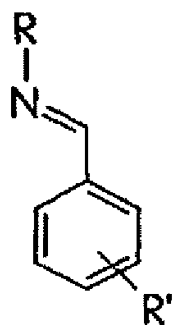
phenylimines
