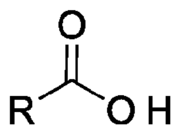
Carboxylic acids
