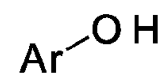
aryl alcohols
