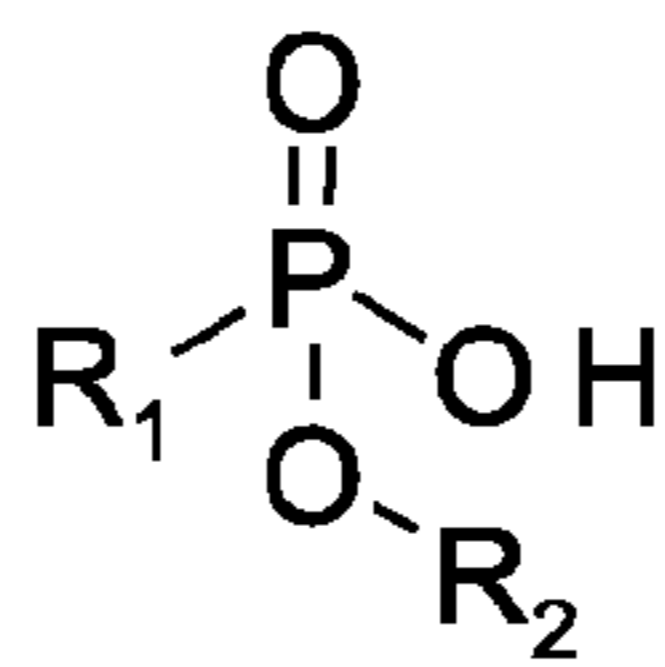
monoalkylphosphonates
