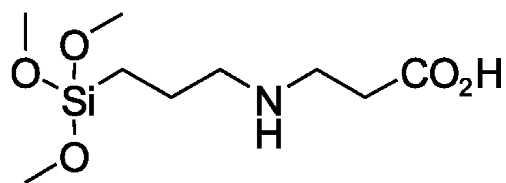
3-(3-(trimethoxysilyl)propylamino)propanoic acid
