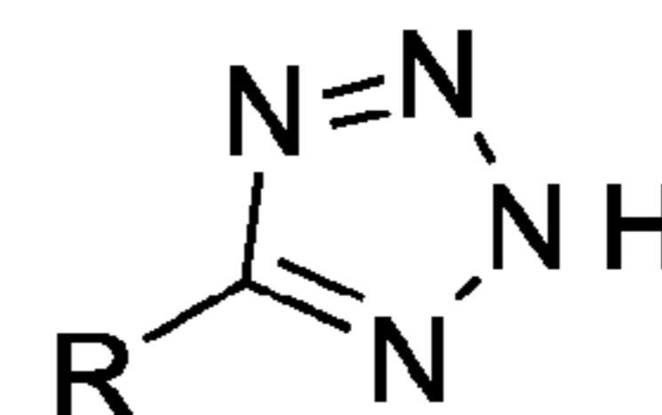
tetrazoles
