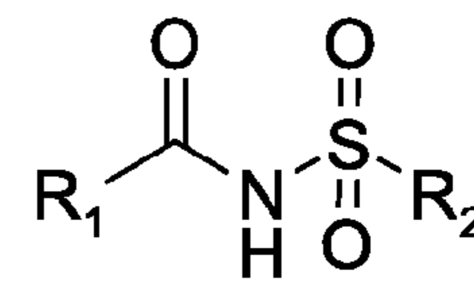
N-acylsulfonamides
