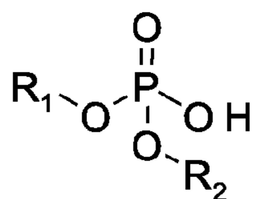
dialkylphosphates
