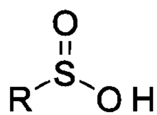
sulfinic acids
