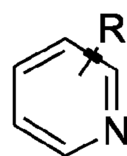
pyridines
