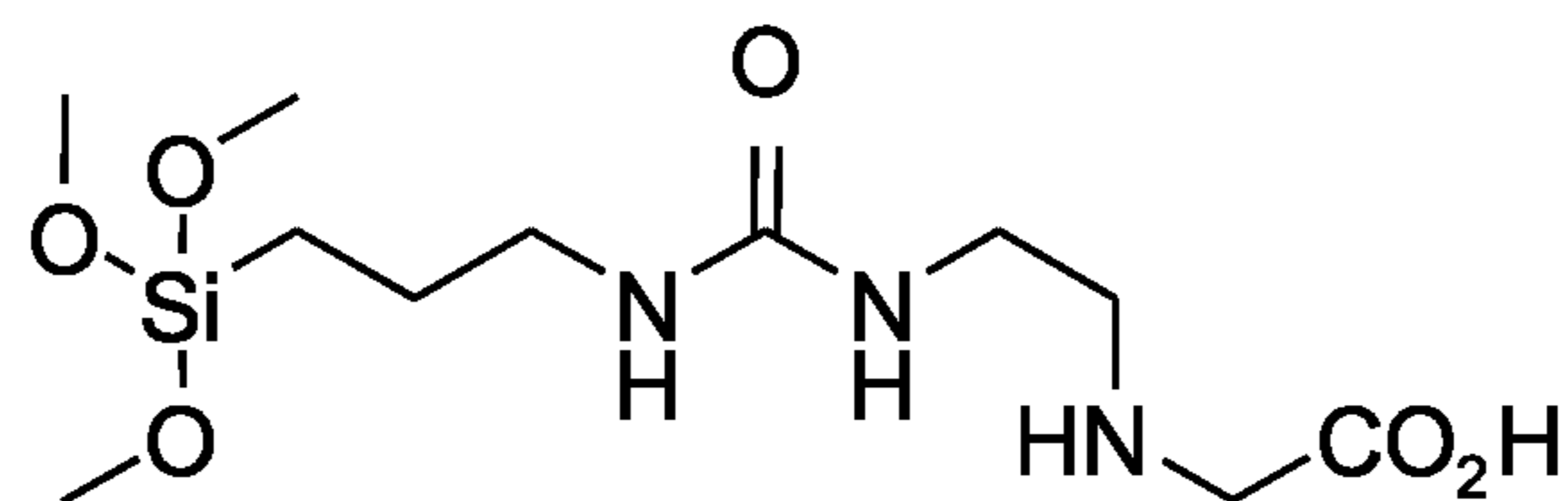
2-(2-(3-(trimethoxysilyl)propylureido)ethyl)aminoacetic acid
