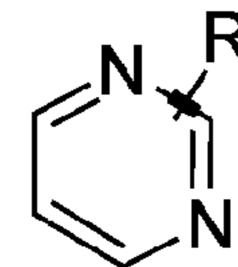
pyrimidines
