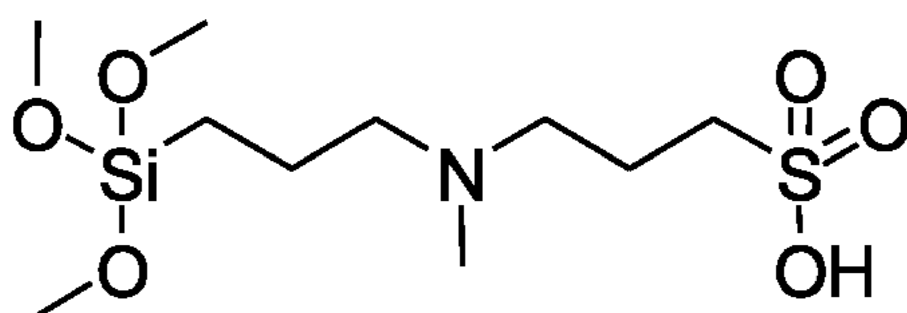
3-(methyl(3-(trimethoxysilyl)propyl)amino)propane-1-sulfonic acid
