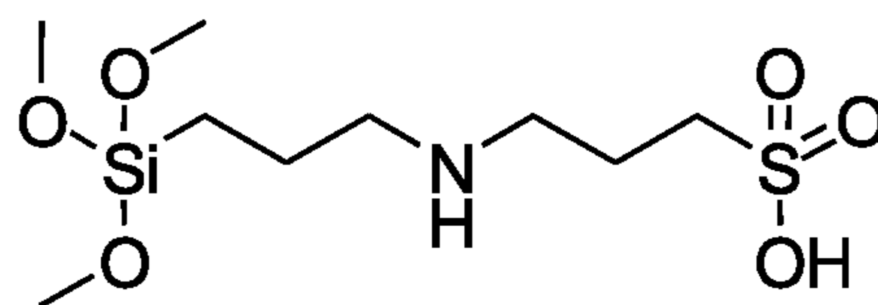
3-(3-(trimethoxysilyl)propylamino)propane-1-sulfonic acid
