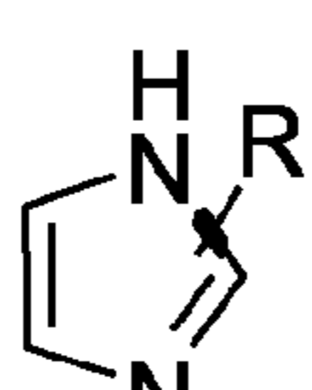
imidazoles
