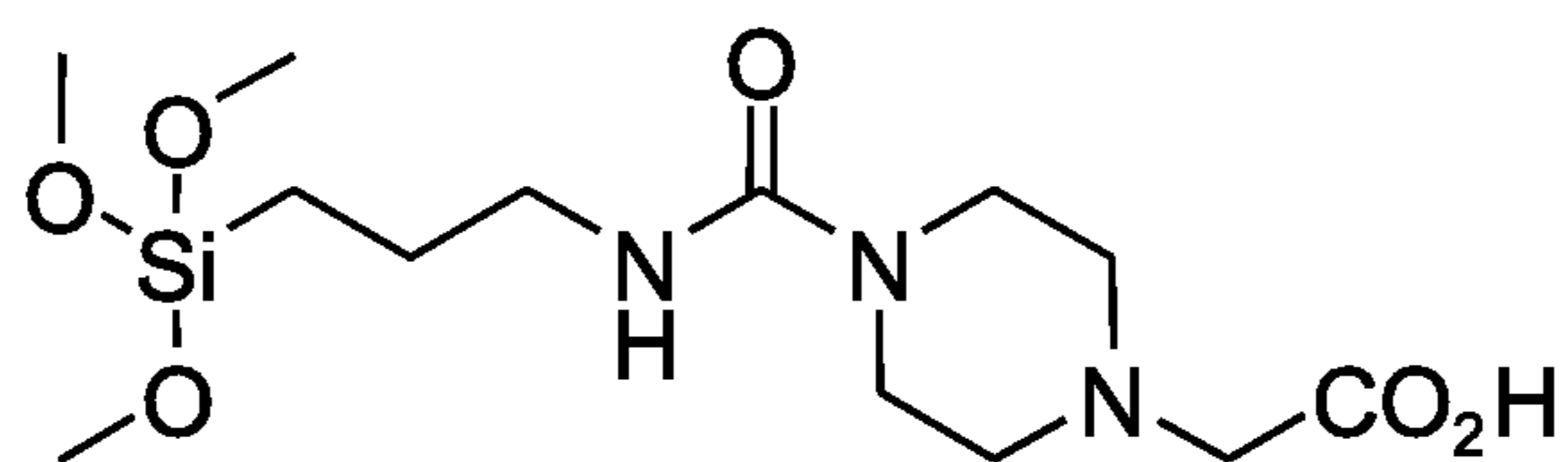
2-(4-(3-(trimethoxysilyl)propylcarbamoyl)piperazin-1-yl)acetic acid
