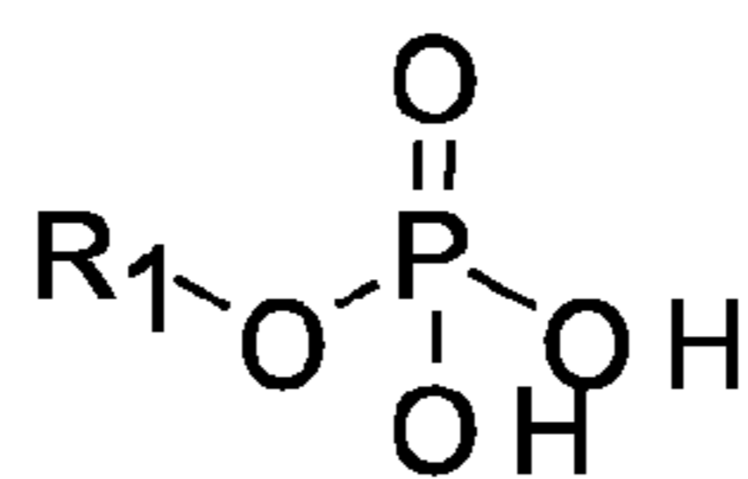
monoalkylphosphates
