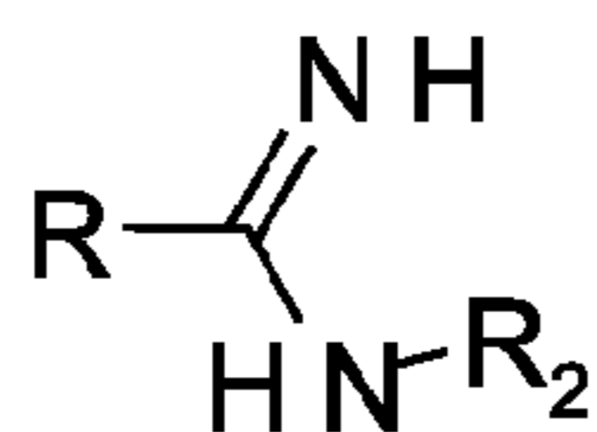
amidines
