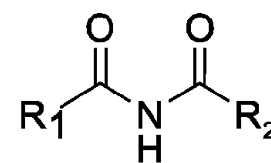
imides
