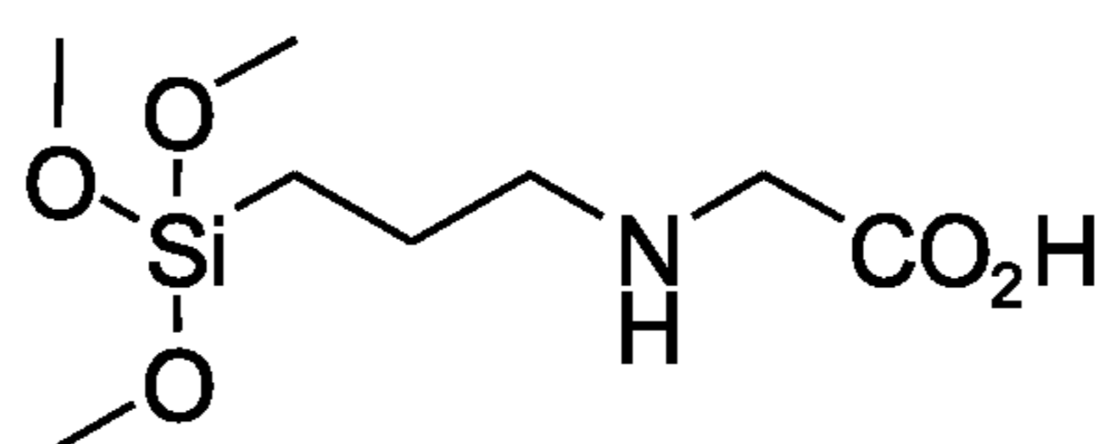
2-(3-(trimethoxysilyl)propylamino)acetic acid
