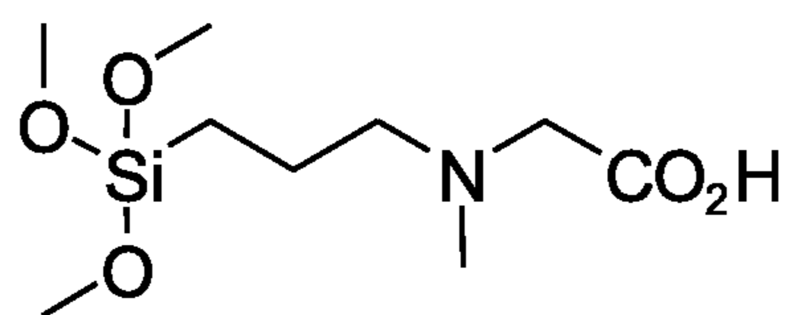
2-(methyl(3-(trimethoxysilyl)propyl)amino)acetic acid
