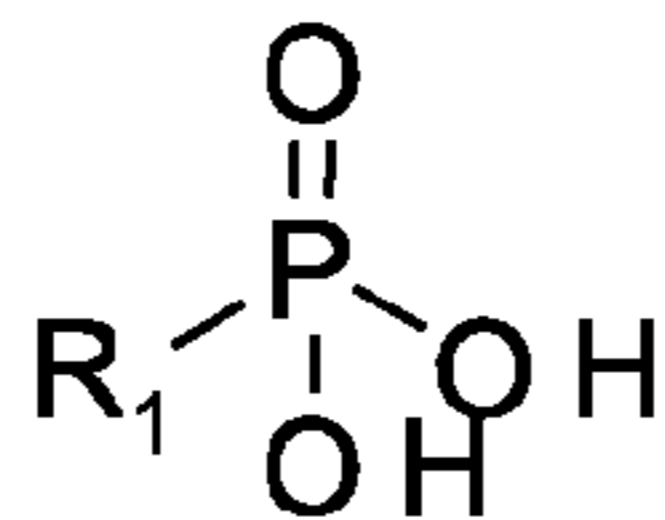
phosphonic acids
