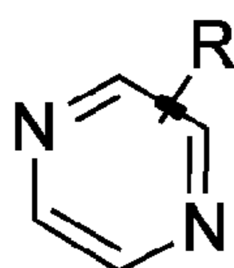
pyrazines
