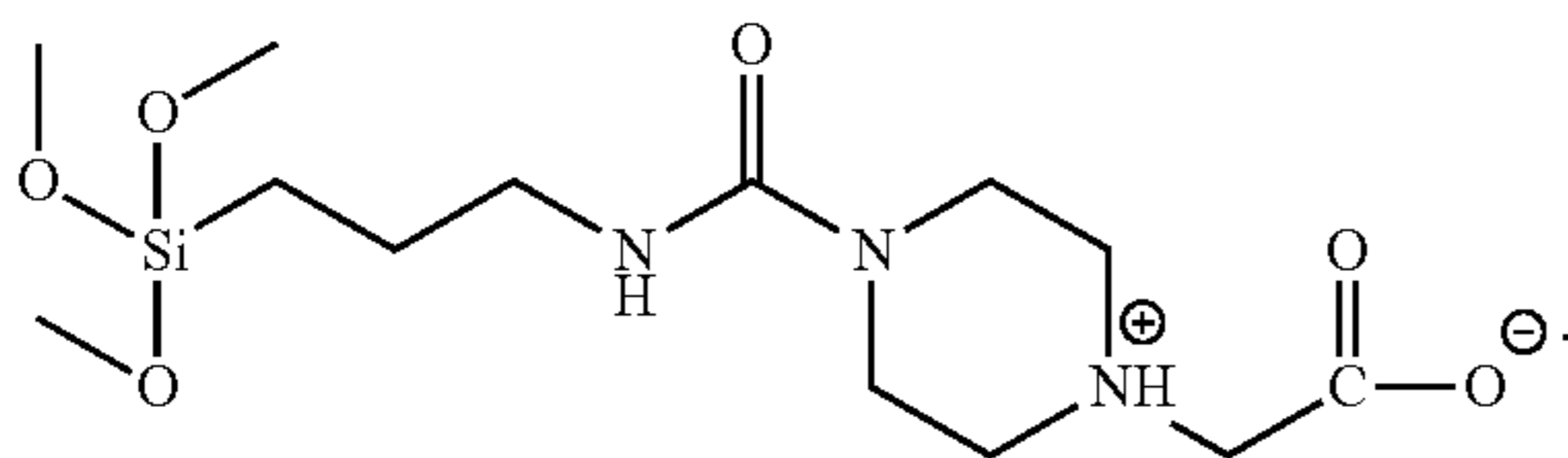
Structure II
