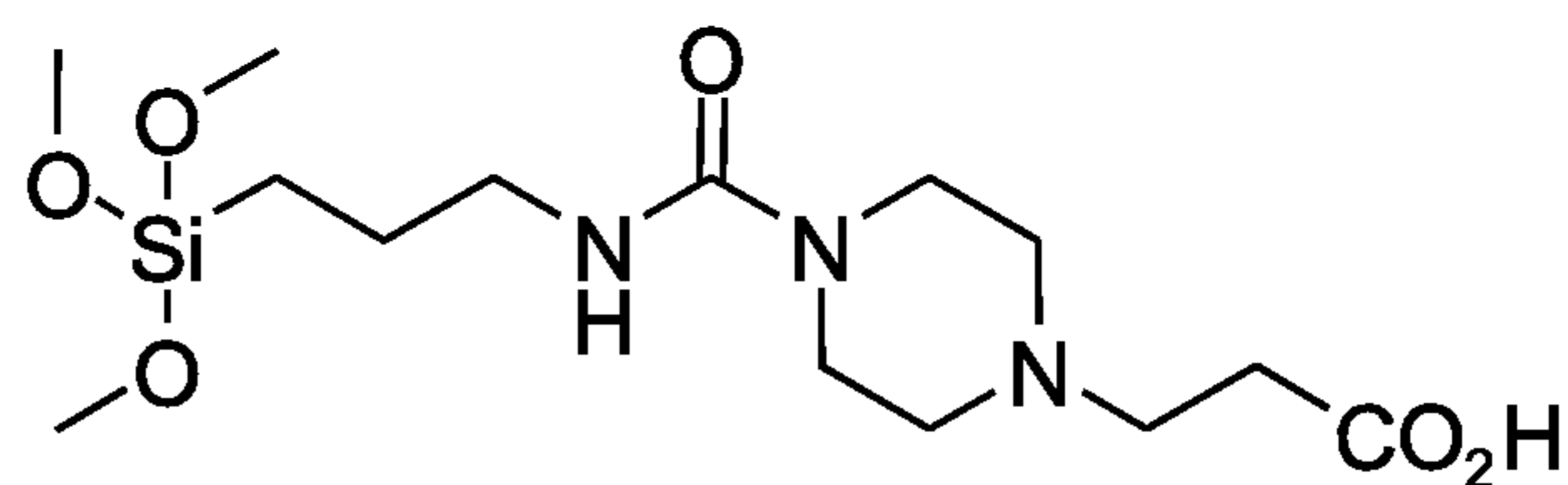
3-(4-(3-(trimethoxysilyl)propylcarbamoyl)piperazin-1-yl)propanoic acid
