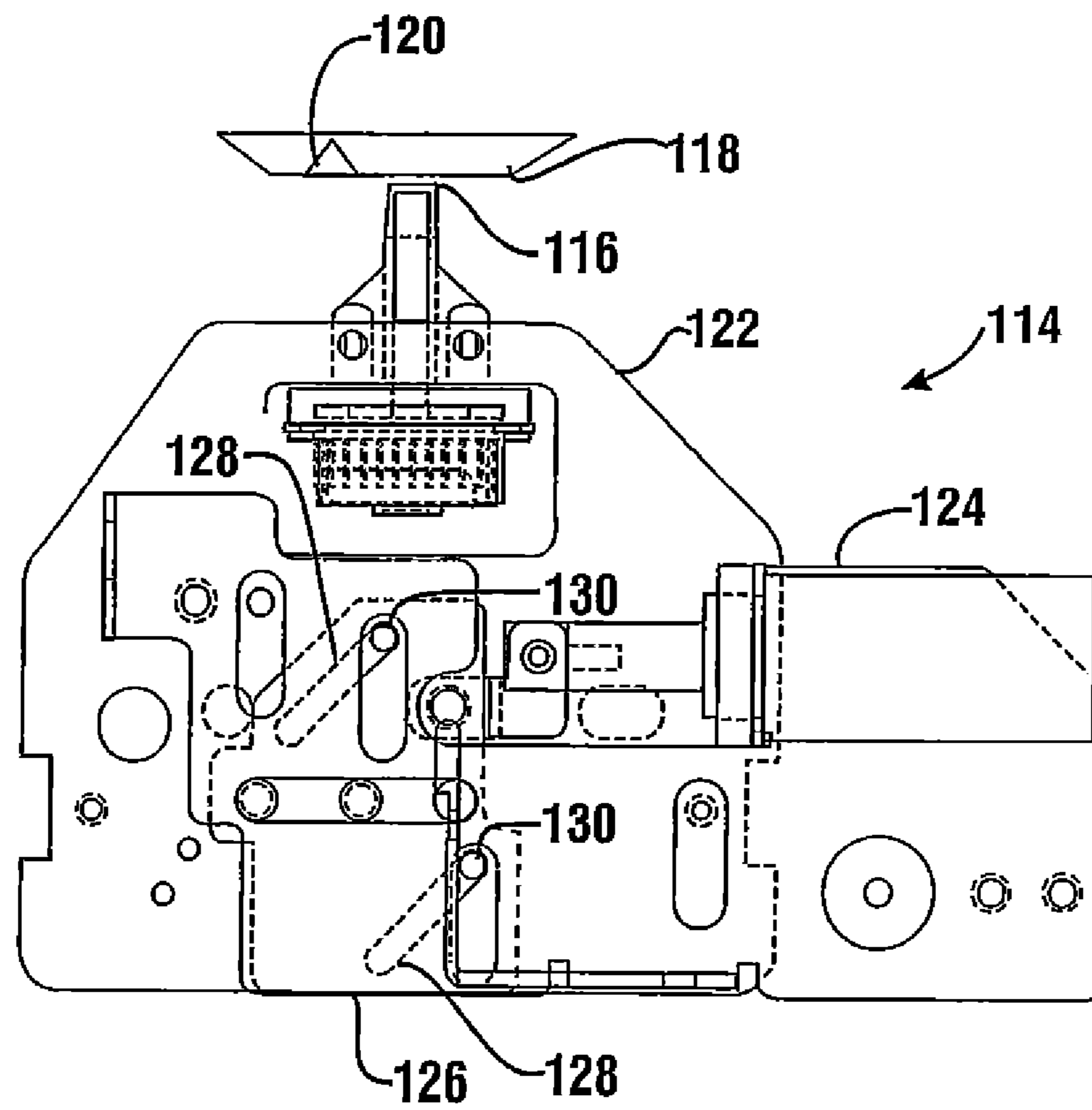
Printing Position
