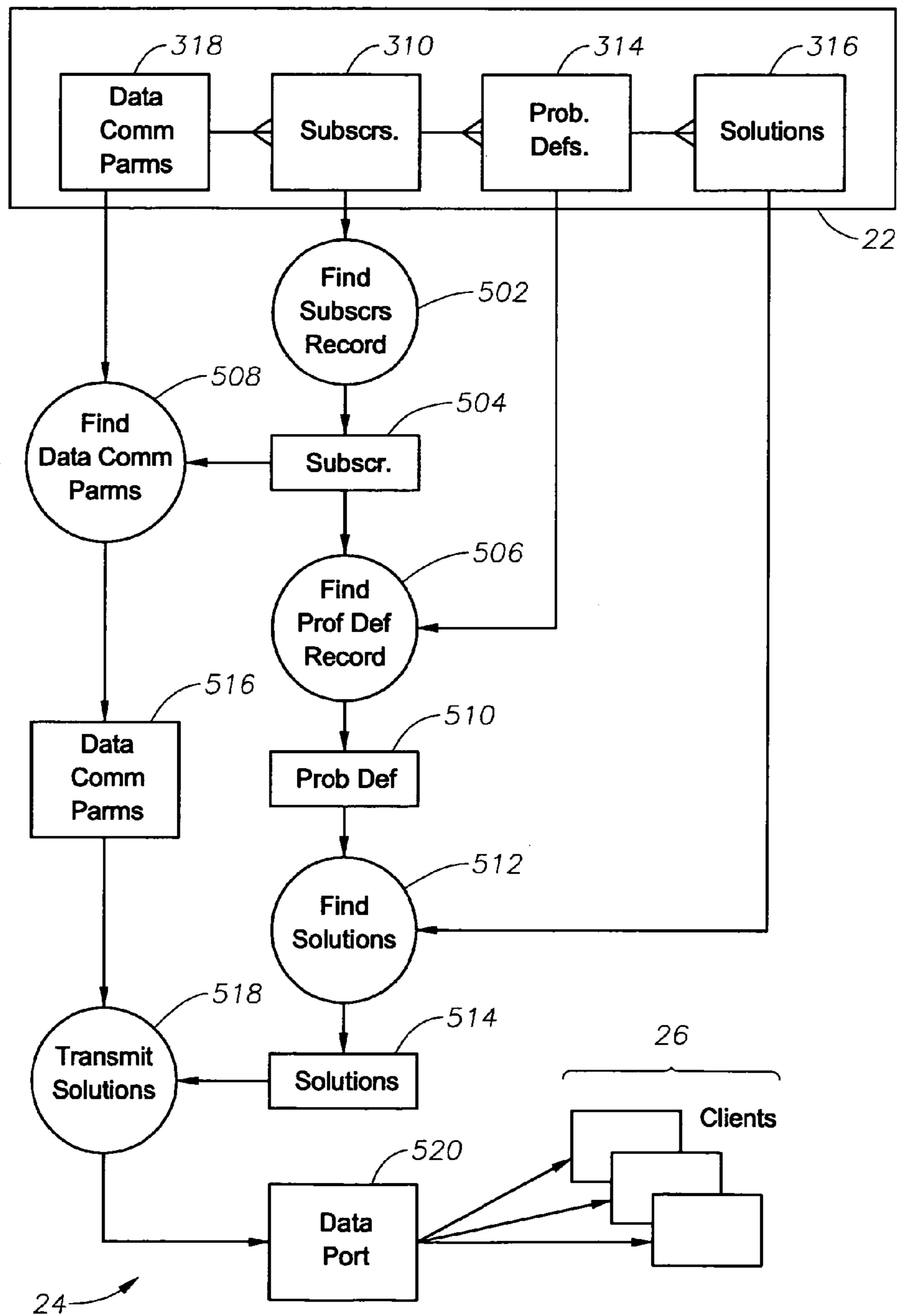
Solution Retrieval and Transmission
