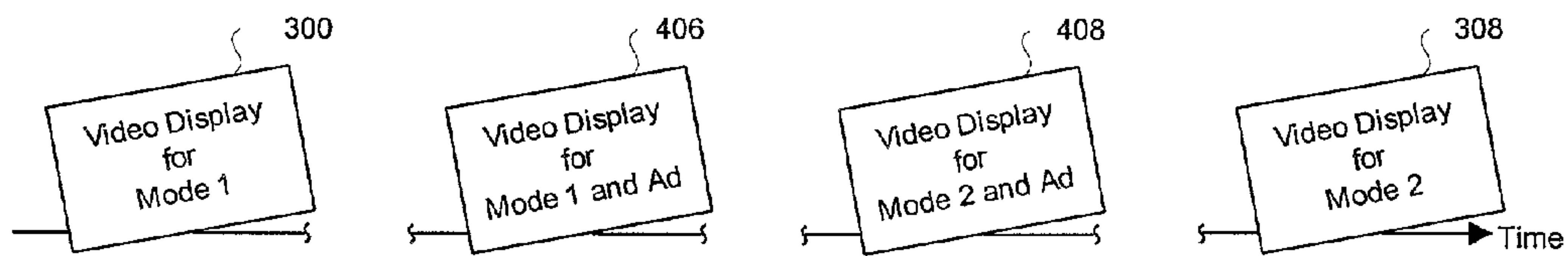
Fig. 4(e) - Video Output Stream with Overlap
