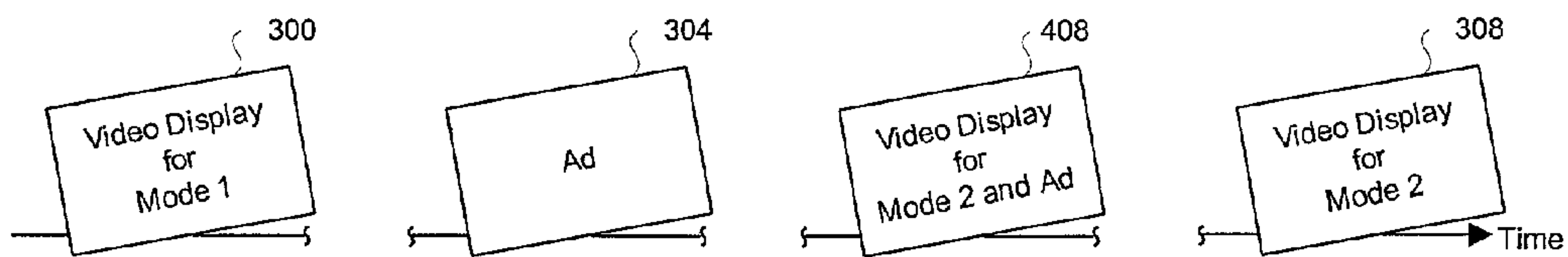
Fig. 4(c) - Video Output Stream with Overlap
