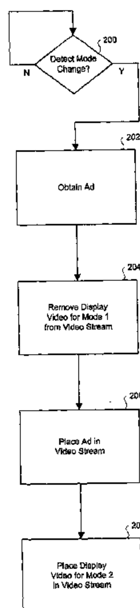
Ad Placement Flow Chart
