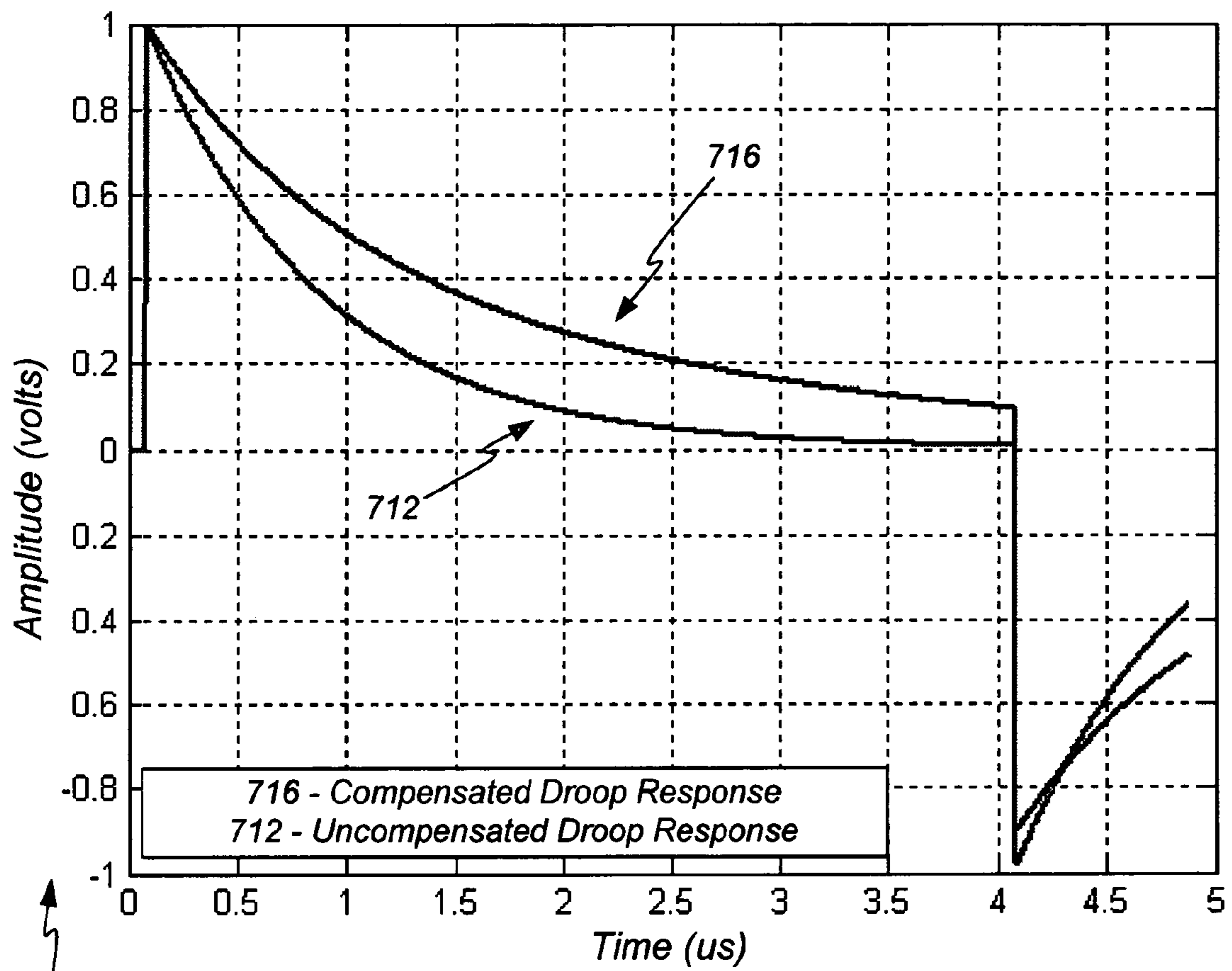
Example of Transmitter Droop Response
