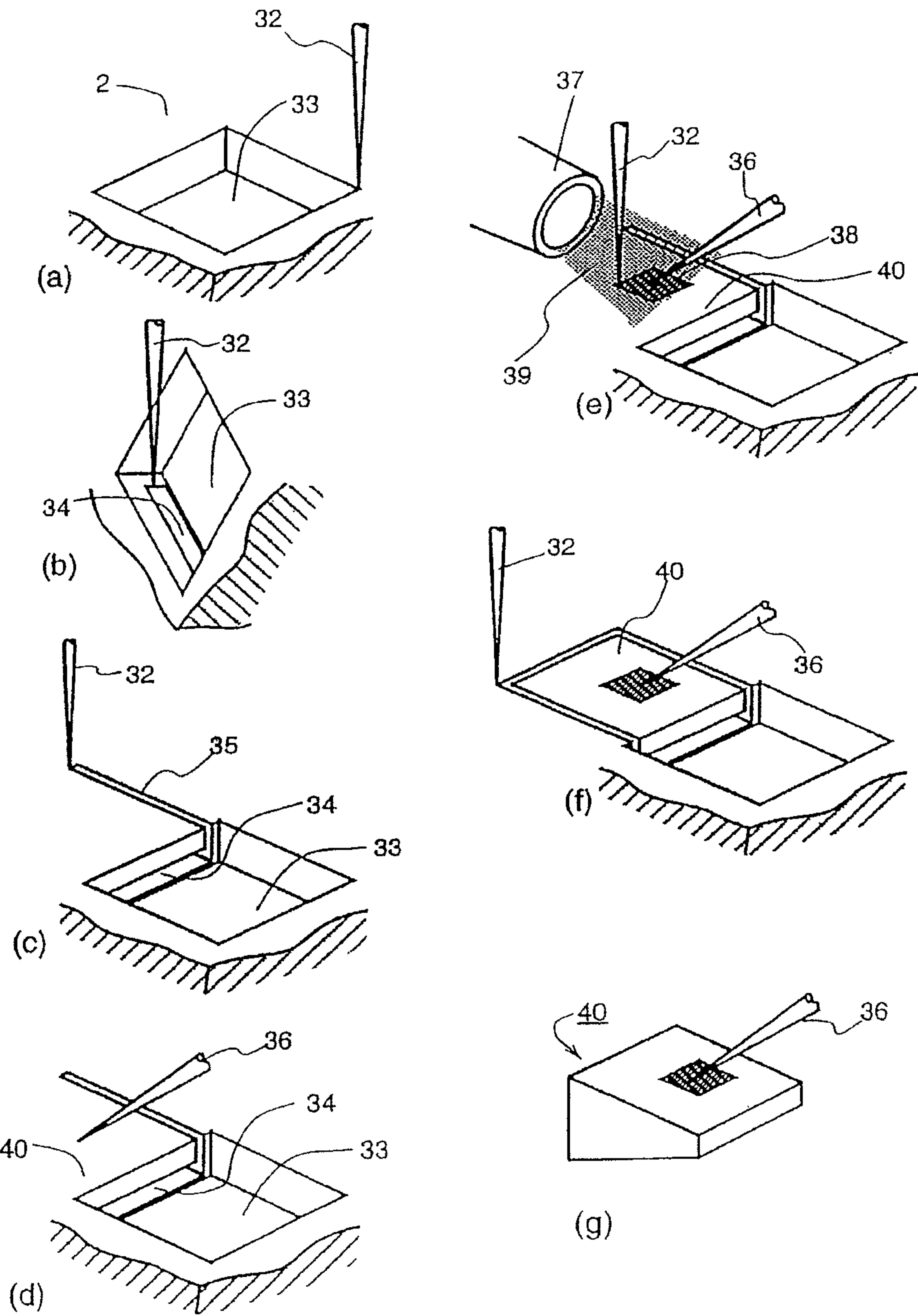
FIG.4 (PRIOR ART)
