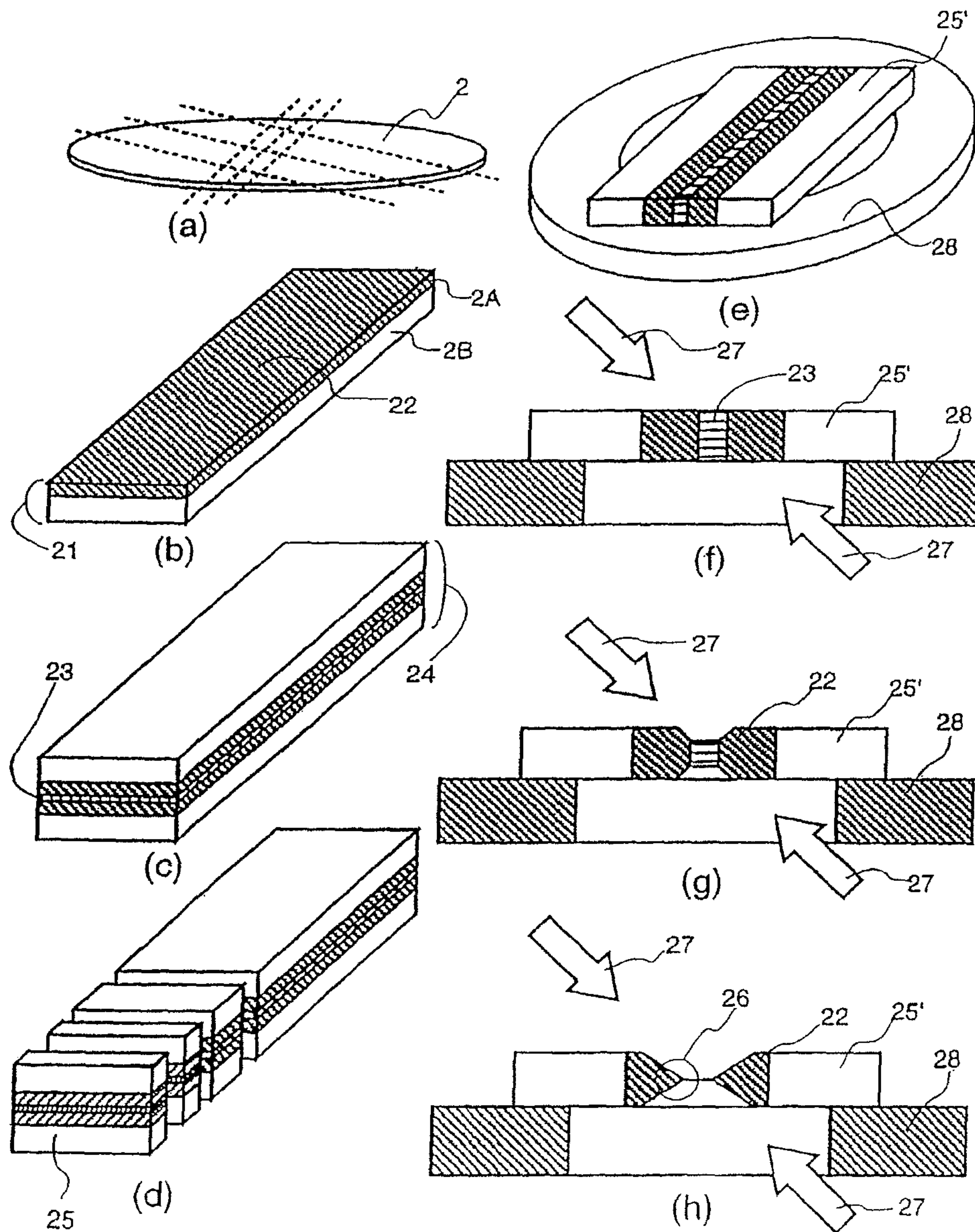
FIG.2 (PRIOR ART)
