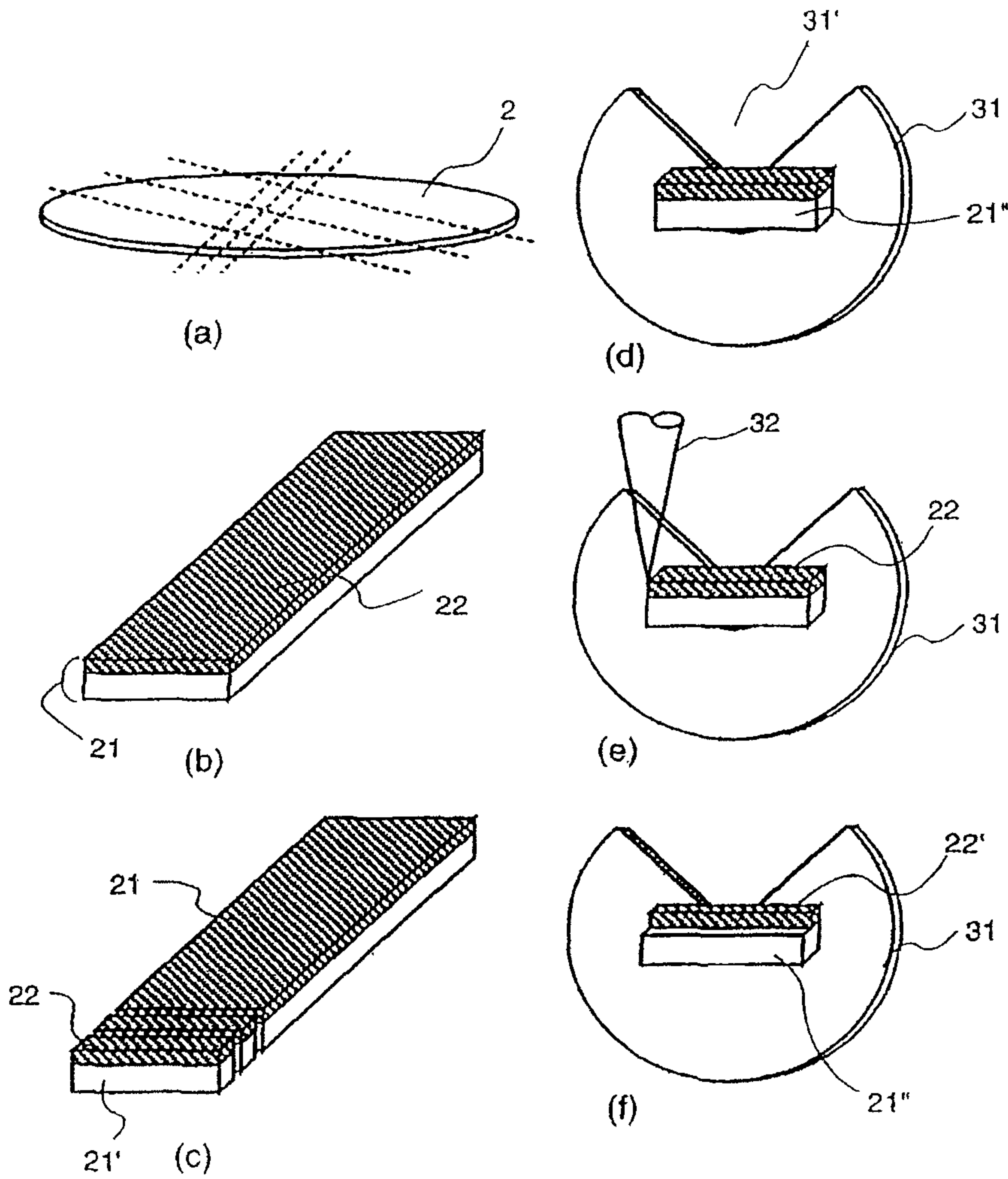
FIG.3 (PRIOR ART)
