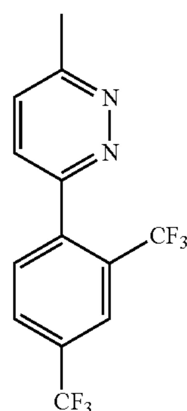
Compound 2a
