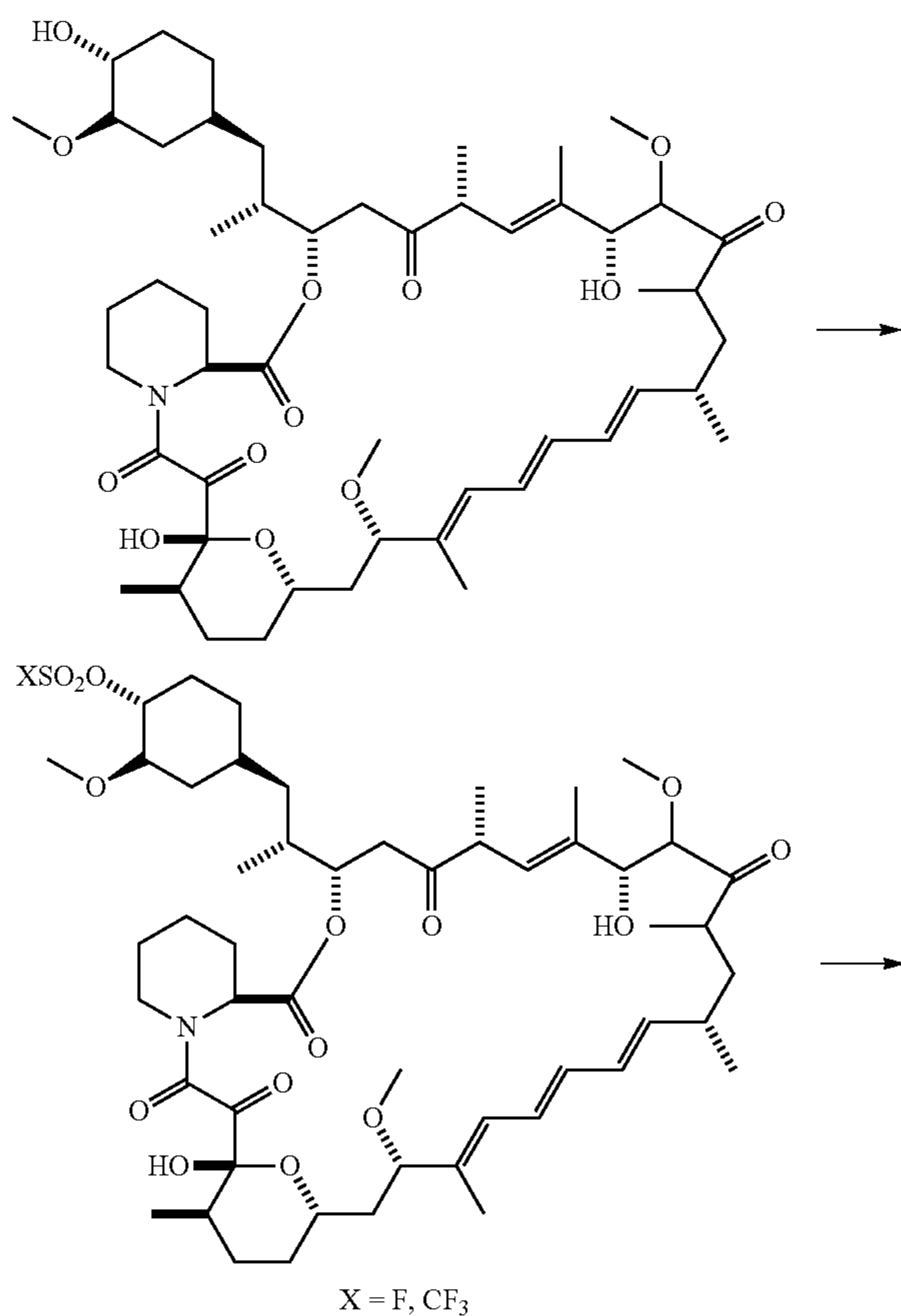
Scheme 1
