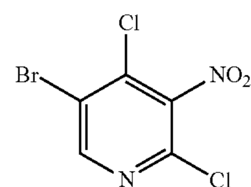
5-Bromo-2,4-dichloro-3-nitropyridine
