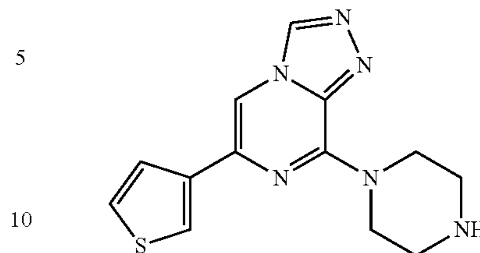
8-(piperazin-1-yl)-6-(thiophen-3-yl)-[1,2,4]triazolo[4,3-a]pyrazine
