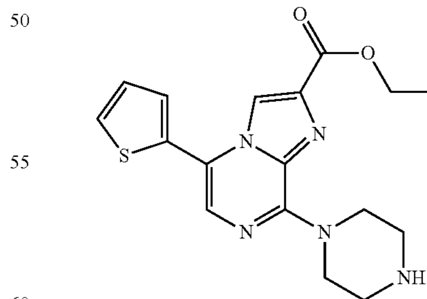
Ethyl 8-(piperazin-1-yl)-5-(thiophen-2-yl)imidazo[1,2-a]pyrazine-2-carboxylate
