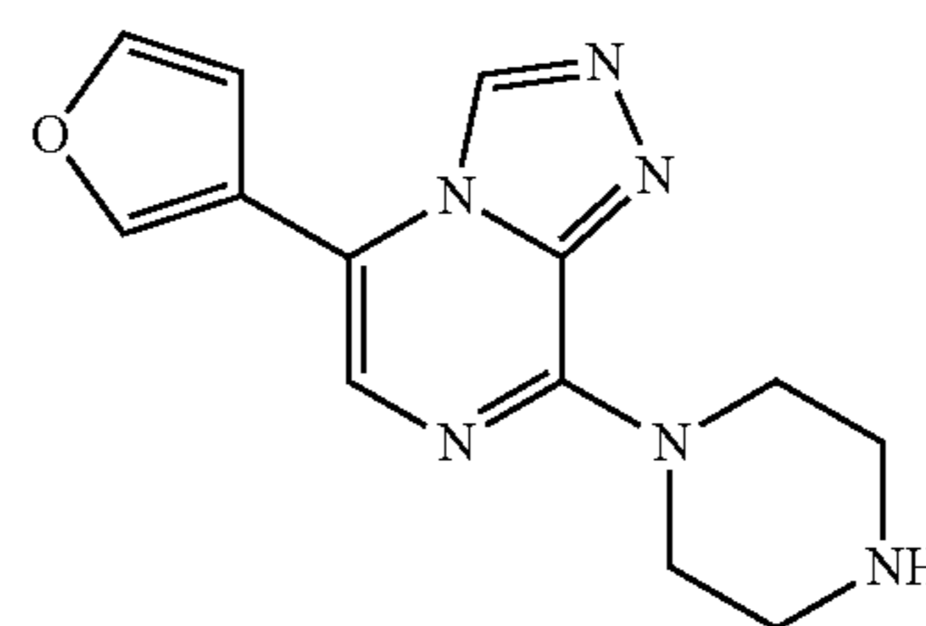
5-(Furan-3-yl)-8-(piperazin-1-yl)-[1,2,4]triazolo[4,3- a]pyrazine
