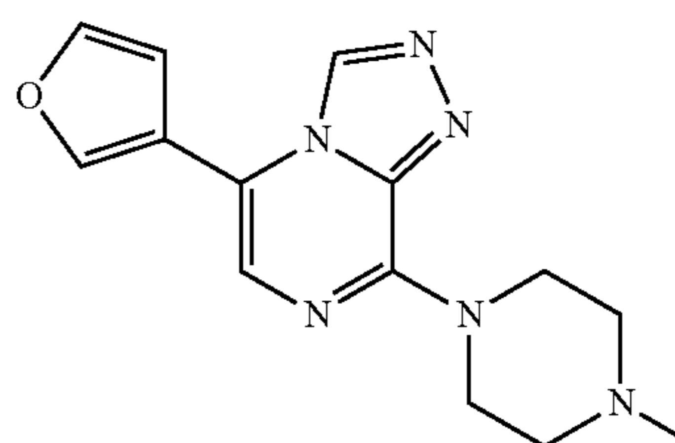
5-(Furan-3-yl)-8-(4-methylpiperazin-1-yl)-[1,2,4] triazolo[4,3-a]pyrazine
