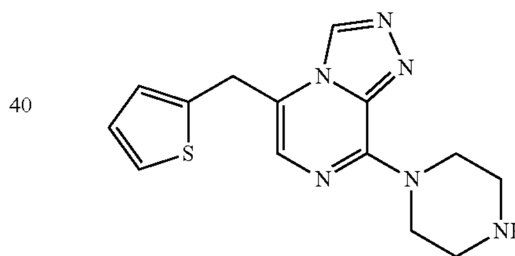
8-(piperazin-1-yl)-5-(thiophen-2-ylmethyl)-[1,2,4]triazolo[4,3-a]pyrazine
