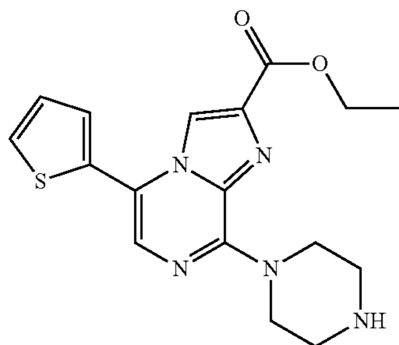
Ethyl 8-(piperazin-1-yl)-5-(thiophen-2-yl)imidazo[1,2-a]pyrazine-2-carboxylate
