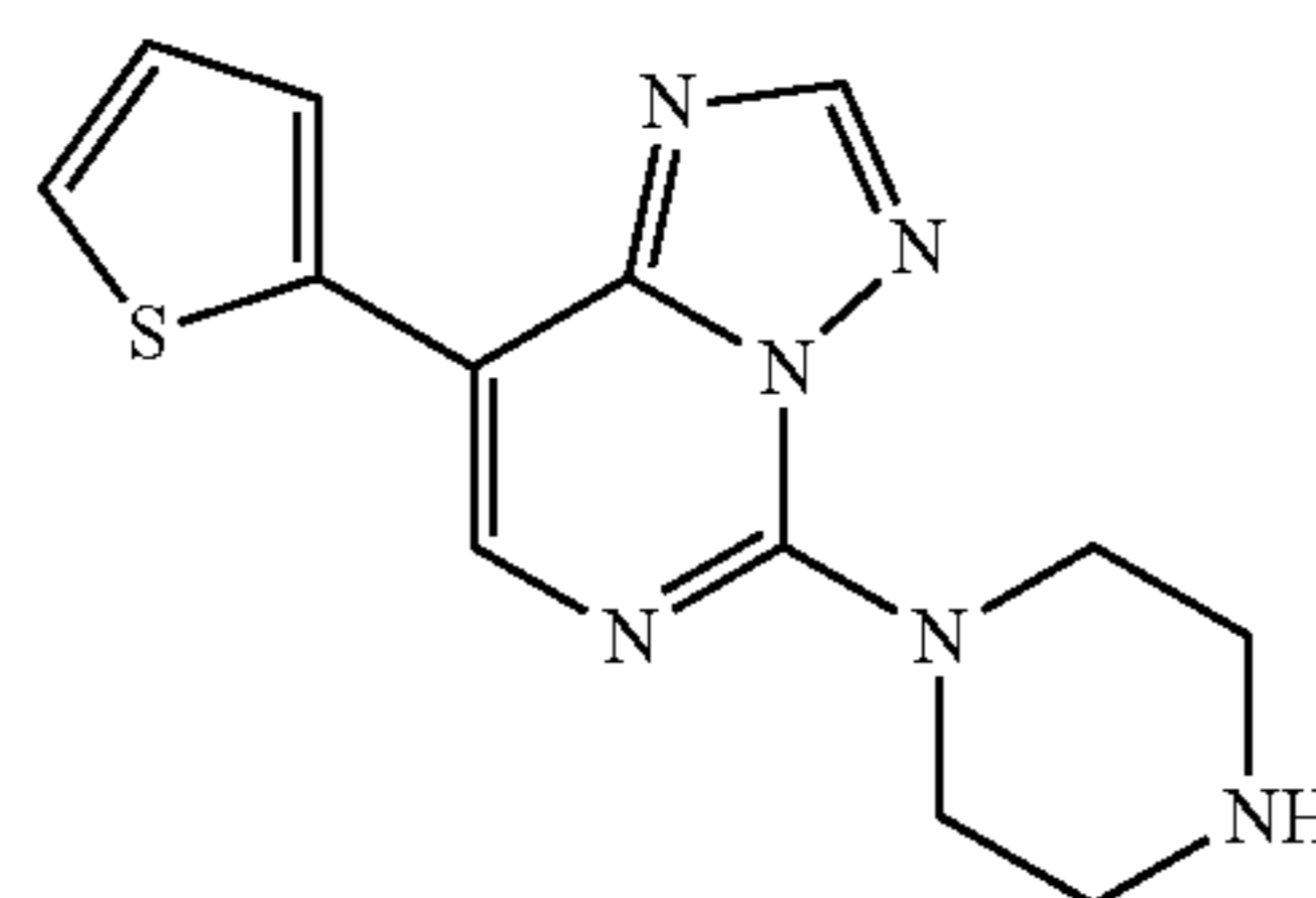
5-(piperazin-1-yl)-8-(thiophen-2-yl)-[1,2,4]triazolo[1,5-c]pyrimidine
