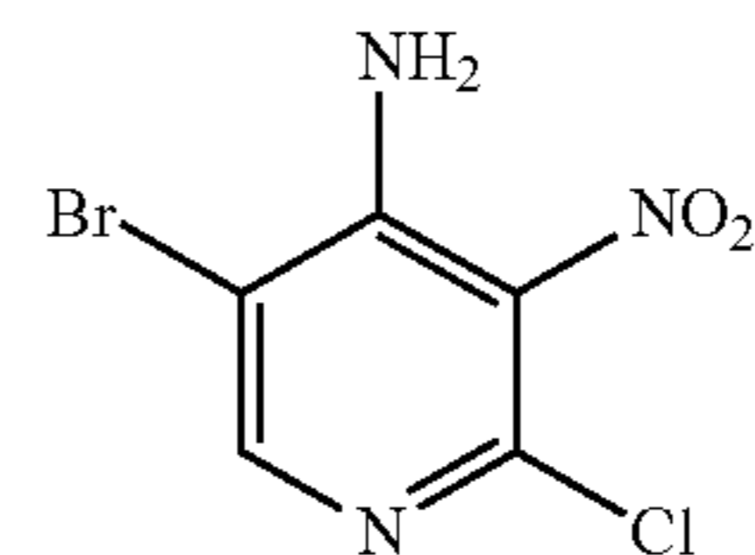
5-Bromo-2-chloro-3-nitropyridin-4-amine
