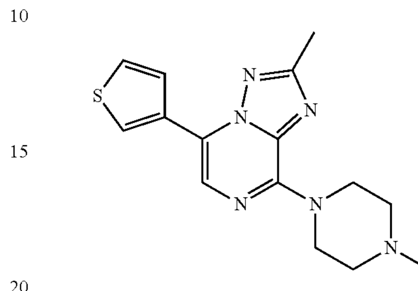
2-Methyl-8-(4-methylpiperazin-1-yl)-5-(thiophen-2-yl)-[1,2,4]triazolo[1,5-a]pyrazine
