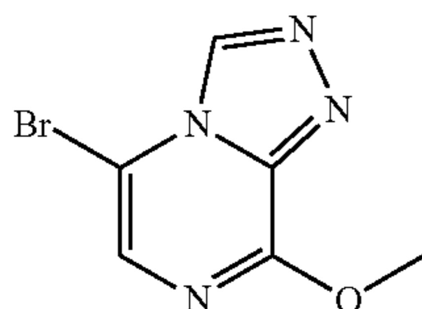
5-Bromo-8-methoxy-[1,2,4]triazolo[4,3-a]pyrazine
