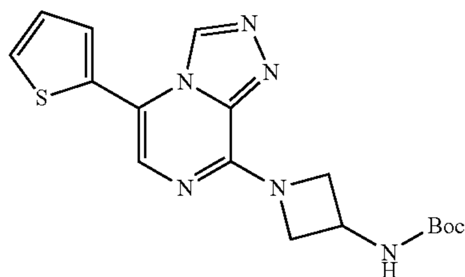
tert-Butyl (1-(5-(thiophen-2-yl)-[1,2,4]triazolo[4,3-a]pyrazin-8-yl)azetidin-3-yl)carbamate
