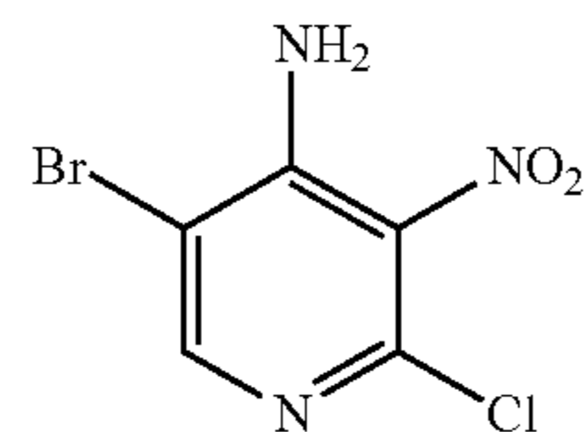
5-Bromo-2-chloro-3-nitropyridin-4-amine
