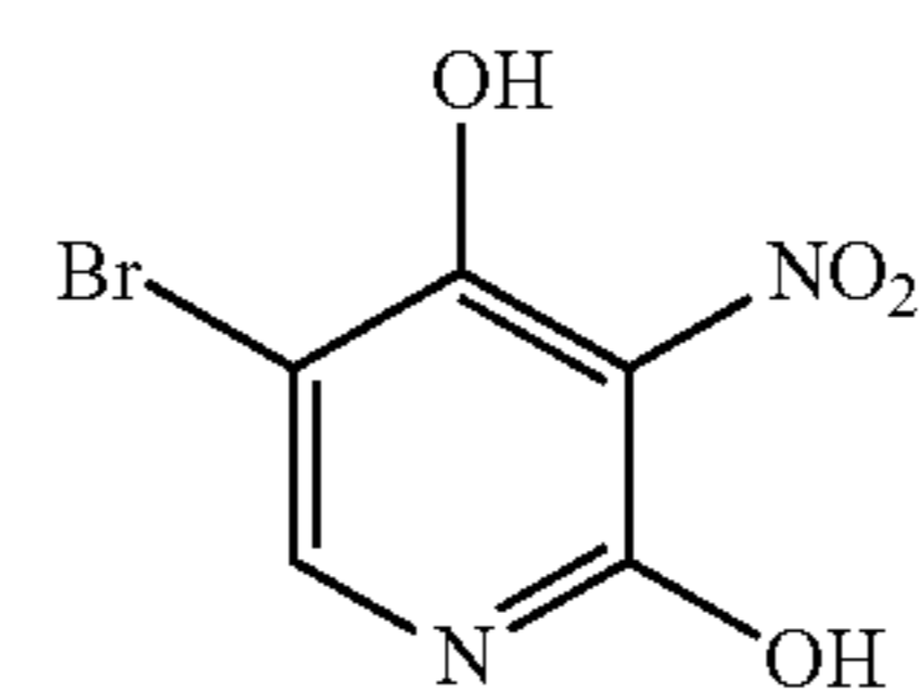
5-Bromo-3-nitropyridine-2,4-diol
