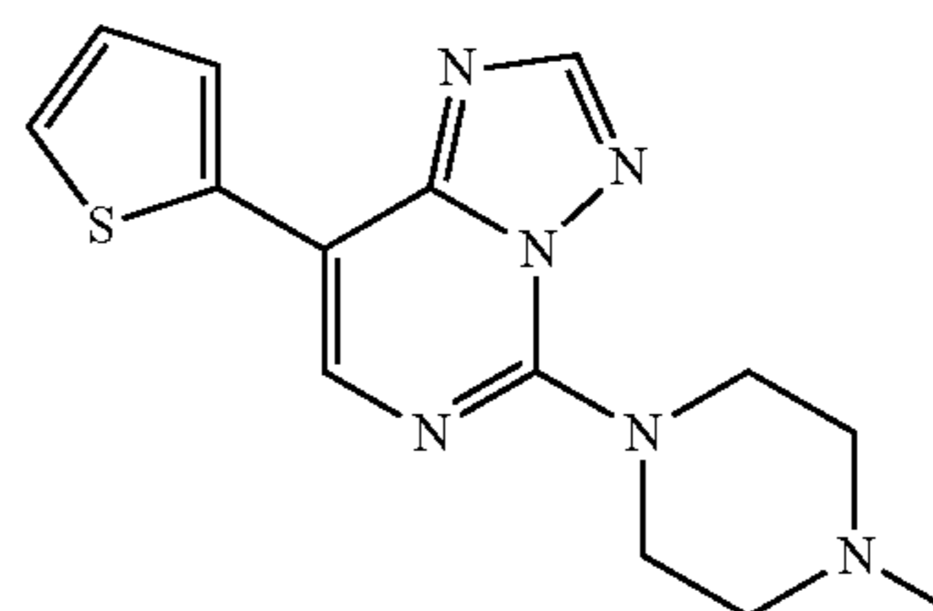
5-(4-Methylpiperazin-1-yl)-8-(thiophen-2-yl)-[1,2,4]triazolo[1,5-c]pyrimidine
