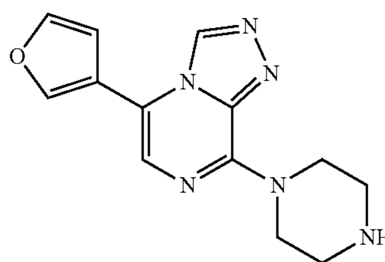
5-(Furan-3-yl)-8-(piperazin-1-yl)-[1,2,4]triazolo[4,3- a]pyrazine
