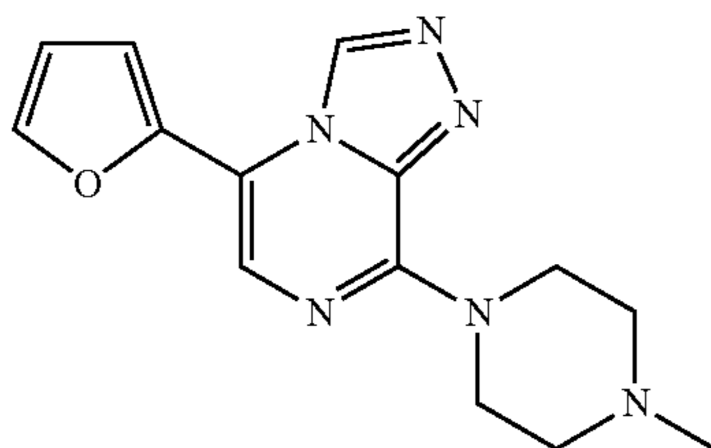
5-(Furan-2-yl)-8-(4-methylpiperazin-1-yl)-[1,2,4]triazolo[4,3-a]pyrazine
