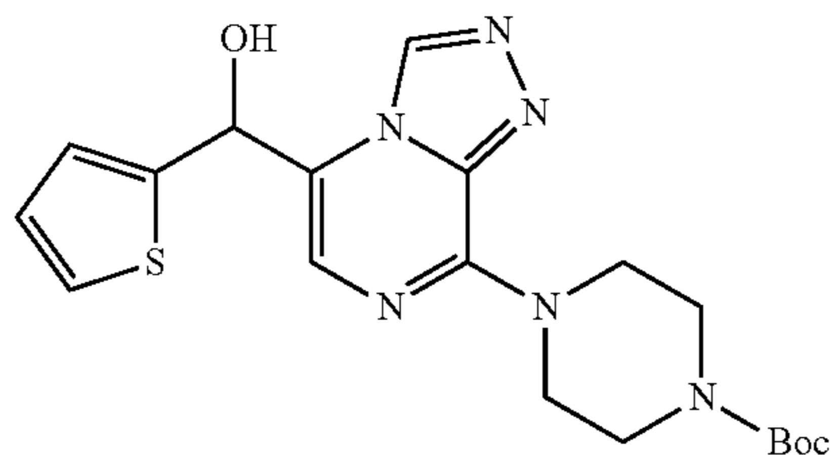
tert-Butyl 4-(5-(hydroxy(thiophen-2-yl)methyl)-[1,2,4]triazolo[4,3-a]pyrazin-8-yl)piperazine-1-carboxylate
