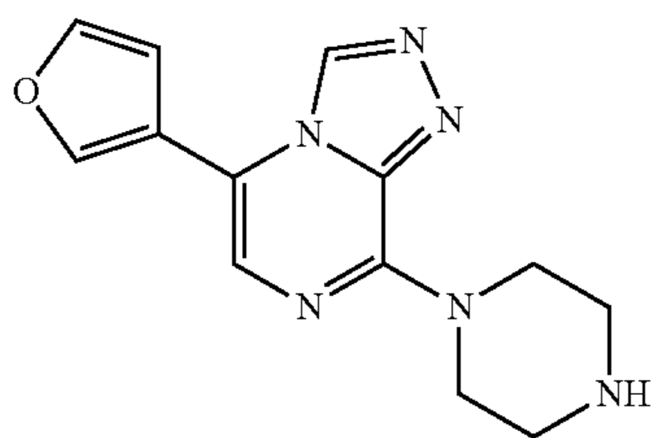
5-(Furan-3-yl)-8-(piperazin-1-yl)-[1,2,4]triazolo[4,3-a]pyrazine
