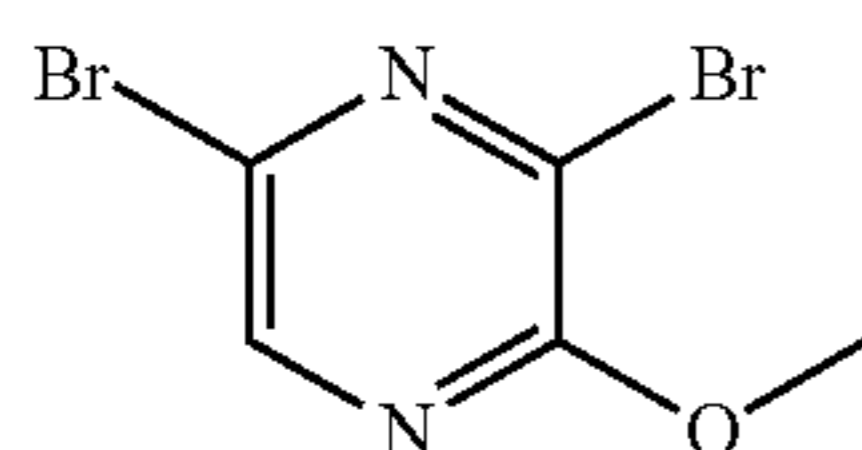
3,5-Dibromo-2-methoxypyrazine
