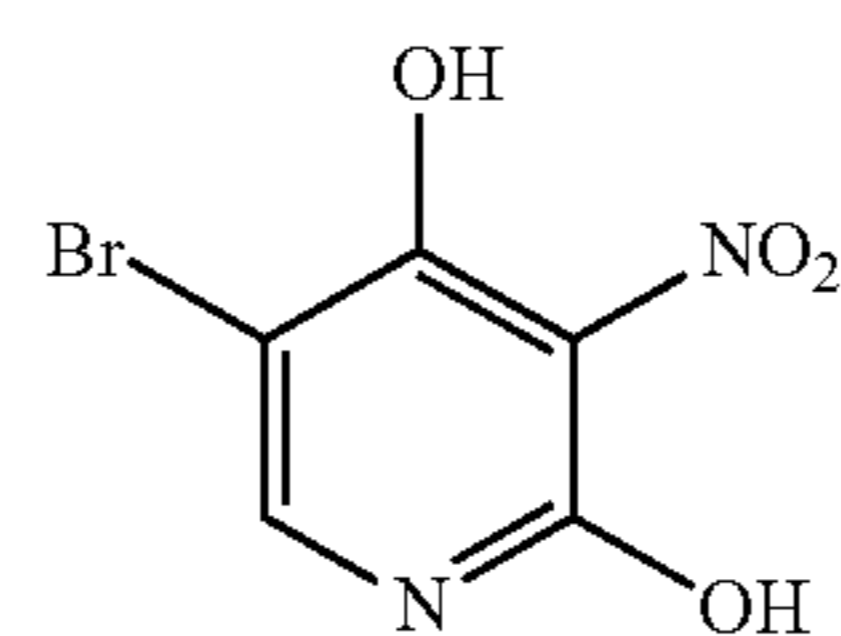
5-Bromo-3-nitropyridine-2,4-diol
