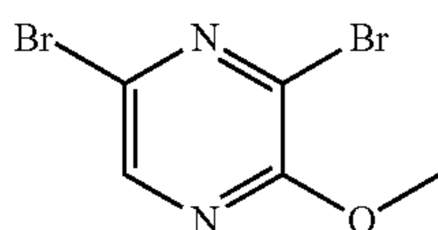
3,5-Dibromo-2-methoxypyrazine
