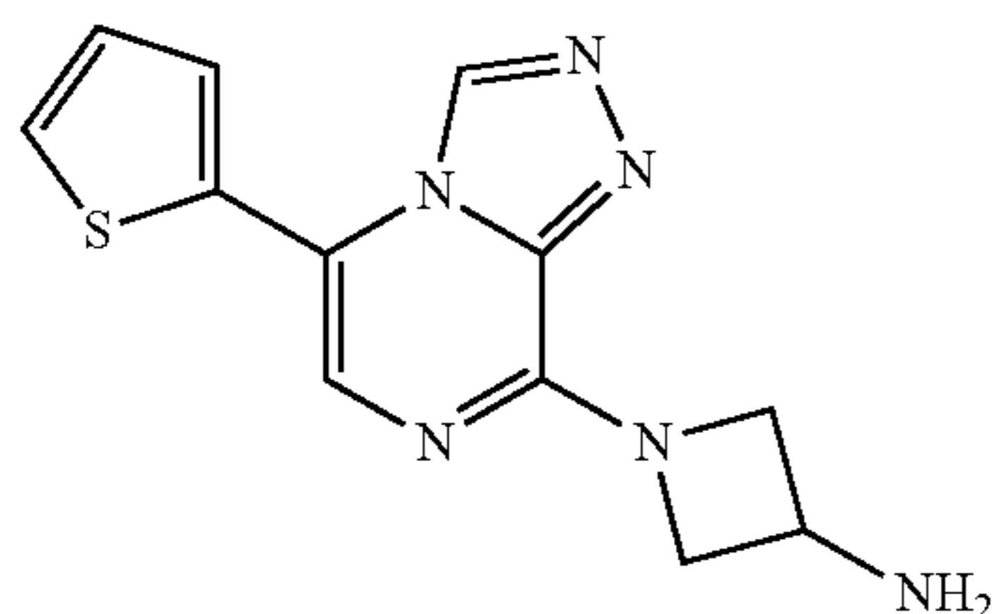
1-(5-(Thiophen-2-yl)-[1,2,4]triazolo[4,3-a]pyrazin-8-yl)azetidin-3-amine
