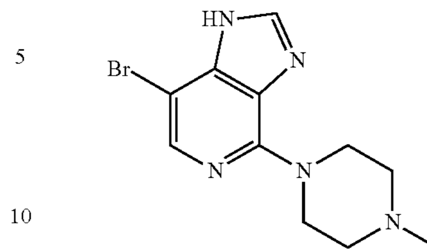
7-Bromo-4-(4-methylpiperazin-1-yl)-1H-imidazo[4,5-c]pyridine
