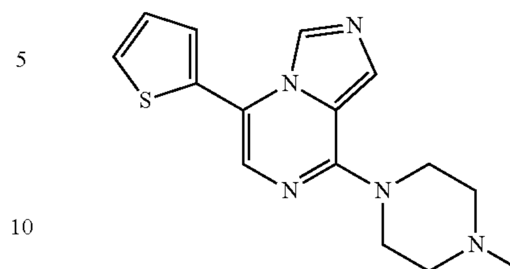
8-(4-Methylpiperazin-1-yl)-5-(thiophen-2-yl)imidazo[1,5-a]pyrazine
