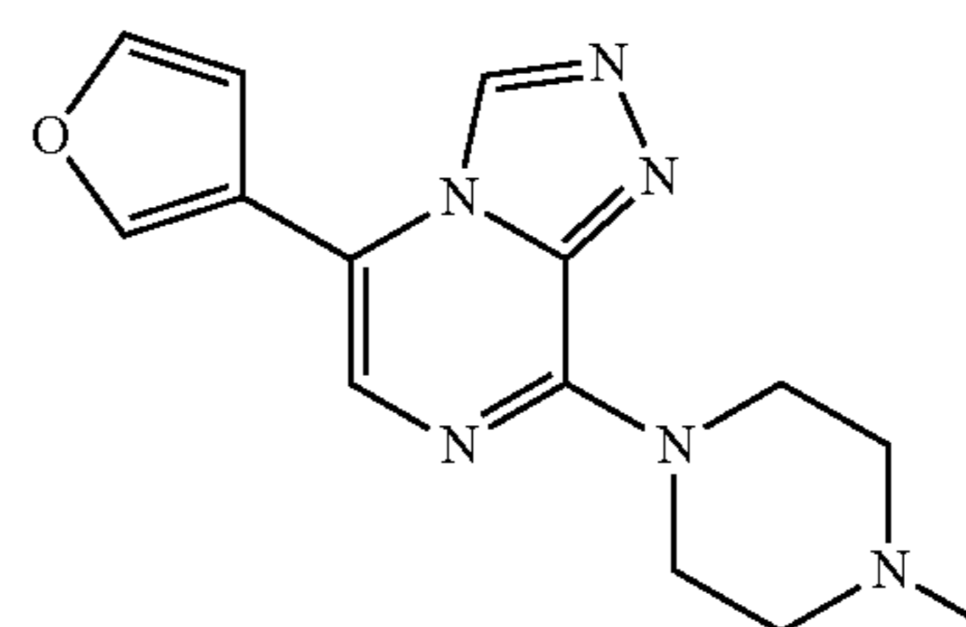
5-(Furan-3-yl)-8-(4-methylpiperazin-1-yl)-[1,2,4] triazolo[4,3-a]pyrazine
