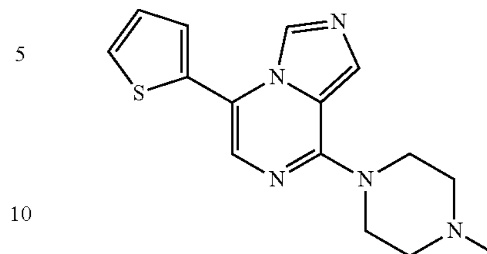
8-(4-Methylpiperazin-1-yl)-5-(thiophen-2-yl)imidazo[1,5-a]pyrazine
