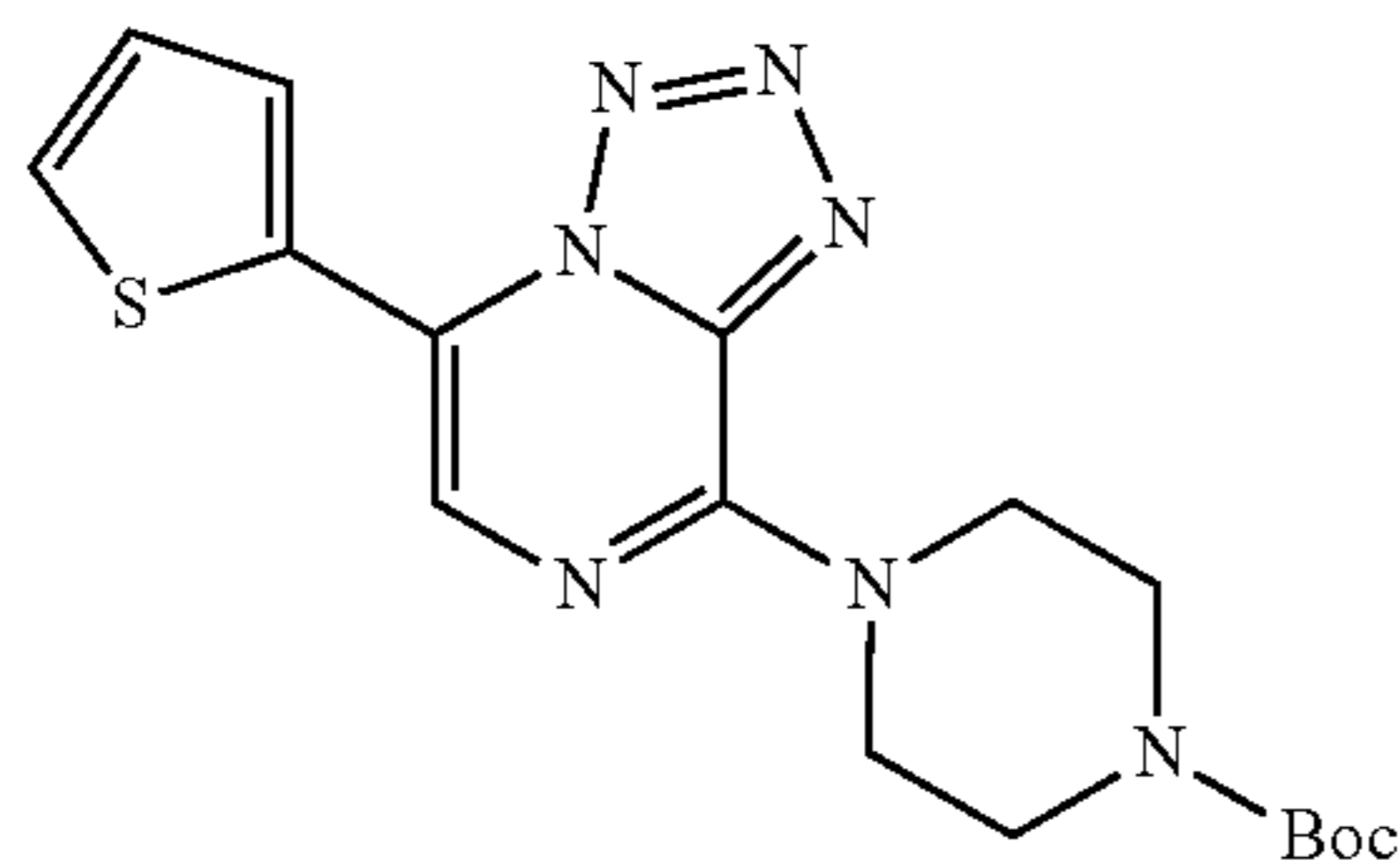
tert-Butyl 4-(5-(thiophen-2-yl)tetrazolo[1,5-a] pyrazin-8-yl)piperazine-1-carboxylate
