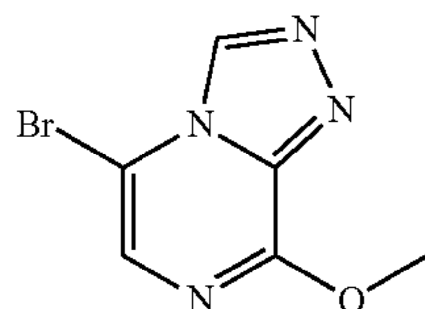
5-Bromo-8-methoxy-[1,2,4]triazolo[4,3-a]pyrazine
