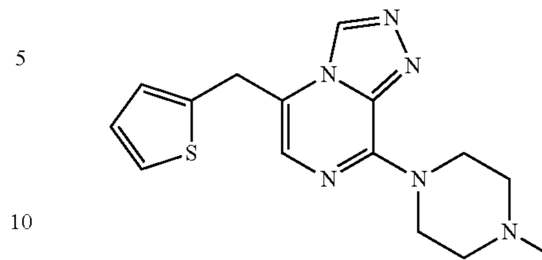
8-(4-Methylpiperazin-1-yl)-5-(thiophen-2-ylmethyl)-[1,2,4]triazolo[4,3-a]pyrazine
