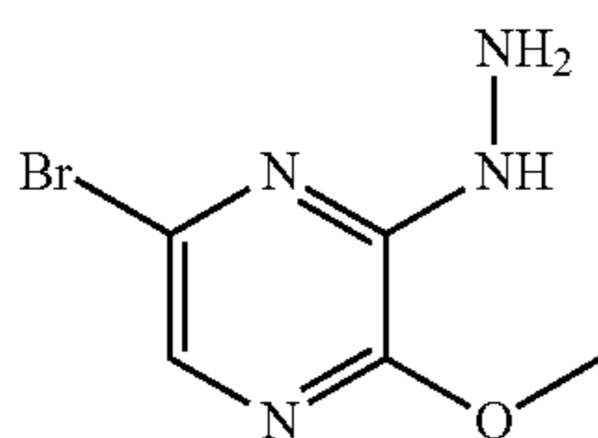
5-Bromo-3-hydrazinyl-2-methoxypyrazine
