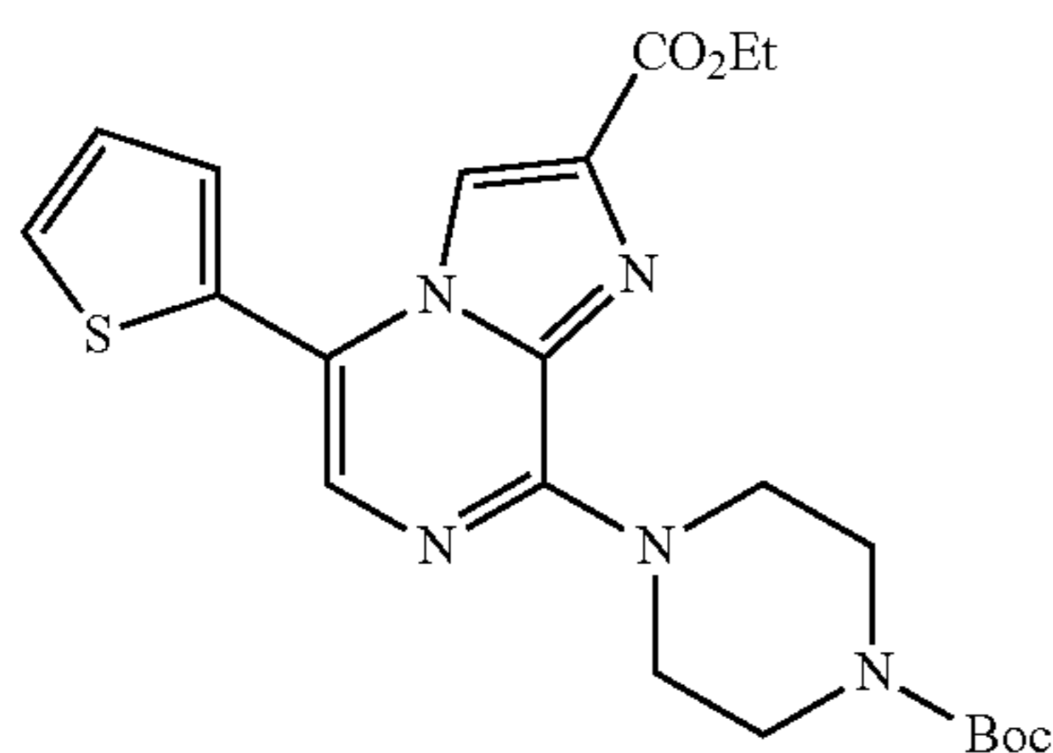
Ethyl 8-(4-(tert-butoxycarbonyl)piperazin-1-yl)-5-(thiophen-2-yl)imidazo[1,2-a]pyrazine-2-carboxylate
