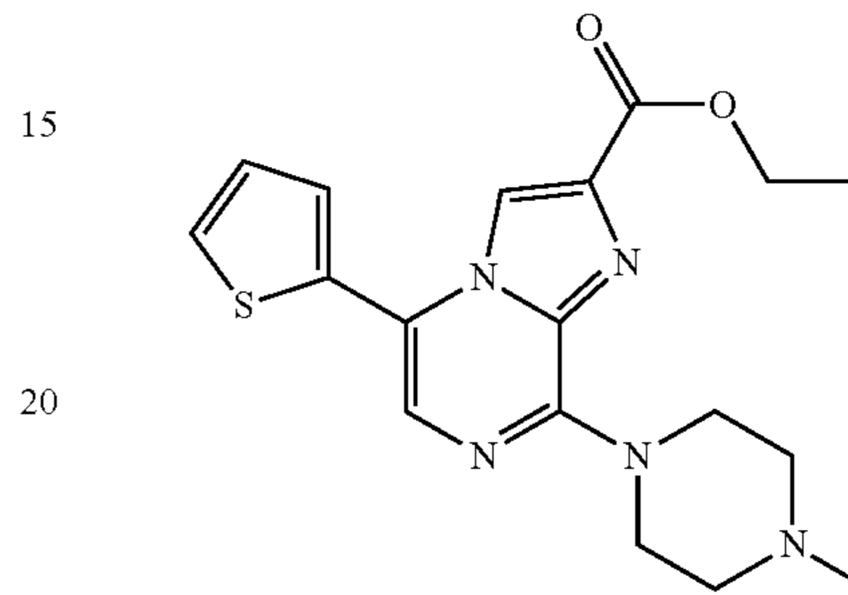
Ethyl 8-(4-methylpiperazin-1-yl)-5-(thiophen-2-yl)imidazo[1,2-a]pyrazine-2-carboxylate
