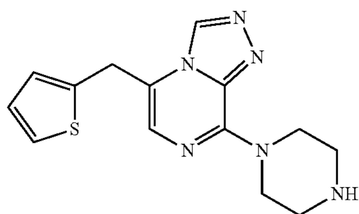
8-(piperazin-1-yl)-5-(thiophen-2-ylmethyl)-[1,2,4]triazolo[4,3-a]pyrazine
