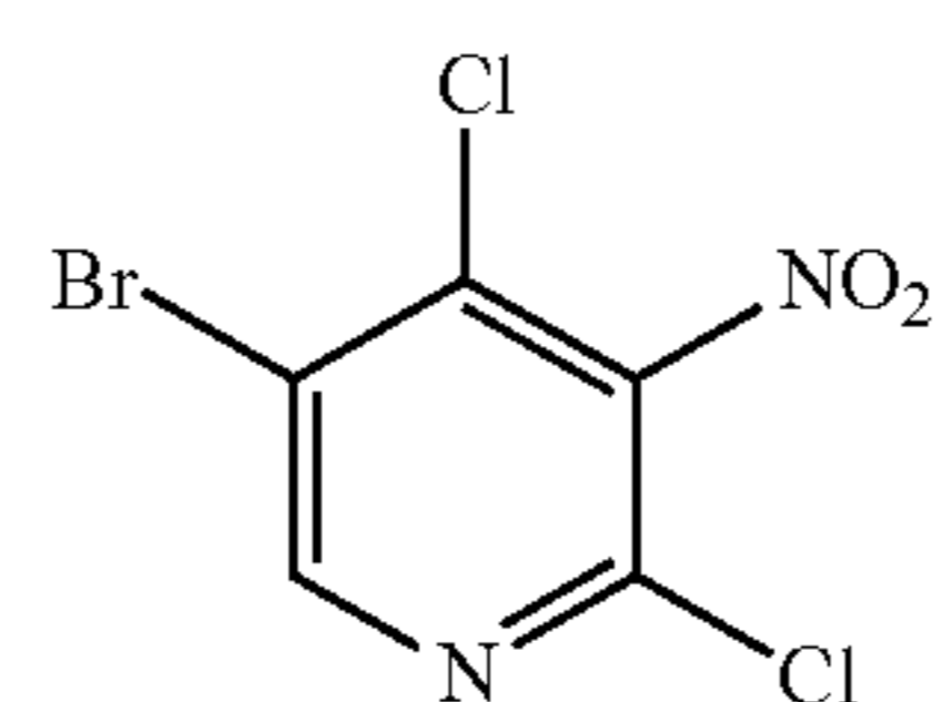
5-Bromo-2,4-dichloro-3-nitropyridine
