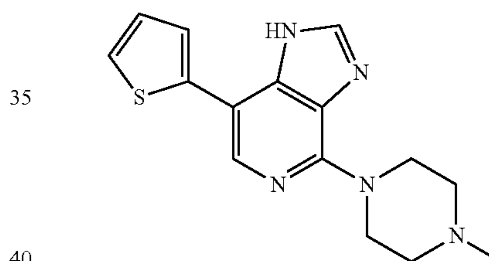
4-(4-Methylpiperazin-1-yl)-7-(thiophen-2-yl)-1H-imidazo[4,5-c]pyridine
