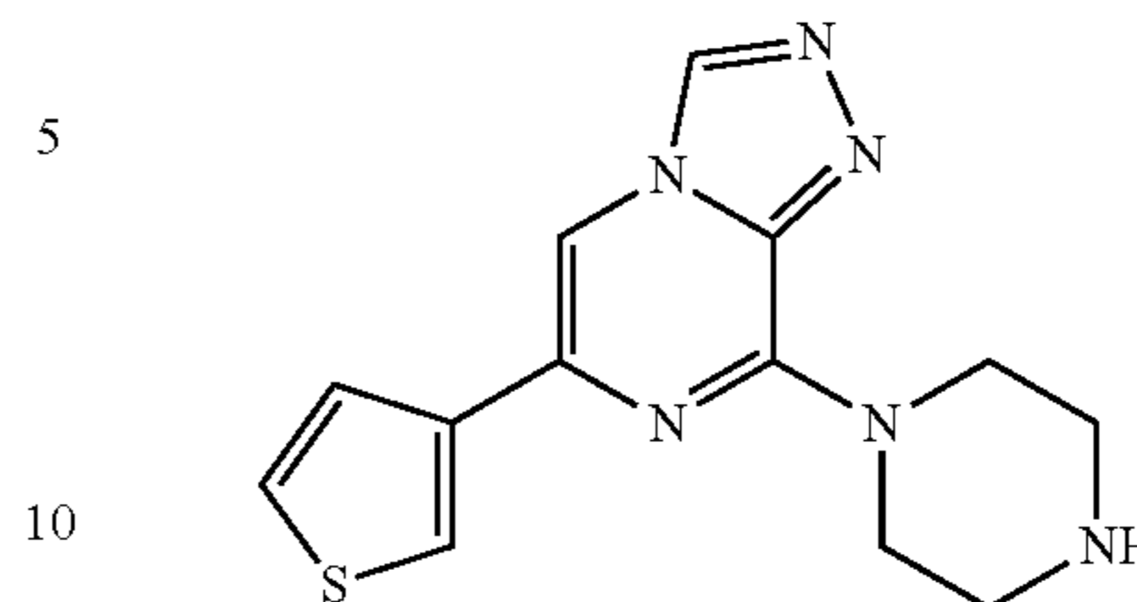
8-(piperazin-1-yl)-6-(thiophen-3-yl)-[1,2,4]triazolo[4,3-a]pyrazine
