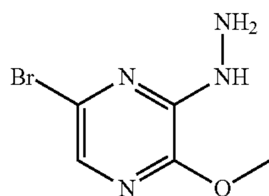
5-Bromo-3-hydrazinyl-2-methoxypyrazine
