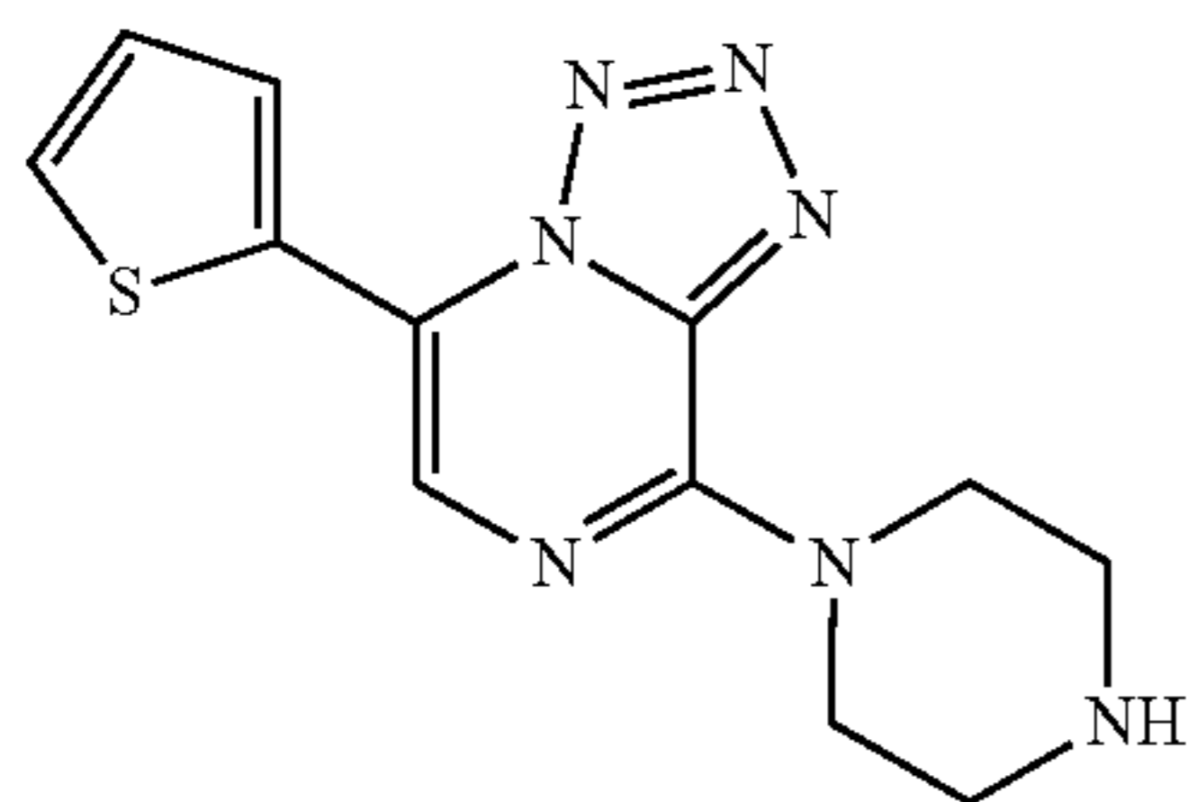
8-(piperazin-1-yl)-5-(thiophen-2-yl)tetrazolo[1,5-a] pyrazine HCl salt
