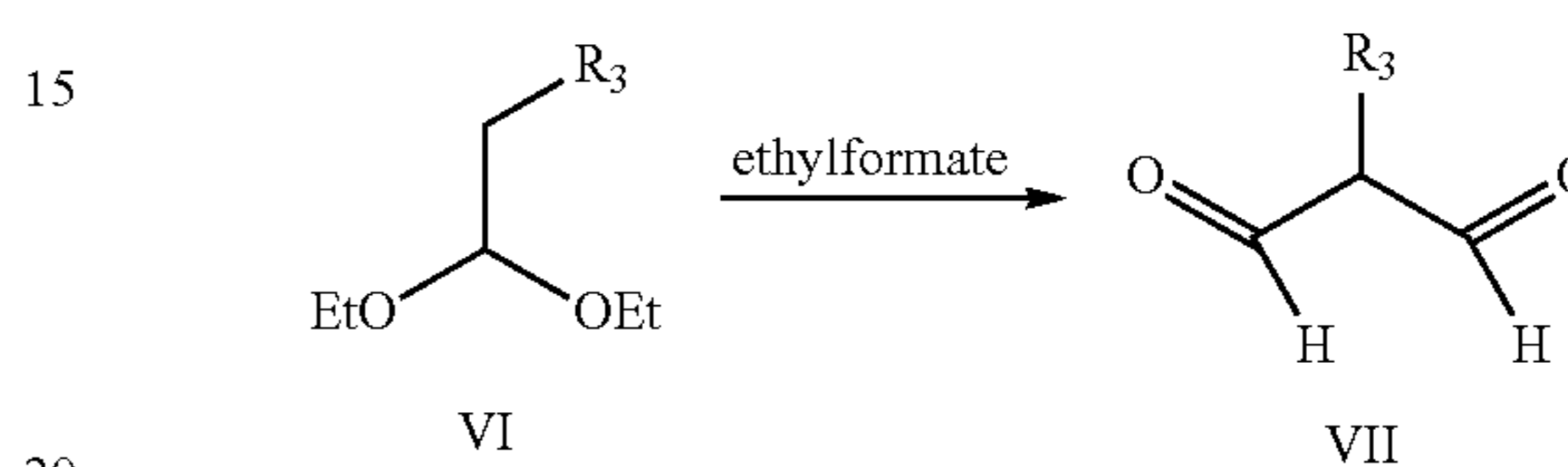
Scheme 4
