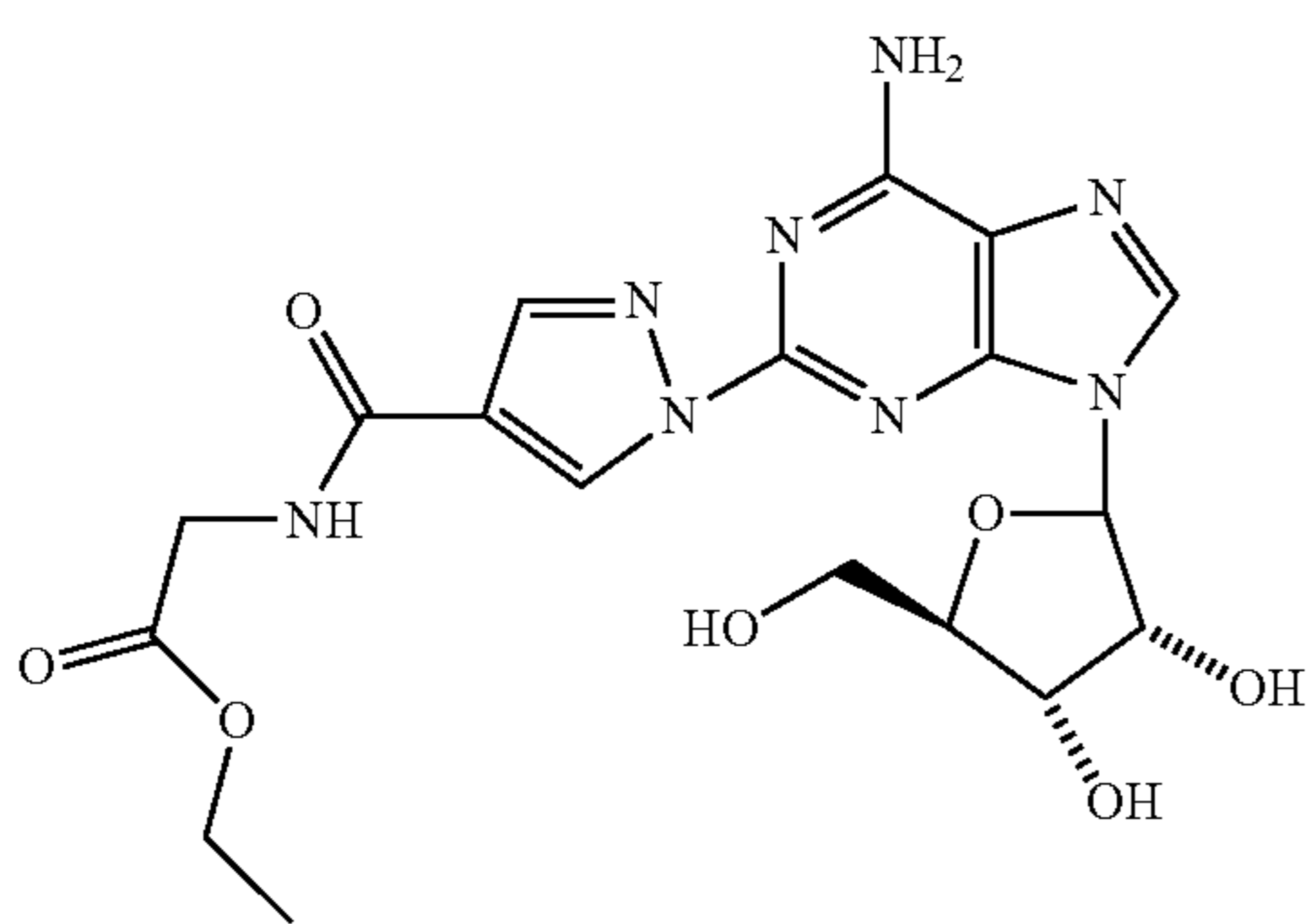
Ethyl 2-[(1-{9-[(4S,2R,3R,5R)-3,4-dihydroxy-5-(hydroxymethyl)oxolan-2-yl]-6-aminopurin-2-yl}pyrazol-4-yl)carbonylamino]acetate (23)
