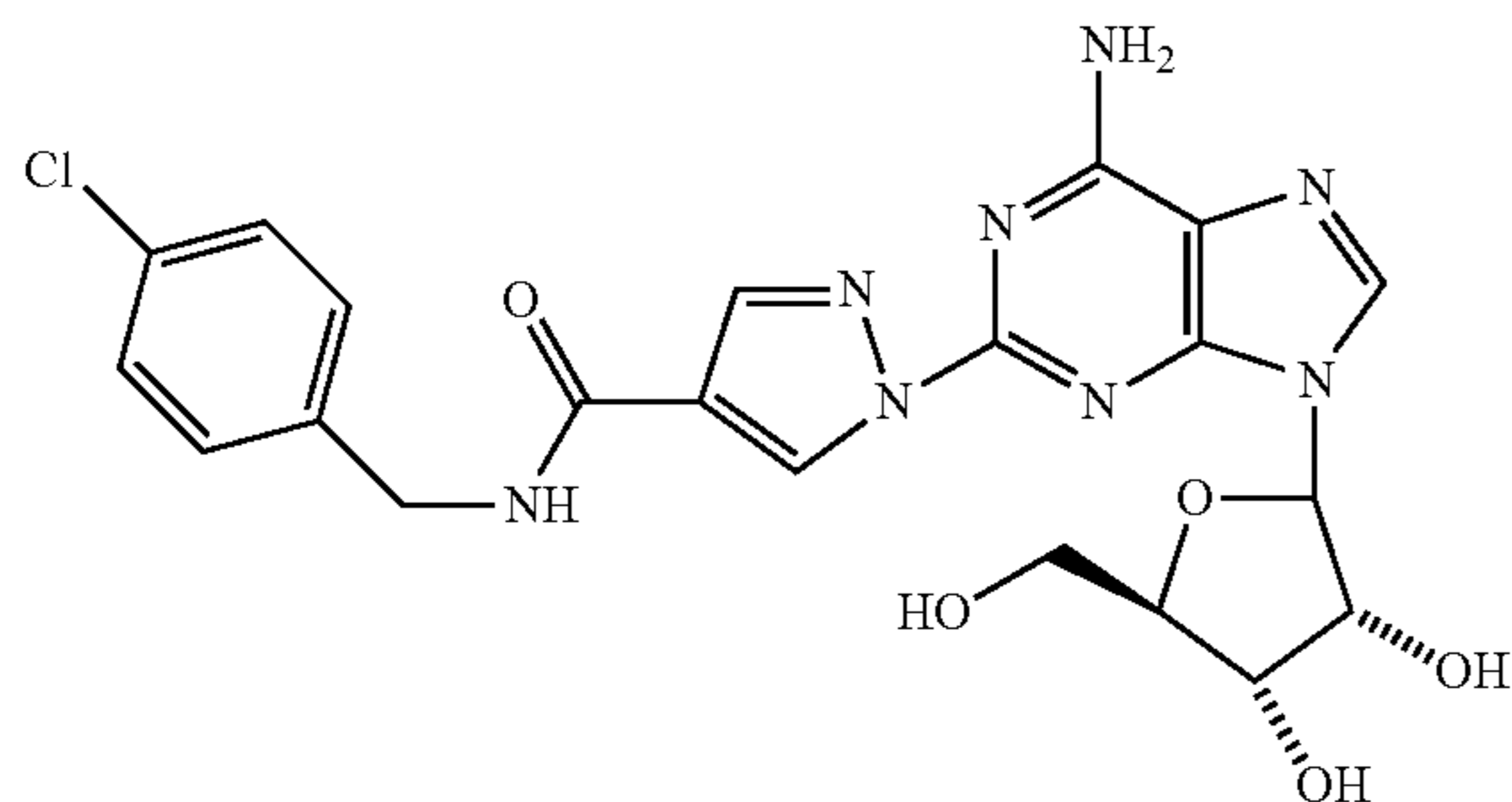
(1-{9-[(4S,2R,3R,5R)-3,4-dihydroxy-5-(hydroxymethyl)oxolan-2-yl]-6-aminopurin-2-yl}pyrazol-4-yl)-N-[(4-chlorophenyl)methyl]carboxamide (22)
