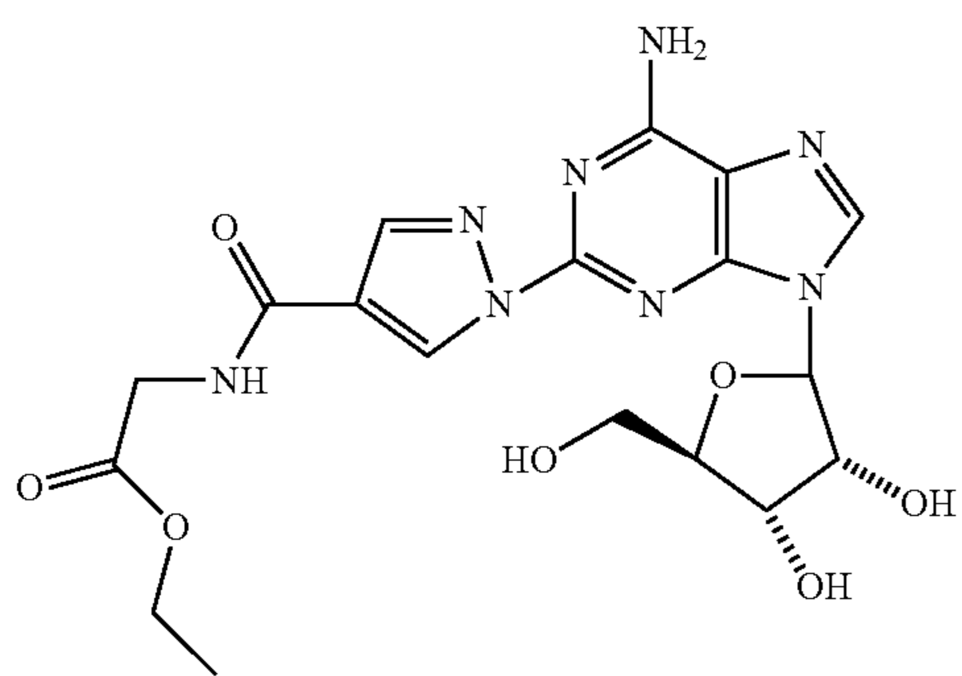
Ethyl 2-[(1-{9-[(4S,2R,3R,5R)-3,4-dihydroxy-5-(hydroxymethyl)oxolan-2-yl]-6-aminopurin-2-yl}pyrazol-4-yl)carbonylamino]acetate (23)
