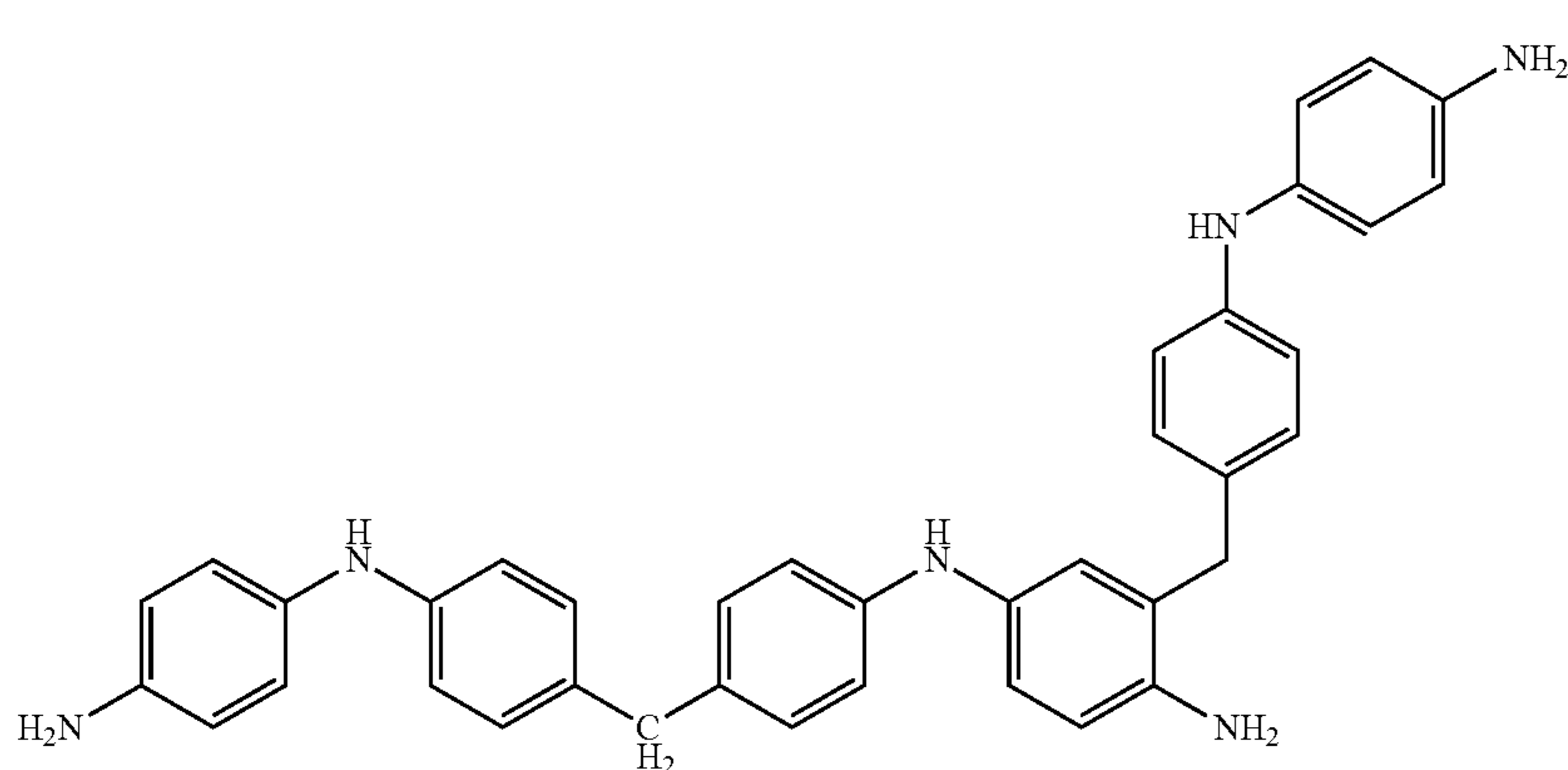
Formula (3)
