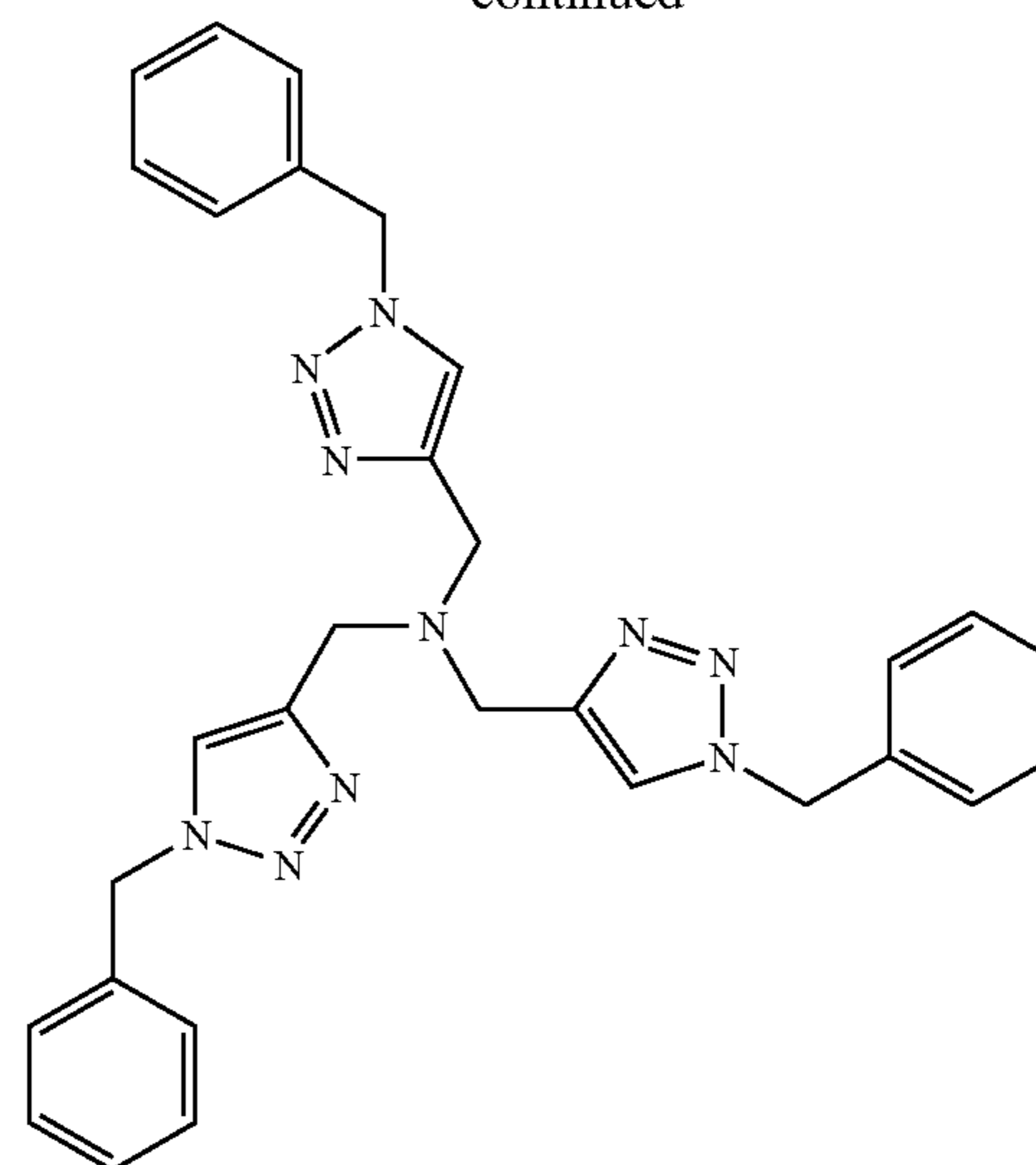
Triazole ligand
