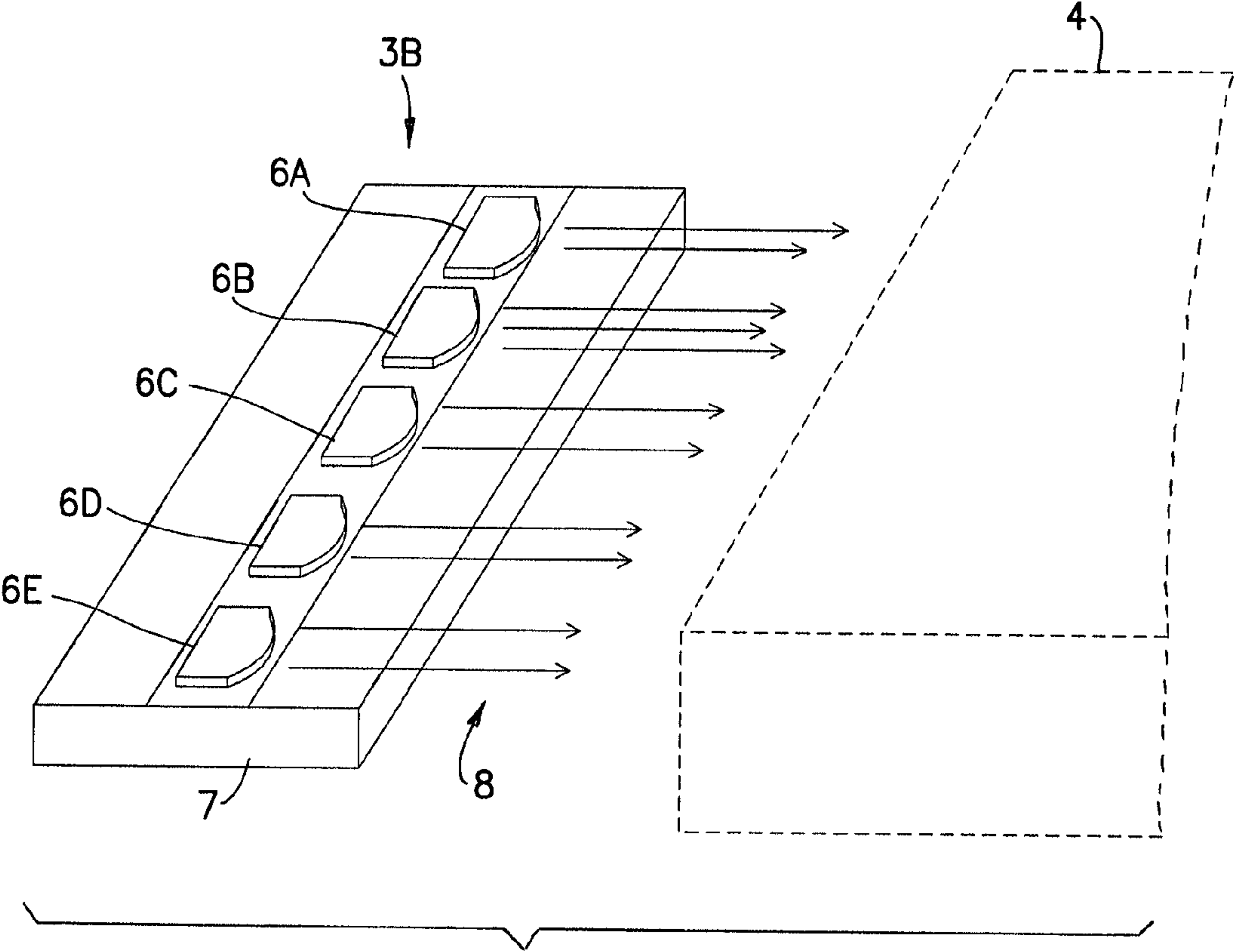
FIG.1C
