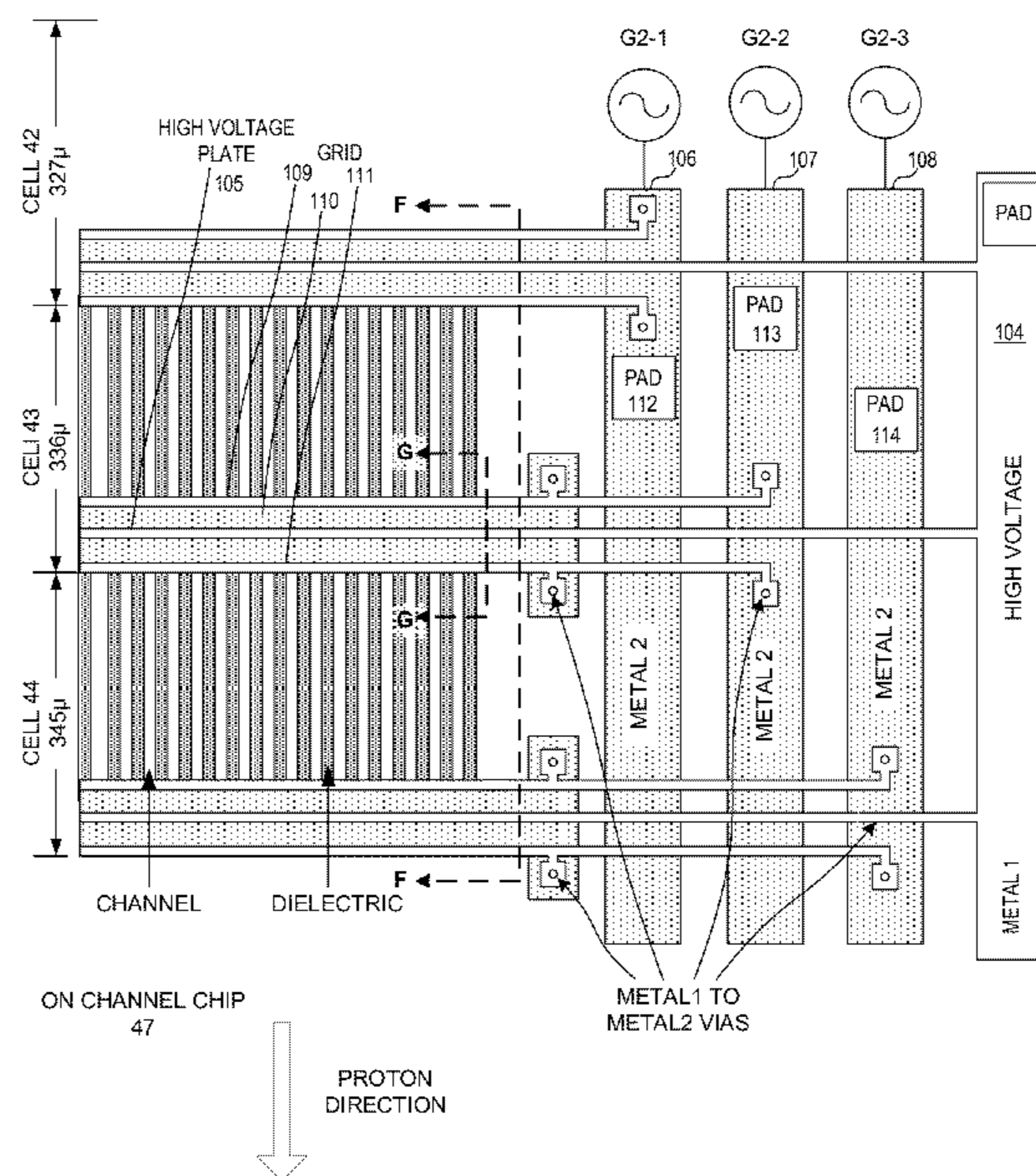
DETAIL D – PLATE/GRID CELL TOP VIEW
