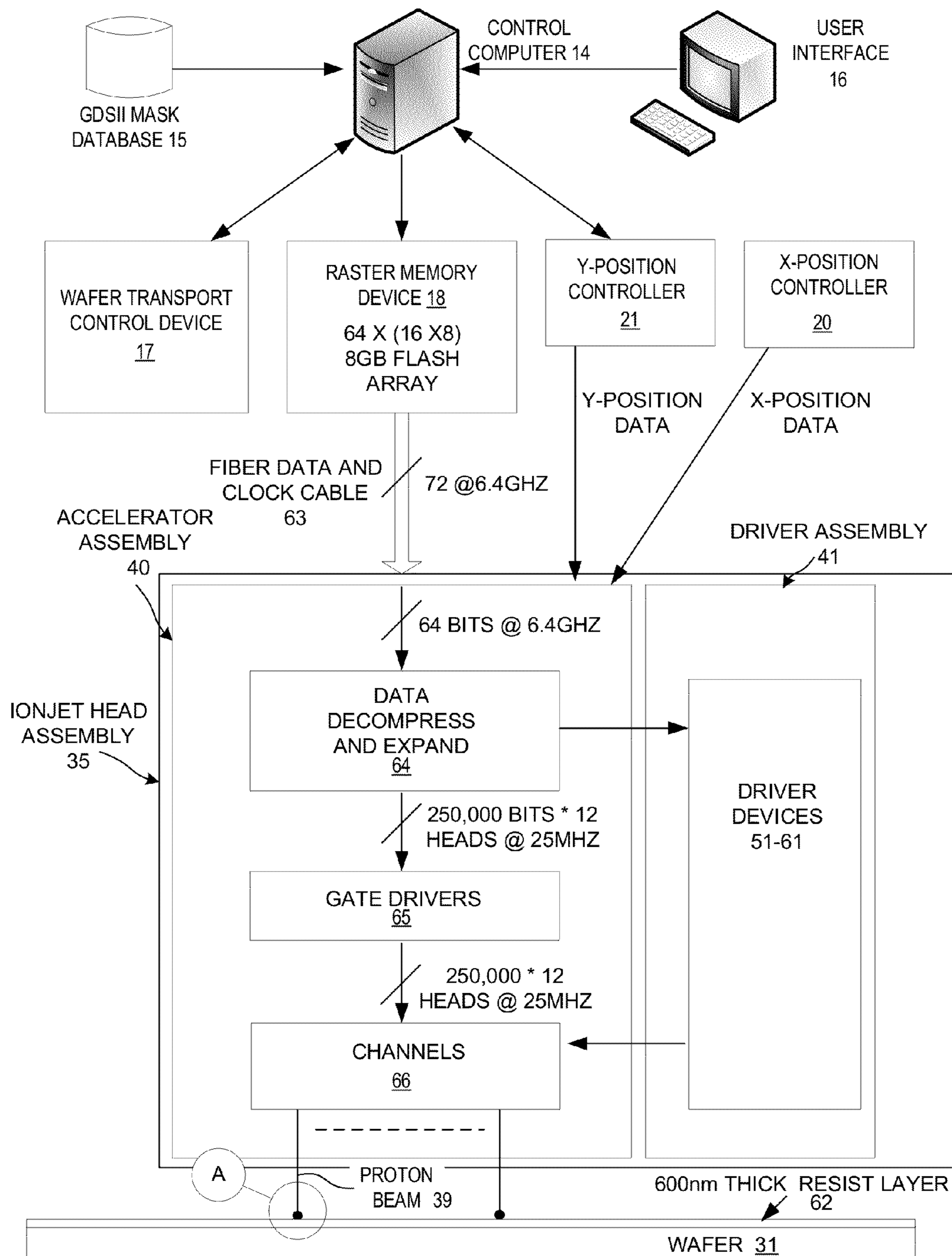
SYSTEM DATA PATH FIG. 11
