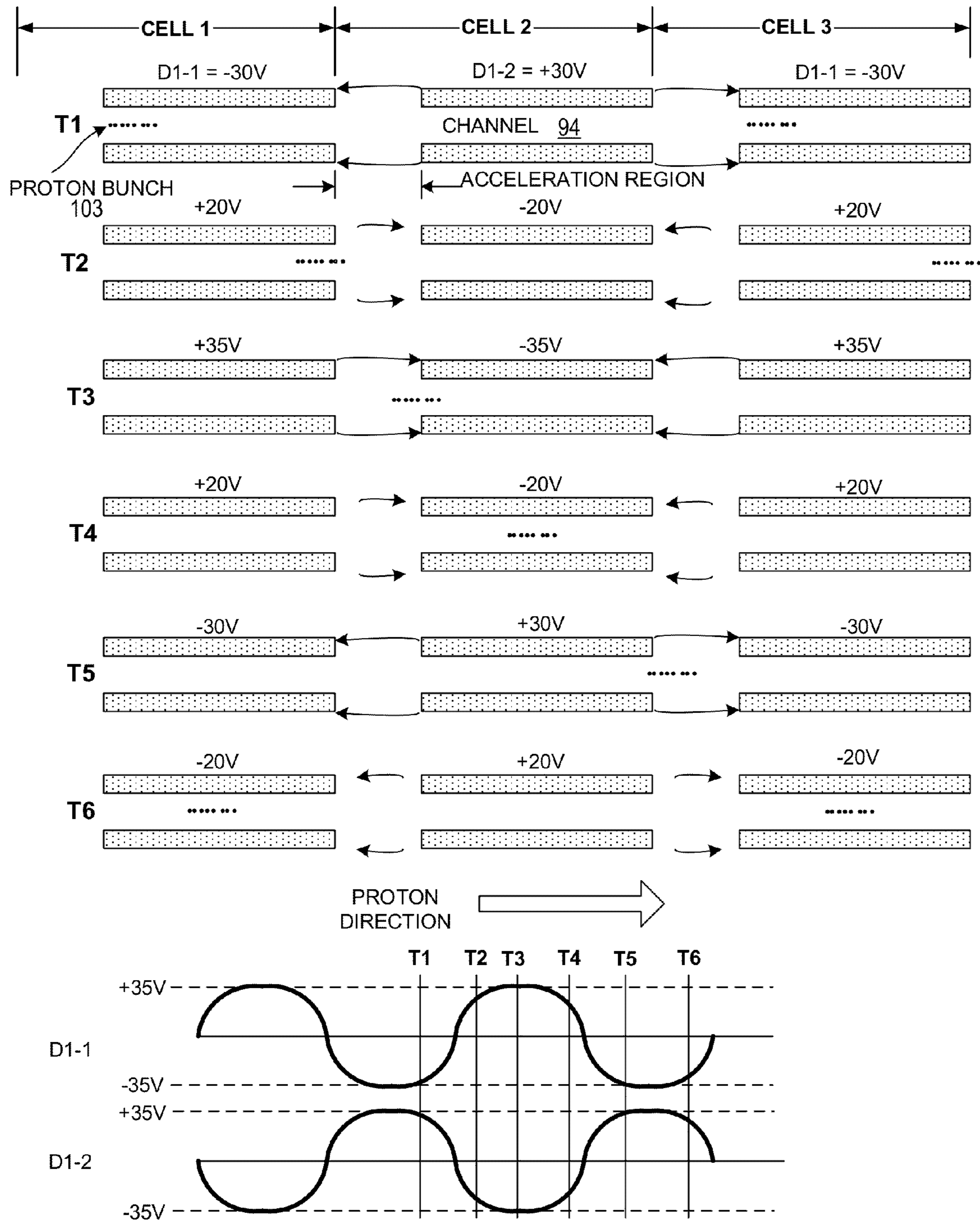
DETAIL E – DRIFT PROTON TIMING SCHEME
