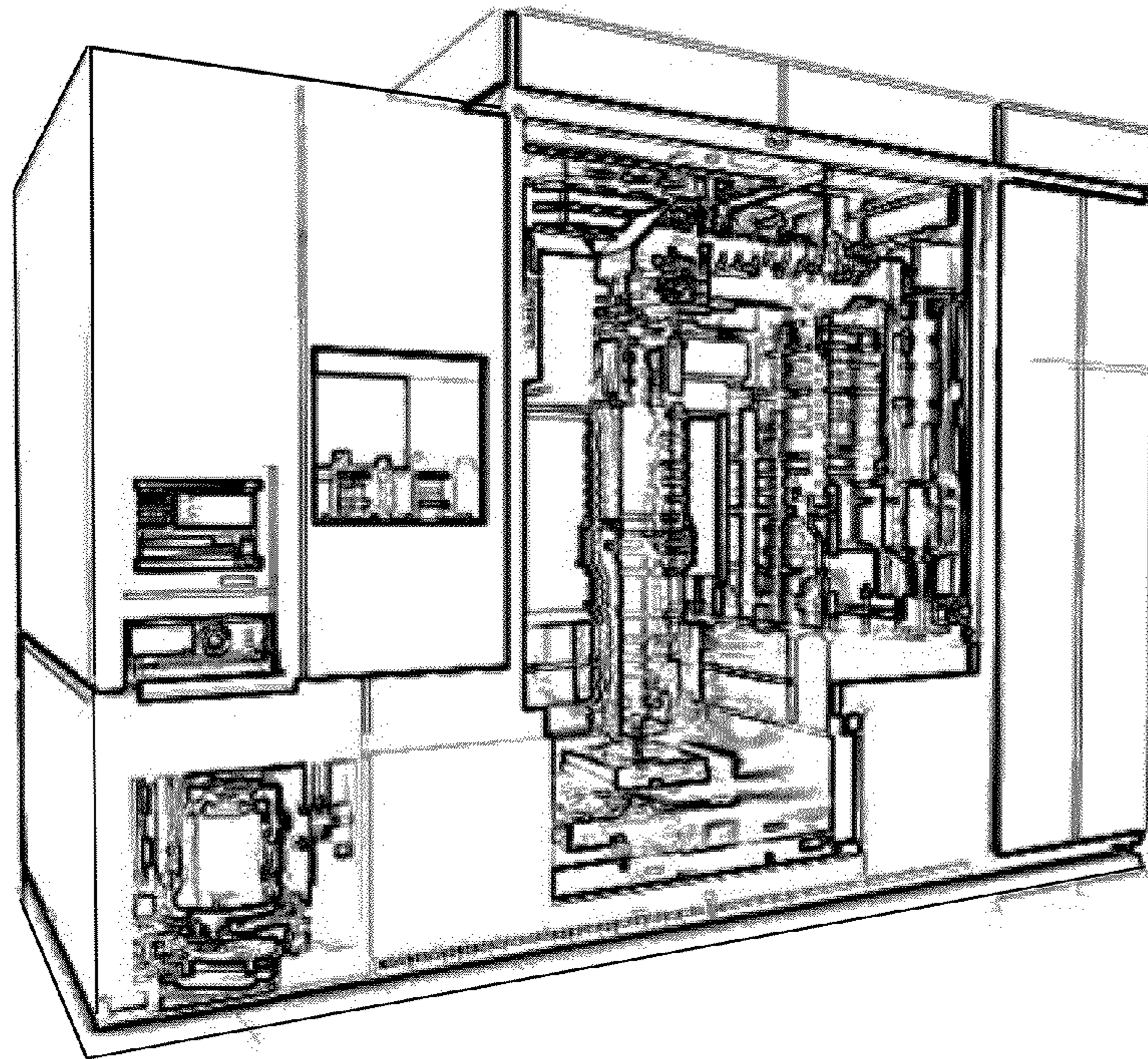
WAFER STEPPER (Prior Art) FIG. 1
