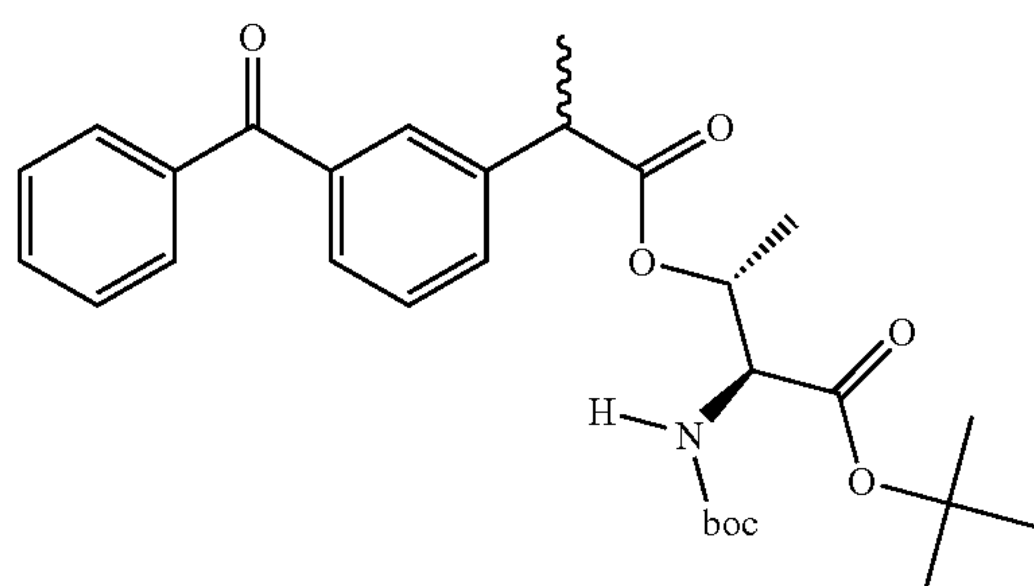
SPI001801 3-[2(R,S)-(3-Benzoyl-phenyl)-propionyloxy]-2(S)-tert-butoxycarbonylamino-butyric acid tert-butyl ester: (mix of diastereomers)
