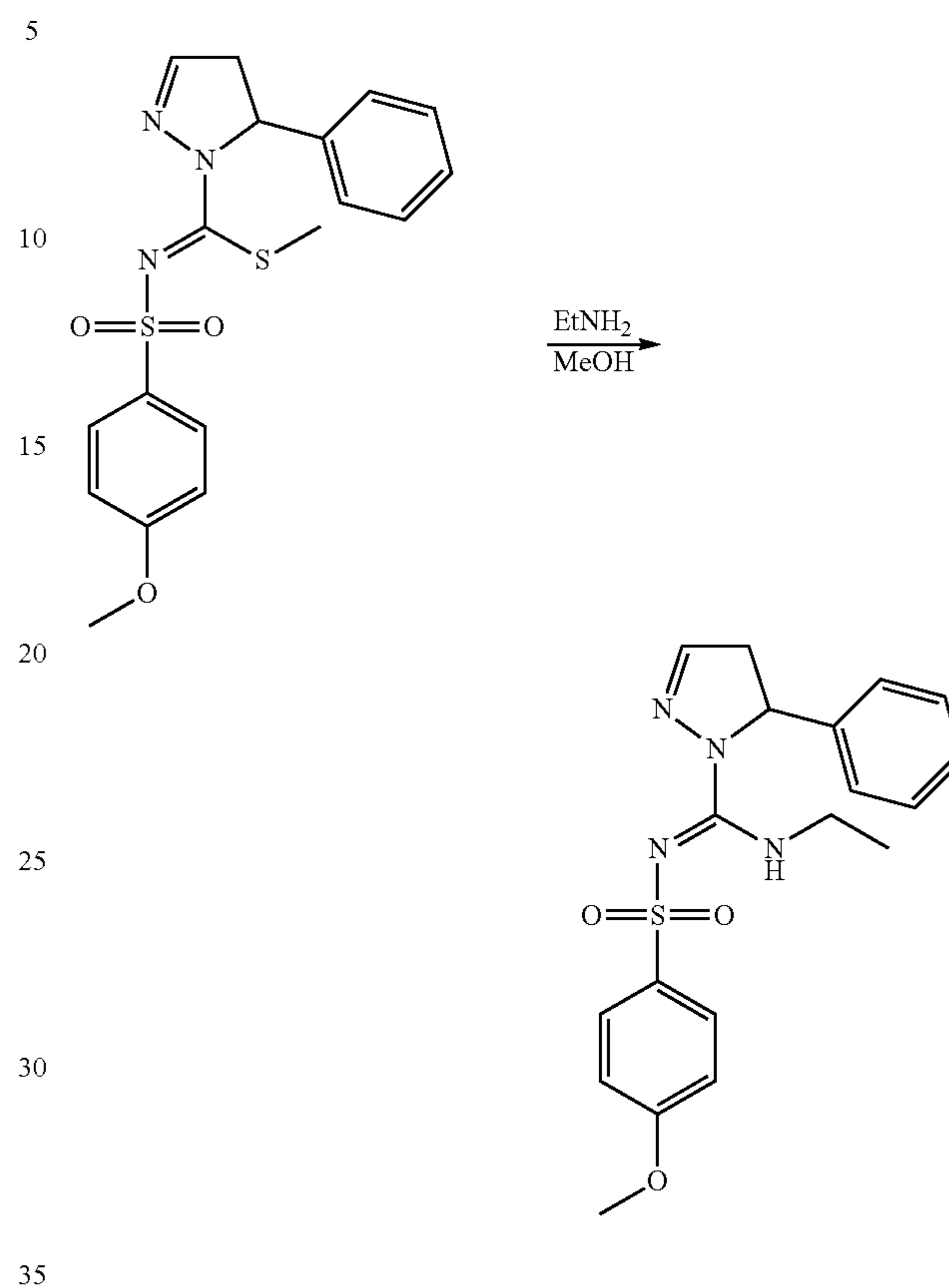
4-Methoxy-N-[methylsulfanyl-(5-phenyl-4,5-dihydro-pyrazol-1-yl)-methylene]benzene-sulfonamide
