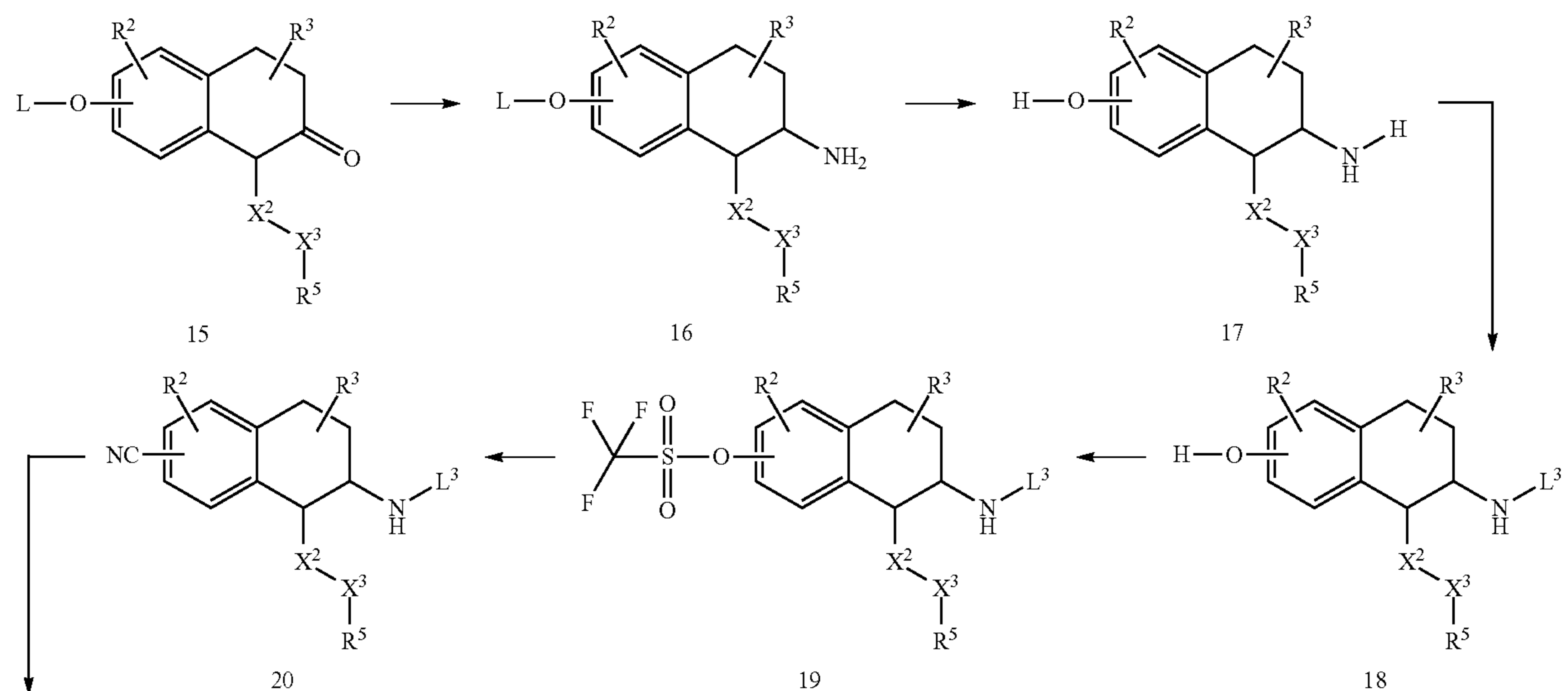
Scheme 4:
