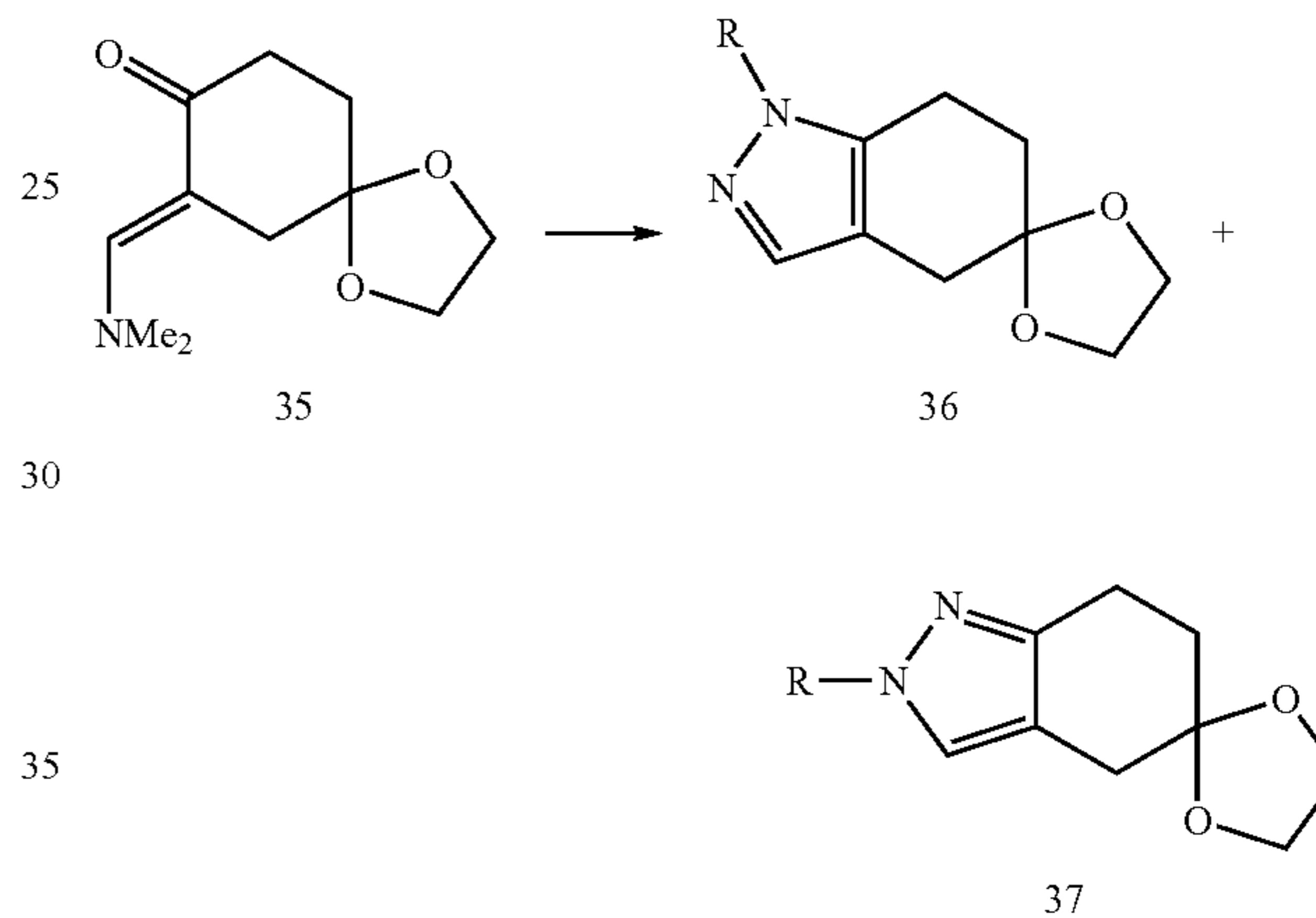
Scheme 8:
