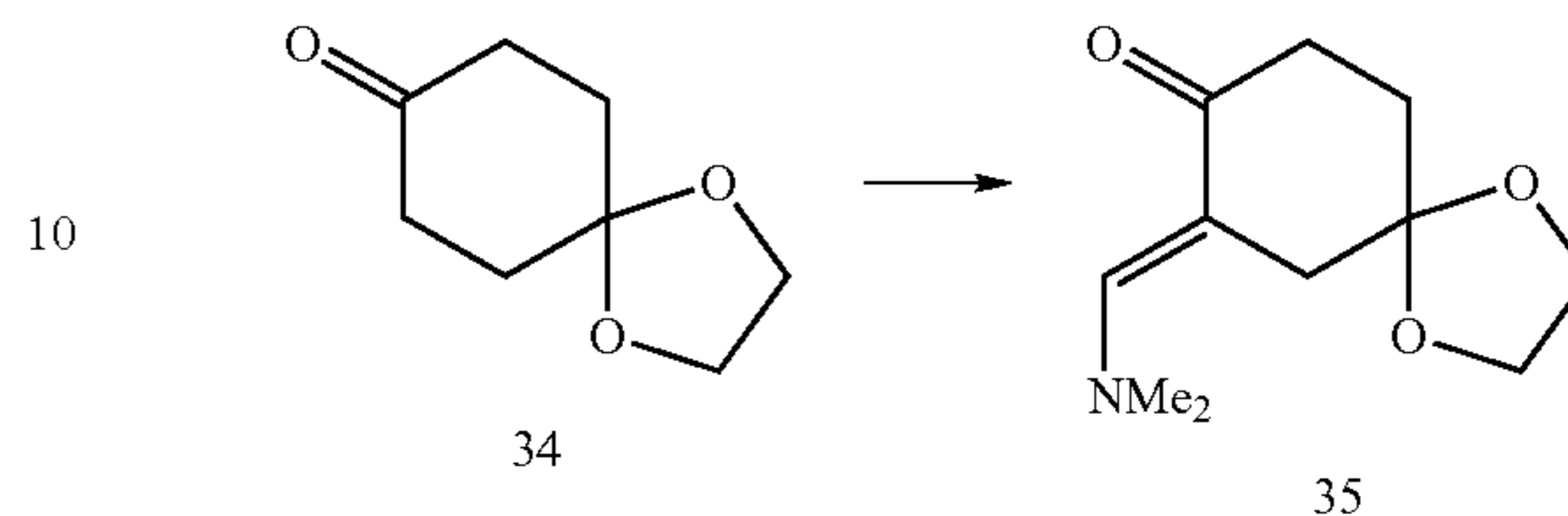
Scheme 7:
