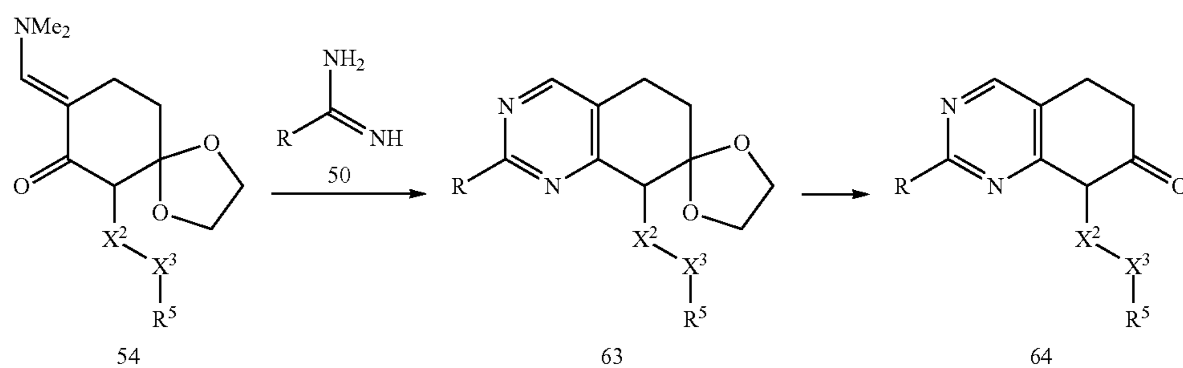
Scheme 15:
