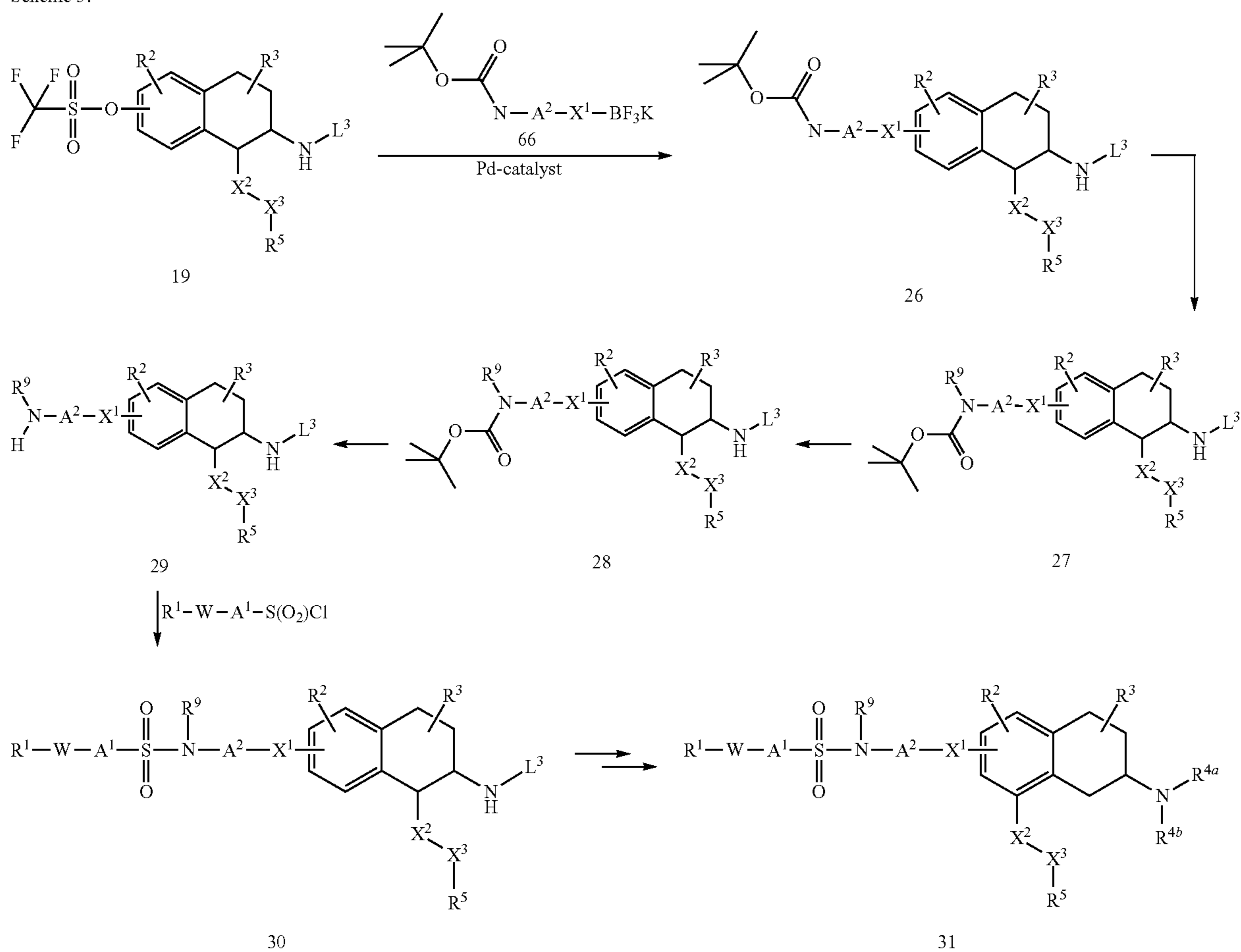
Scheme 5:
