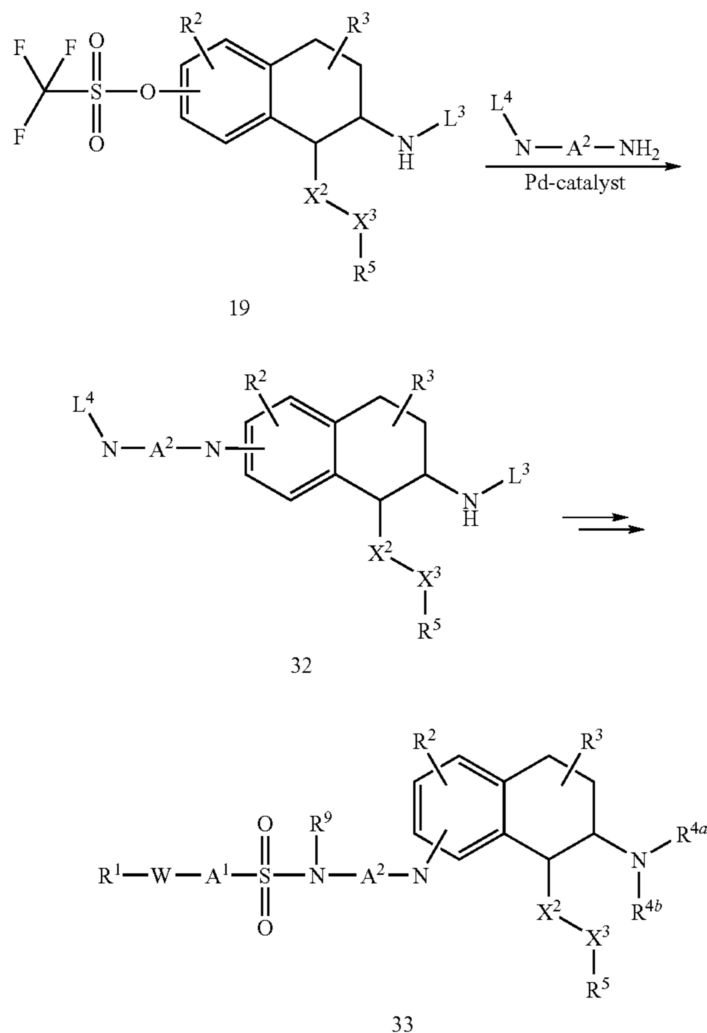
Scheme 6:
