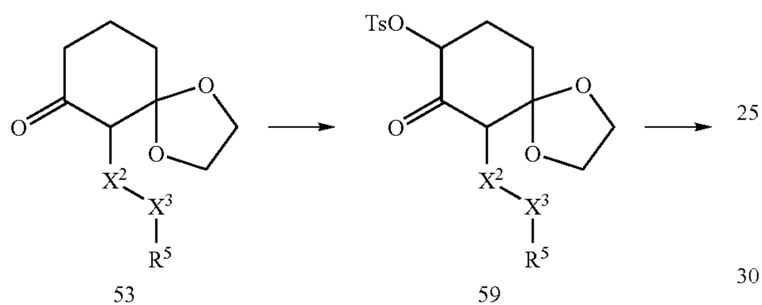
Scheme 14:
