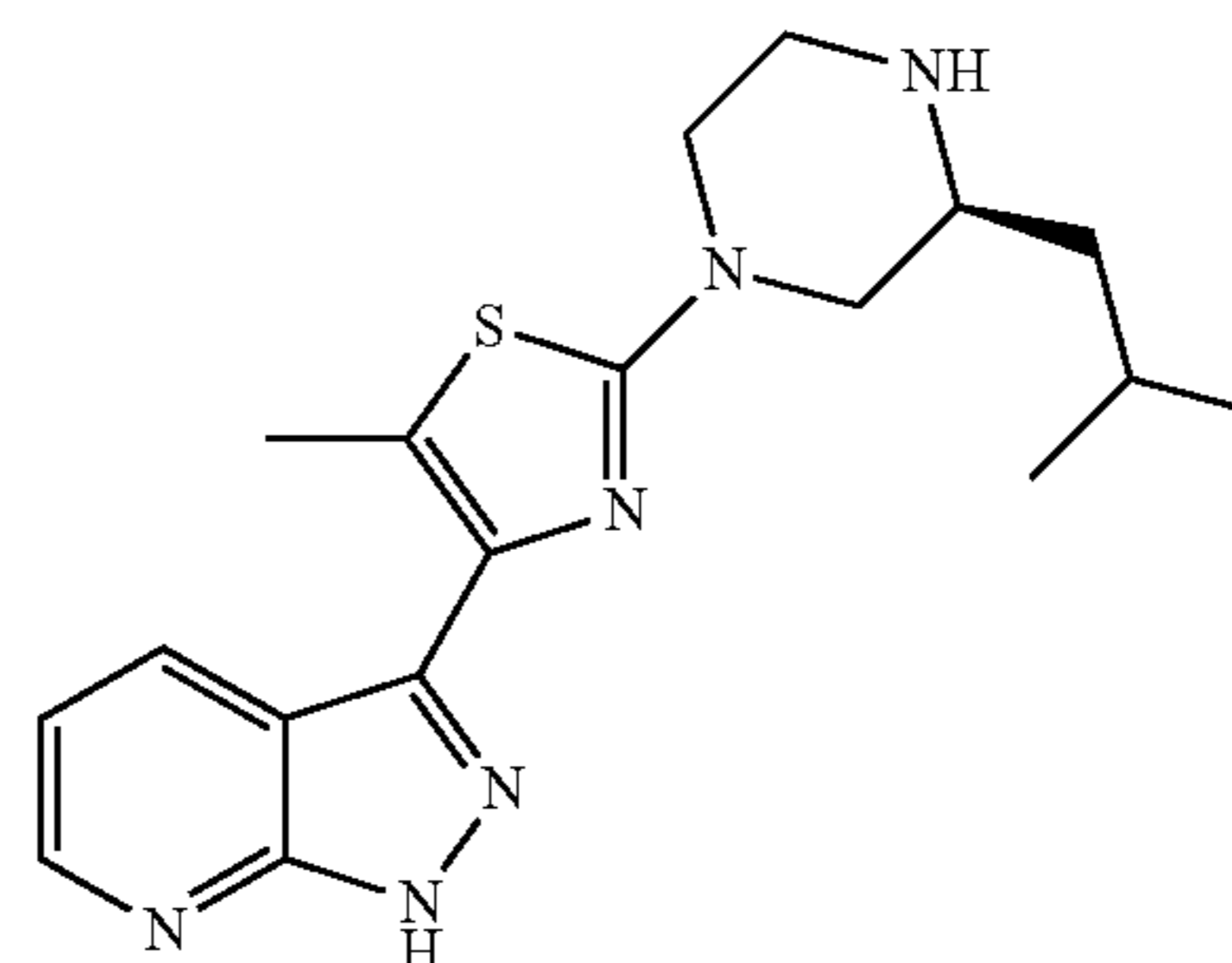
(S)-4-(3-isobutylpiperazin-1-yl)-2-(1H-pyrazolo[3,4-b]pyridin-3-yl)thiazole
