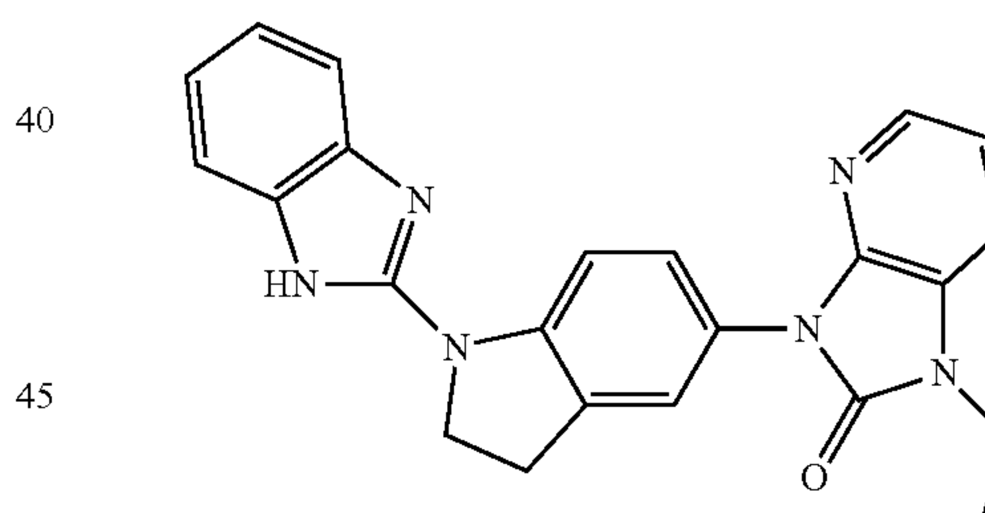
13a) tert-butyl 5-nitro-2,3-dihydro-1H-indole-1-carboxylate
