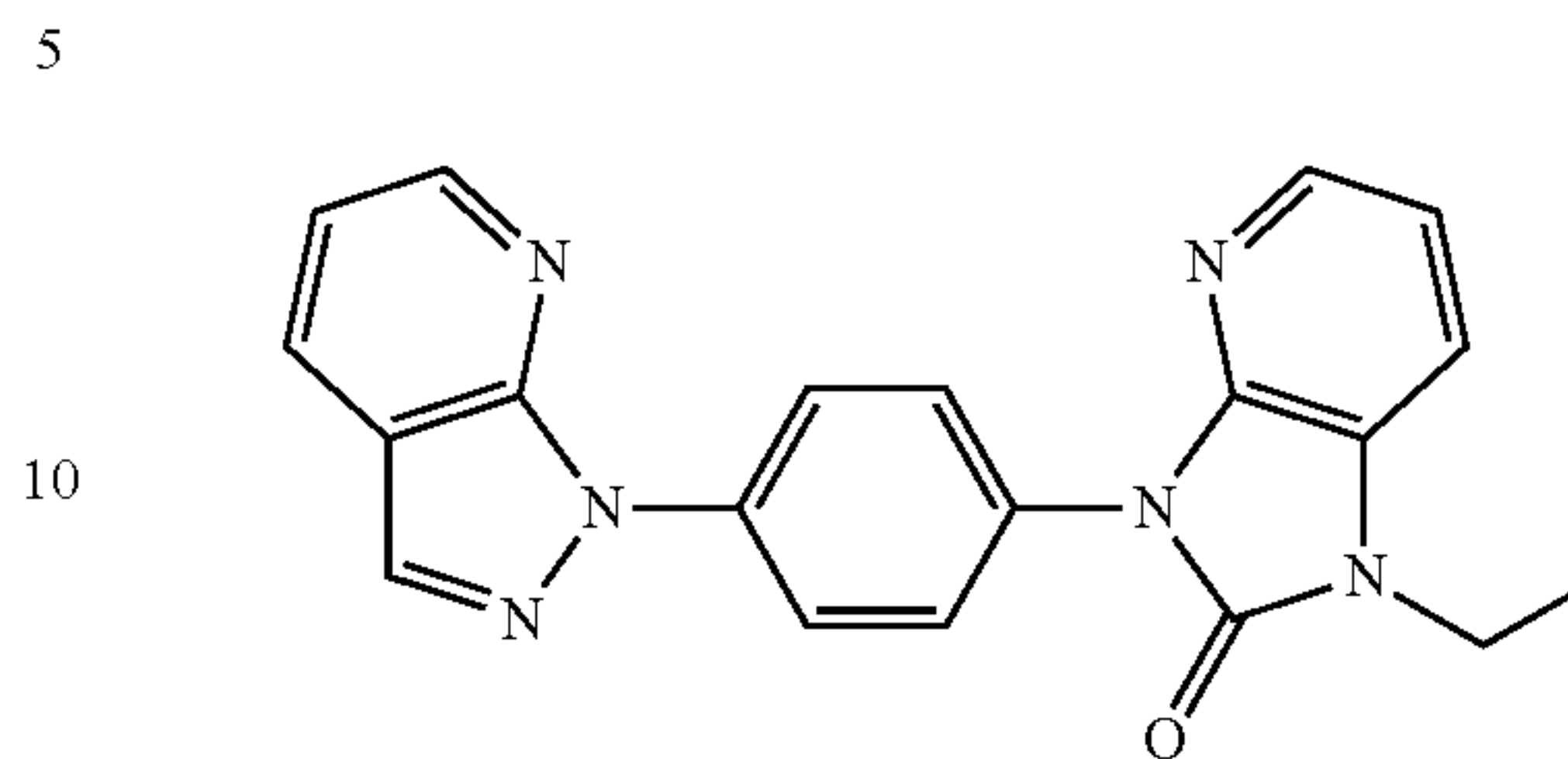
12d) 1-Ethyl-3-[4-(1H-pyrazolo[3,4-b]pyridin-1-yl)phenyl]-1,3-dihydro-2H-imidazo[4,5-b]pyridin-2-one
