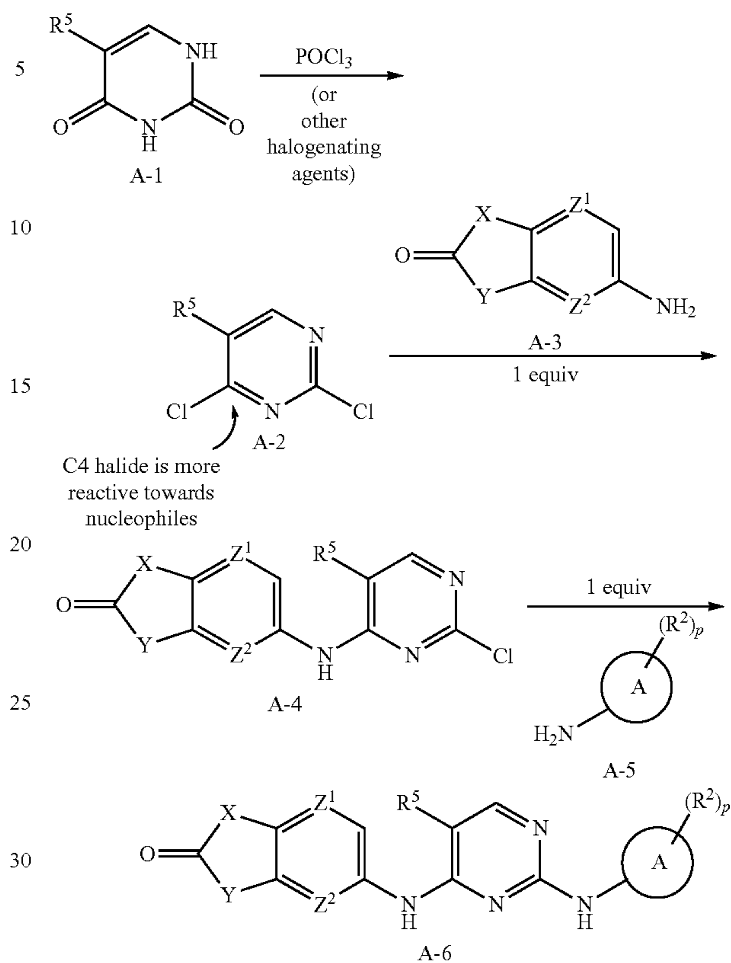
Scheme (I)
