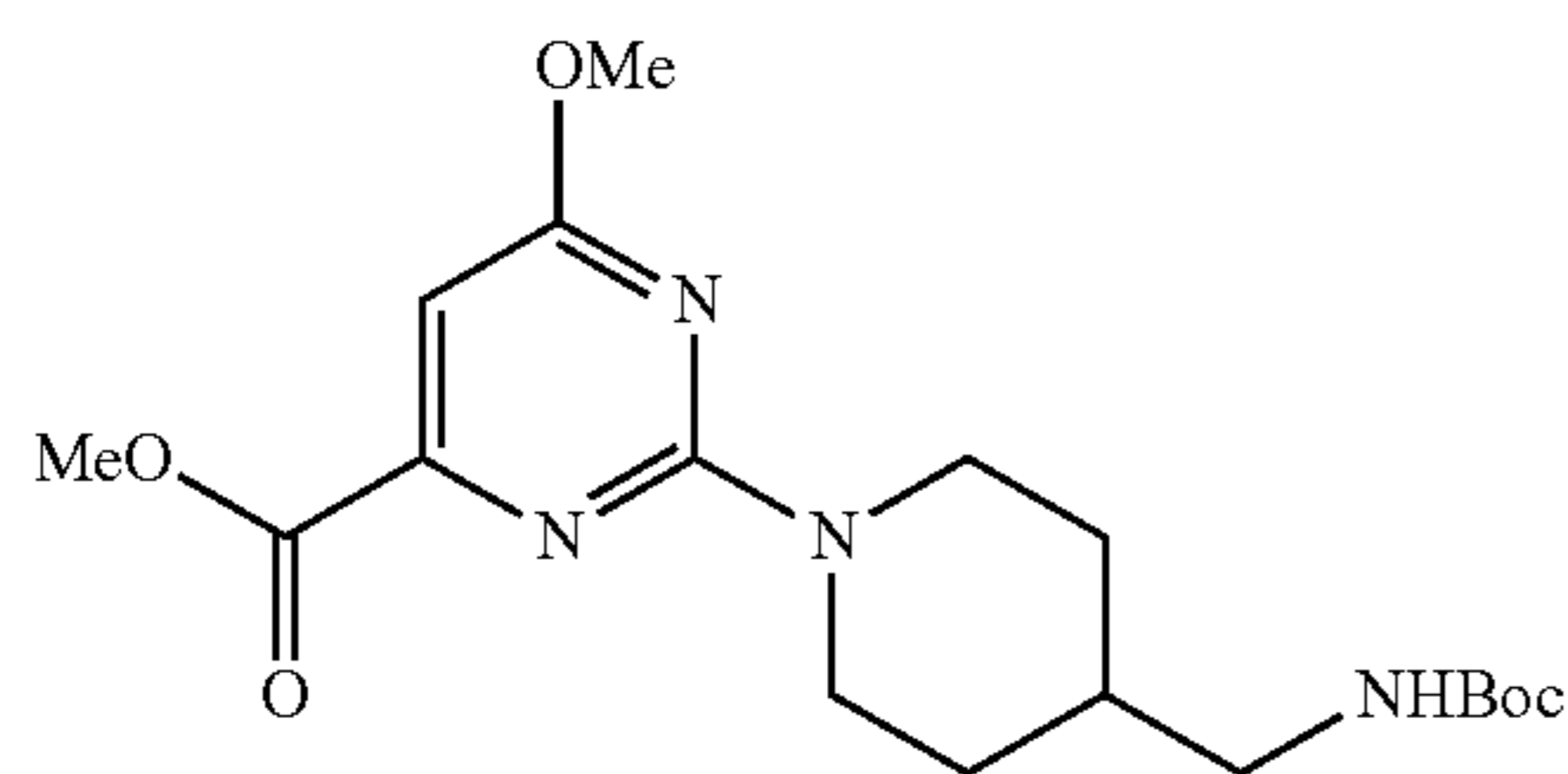
Methyl 2-(4-(((tert-butoxycarbonyl)amino)methyl)piperidin-1-yl)-6-methoxypyrimidine-4-carboxylate
