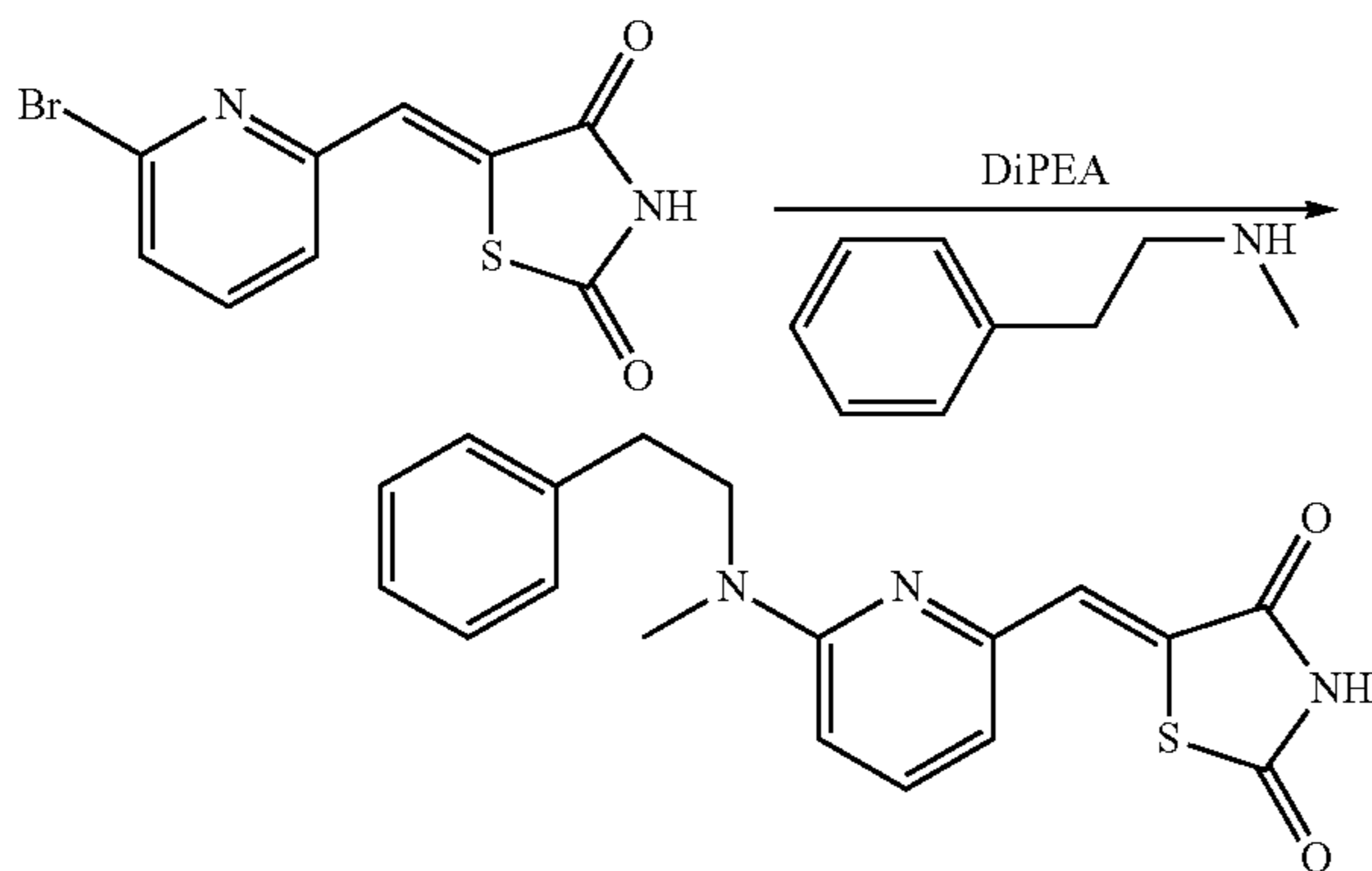
(Z)-5-((6-(methyl(phenethyl)amino)pyridin-2-yl)methylene)thiazolidine-2,4-dione
