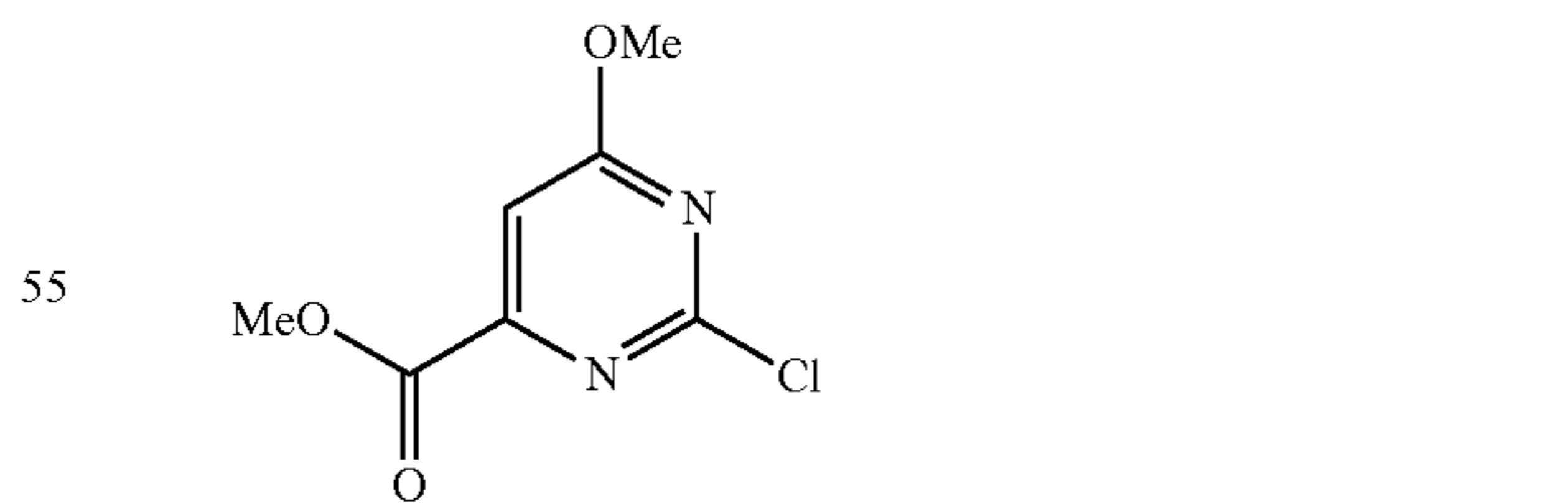
Methyl 2-chloro-6-methoxypyrimidine-4-carboxylate
