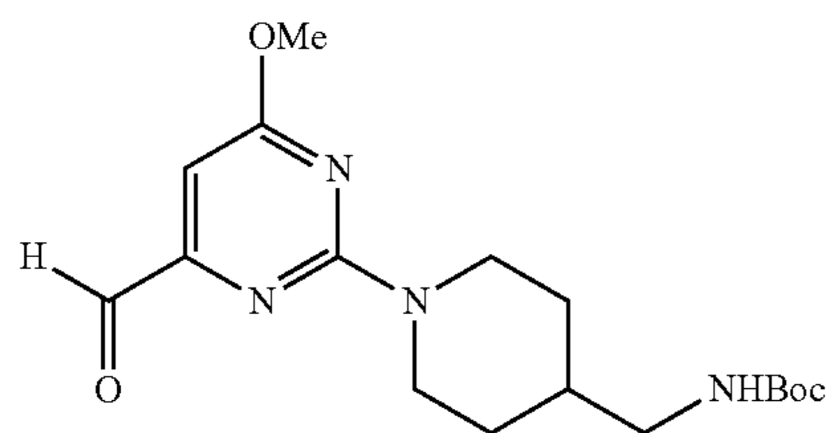
tert-Butyl ((1-(4-formyl-6-methoxypyrimidin-2-yl)piperidin-4-yl)methyl)carbamate
