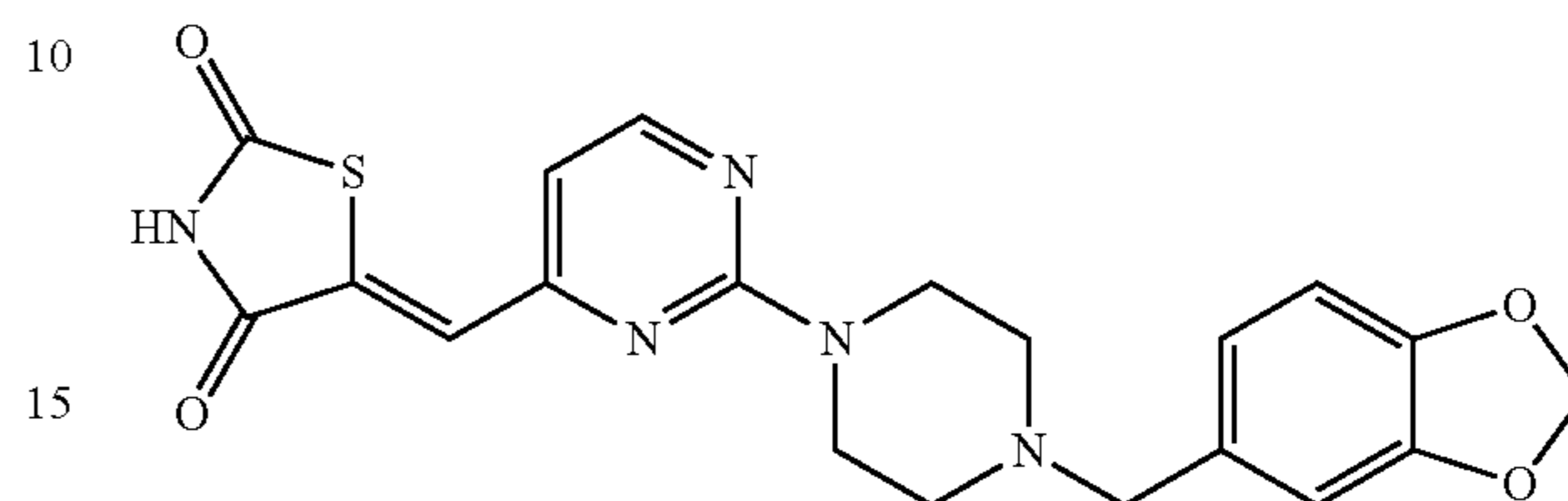
(Z)-5-((2-(methylsulfonyl)pyrimidin-4-yl)methylene)thiazolidine-2,4-dione (6)
