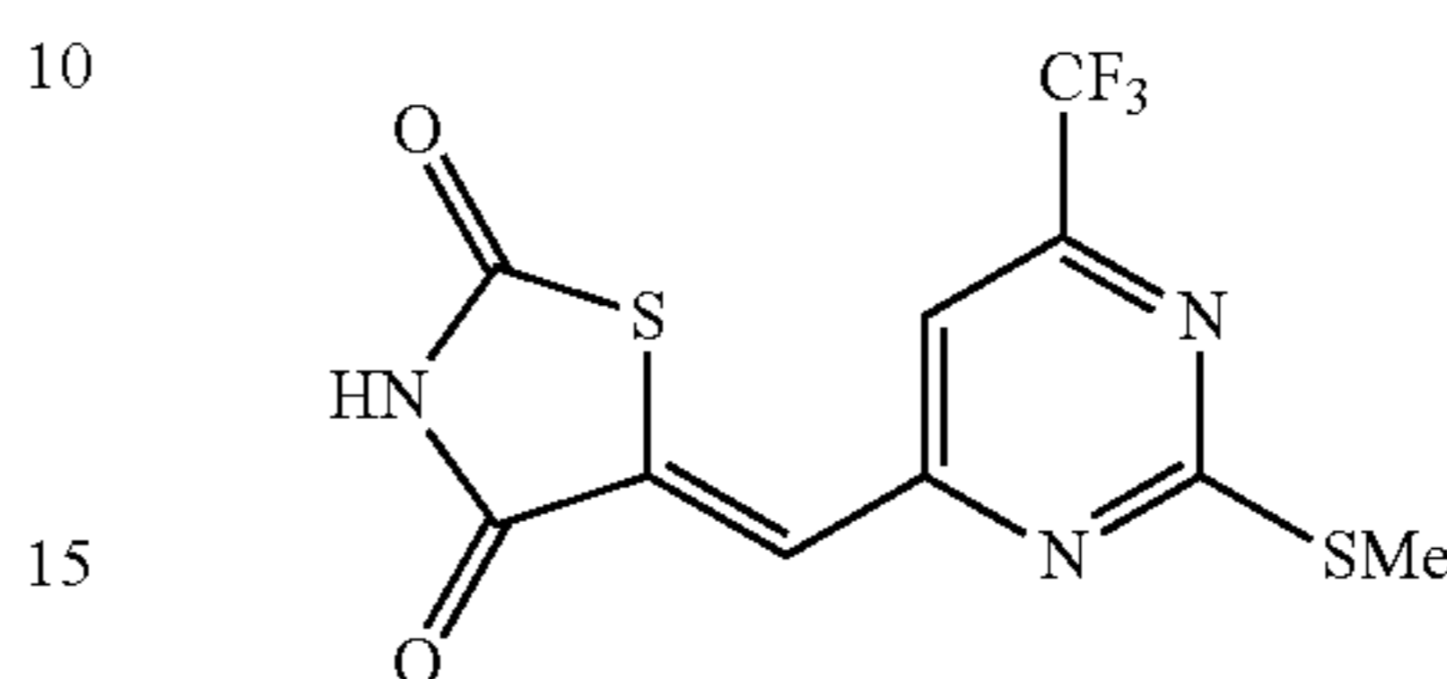
(Z)-5-((2-(Methylthio)-6-(trifluoromethyl)pyrimidin-4-yl)methylene)thiazolidine-2,4-dione
