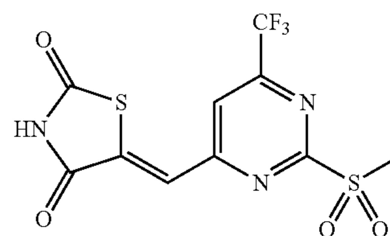
(Z)-5-((2-(Methylsulfonyl)-6-(trifluoromethyl)pyrimidin-4-yl)methylene)thiazolidine-2,4-dione
