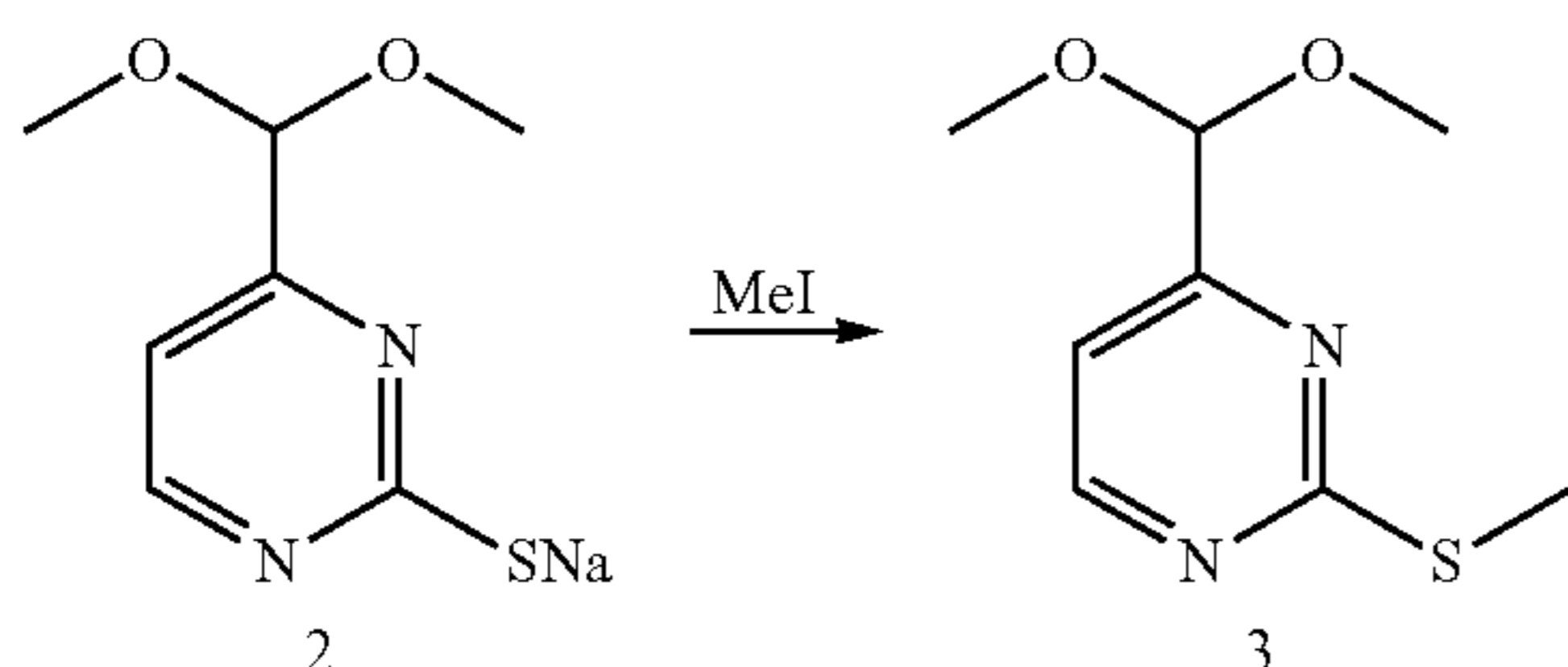
4-(dimethoxymethyl)-2-(methylthio)pyrimidine (3)
