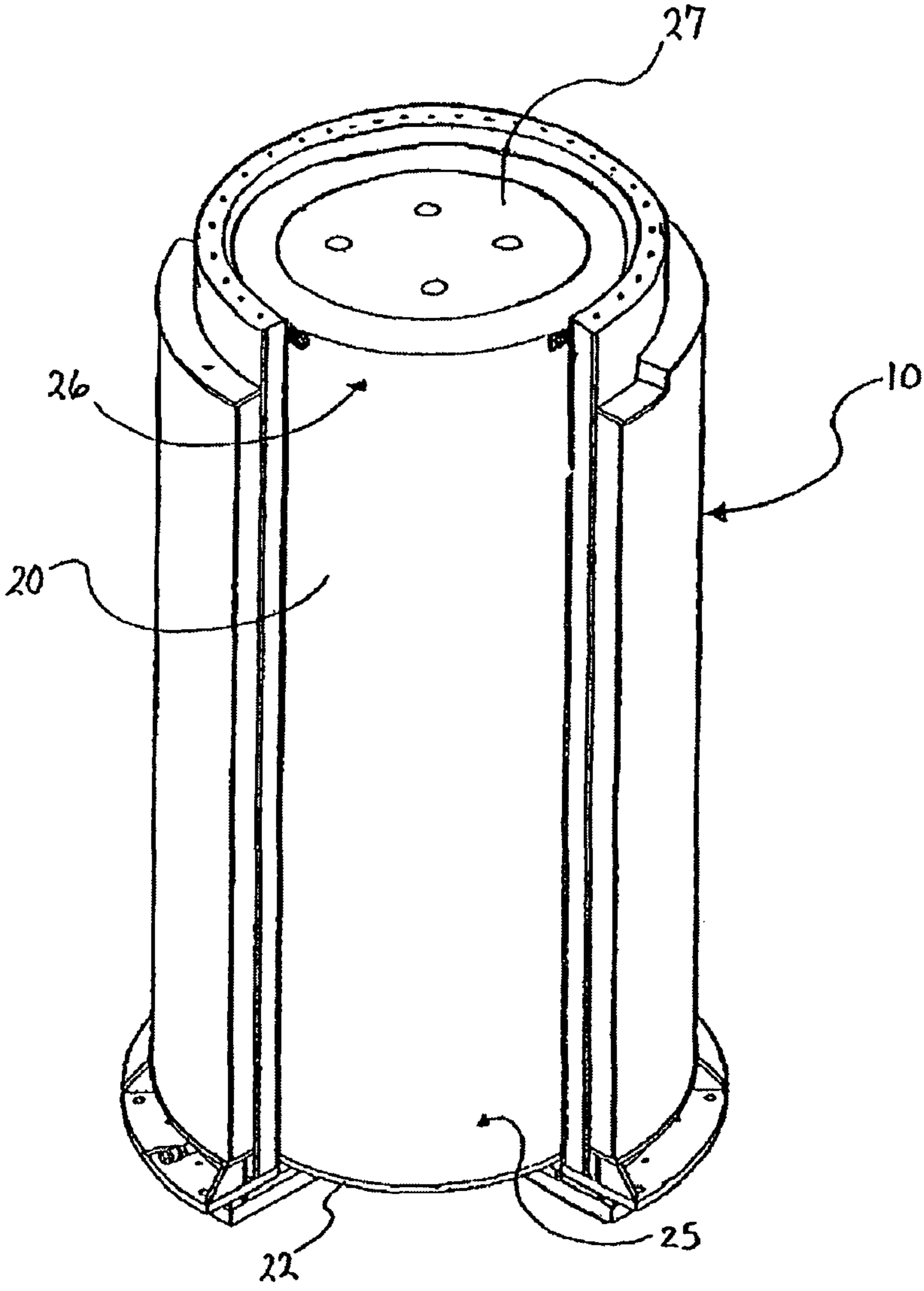
FIGURE 3 (PRIOR ART)
