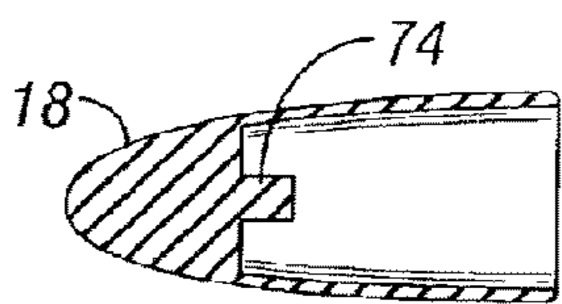
FIG. 7 (PRIOR ART)
