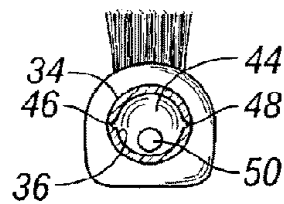
FIG. 8 (PRIOR ART)
