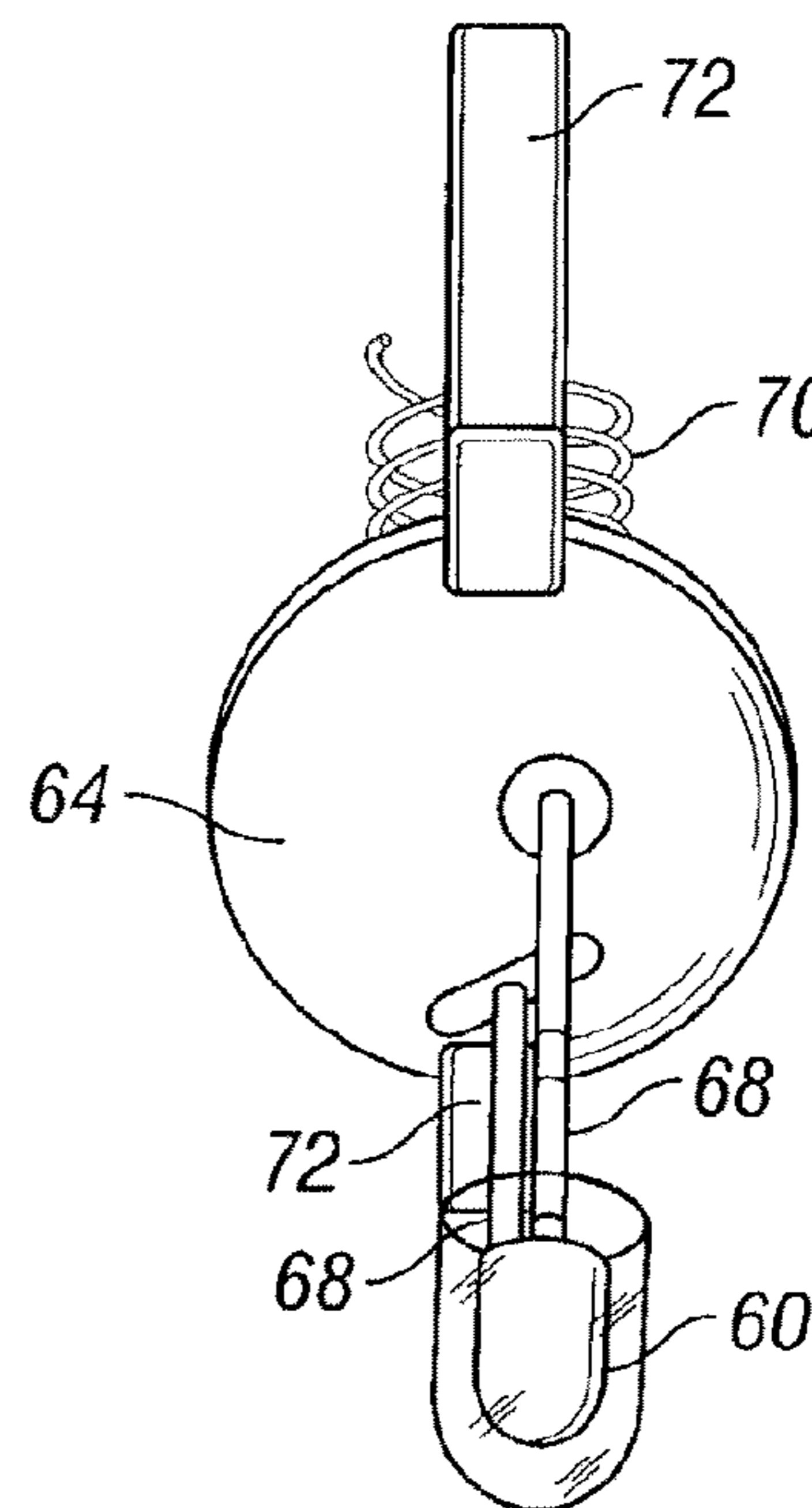
FIG. 11 (PRIOR ART)
