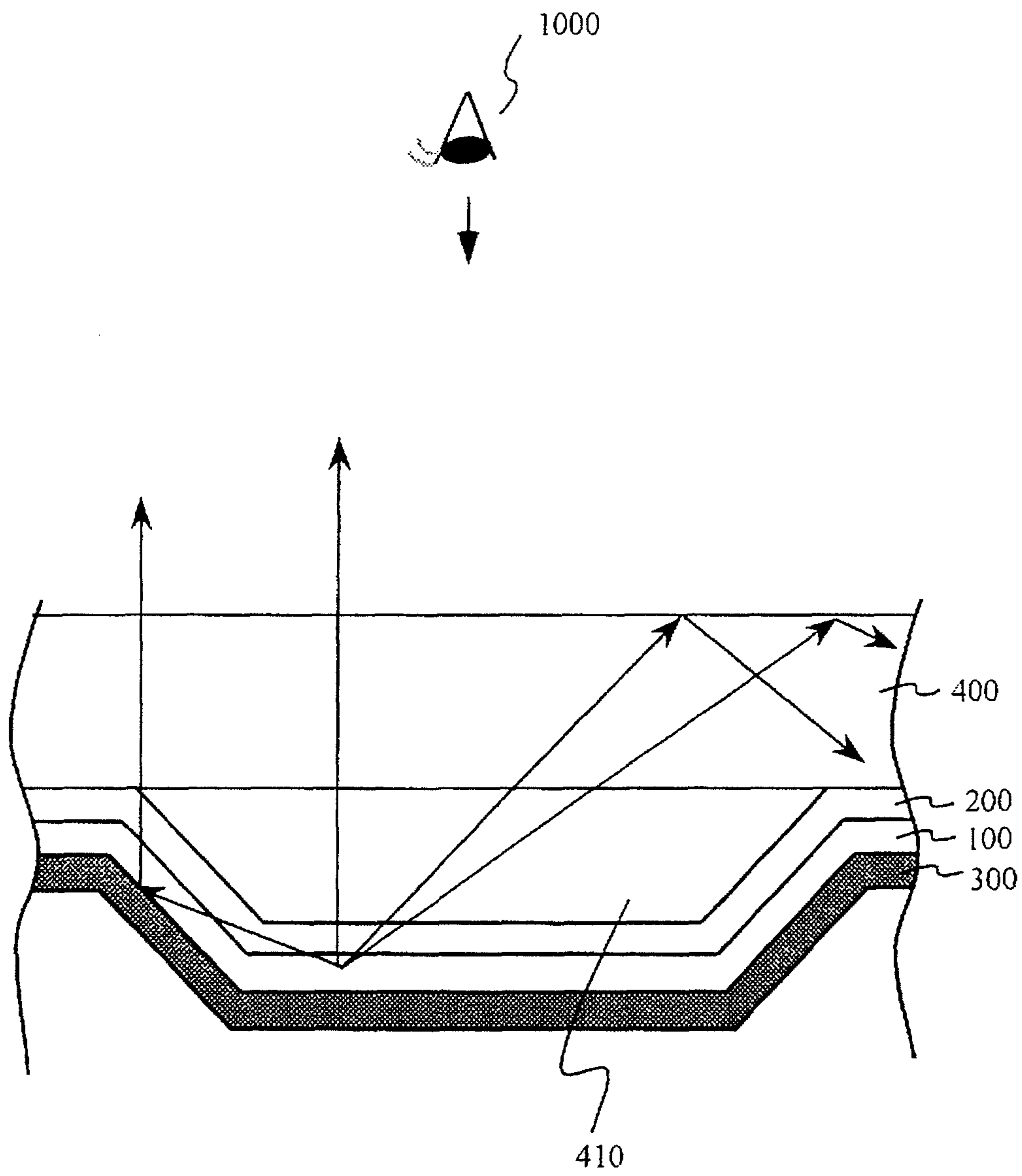
FIG. 34 PRIOR ART
