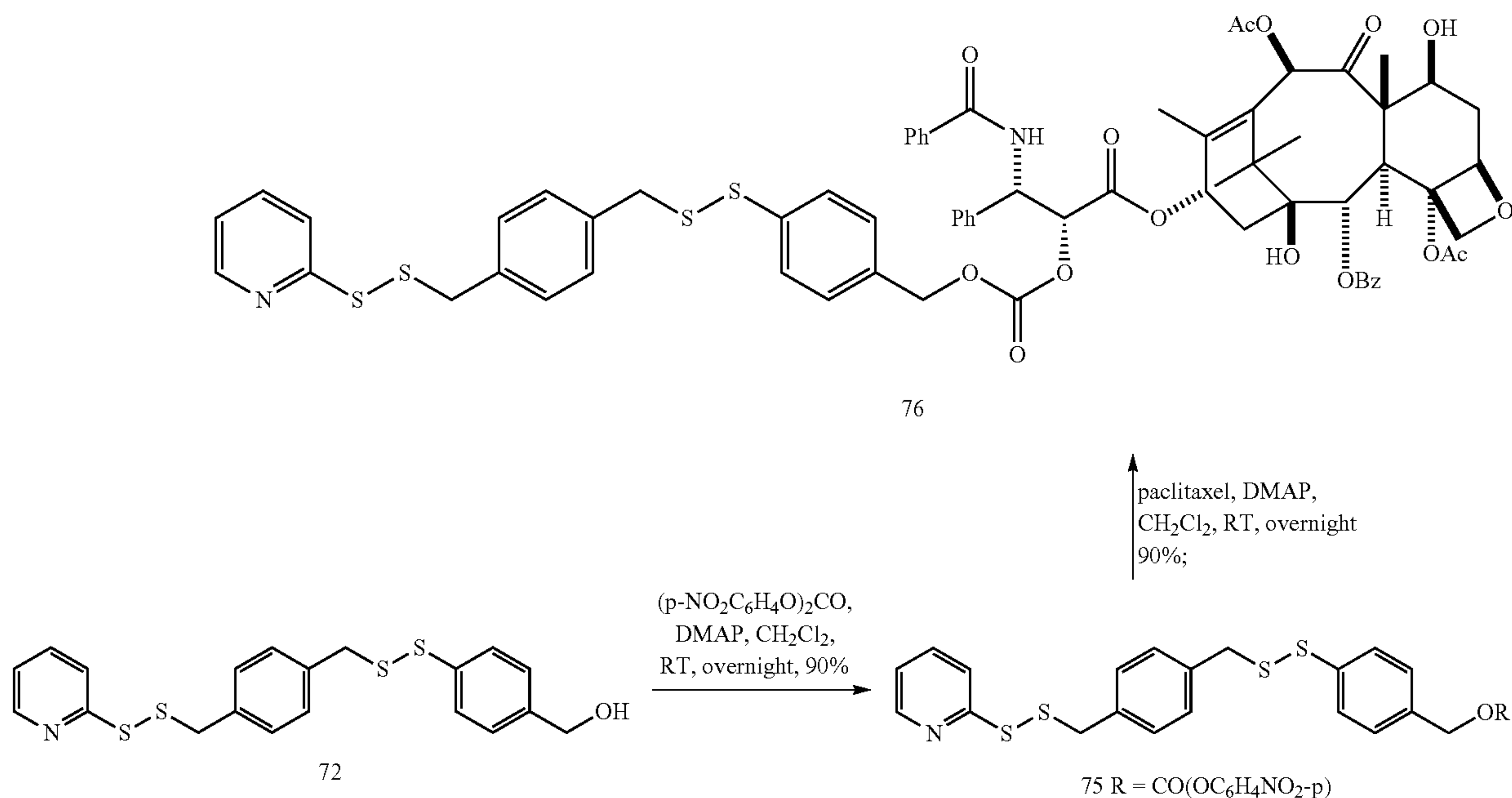
Scheme 17.3
