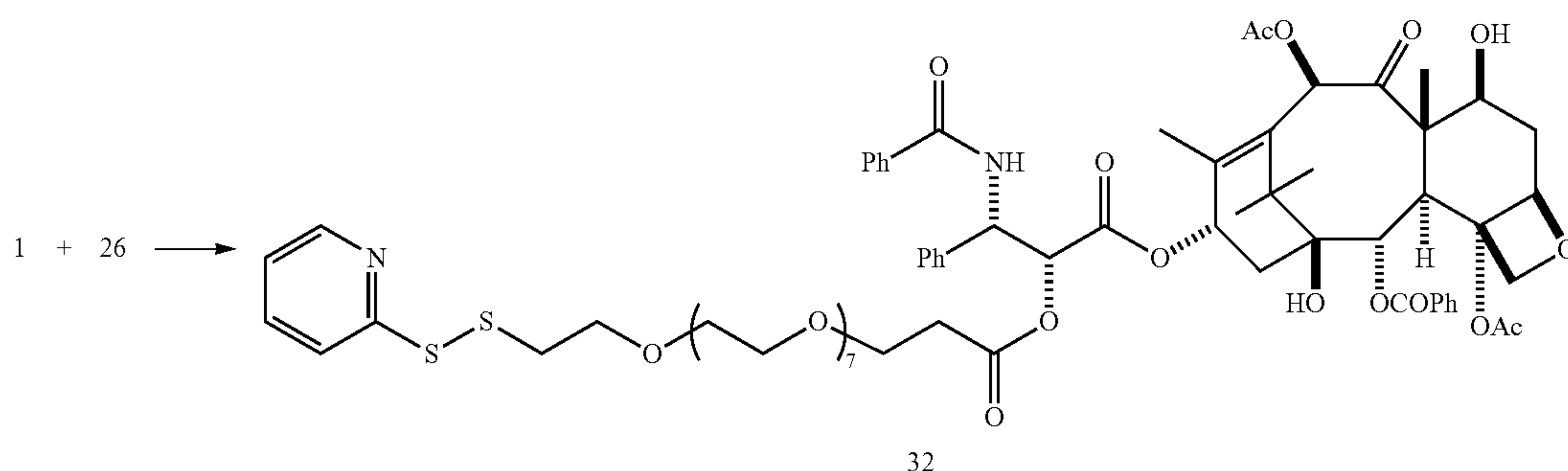
Scheme 6.3
