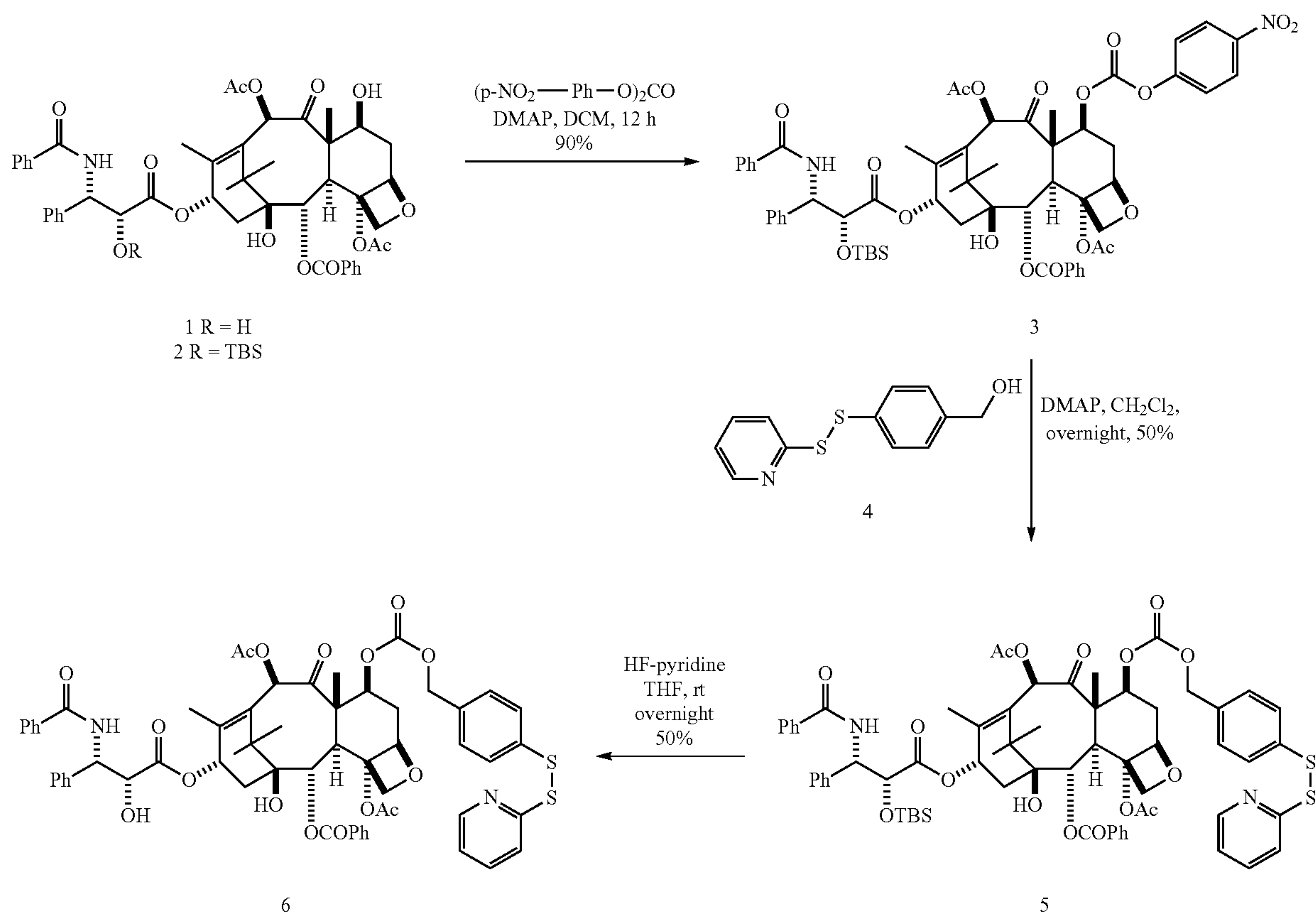
Scheme 1.1
