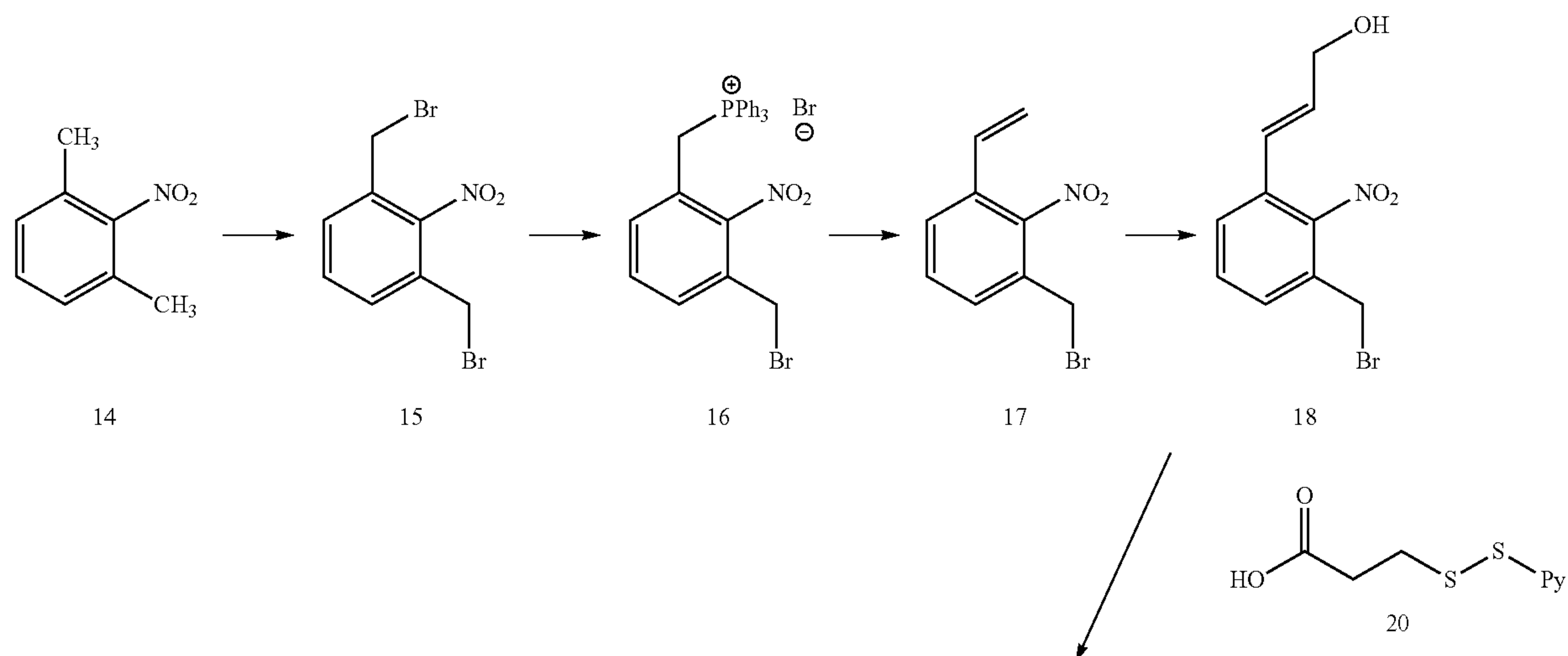
Scheme 3.3
