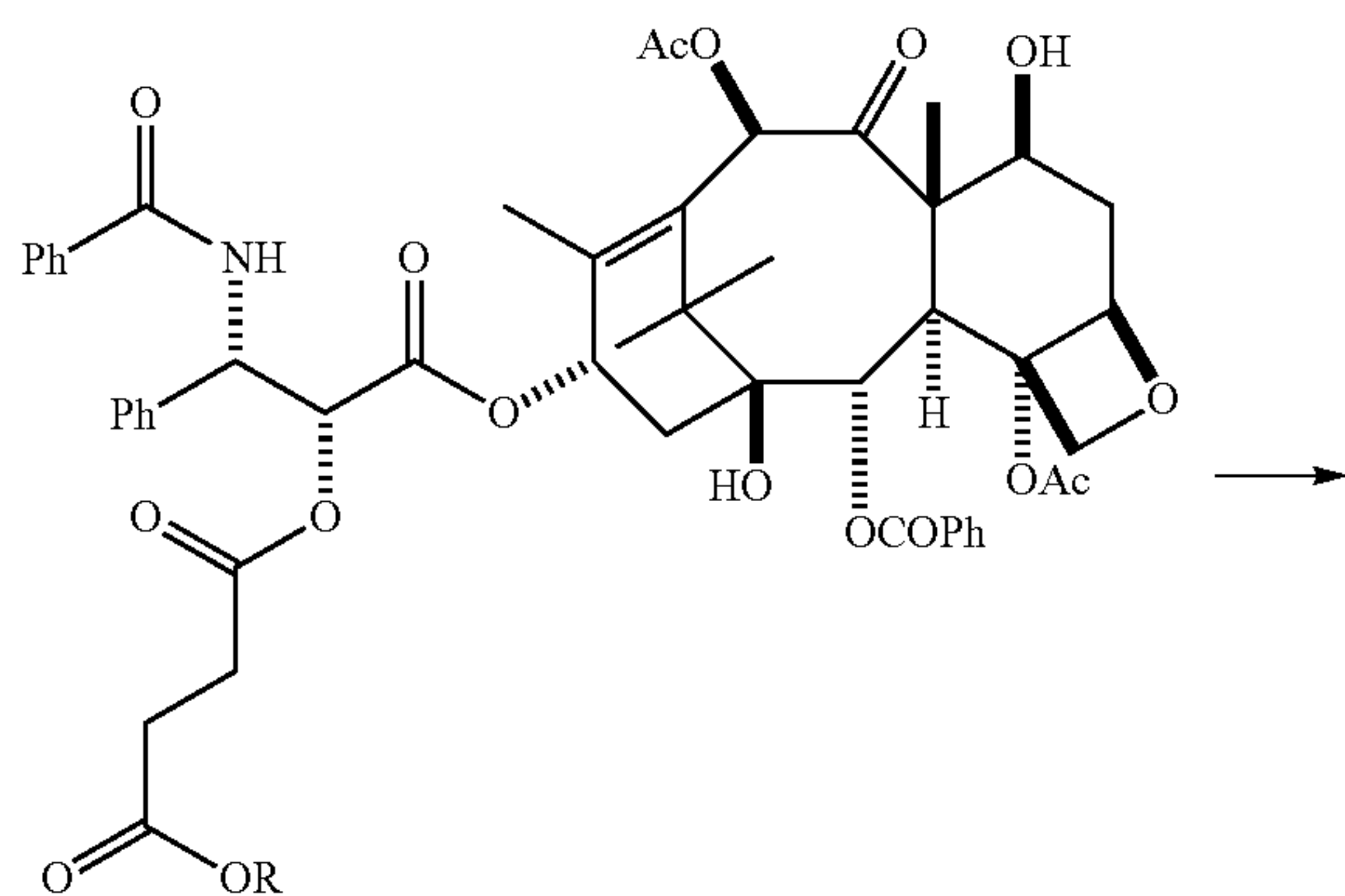
Scheme 10.3
