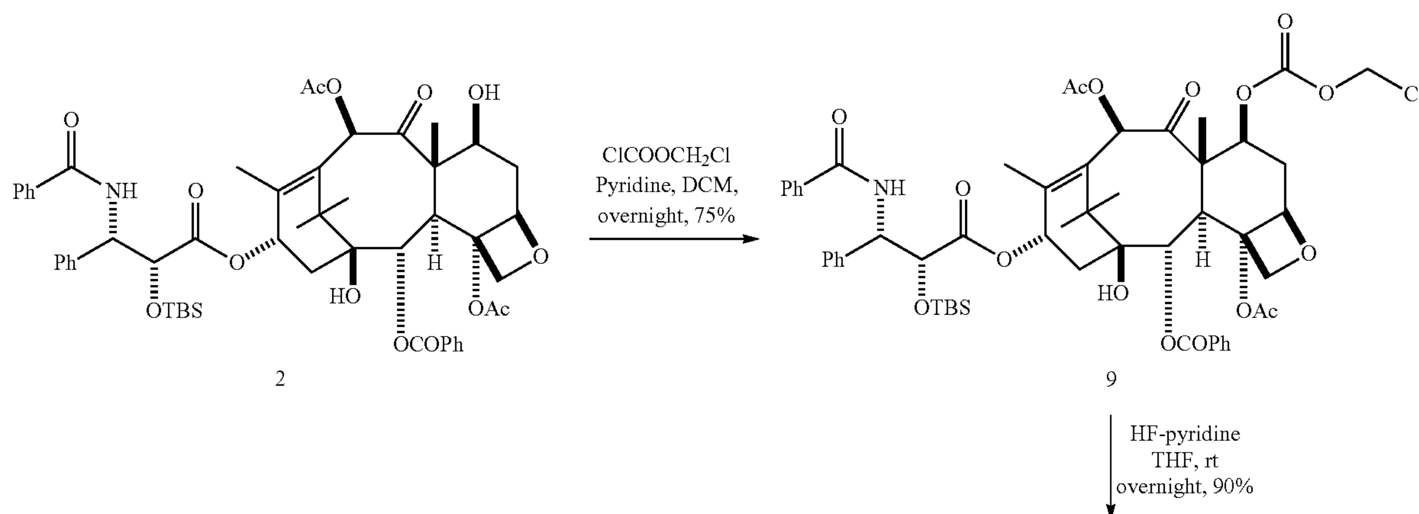
Scheme 2.1
