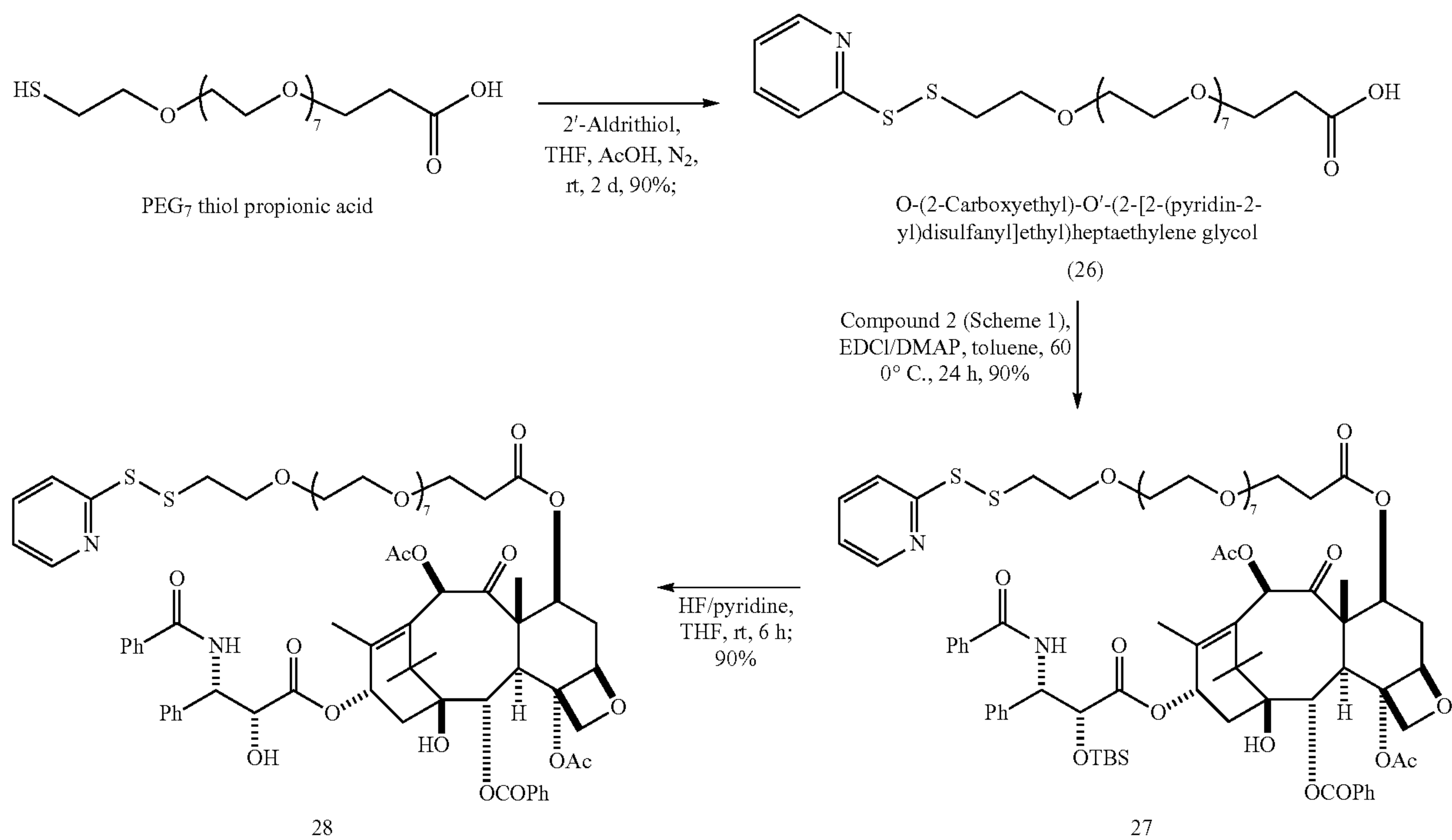
Scheme 6.1
