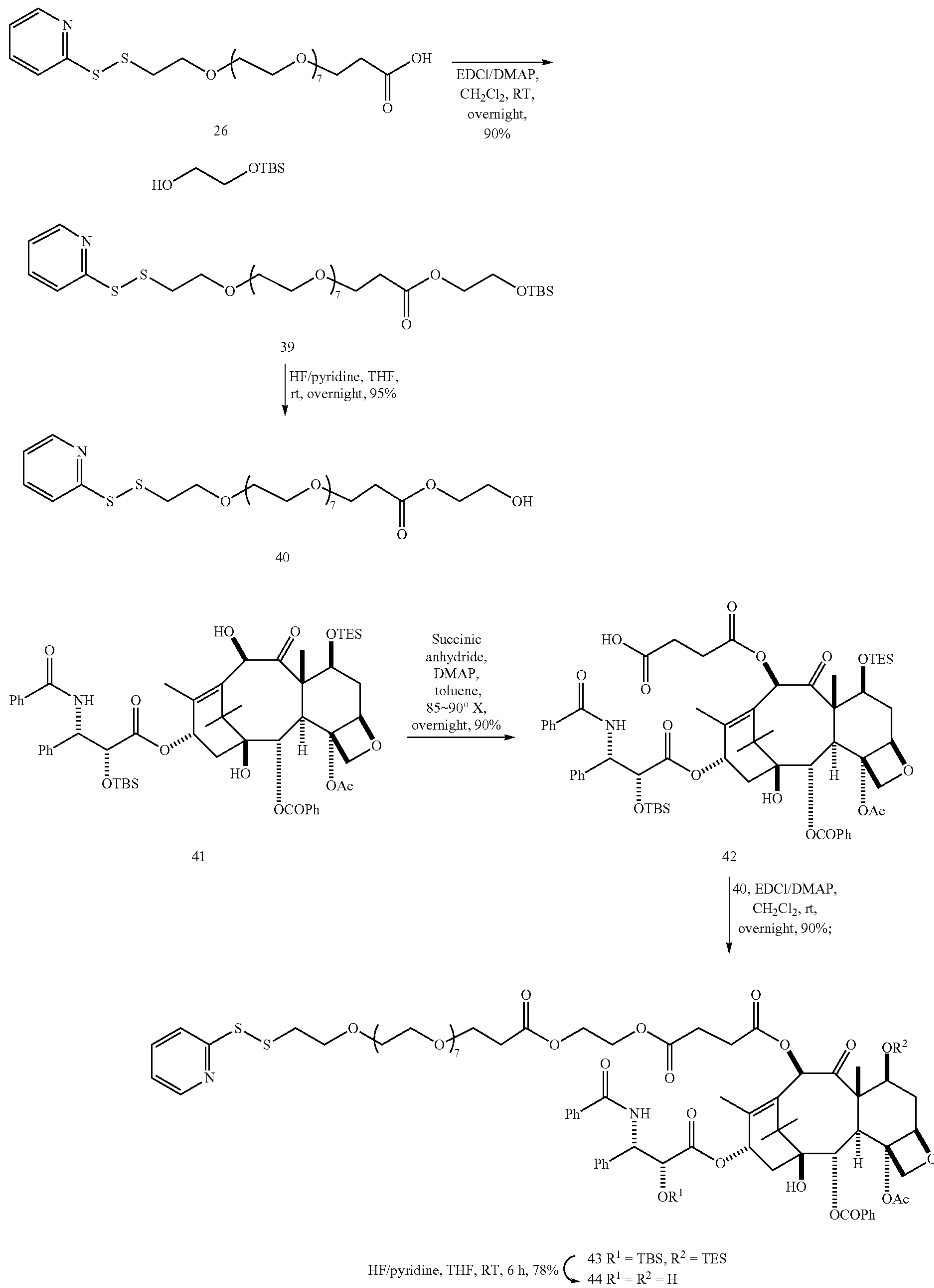
Scheme 8.2
