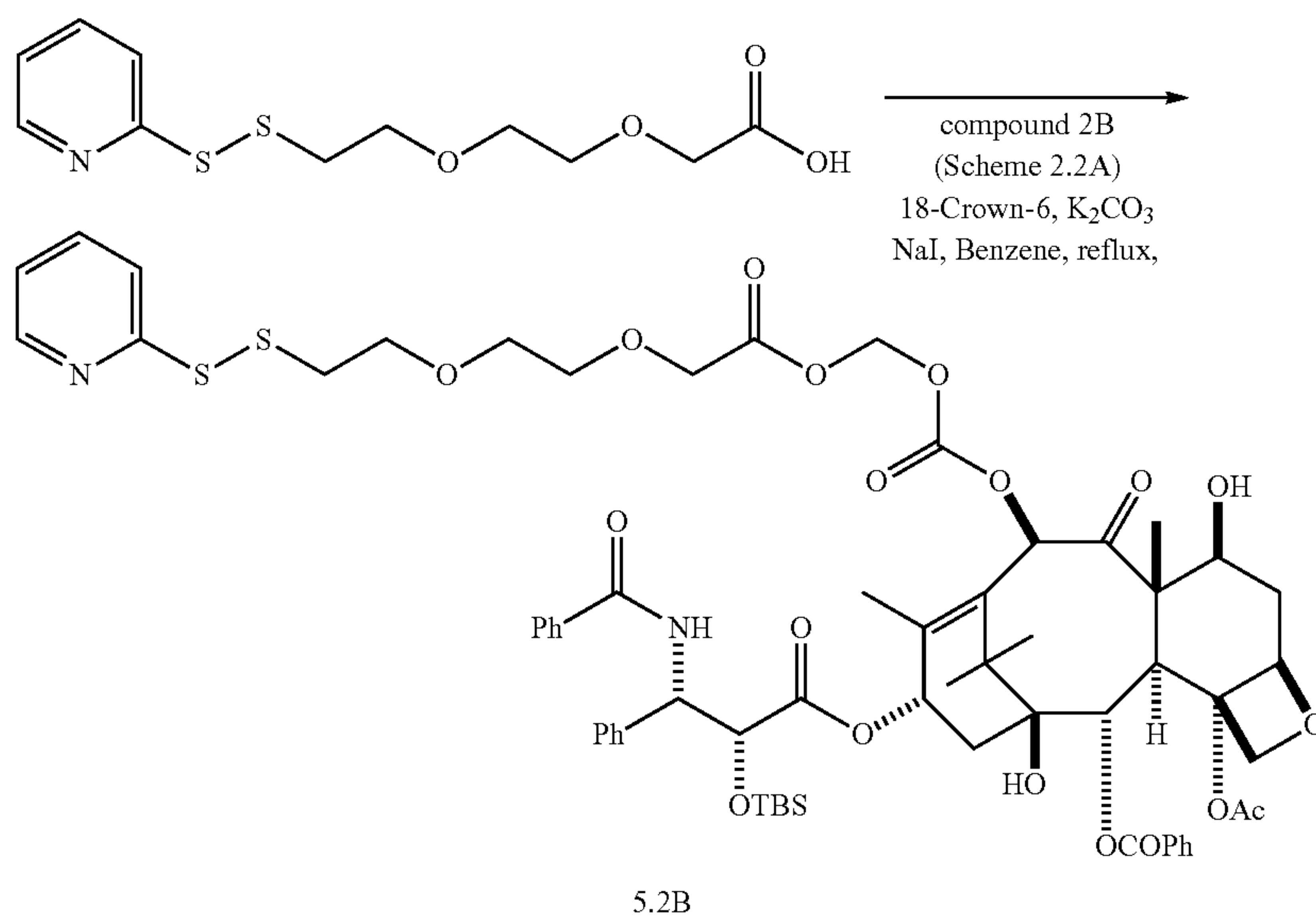
Scheme 5.2
