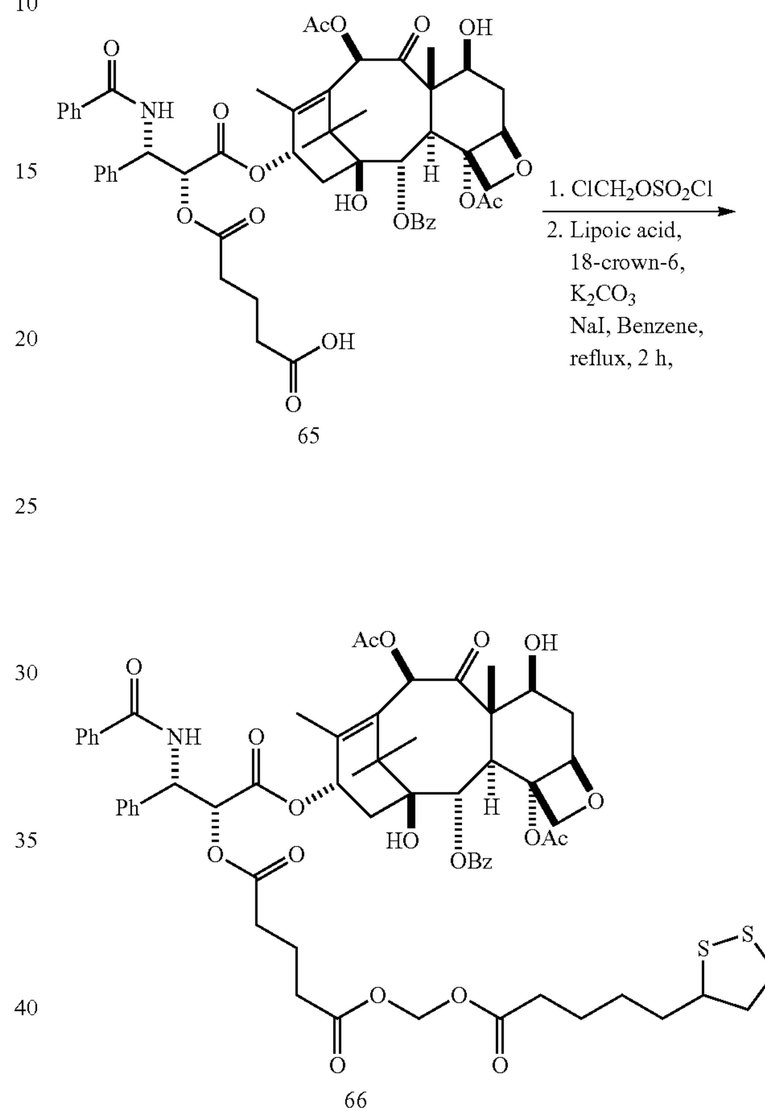
Scheme 12.3
