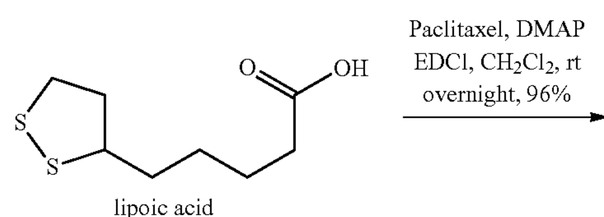
Scheme 14.3
