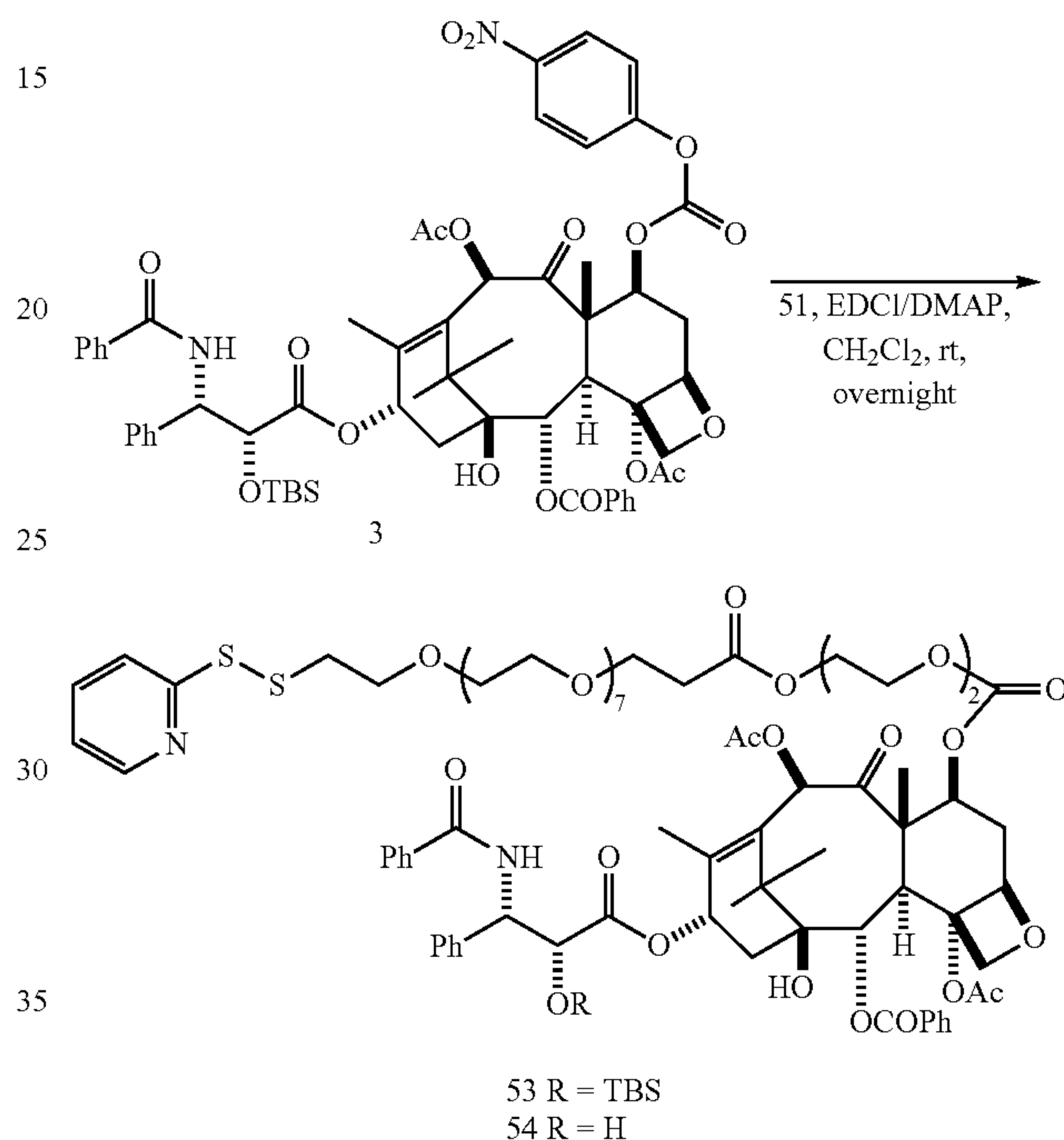
Scheme 9.1
