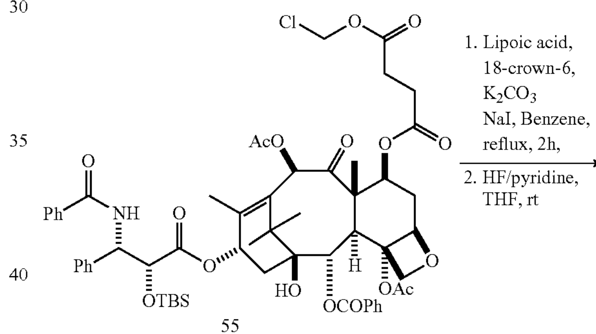
Scheme 11.1
