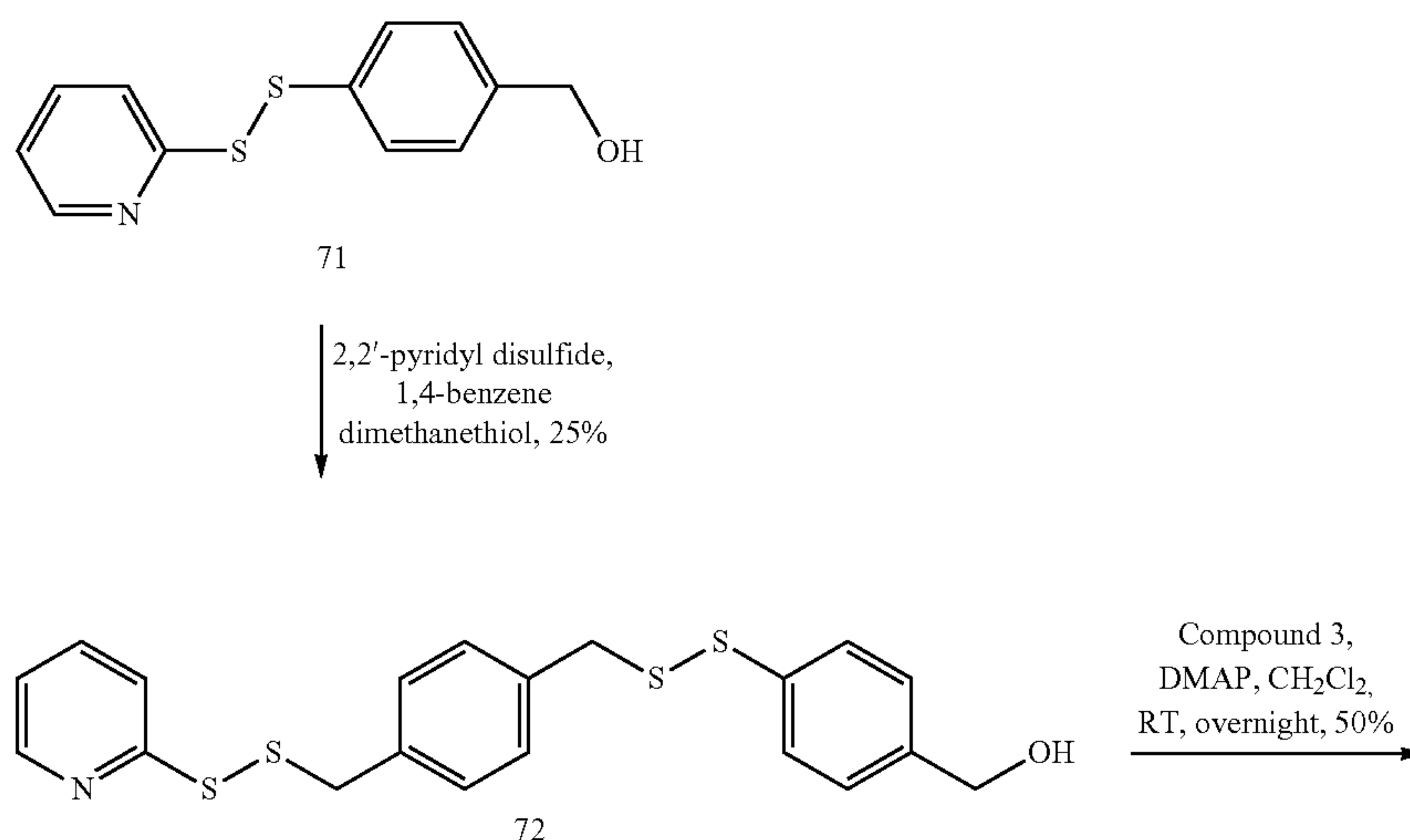
Scheme 17.1
