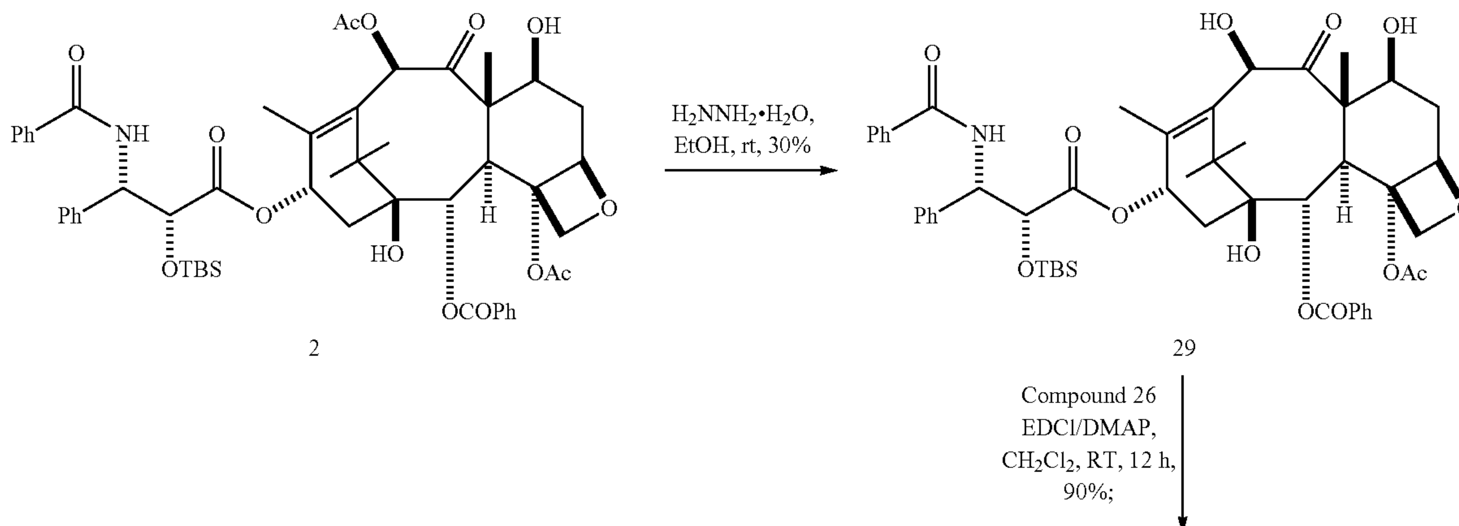
Scheme 6.2
