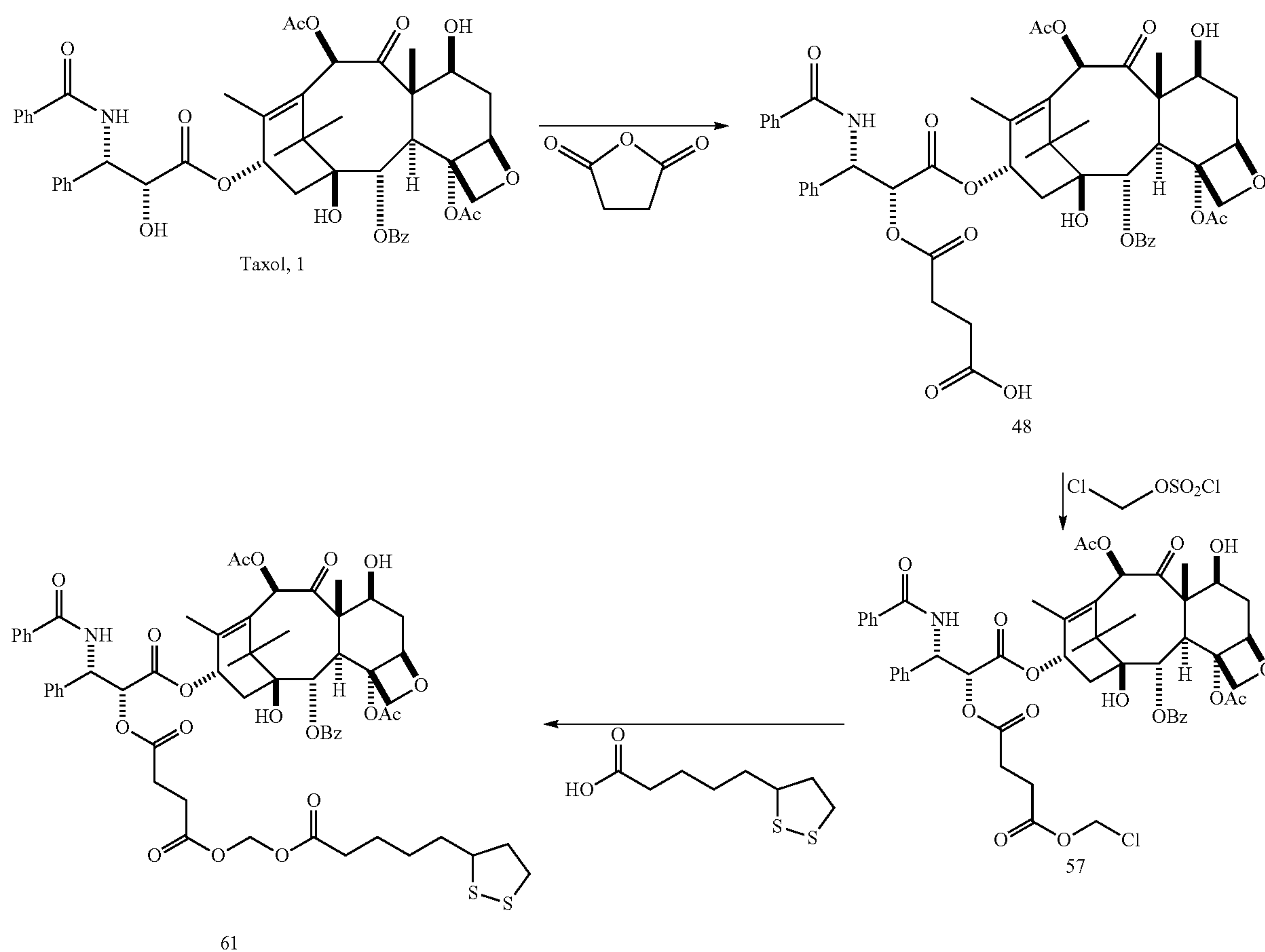
Scheme 11.3
