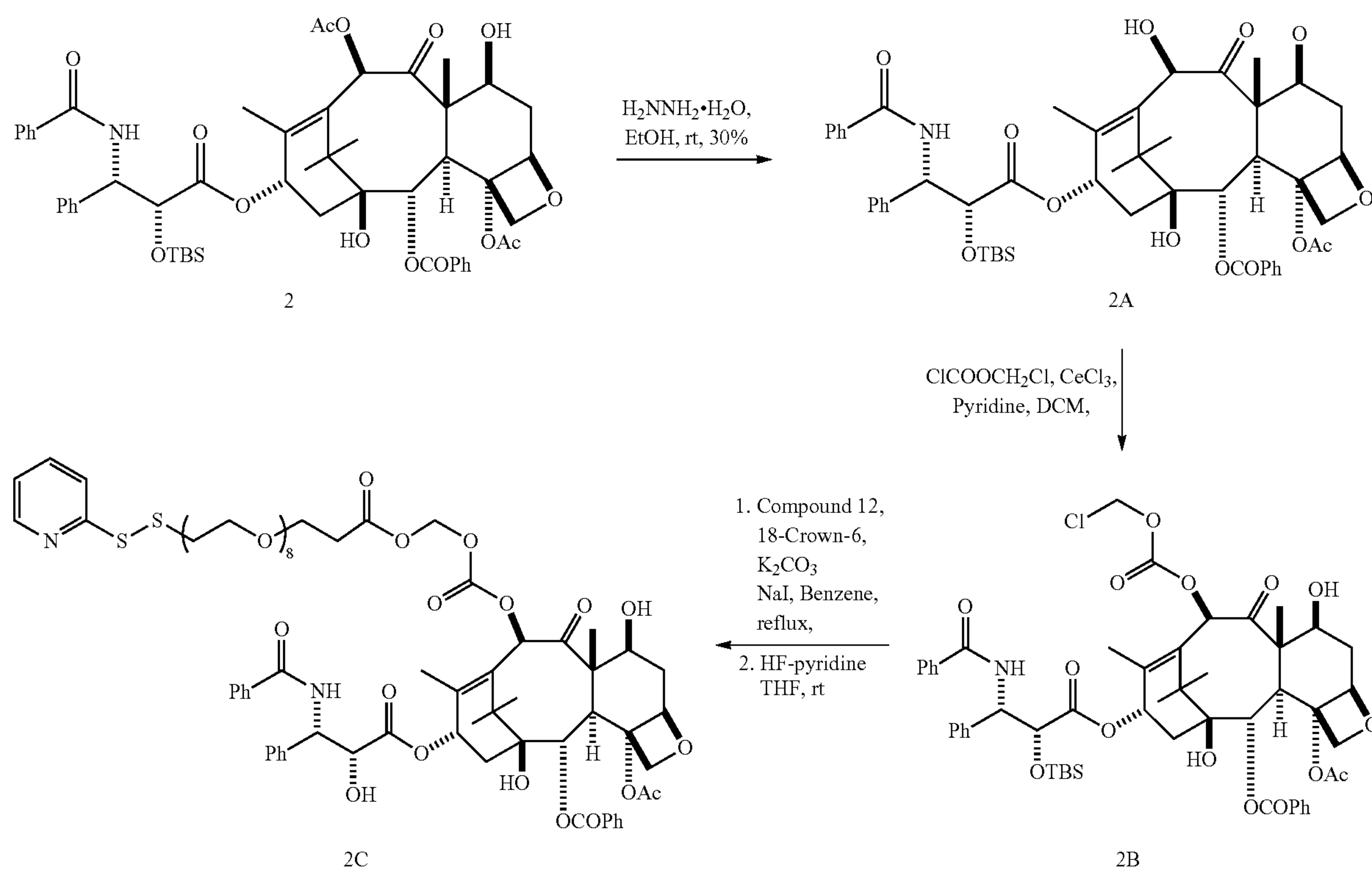
Scheme 2.2A
