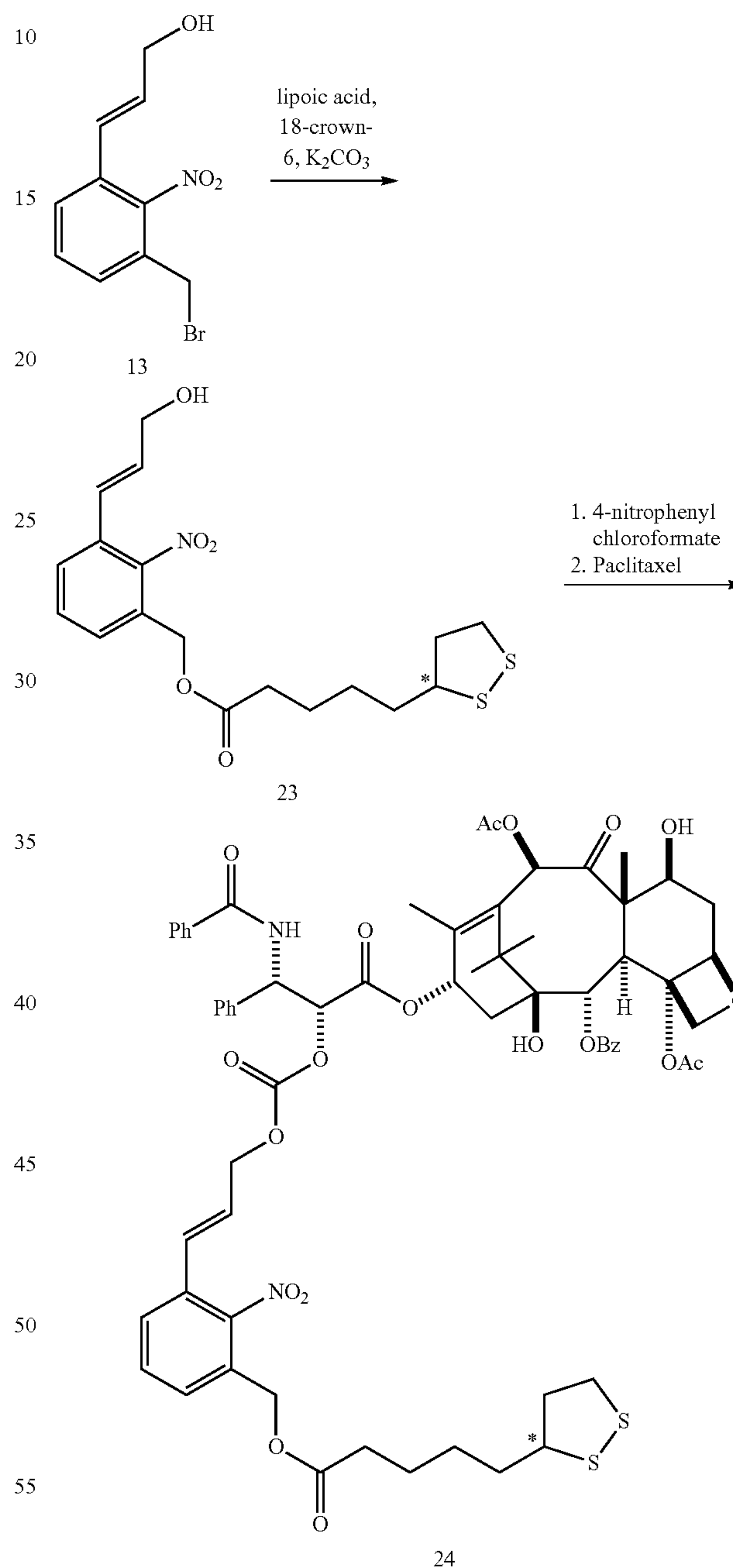
Scheme 4.3
