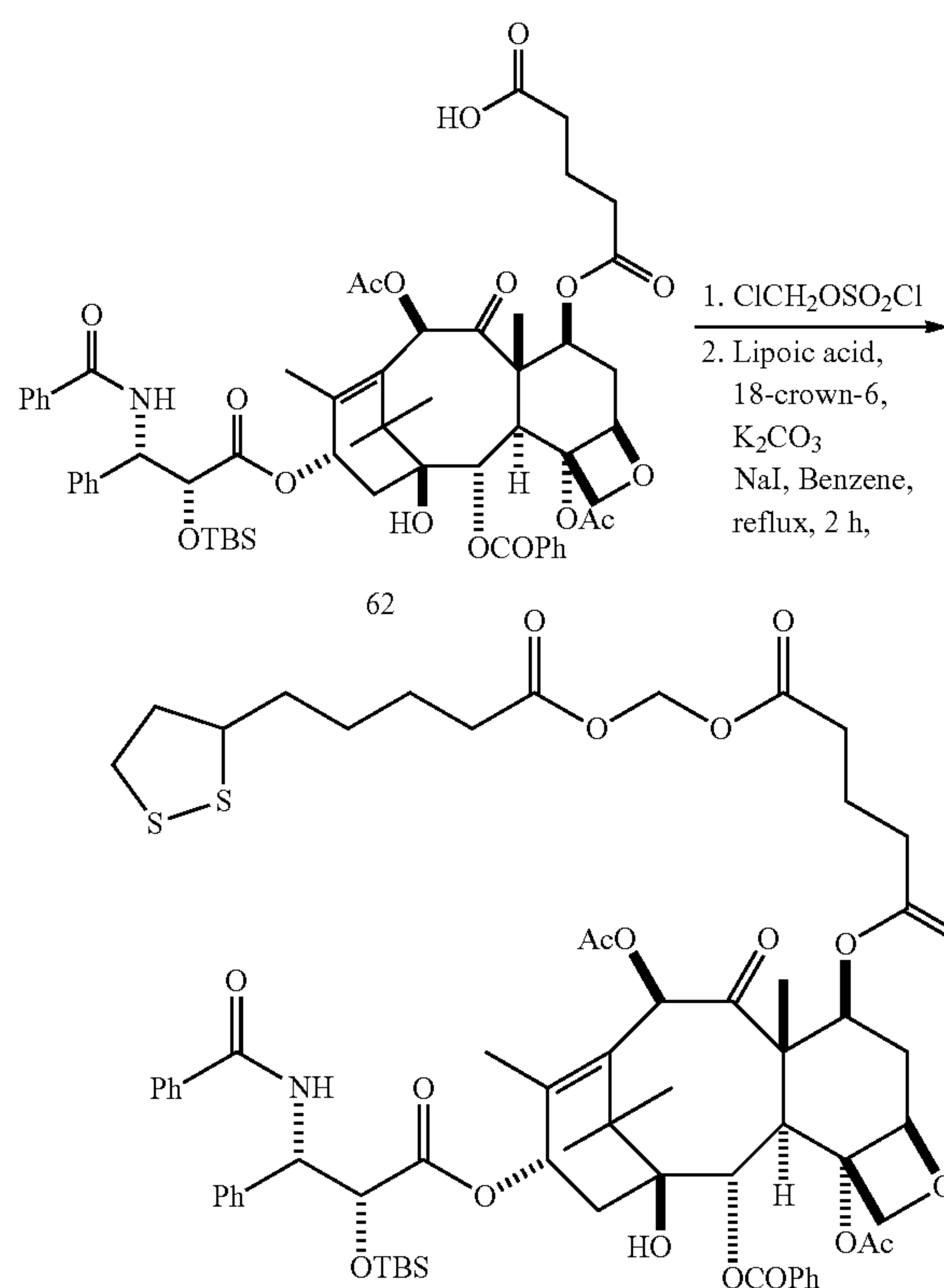
Scheme 12.1
