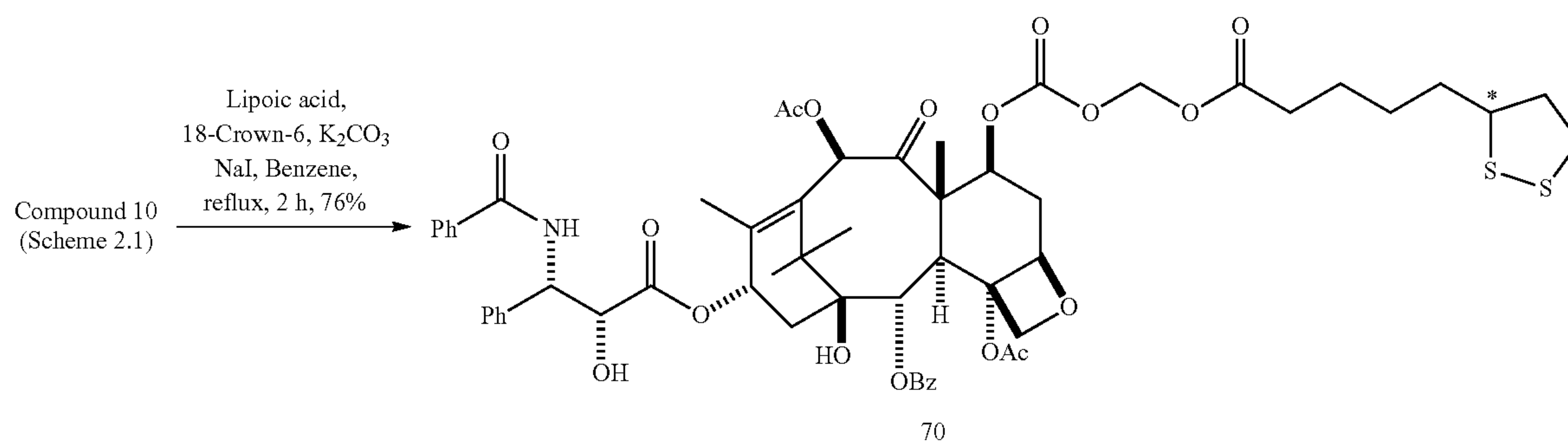
Scheme 15.1
