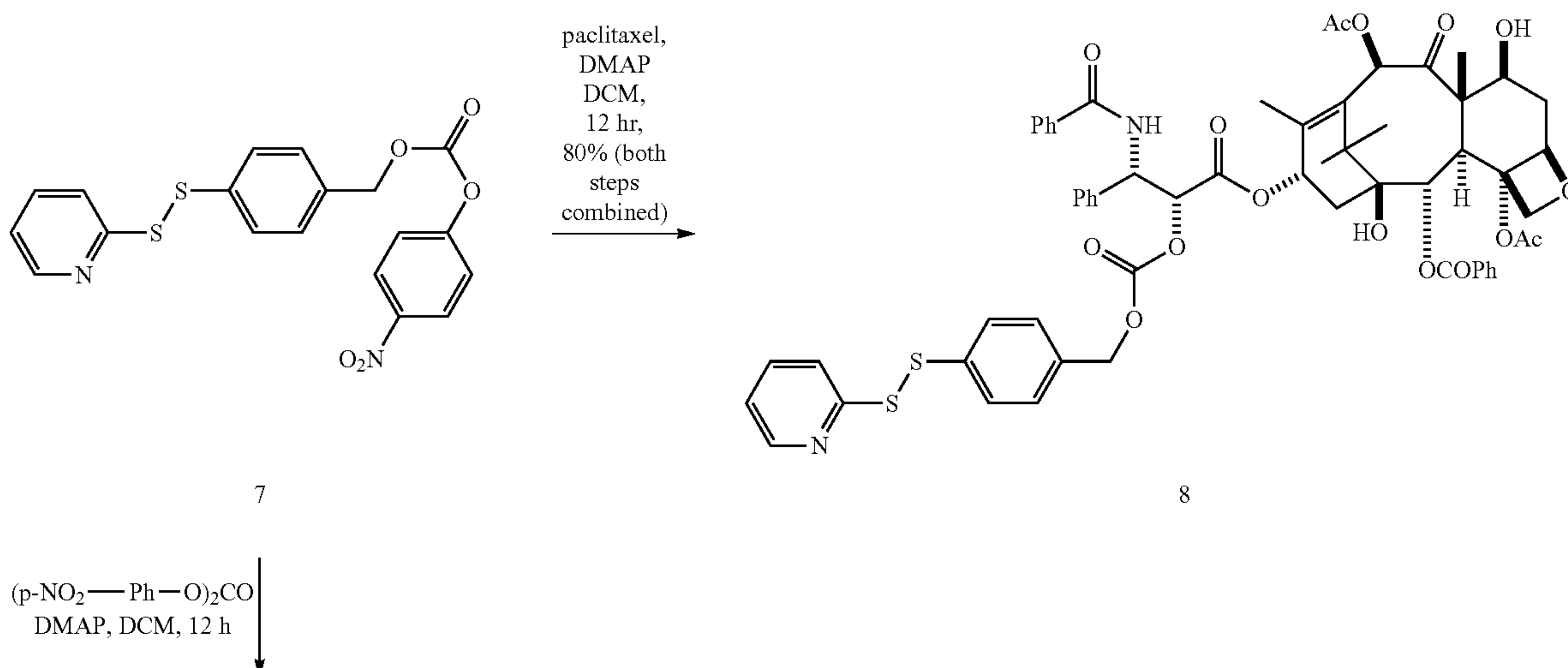
Scheme 1.3
