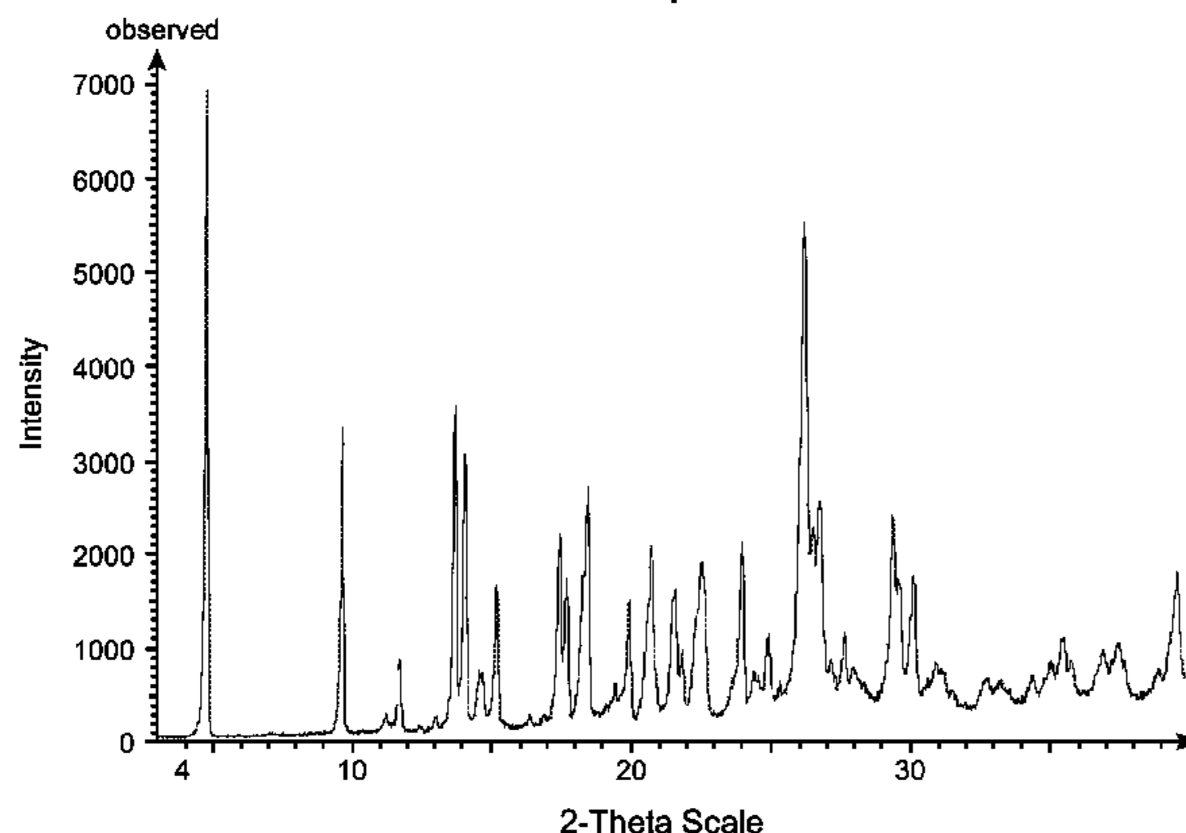
XRPD of the compound of Formula II
