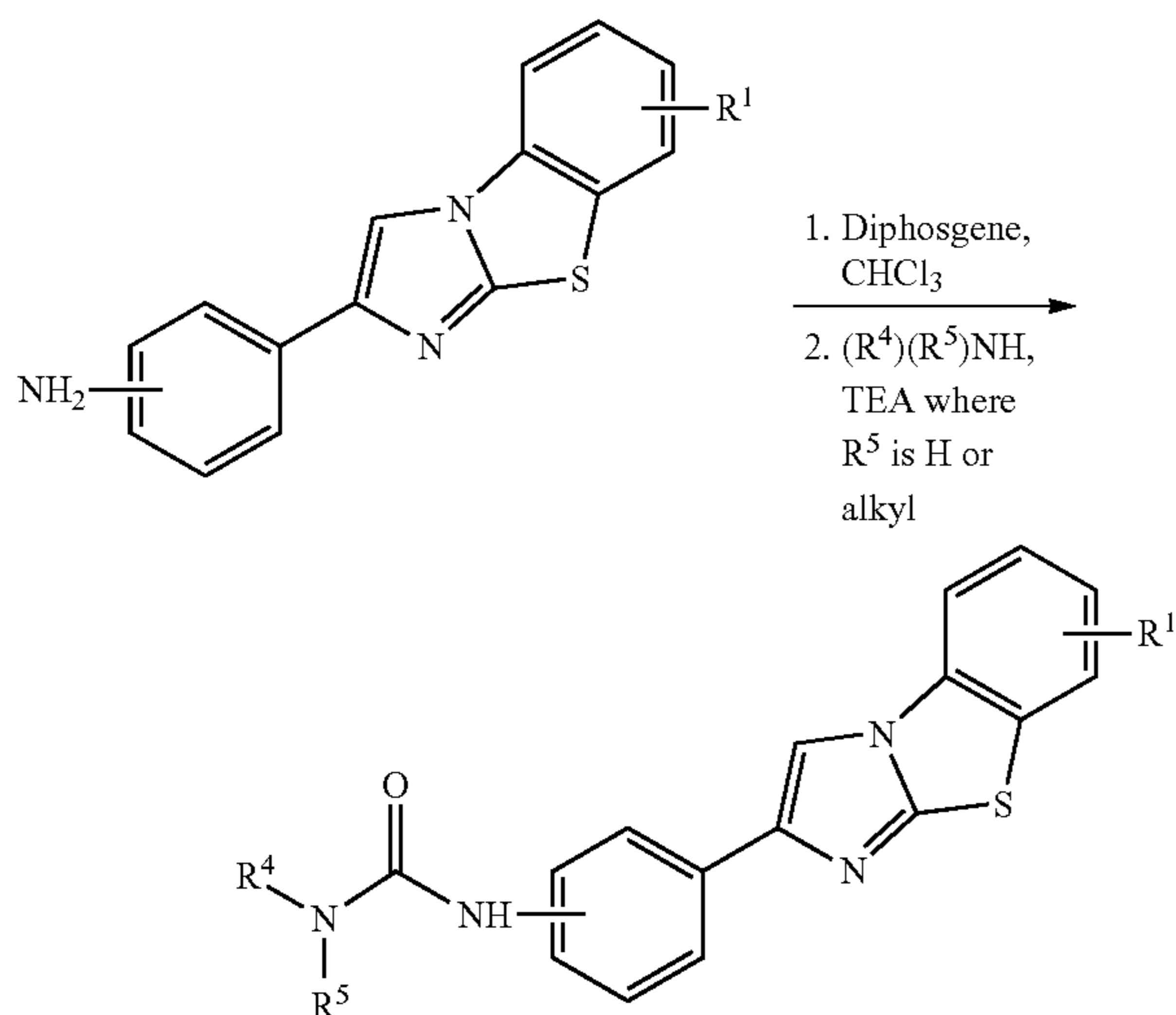
GENERAL SCHEME FOR ALTERNATIVE UREA DERIVATIVES-SCHEME 10
