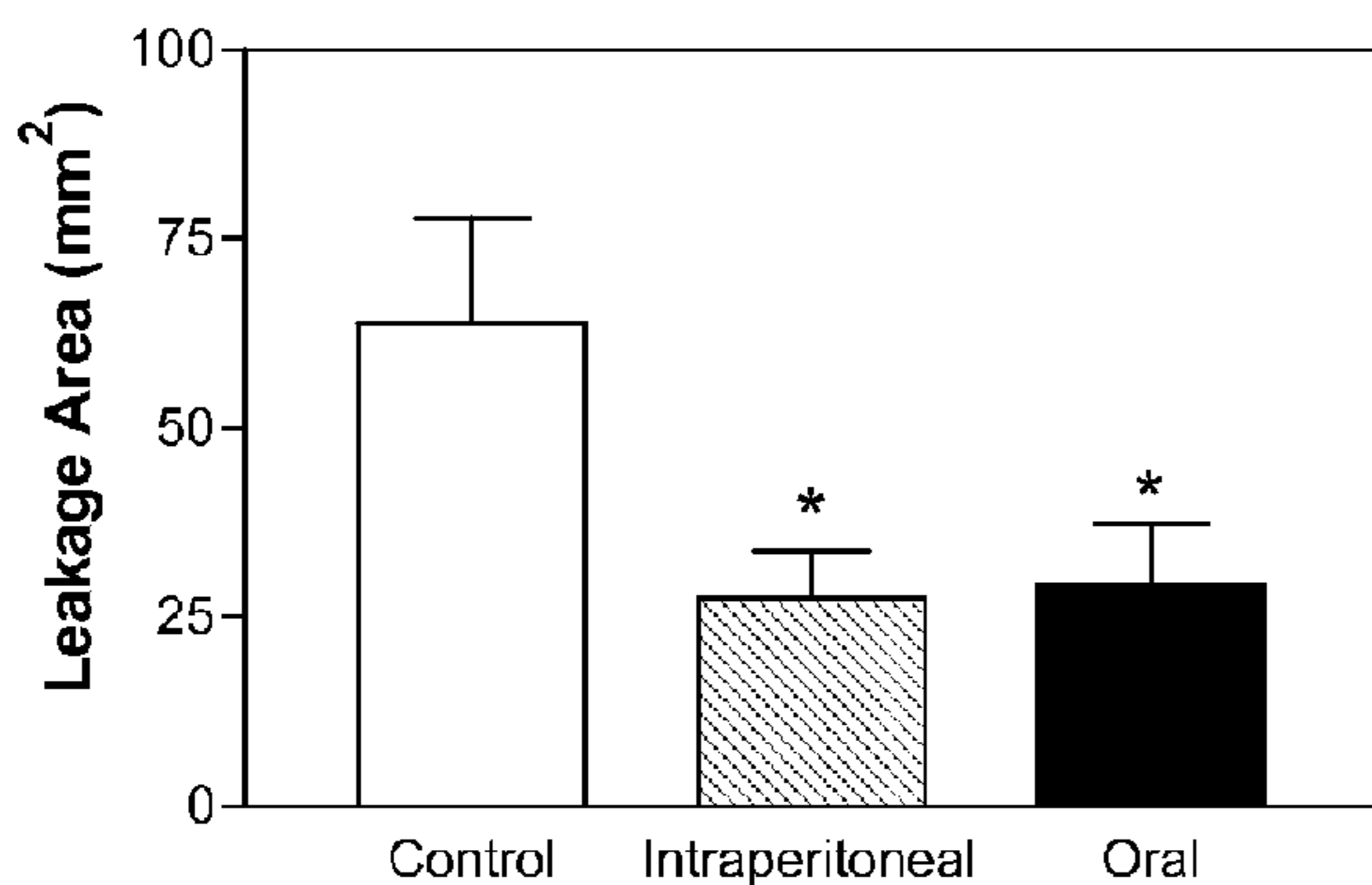
Compound 62
