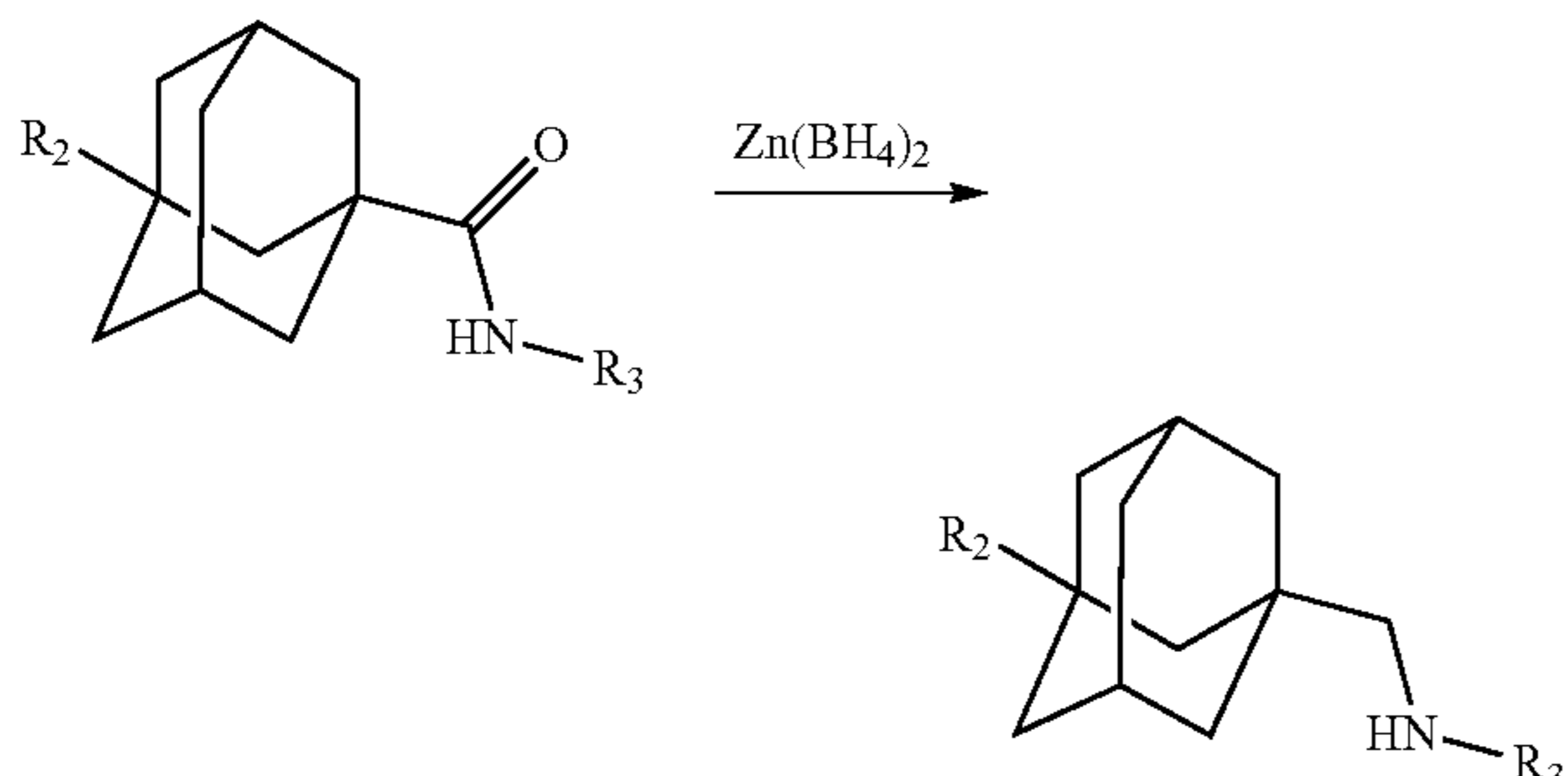
Scheme 3.
