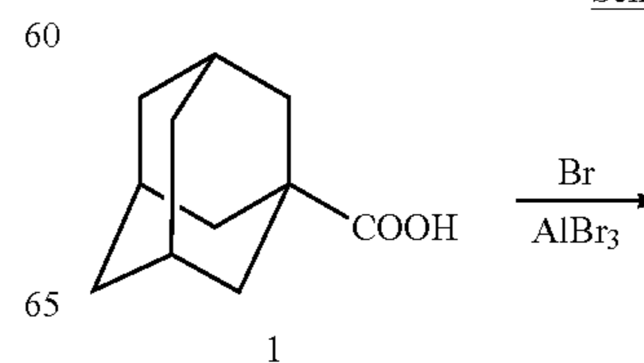
Scheme 1.
