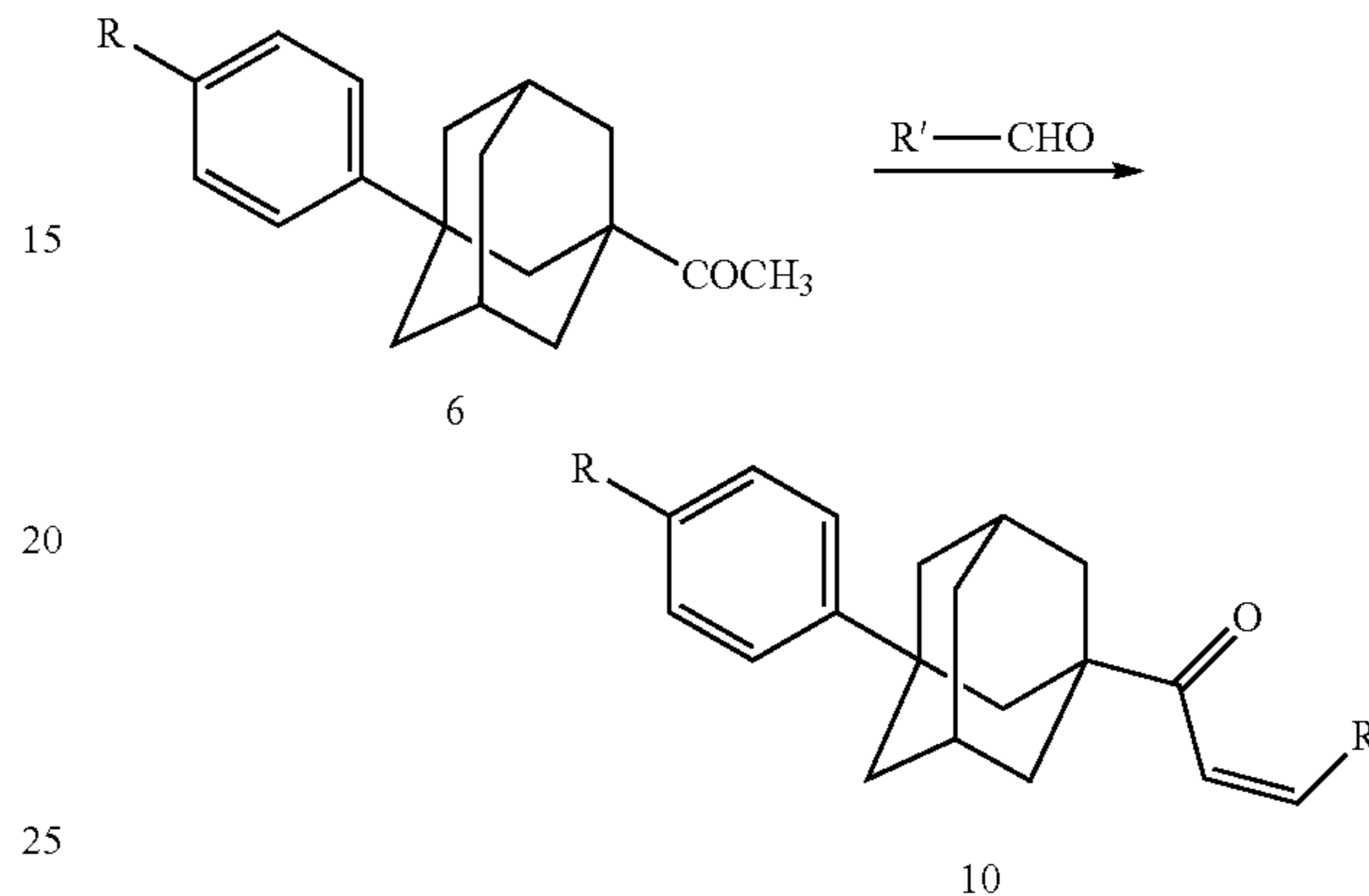
Scheme 5
