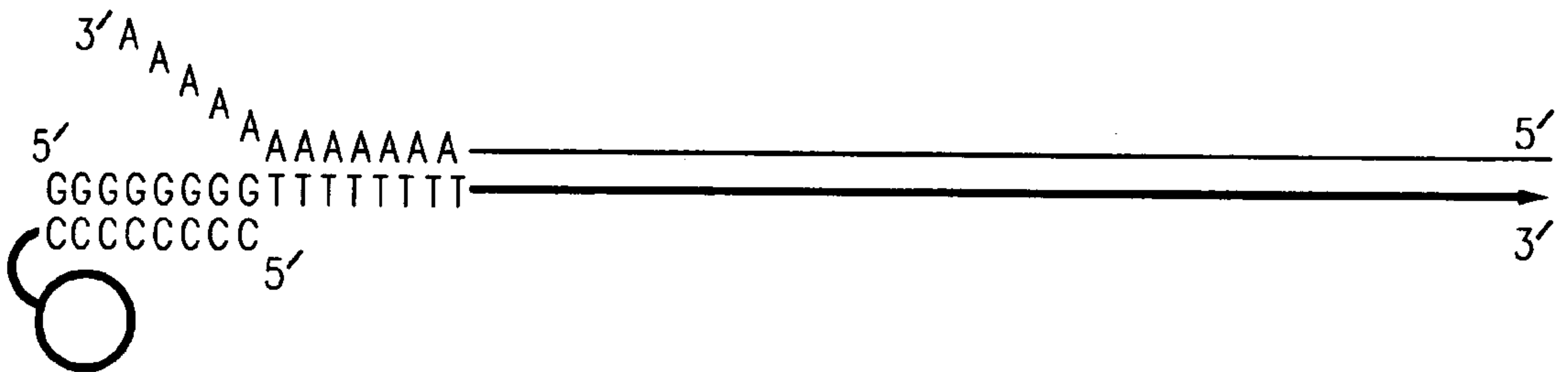
(B) Extension of Oligo T with poly A mRNA as template
