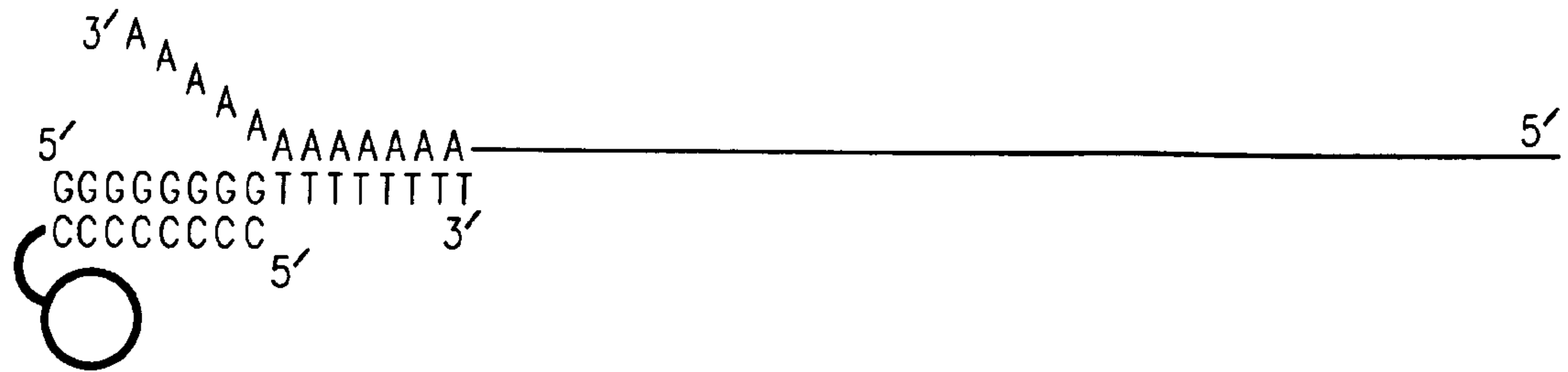
(A) Sandwich Capture of poly A mRNA
