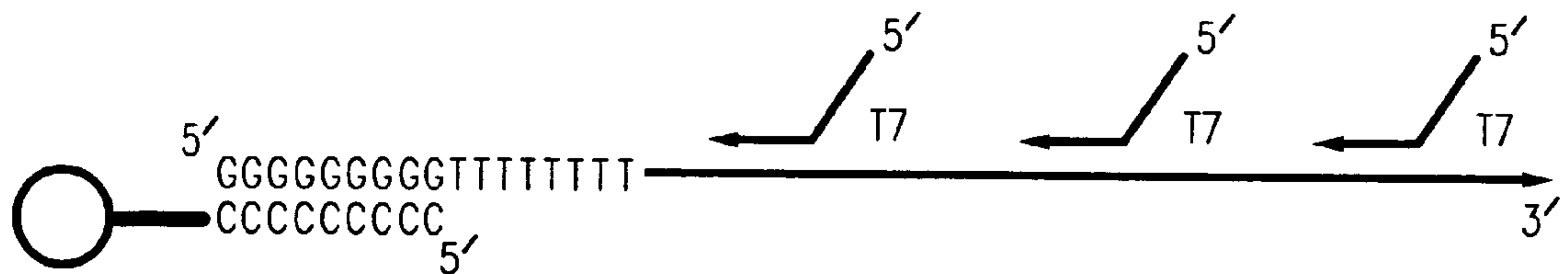
(C) Removal of poly A mRNA and binding of random primers with T7 promoter sequence
