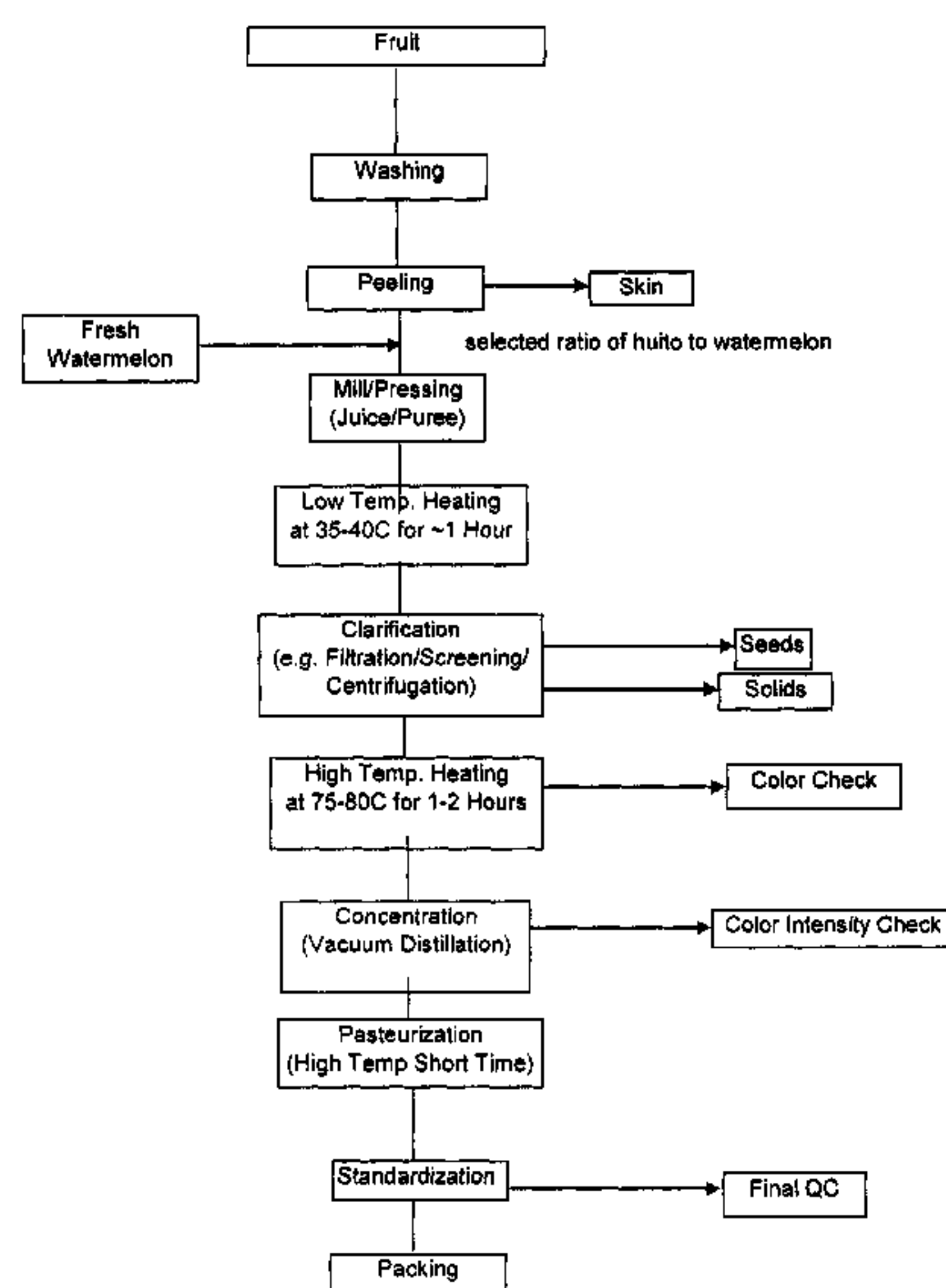
Huito Juice Process Example 3
