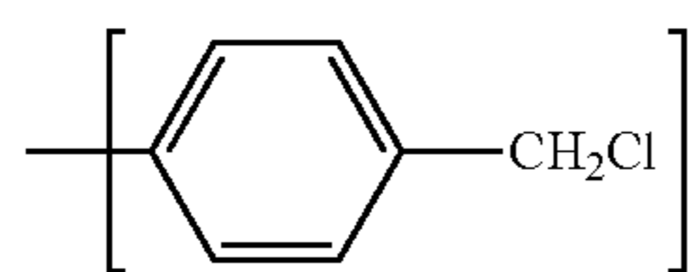
chlorobenzyl moiety
