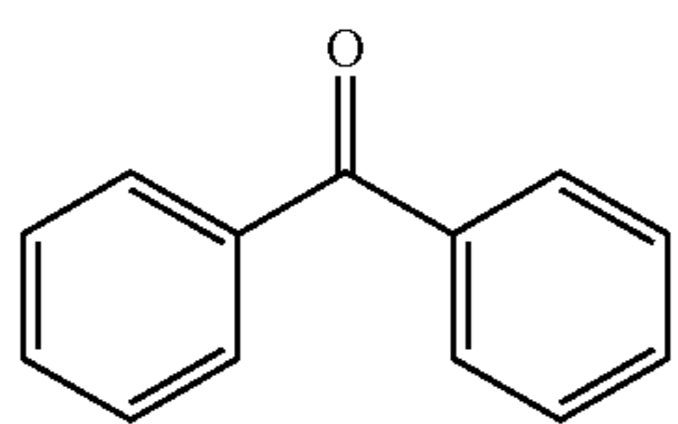
benzophenone
