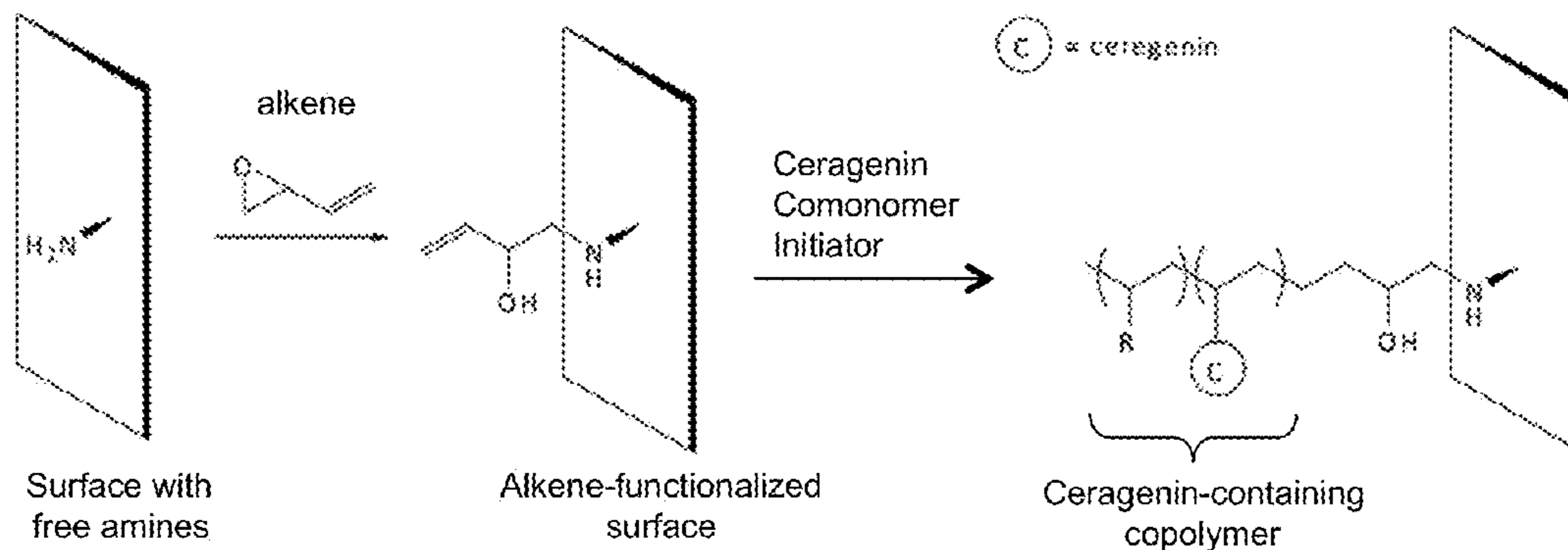
Attachment Scheme-III
