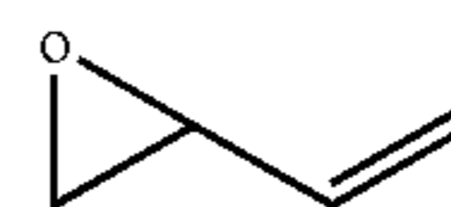
3,4-epoxy-1-butene
