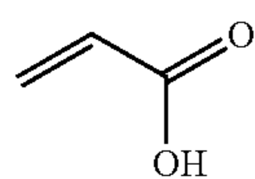
acrylic acid
