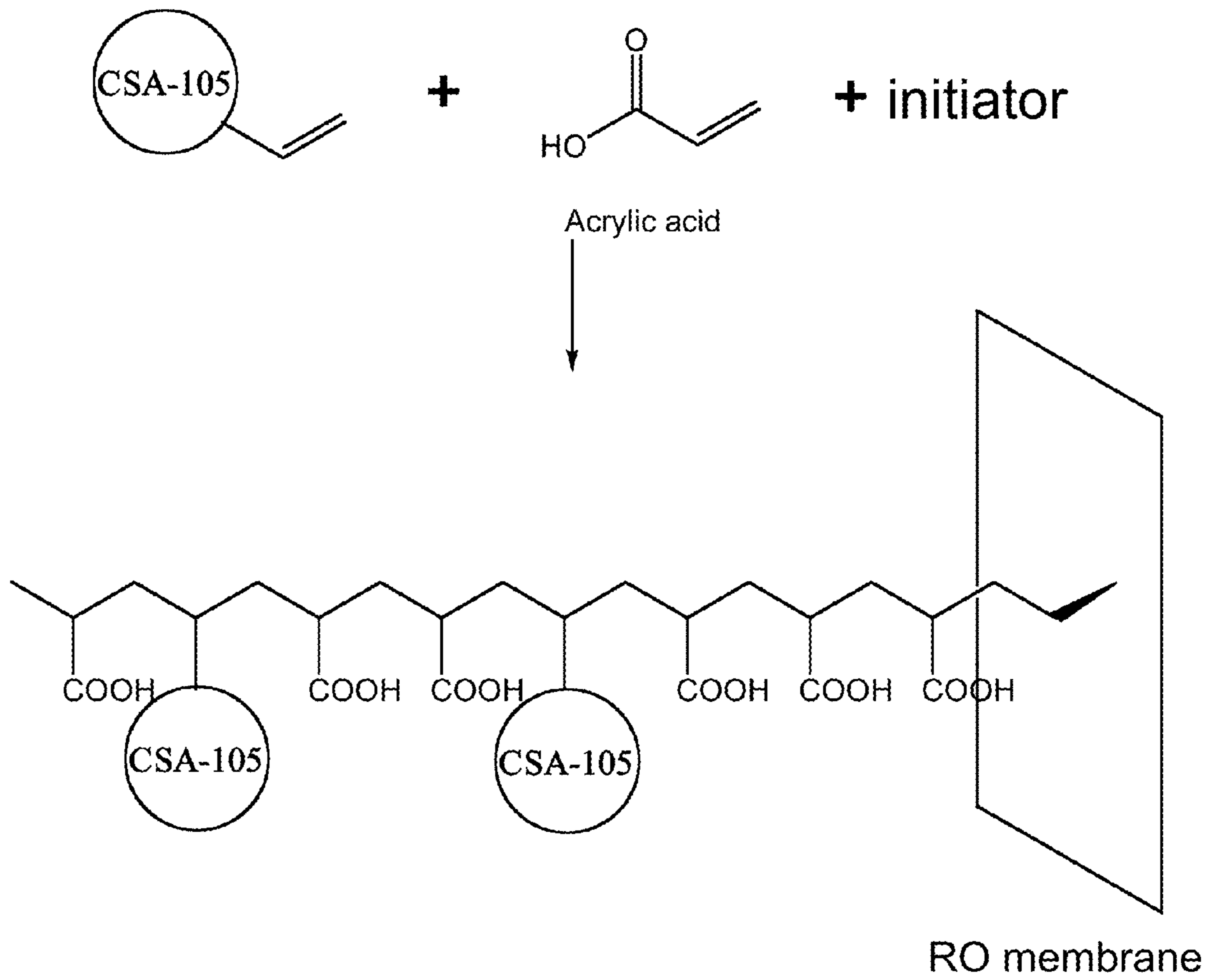
Attachment Scheme-I
