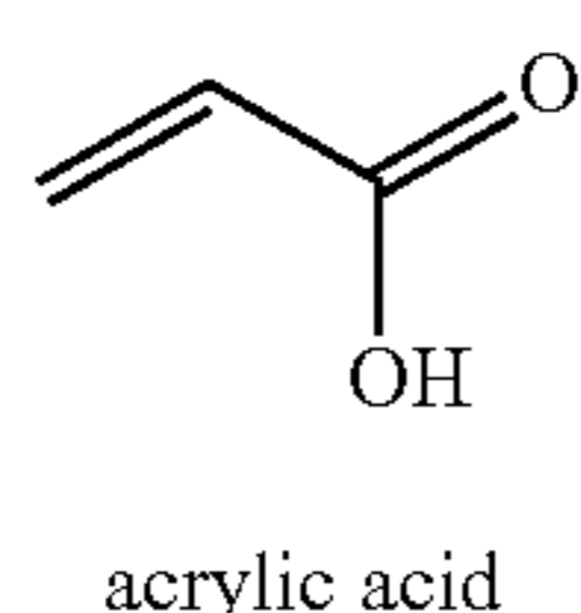
Attachment Scheme-IV
