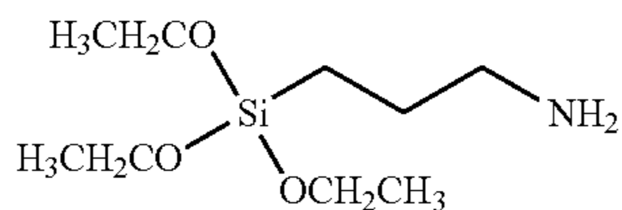
aminopropyltriethoxysilane (APTEOS)
