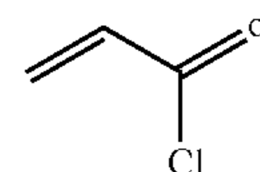
acryloyl chloride
