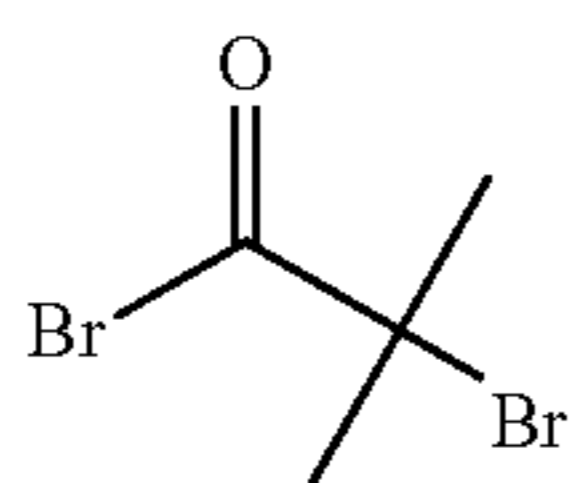
bromoisobutyryl bromide
