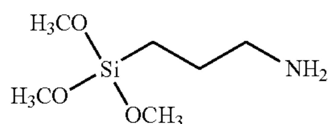
3-aminopropyltrimethoxysilane (APTAMOS)
