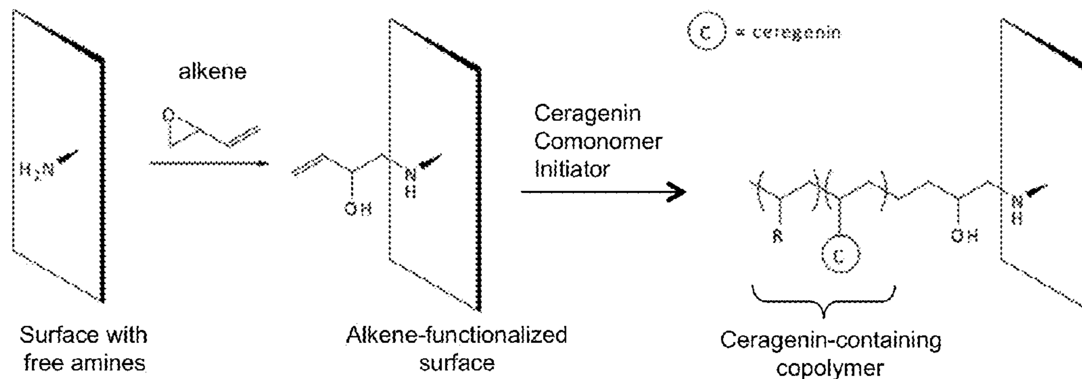
Attachment Scheme-III
