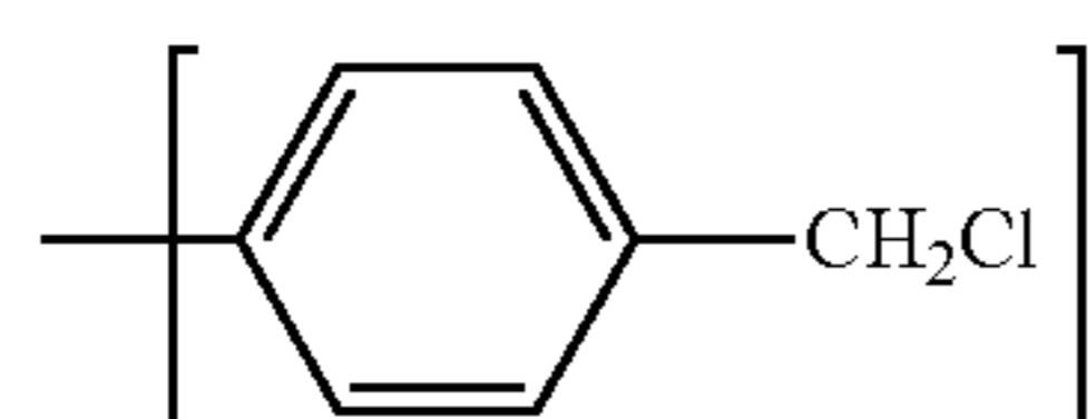
chlorobenzyl moiety
