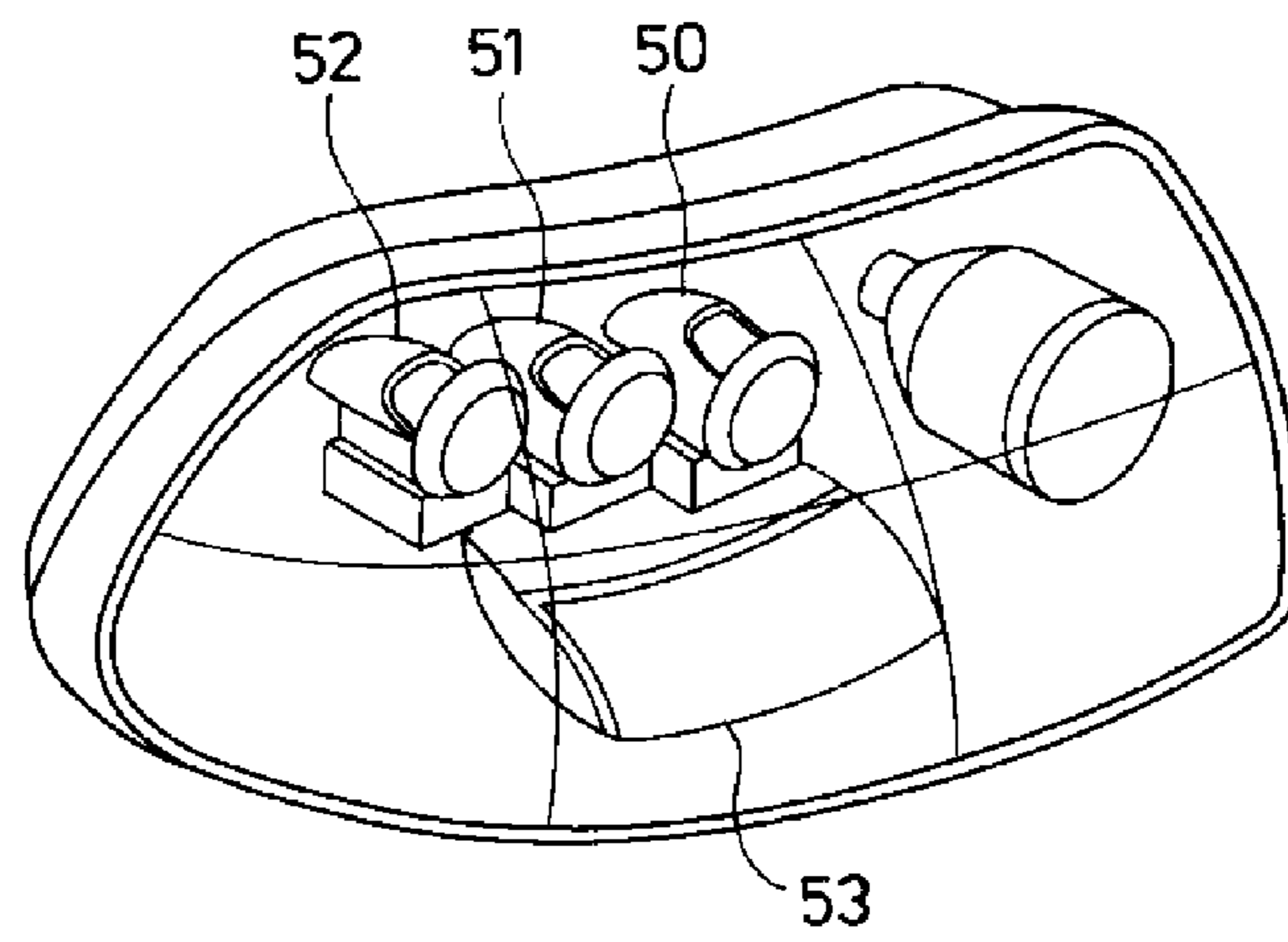
FIG. 15 CONVENTIONAL ART
