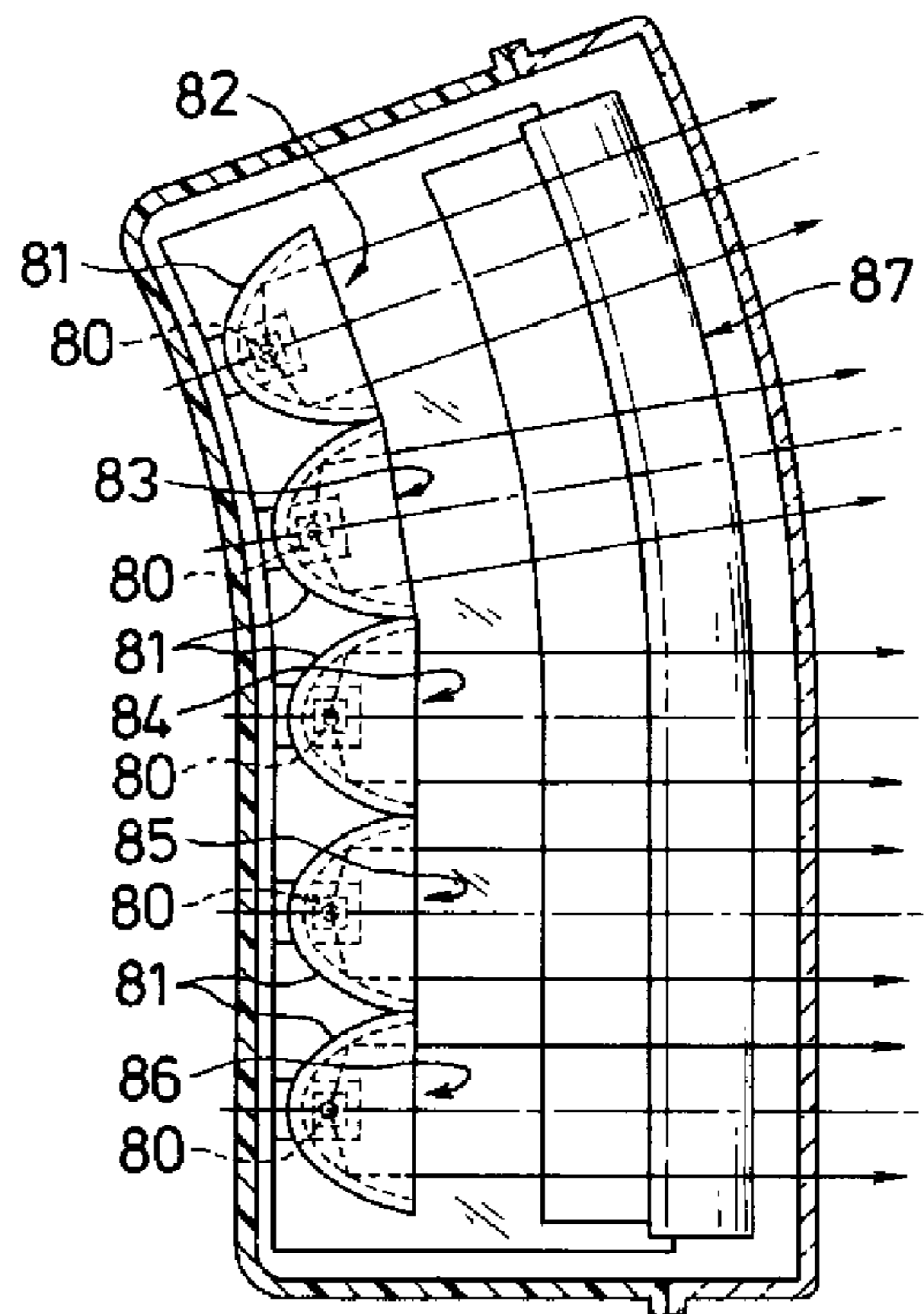
FIG. 13 CONVENTIONAL ART
