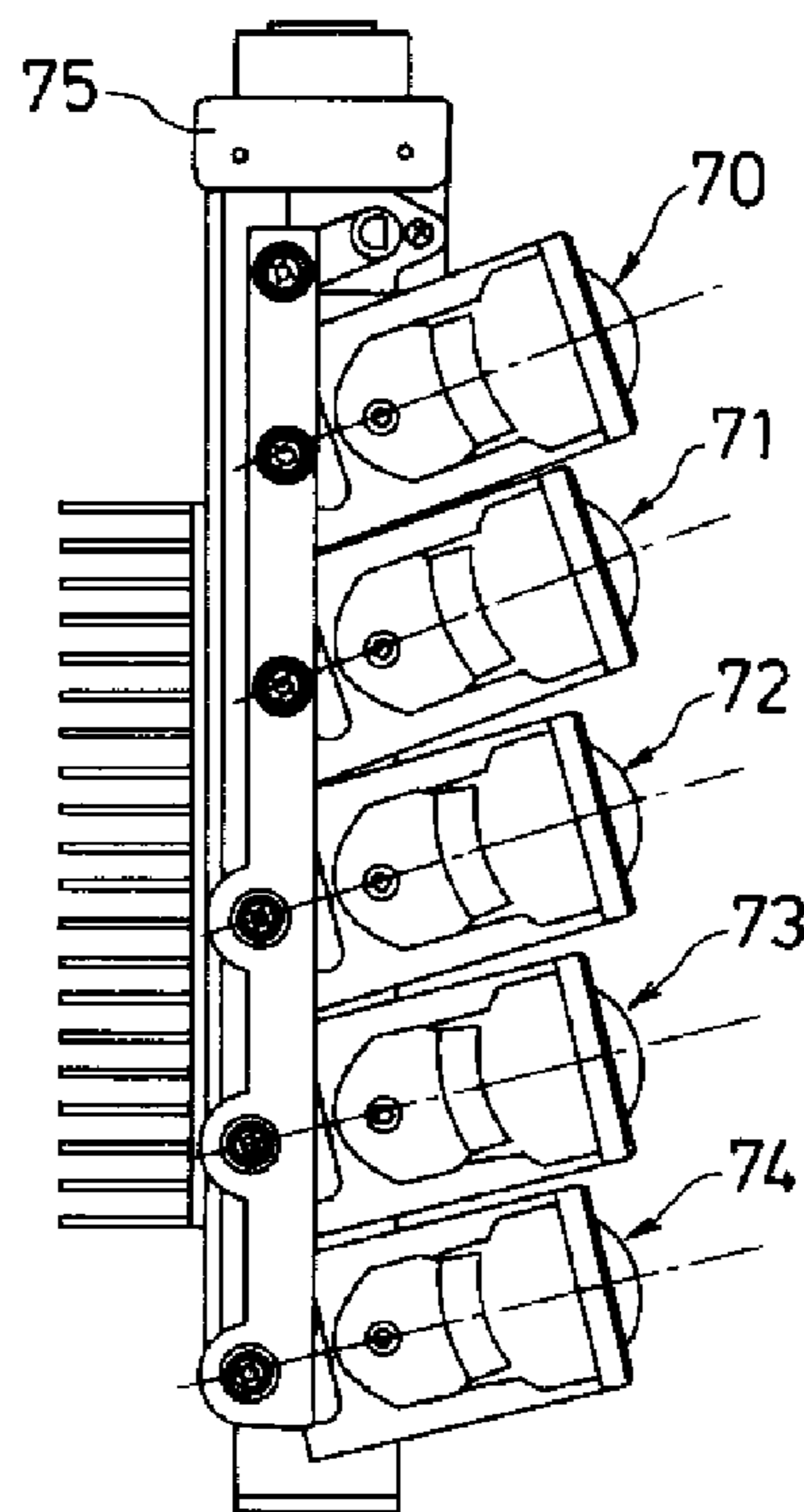
FIG. 12 CONVENTIONAL ART
