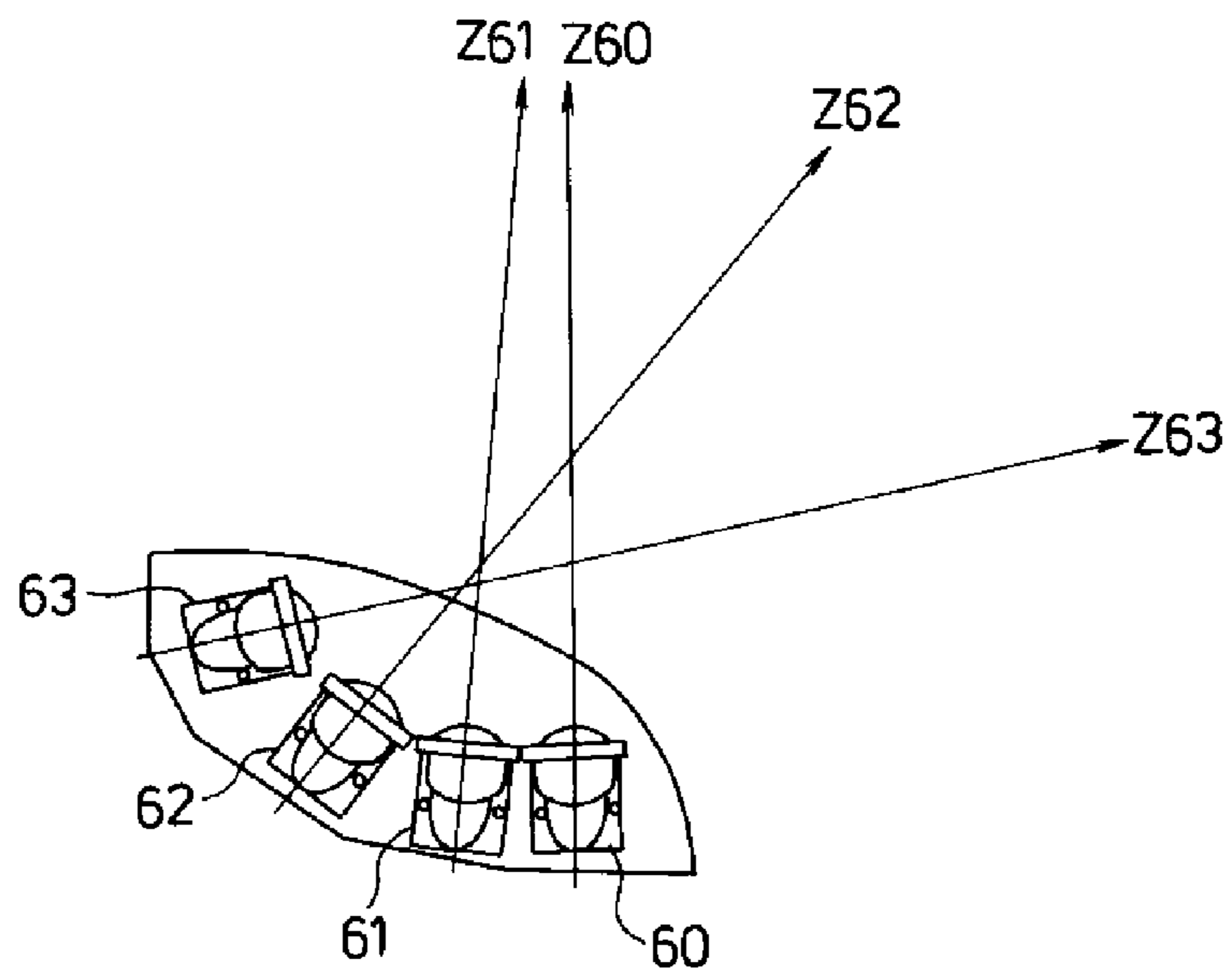
FIG. 11 CONVENTIONAL ART
