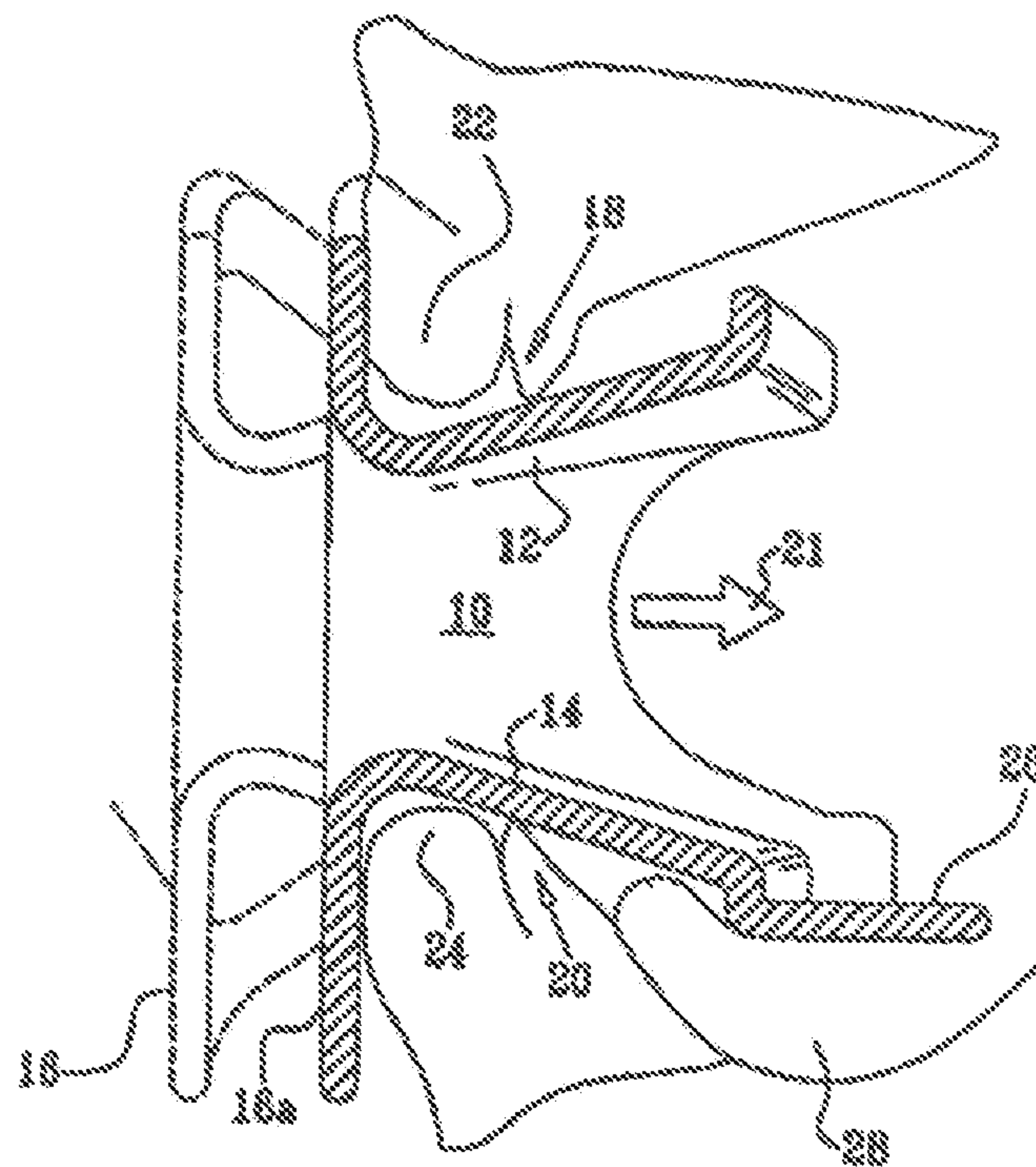
FIG. 1 Prior art
