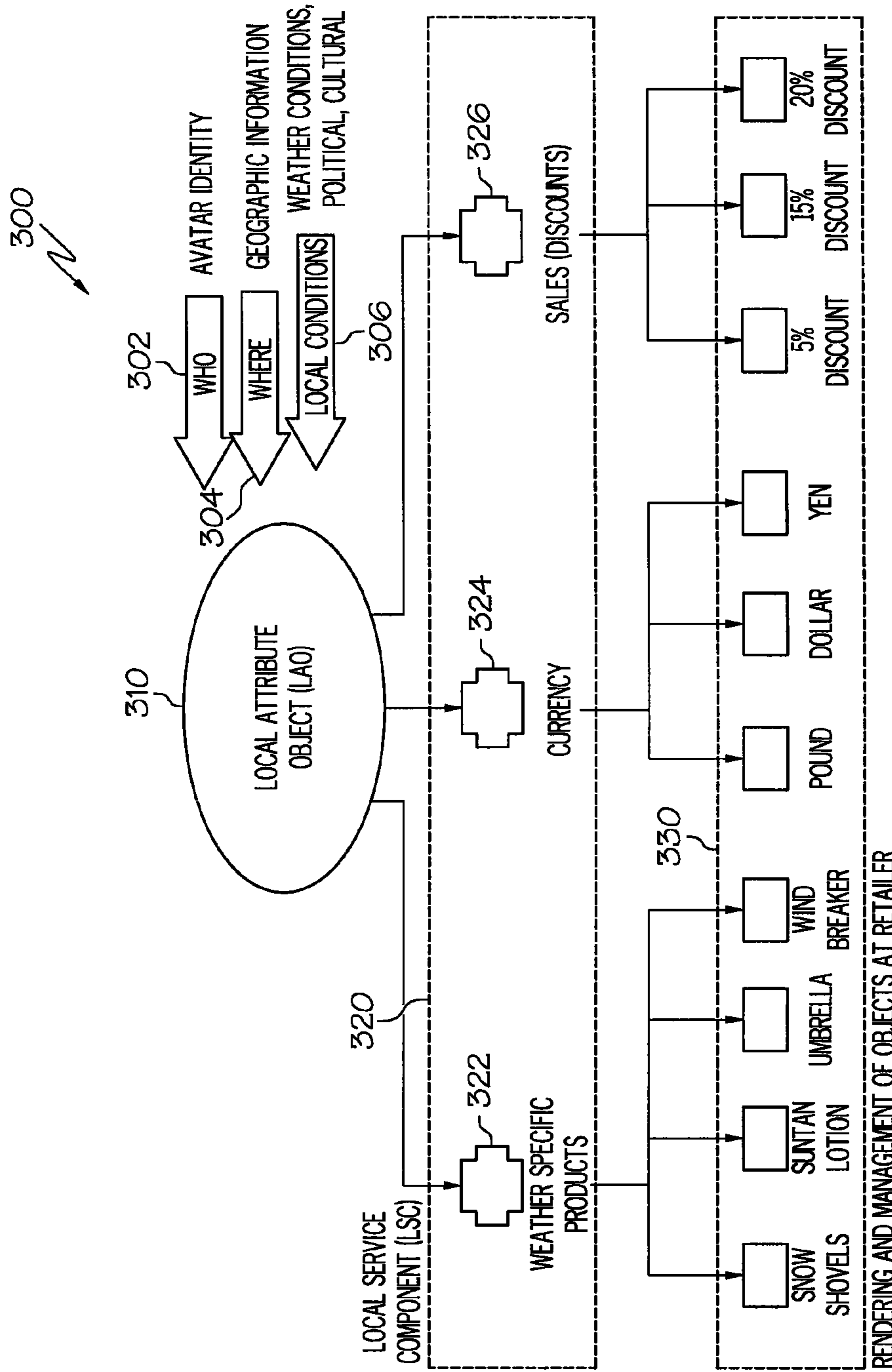
RETAIL STORE EXAMPLE; LOCAL ATTRIBUTE OBJECT AND LOCAL SERVICE COMPONENT
