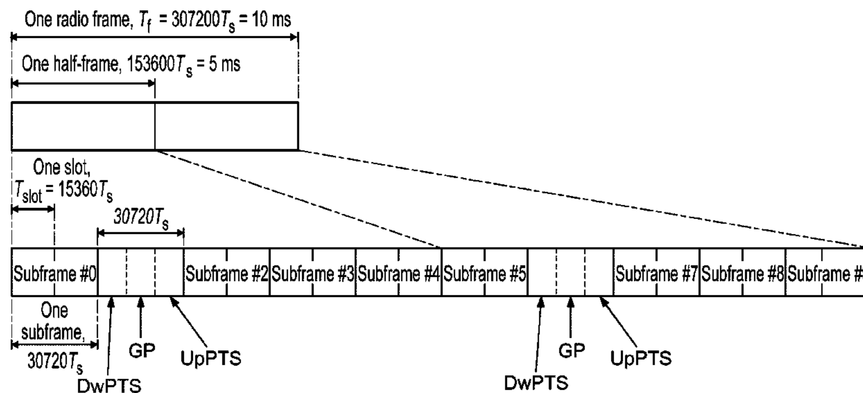
LTE TDD frame structure
