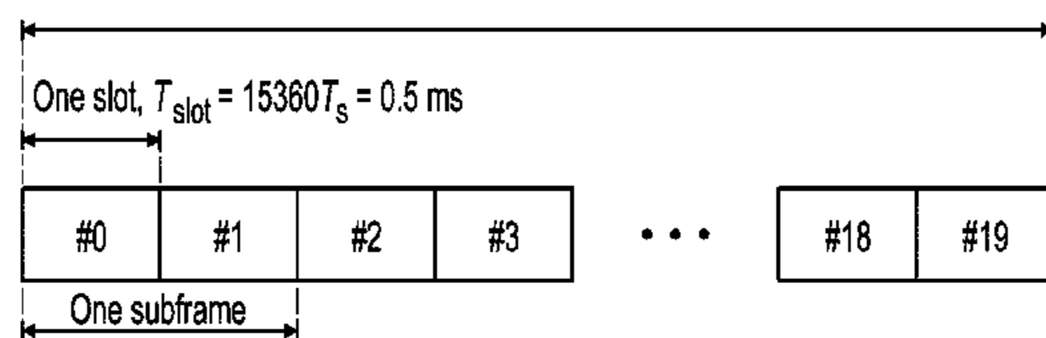
LTE FDD frame structure
