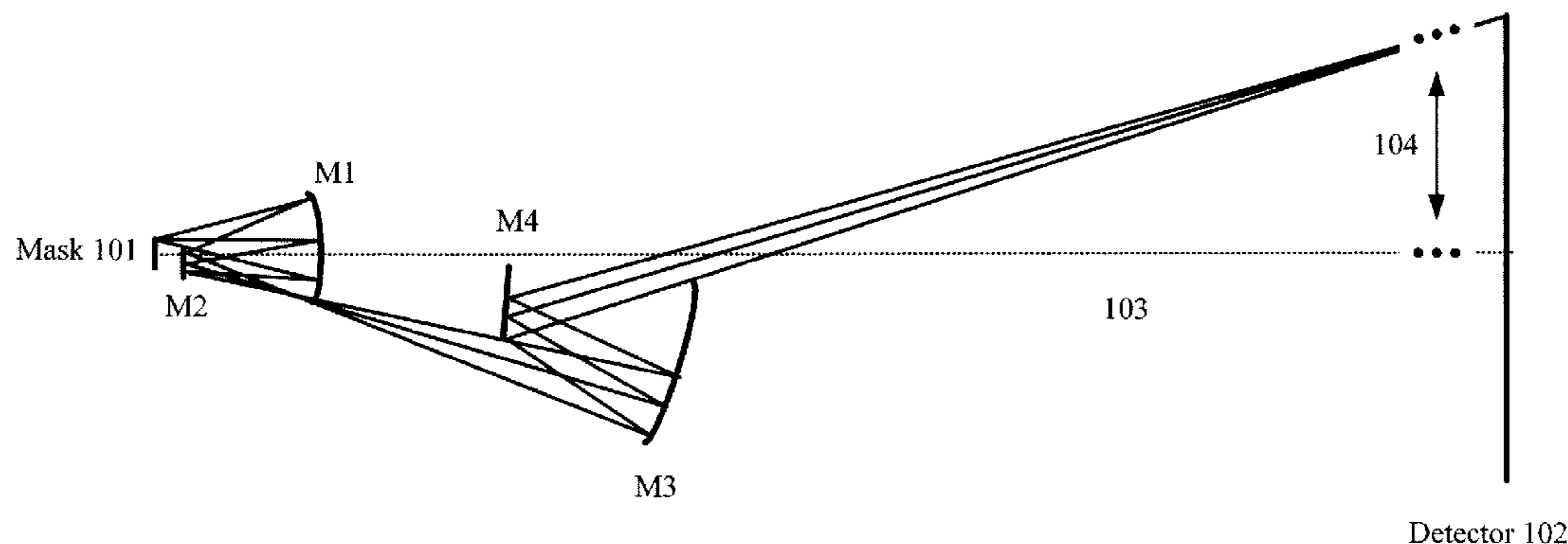
Inspection system 100
