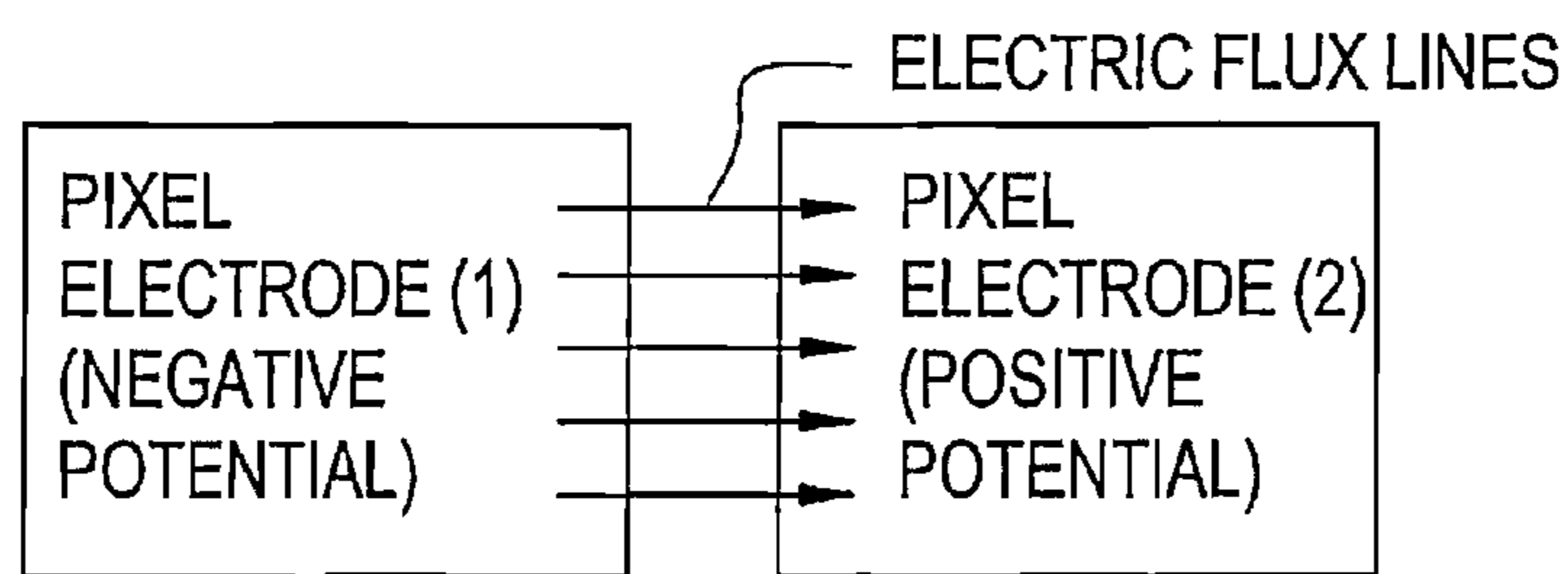
VIEW SHOWING STATE OF ELECTRIC FLUX LINES PRODUCED BETWEEN TWO PIXEL ELECTRODES (TOP VIEW)
