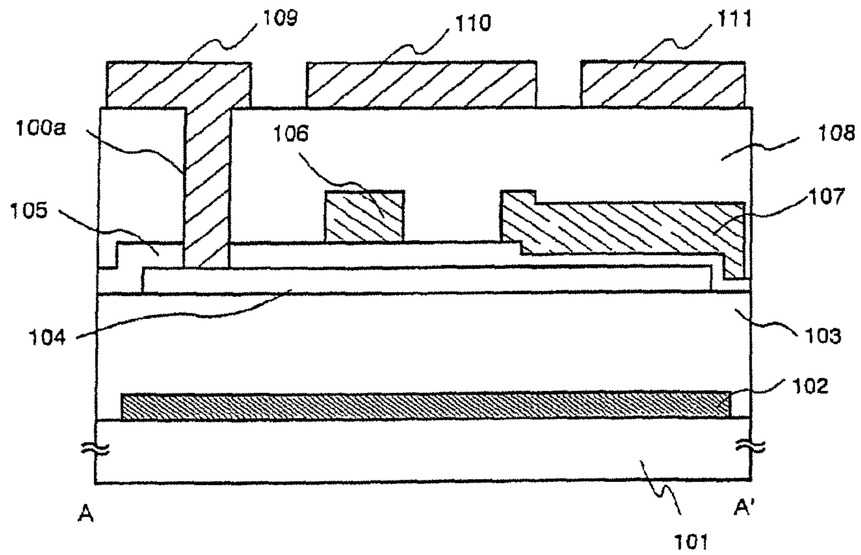
Fig. 3A A-A' cross sectional view
