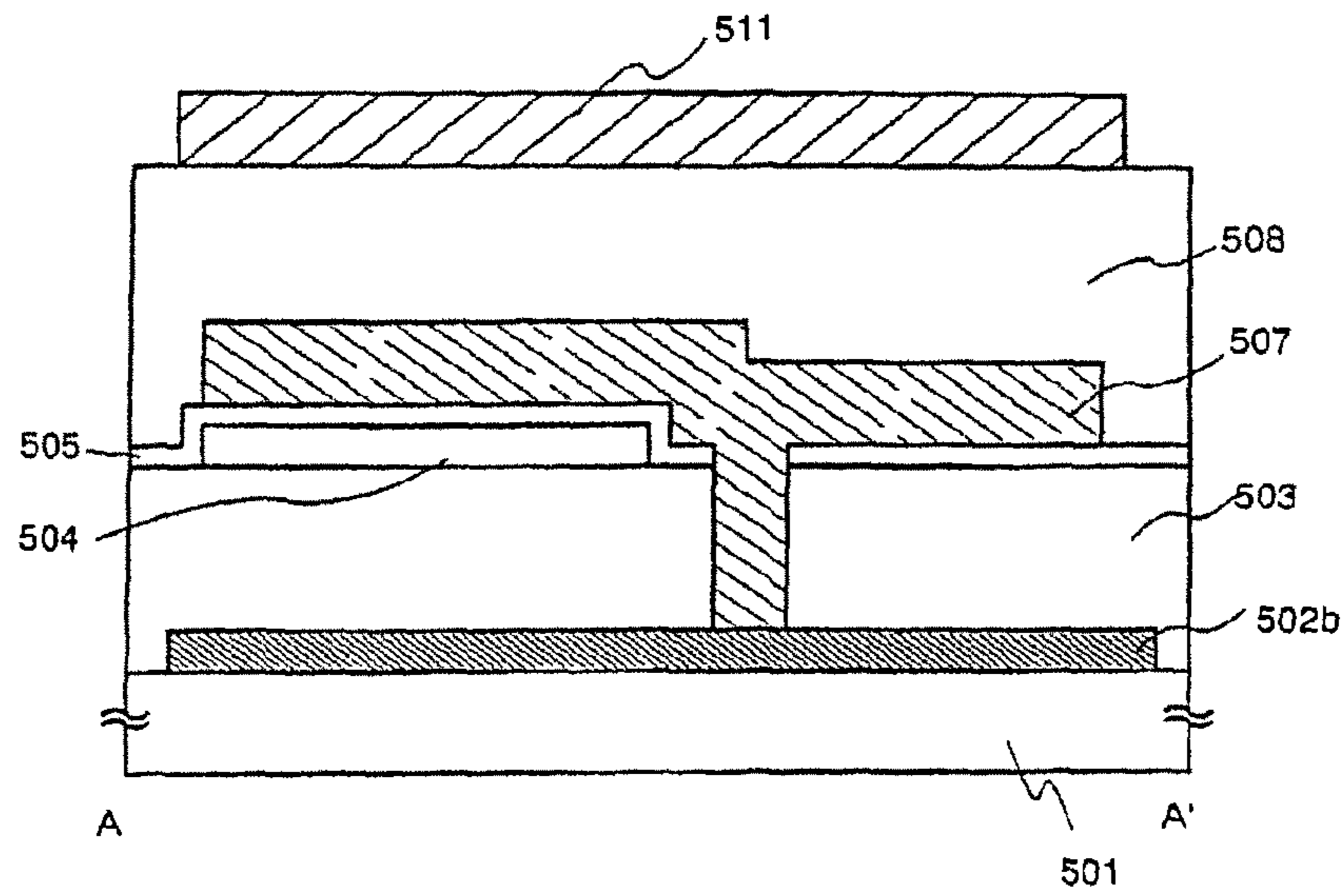
Fig. 15A A-A' Cross sectional view
