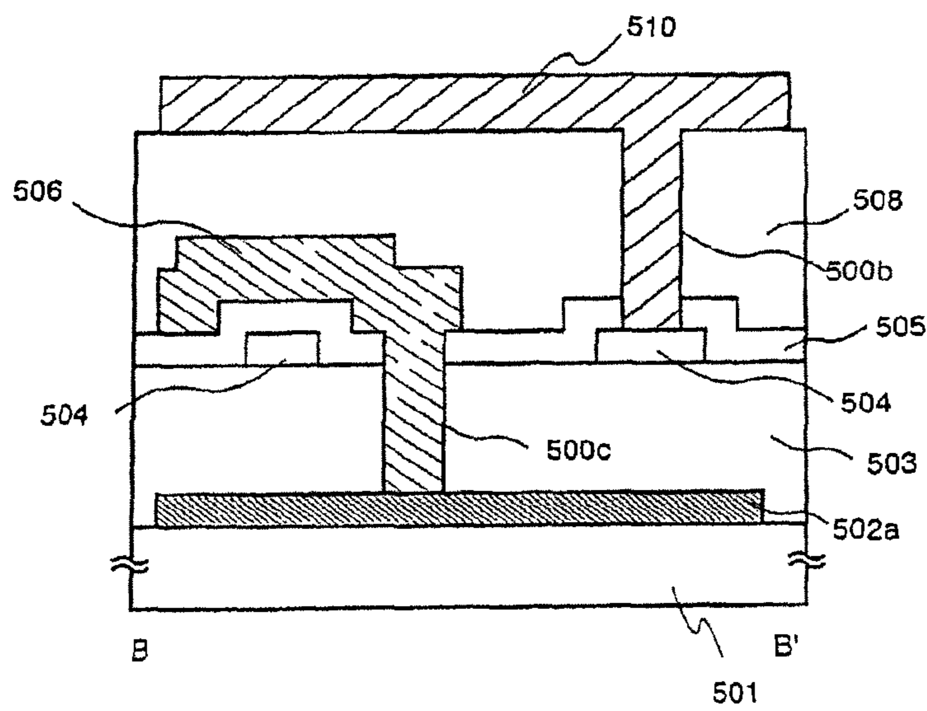
Fig. 15B B-B' Cross sectional view
