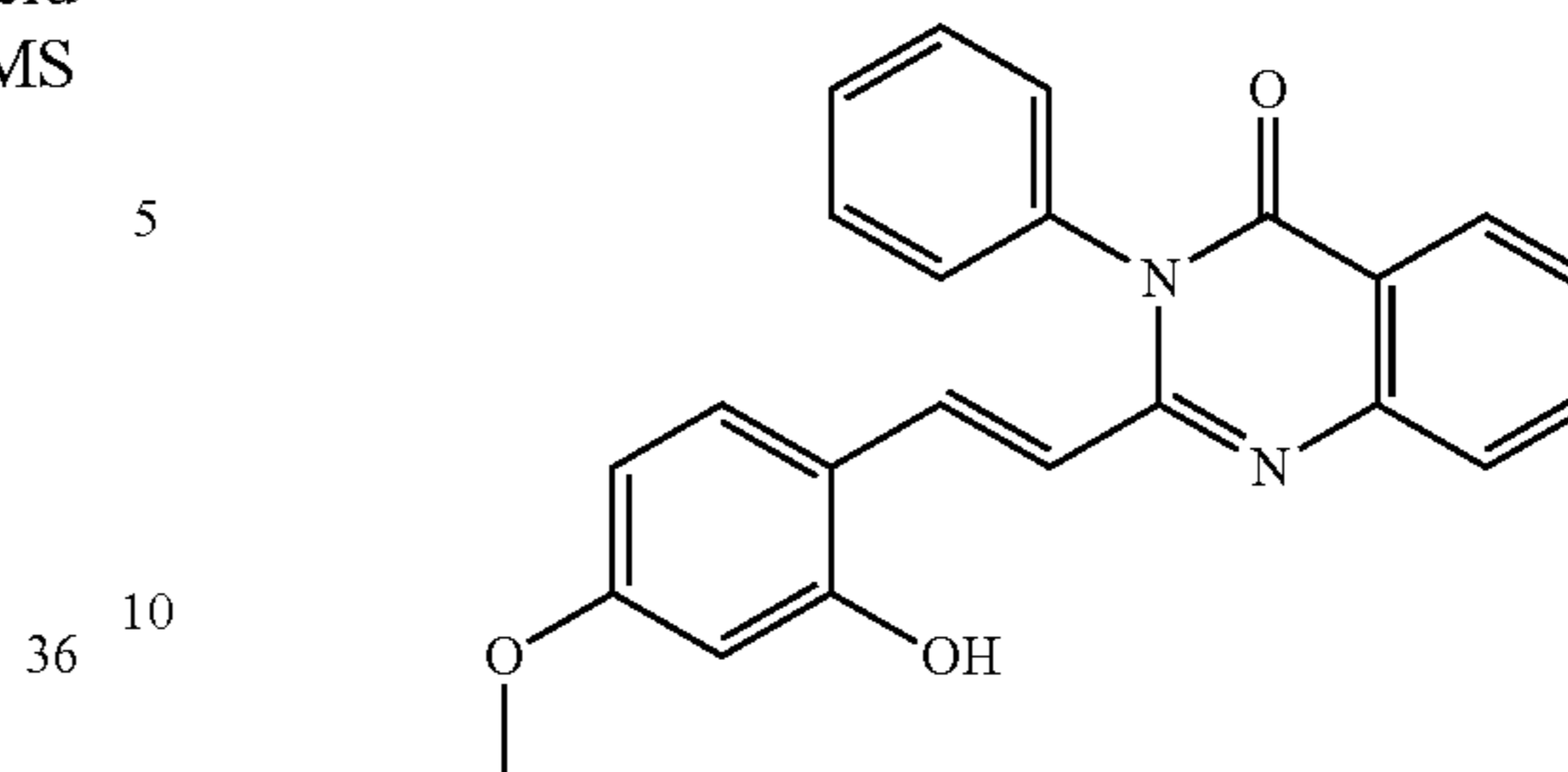
2-[2-(2-Hydroxy-4-methoxy-phenyl)-vinyl]-3-phenyl-3H-quinazolin-4-one (38)
