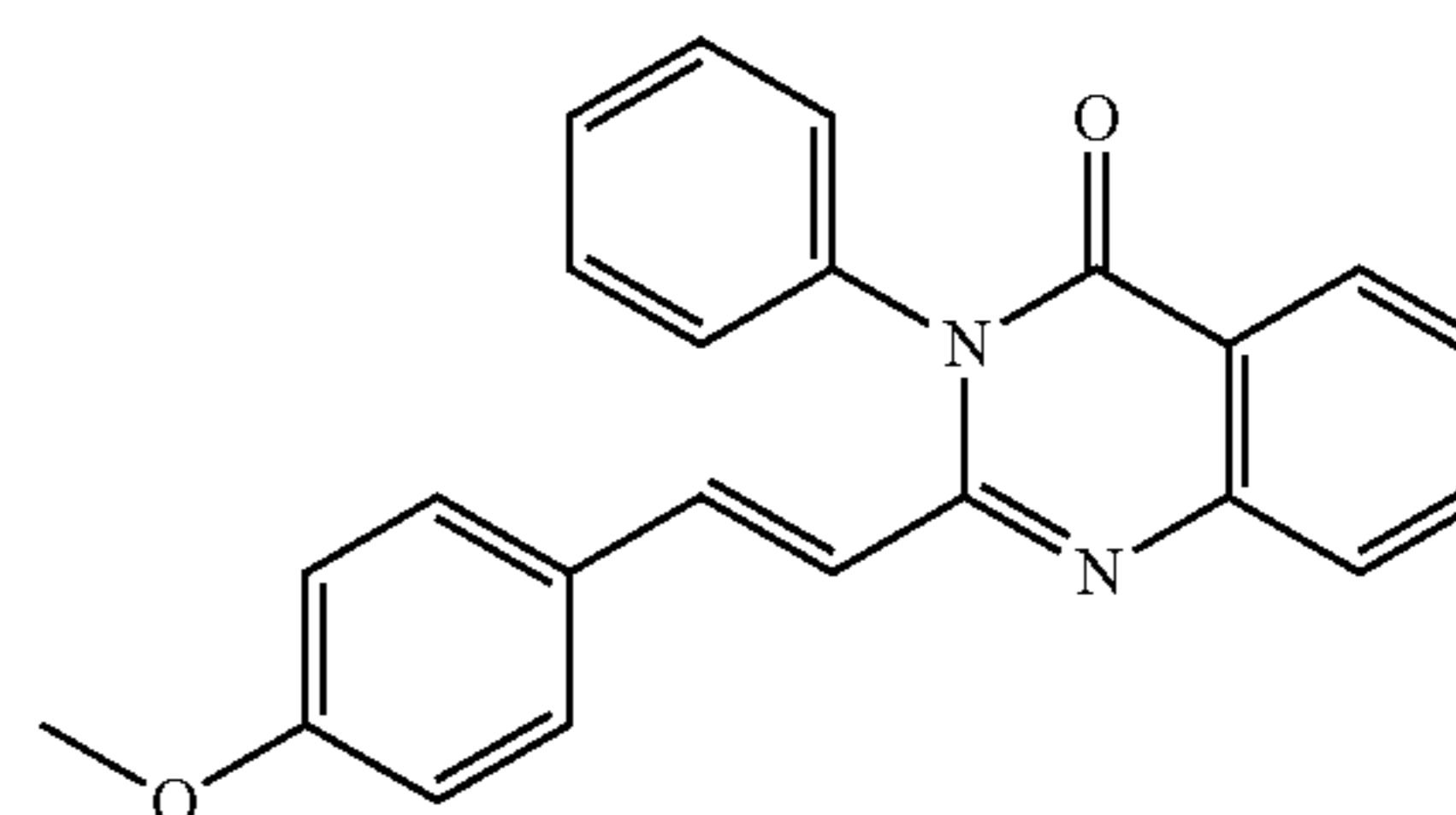
2-[2-(4-Methoxy-phenyl)-vinyl]-3-phenyl-3H-quinazolin-4-one (34)
