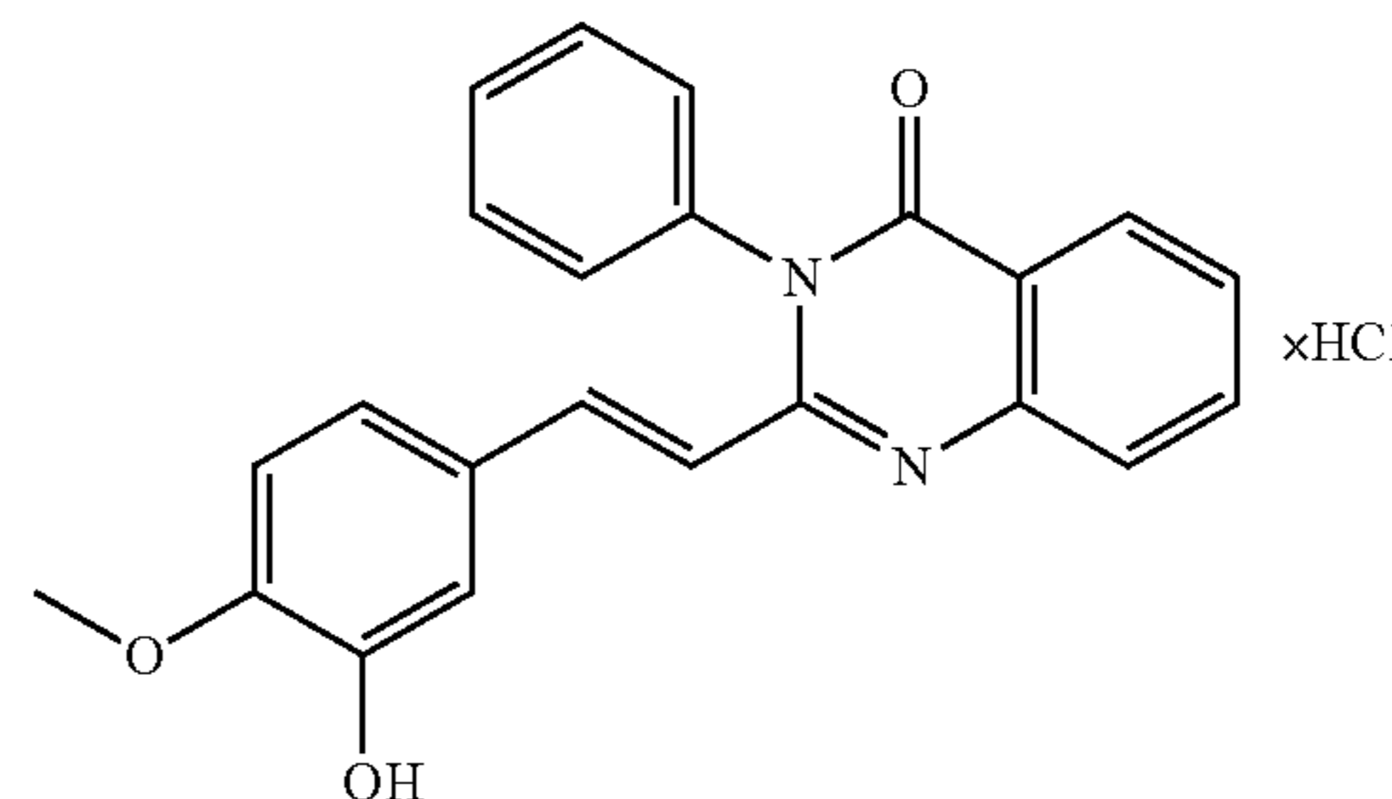
2-[2-(3-Hydroxy-4-methoxy-phenyl)-vinyl]-3-phenyl-3H-quinazolin-4-one hydrochloride (39)
