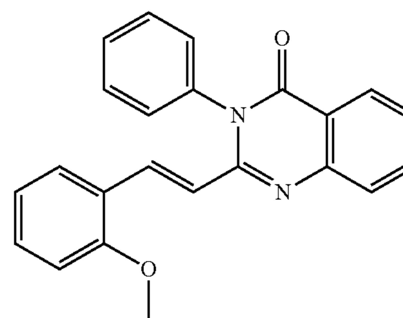
2-[2-(2-Methoxy-phenyl)-vinyl]-3-phenyl-3H-quinazolin-4-one (33)
