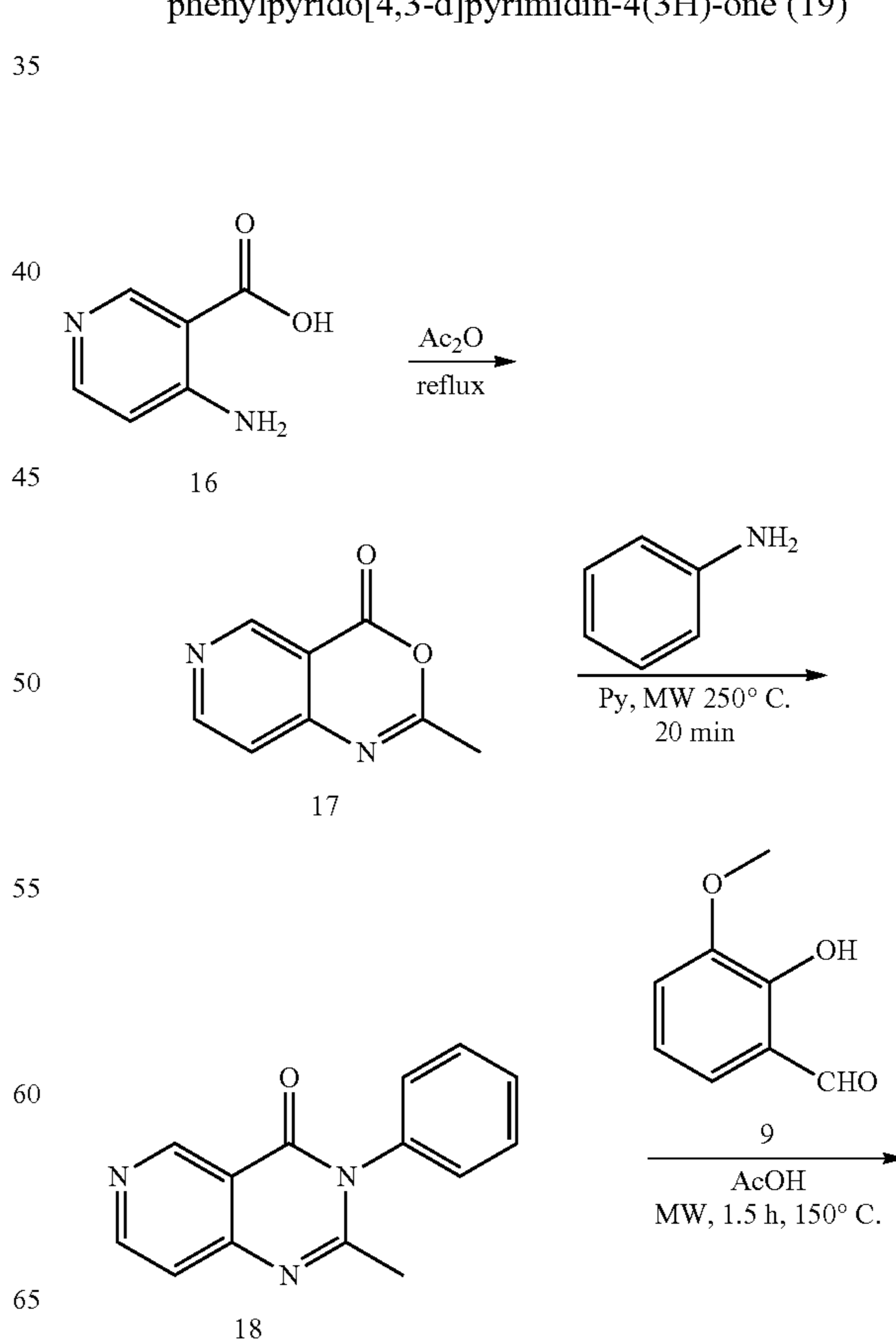
Synthesis of (E)-2-(2-hydroxy-3-methoxystyryl)-3-phenylpyrido[4,3-d]pyrimidin-4(3H)-one (19)
