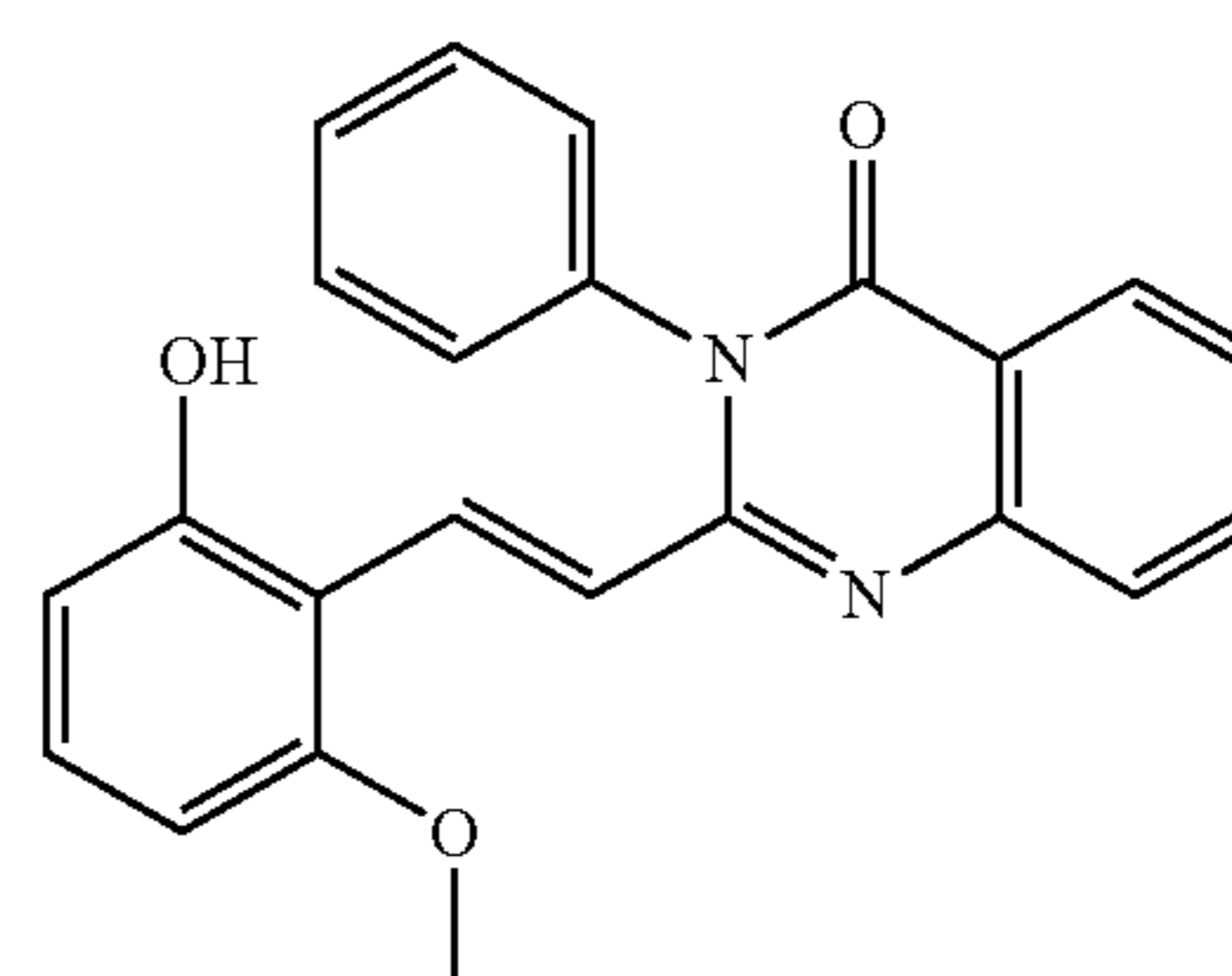
2-[2-(2-Hydroxy-6-methoxy-phenyl)-vinyl]-3-phenyl-3H-quinazolin-4-one (35)
