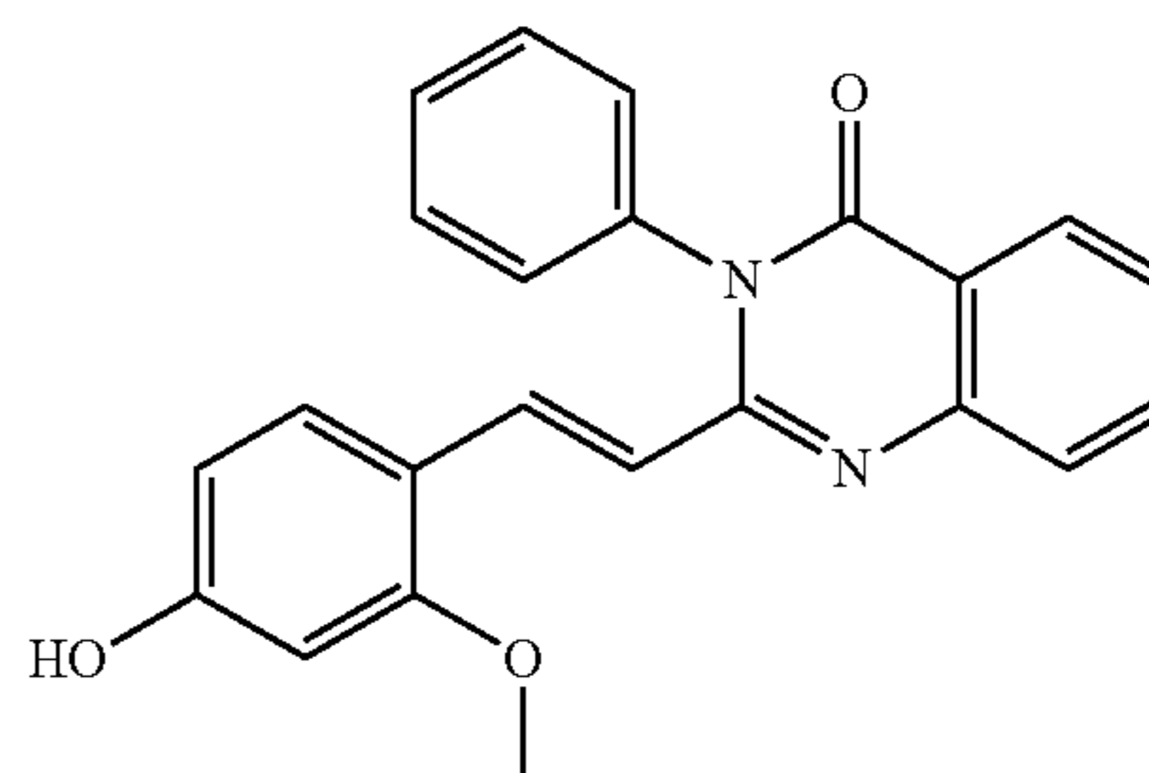
2-[2-(4-Hydroxy-2-methoxy-phenyl)-vinyl]-3-phenyl-3H-quinazolin-4-one (40)
