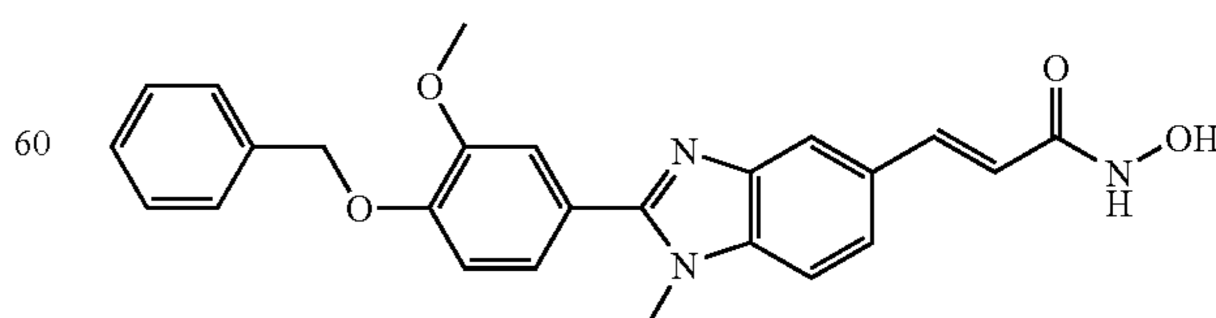
N-Hydroxy-3-[2-(4-benzyloxy-3-methoxy-phenyl)-1-methyl-1H-benzimidazole-5-yl]-acrylamide
