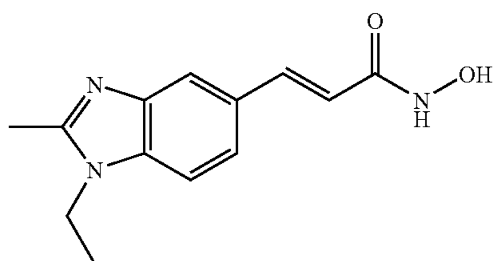
N-Hydroxy-3-(1-Ethyl-2-methyl-1H-benzimidazol-5-yl)-acrylamide
