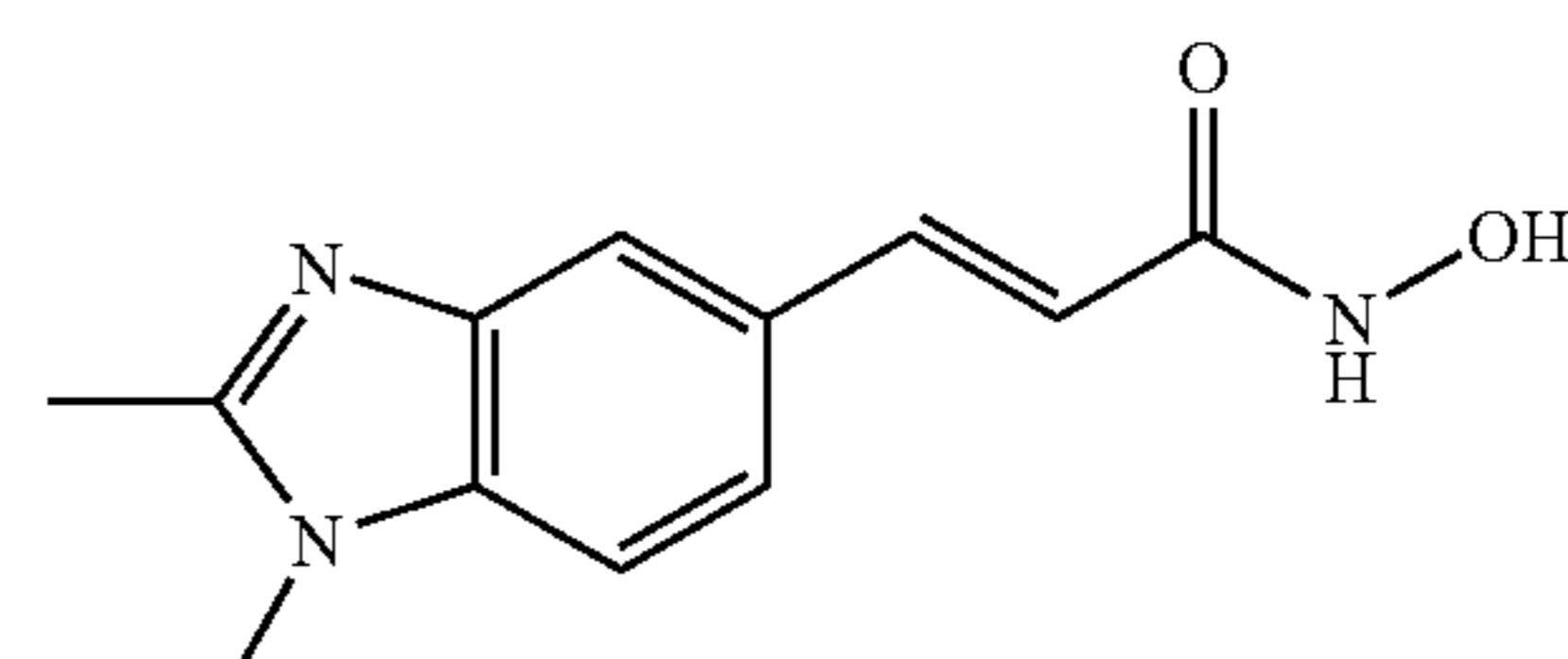
N-Hydroxy-3-(1,2-dimethyl-1H-benzimidazol-5-yl)-acrylamide
