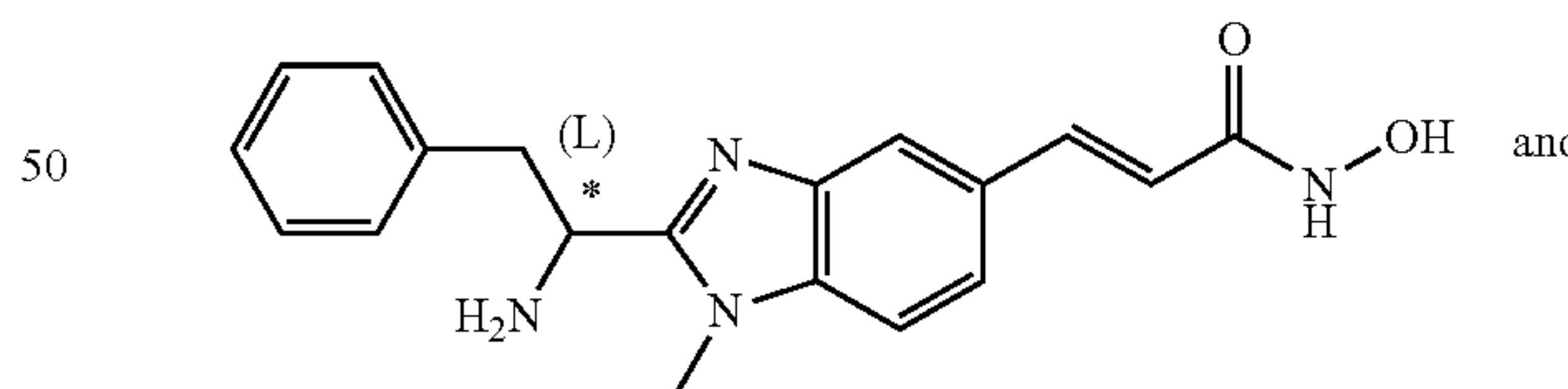
(L)-N-Hydroxy-3-[2-(1-amino-2-phenyl-ethyl)-1-methyl-1H-benzimidazol-5-yl]-acrylamide
