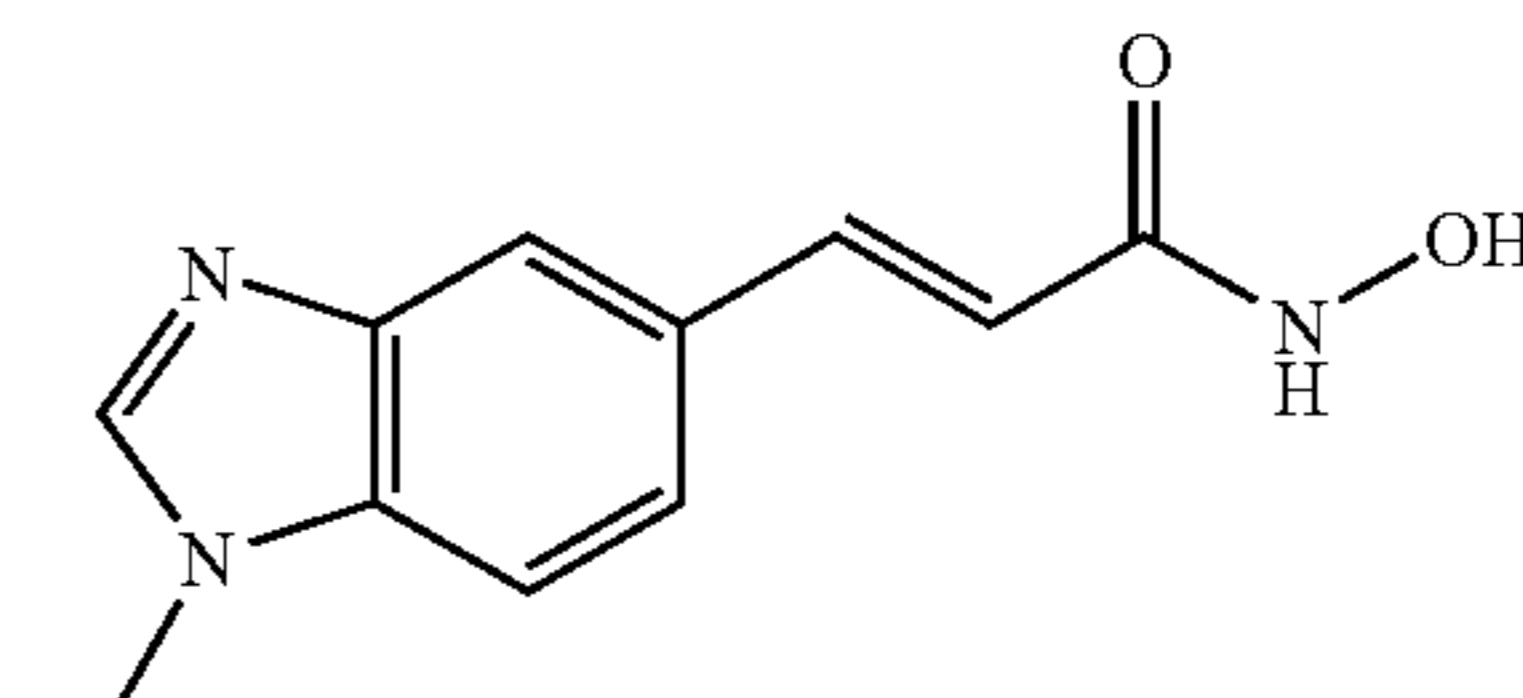
N-Hydroxy-3-(1-methyl-1H-benzimidazol-5-yl)-acrylamide
