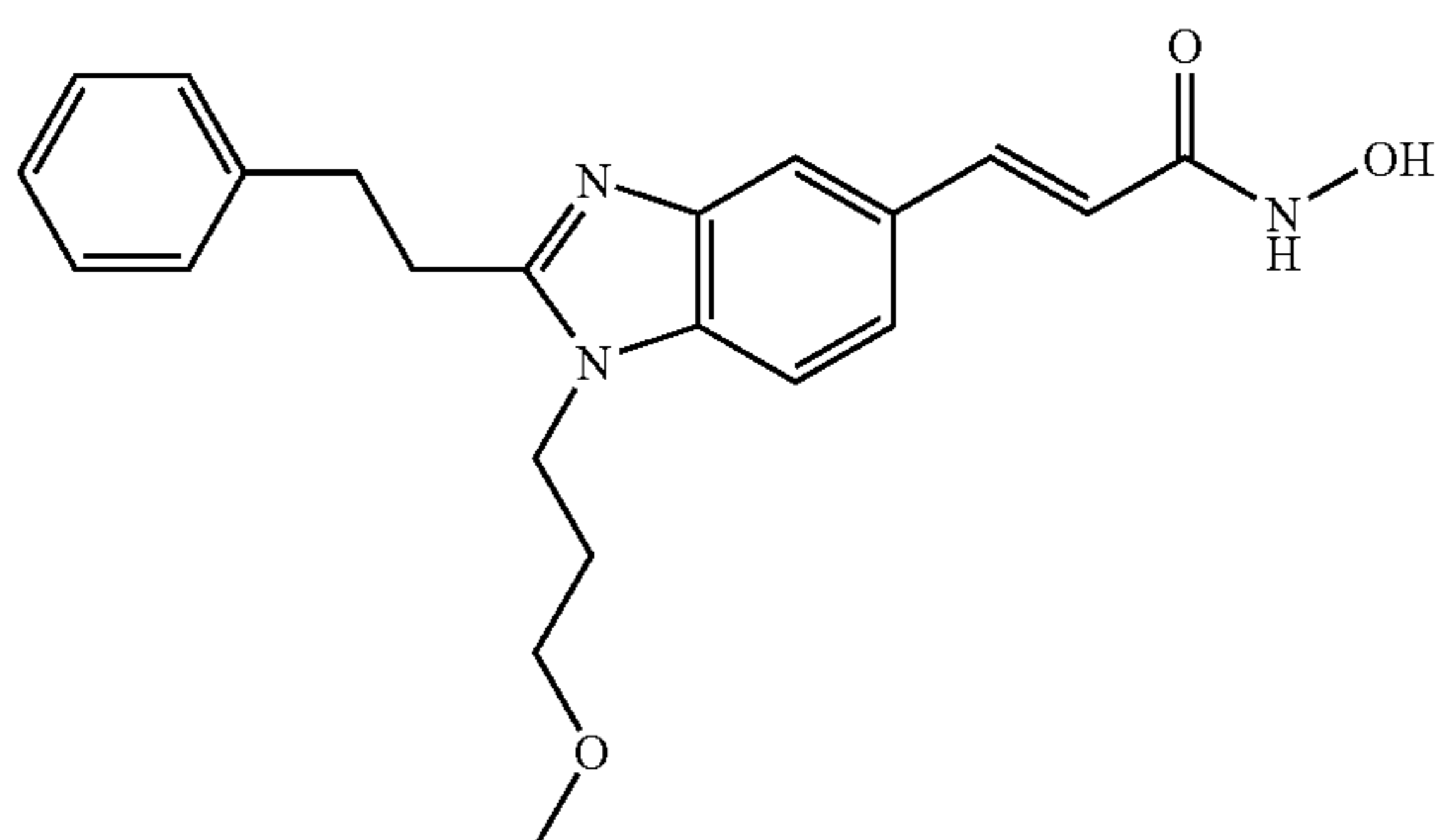
N-Hydroxy-3-[1-(3-methoxy-propyl)-2-phenethyl-1H-benzimidazol-5-yl]-acrylamide
