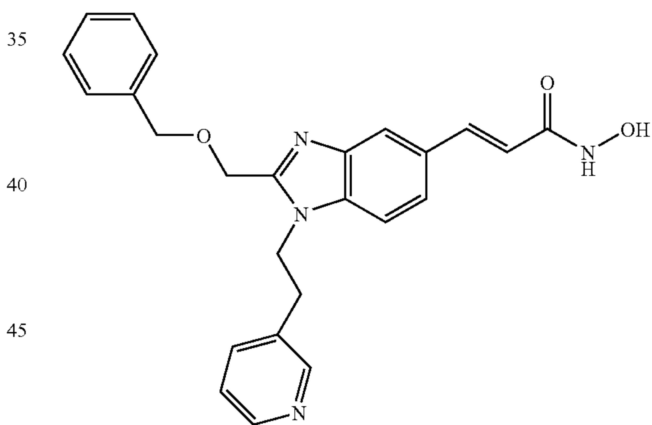
N-Hydroxy-3-[2-Benzyloxymethyl-1-(2-pyridin-3-ethyl)-1H-benzimidazol-5-yl]-acrylamide
