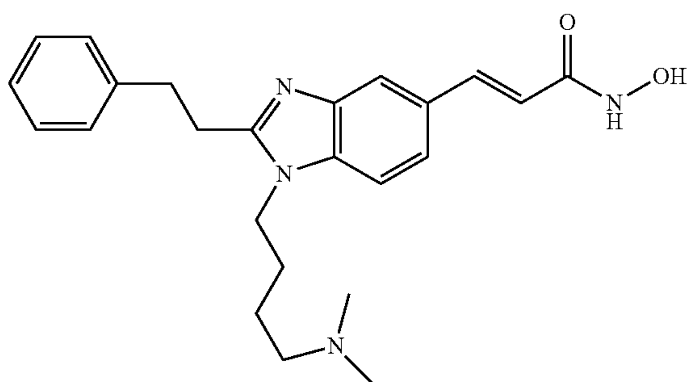
N-Hydroxy-3-[1-(4-dimethylamino-butyl)-2-phenethyl-1H-benzimidazol-5-yl]-acrylamide
