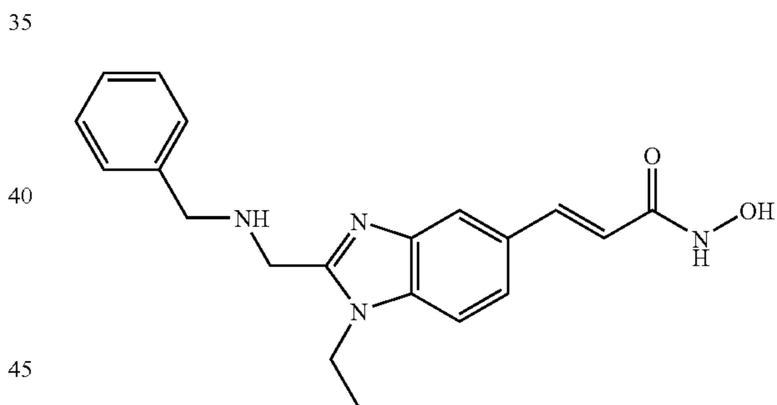
N-Hydroxy-3-[2-(benzylamino-methyl)-ethyl-1H-benzimidazol-5-yl]-acrylamide
