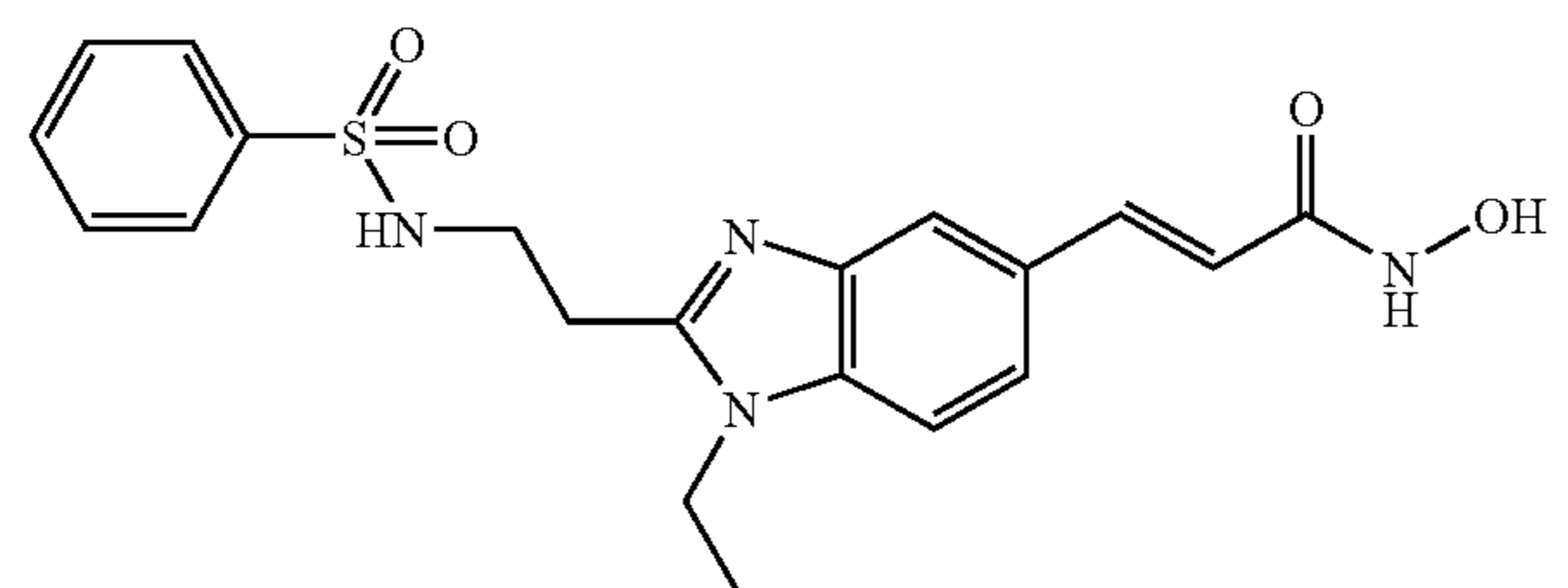
N-Hydroxy-3-[2-(2-benzenesulfonylamino-ethyl)-1-ethyl-1H-benzimidazol-5-yl]-acrylamide
