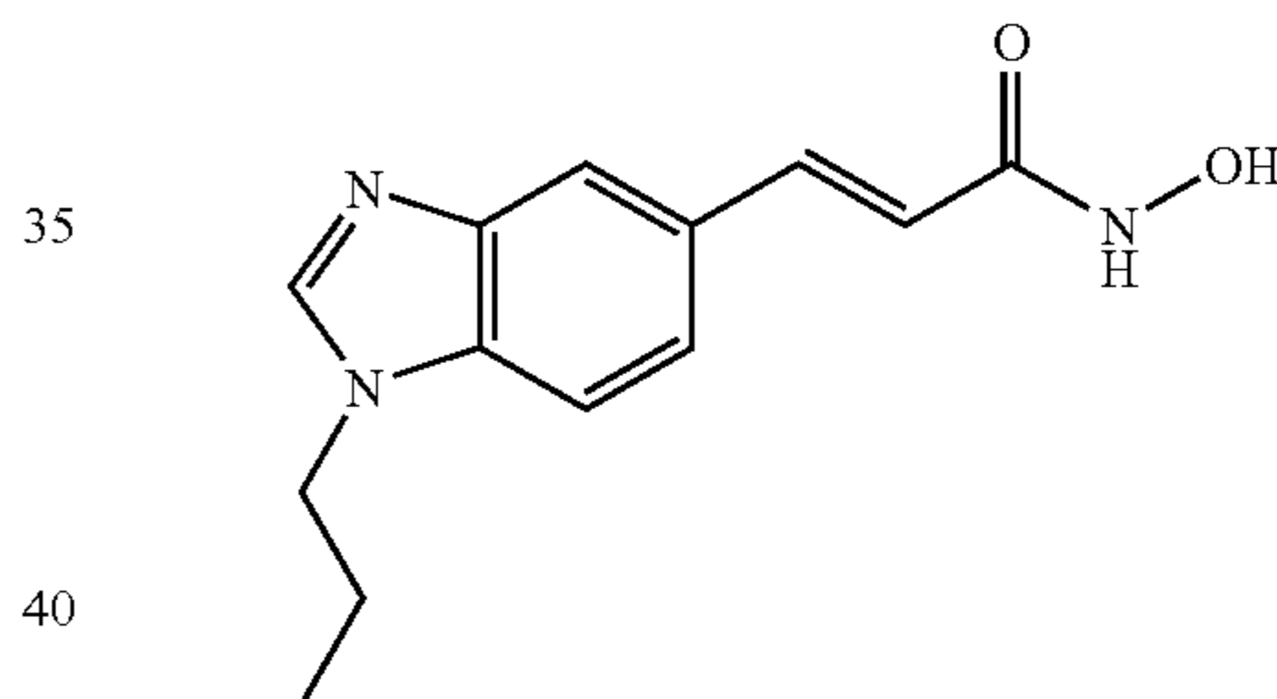
N-Hydroxy-3-(1-propyl-1H-benzimidazol-5-yl)-acrylamide
