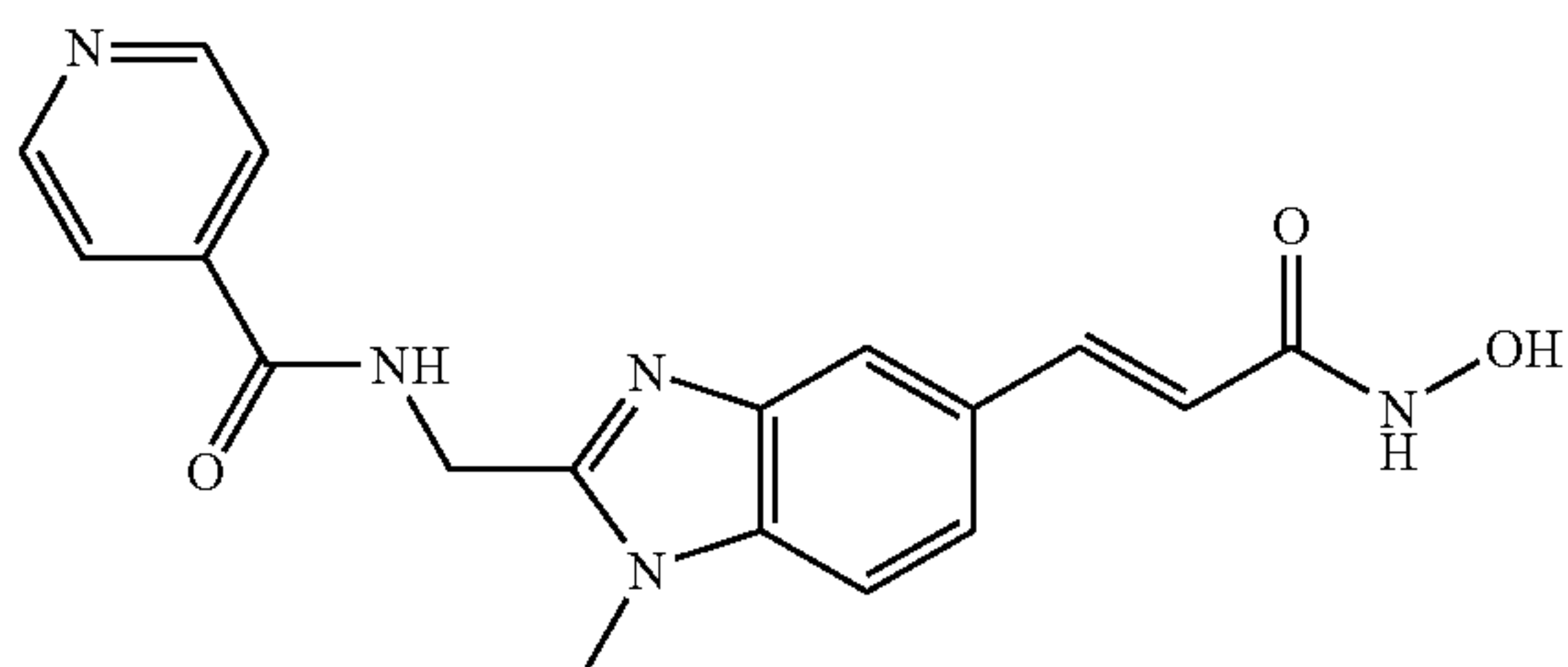
N-[5-(2-Hydroxycarbonyl-vinyl)-1-methyl-1H-benzimidazol-2-ylmethyl]-isonicotinamide
