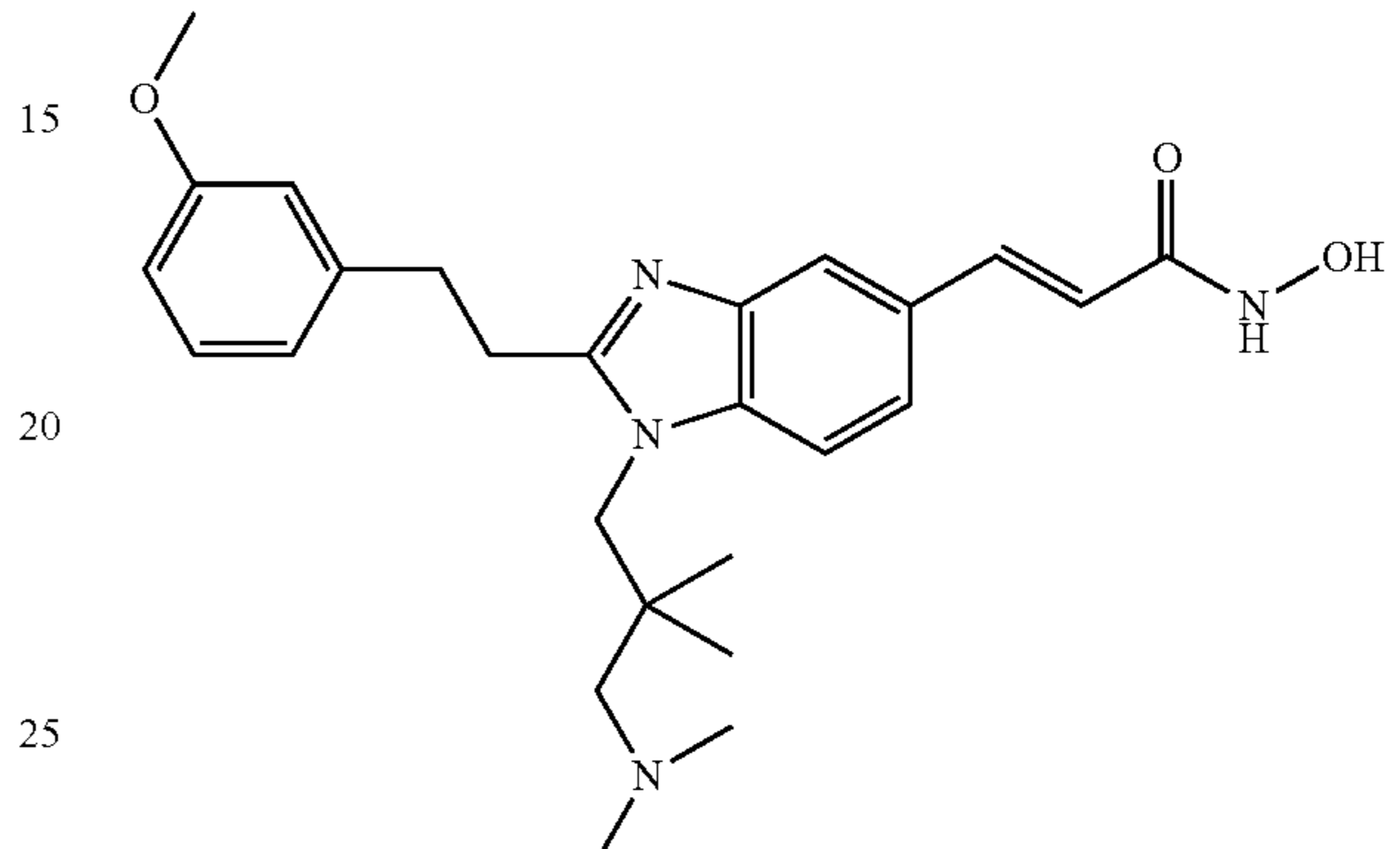
N-Hydroxy-3-[1-(3-dimethylamino-2,2-dimethyl-propyl)-2-[2-(3-methoxy-phenyl)-ethyl]-1H-benzimidazol-5-yl]-acrylamide
