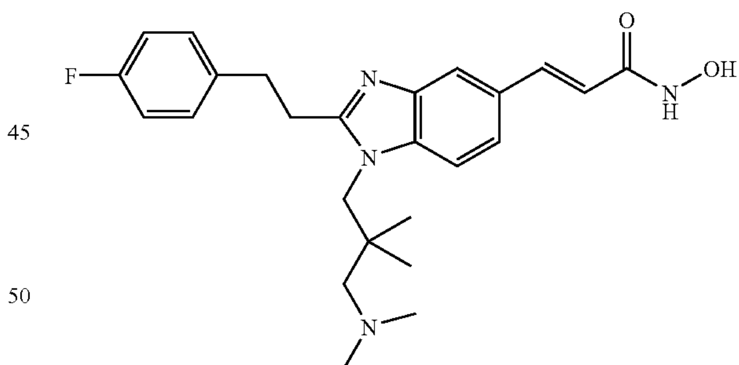
N-Hydroxy-3-{1-(3-Dimethylamino-2,2-dimethyl-propyl)-2-[2-(4-fluoro-phenyl)-ethyl]-1H-benzimidazol-5-yl}-acrylamide
