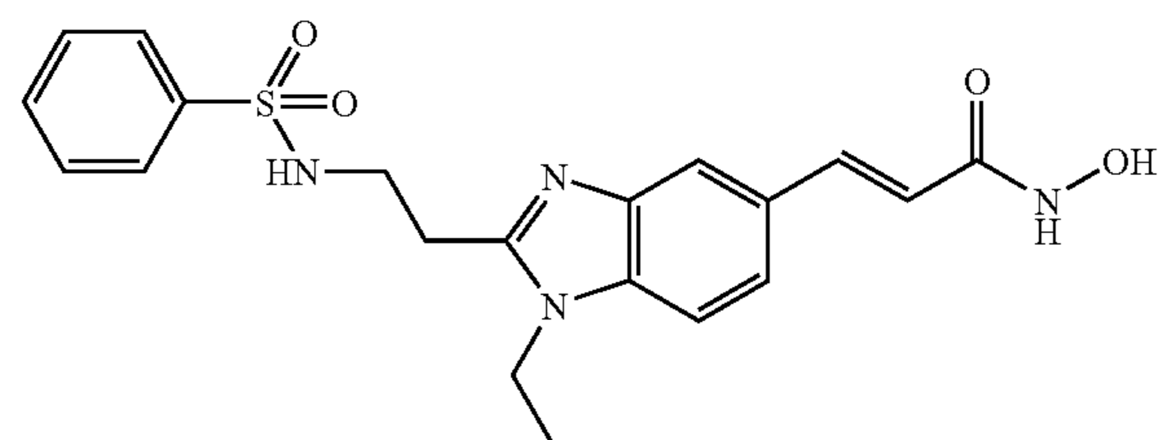
N-Hydroxy-3-[2-(2-benzenesulfonylamino-ethyl)-1-ethyl-1H-benzimidazol-5-yl]-acrylamide
