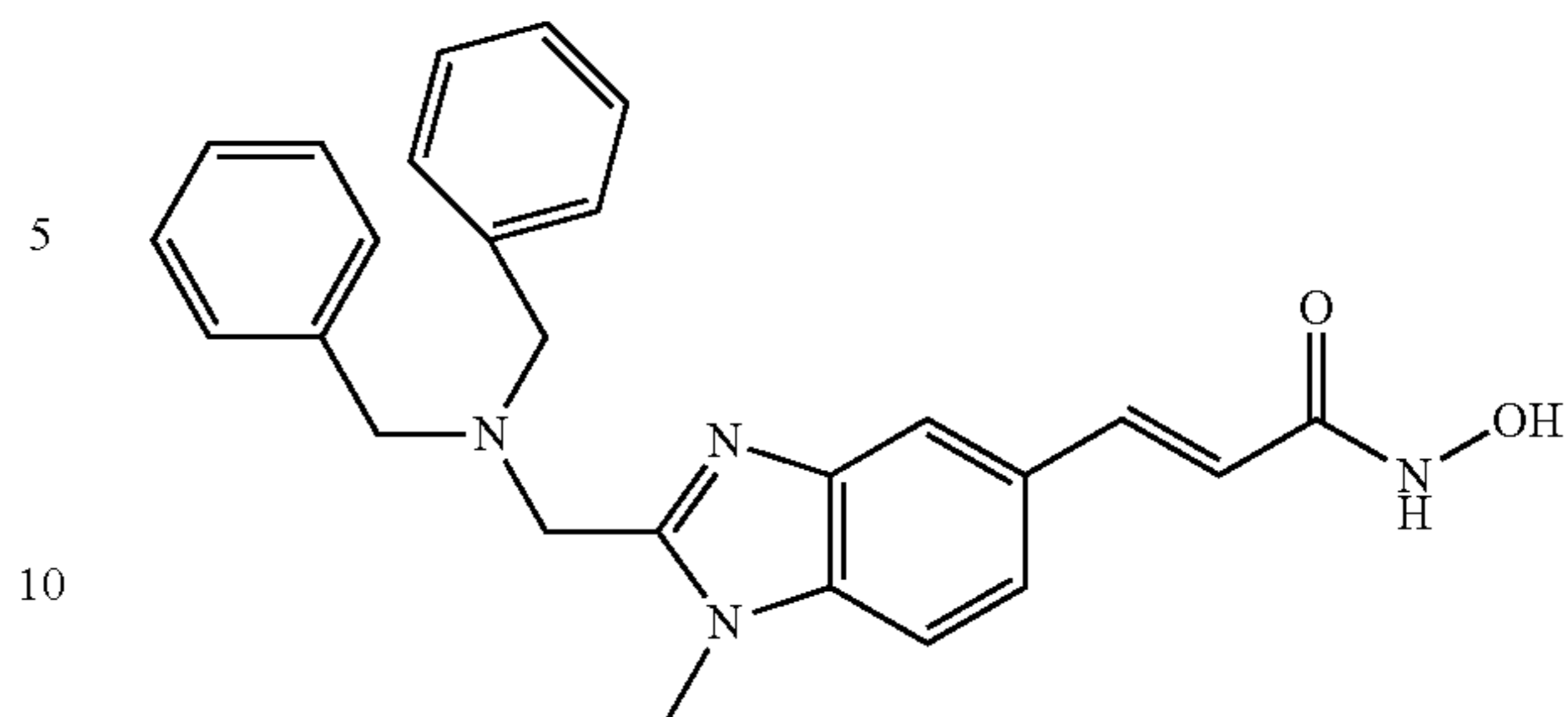
N-Hydroxy-3-{2-[dibenzylamino)-methyl]-1-methyl-1H-benzimidazol-5-yl}-acrylamide
