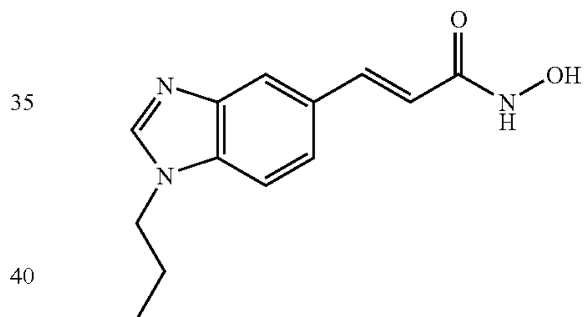
N-Hydroxy-3-(1-propyl-1H-benzimidazol-5-yl)-acrylamide
