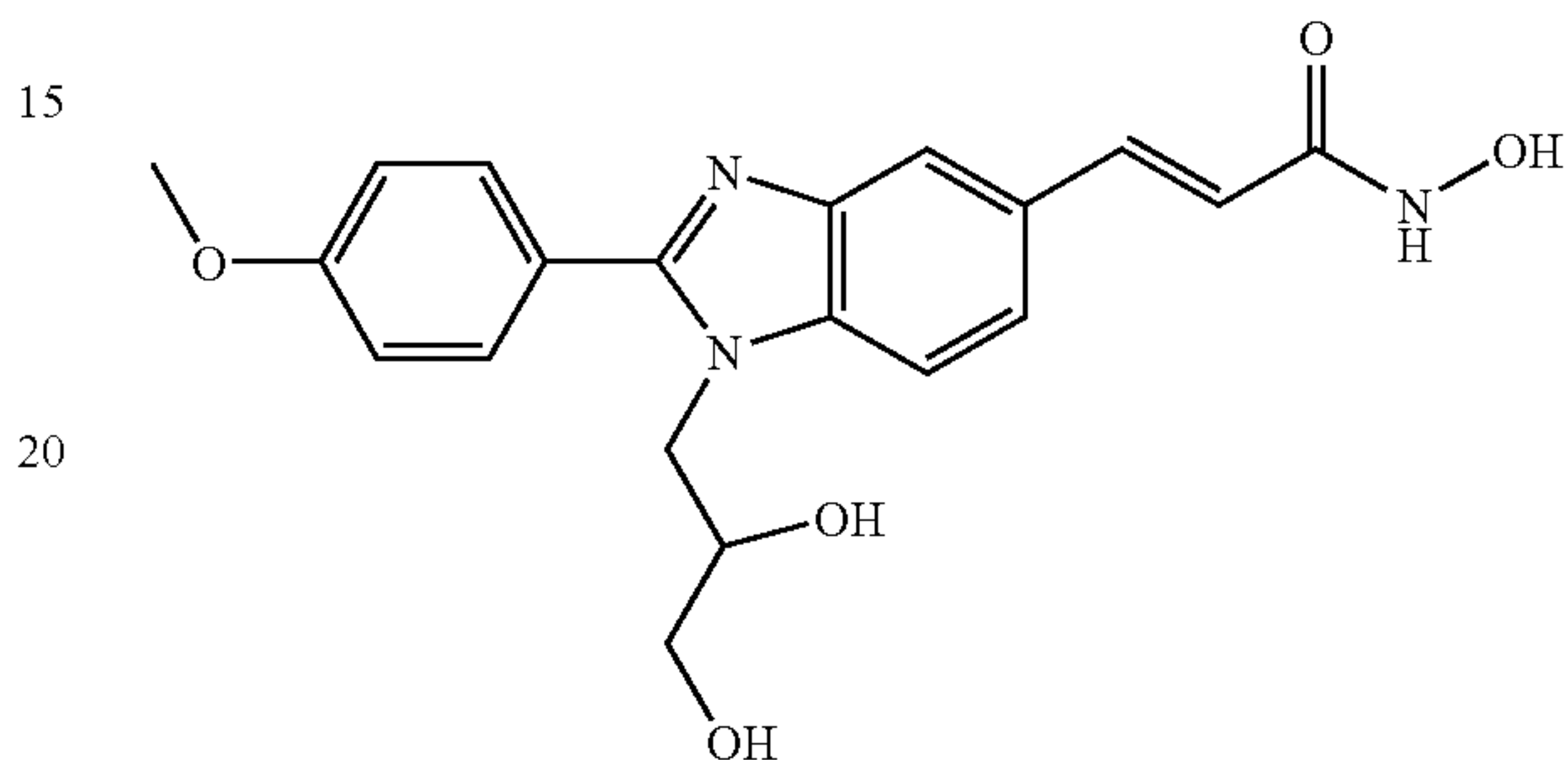
N-Hydroxy-3-[1-(2,3-hydroxy-propyl)-2-(4-methoxy-phenyl)-1H-benzimidazole-5-yl]-acrylamide
