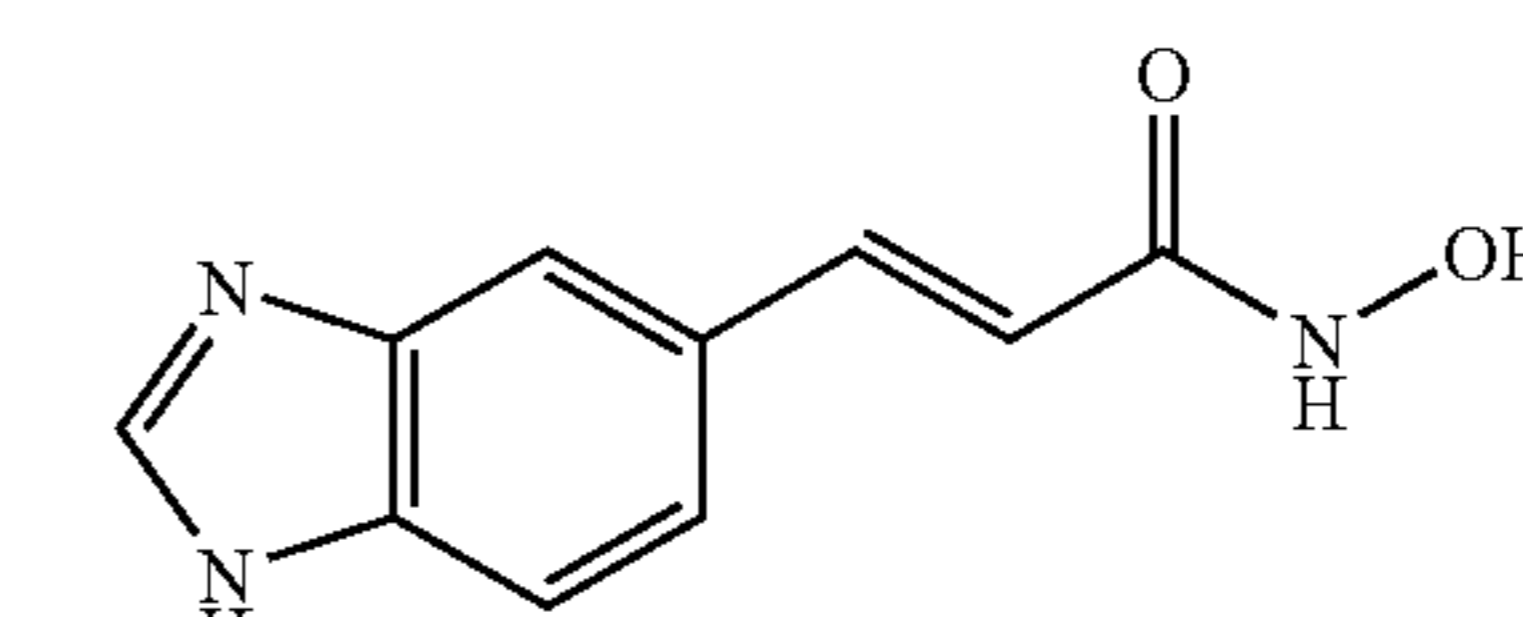
N-Hydroxy-3-(1H-benzimidazol-5-yl)-acrylamide
