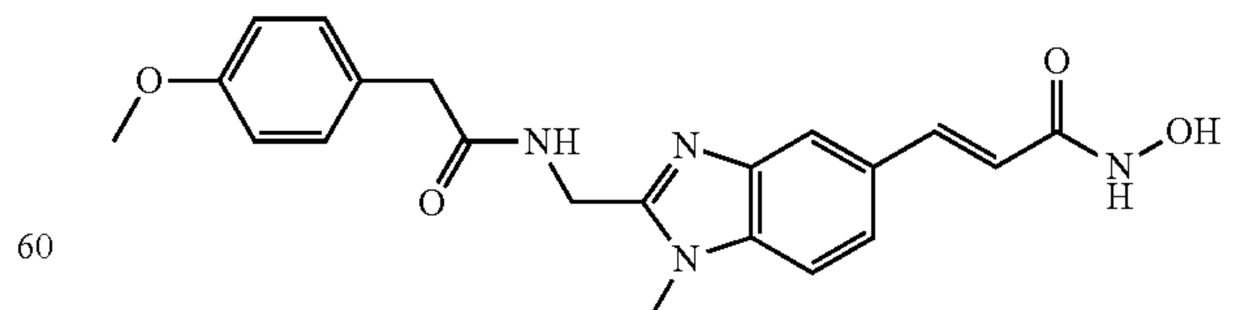
N-Hydroxy-3-(2-[2-(4-methoxy-phenyl)-acetylamino]-methyl)-1-methyl-1H-benzimidazol-5-yl]-acrylamide;
