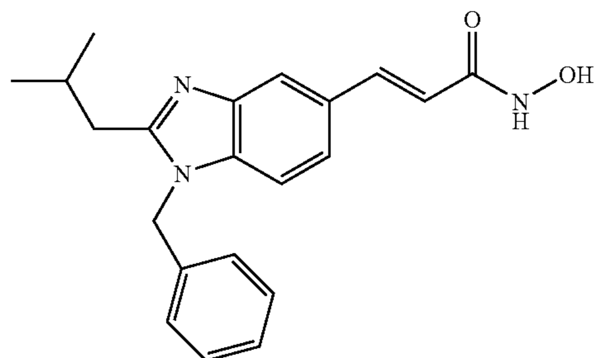
N-Hydroxy-3-(1-Benzyl-2-isobutyl-1H-benzimidazol-5-yl)-acrylamide
