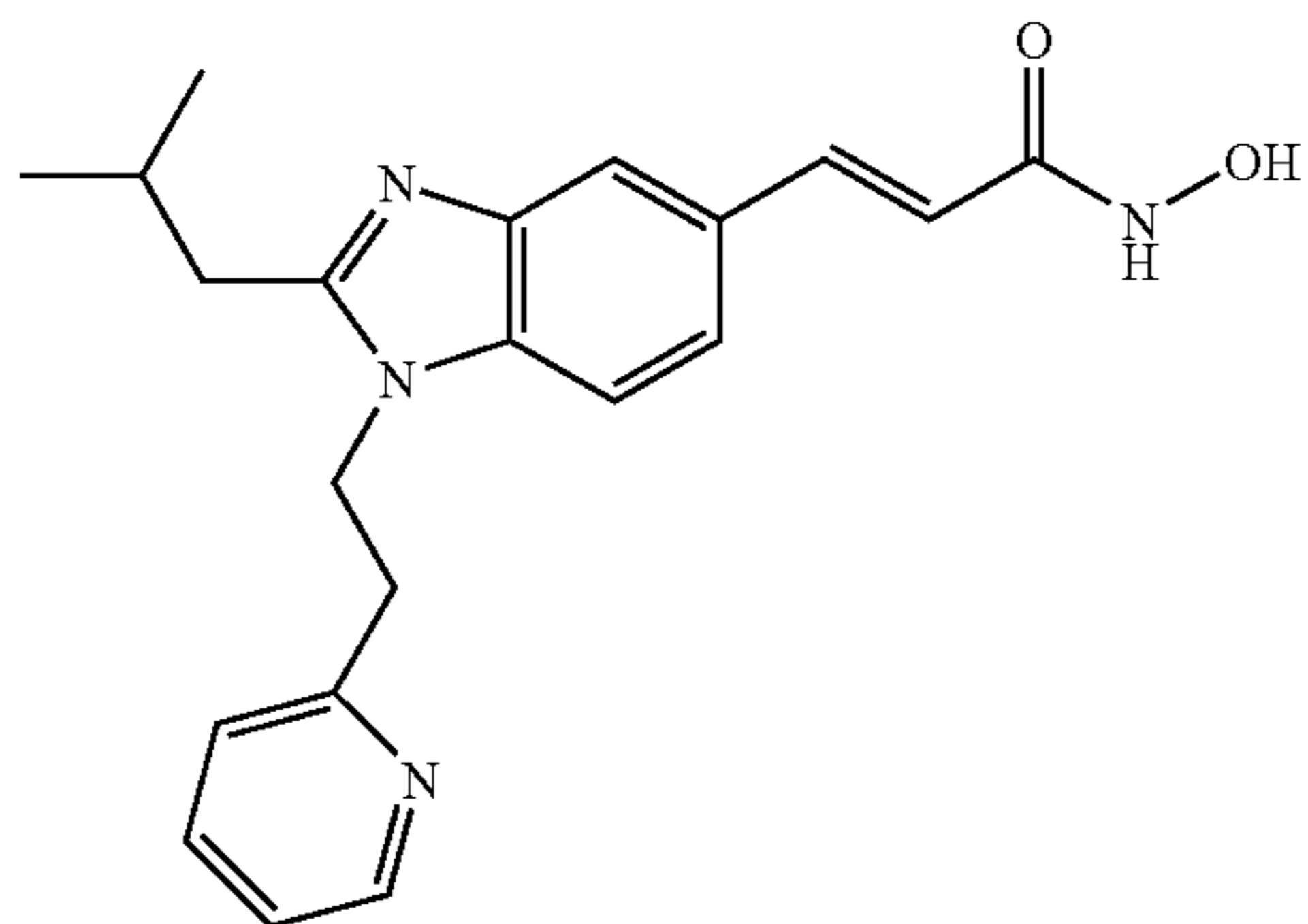
N-Hydroxy-3-[2-isobutyl-1-(2-pyridin-2-yl-ethyl)-1H-benzimidazol-5-yl]-acrylamide
