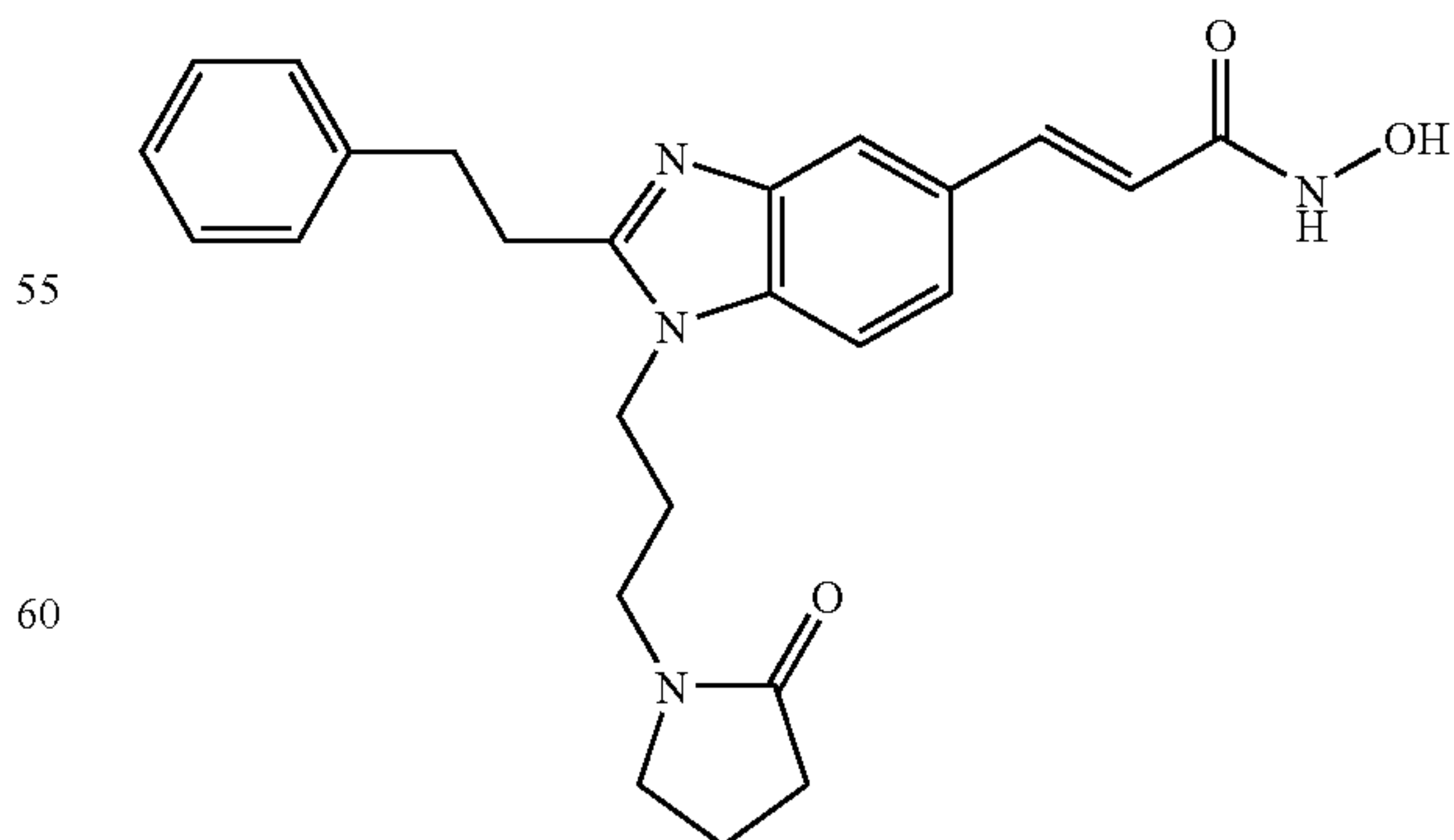
N-Hydroxy-3-{1-[3-(2-oxo-pyrrolidin-1-yl)-propyl]-2-phenethyl-1H-benzimidazol-5-yl}-acrylamide
