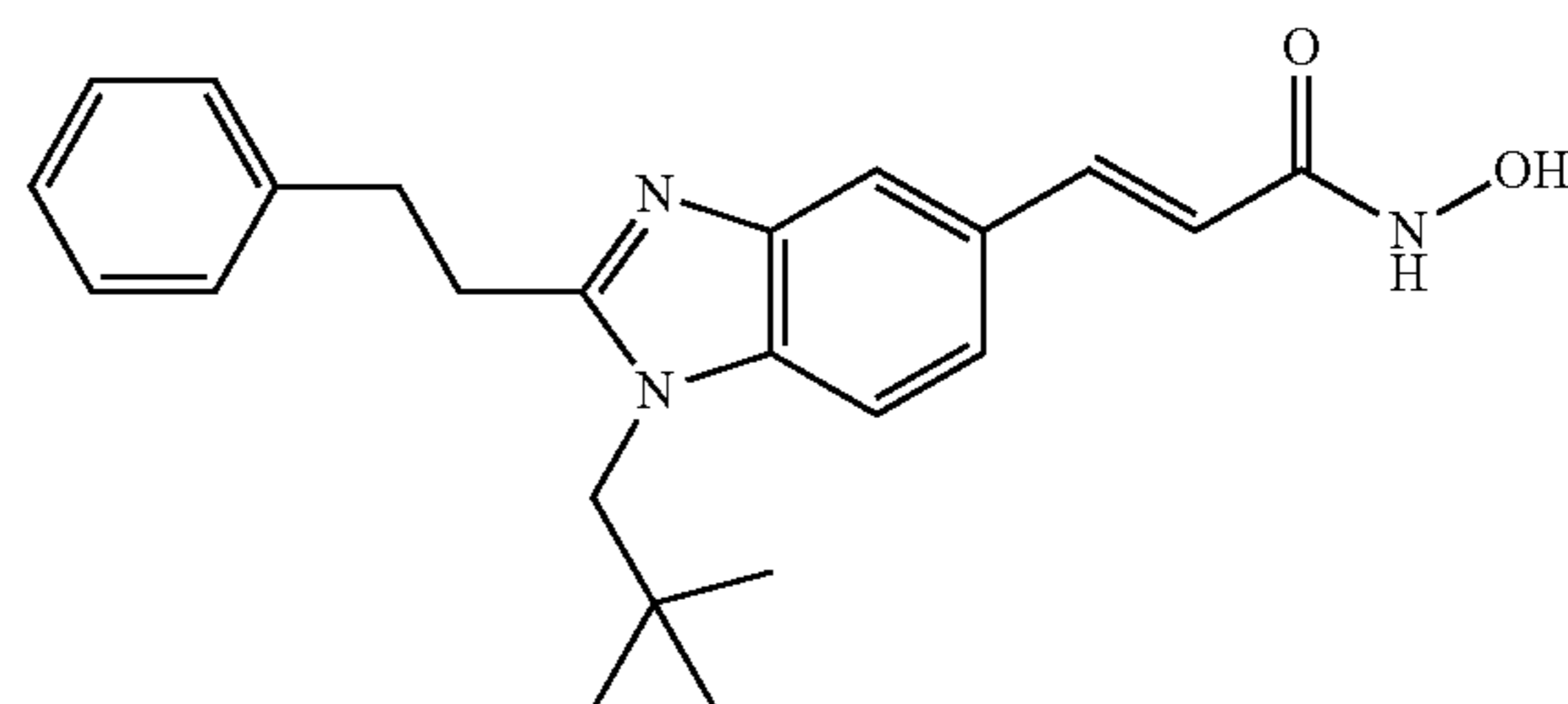
N-Hydroxy-3-[1-(2,2-dimethyl-propyl)-2-phenethyl-1H-benzimidazol-5-yl]-acrylamide
