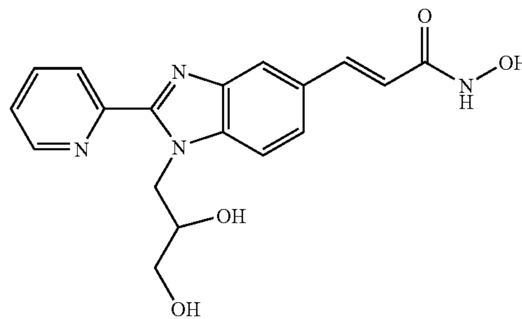
N-Hydroxy-3-[1-(2,3-hydroxy-propyl)-2-(2-pyridyl)-1H-benzimidazole-5-yl]-acrylamide
