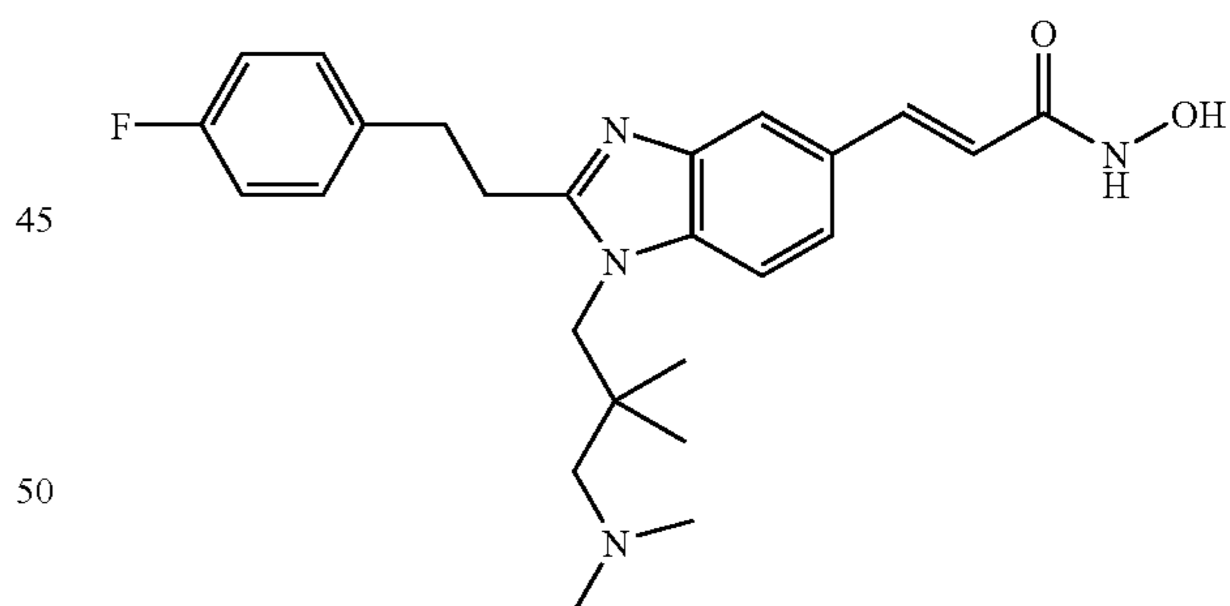
N-Hydroxy-3-{1-(3-Dimethylamino-2,2-dimethyl-propyl)-2-[2-(4-fluoro-phenyl)-ethyl]-1H-benzimidazol-5-yl}-acrylamide
