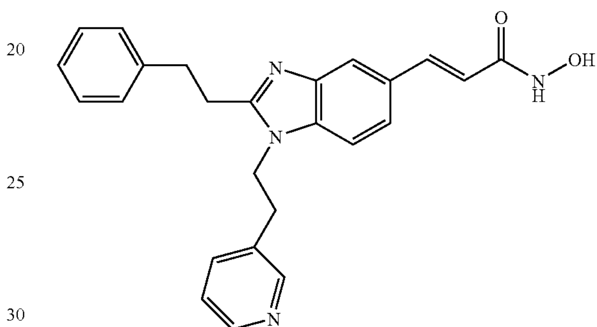
N-Hydroxy-3-(2-phenethyl-1-(2-pyridin-3-yl-ethyl)-1H-benzimidazol-5-yl)-acrylamide
