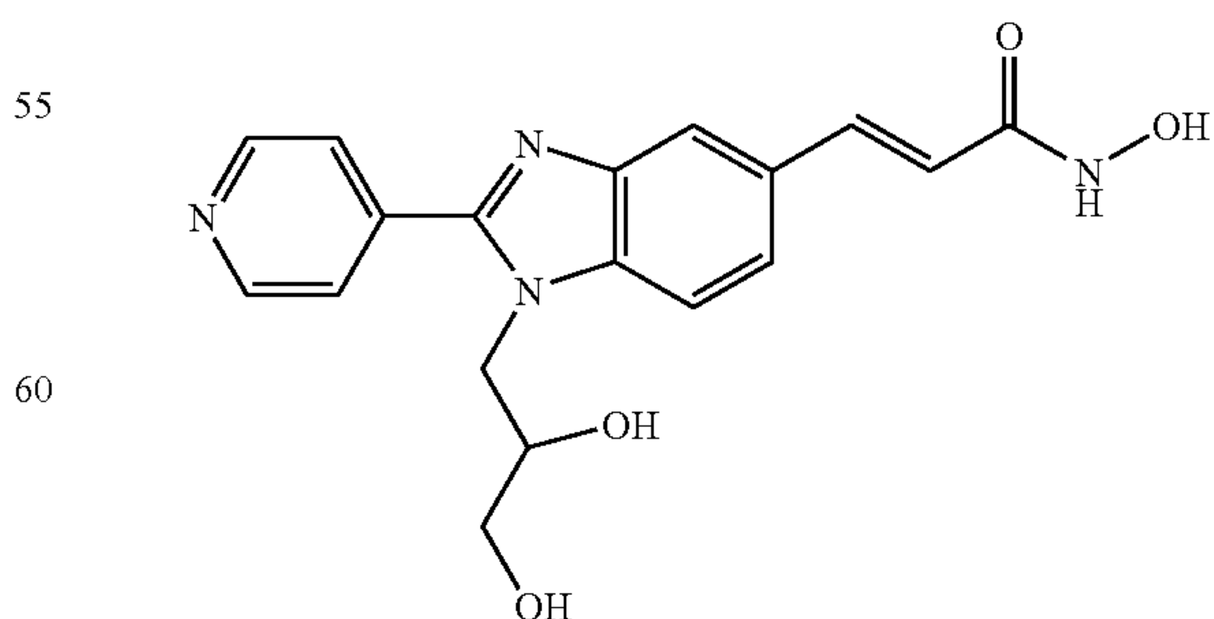
N-Hydroxy-3-[1-(2,3-hydroxy-propyl)-2-(4-pyridyl)-1H-benzimidazole-5-yl]-acrylamide
