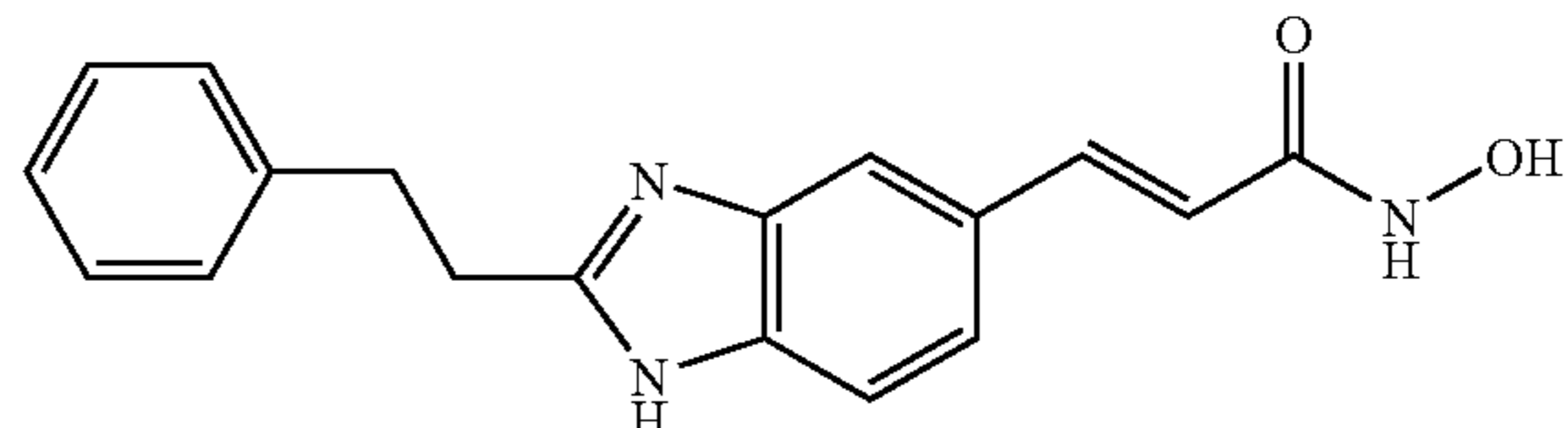
N-Hydroxy-3-(2-phenethyl-1H-benzimidazol-5-yl)-acrylamide
