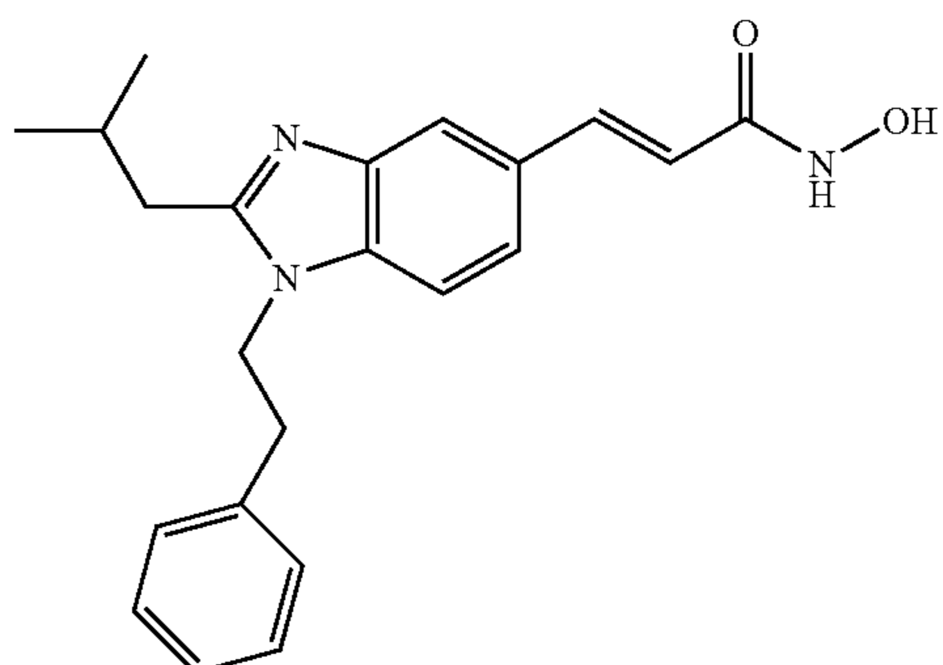
N-Hydroxy-3-(2-isobutyl-1-phenethyl-1H-benzimidazol-5-yl)-acrylamide
