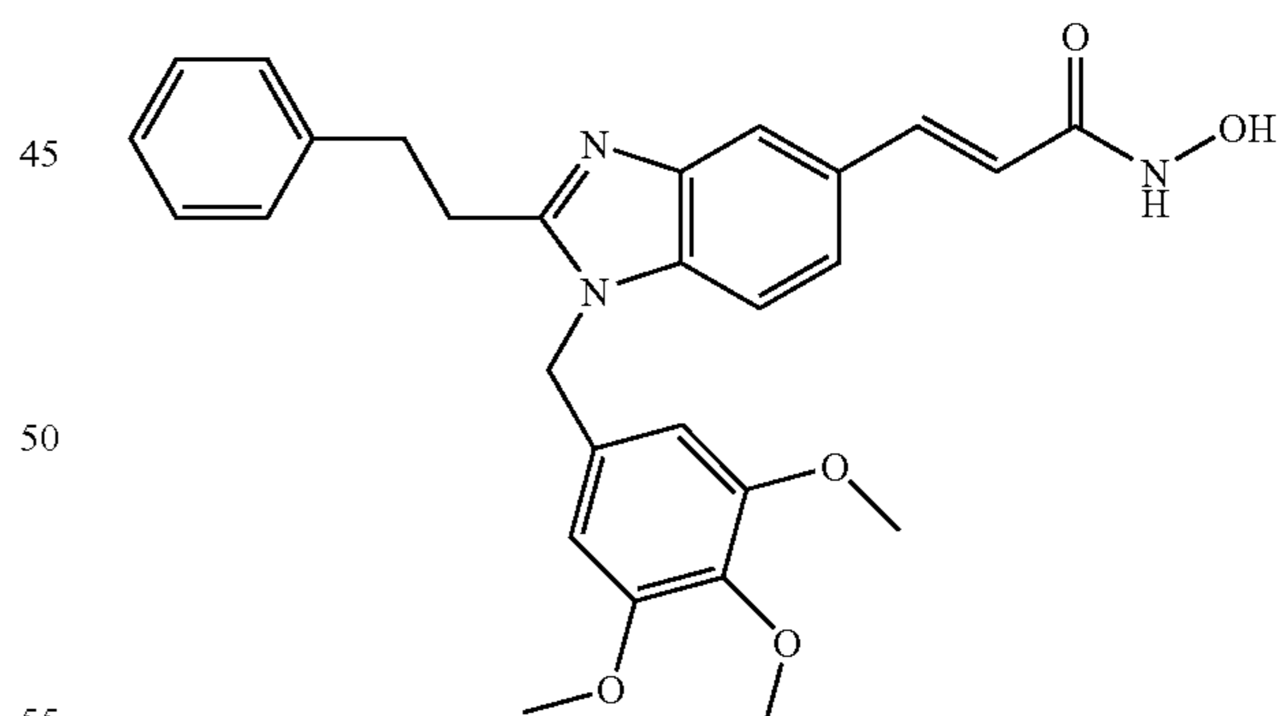
N-Hydroxy-3-[1-(3,4,5-trimethoxybenzyl)-2-(2-phenyl-ethyl)-1H-benzimidazol-5-yl]-acrylamide
