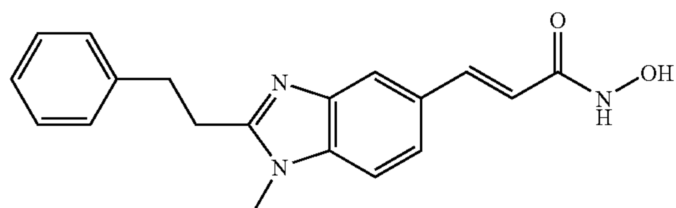
N-Hydroxy-3-(1-methyl-2-phenethyl-1H-benzimidazol-5-yl)-acrylamide
