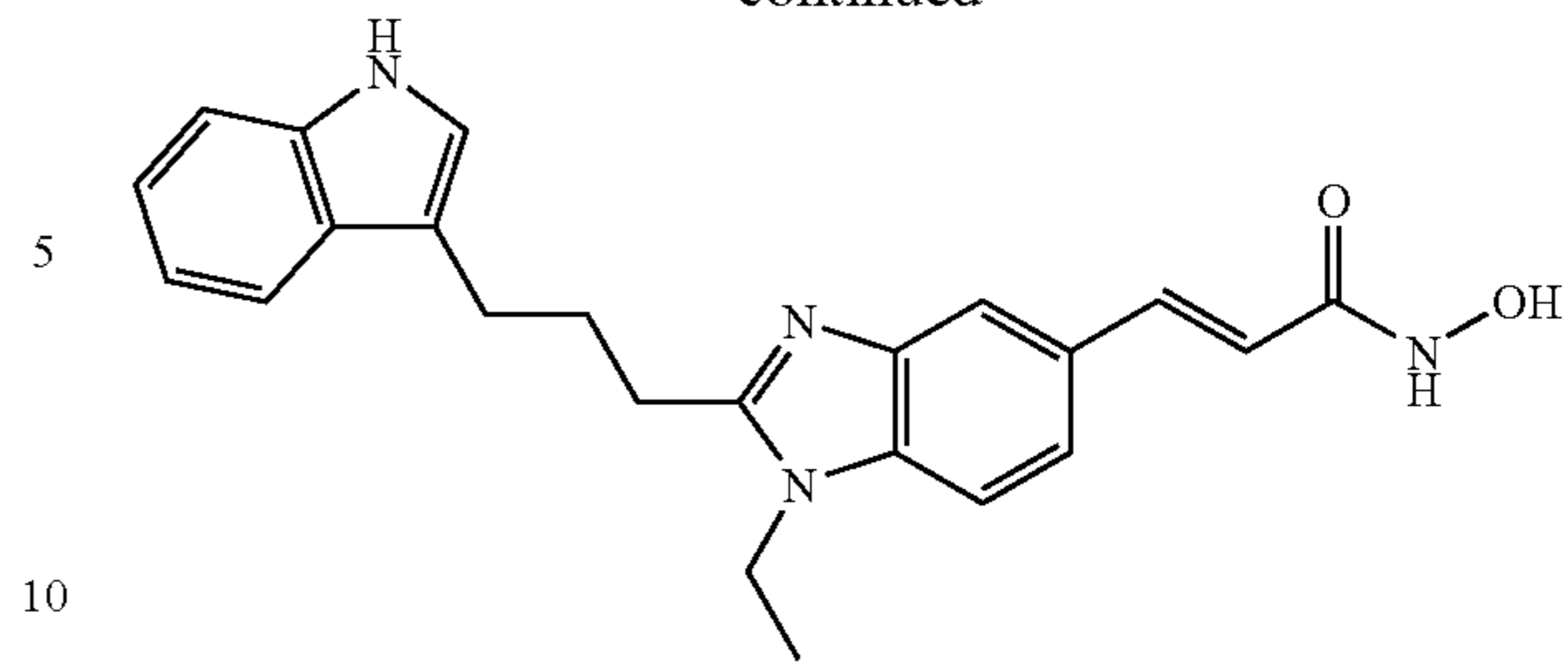
N-Hydroxy-3-[1-ethyl-2-[3-(1H-indol-3-yl)-propyl]-1H-benzimidazol-5-yl]-acrylamide
