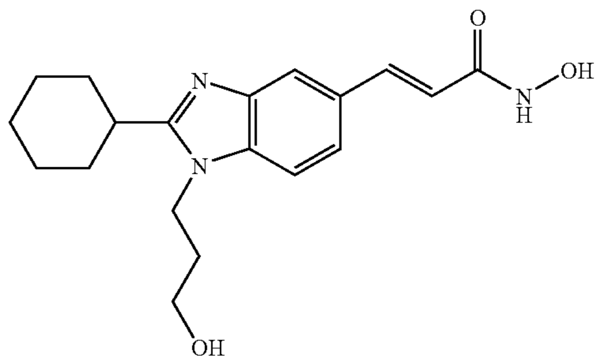
N-Hydroxy-2-cyclohexyl-1-(3-hydroxy-propyl)-1H-benzimidazol-5-yl]-acrylamide
