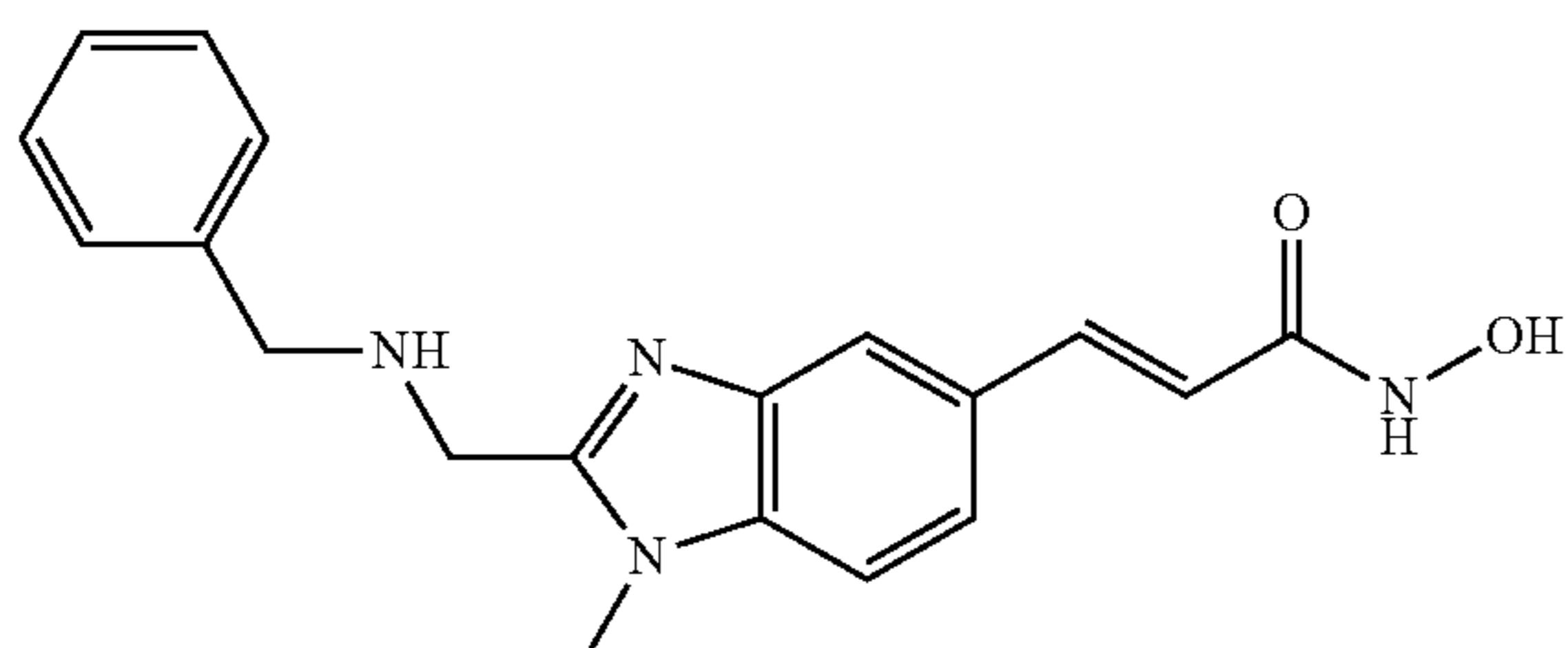
N-Hydroxy-3-[2-(benzylamino-methyl)-1-methyl-1H-benzimidazol-5-yl]-acrylamide
