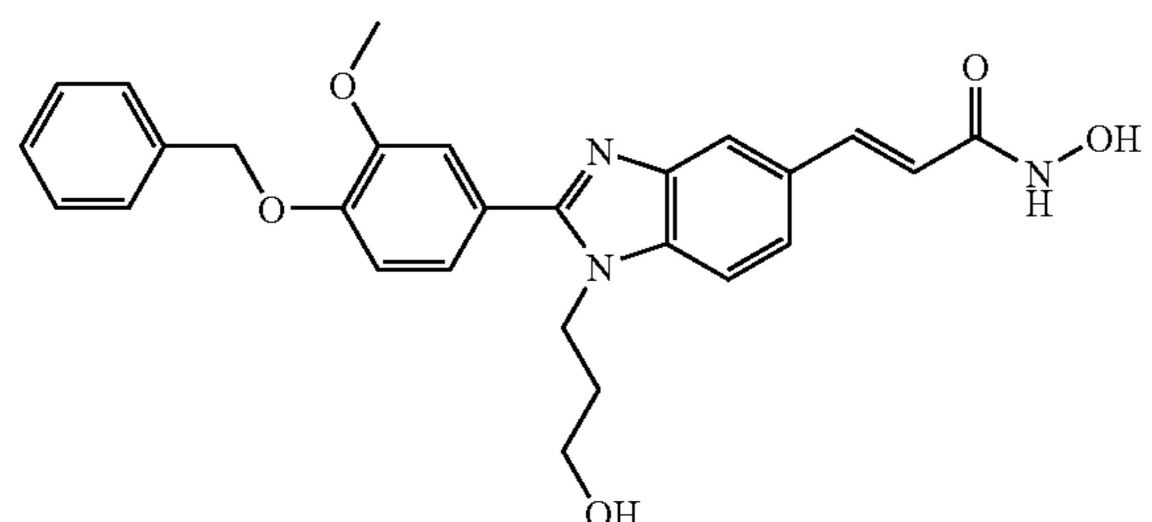
N-Hydroxy-3-[2-(4-benzyloxy-3-methoxy-phenyl)-1-(3-hydroxy-propyl)-1H-benzimidazole-5-yl]-acrylamide
