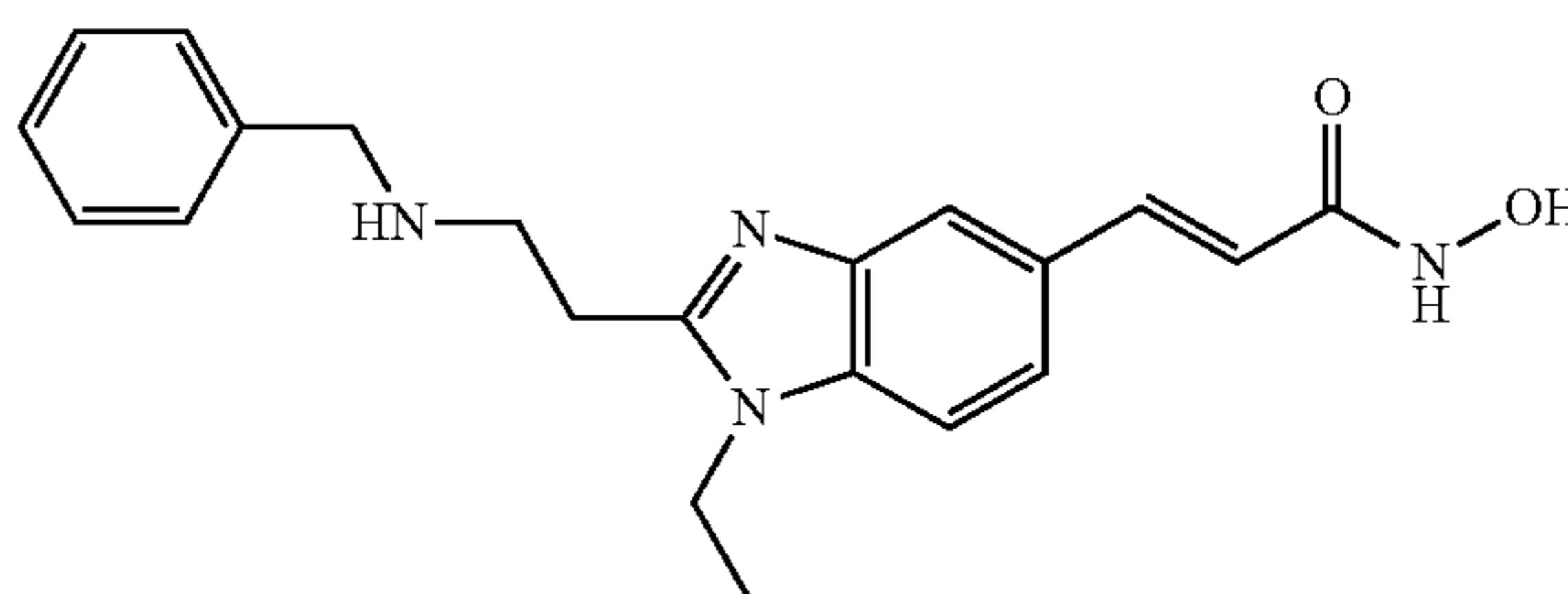
N-Hydroxy-3-[2-(2-benzylamino-ethyl)-1-ethyl-1H-benzimidazol-5-yl]-acrylamide
