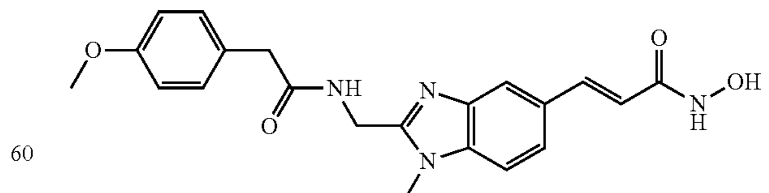
N-Hydroxy-3-(2-[2-(4-methoxy-phenyl)-acetylamino]-methyl)-1-methyl-1H-benzimidazol-5-yl]-acrylamide;
