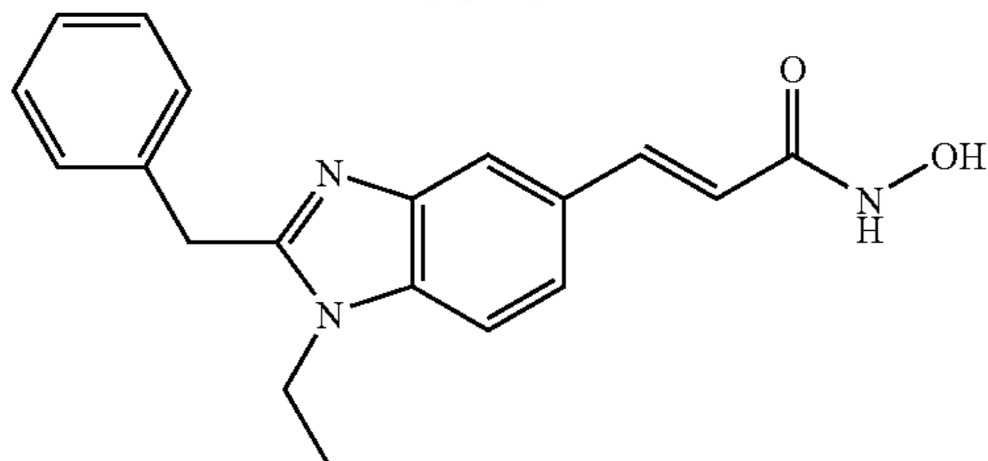
N-Hydroxy-3-(2-benzyl-1-ethyl-1H-benzimidazol-5-yl)-acrylamide
