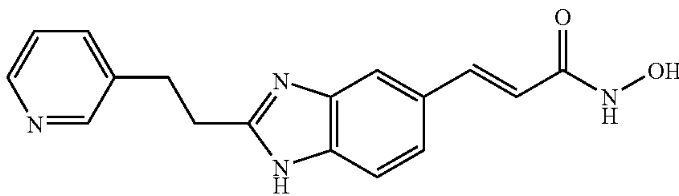
N-Hydroxy-3-[2-(2-pyridin-3-yl-propyl)-1H-benzimidazol-5-yl]-acrylamide
