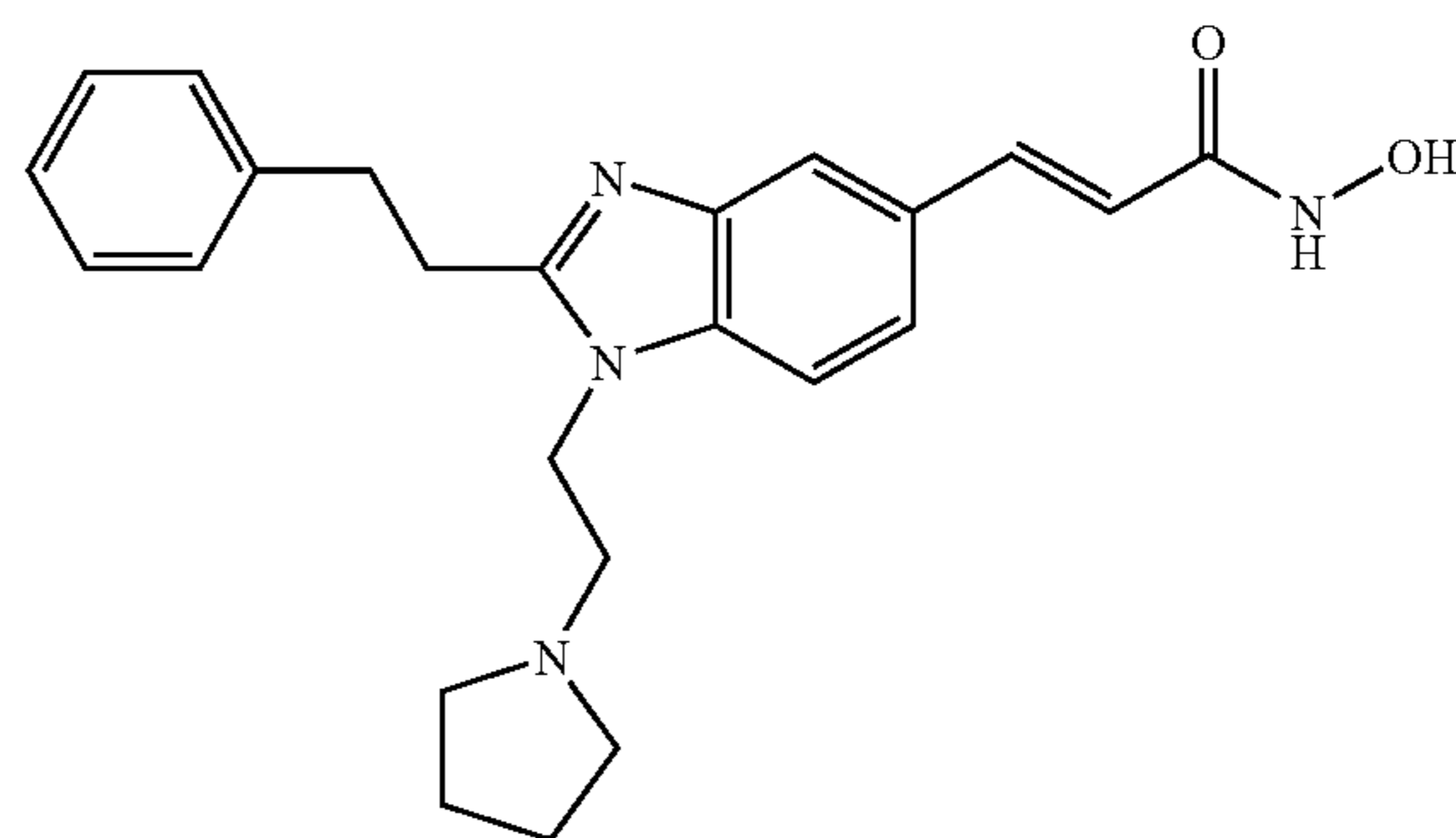
N-Hydroxy-3-[2-phenethyl-1-(2-pyrrolidin-1-yl-ethyl)-1H-benzimidazol-5-yl]-acrylamide
