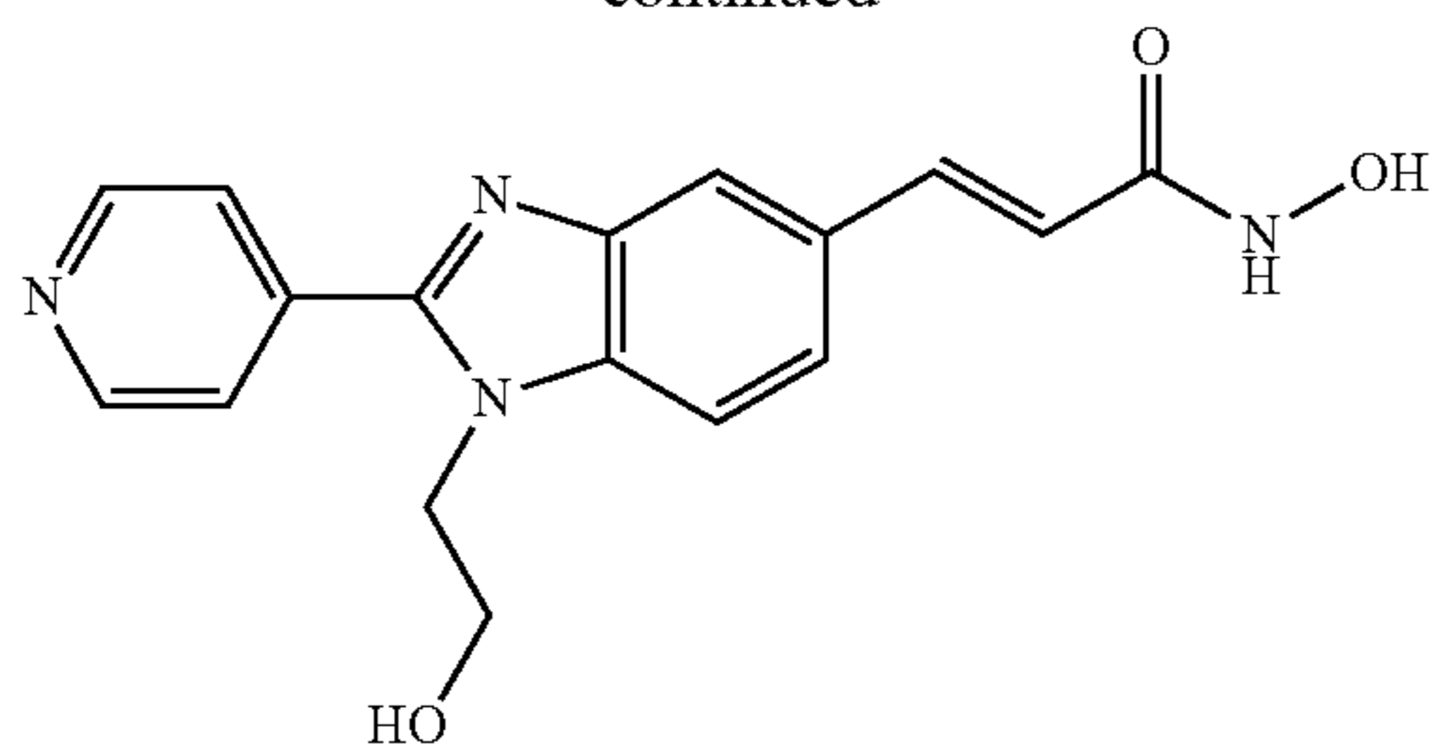
N-Hydroxy-3-[1-(2-hydroxy-ethyl)-2-(4-pyridyl)-1H-benzimidazol-5-yl]-acrylamide
