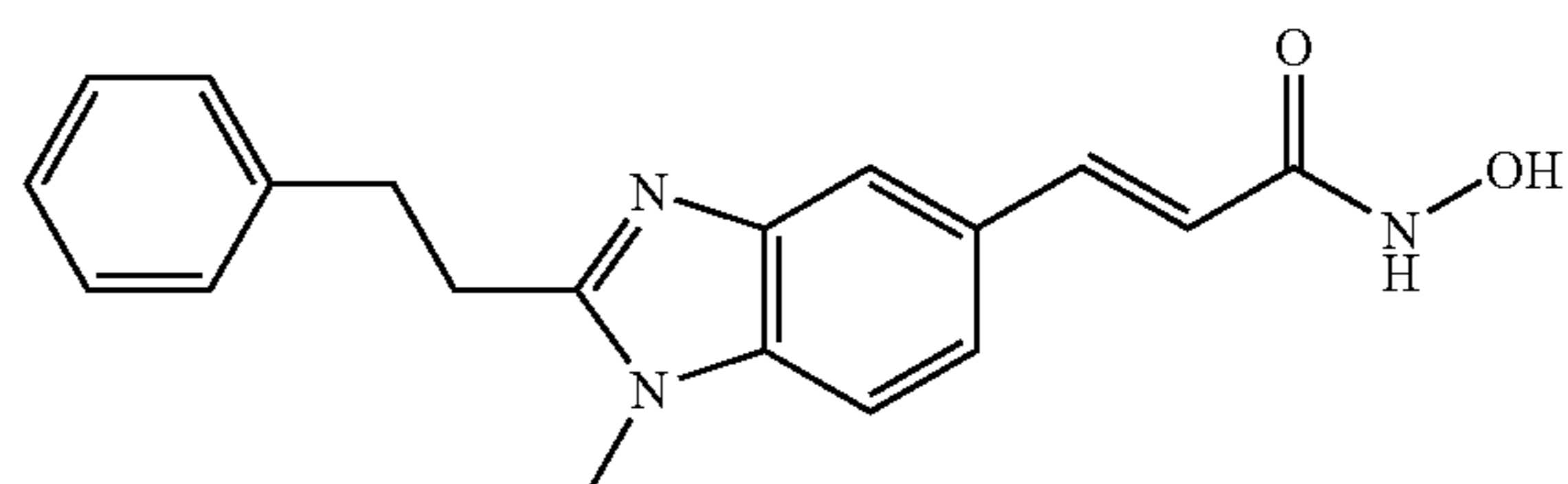
N-Hydroxy-3-(1-methyl-2-phenethyl-1H-benzimidazol-5-yl)-acrylamide
