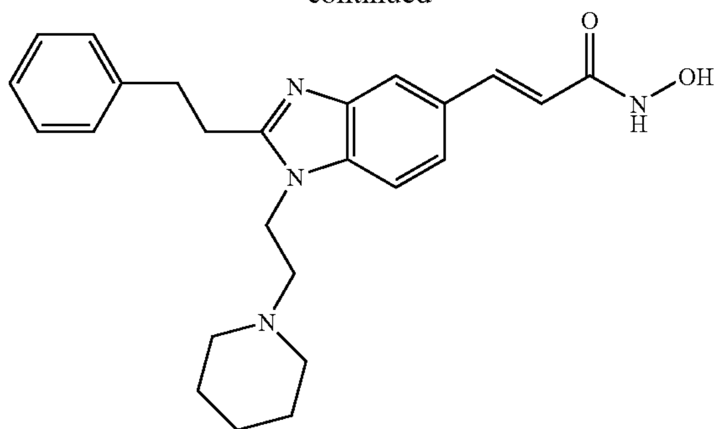
N-Hydroxy-3-[2-phenethyl-1-(piperidin-1-yl-ethyl)-1H-benzimidazol-5-yl]-acrylamide
