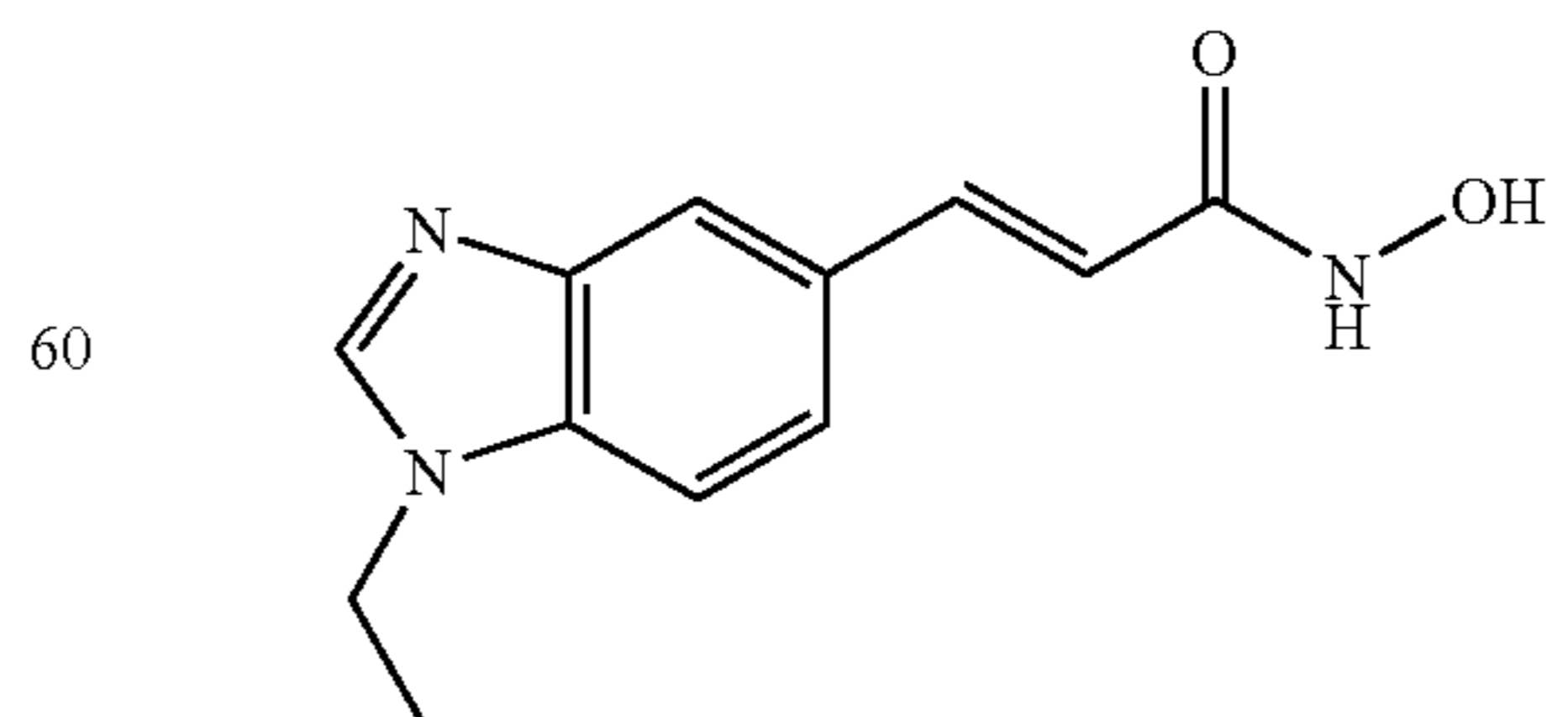
N-Hydroxy-3-(1-Ethyl-1H-benzimidazol-5-yl)-acrylamide
