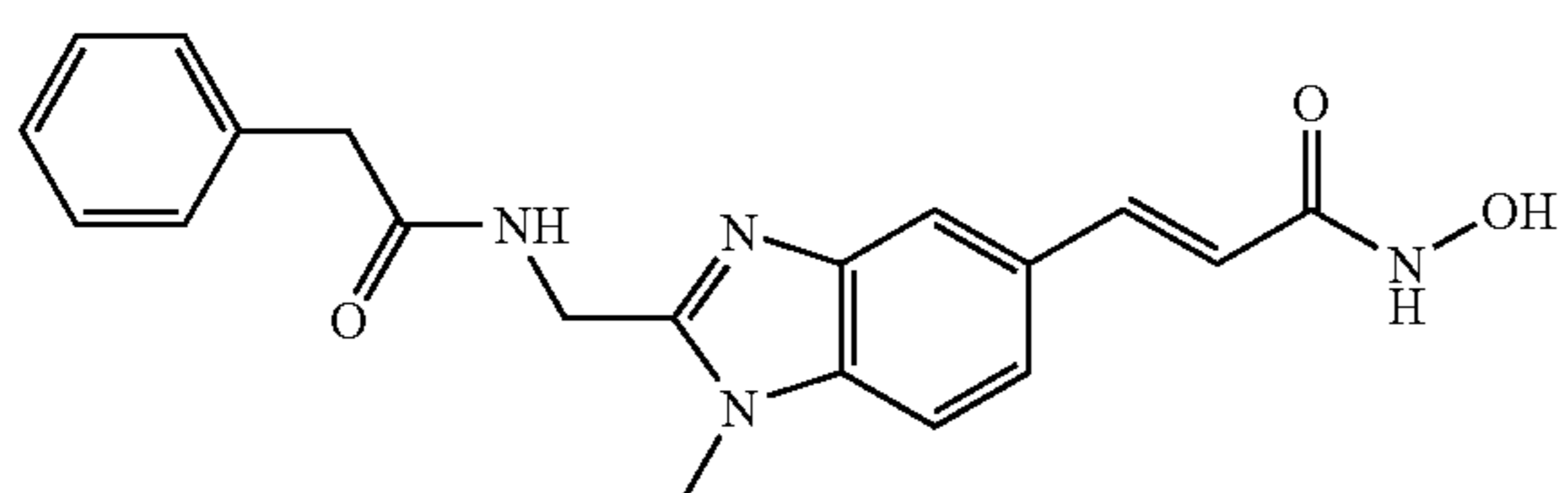
N-Hydroxy-3-[1-methyl-2-(phenylacetyl-amino-methyl)-1H-benzimidazol-5-yl]-acrylamide
