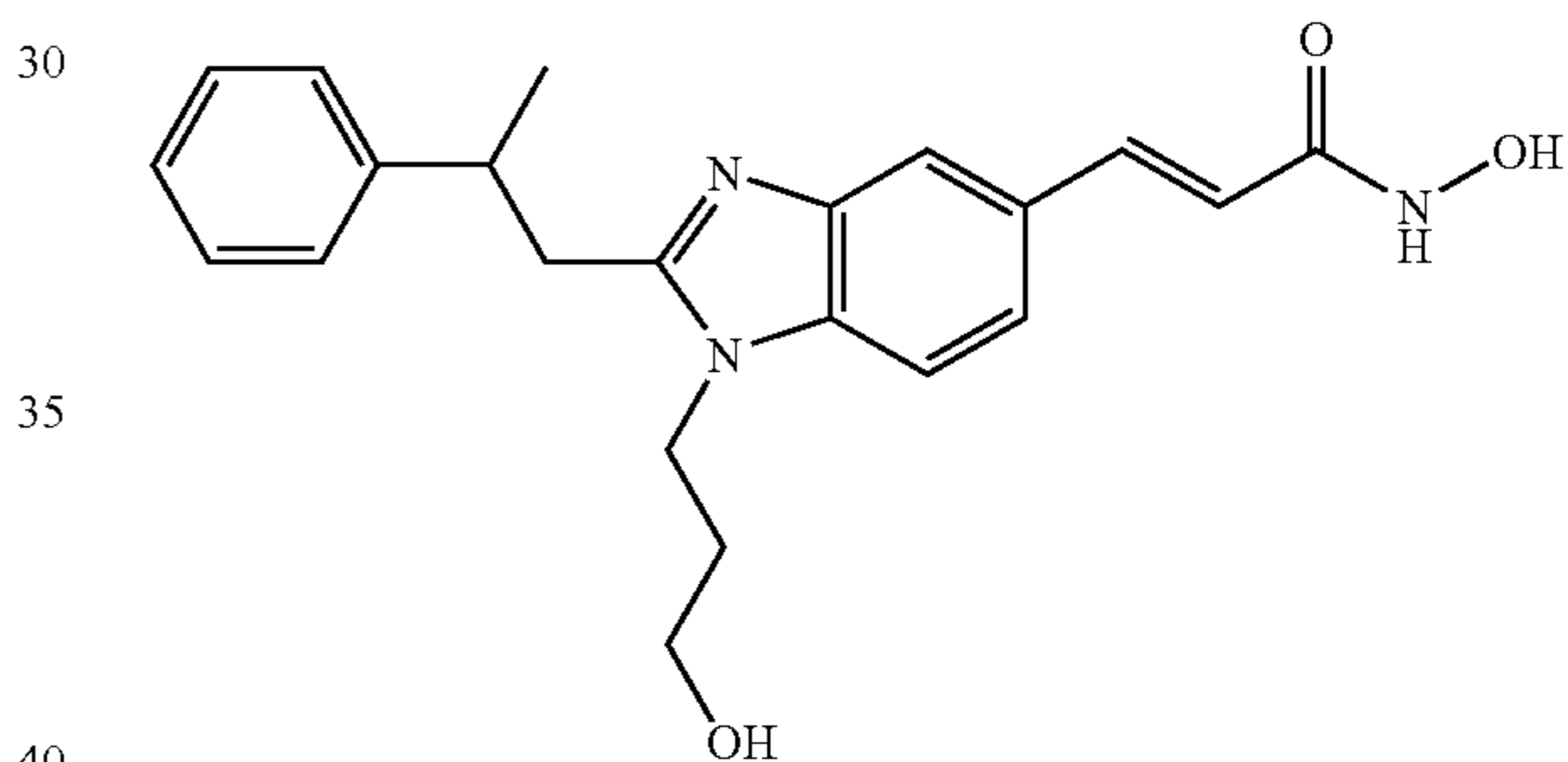
N-Hydroxy-3-[1-(3-hydroxy-propyl)-2-(2-phenyl-propyl)-1H-benzimidazol-5-yl]-acrylamide
