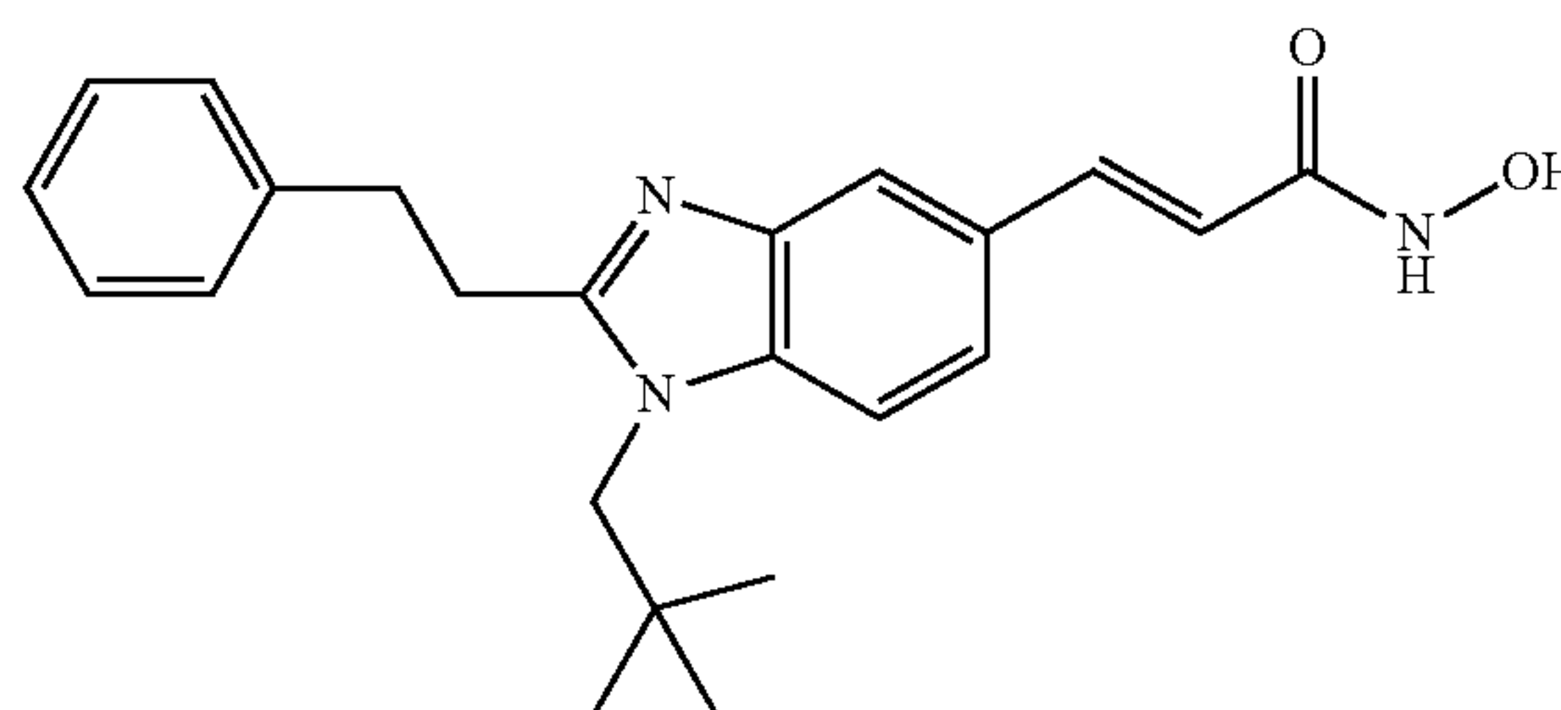
N-Hydroxy-3-[1-(2,2-dimethyl-propyl)-2-phenethyl-1H-benzimidazol-5-yl]-acrylamide
