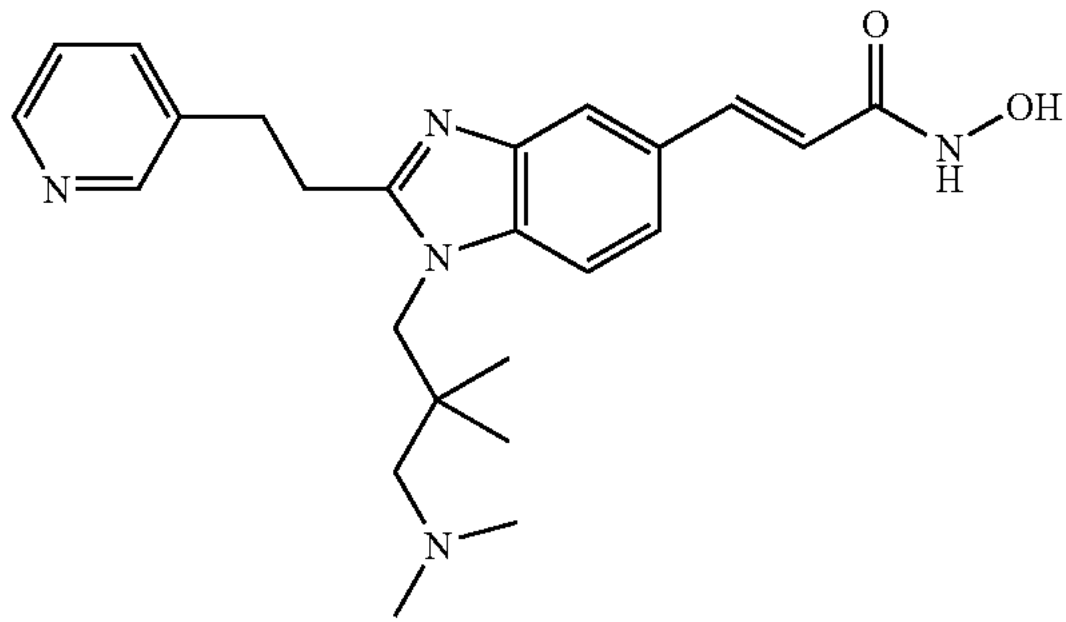
N-Hydroxy-3-[1-(3-Dimethylamino-2,2-dimethyl-propyl)-2-(2-pyridin-3-yl-ethyl)-1H-benzimidazol-5-yl]-acrylamide
