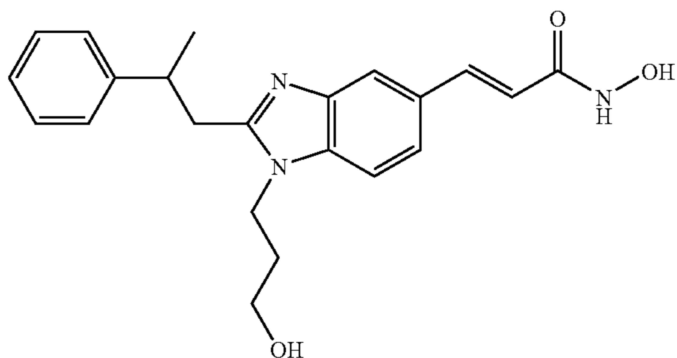
N-Hydroxy-3-[1-(3-hydroxy-propyl)-2-(2-phenyl-propyl)-1H-benzimidazol-5-yl]-acrylamide
