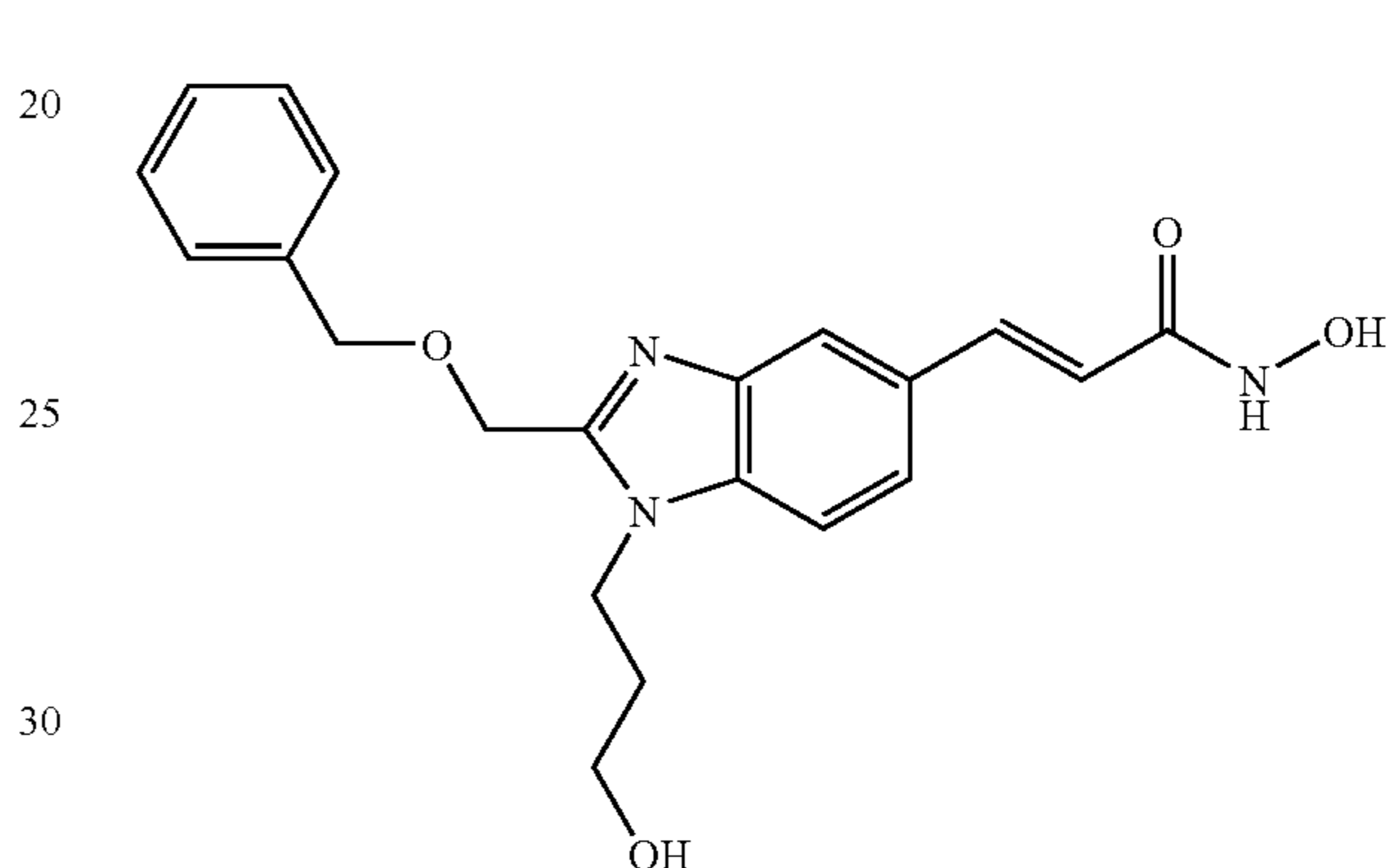
N-Hydroxy-3-[2-Benzyloxymethyl-1-(3-hydroxy-propyl)-1H-benzimidazol-5-yl]-acrylamide
