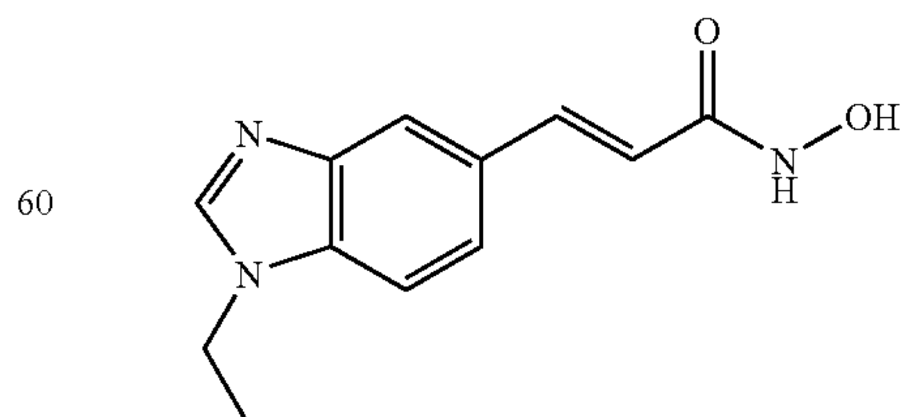
N-Hydroxy-3-(1-Ethyl-1H-benzimidazol-5-yl)-acrylamide
