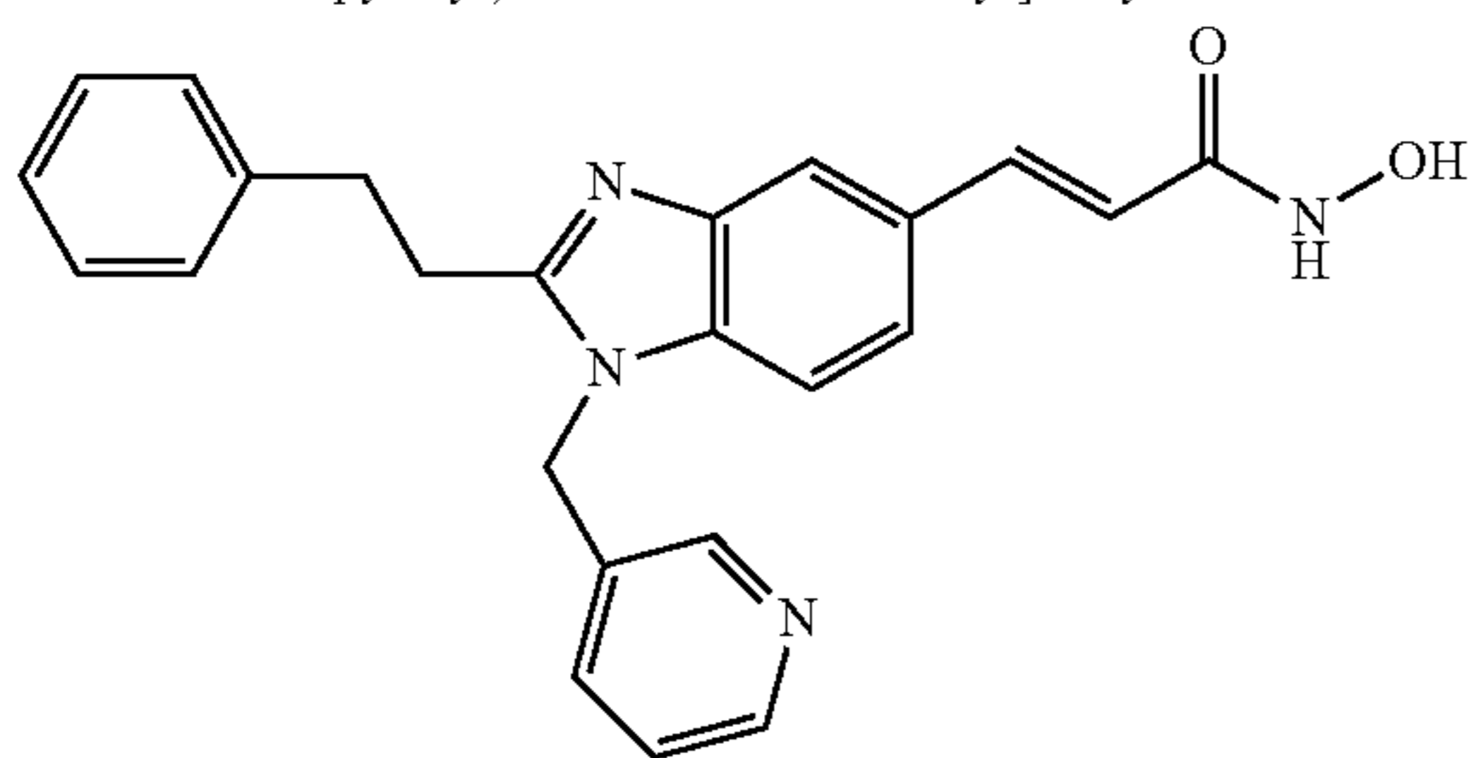
N-Hydroxy-3-[1-(3-pyridylmethyl)-2-(2-phenylethyl)-1H-benzimidazol-5-yl]-acrylamide
