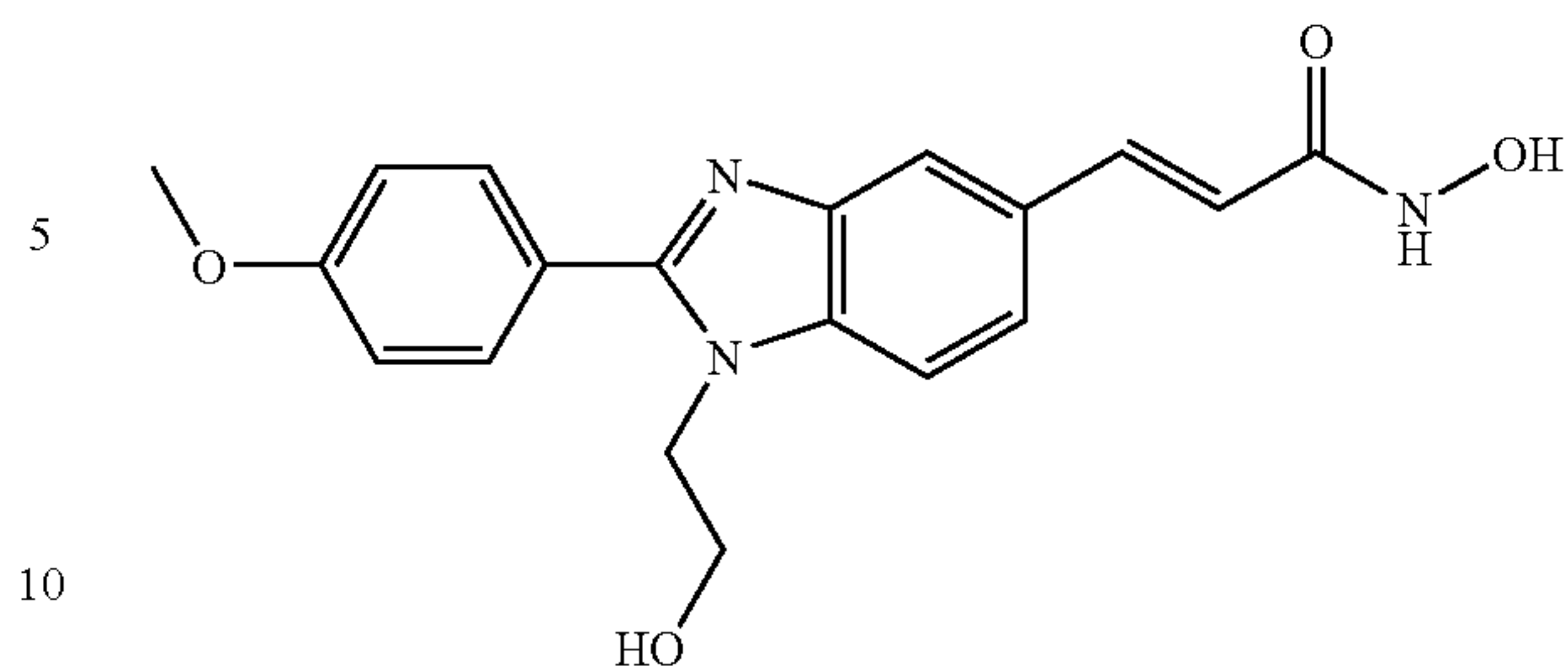
N-Hydroxy-3-[1-(2-hydroxy-ethyl)-2-(4-methoxy-phenyl)-1H-benzimidazole-5-yl]-acrylamide
