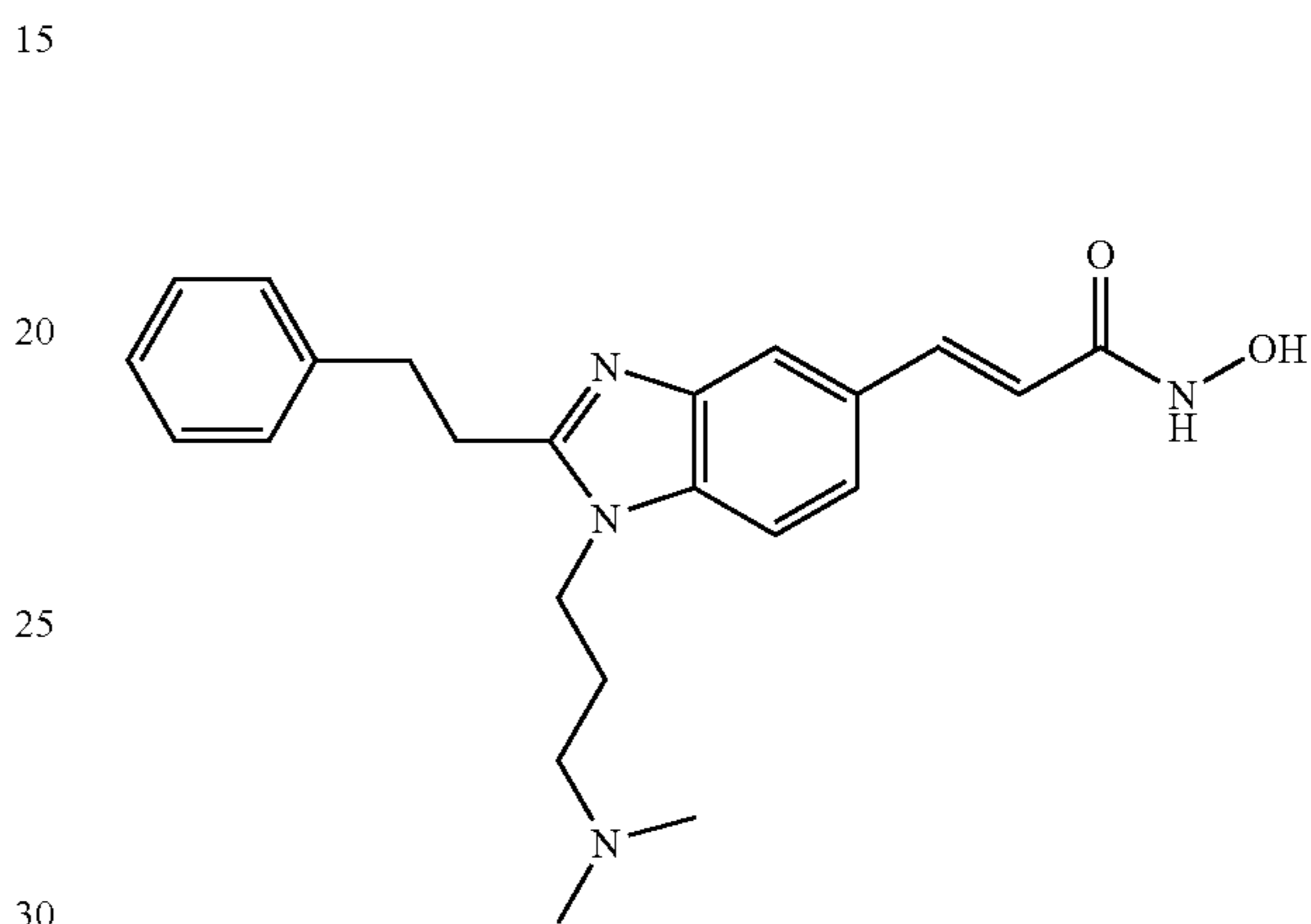
N-Hydroxy-3-[1-(3-dimethylamino-propyl)-2-phenethyl-1H-benzimidazol-5-yl]-acrylamide
