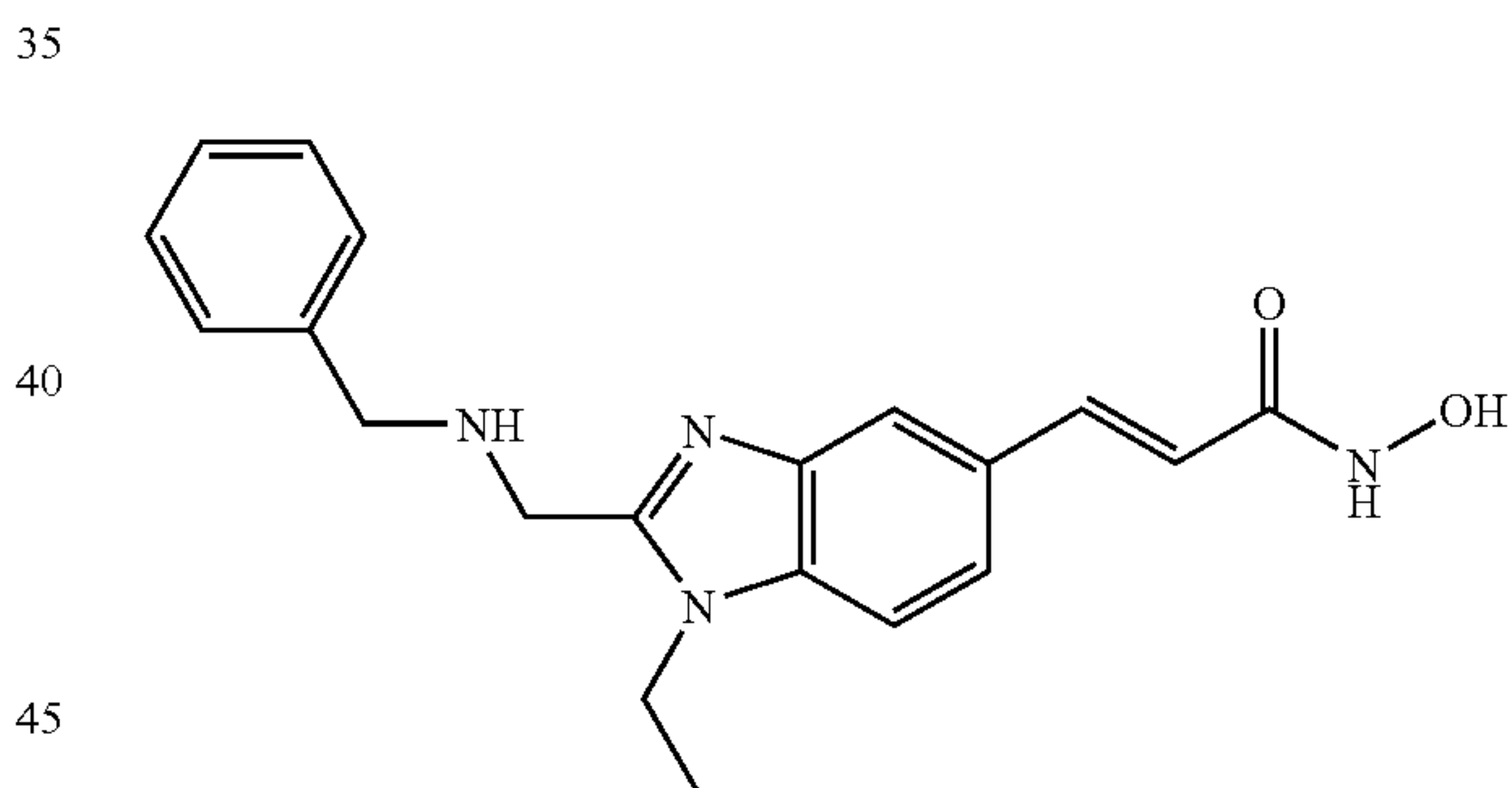
N-Hydroxy-3-[2-(benzylamino-methyl)-ethyl-1H-benzimidazol-5-yl]-acrylamide
