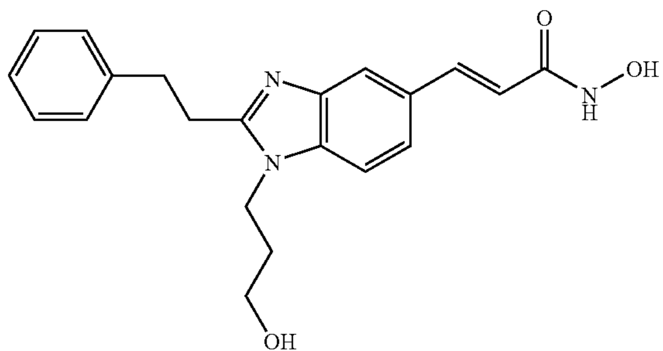
N-Hydroxy-3-[1-(3-hydroxy-propyl)-2-phenethyl-1H-benzimidazol-5-yl]-acrylamide
