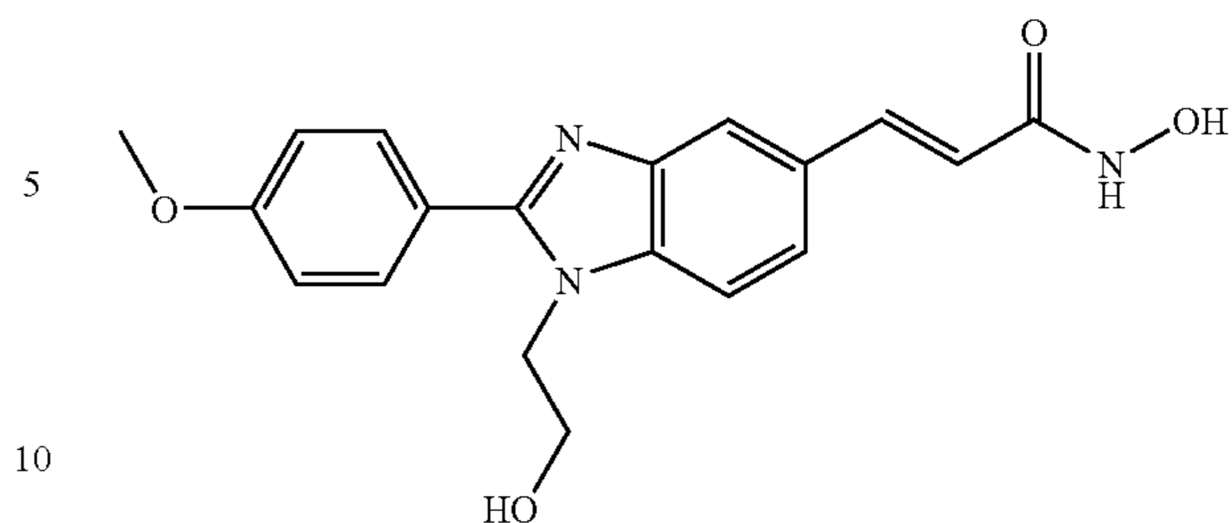
N-Hydroxy-3-[1-(2-hydroxy-ethyl)-2-(4-methoxy-phenyl)-1H-benzimidazole-5-yl]-acrylamide
