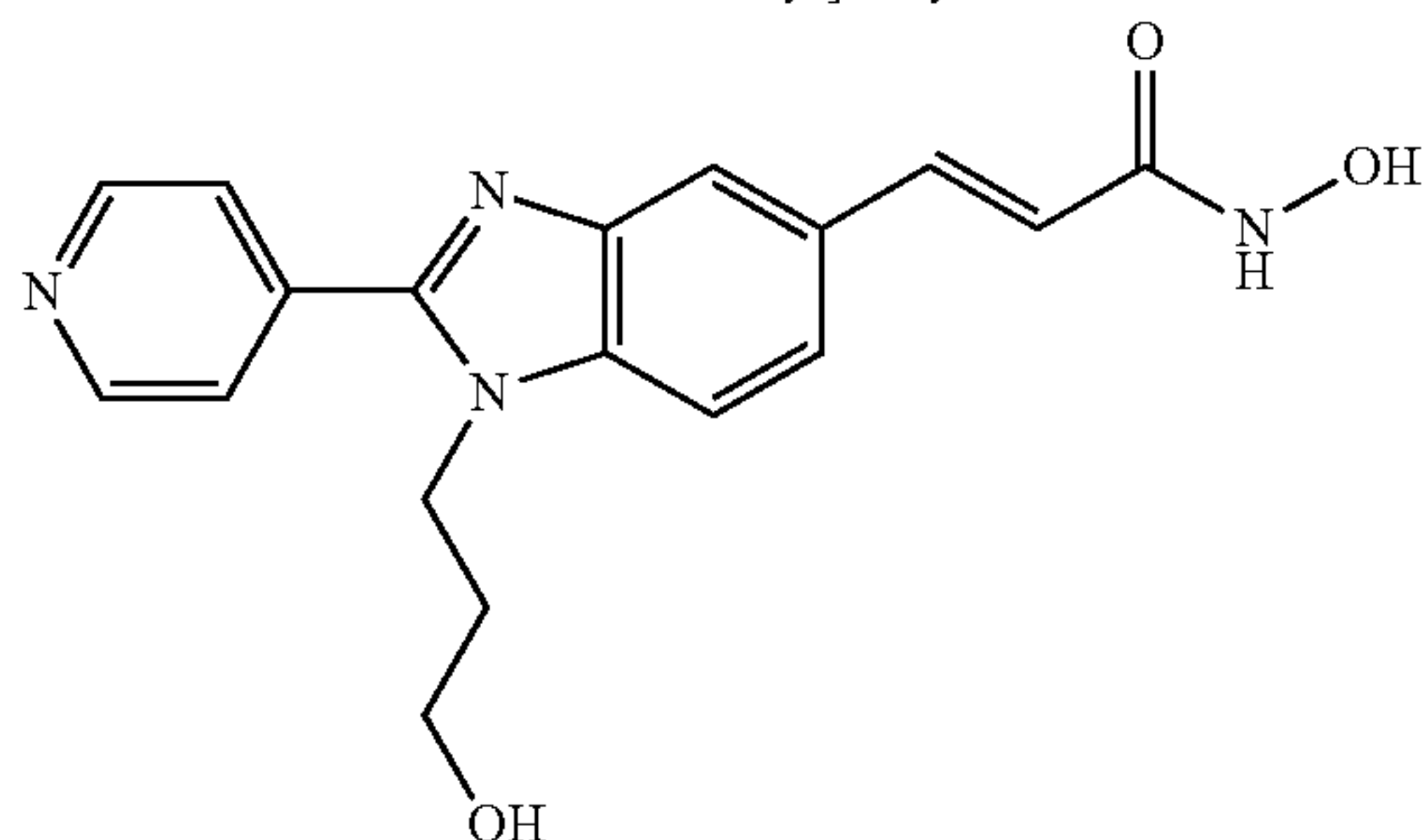
N-Hydroxy-3-[1-(3-hydroxy-propyl)-2-(4-pyridyl)-1H-benzimidazol-5-yl]-acrylamide
