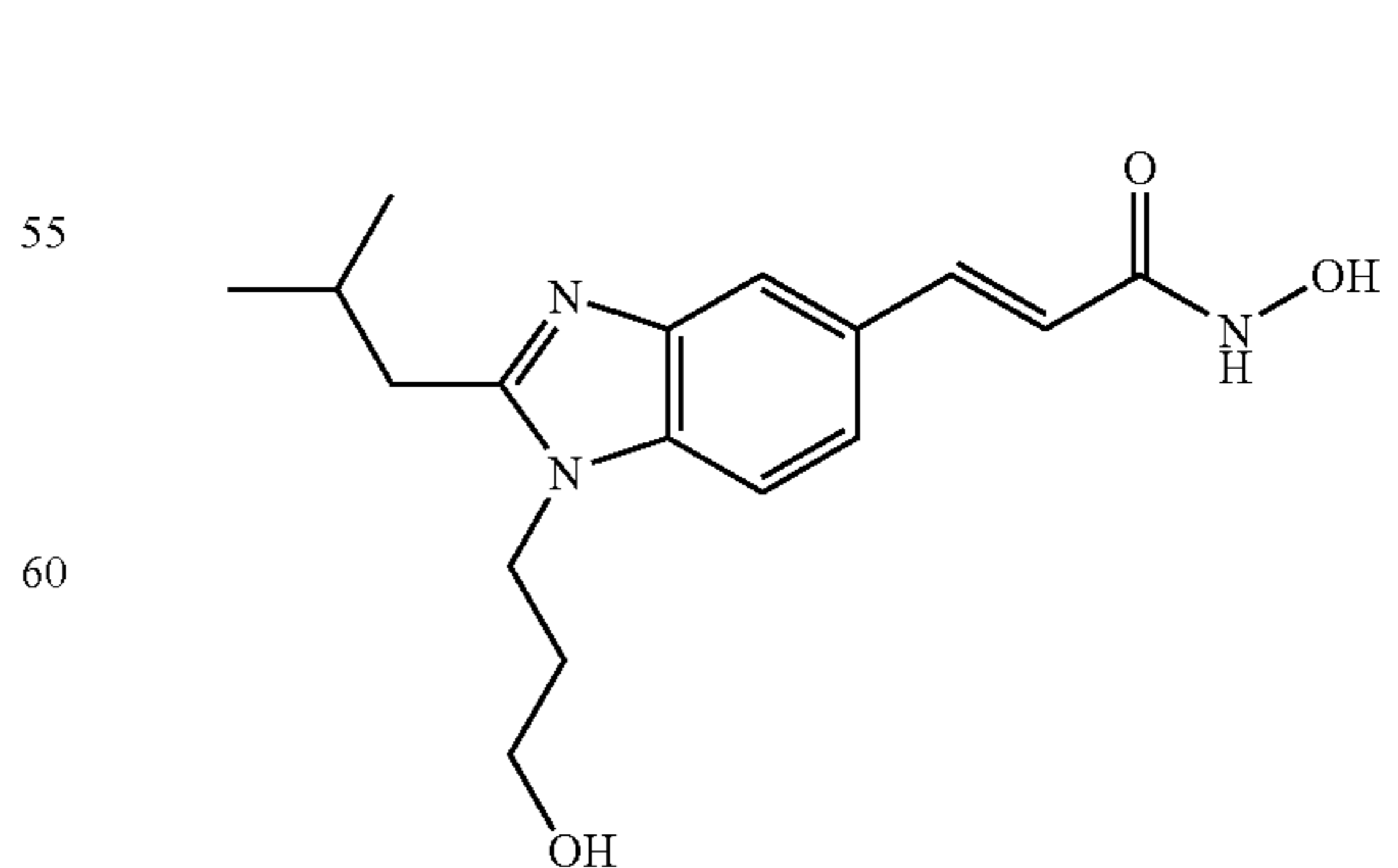
N-Hydroxy-3-[1-(3-hydroxy-propyl)-2-isobutyl-1H-benzimidazol-5-yl]-acrylamide
