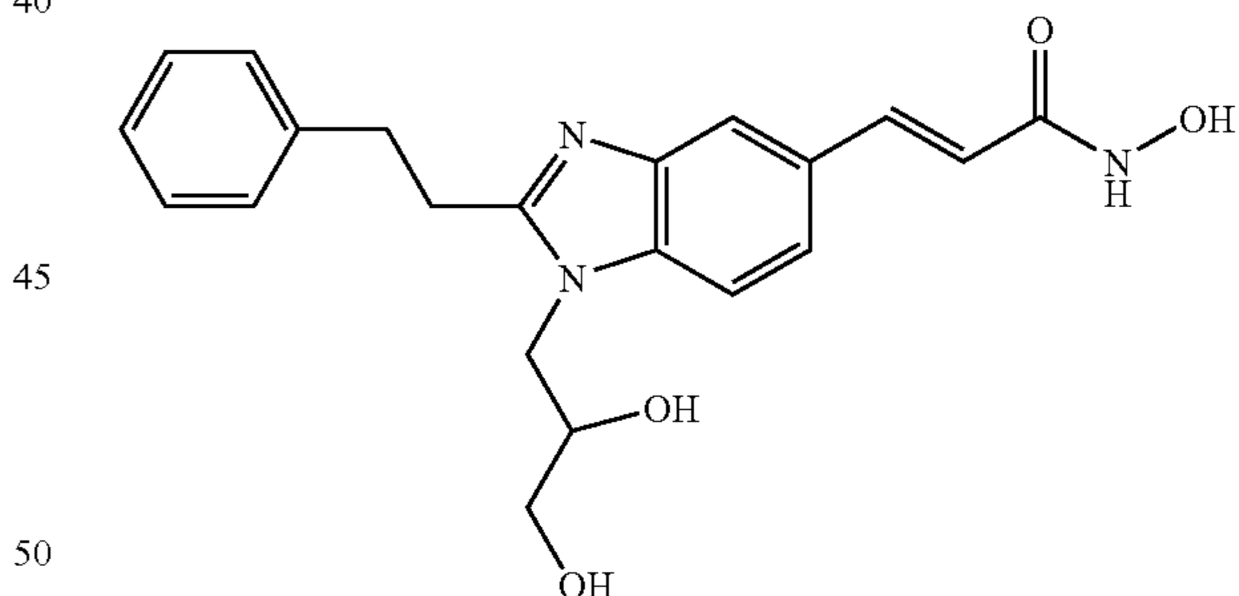
N-Hydroxy-3-[1-(2,3-hydroxy-propyl)-2-(2-phenyl-ethyl)-1H-benzimidazol-5-yl]-acrylamide
