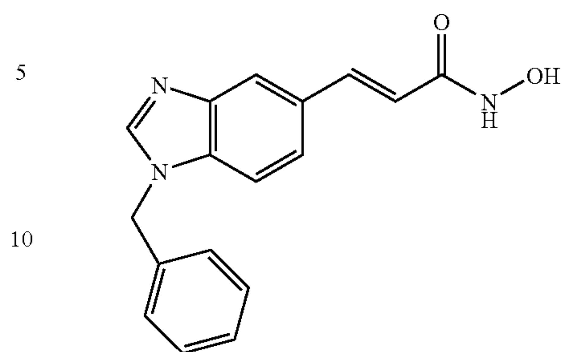
N-Hydroxy-3-(1-benzyl-1H-benzimidazol-5-yl)-acrylamide
