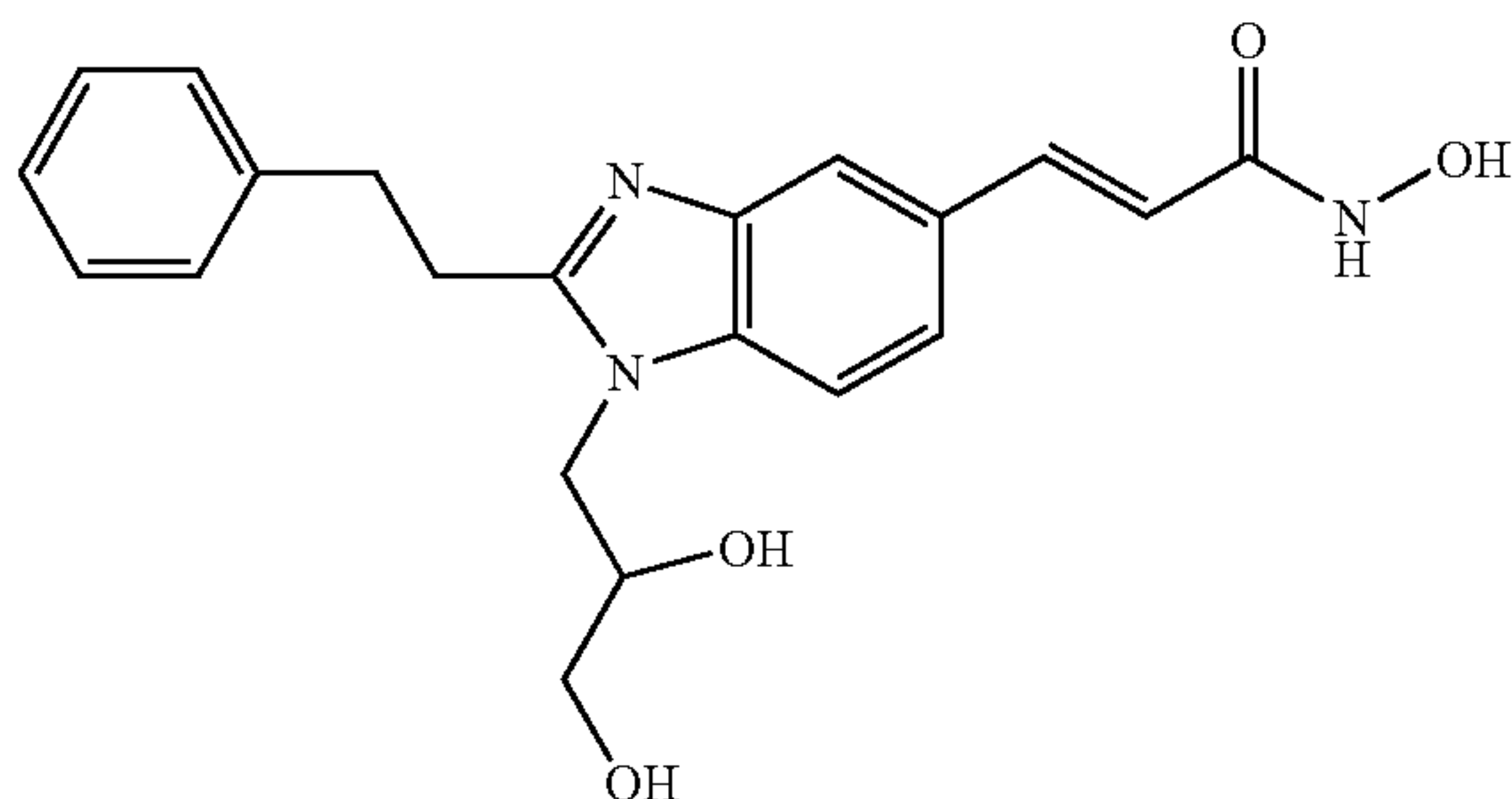
N-Hydroxy-3-[1-(2,3-hydroxy-propyl)-2-(2-phenyl-ethyl)-1H-benzimidazole-5-yl]-acrylamide
