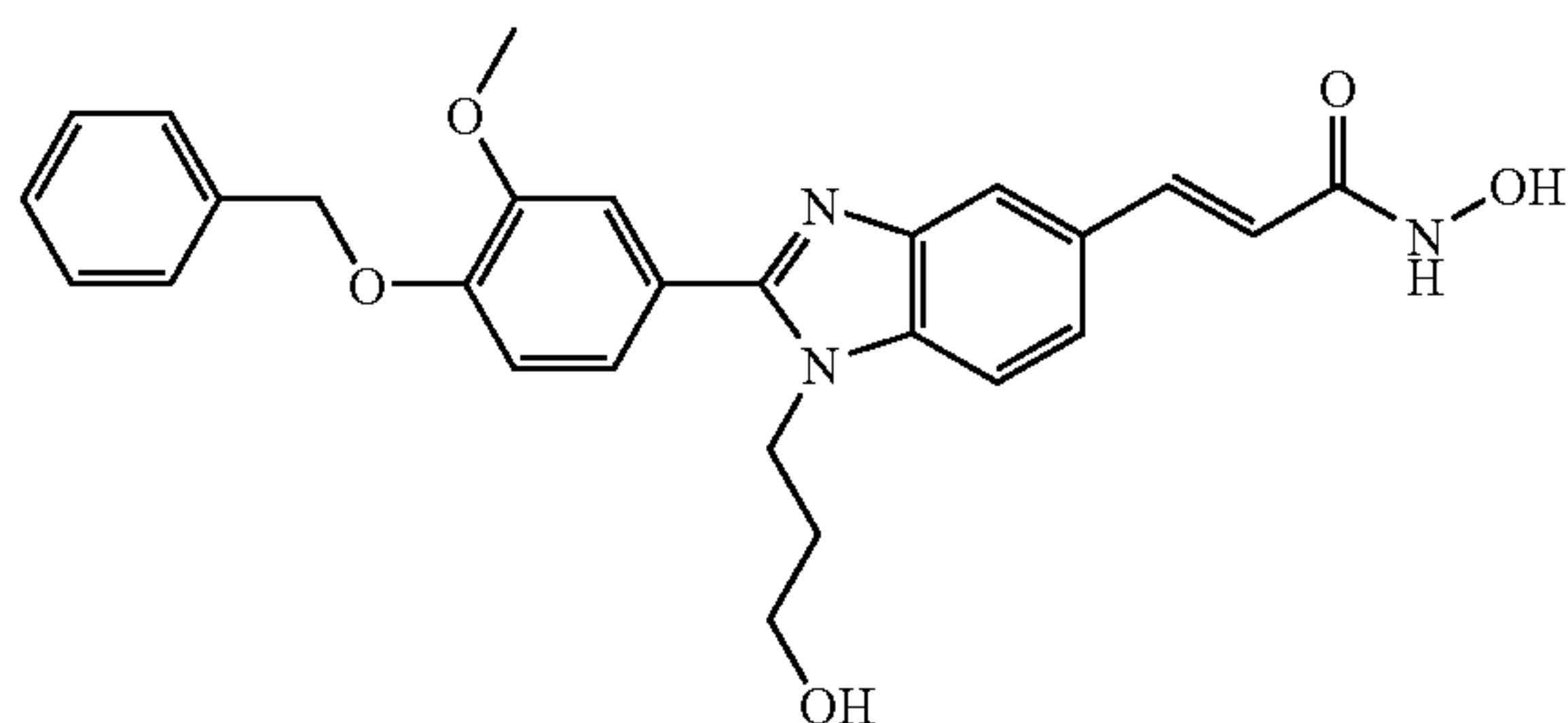
N-Hydroxy-3-[2-(4-benzyloxy-3-methoxy-phenyl)-1-(3-hydroxy-propyl)-1H-benzimidazole-5-yl]-acrylamide
