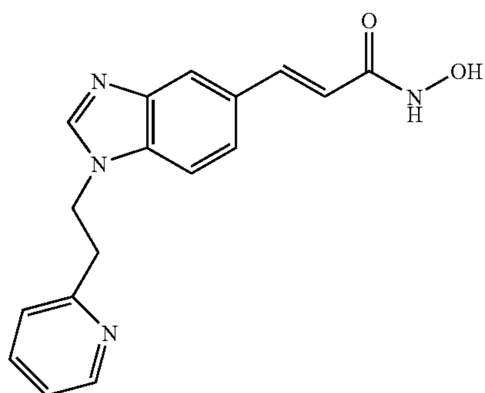
N-Hydroxy-3-[1-(2-pyridin-2-yl-ethyl)-1H-benzimidazol-5-yl]-acrylamide
