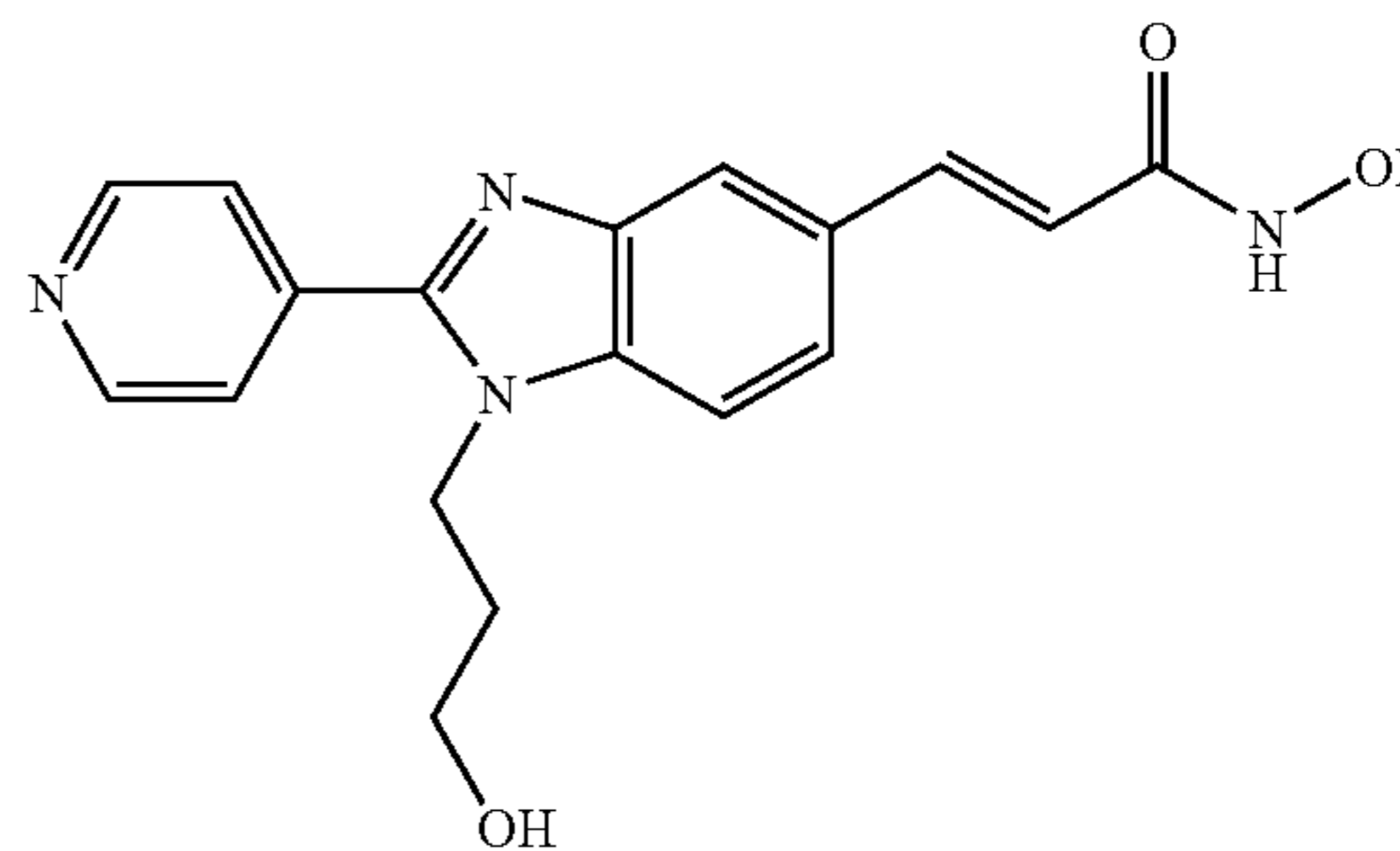
N-Hydroxy-3-[1-(3-hydroxy-propyl)-2-(4-pyridyl)-1H-benzimidazole-5-yl]-acrylamide
