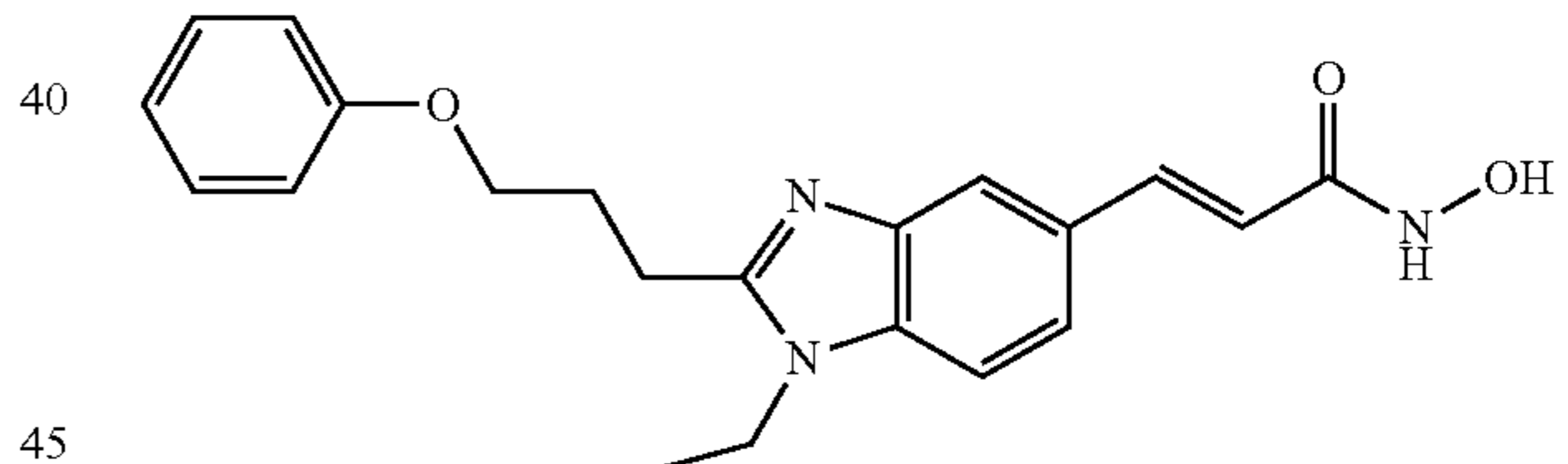
N-Hydroxy-3-[1-ethyl-2-(3-phenoxy-propyl)-1H-benzimidazol-5-yl]-acrylamide
