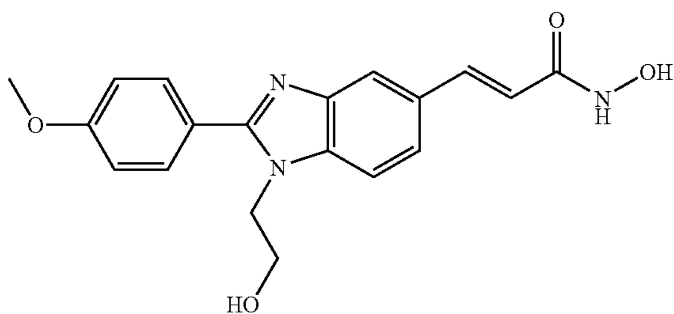
N-Hydroxy-3-[1-(2-hydroxy-ethyl)-2-(4-methoxy-phenyl)-1H-benzimidazole-5-yl]-acrylamide
