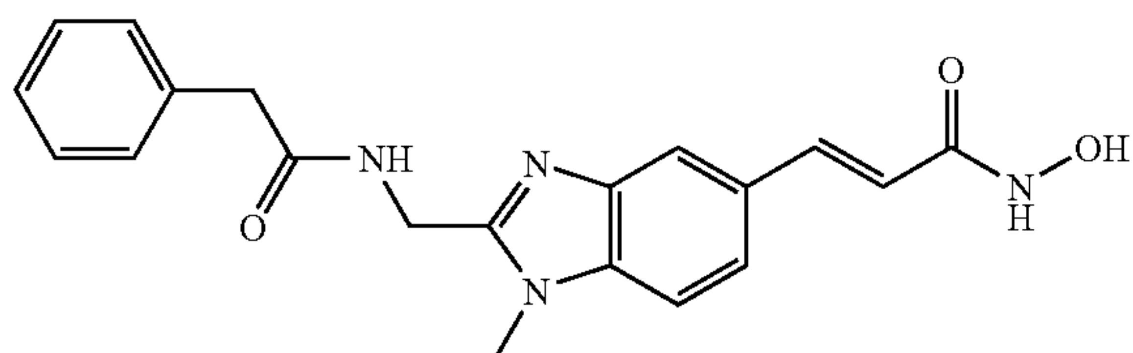
N-Hydroxy-3-[1-methyl-2-(phenylacetyl-amino-methyl)-1H-benzimidazol-5-yl]-acrylamide
