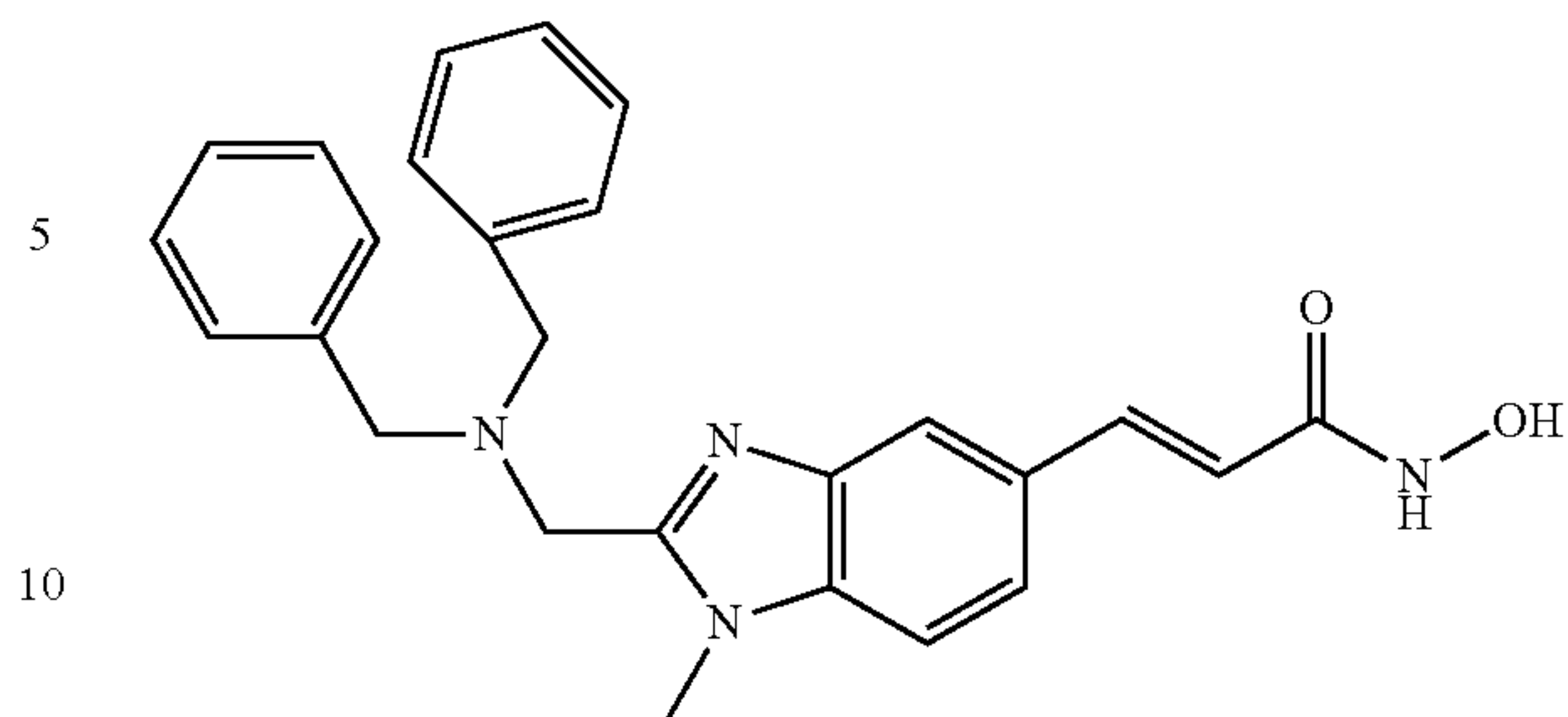
N-Hydroxy-3-{2-[dibenzylamino)-methyl]-1-methyl-1H-benzimidazol-5-yl}-acrylamide
