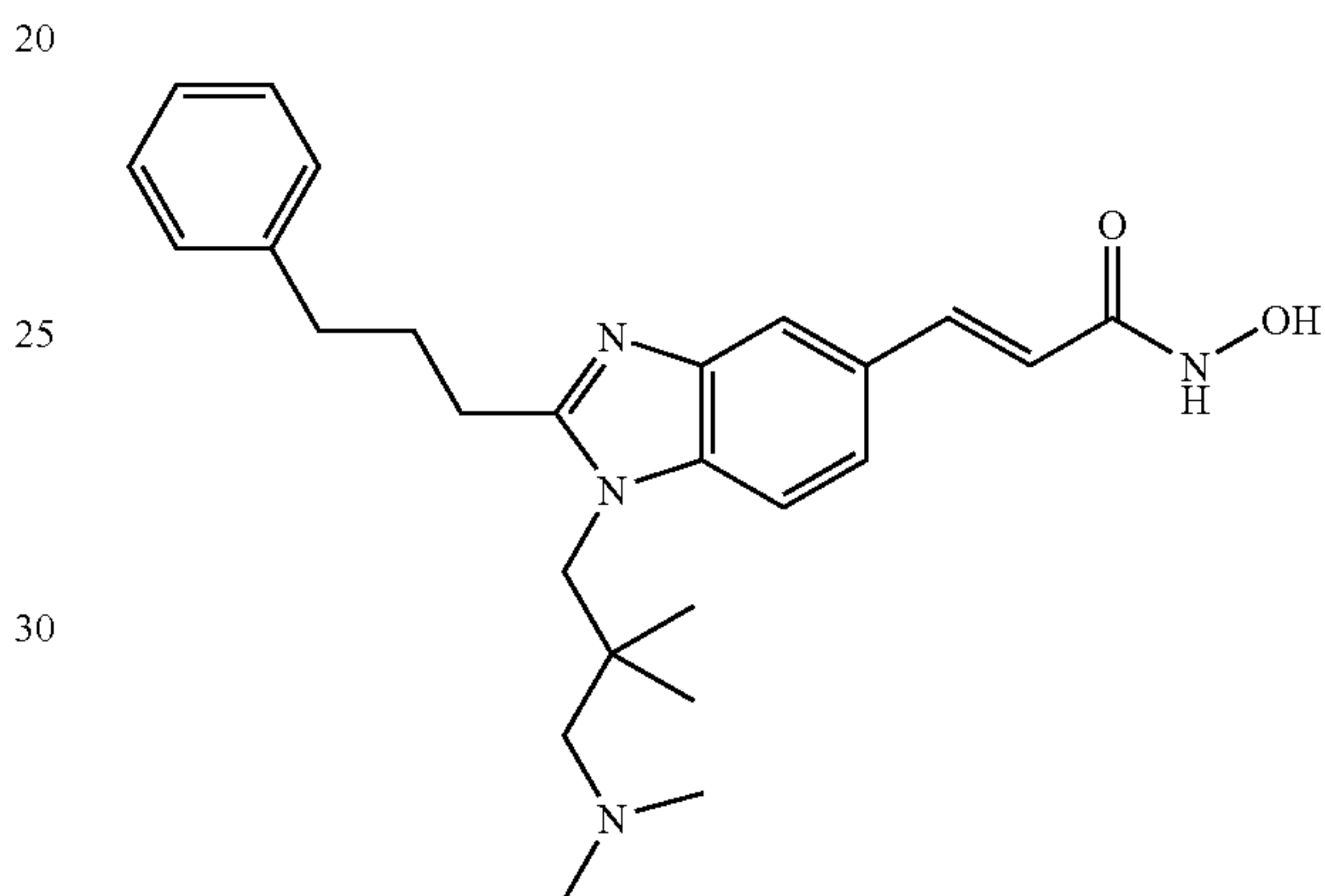
N-Hydroxy-3-[1-(3-Dimethylamino-2,2-dimethyl-propyl)-2-(3-phenyl-propyl)-1H-benzimidazol-5-yl]-acrylamide
