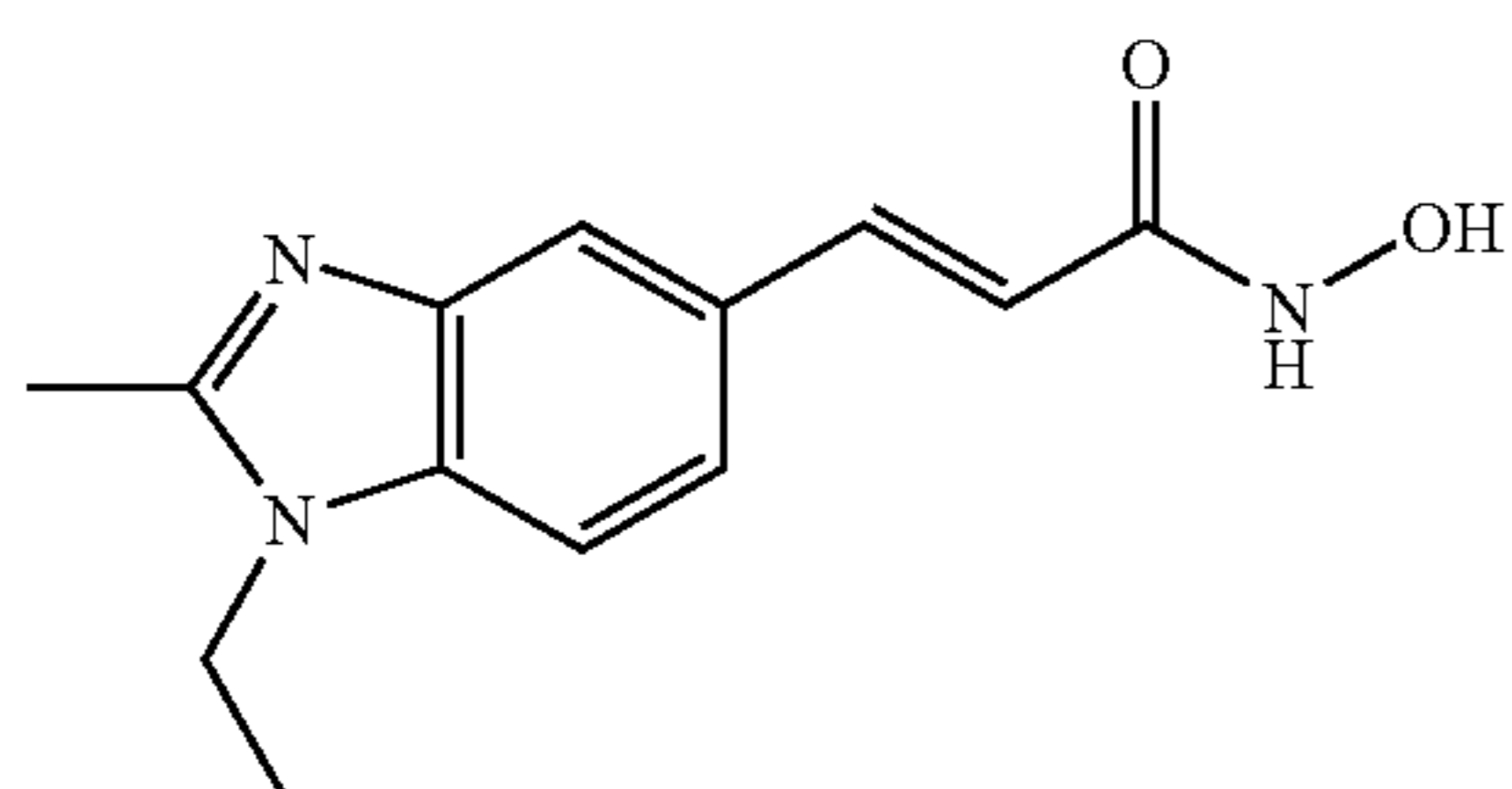
N-Hydroxy-3-(1-Ethyl-2-methyl-1H-benzimidazol-5-yl)-acrylamide
