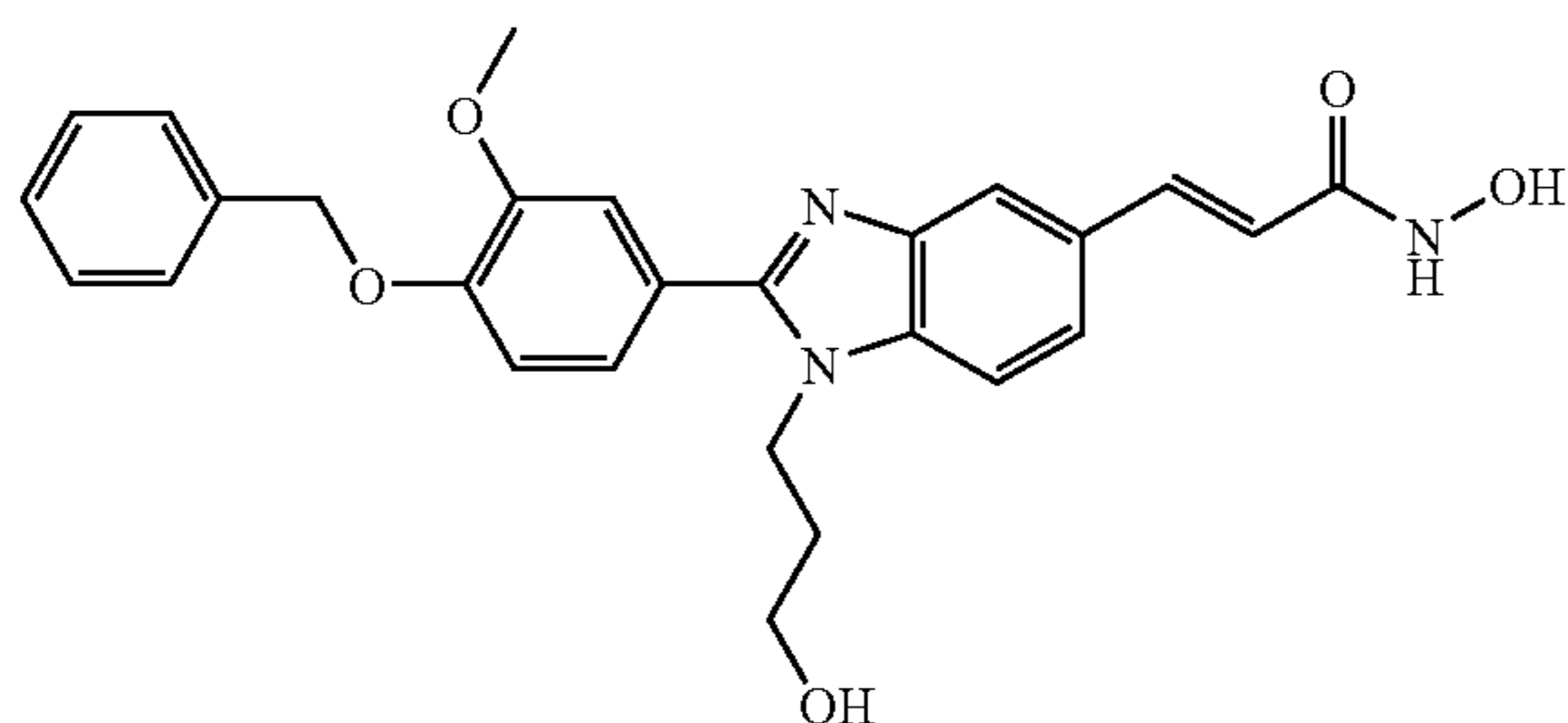
N-Hydroxy-3-[2-(4-benzyloxy-3-methoxy-phenyl)-1-(3-hydroxy-propyl)-1H-benzimidazole-5-yl]-acrylamide
