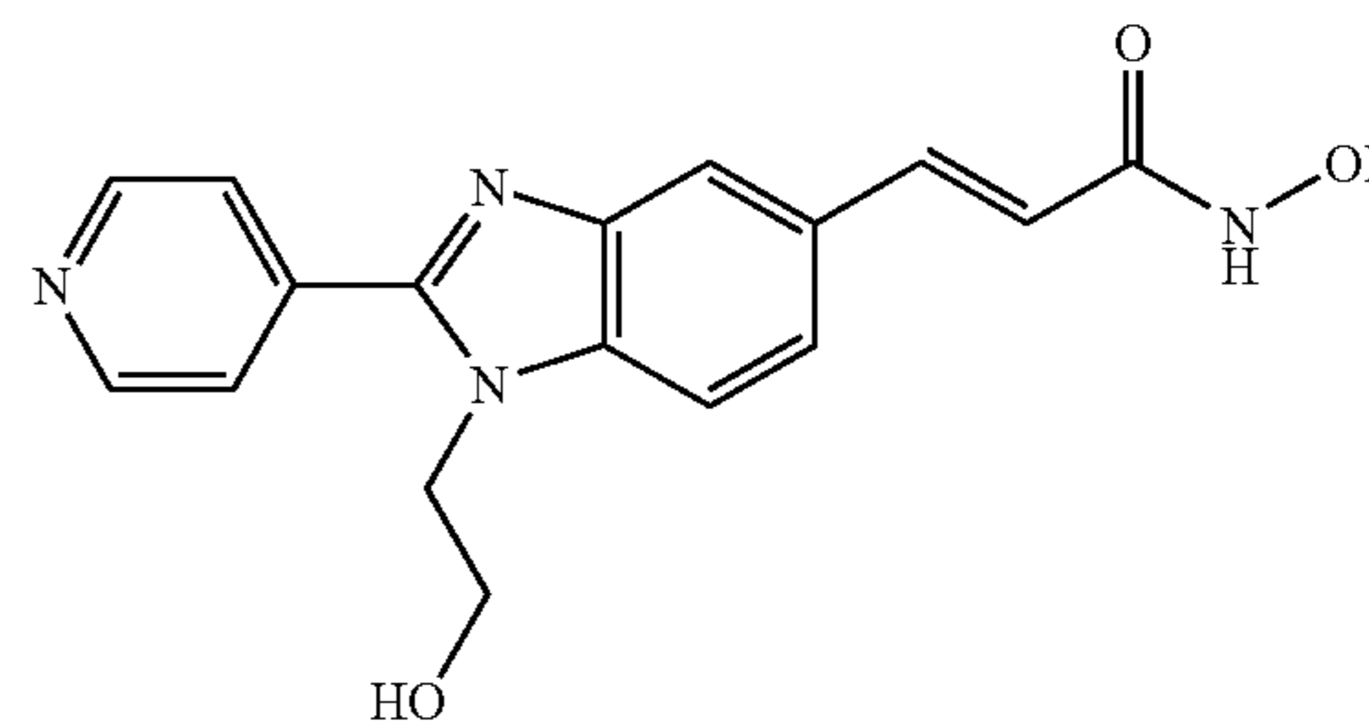
N-Hydroxy-3-[1-(2-hydroxy-ethyl)-2-(4-pyridyl)-1H-benzimidazole-5-yl]-acrylamide
