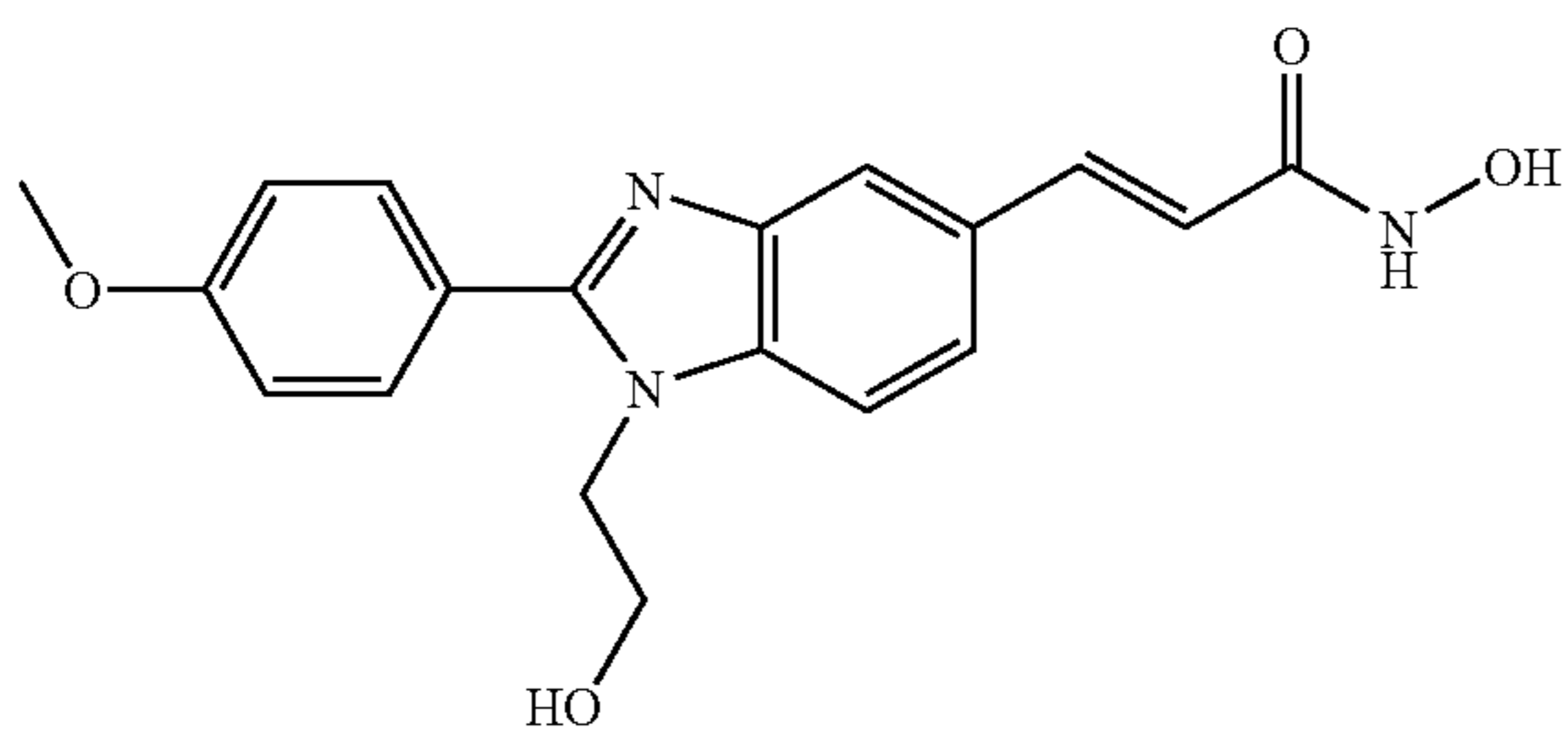
N-Hydroxy-3-[1-(2-hydroxy-ethyl)-2-(4-methoxy-phenyl)-1H-benzimidazole-5-yl]-acrylamide
