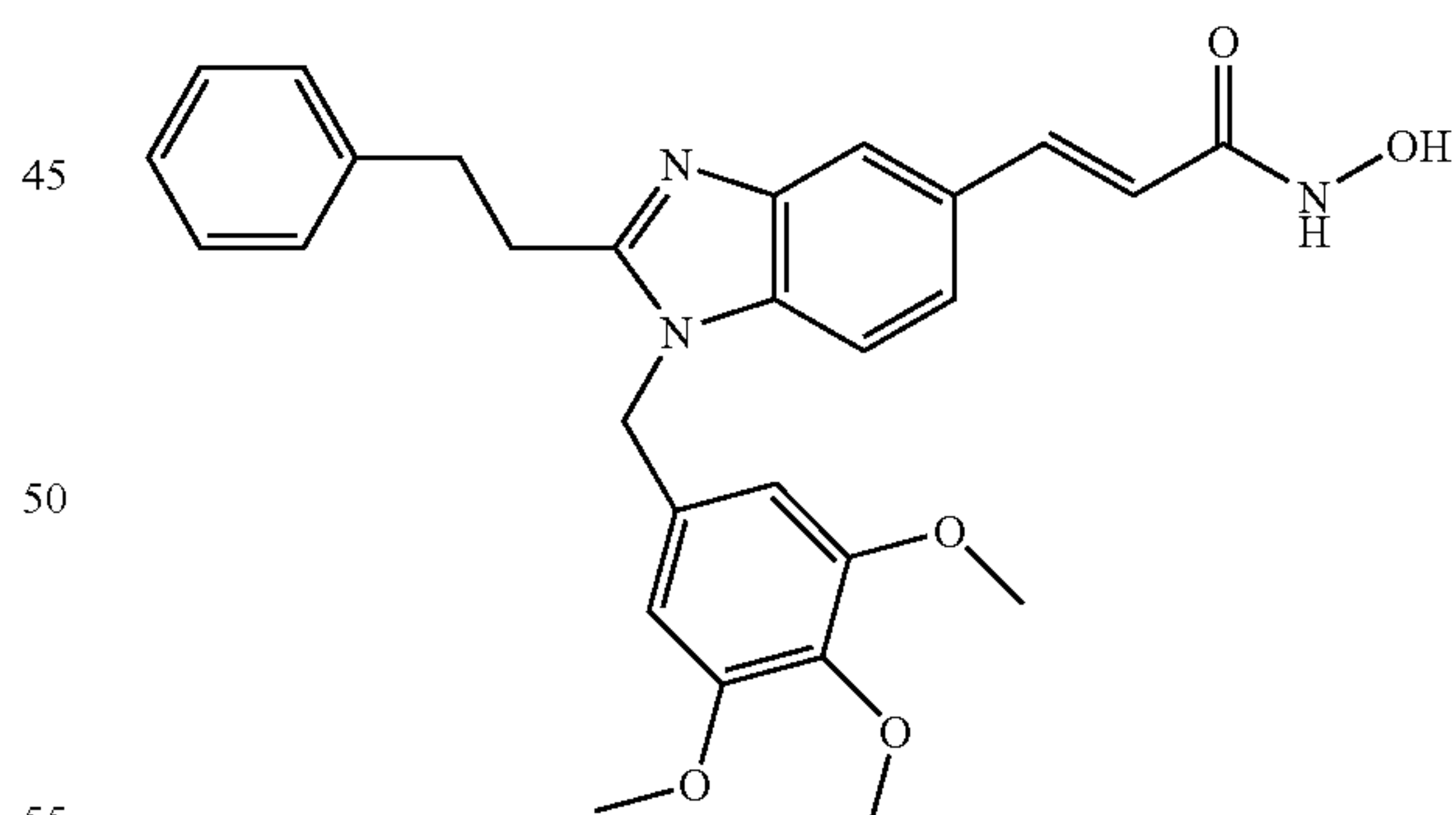
N-Hydroxy-3-[1-(3,4,5-trimethoxybenzyl)-2-(2-phenyl-ethyl)-1H-benzimidazol-5-yl]-acrylamide
