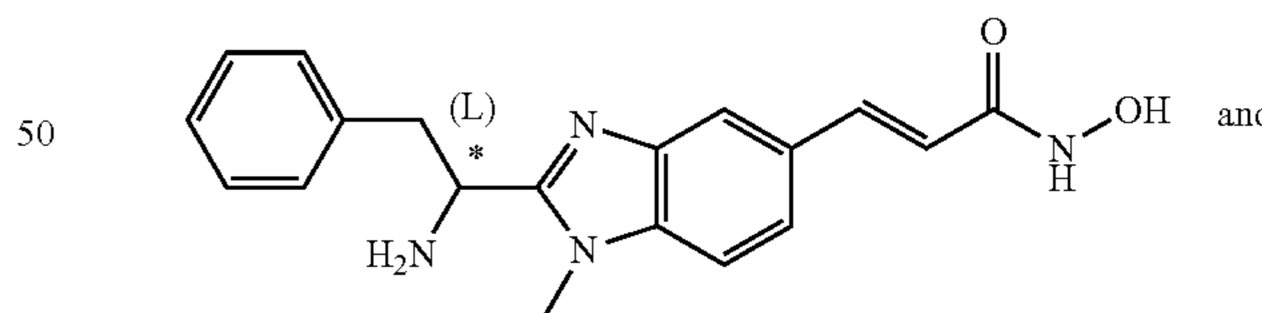
(L)-N-Hydroxy-3-[2-(1-amino-2-phenyl-ethyl)-1-methyl-1H-benzimidazol-5-yl]-acrylamide
