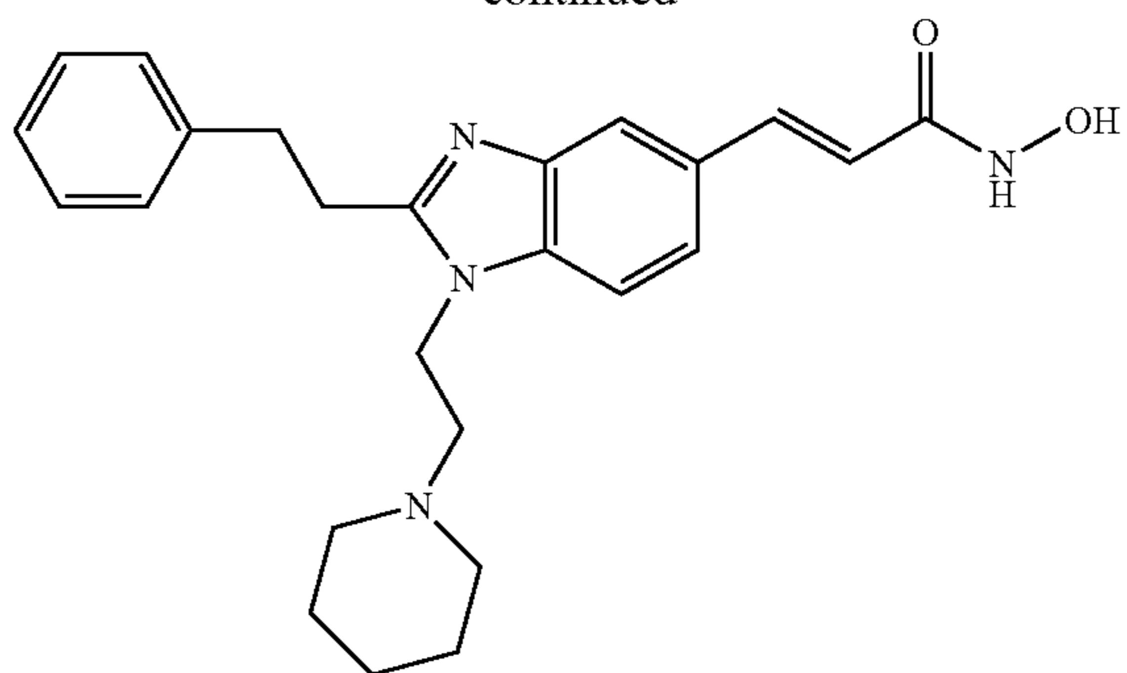
N-Hydroxy-3-[2-phenethyl-1-(piperidin-1-yl-ethyl)-1H-benzimidazol-5-yl]-acrylamide
