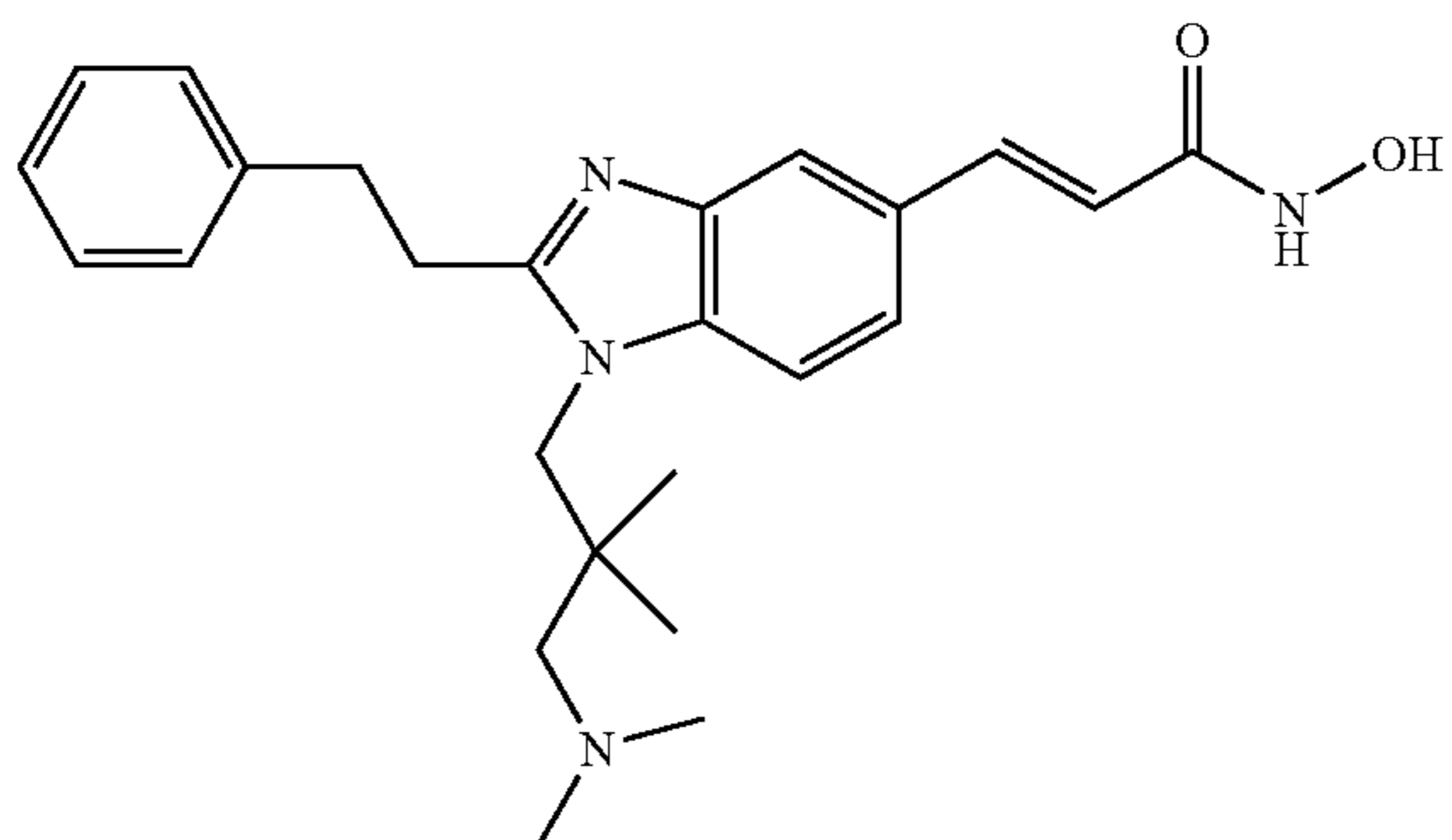
N-Hydroxy-3-[1-(3-Dimethylamino-2,2-dimethyl-propyl)-2-phenethyl-1H-benzimidazol-5-yl]-acrylamide
