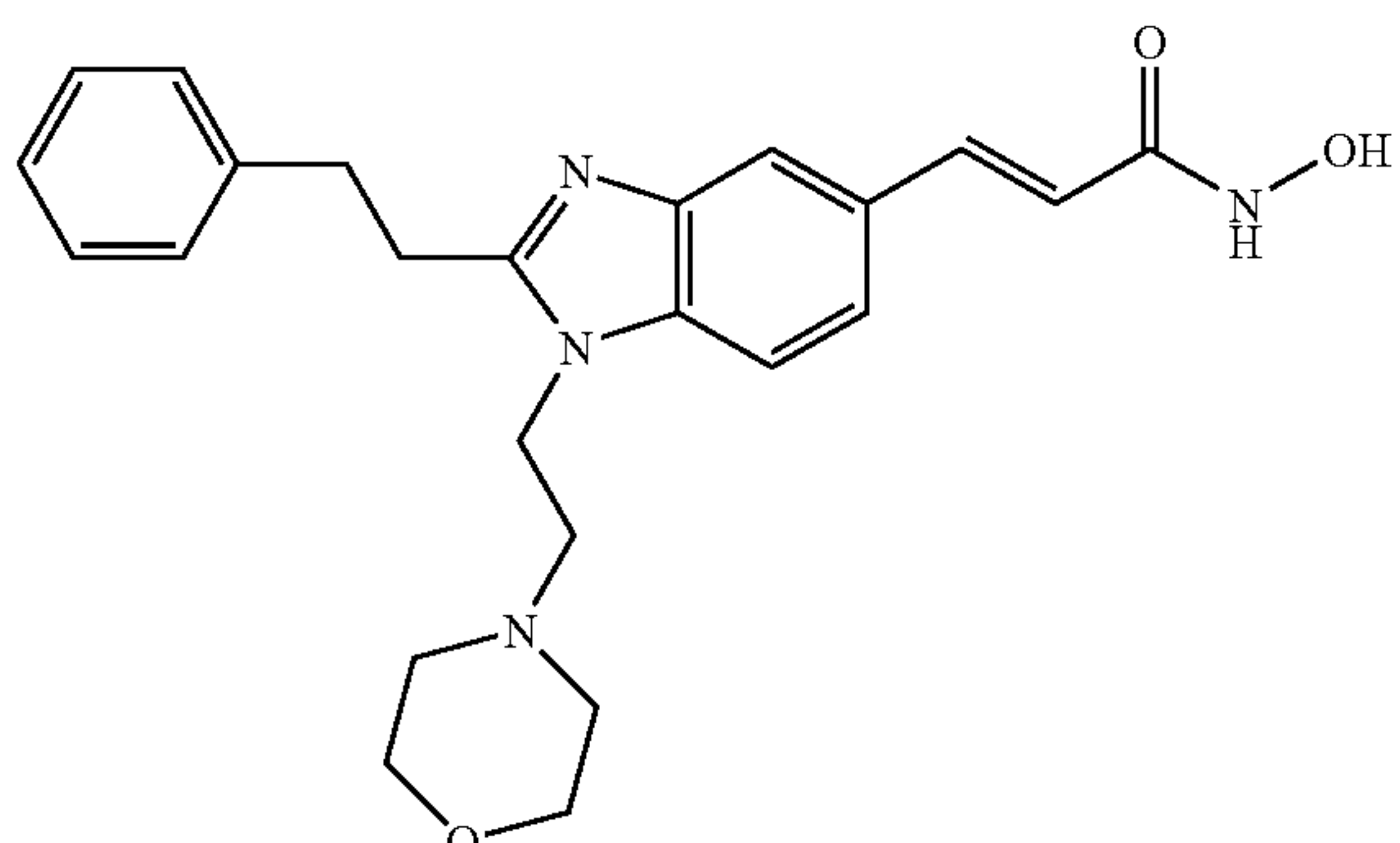
N-Hydroxy-3-[1-(2-morpholin-4-yl-ethyl)-2-phenethyl-1H-benzimidazol-5-yl]-acrylamide
