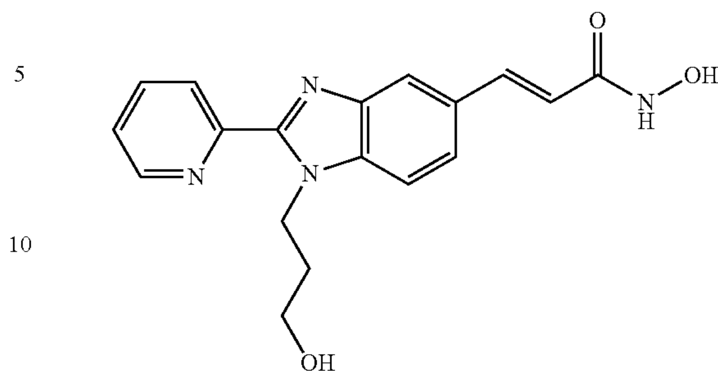
N-Hydroxy-3-[1-(3-hydroxy-propyl)-2-(2-pyridyl)-1H-benzimidazol-5-yl]-acrylamide;
