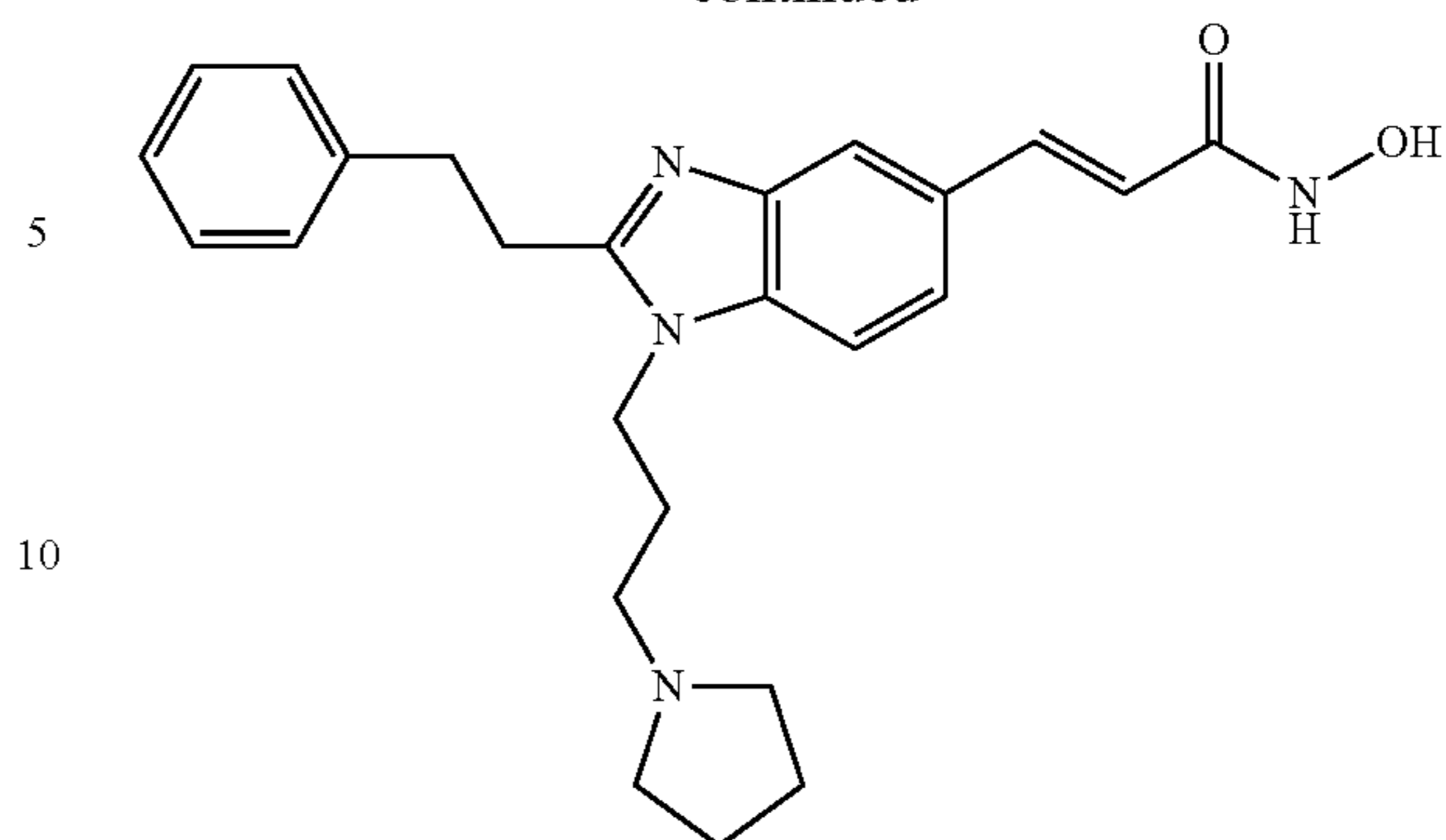
N-Hydroxy-3-[2-phenethyl-1-(3-pyrrolidin-1-yl-propyl)-1H-benzimidazol-5-yl]-acrylamide
