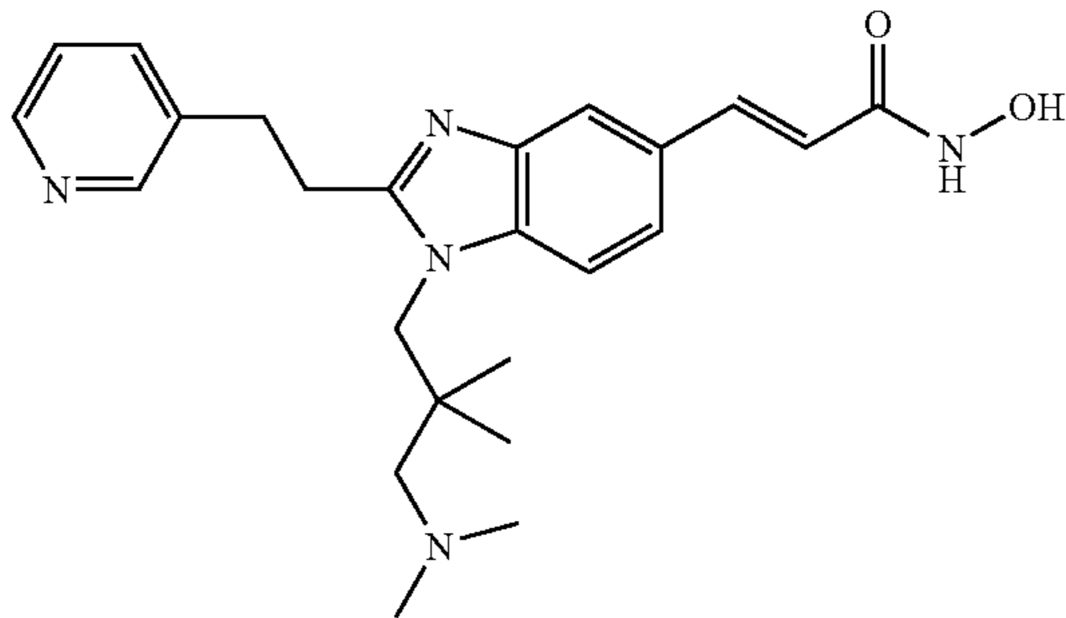
N-Hydroxy-3-[1-(3-Dimethylamino-2,2-dimethyl-propyl)-2-(2-pyridin-3-yl-ethyl)-1H-benzimidazol-5-yl]-acrylamide
