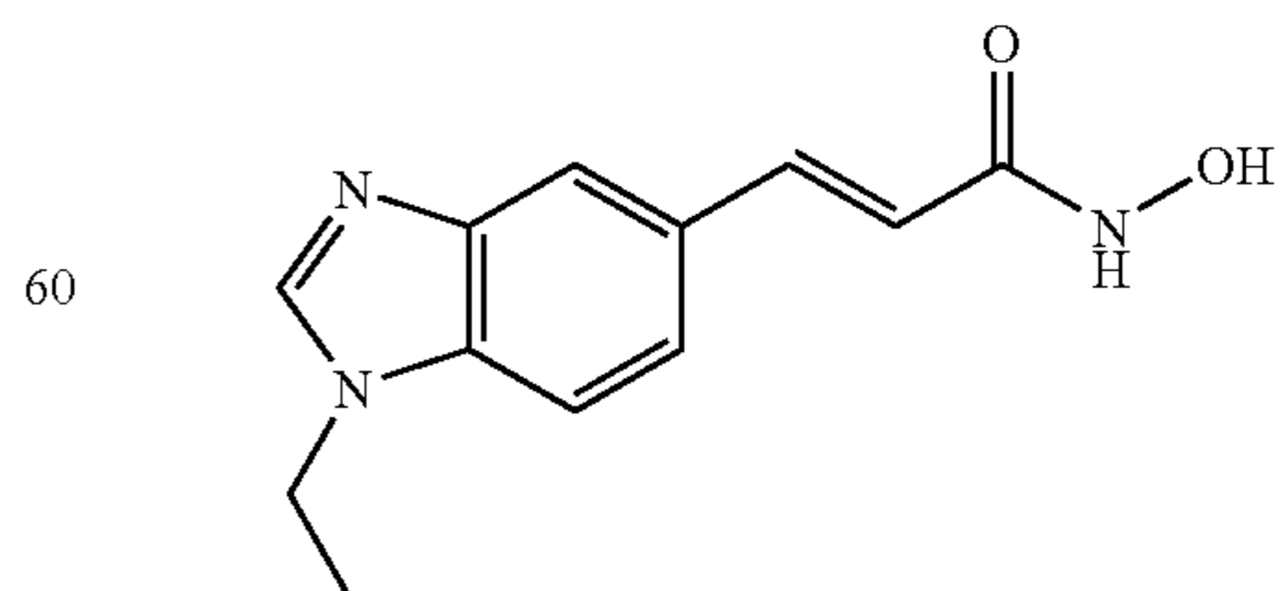
N-Hydroxy-3-(1-Ethyl-1H-benzimidazol-5-yl)-acrylamide
