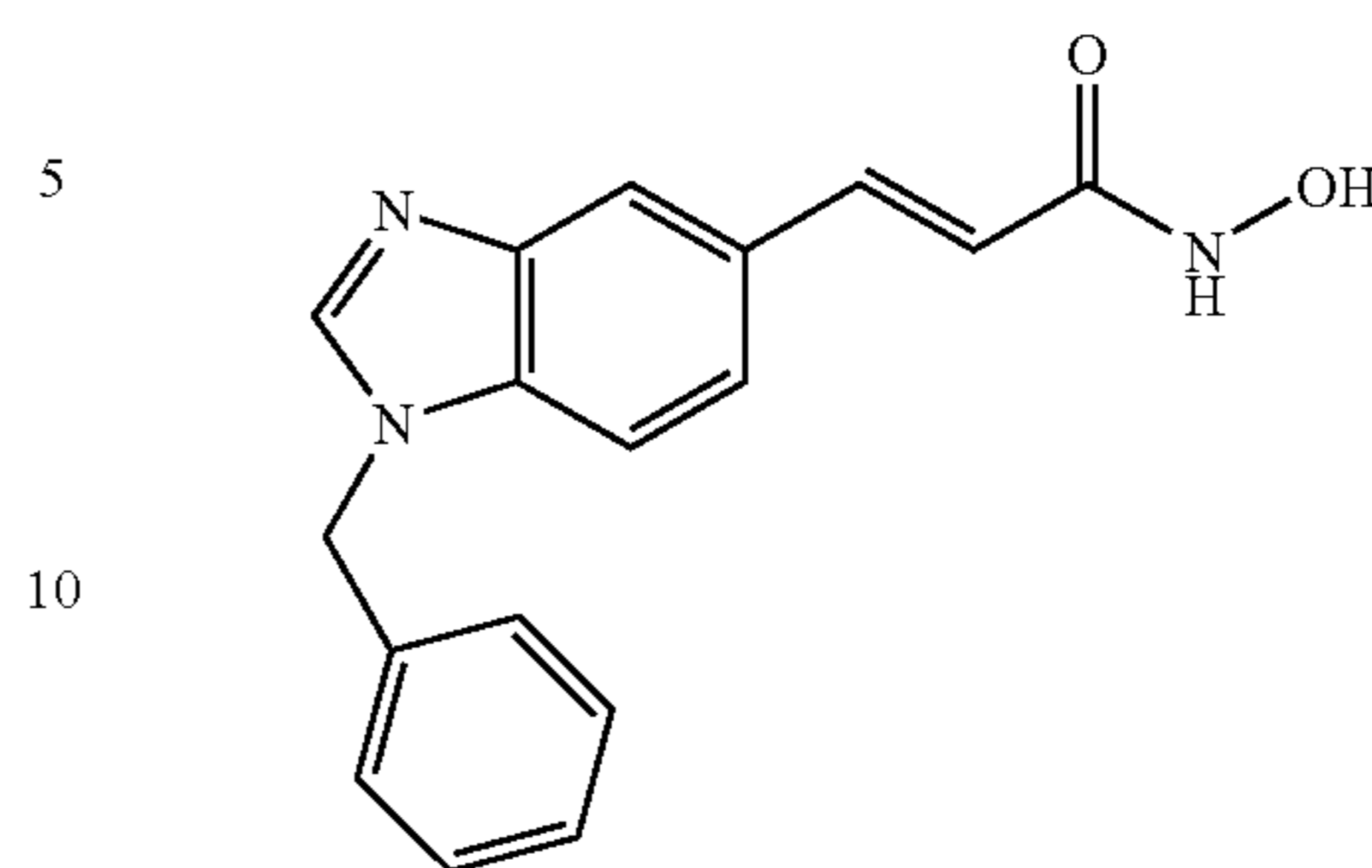
N-Hydroxy-3-(1-benzyl-1H-benzimidazol-5-yl)-acrylamide
