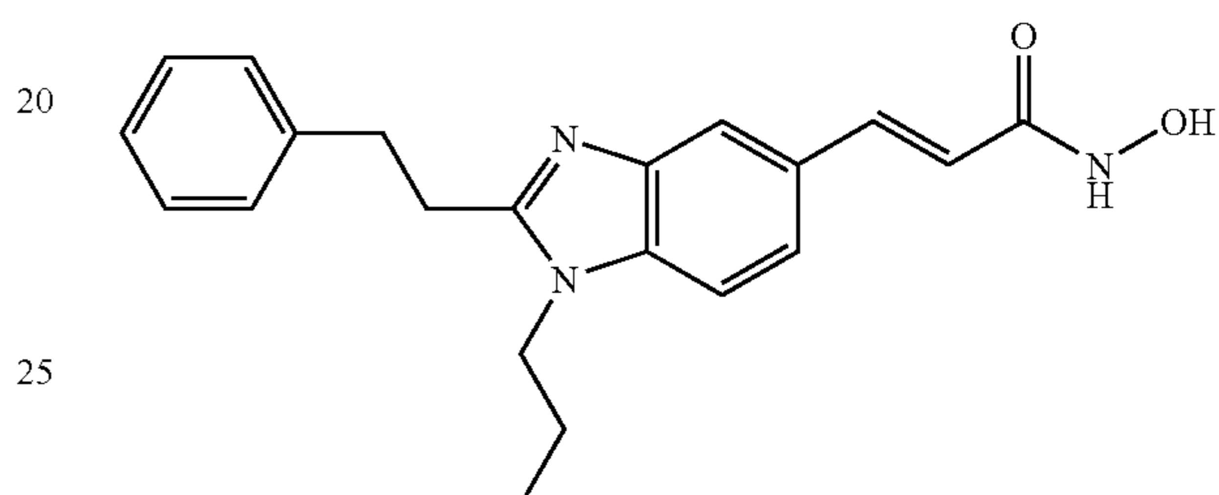
N-Hydroxy-3-(2-phenethyl-1-propyl-1H-benzimidazol-5-yl)-acrylamide
