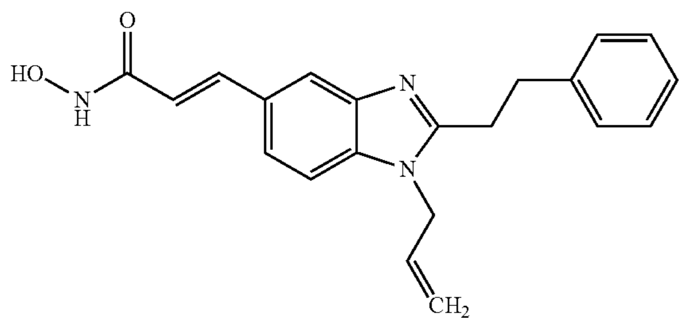
N-Hydroxy-3-(1-allyl-2-phenethyl-1H-benzimidazol-5-yl)-acrylamide
