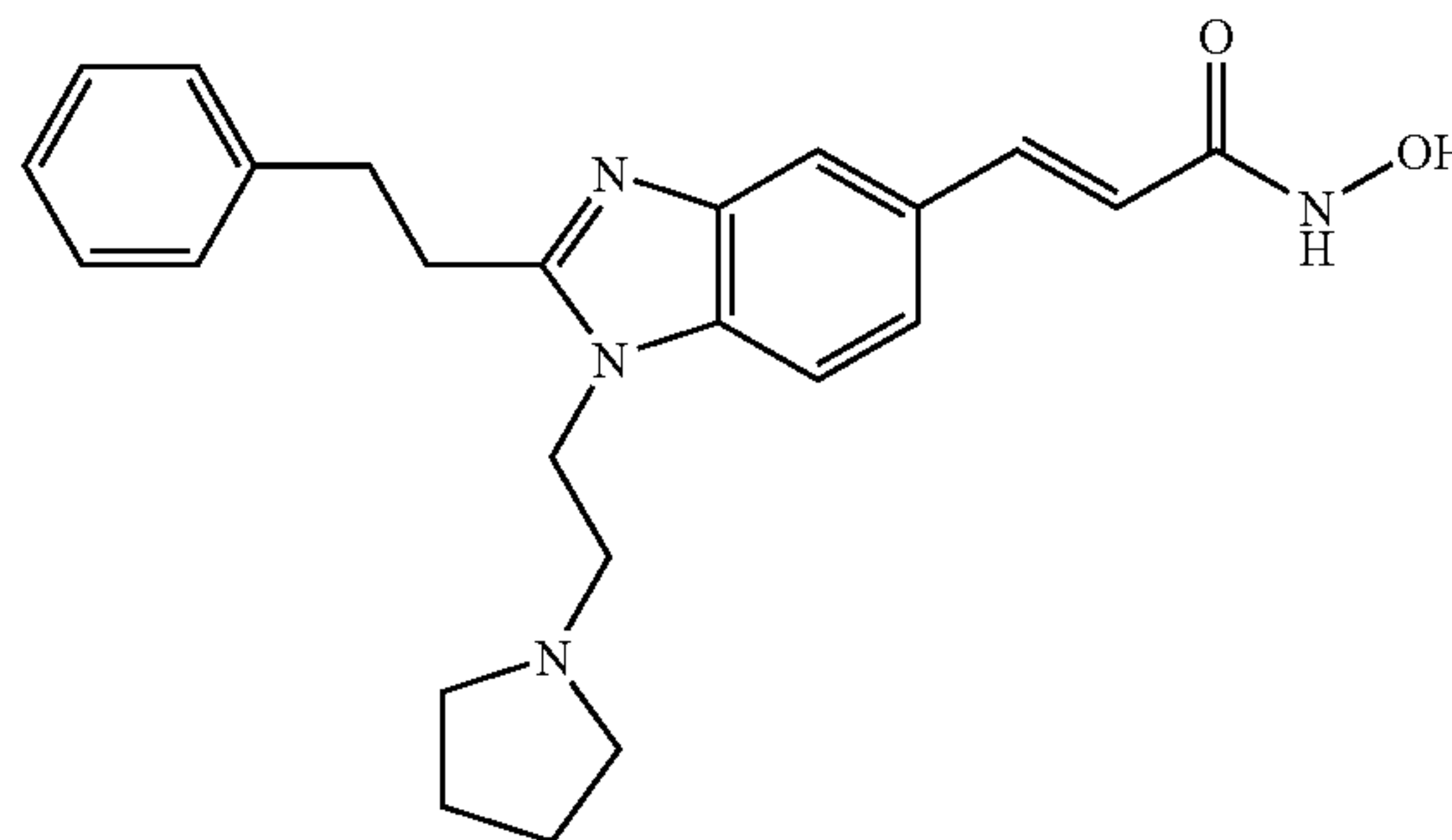
N-Hydroxy-3-[2-phenethyl-1-(2-pyrrolidin-1-yl-ethyl)-1H-benzimidazol-5-yl]-acrylamide
