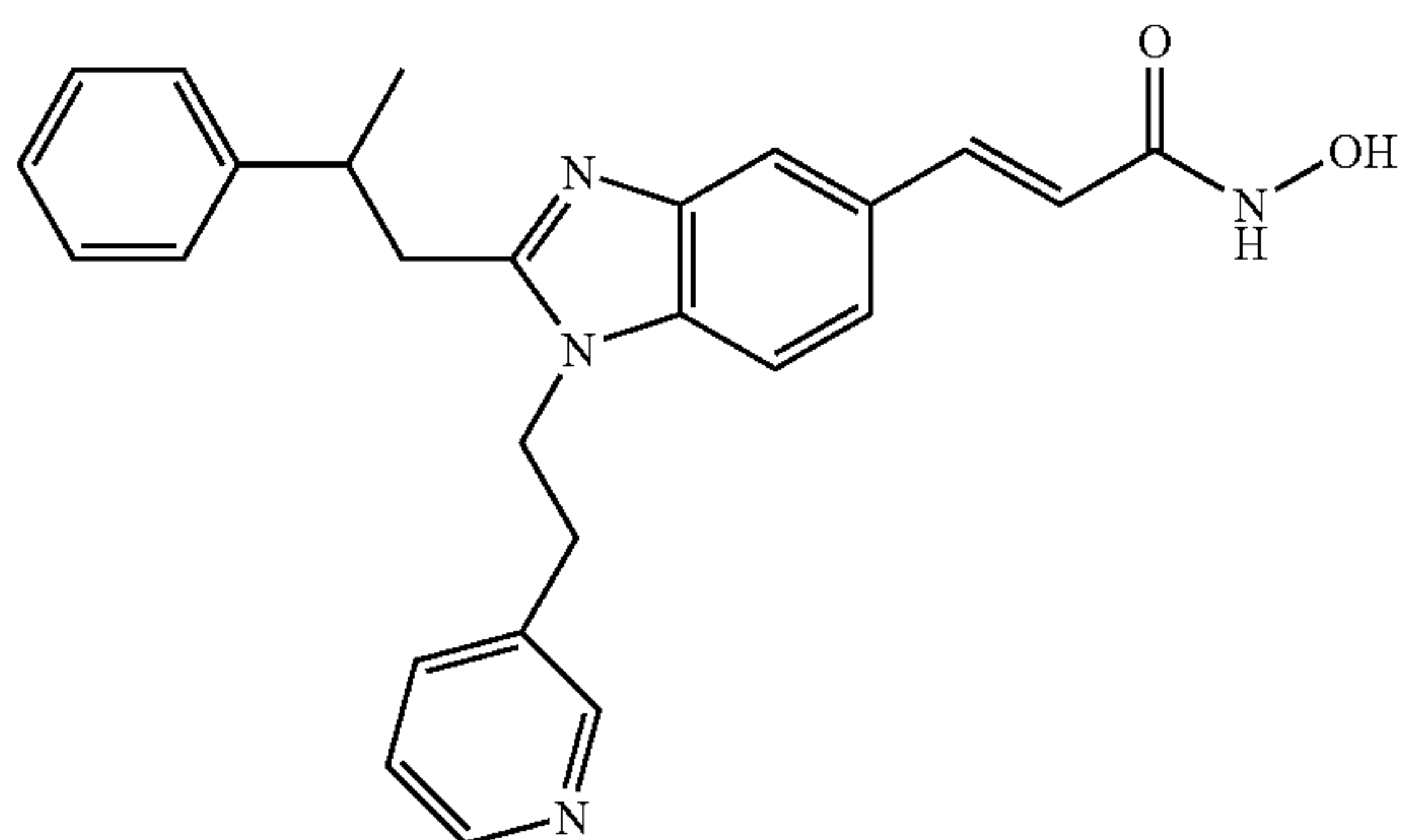
N-Hydroxy-3-[2-(2-phenyl-propyl)-1-(2-pyridin-3-yl-ethyl)-1H-benzimidazol-5-yl]-acrylamide
