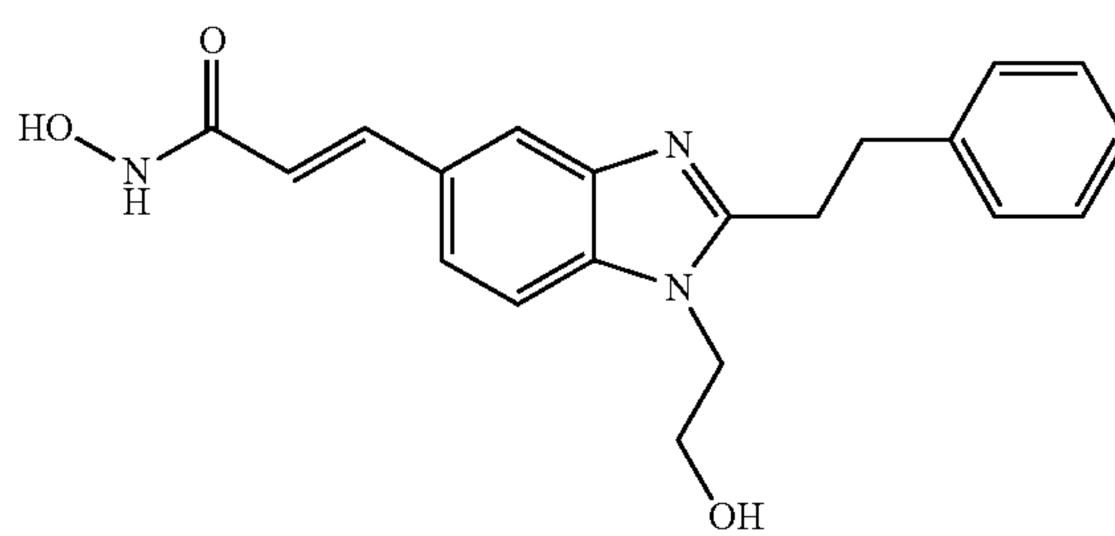
N-Hydroxy-3-[1-(2-hydroxyethyl)-2-phenethyl-1H-benzimidazol-5-yl]-acrylamide
