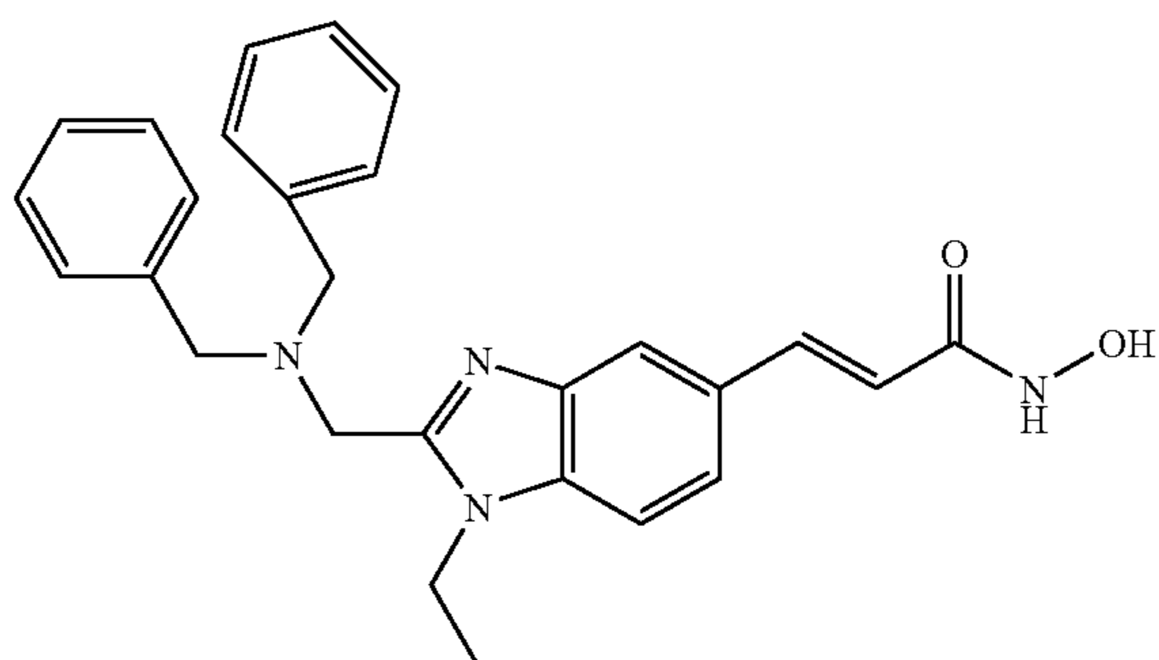
N-Hydroxy-3-{2-[(dibenzylamino)-methyl]-1-ethyl-1H-benzimidazol-5-yl}-acrylamide
