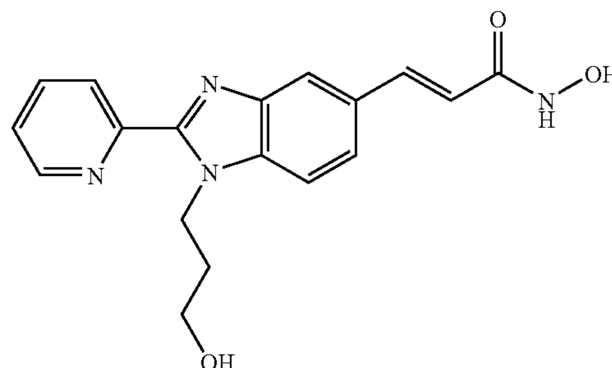
N-Hydroxy-3-[1-(3-hydroxy-propyl)-2-(2-pyridyl)-1H-benzimidazole-5-yl]-acrylamide
