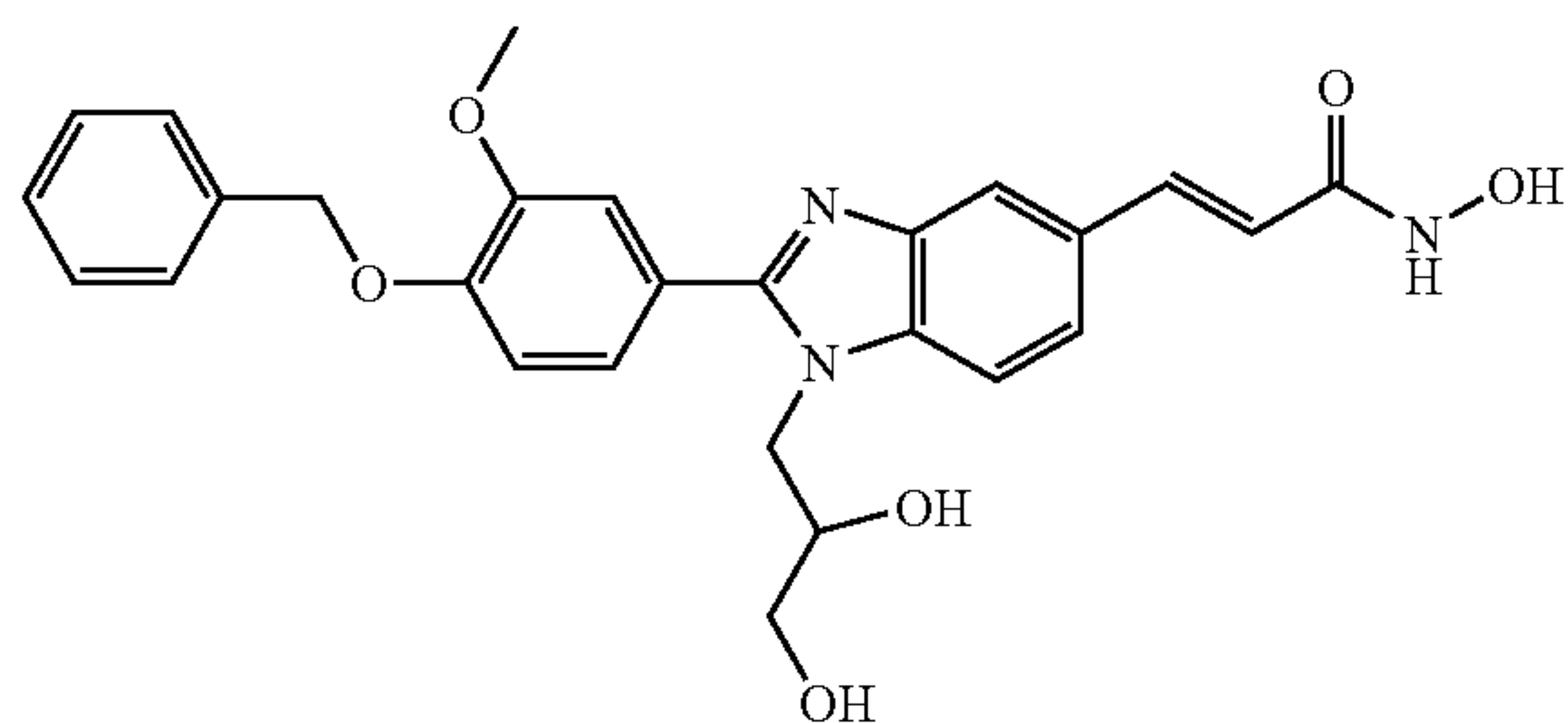
N-Hydroxy-3-[2-(4-benzyloxy-3-methoxy-phenyl)-1-(2,3-hydroxy-propyl)-1H-benzimidazole-5-yl]-acrylamide
