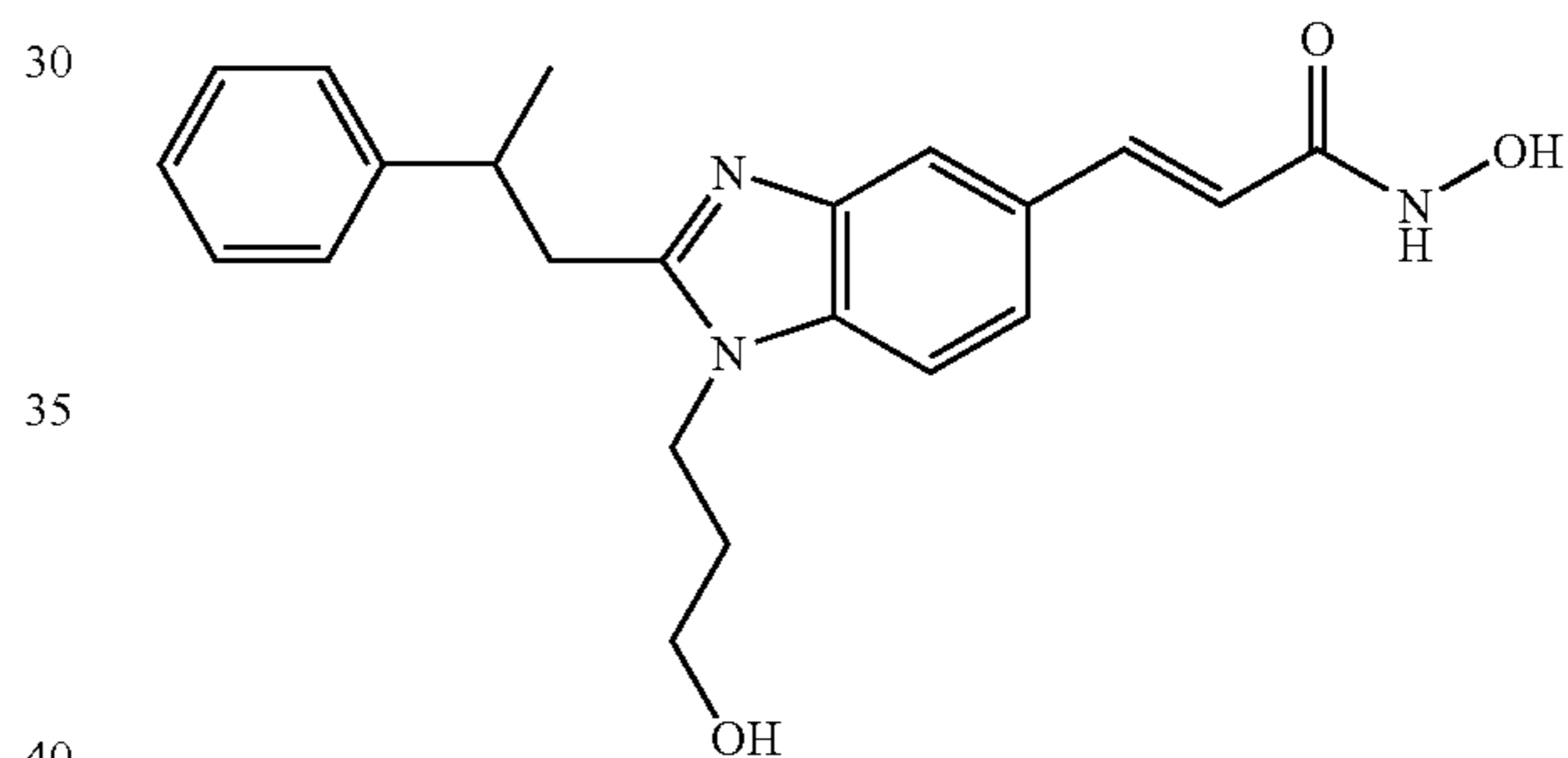
N-Hydroxy-3-[1-(3-hydroxy-propyl)-2-(2-phenyl-propyl)-1H-benzimidazol-5-yl]-acrylamide
