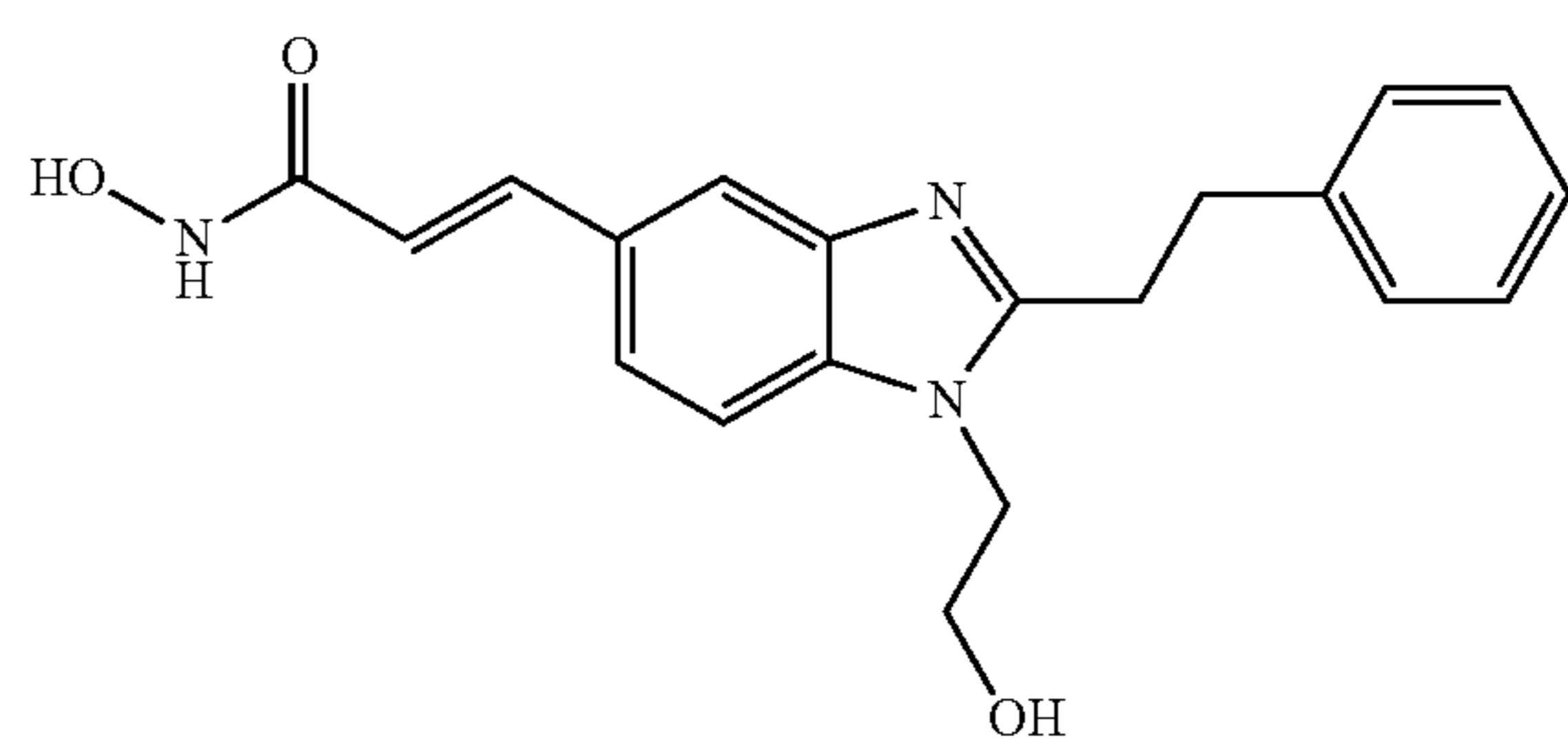
N-Hydroxy-3-[1-(2-hydroxyethyl)-2-phenethyl-1H-benzimidazol-5-yl]-acrylamide
