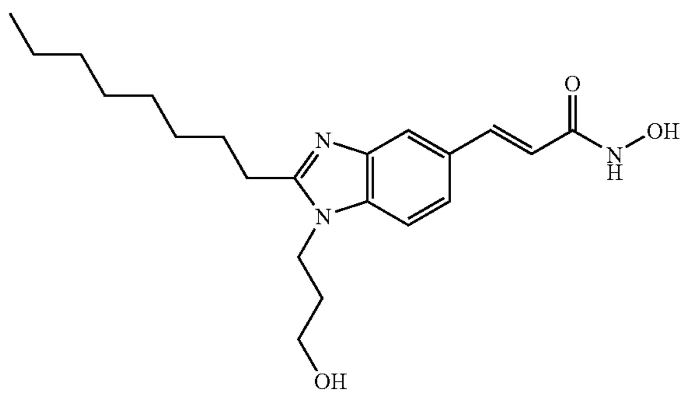
N-Hydroxy-3-[1-(3-hydroxy-propyl)-2-octyl-1H-benzimidazol-5-yl]-acrylamide
