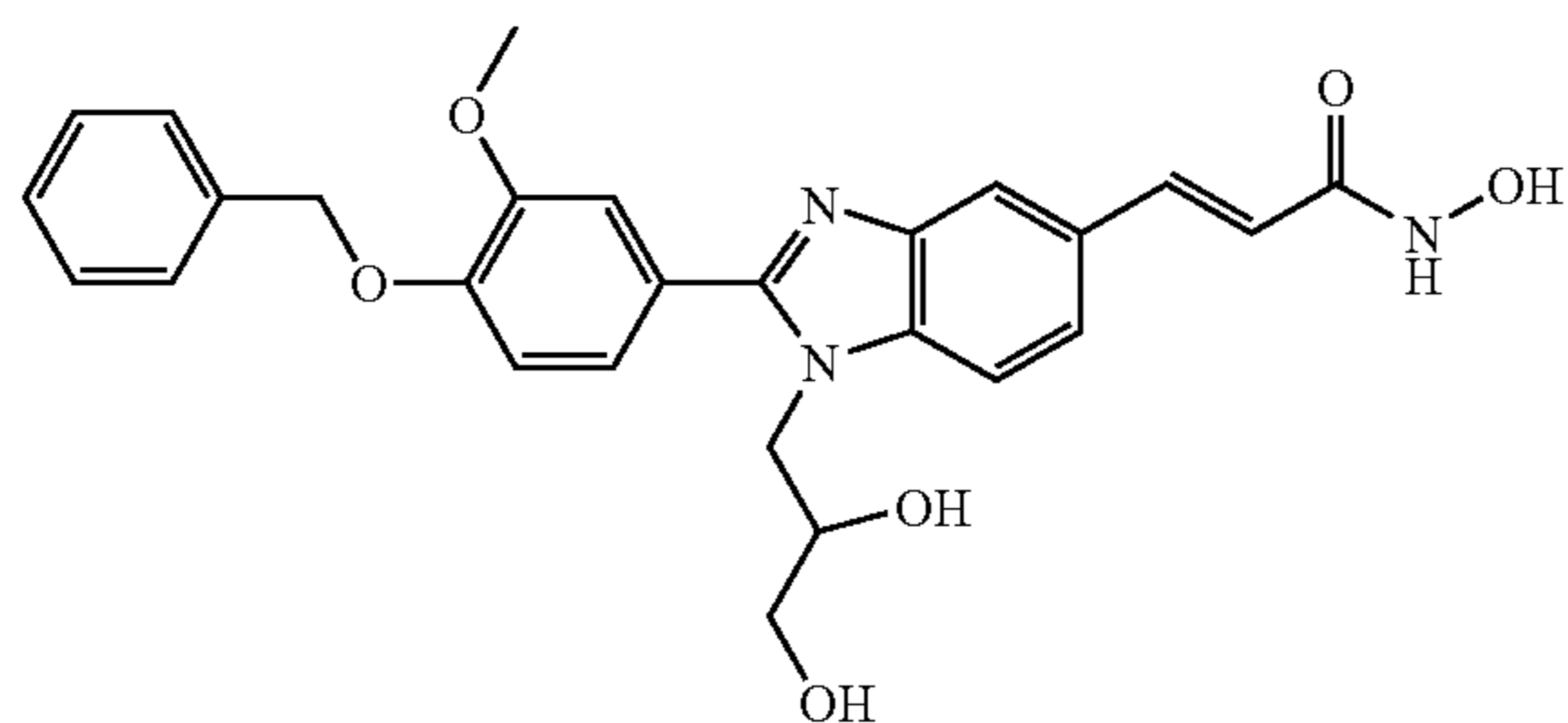
N-Hydroxy-3-[2-(4-benzyloxy-3-methoxy-phenyl)-1-(2,3-hydroxy-propyl)-1H-benzimidazole-5-yl]-acrylamide
