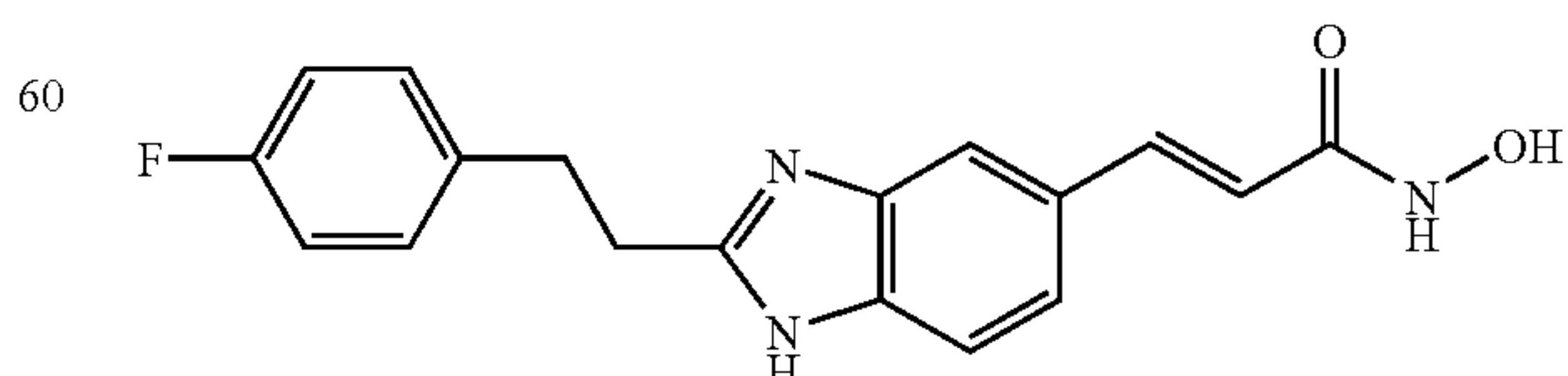
N-Hydroxy-3-(2-(4-fluoro-phenyl)-ethyl)-1H-benzimidazol-5-yl]-acrylamide
