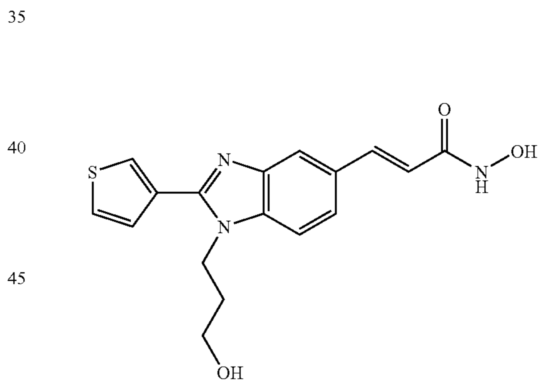
N-Hydroxy-3-[1-(3-hydroxy-propyl)-2-thiophen-3-yl-1H-benzimidazol-5-yl]-acrylamide
