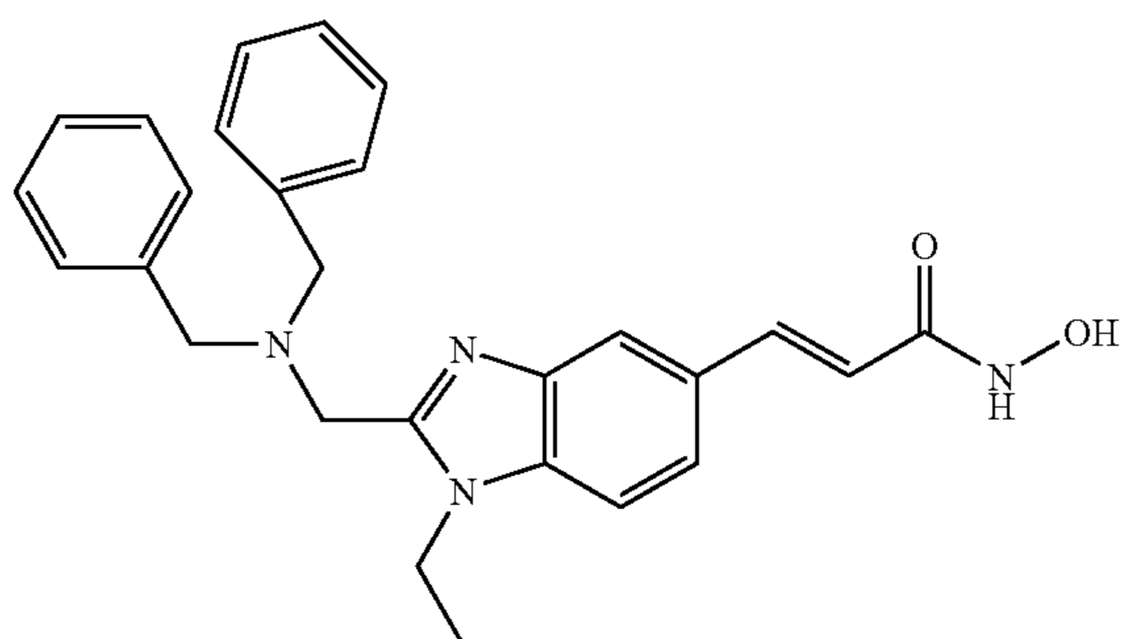
N-Hydroxy-3-{2-[(dibenzylamino)-methyl]-1-ethyl-1H-benzimidazol-5-yl}-acrylamide
