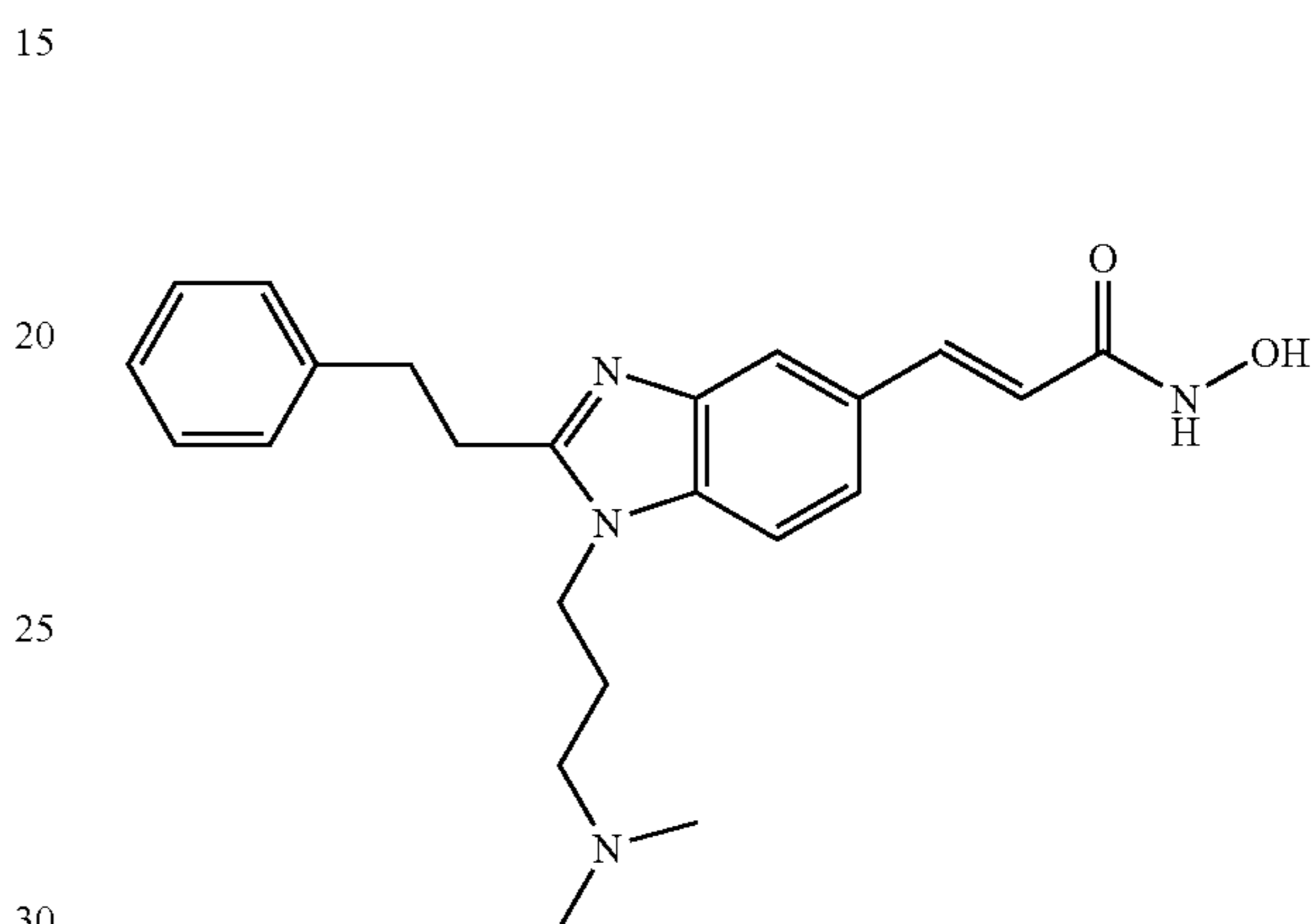
N-Hydroxy-3-[1-(3-dimethylamino-propyl)-2-phenethyl-1H-benzimidazol-5-yl]-acrylamide
