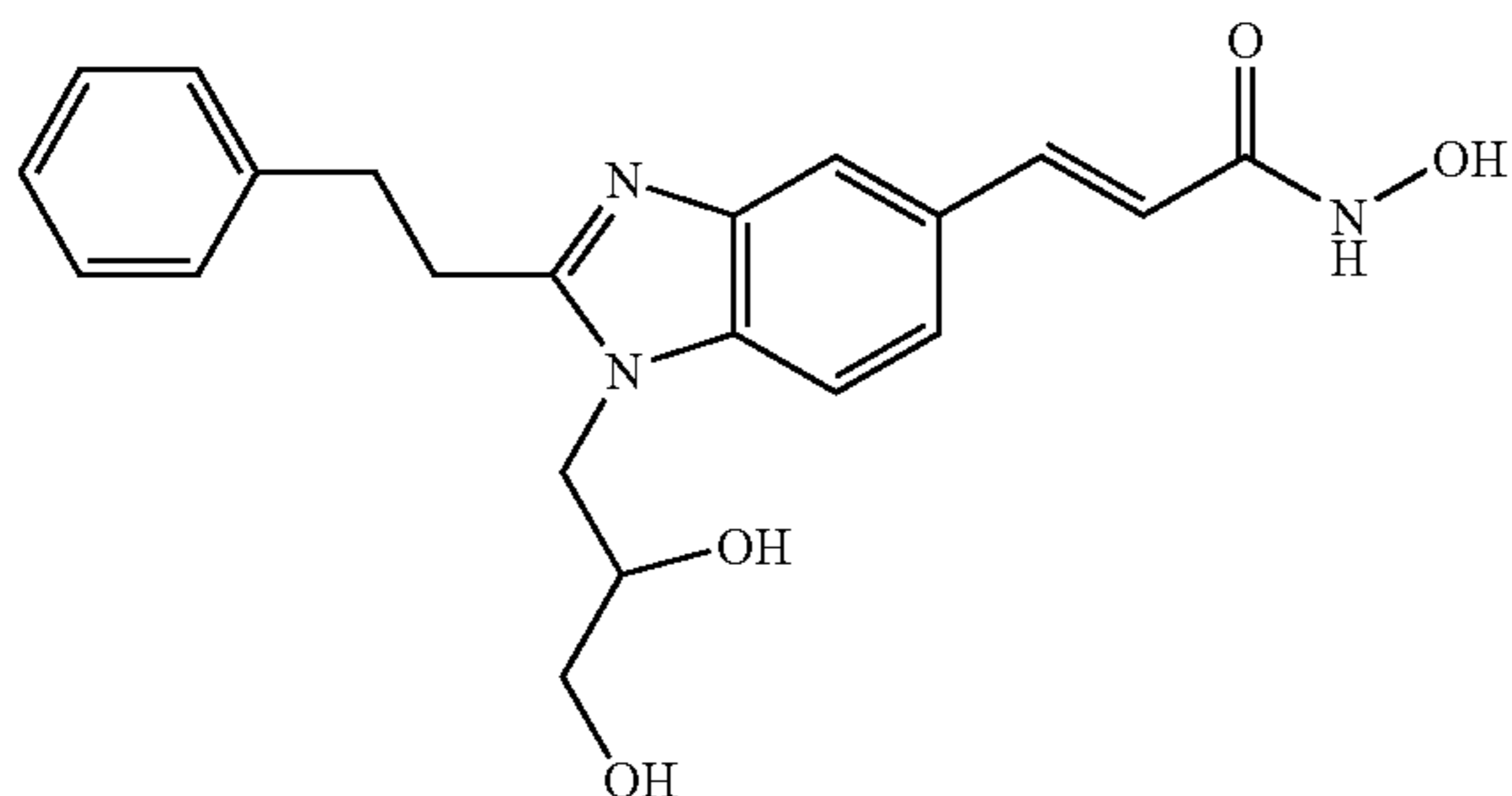
N-Hydroxy-3-[1-(2,3-hydroxy-propyl)-2-(2-phenyl-ethyl)-1H-benzimidazole-5-yl]-acrylamide
