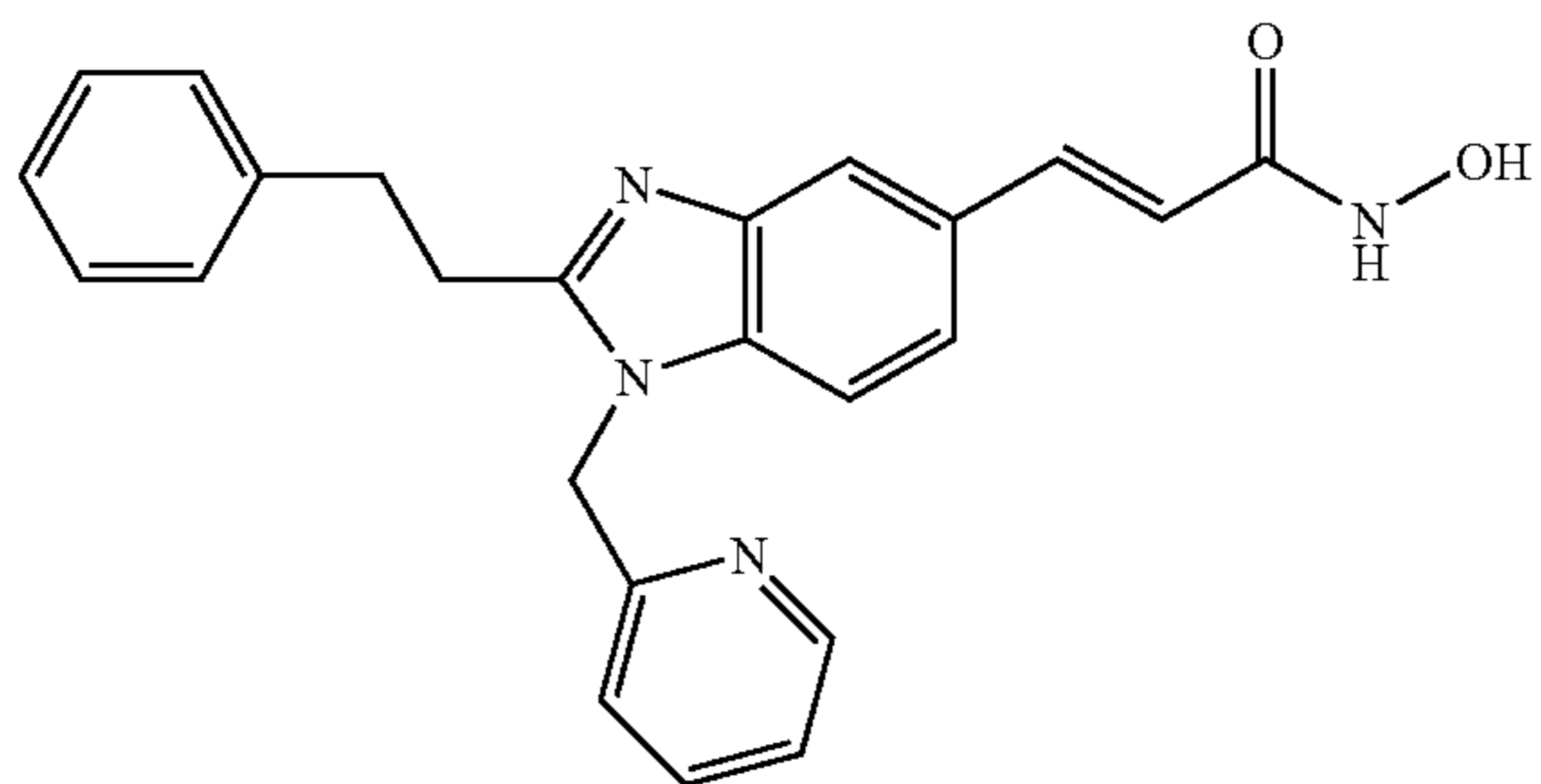
N-Hydroxy-3-[2-phenethyl-1-(pyridin-2-yl)methyl-1H-benzimidazol-5-yl]-acrylamide
