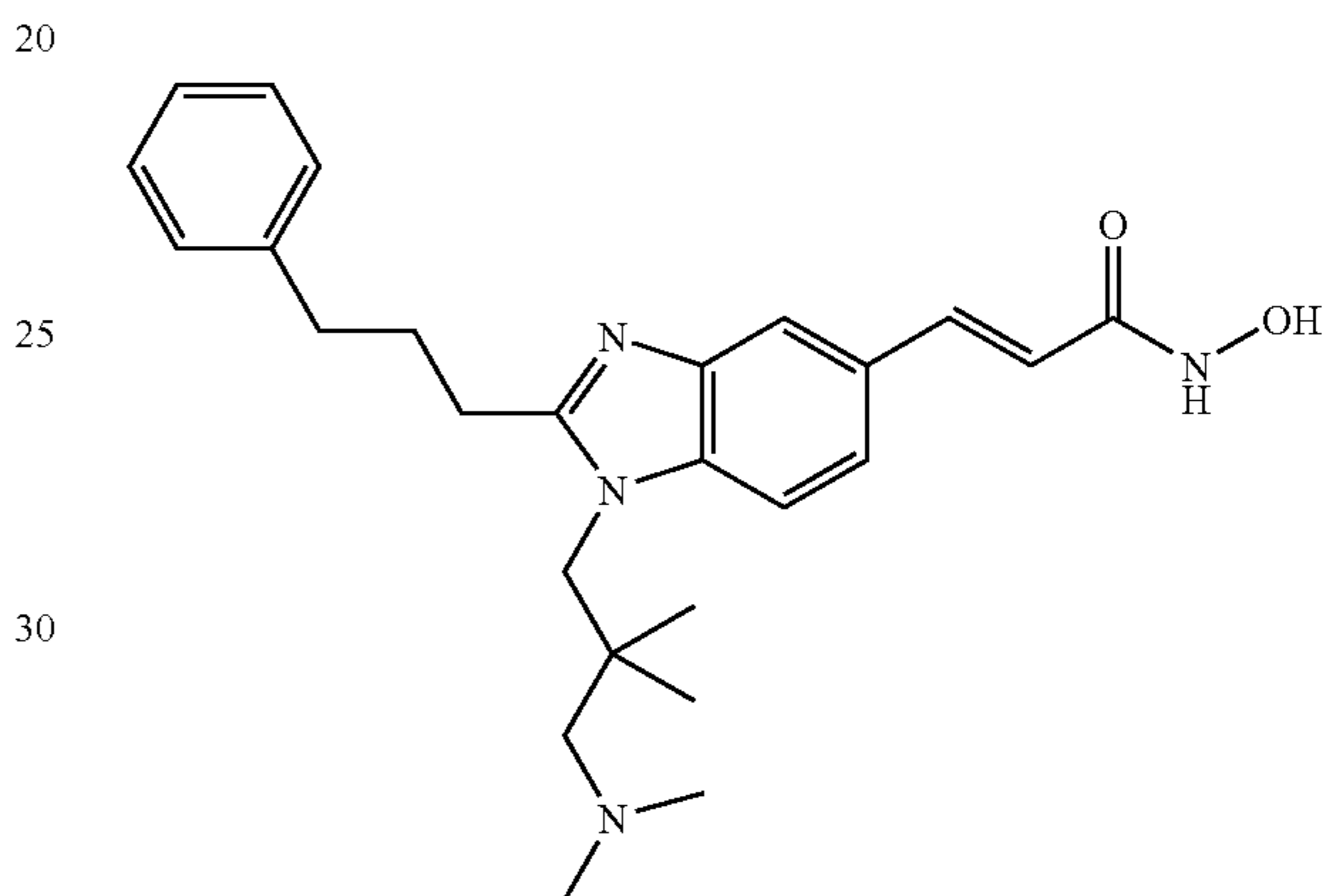
N-Hydroxy-3-[1-(3-Dimethylamino-2,2-dimethyl-propyl)-2-(3-phenyl-propyl)-1H-benzimidazol-5-yl]-acrylamide
