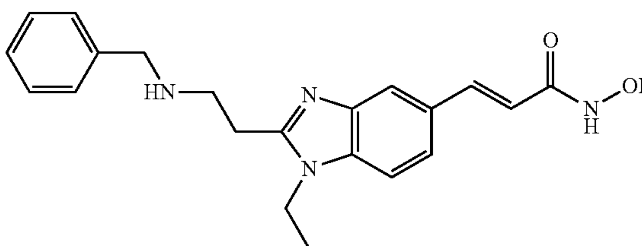
N-Hydroxy-3-[2-(2-benzylamino-ethyl)-1-ethyl-1H-benzimidazol-5-yl]-acrylamide
