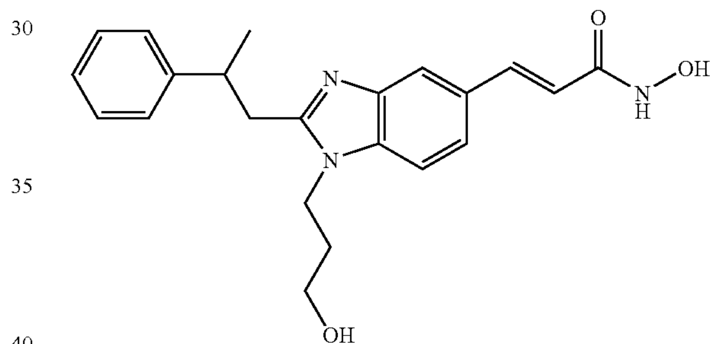
N-Hydroxy-3-[1-(3-hydroxy-propyl)-2-(2-phenyl-propyl)-1H-benzimidazol-5-yl]-acrylamide
