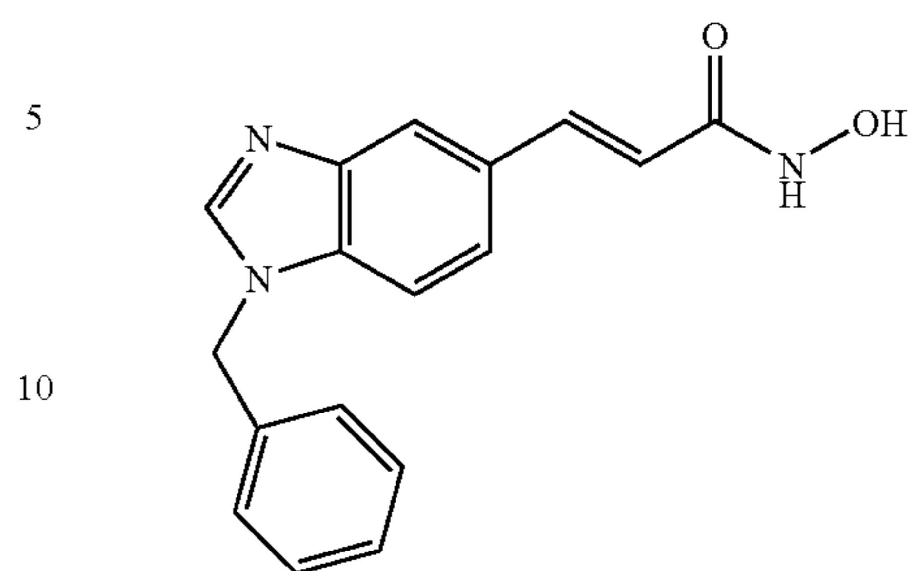
N-Hydroxy-3-(1-benzyl-1H-benzimidazol-5-yl)-acrylamide
