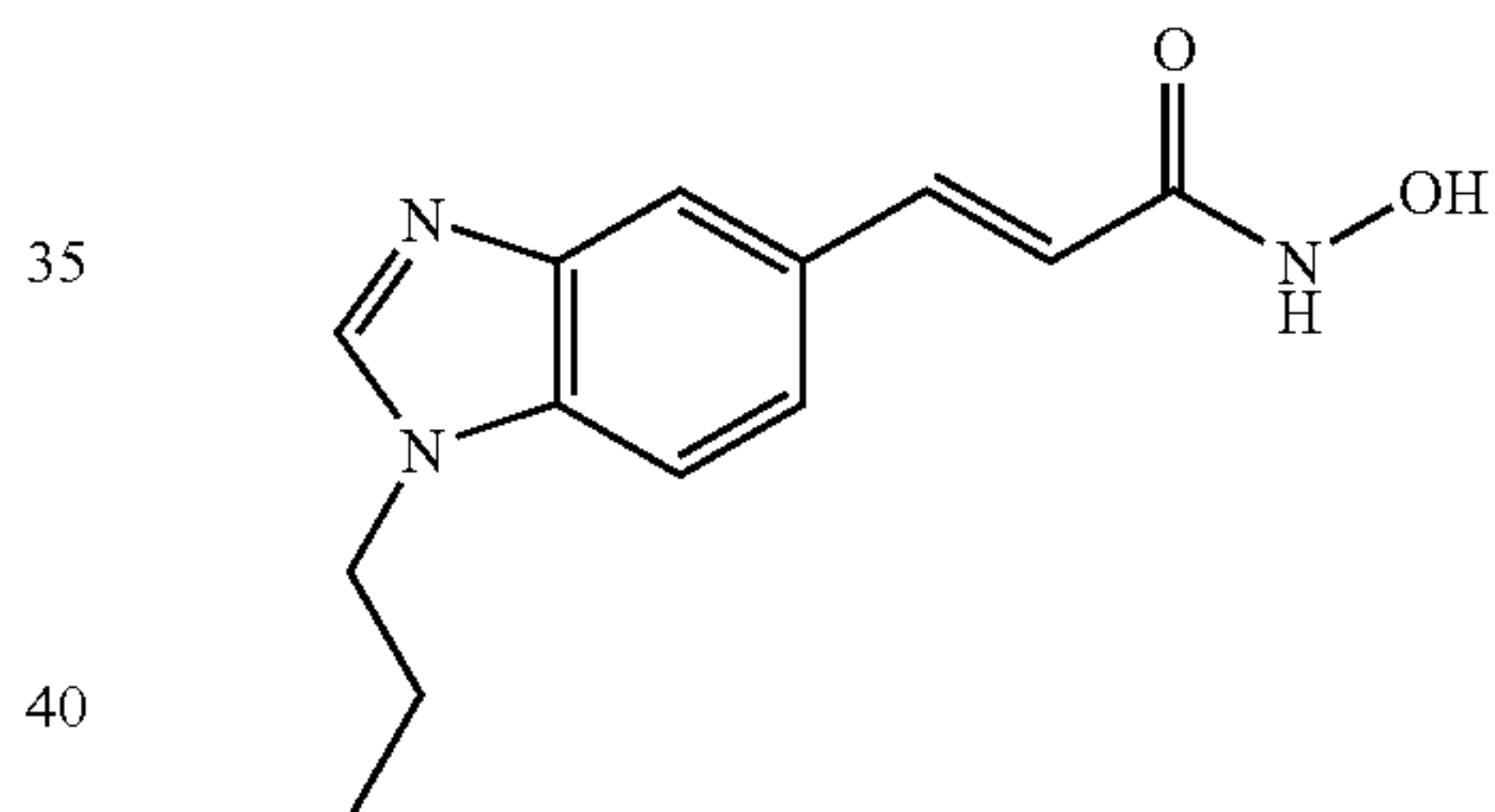
N-Hydroxy-3-(1-propyl-1H-benzimidazol-5-yl)-acrylamide
