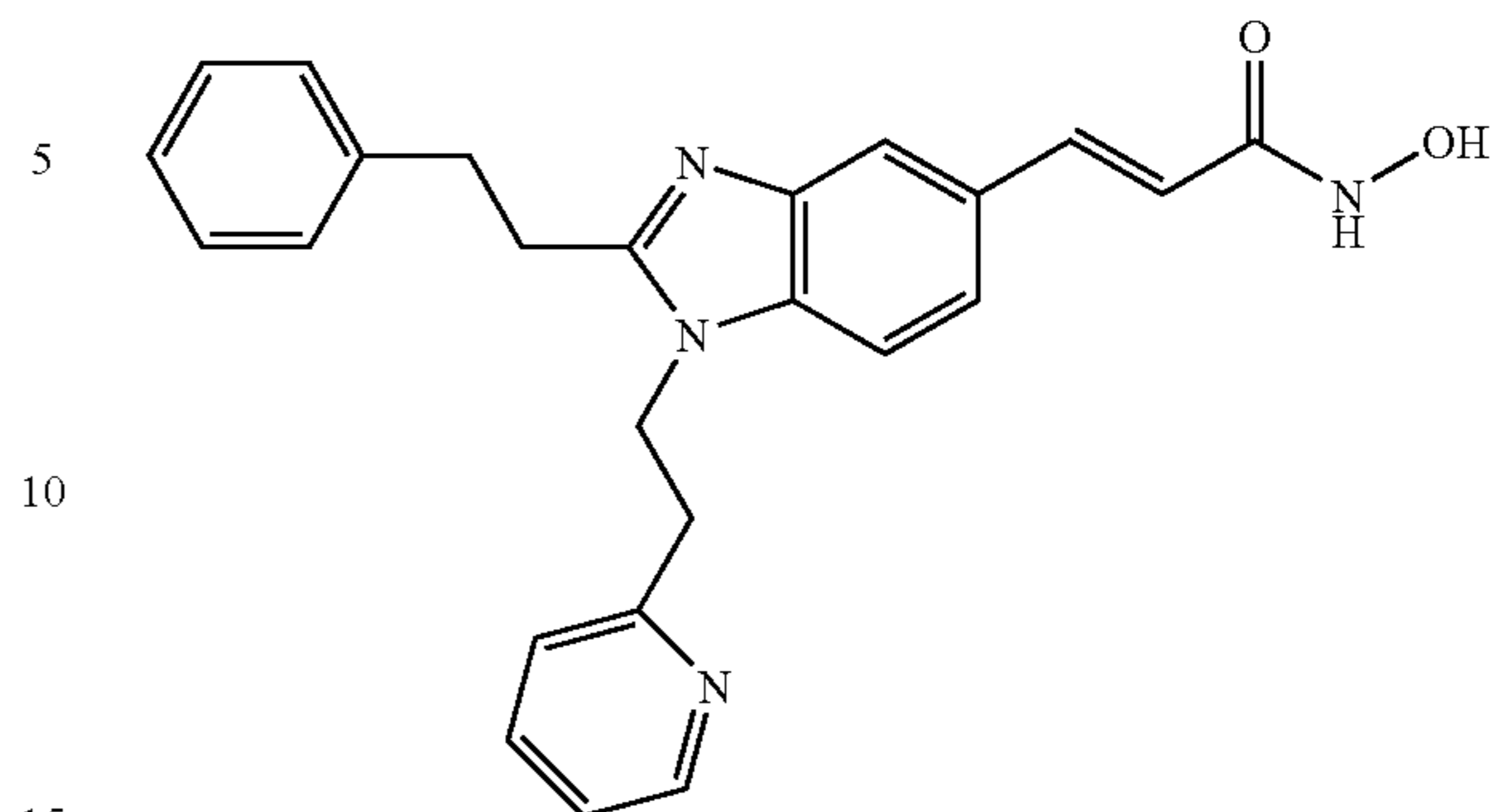
N-Hydroxy-3-[2-phenethyl-1-(2-pyridin-2-yl-ethyl)-1H-benzimidazol-5-yl]-acrylamide
