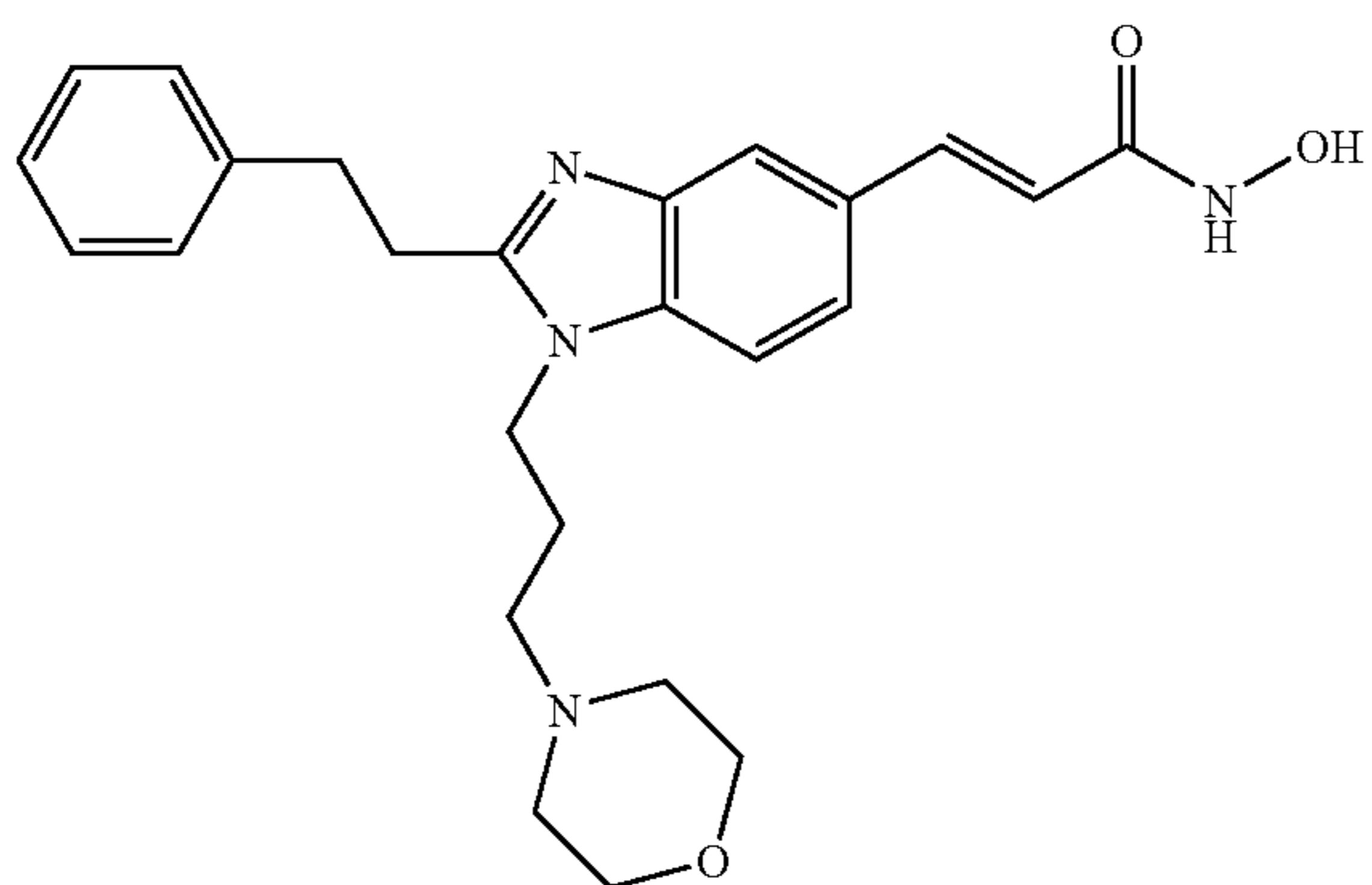
N-Hydroxy-3-[1-(3-morpholin-4-propyl)-2-phenethyl-1H-benzimidazol-5-yl]-acrylamide
