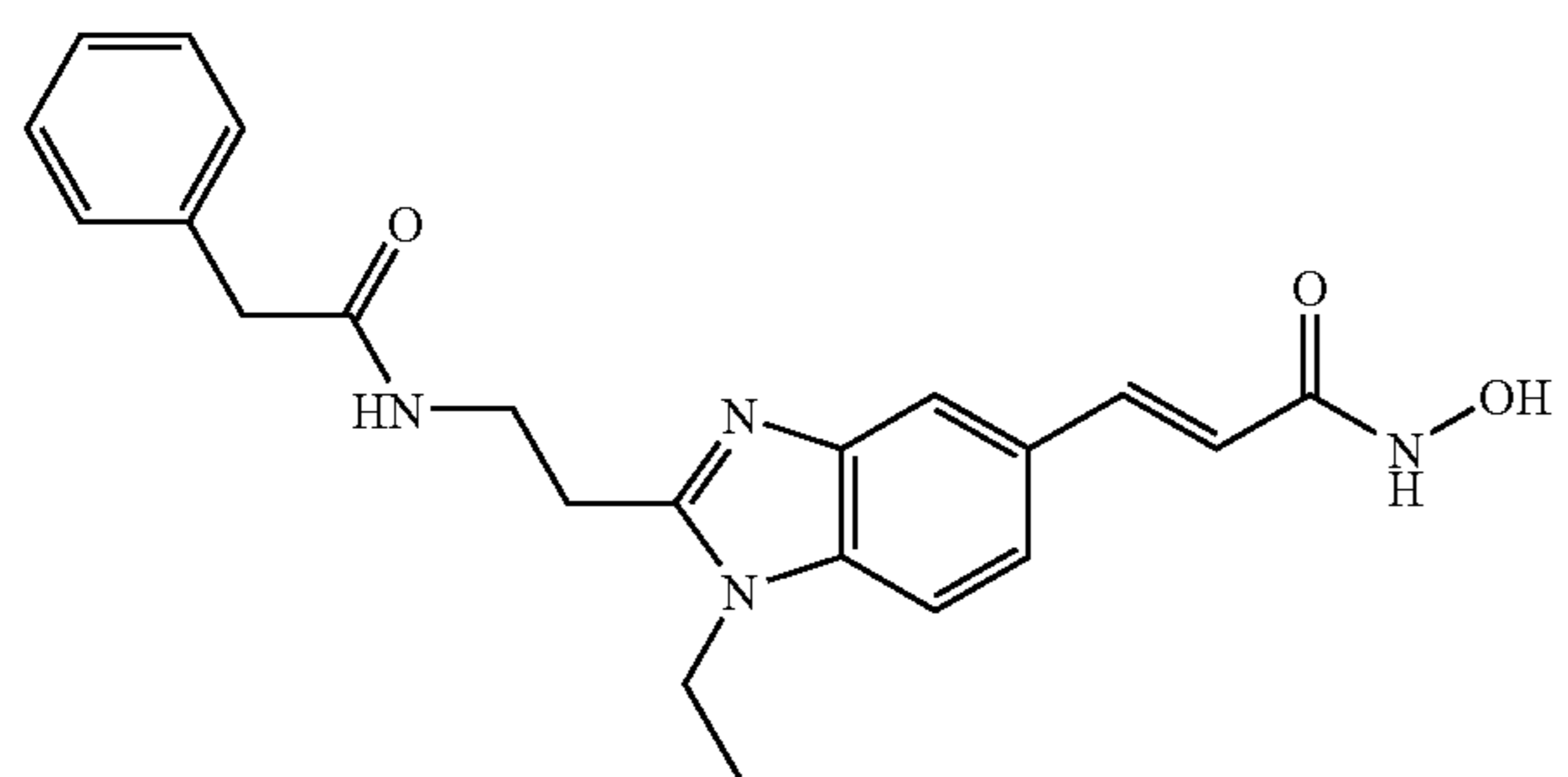
N-Hydroxy-3-[1-ethyl-2-(2-phenylacetyl-amino-ethyl)-1H-benzimidazol-5-yl]-acrylamide
