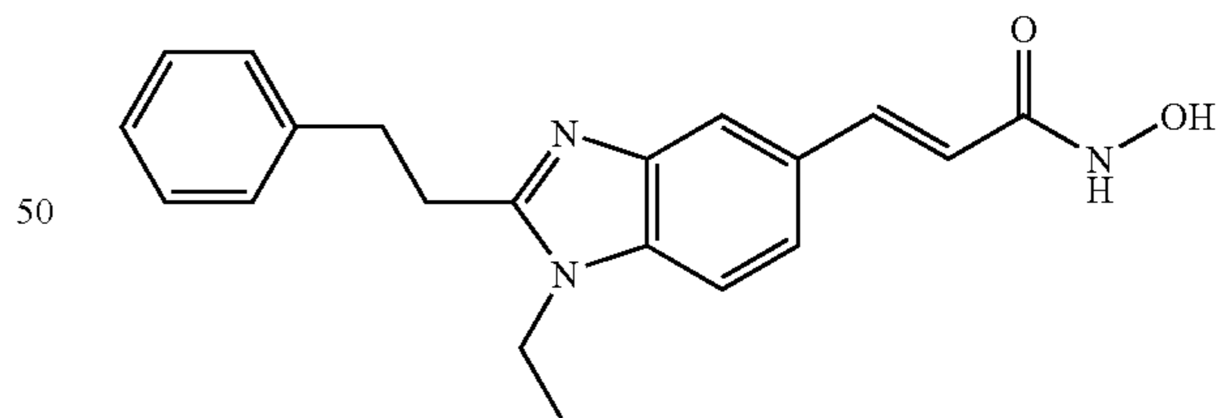
N-Hydroxy-3-(1-Ethyl-2-phenethyl-1H-benzimidazol-5-yl)-acrylamide
