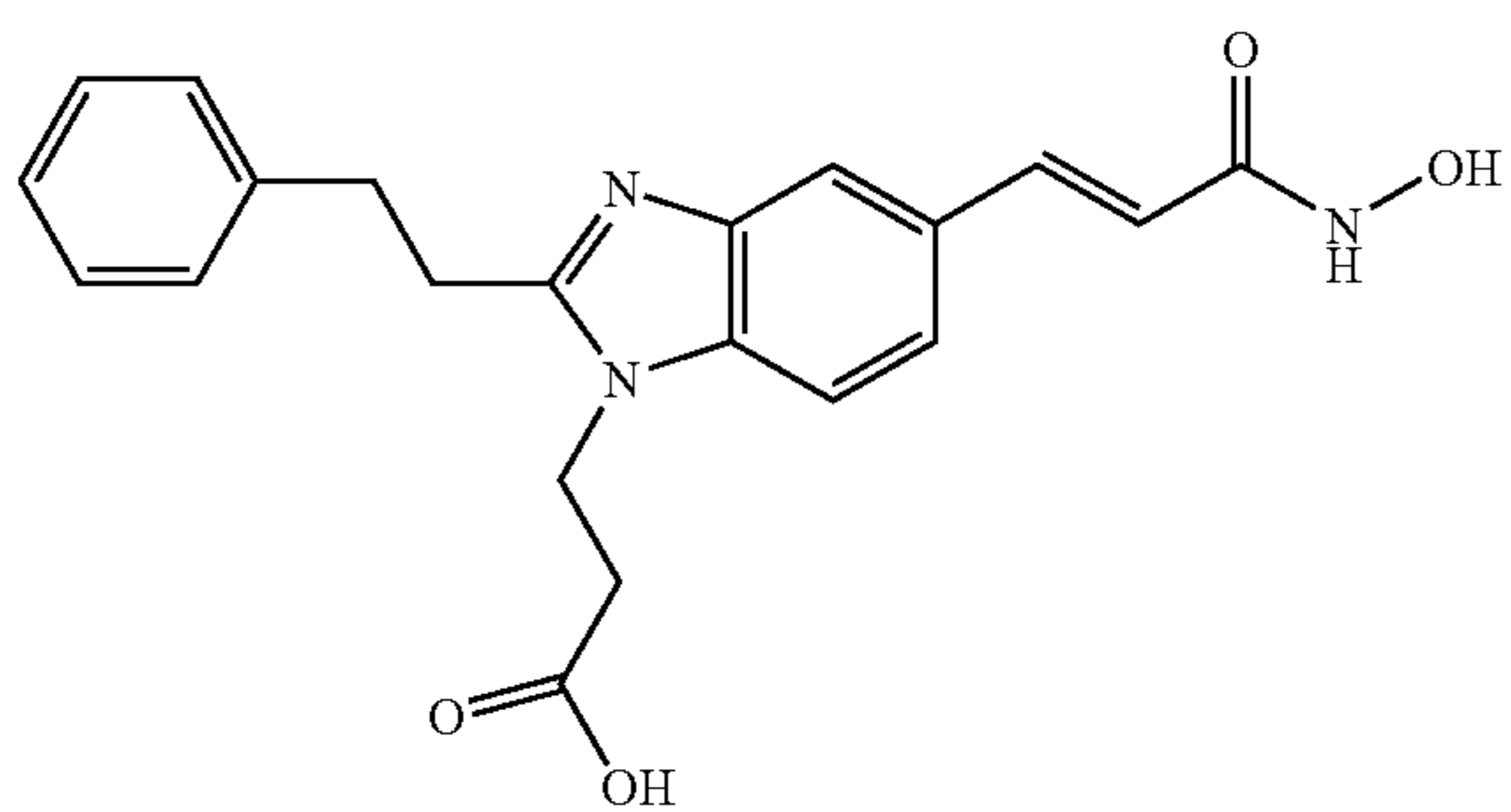
3-[5-(2-Hydroxycarbonyl-vinyl)-2-phenethyl-1H-benzimidazol-5-yl]-propionic acid
