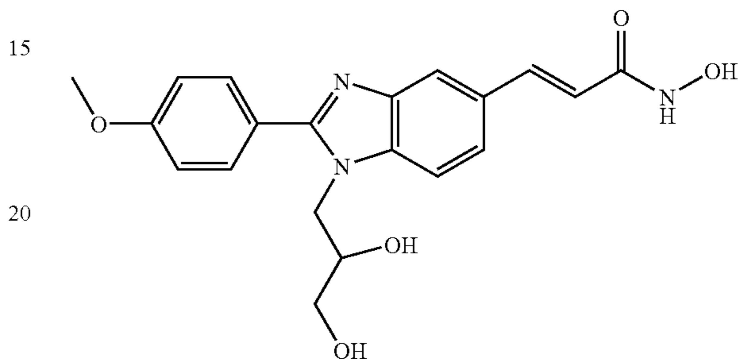
N-Hydroxy-3-[1-(2,3-hydroxy-propyl)-2-(4-methoxy-phenyl)-1H-benzimidazole-5-yl]-acrylamide
