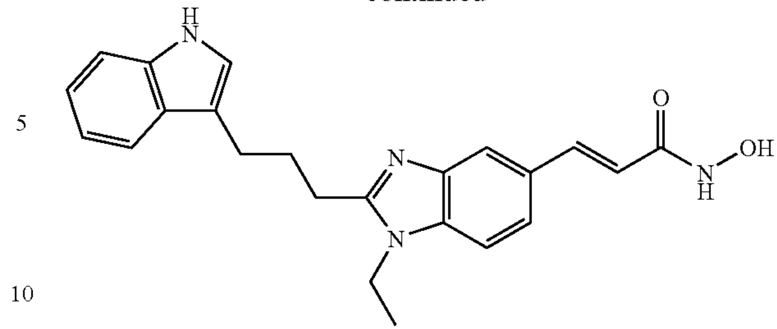
N-Hydroxy-3-[1-ethyl-2-[3-(1H-indol-3-yl)-propyl]-1H-benzimidazol-5-yl]-acrylamide
