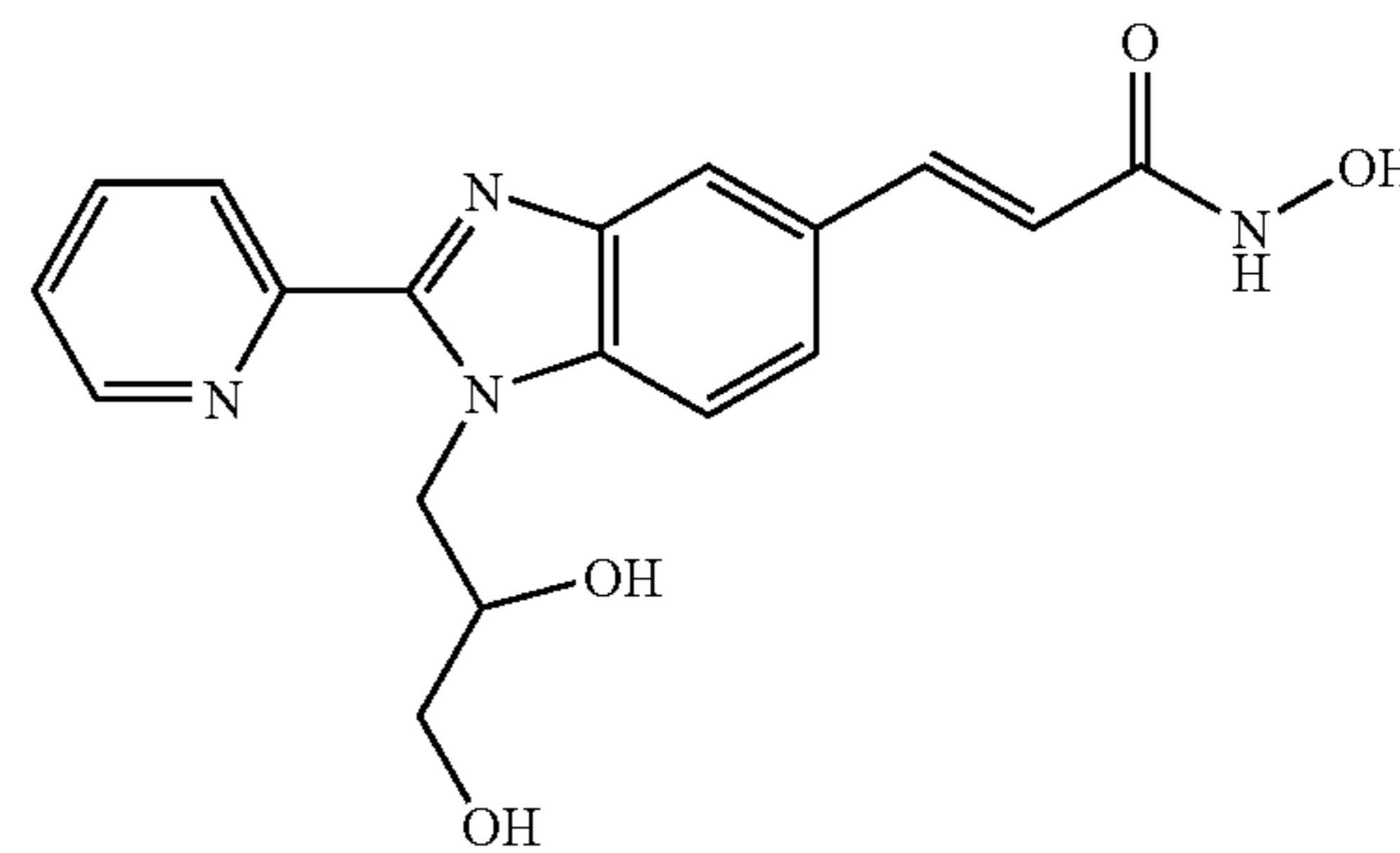
N-Hydroxy-3-[1-(2,3-hydroxy-propyl)-2-(2-pyridyl)-1H-benzimidazole-5-yl]-acrylamide
