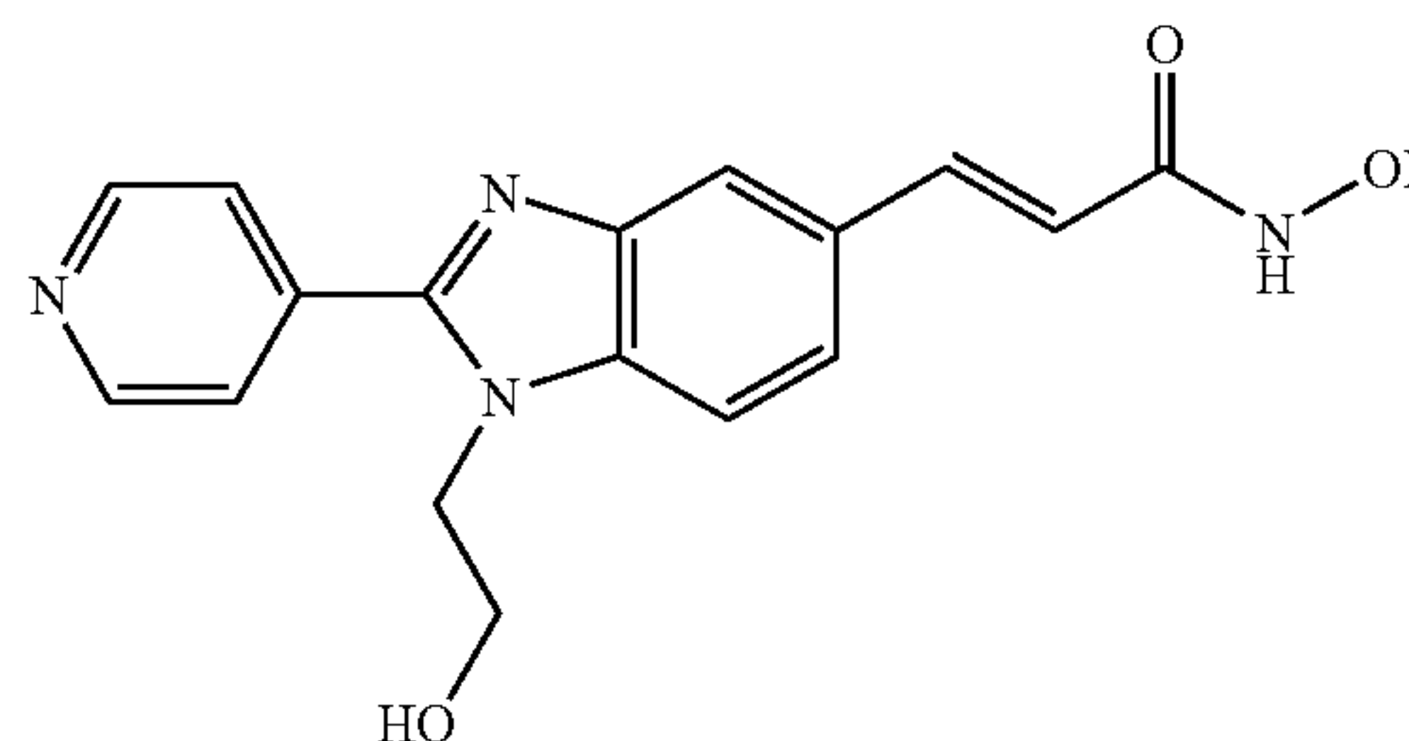
N-Hydroxy-3-[1-(2-hydroxy-ethyl)-2-(4-pyridyl)-1H-benzimidazole-5-yl]-acrylamide
