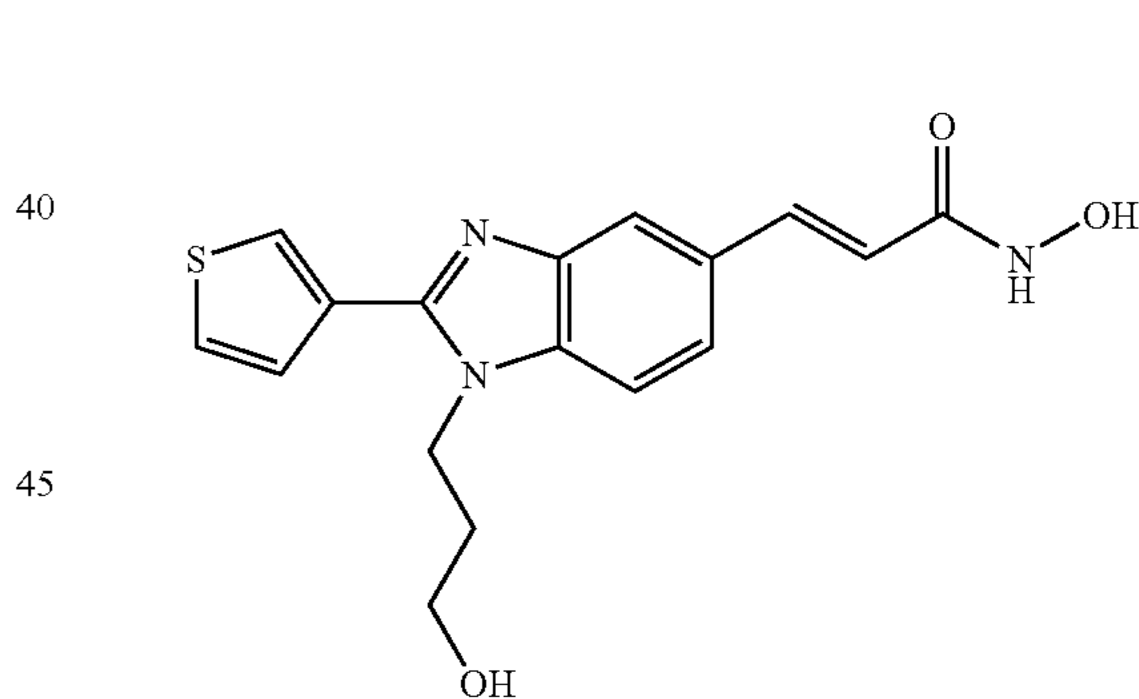
N-Hydroxy-3-[1-(3-hydroxy-propyl)-2-thiophen-3-yl-1H-benzimidazol-5-yl]-acrylamide
