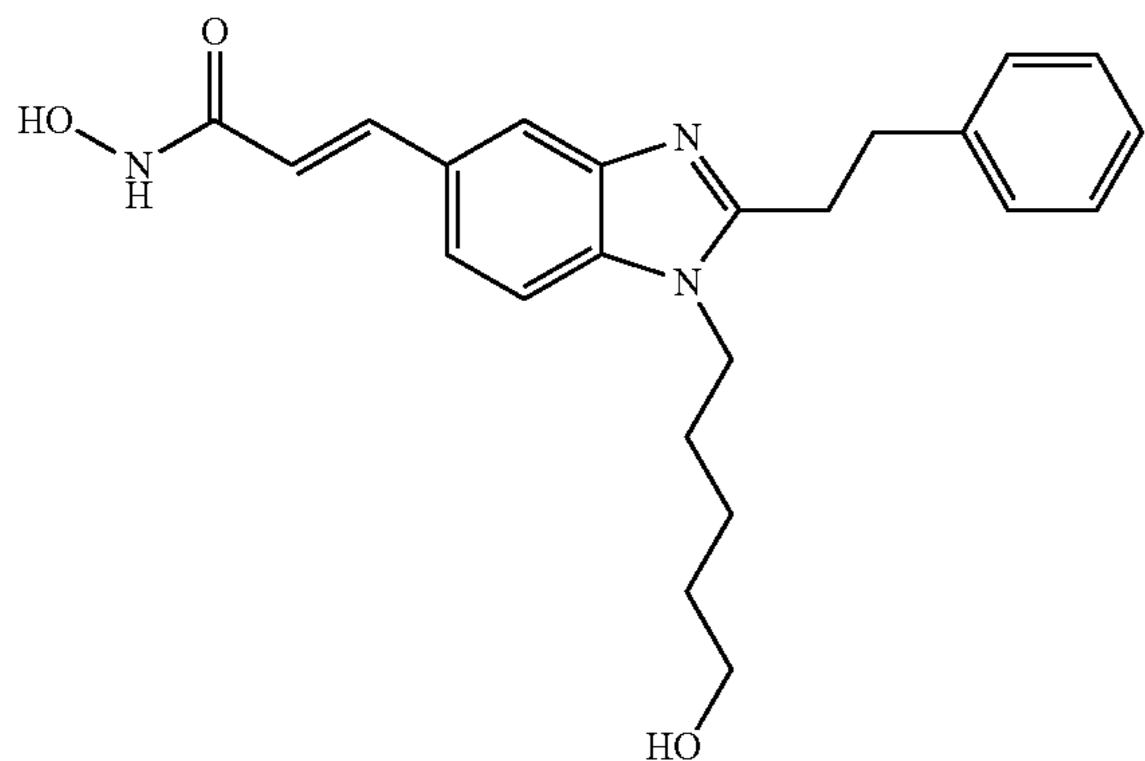
N-Hydroxy-3-[1-(5-hydroxy-pentyl)-2-phenethyl-1H-benzimidazol-5-yl]-acrylamide
