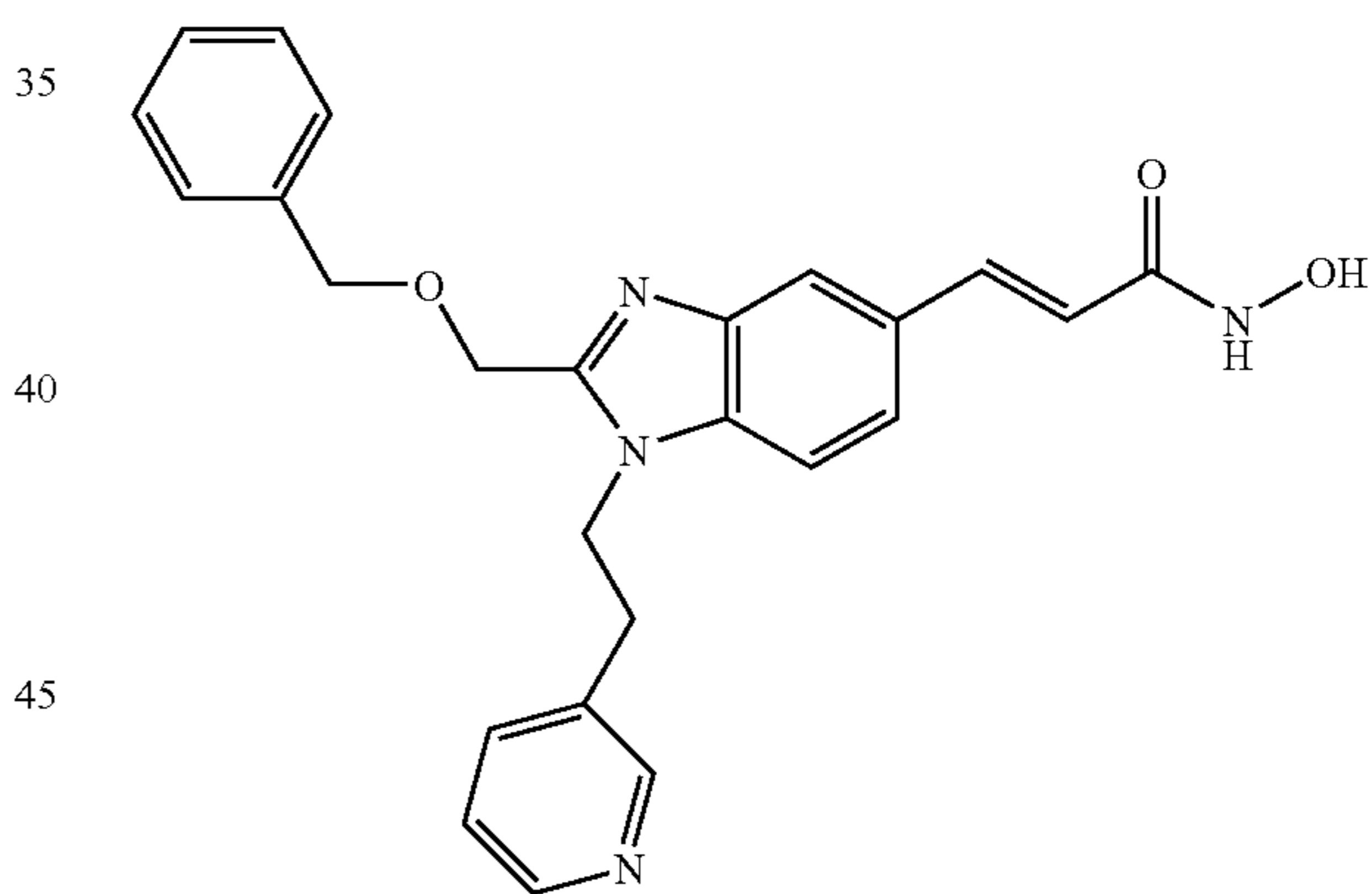
N-Hydroxy-3-[2-Benzyloxymethyl-1-(2-pyridin-3-ethyl)-1H-benzimidazol-5-yl]-acrylamide
