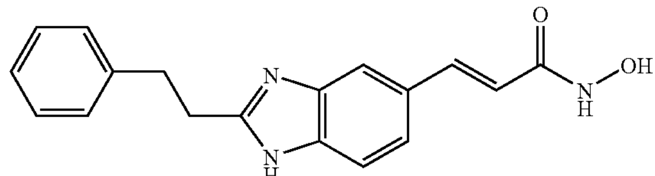
N-Hydroxy-3-(2-phenethyl-1H-benzimidazol-5-yl)-acrylamide
