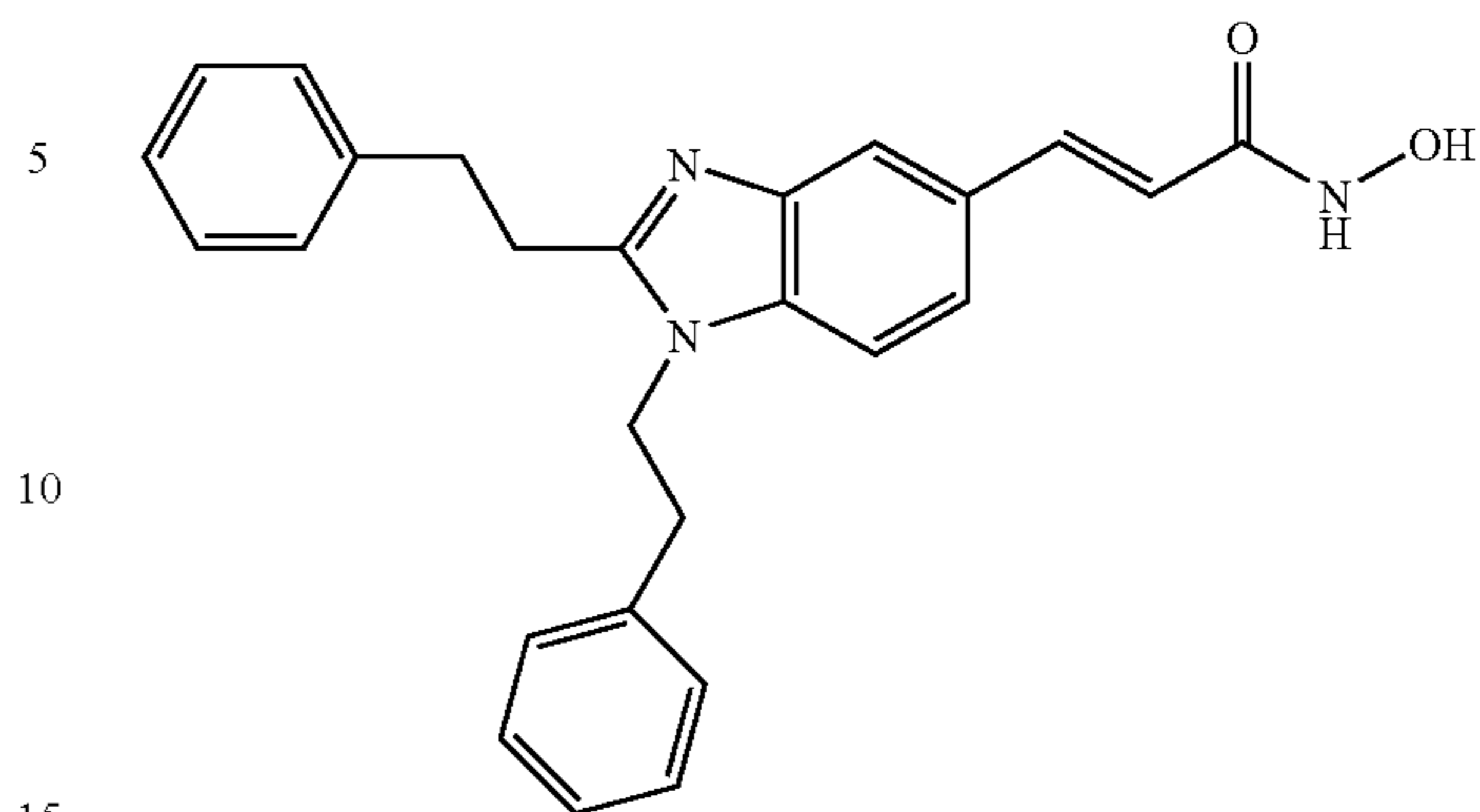
N-Hydroxy-3-(1,2-Diphenethyl-1H-benzimidazol-5-yl)-acrylamide
