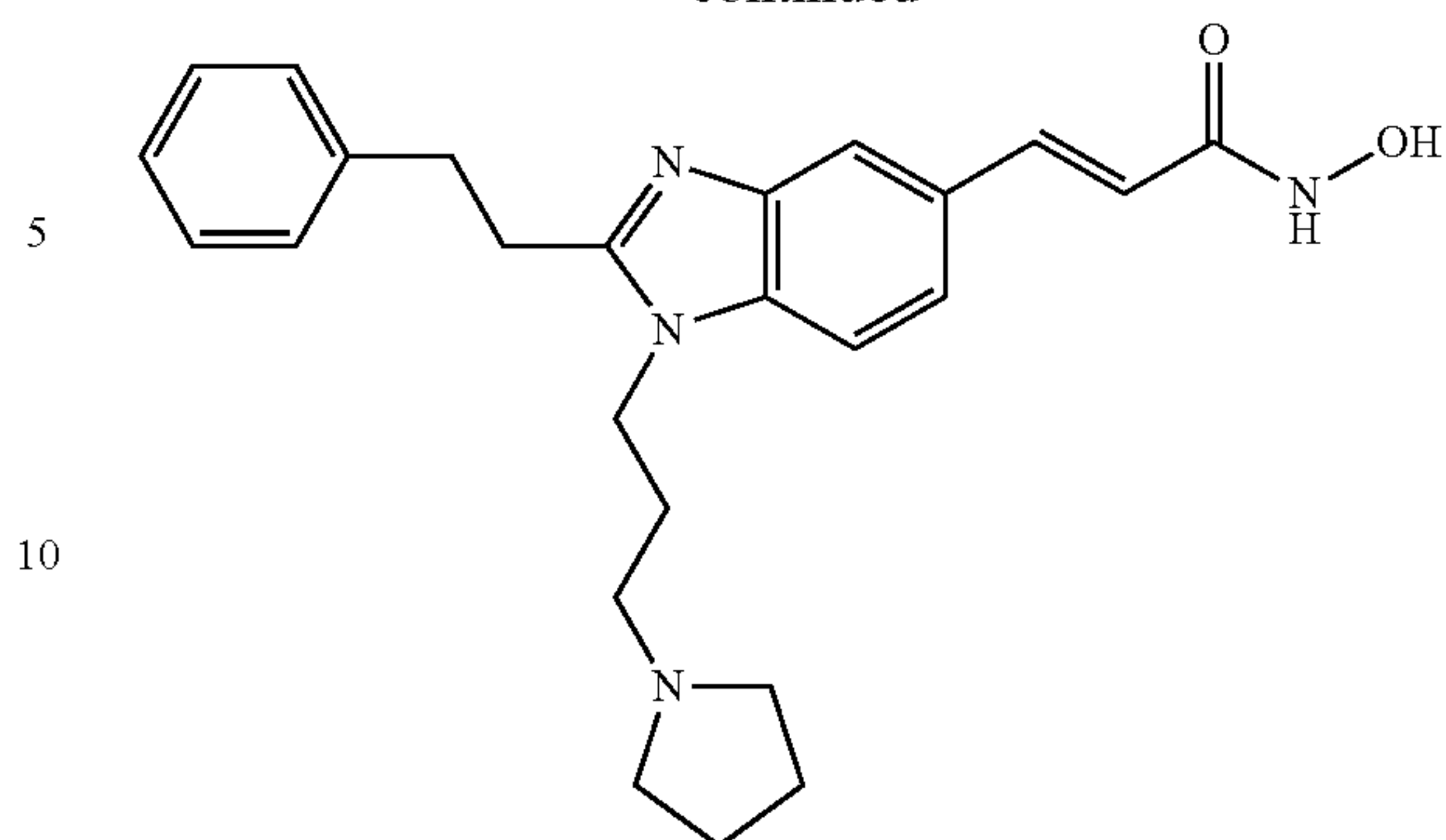
N-Hydroxy-3-[2-phenethyl-1-(3-pyrrolidin-1-yl-propyl)-1H-benzimidazol-5-yl]-acrylamide
