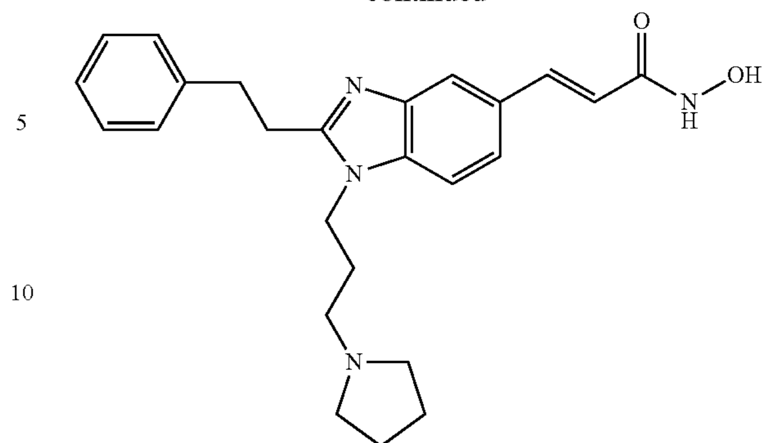
N-Hydroxy-3-[2-phenethyl-1-(3-pyrrolidin-1-yl-propyl)-1H-benzimidazol-5-yl]-acrylamide
