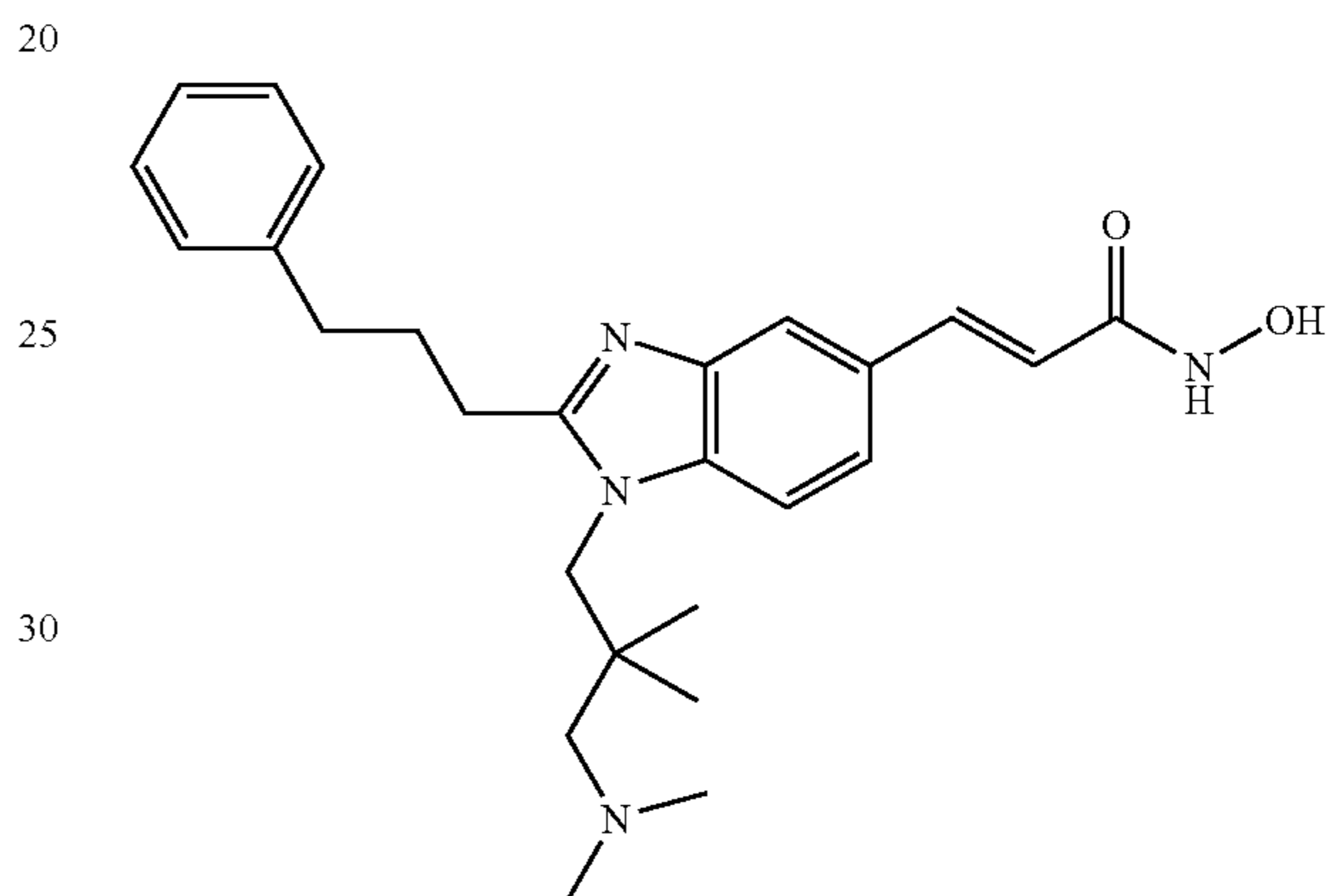
N-Hydroxy-3-[1-(3-Dimethylamino-2,2-dimethyl-propyl)-2-(3-phenyl-propyl)-1H-benzimidazol-5-yl]-acrylamide
