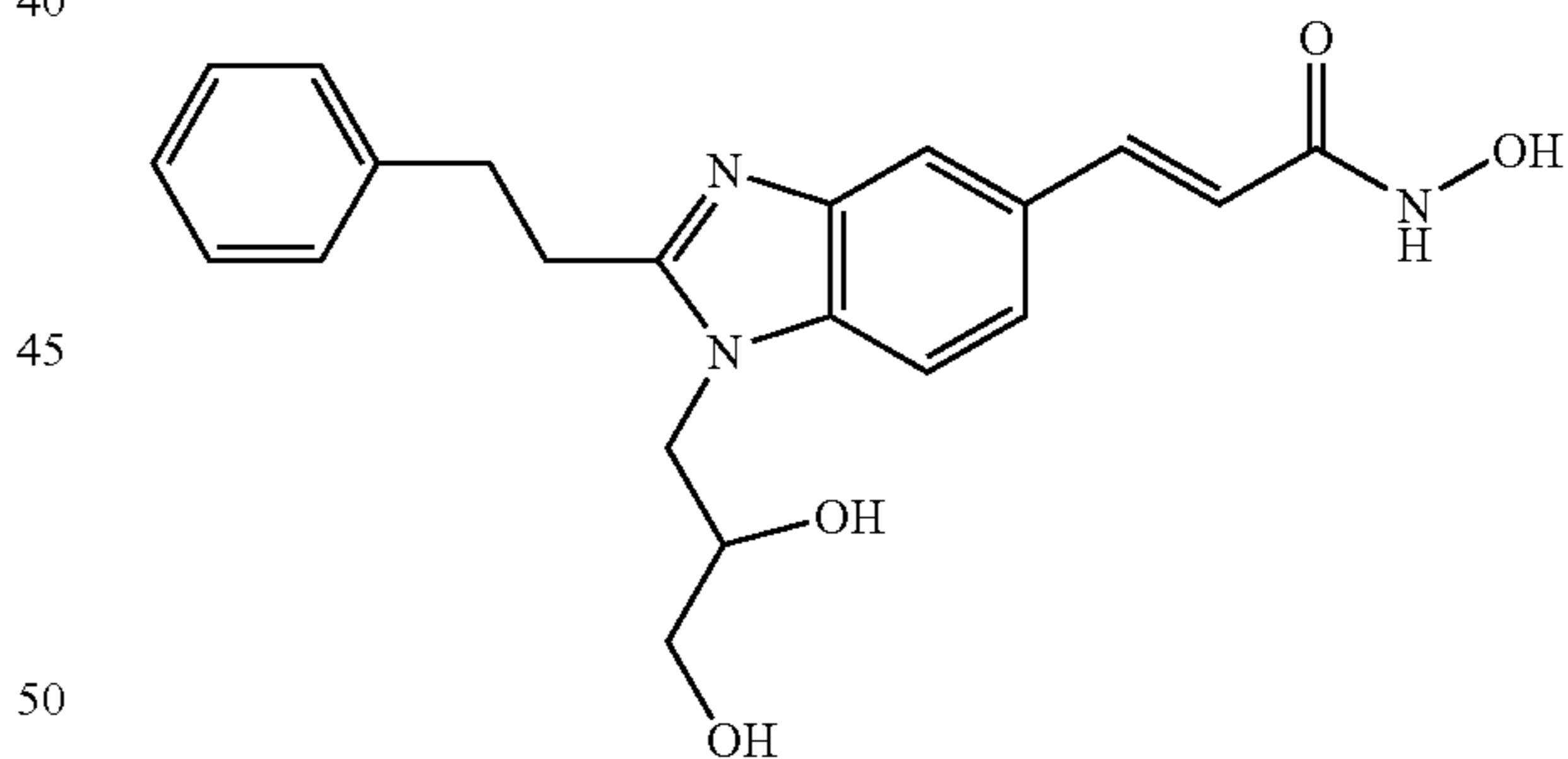
N-Hydroxy-3-[1-(2,3-hydroxy-propyl)-2-(2-phenyl-ethyl)-1H-benzimidazol-5-yl]-acrylamide
