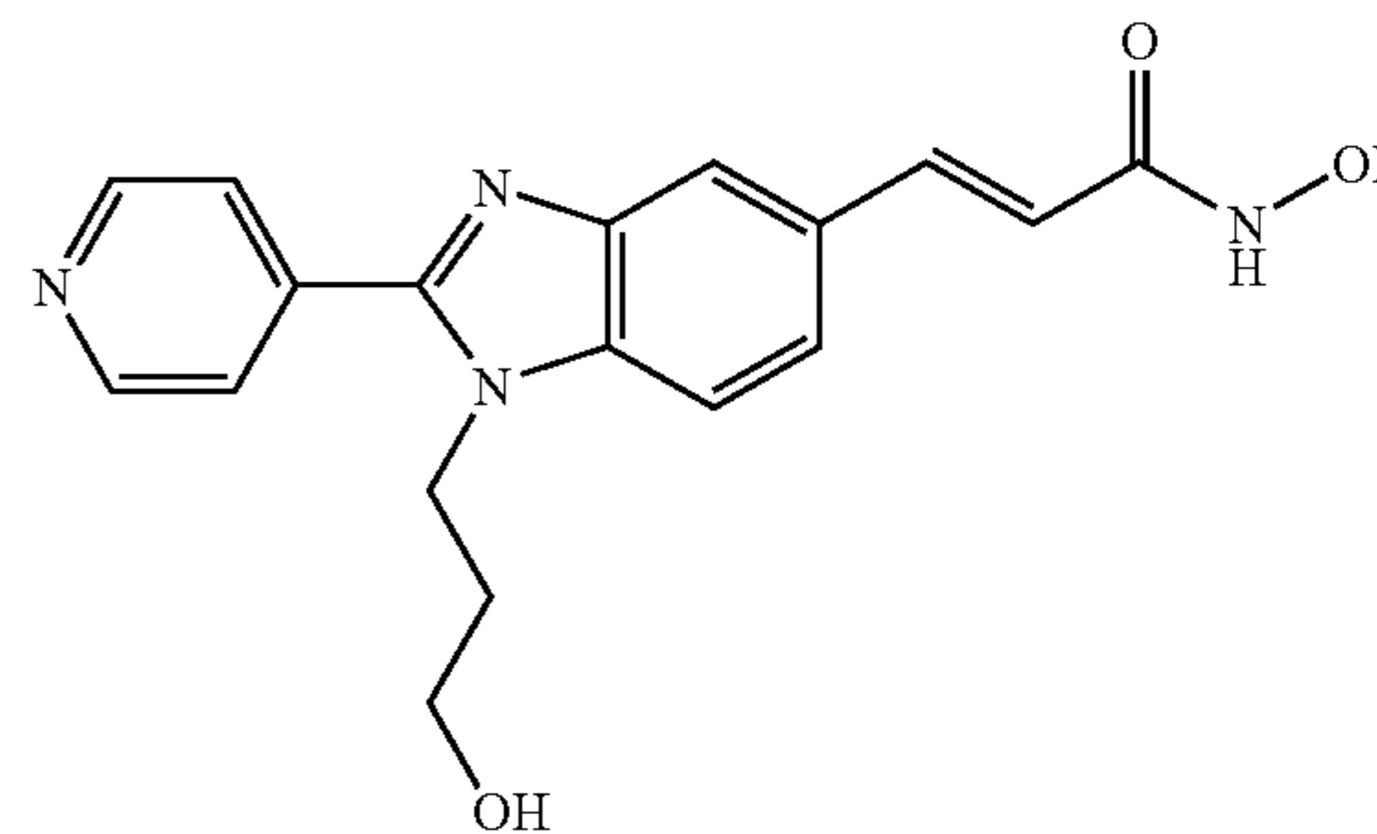
N-Hydroxy-3-[1-(3-hydroxy-propyl)-2-(4-pyridyl)-1H-benzimidazole-5-yl]-acrylamide
