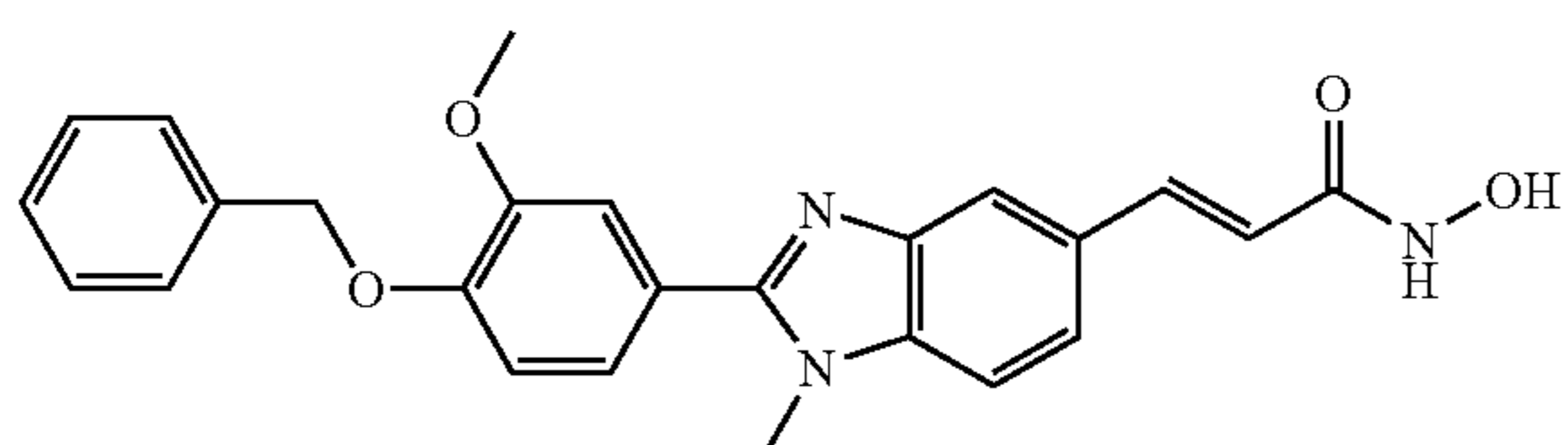
N-Hydroxy-3-[2-(4-benzyloxy-3-methoxy-phenyl)-1-methyl-1H-benzimidazol-5-yl]-acrylamide
