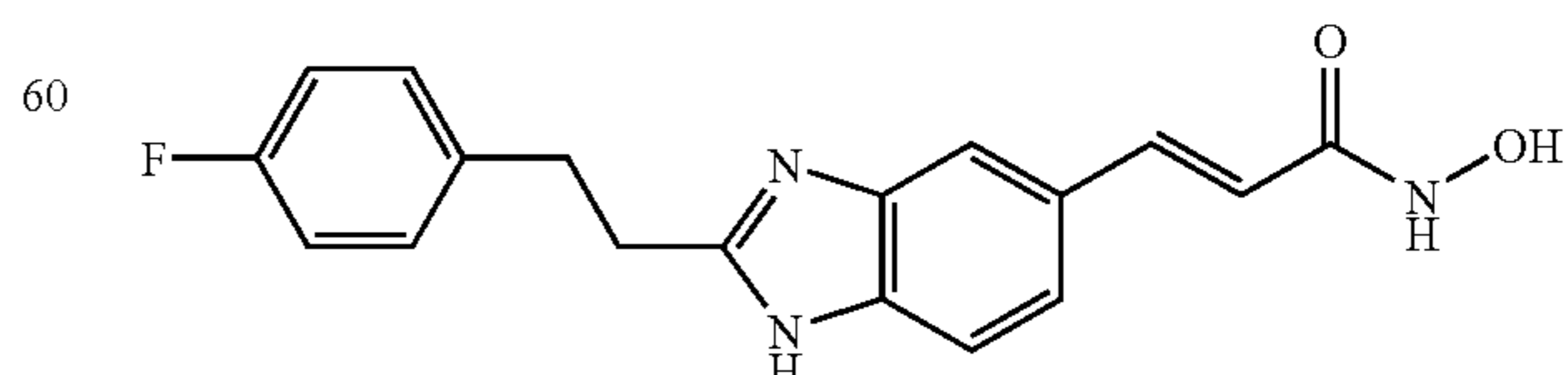
N-Hydroxy-3-{2-(4-fluoro-phenyl)-ethyl}-1H-benzimidazol-5-yl}-acrylamide
