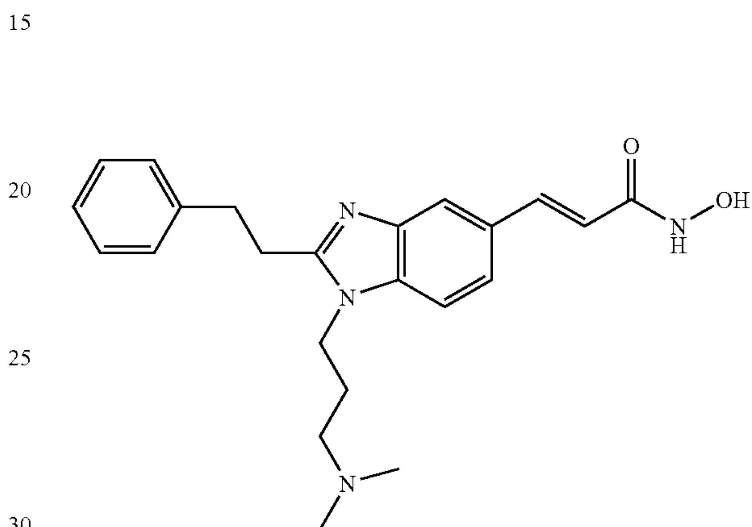
N-Hydroxy-3-[1-(3-dimethylamino-propyl)-2-phenethyl-1H-benzimidazol-5-yl]-acrylamide
