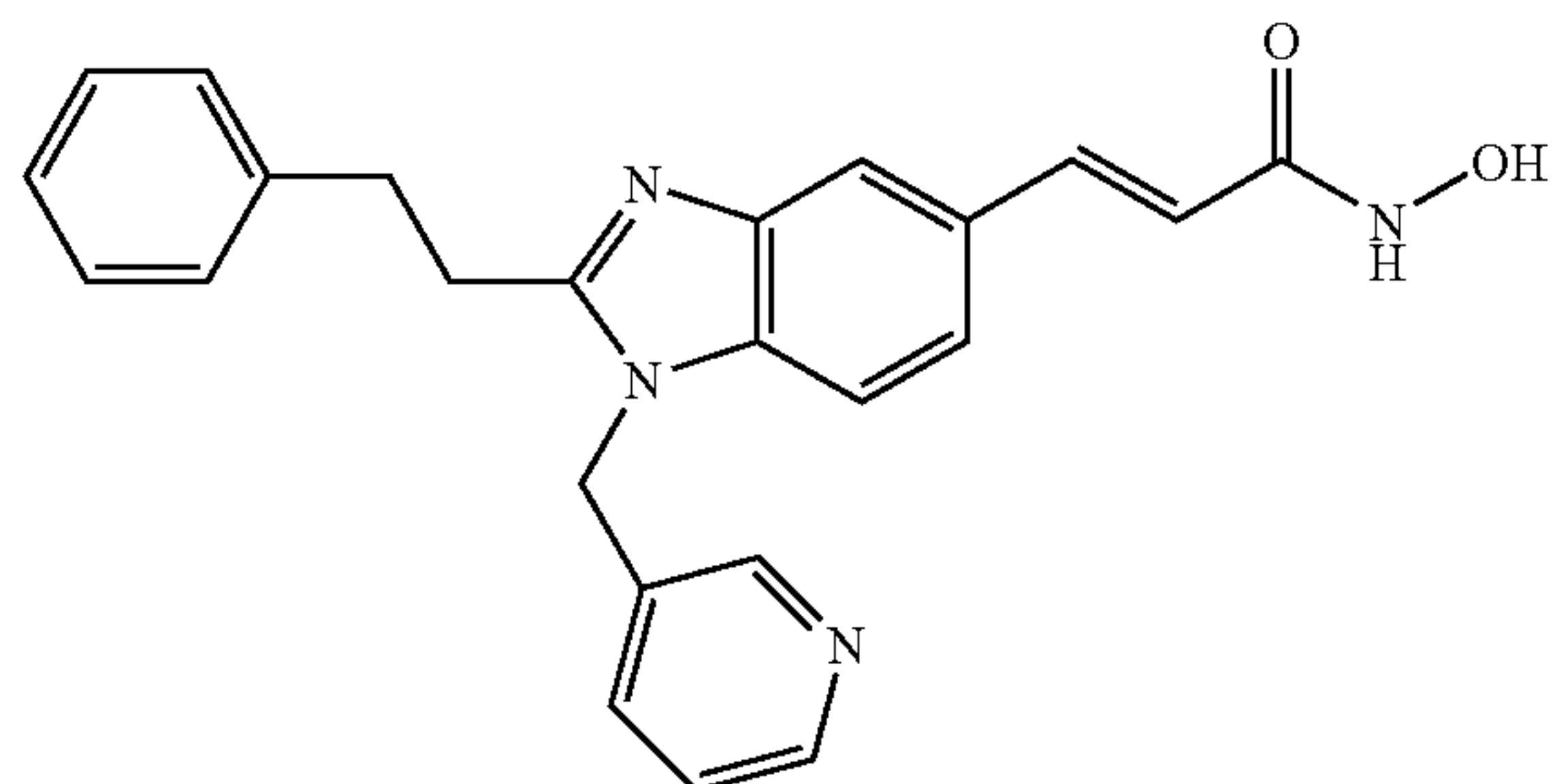
N-Hydroxy-3-[1-(3-pyridylmethyl)-2-(2-phenyl-ethyl)-1H-benzimidazole-5-yl]-acrylamide
