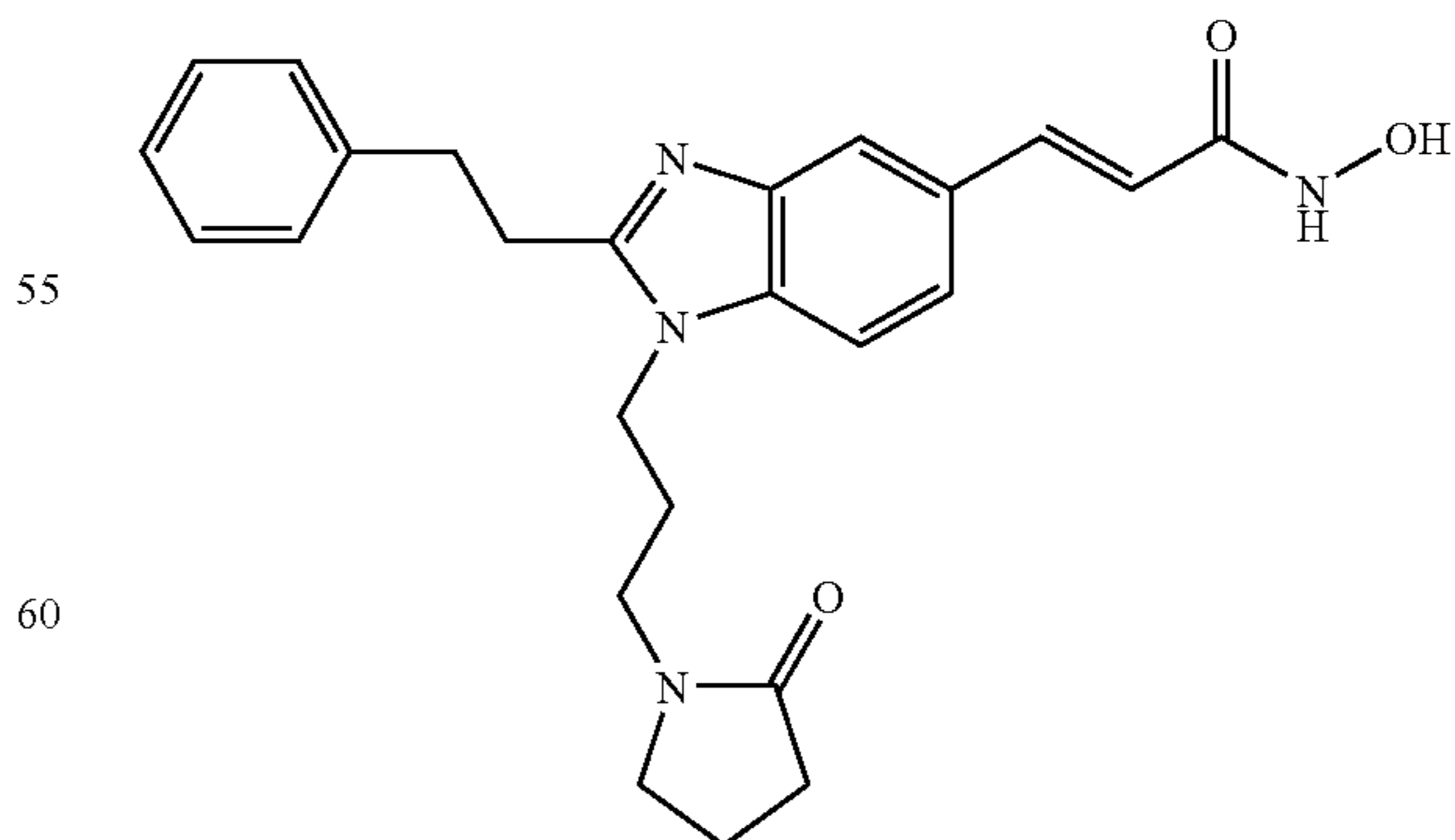
N-Hydroxy-3-{1-[3-(2-oxo-pyrrolidin-1-yl)-propyl]-2-phenethyl-1H-benzimidazol-5-yl}-acrylamide
