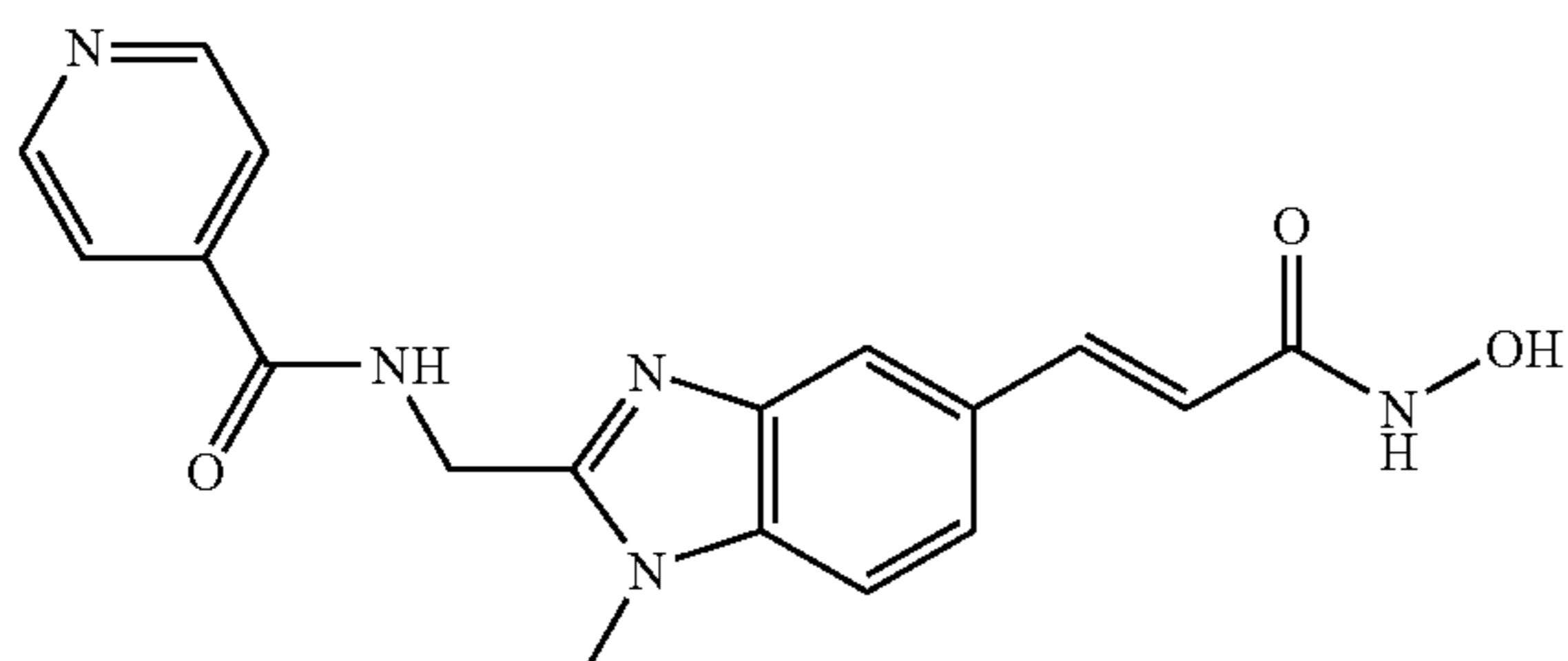
N-[5-(2-Hydroxycarbonyl-vinyl)-1-methyl-1H-benzimidazol-2-ylmethyl]-isonicotinamide
