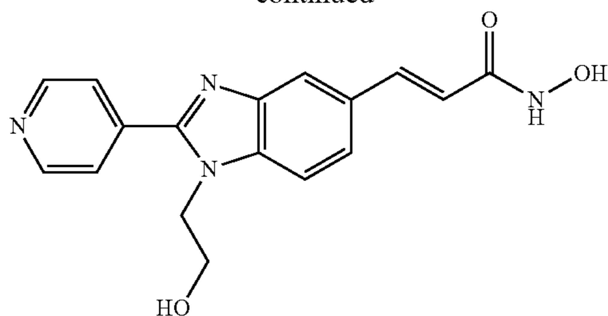
N-Hydroxy-3-[1-(2-hydroxy-ethyl)-2-(4-pyridyl)-1H-benzimidazol-5-yl]-acrylamide
