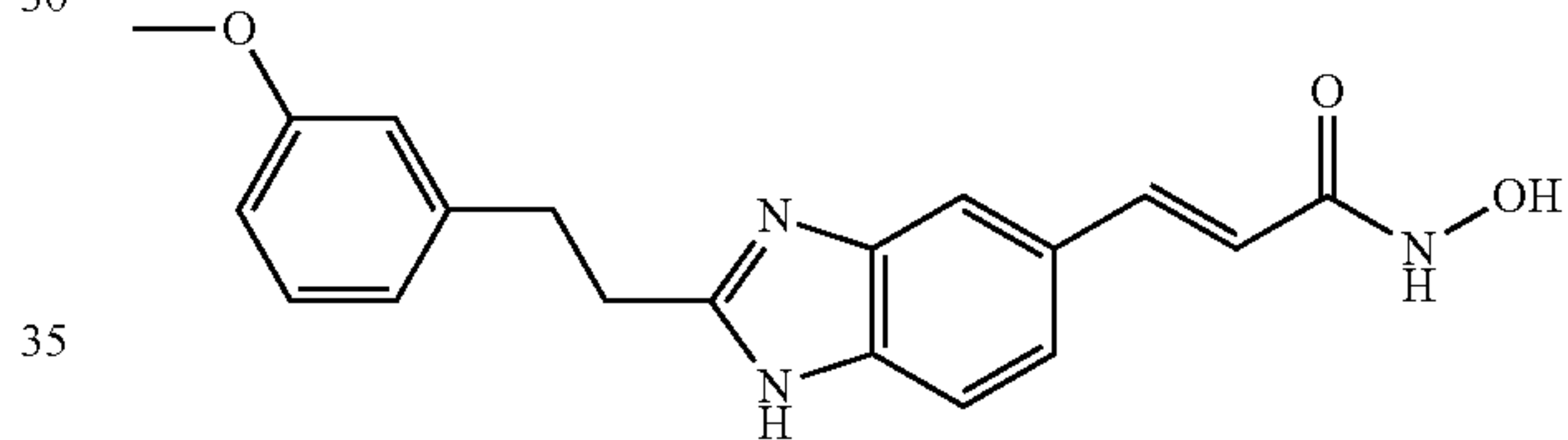
N-Hydroxy-3-[2-(3-methoxy-phenyl)-ethyl]-1H-benzimidazol-5-yl]-acrylamide
