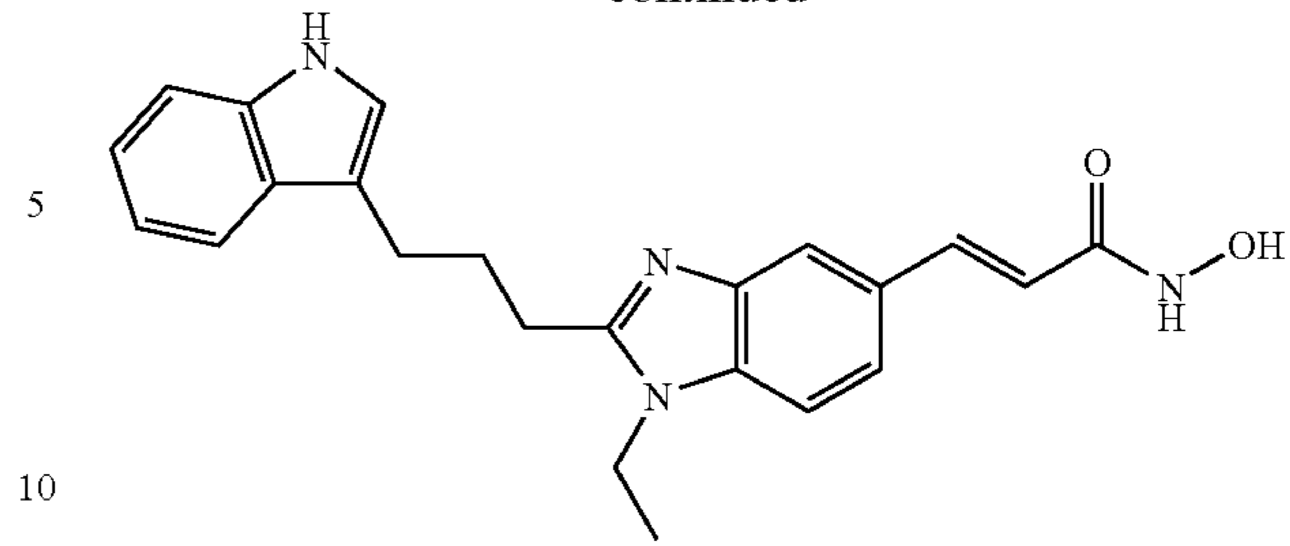
N-Hydroxy-3-[1-ethyl-2-[3-(1H-indol-3-yl)-propyl]-1H-benzimidazol-5-yl]-acrylamide
