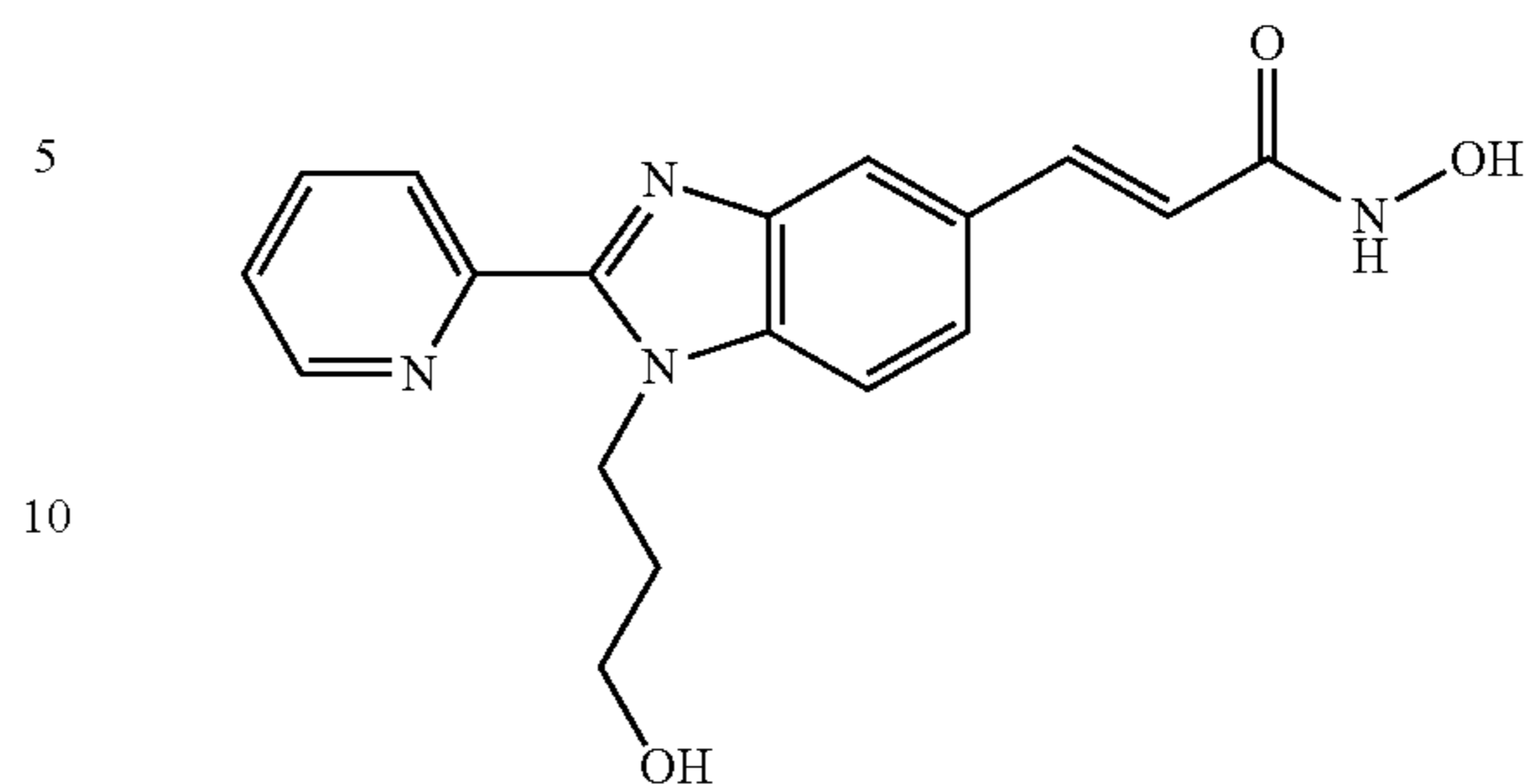
N-Hydroxy-3-[1-(3-hydroxy-propyl)-2-(2-pyridyl)-1H-benzimidazol-5-yl]-acrylamide;
