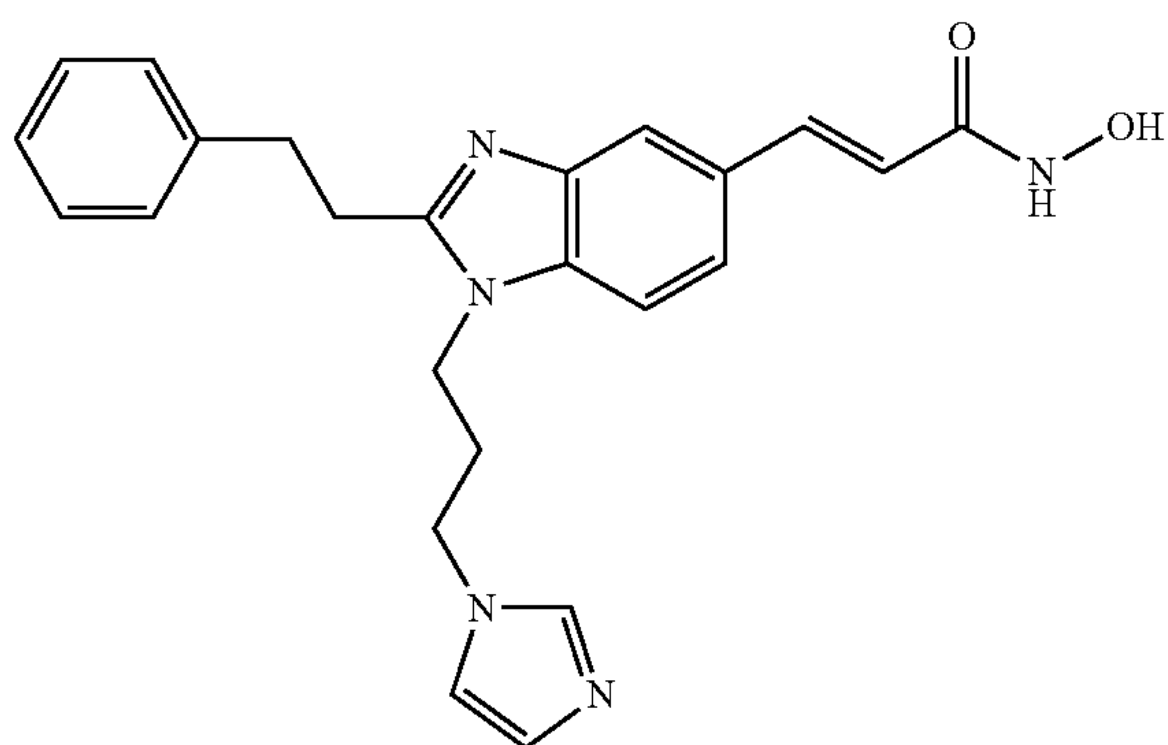
N-Hydroxy-3-[1-(3-imidazol-1-yl-propyl)-2-phenethyl-1H-benzimidazol-5-yl]-acrylamide
