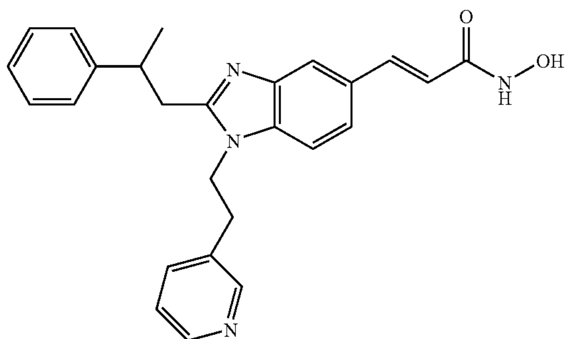
N-Hydroxy-3-[2-(2-phenyl-propyl)-1-(2-pyridin-3-yl-ethyl)-1H-benzimidazol-5-yl]-acrylamide
