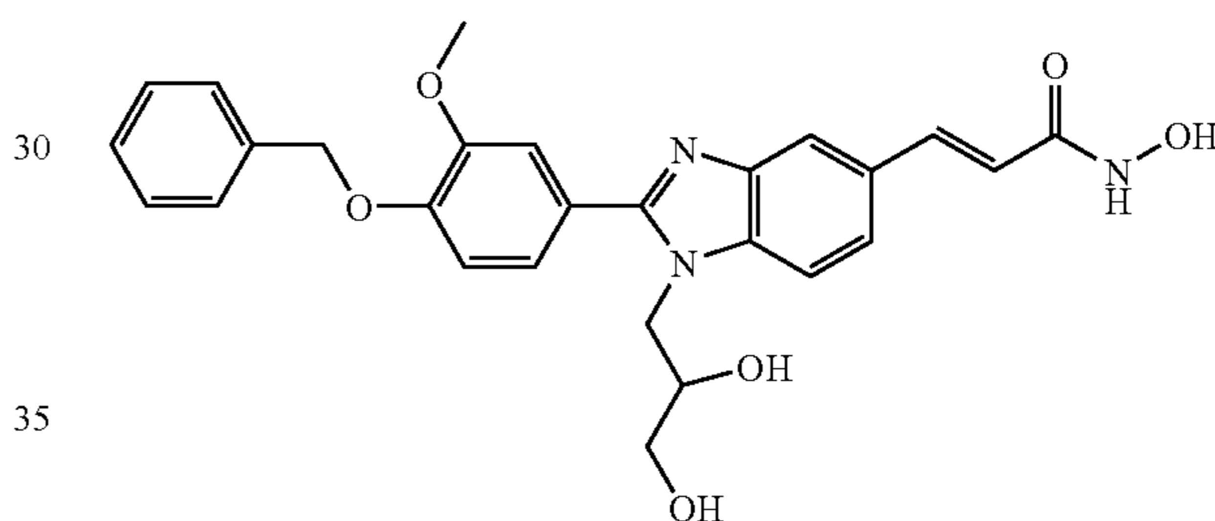
N-Hydroxy-3-[2-(4-benzyloxy-3-methoxy-phenyl)-1-(2,3-hydroxy-propyl)-1H-benzimidazole-5-yl]-acrylamide
