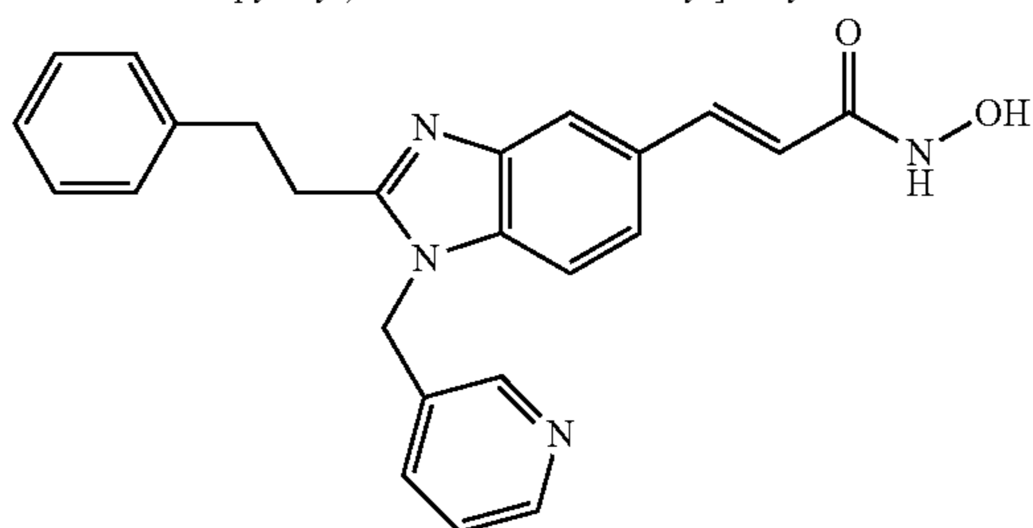
N-Hydroxy-3-[1-(3-pyridylmethyl)-2-(2-phenylethyl)-1H-benzimidazol-5-yl]-acrylamide
