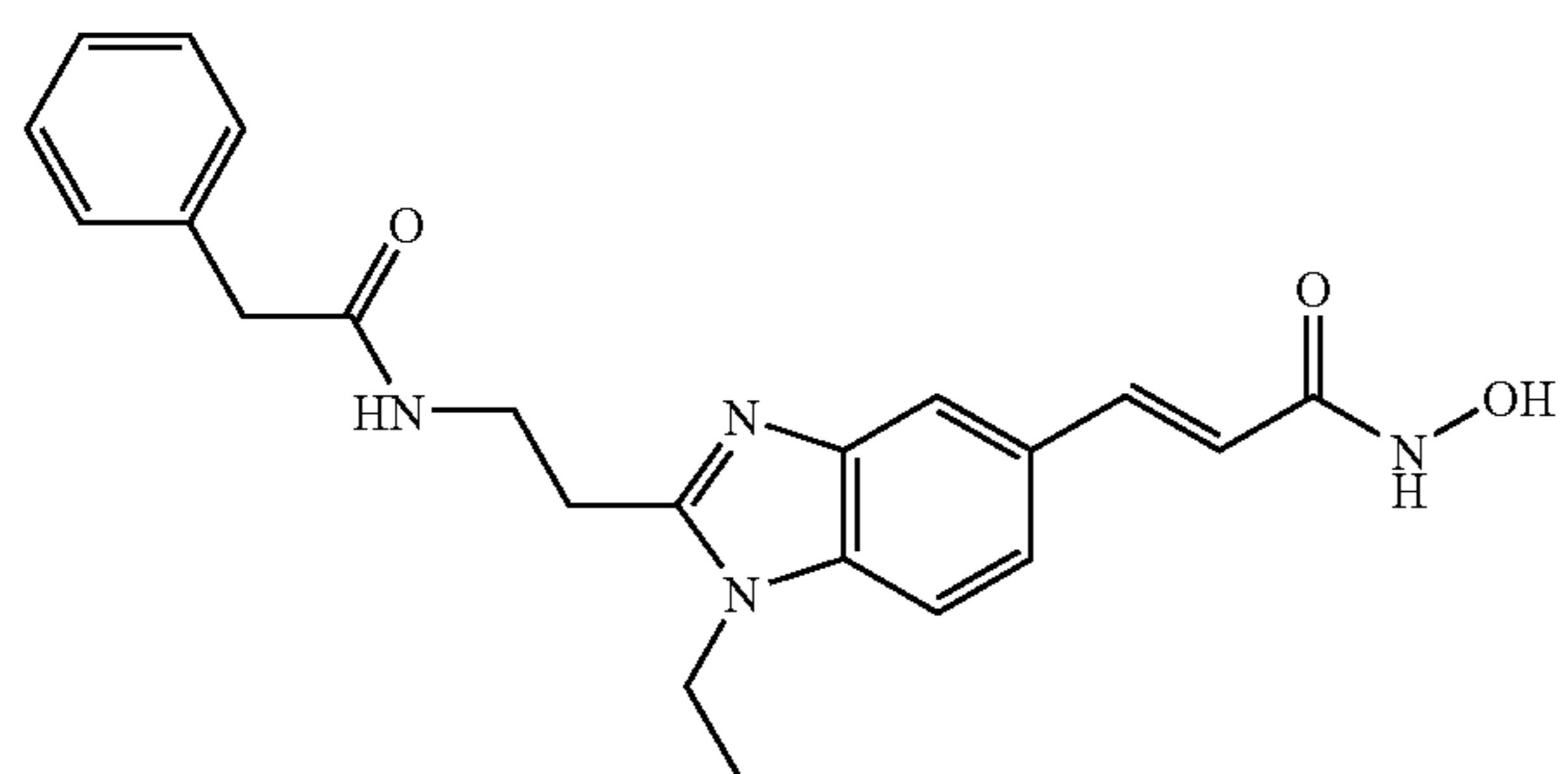
N-Hydroxy-3-[1-ethyl-2-(2-phenylacetyl-amino-ethyl)-1H-benzimidazol-5-yl]-acrylamide
