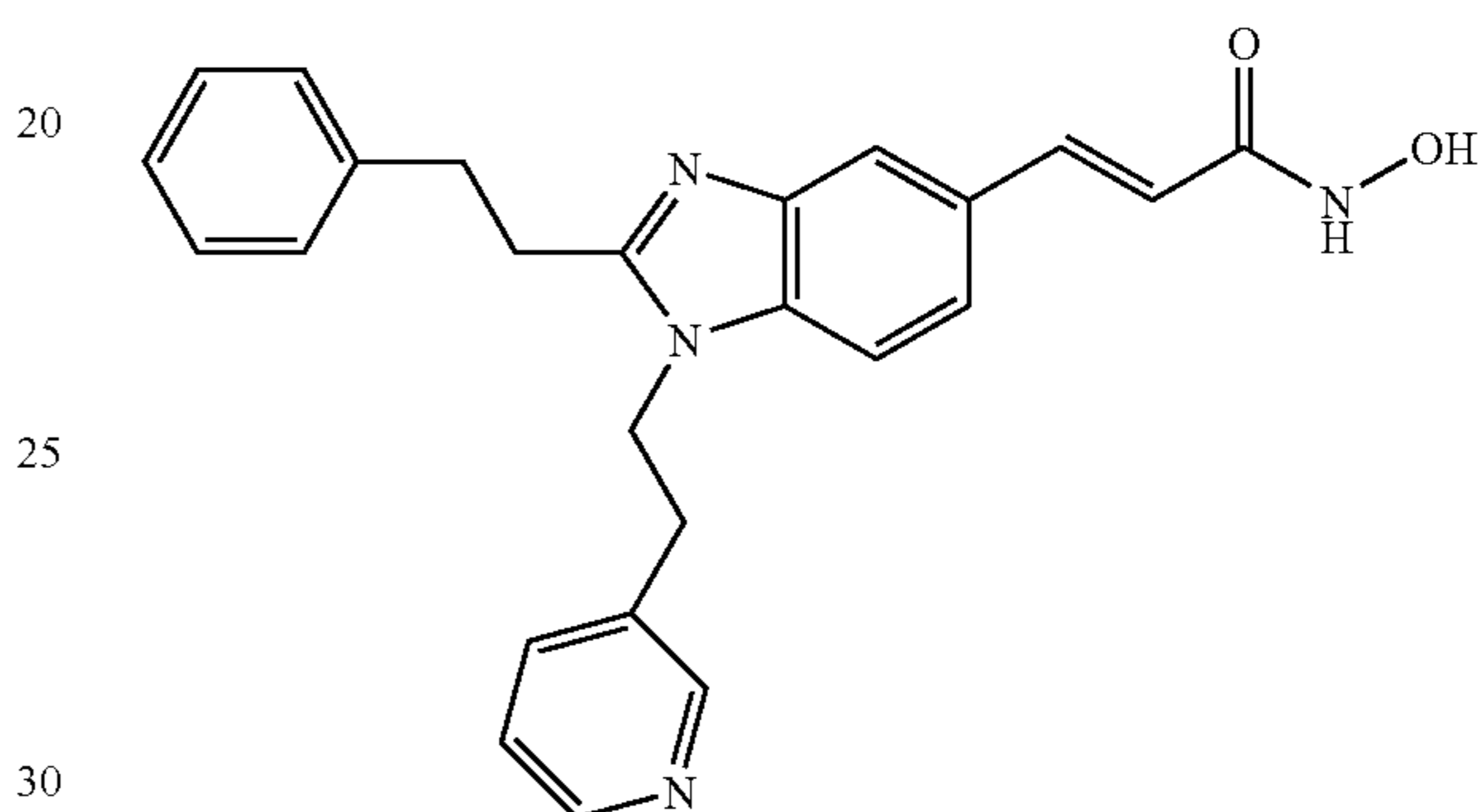
N-Hydroxy-3-(2-phenethyl-1-(2-pyridin-3-yl-ethyl)-1H-benzimidazol-5-yl)-acrylamide
