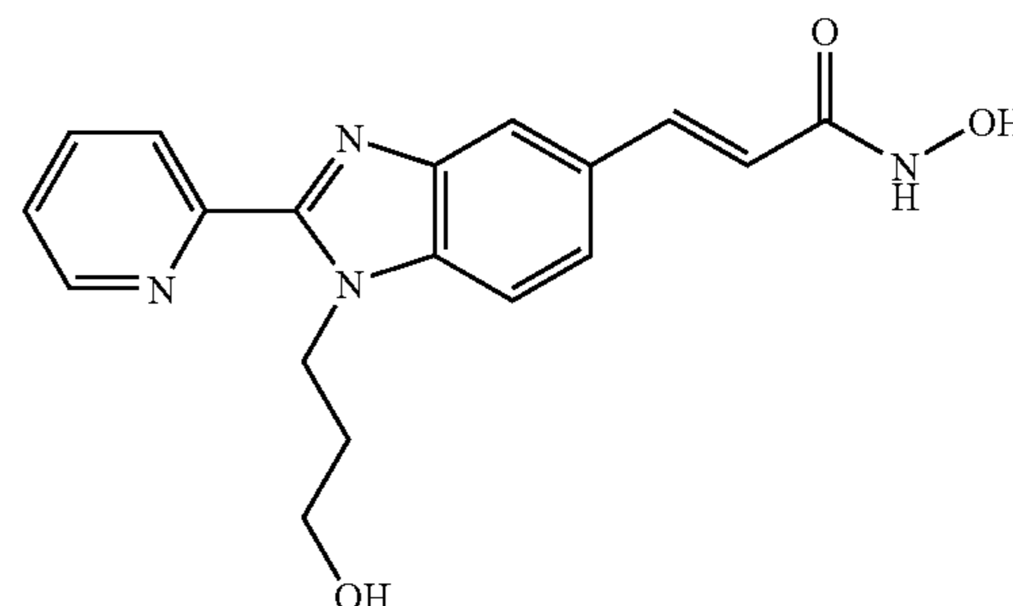
N-Hydroxy-3-[1-(3-hydroxy-propyl)-2-(2-pyridyl)-1H-benzimidazole-5-yl]-acrylamide
