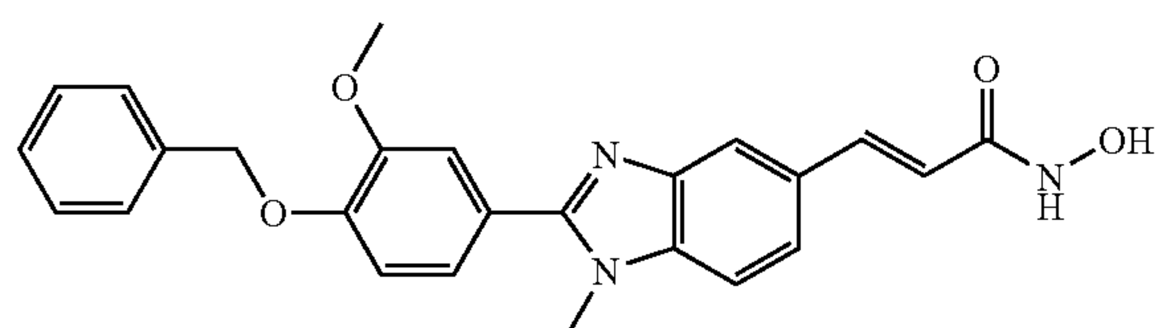
N-Hydroxy-3-[2-(4-benzyloxy-3-methoxy-phenyl)-1-methyl-1H-benzimidazol-5-yl]-acrylamide
