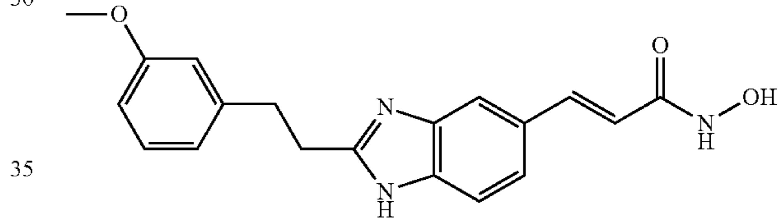
N-Hydroxy-3-[2-(3-methoxy-phenyl)-ethyl]-1H-benzimidazol-5-yl]-acrylamide
