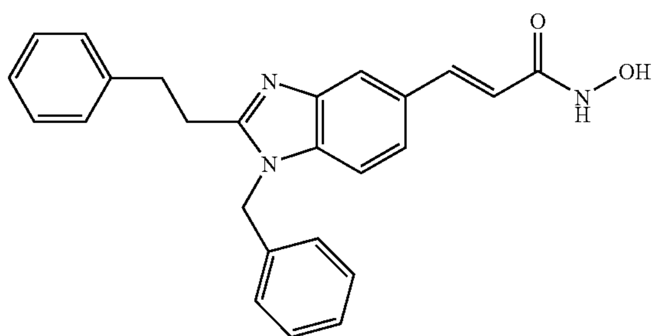
N-Hydroxy-3-(1-Benzyl-2-phenethyl-1H-benzimidazol-5-yl)-acrylamide
