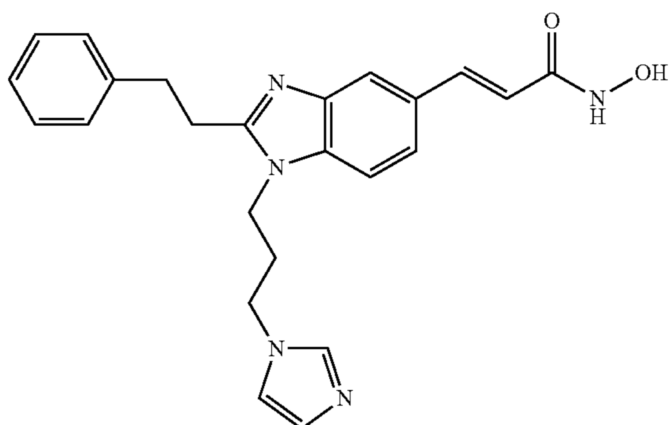
N-Hydroxy-3-[1-(3-imidazol-1-yl-propyl)-2-phenethyl-1H-benzimidazol-5-yl]-acrylamide
