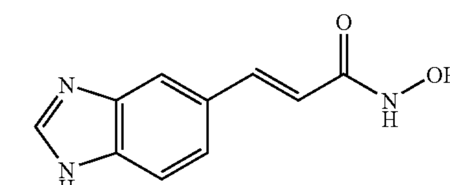
N-Hydroxy-3-(1H-benzimidazol-5-yl)-acrylamide
