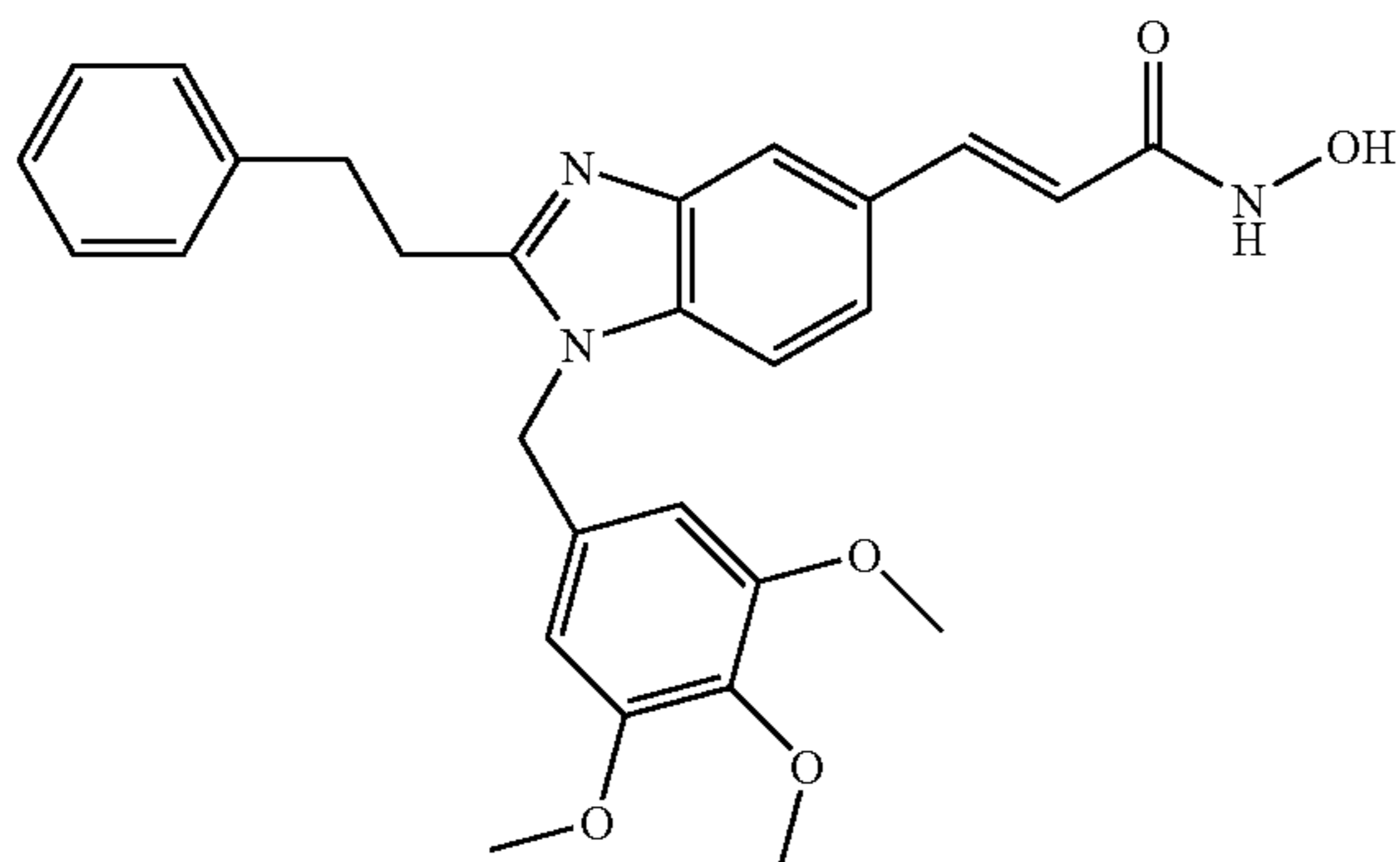
N-Hydroxy-3-[1-(3,4,5-trimethoxybenzyl)-2-(2-phenyl-ethyl)-1H-benzimidazol-5-yl]-acrylamide
