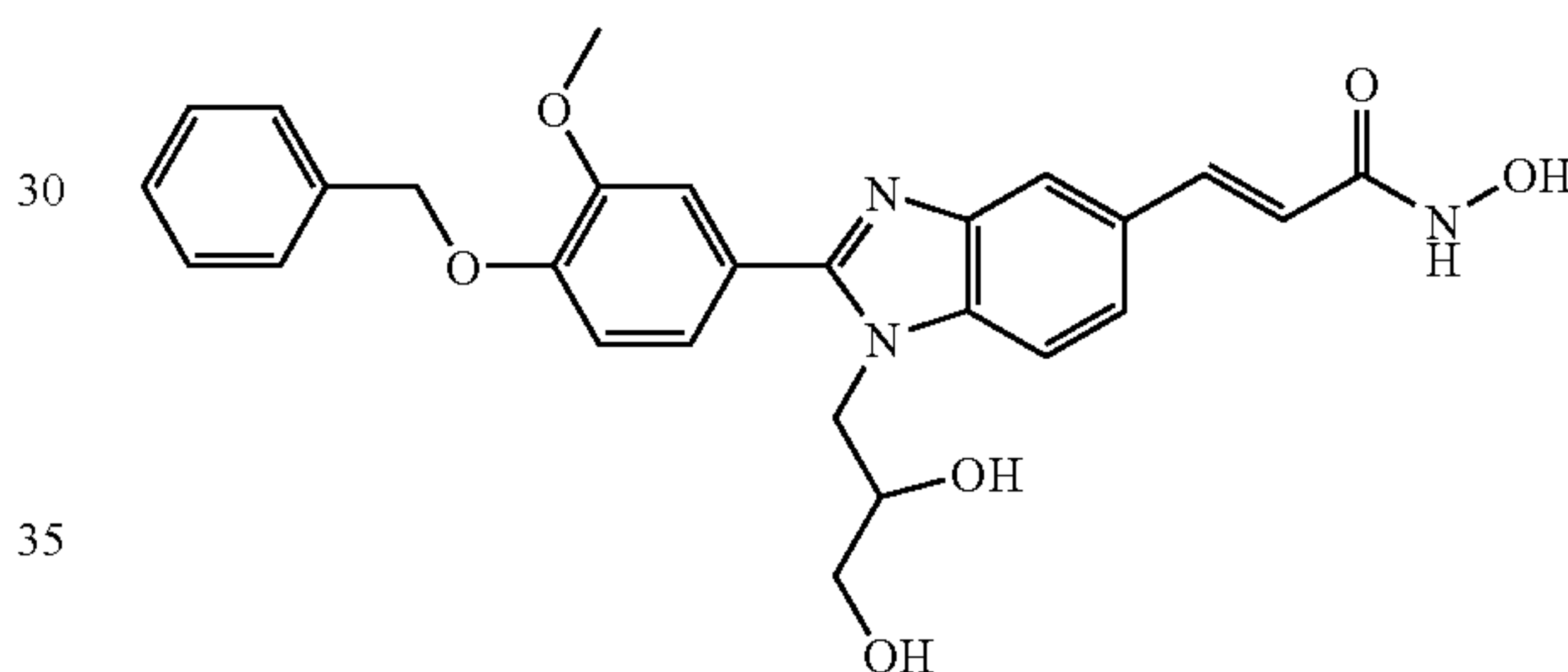
N-Hydroxy-3-[2-(4-benzyloxy-3-methoxy-phenyl)-1-(2,3-hydroxy-propyl)-1H-benzimidazole-5-yl]-acrylamide
