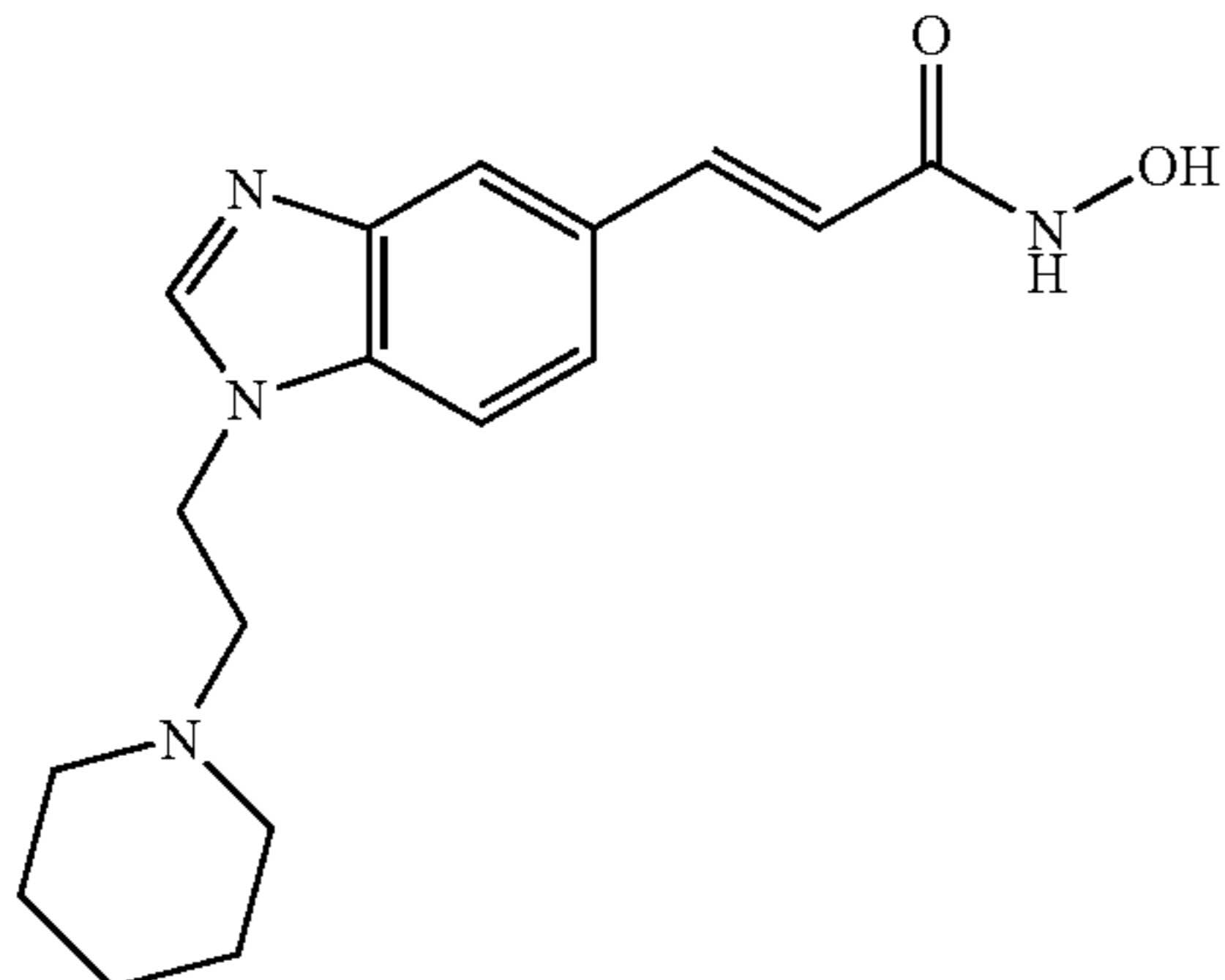
N-Hydroxy-3-[1-(2-piperidin-1-yl-ethyl)-1H-benzimidazol-5-yl]-acrylamide
