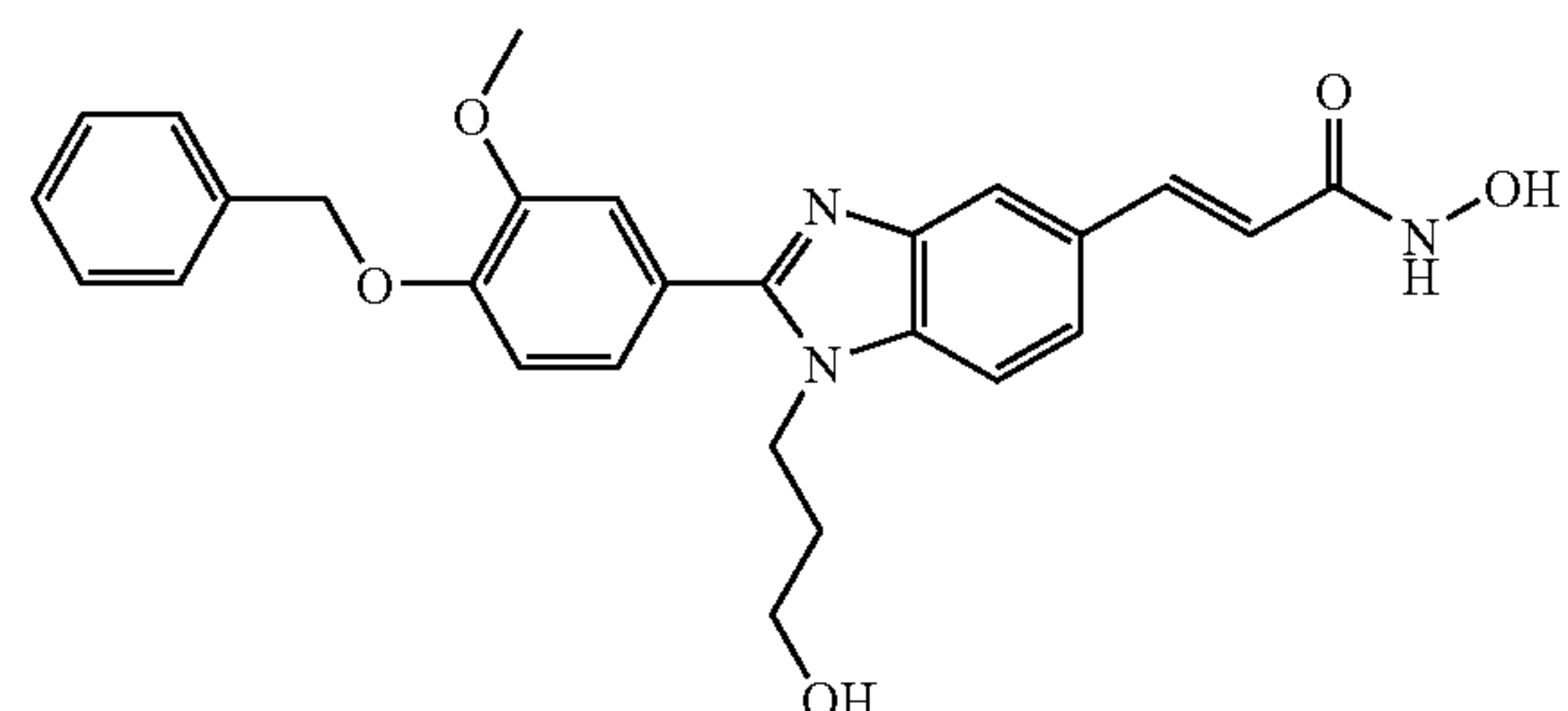
N-Hydroxy-3-[2-(4-benzyloxy-3-methoxy-phenyl)-1-(3-hydroxy-propyl)-1H-benzimidazole-5-yl]-acrylamide
