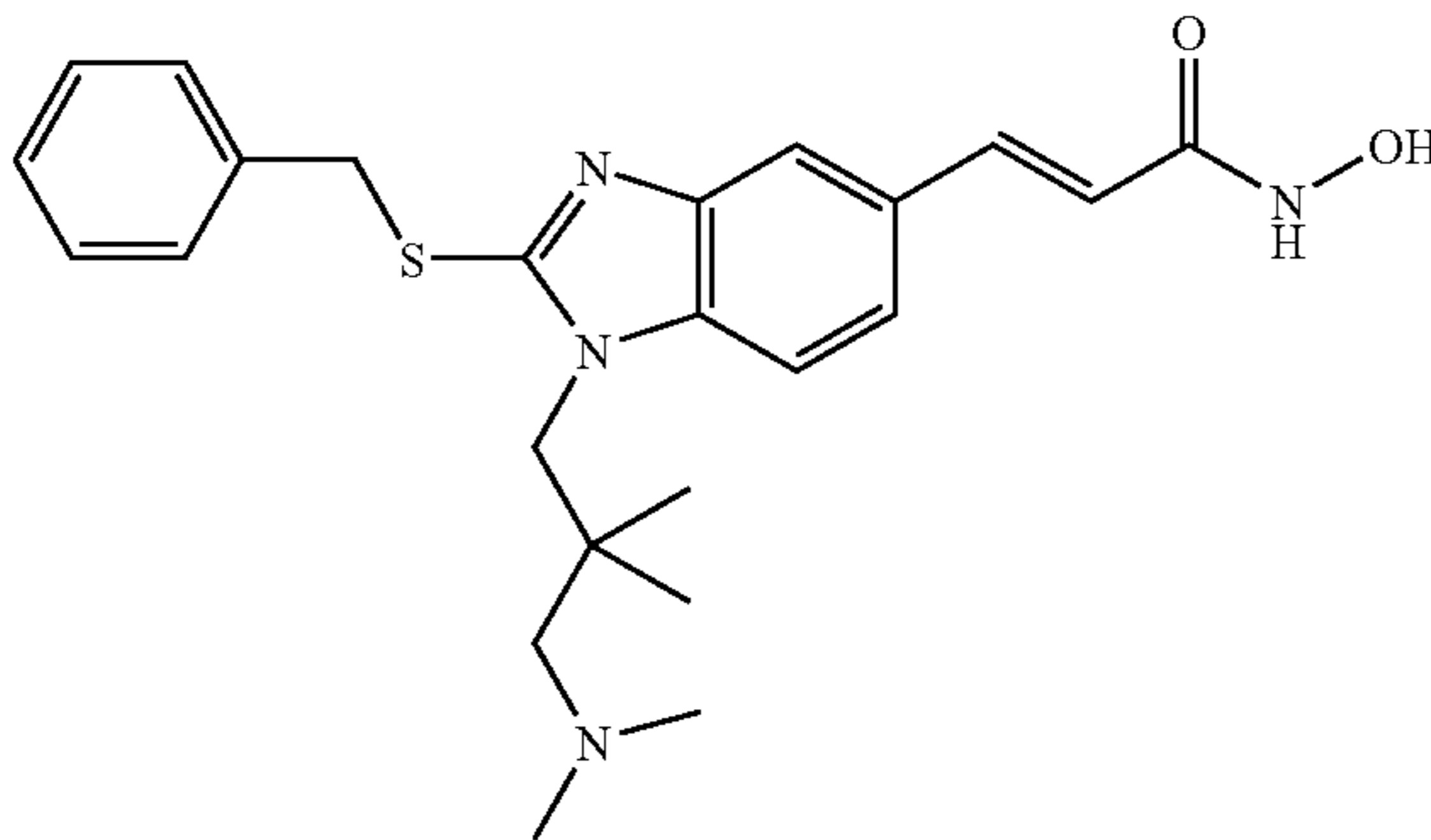
N-Hydroxy-3-[2-benzylsulfanyl-1-(3-dimethylamino-2,2-dimethyl-propyl)-1H-benzimidazol-5-yl]-acrylamide
