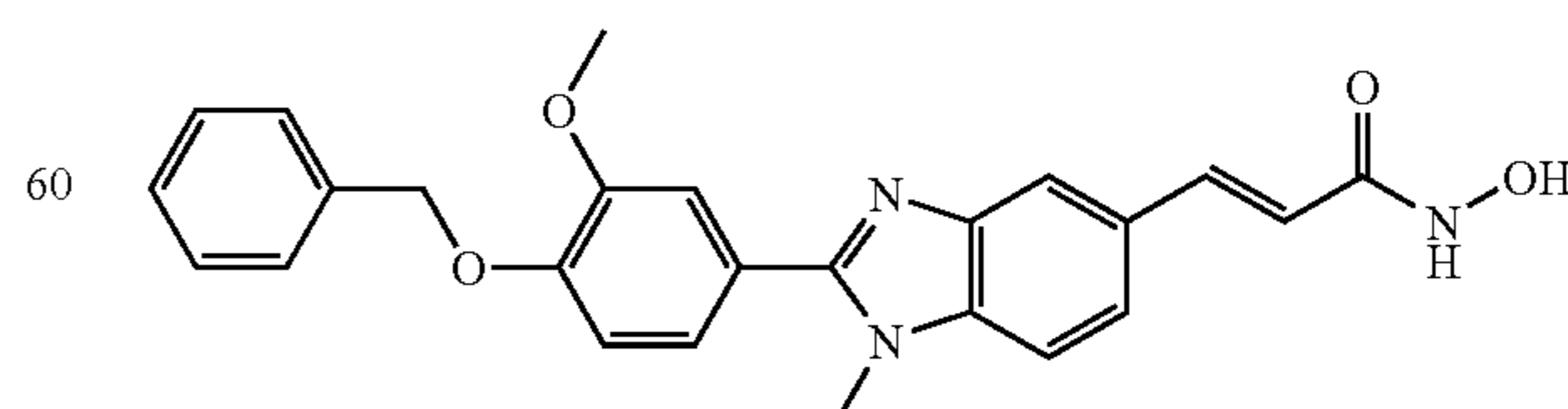
N-Hydroxy-3-[2-(4-benzyloxy-3-methoxy-phenyl)-1-methyl-1H-benzimidazole-5-yl]-acrylamide
