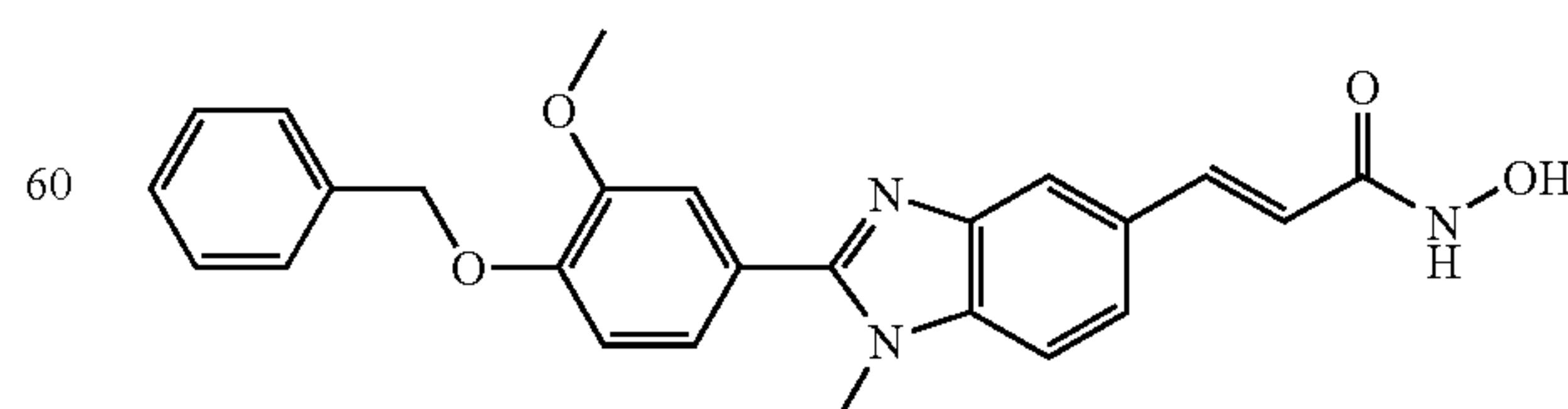
N-Hydroxy-3-[2-(4-benzyloxy-3-methoxy-phenyl)-1-methyl-1H-benzimidazole-5-yl]-acrylamide
