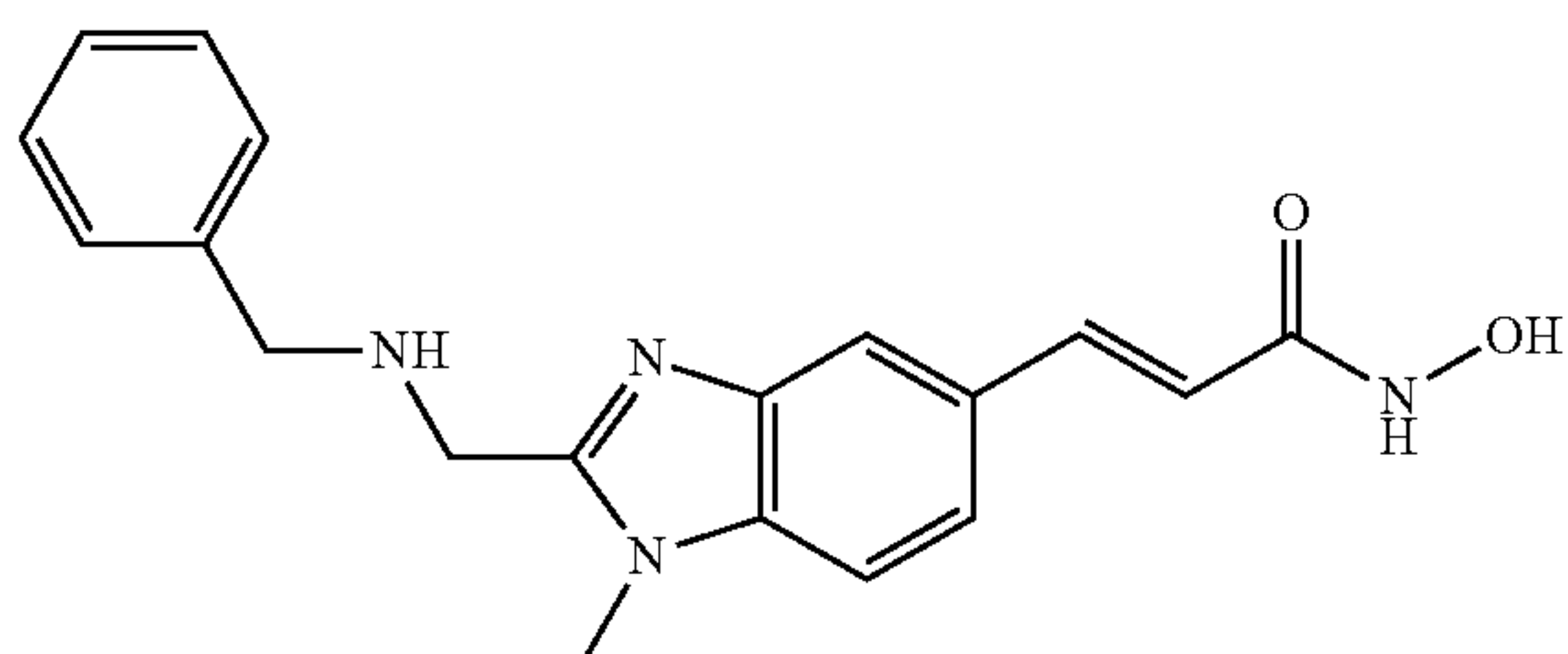
N-Hydroxy-3-[2-(benzylamino-methyl)-1-methyl-1H-benzimidazol-5-yl]-acrylamide
