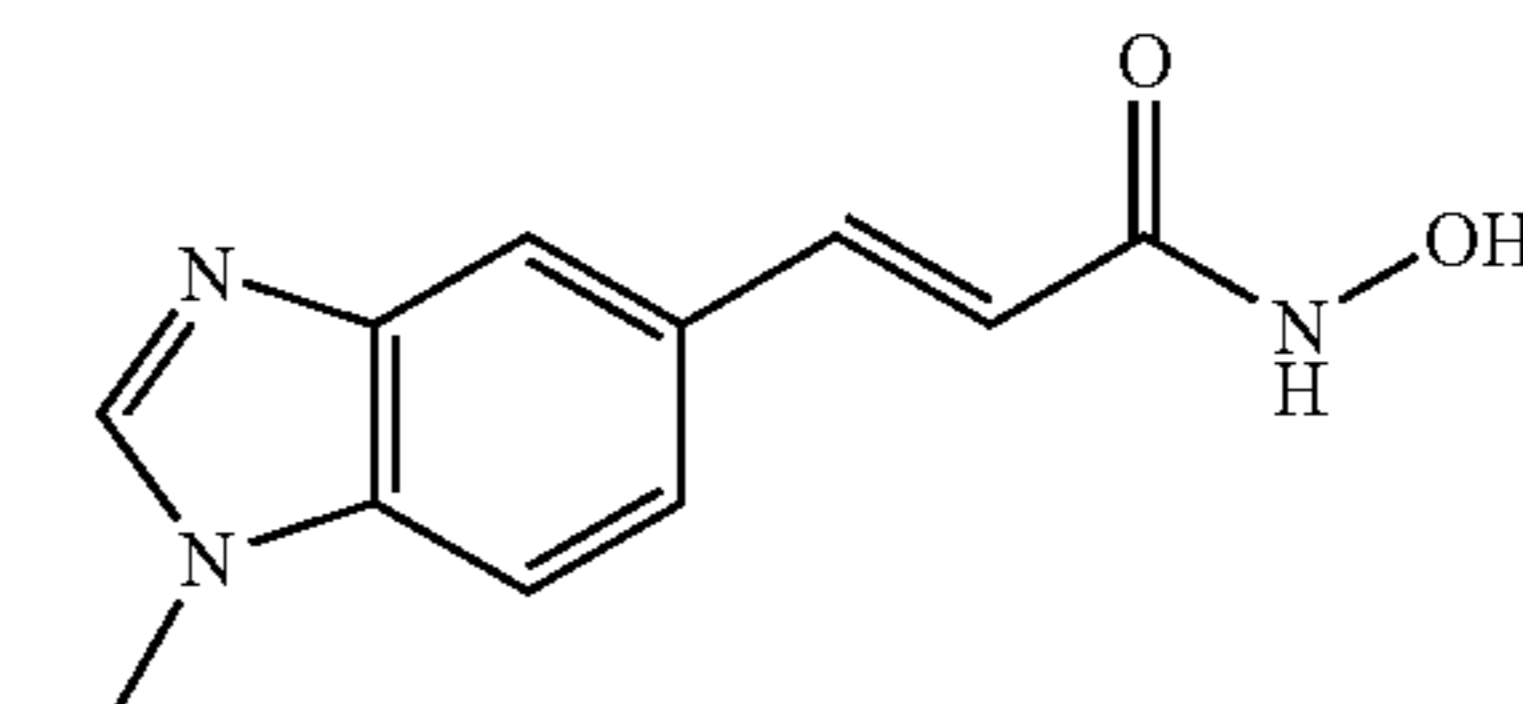
N-Hydroxy-3-(1-methyl-1H-benzimidazol-5-yl)-acrylamide
