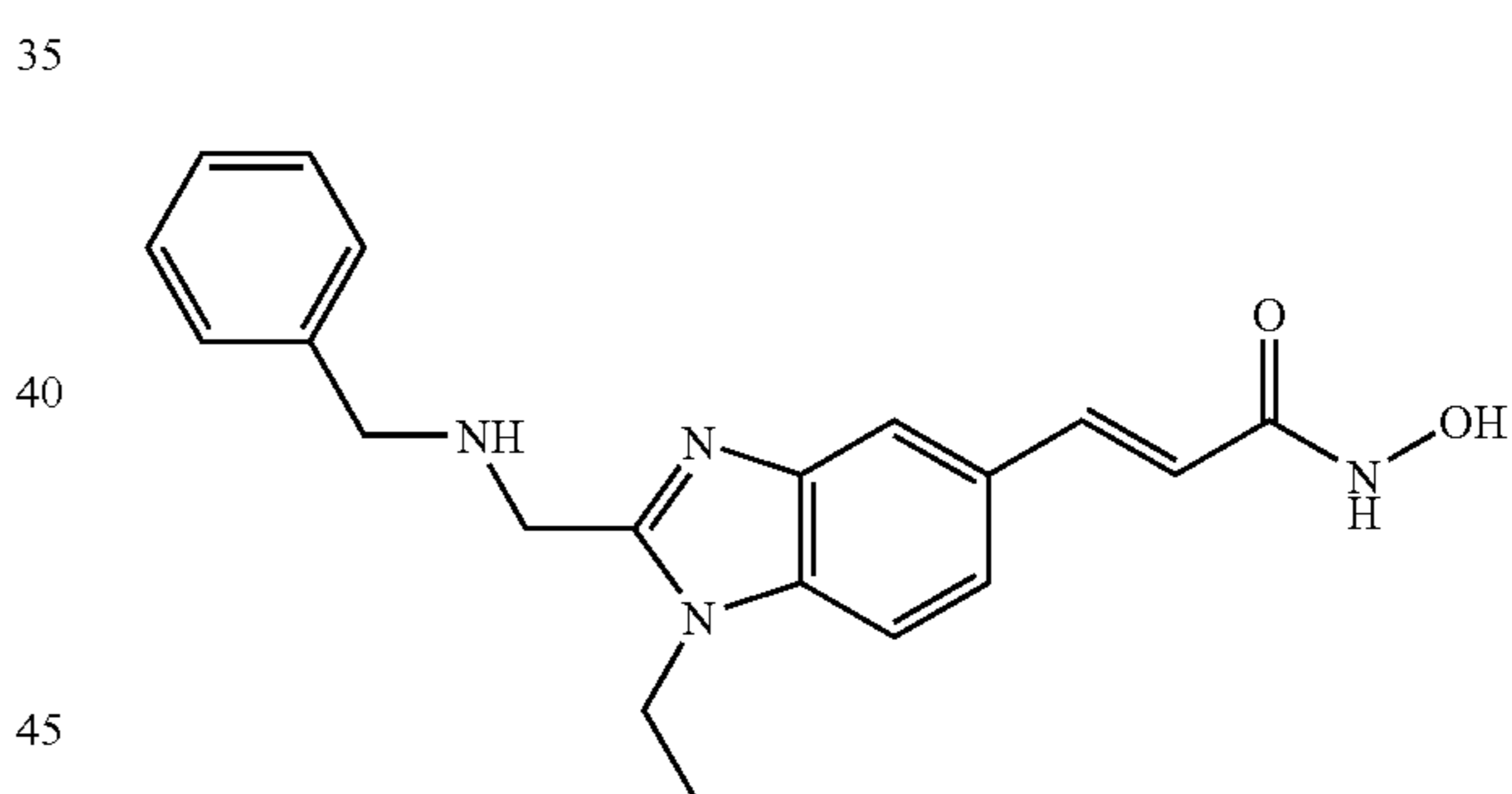
N-Hydroxy-3-[2-(benzylamino-methyl)-ethyl-1H-benzimidazol-5-yl]-acrylamide
