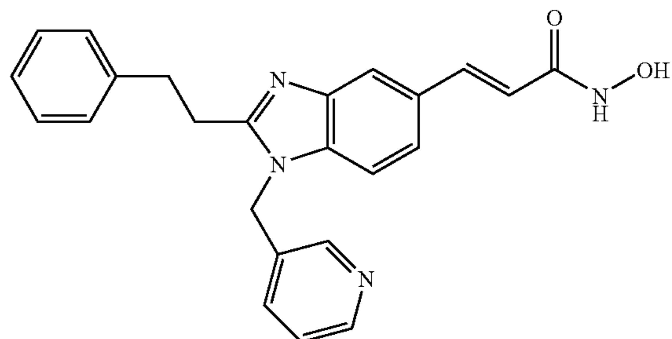
N-Hydroxy-3-[1-(3-pyridylmethyl)-2-(2-phenyl-ethyl)-1H-benzimidazole-5-yl]-acrylamide
