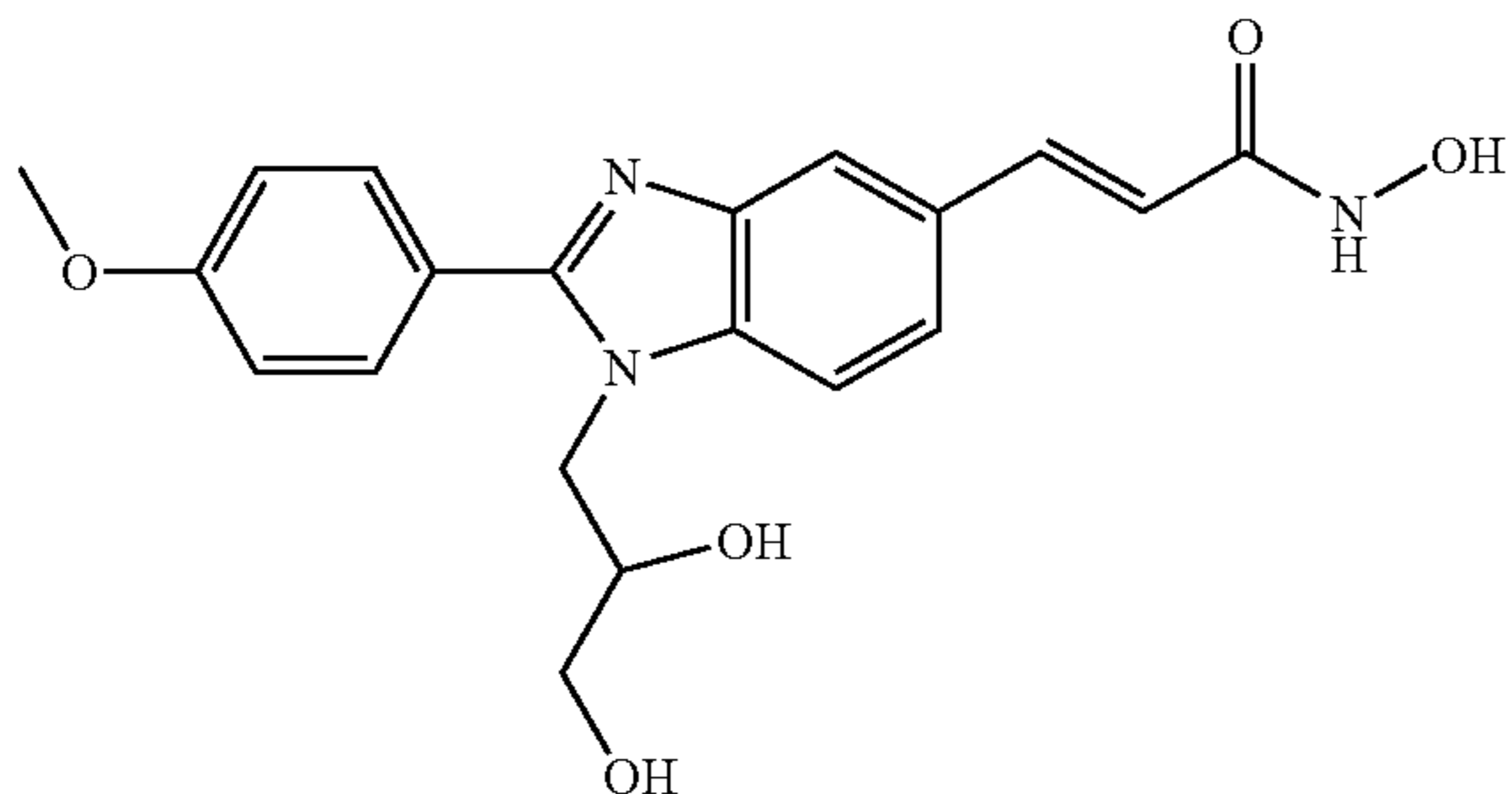
N-Hydroxy-3-[1-(2,3-hydroxy-propyl)-2-(4-methoxy-phenyl)-1H-benzimidazole-5-yl]-acrylamide
