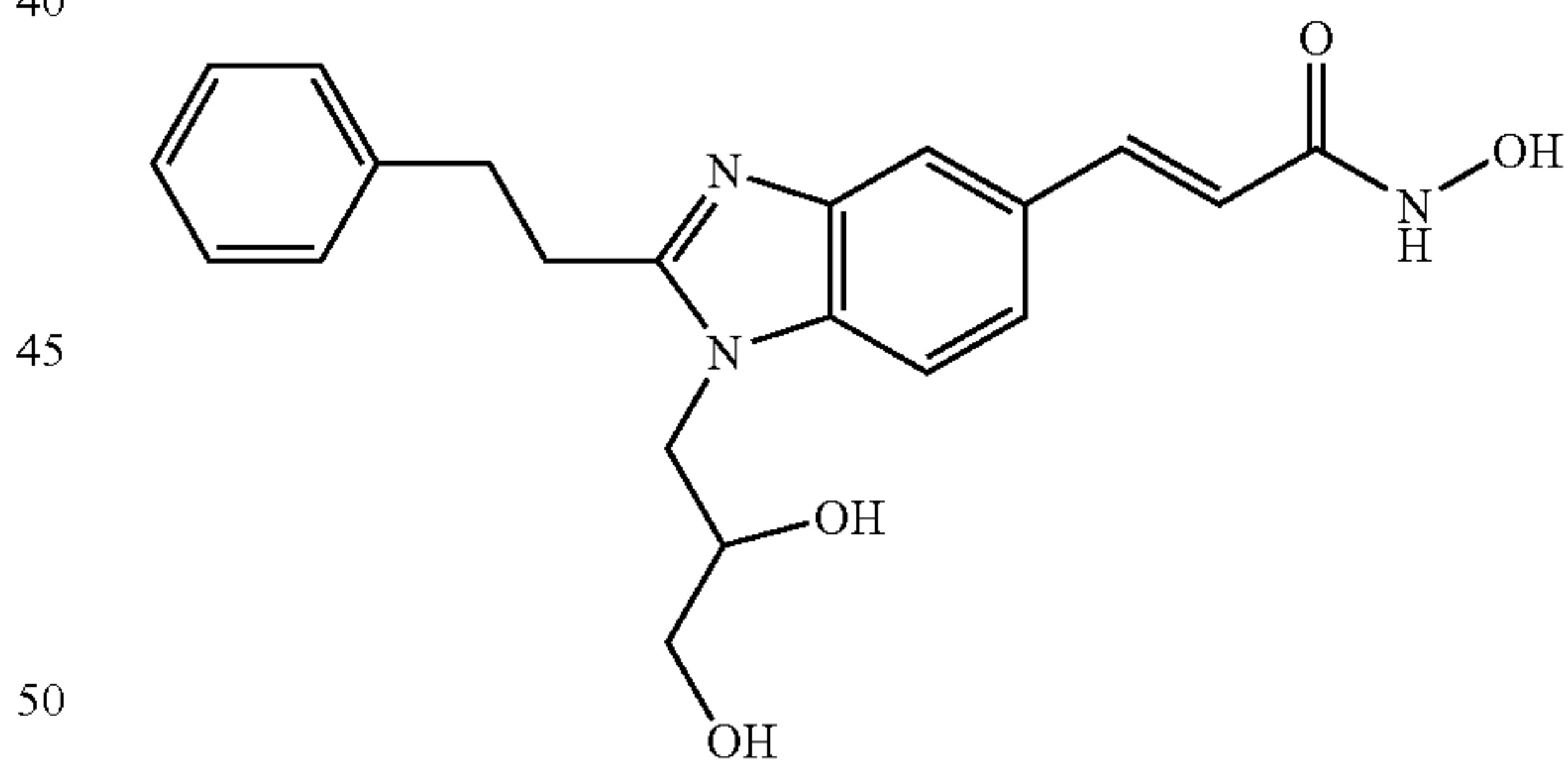
N-Hydroxy-3-[1-(2,3-hydroxy-propyl)-2-(2-phenyl-ethyl)-1H-benzimidazol-5-yl]-acrylamide
