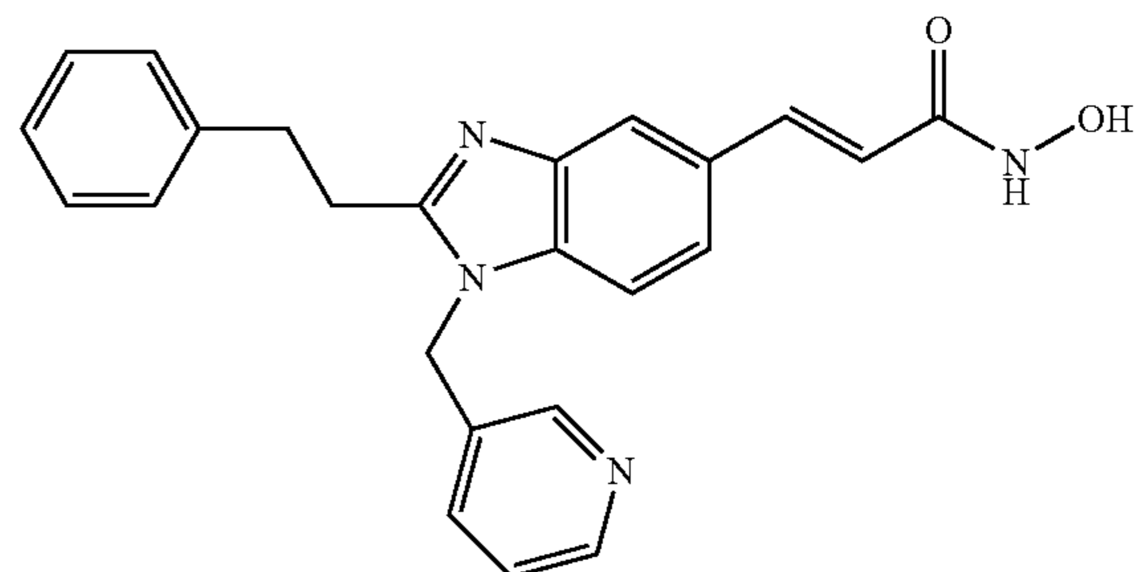
N-Hydroxy-3-[1-(3-pyridylmethyl)-2-(2-phenyl-ethyl)-1H-benzimidazole-5-yl]-acrylamide
