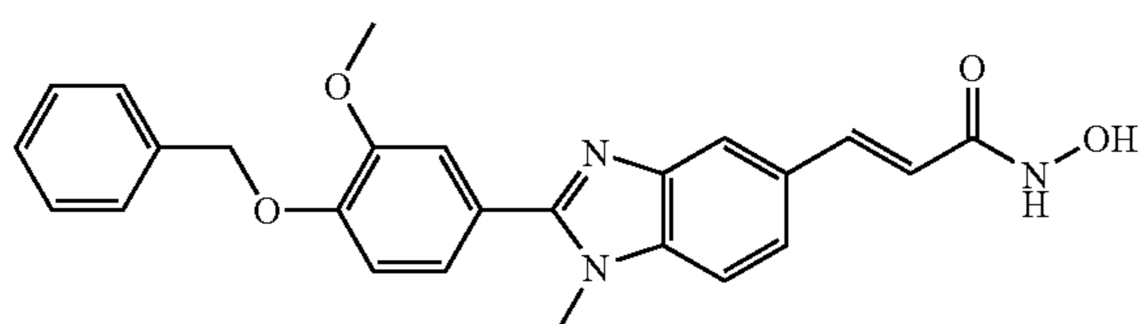
N-Hydroxy-3-[2-(4-benzyloxy-3-methoxy-phenyl)-1-methyl-1H-benzimidazol-5-yl]-acrylamide
