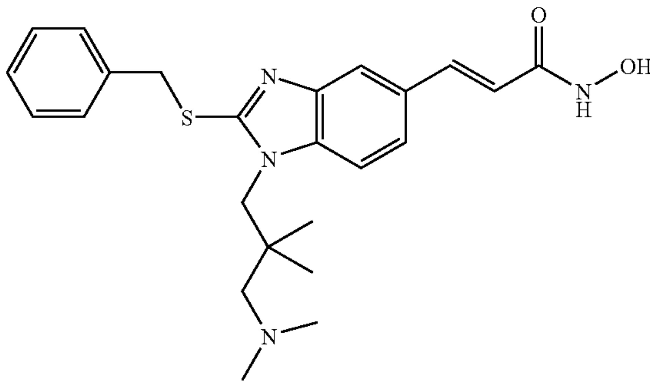
N-Hydroxy-3-[2-benzylsulfanyl-1-(3-dimethylamino-2,2-dimethyl-propyl)-1H-benzimidazol-5-yl]-acrylamide
