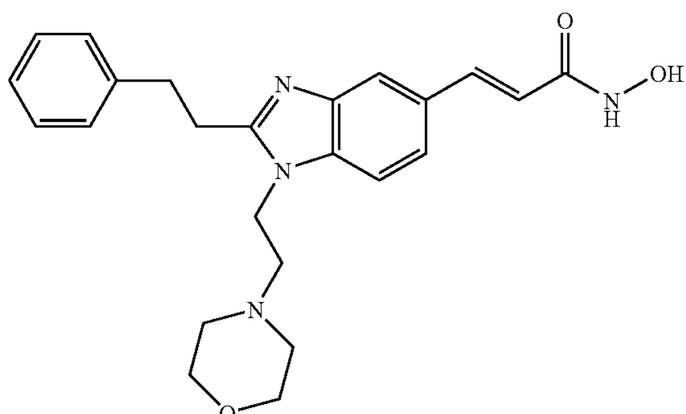
N-Hydroxy-3-[1-(2-morpholin-4-yl-ethyl)-2-phenethyl-1H-benzimidazol-5-yl]-acrylamide
