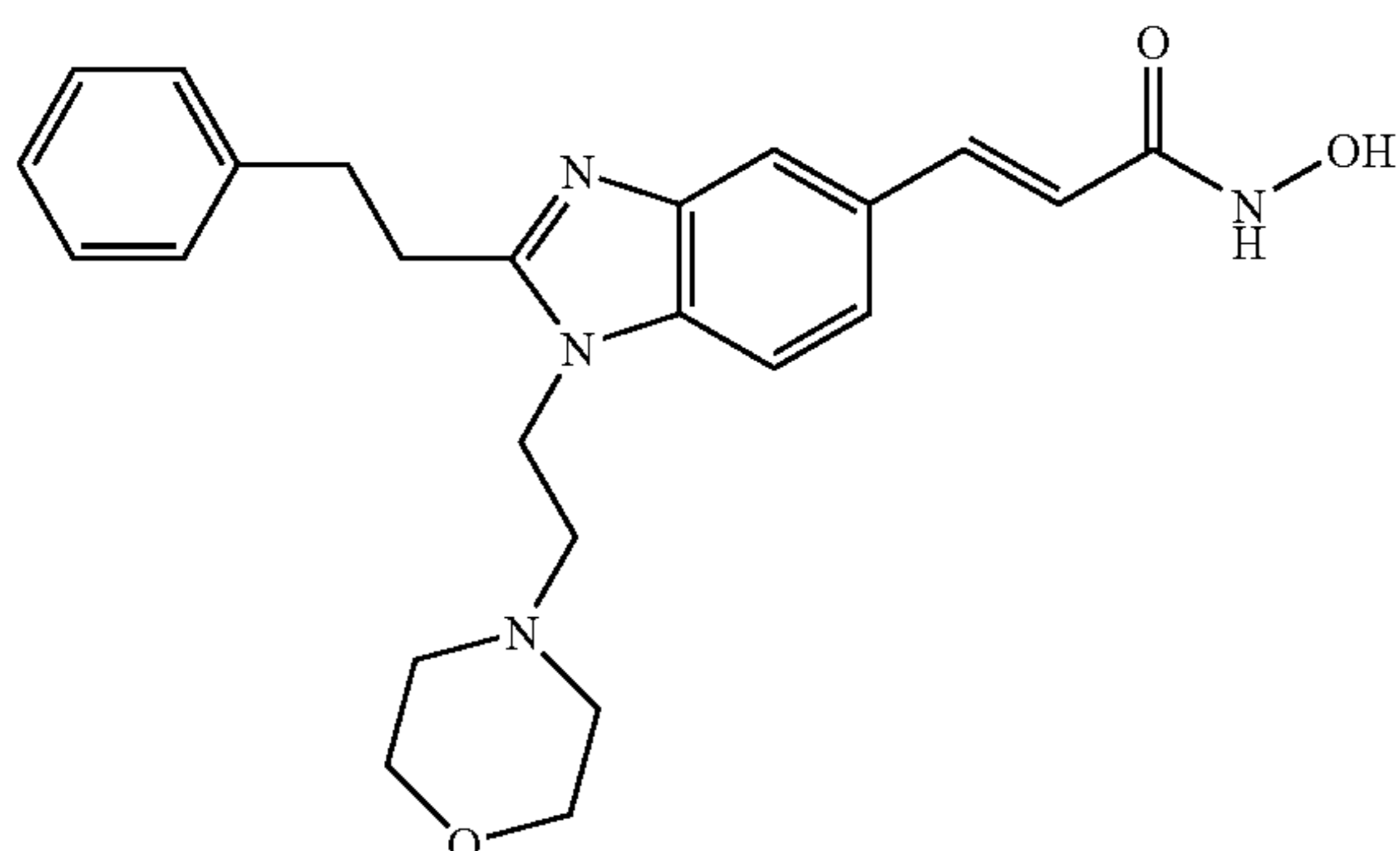
N-Hydroxy-3-[1-(2-morpholin-4-yl-ethyl)-2-phenethyl-1H-benzimidazol-5-yl]-acrylamide
