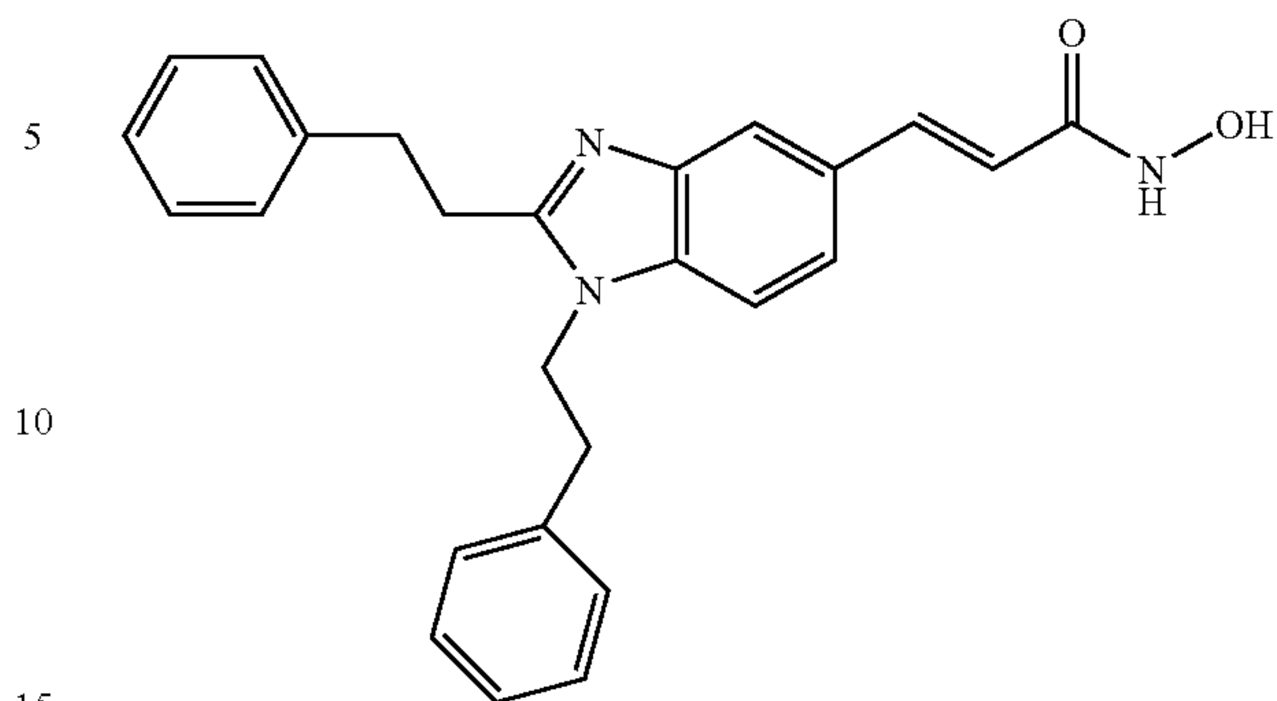
N-Hydroxy-3-(1,2-Diphenethyl-1H-benzimidazol-5-yl)-acrylamide
