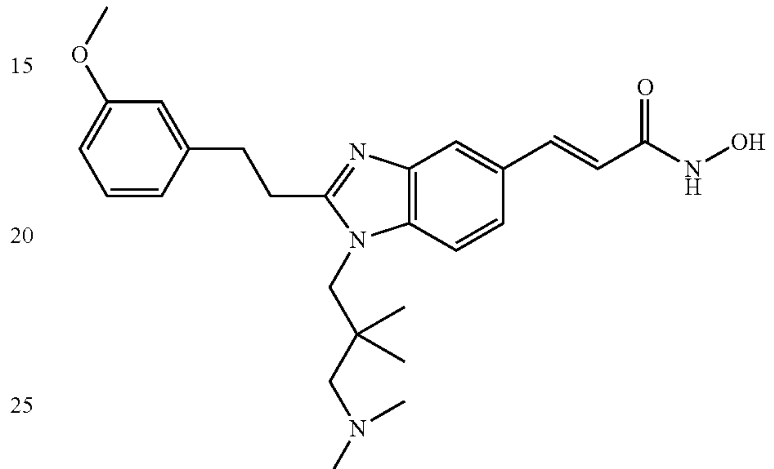
N-Hydroxy-3-[1-(3-dimethylamino-2,2-dimethyl-propyl)-2-[2-(3-methoxy-phenyl)-ethyl]-1H-benzimidazol-5-yl]-acrylamide
