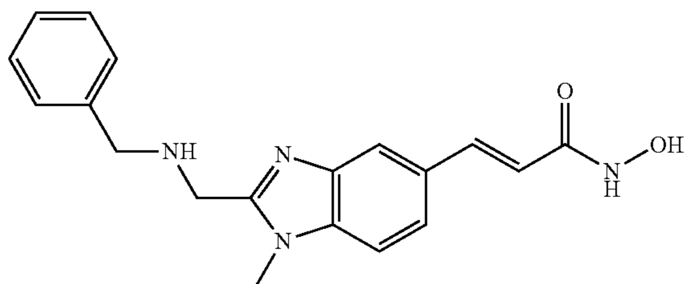
N-Hydroxy-3-[2-(benzylamino-methyl)-1-methyl-1H-benzimidazol-5-yl]-acrylamide
