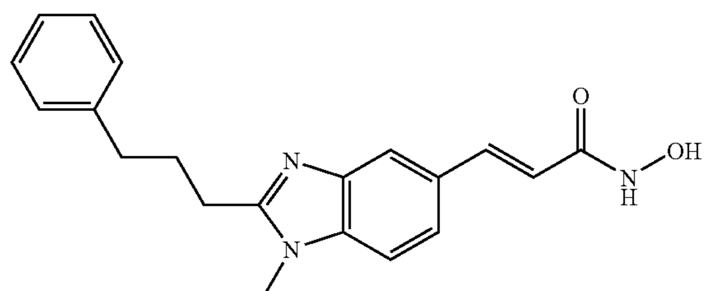
N-Hydroxy-3-[1-methyl-2-(3-phenyl-propyl)-1H-benzimidazol-5-yl]-acrylamide
