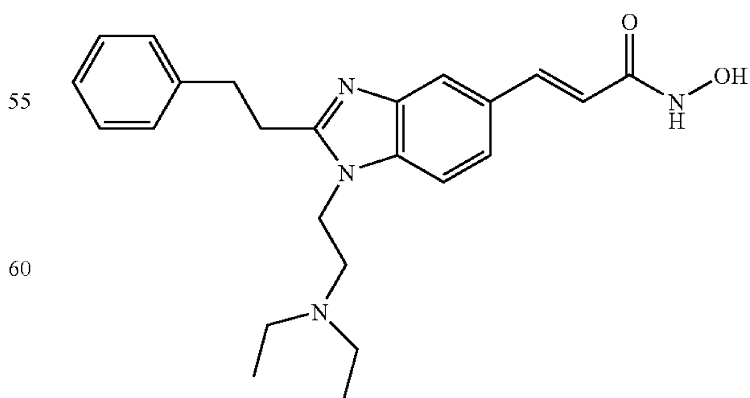
N-Hydroxy-3-[1-(2-diethylamino-ethyl)-2-phenethyl-1H-benzimidazol-5-yl]-acrylamide
