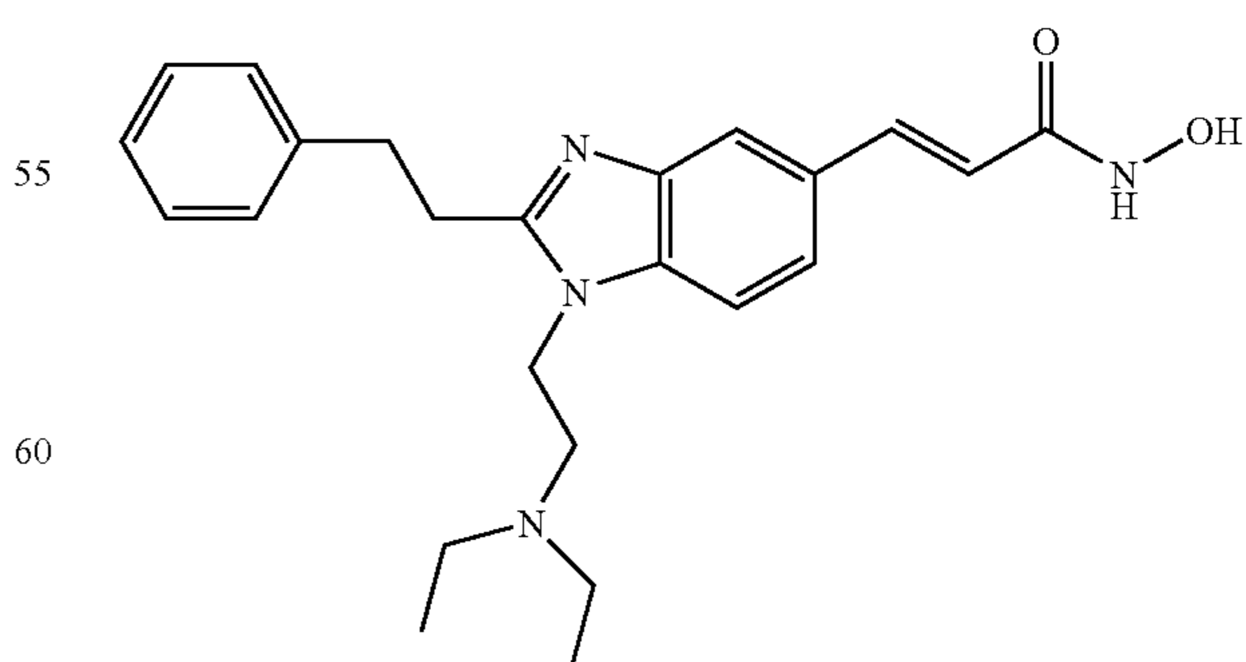
N-Hydroxy-3-[1-(2-diethylamino-ethyl)-2-phenethyl-1H-benzimidazol-5-yl]-acrylamide
