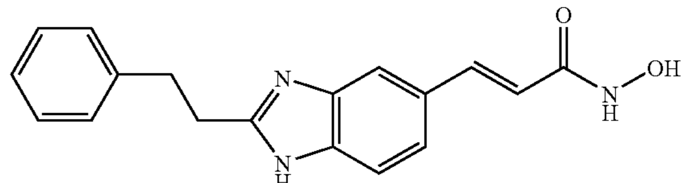
N-Hydroxy-3-(2-phenethyl-1H-benzimidazol-5-yl)-acrylamide
