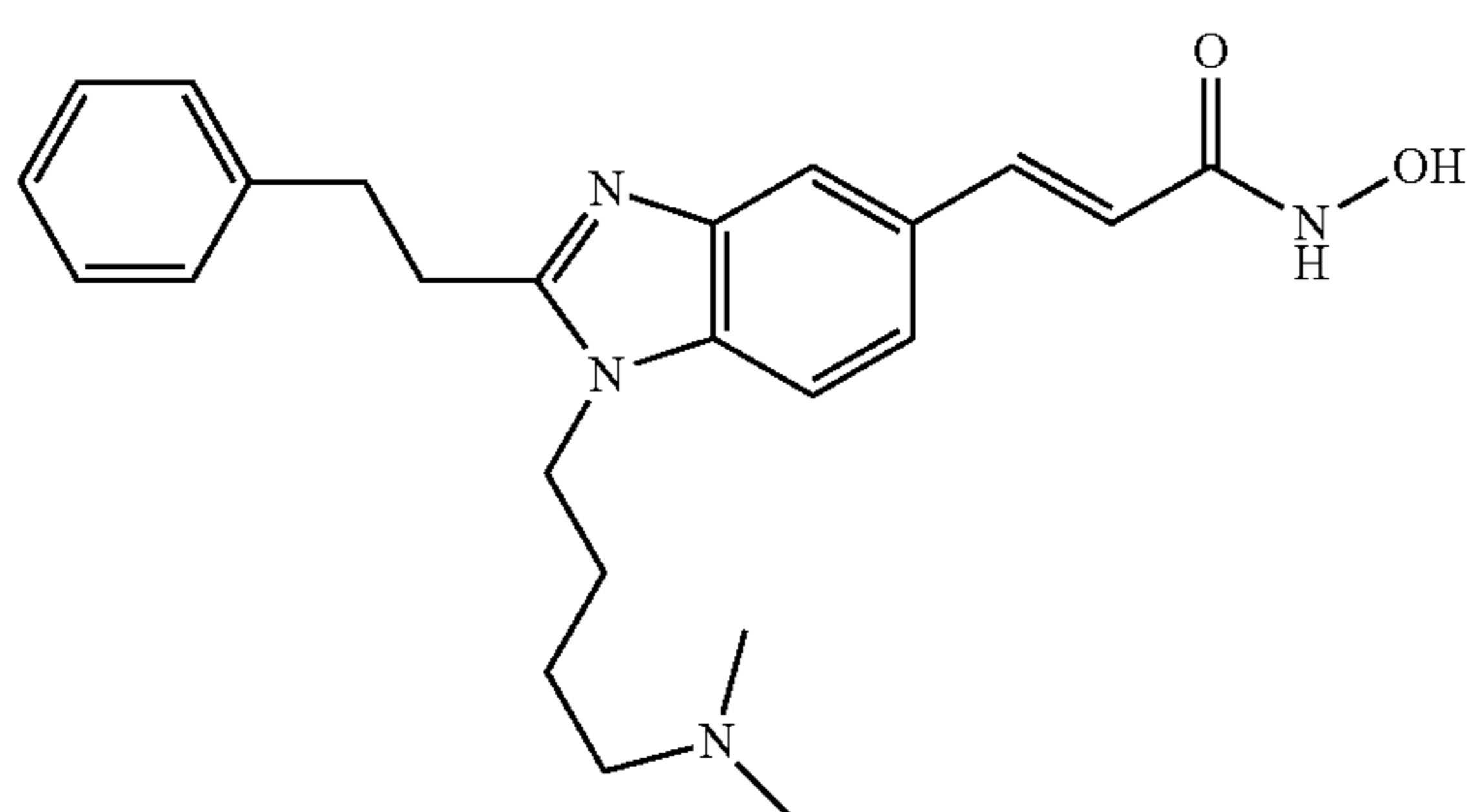
N-Hydroxy-3-[1-(4-dimethylamino-butyl)-2-phenethyl-1H-benzimidazol-5-yl]-acrylamide
