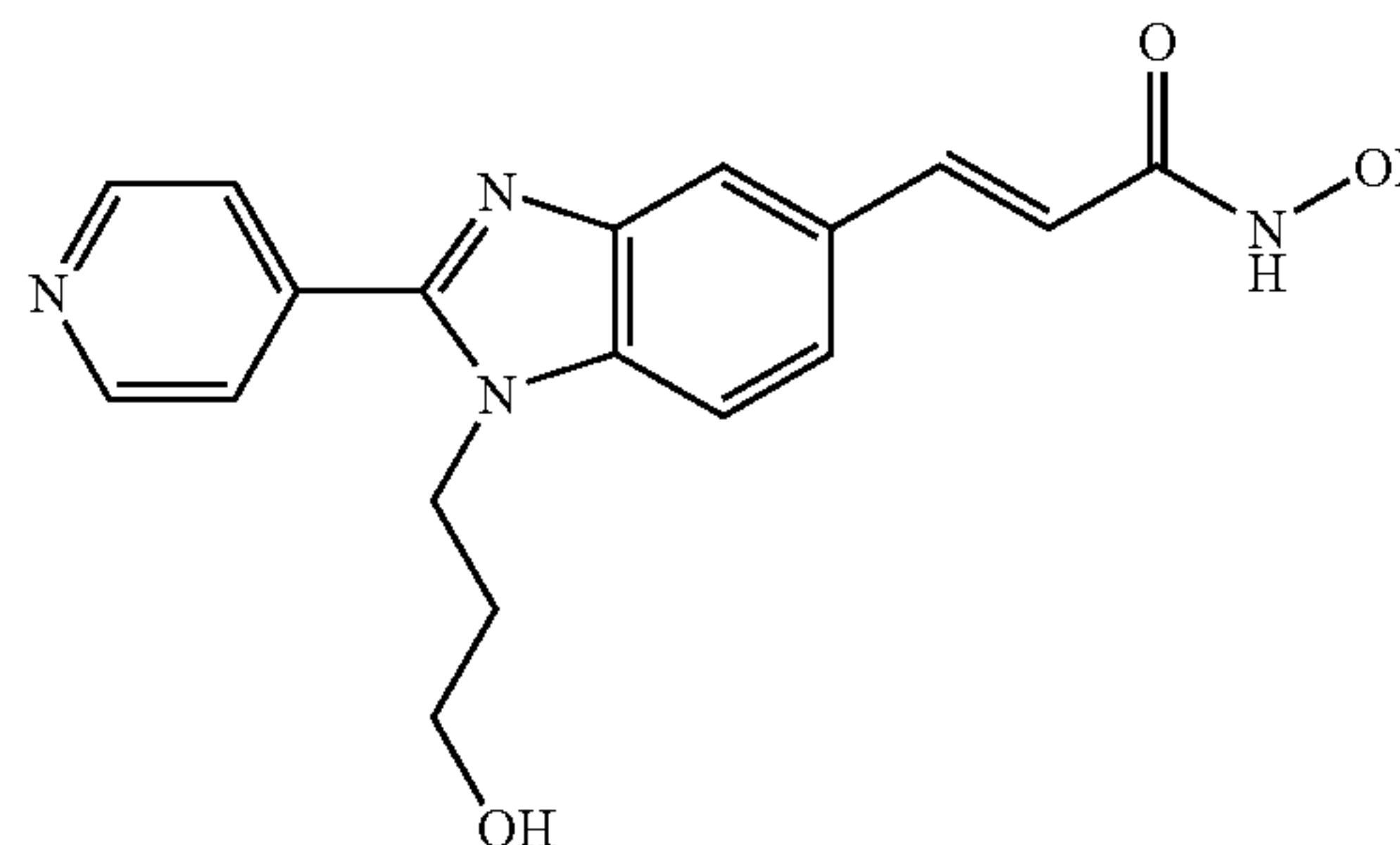
N-Hydroxy-3-[1-(3-hydroxy-propyl)-2-(4-pyridyl)-1H-benzimidazole-5-yl]-acrylamide
