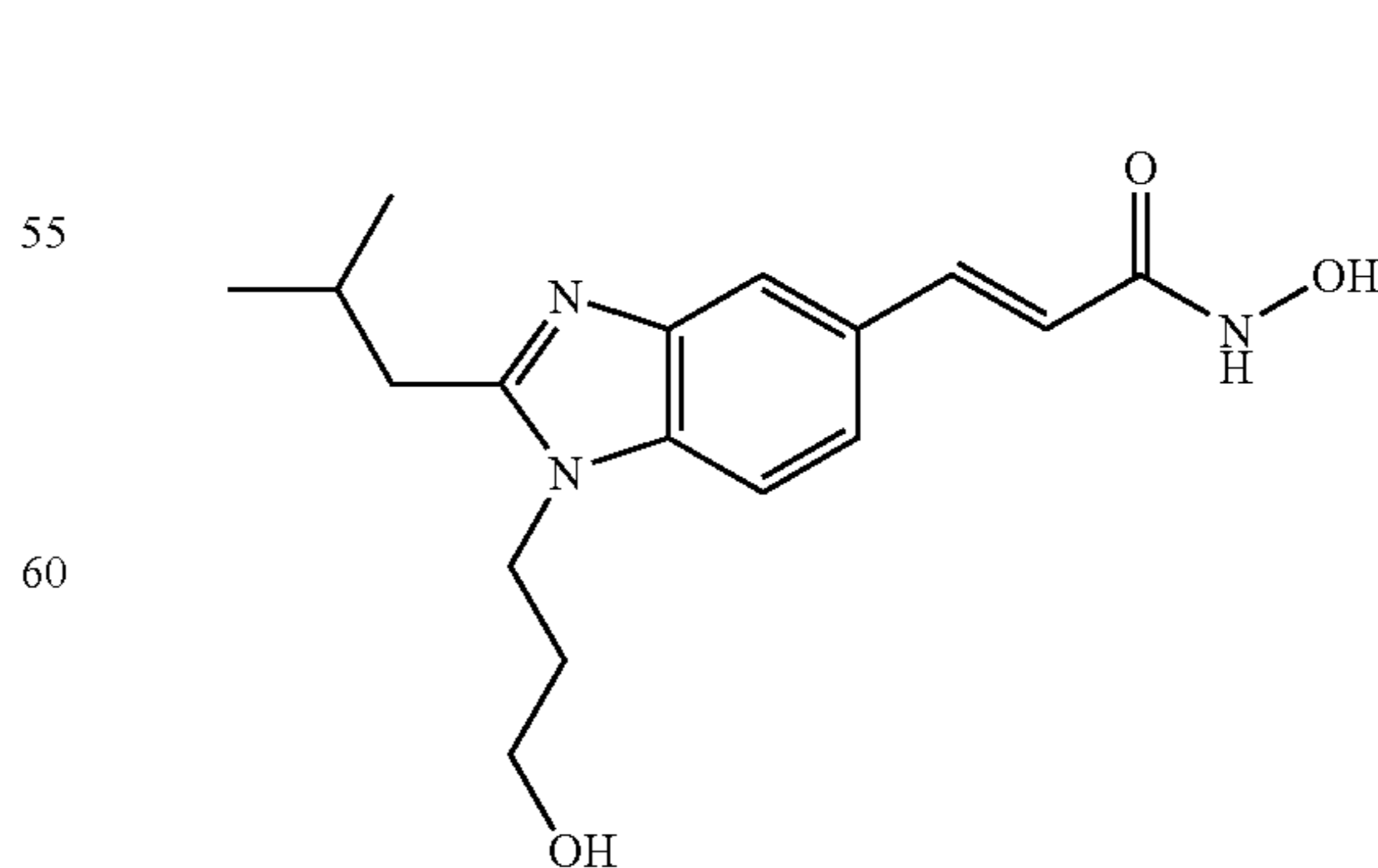
N-Hydroxy-3-[1-(3-hydroxy-propyl)-2-isobutyl-1H-benzimidazol-5-yl]-acrylamide
