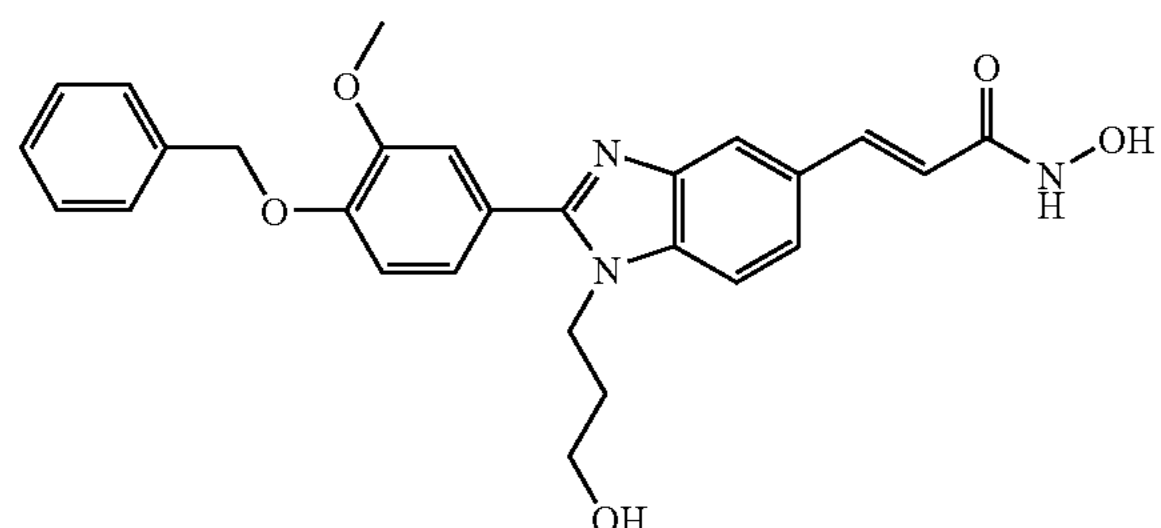
N-Hydroxy-3-[2-(4-benzyloxy-3-methoxy-phenyl)-1-(3-hydroxy-propyl)-1H-benzimidazole-5-yl]-acrylamide
