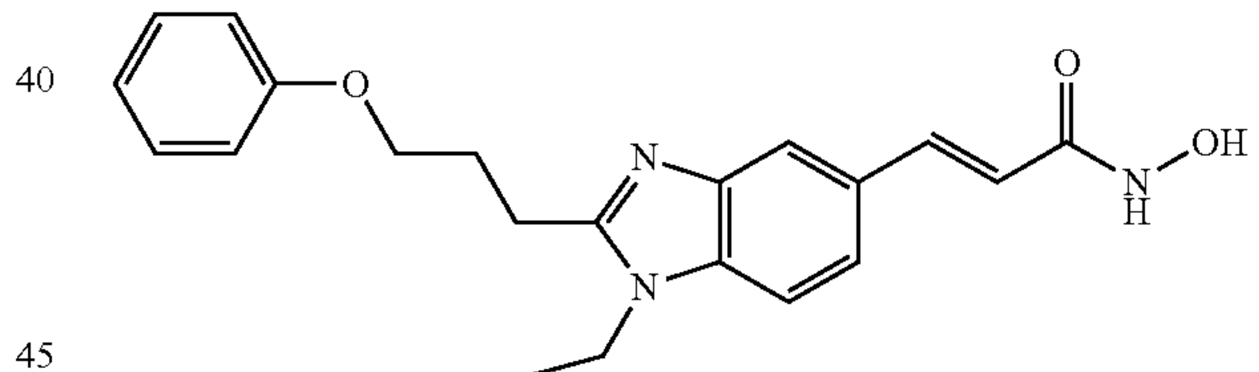
N-Hydroxy-3-[1-ethyl-2-(3-phenoxy-propyl)-1H-benzimidazol-5-yl]-acrylamide
