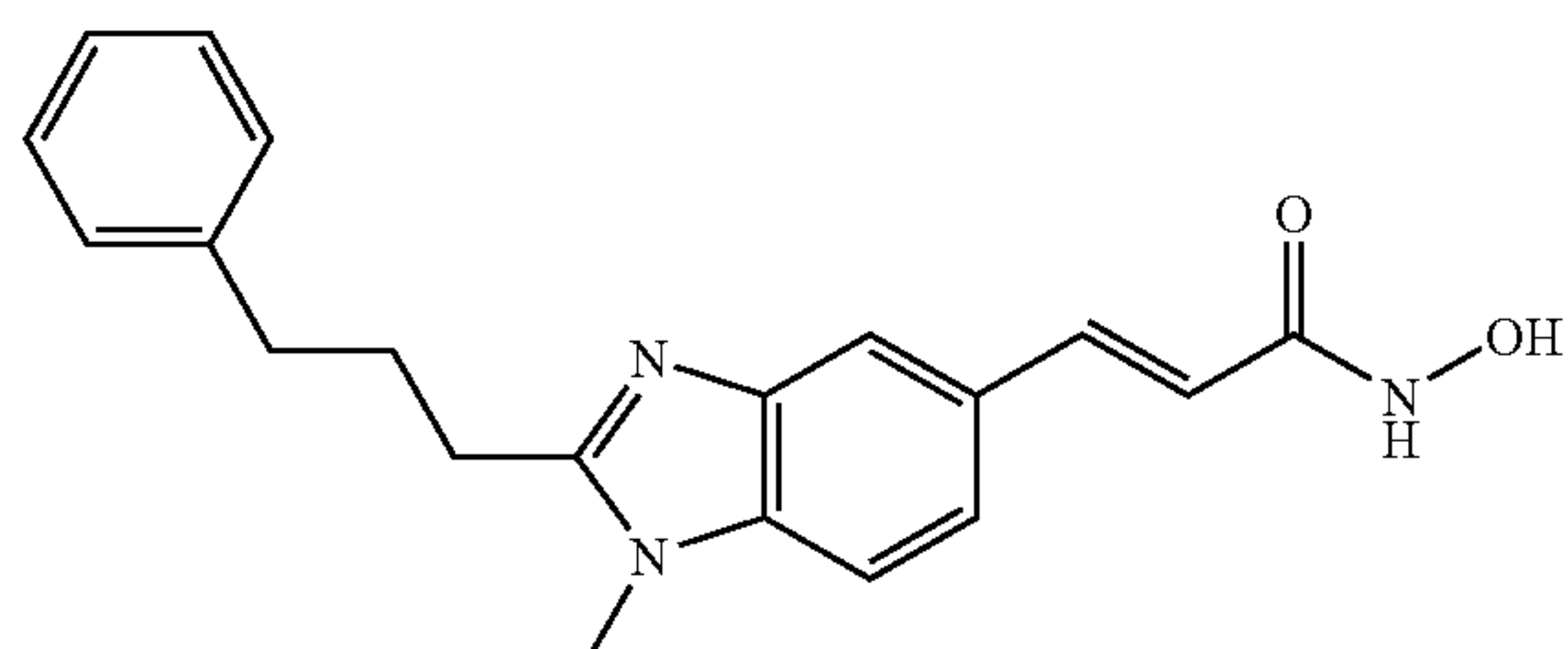
N-Hydroxy-3-[1-methyl-2-(3-phenyl-propyl)-1H-benzimidazol-5-yl]-acrylamide
