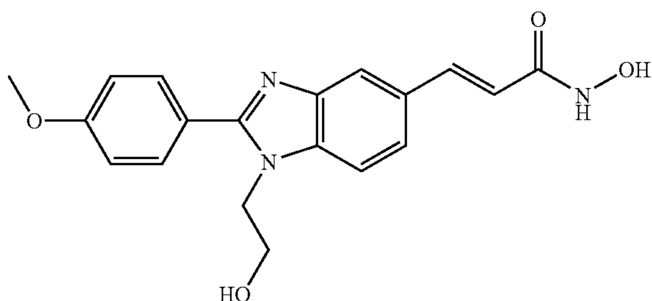
N-Hydroxy-3-[1-(2-hydroxy-ethyl)-2-(4-methoxy-phenyl)-1H-benzimidazole-5-yl]-acrylamide
