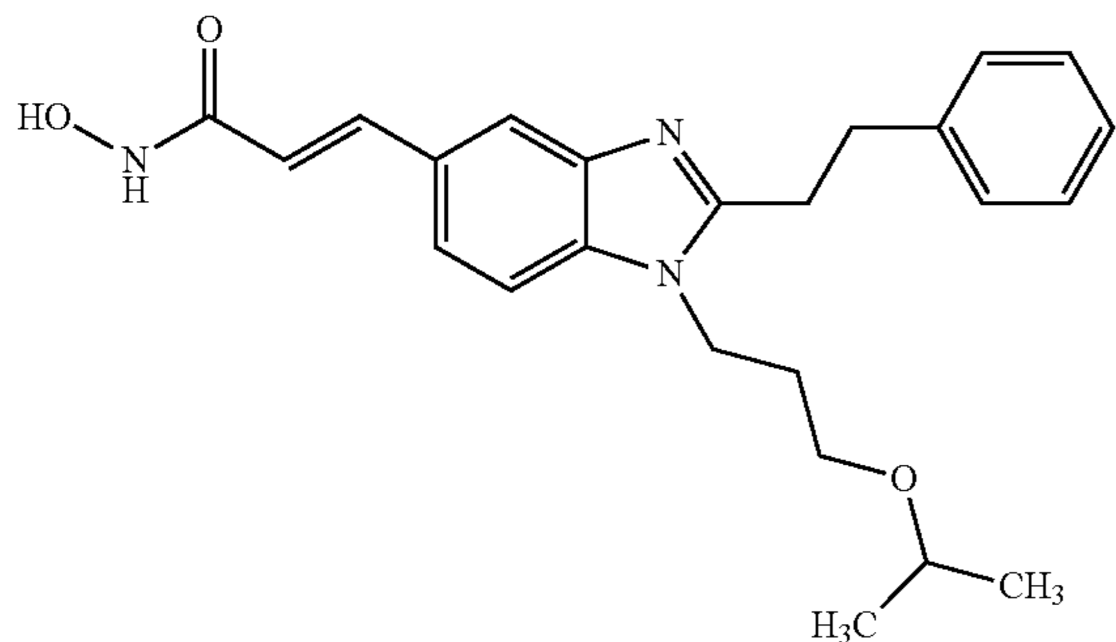
N-Hydroxy-3-(1-(3-isopropoxy-propyl)-2-phenethyl-1H-benzimidazol-5-yl)-acrylamide
