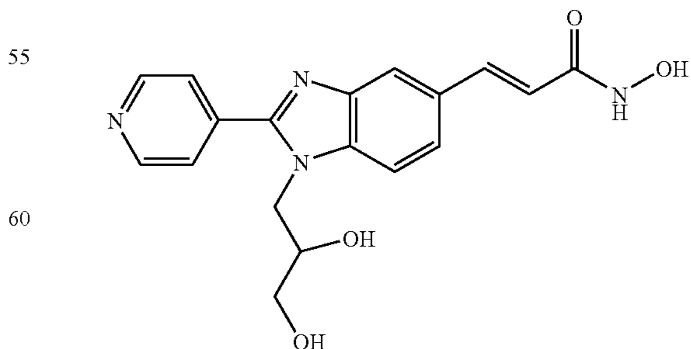
N-Hydroxy-3-[1-(2,3-hydroxy-propyl)-2-(4-pyridyl)-1H-benzimidazole-5-yl]-acrylamide
