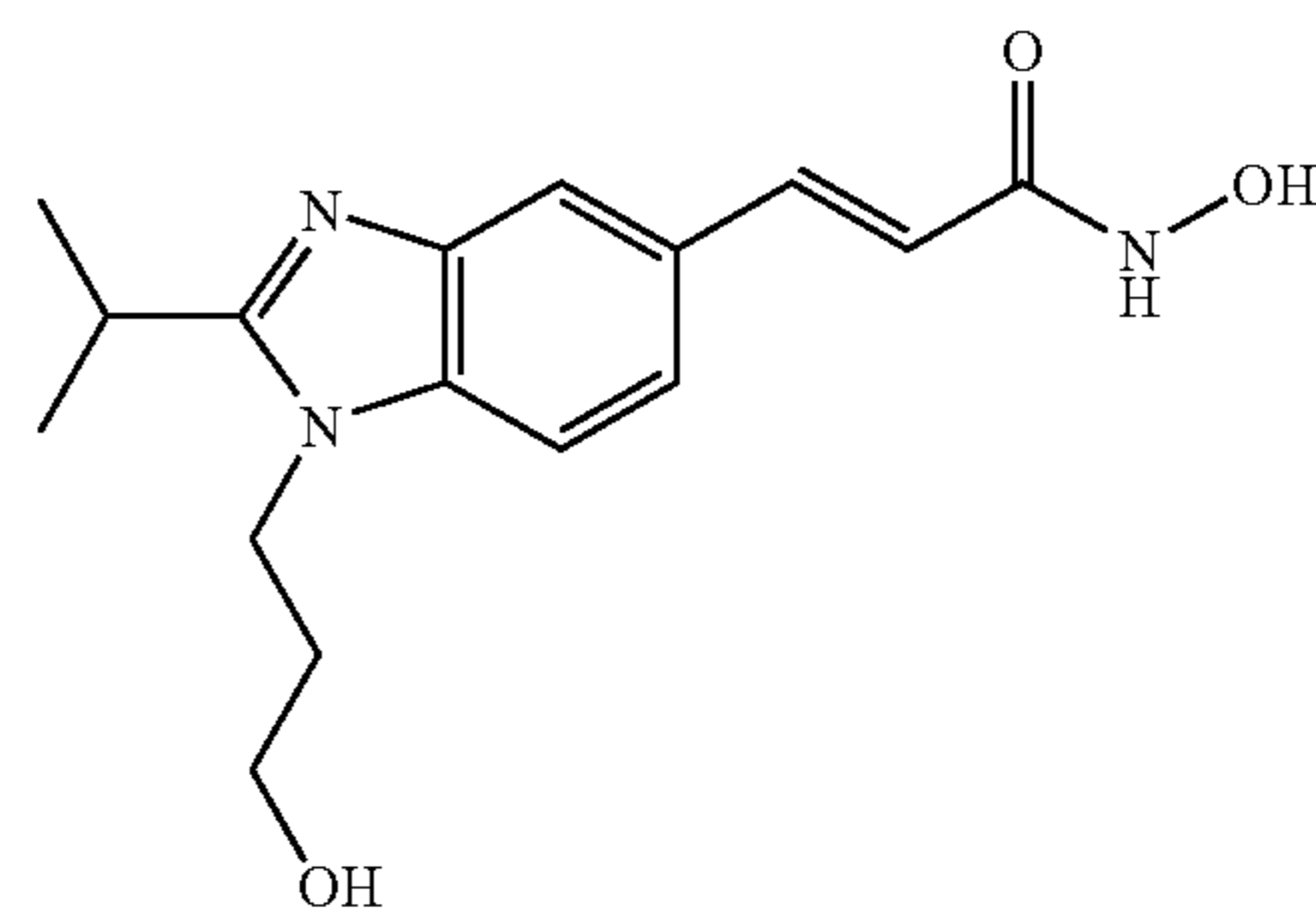
N-hydroxy-3-[1-(3-hydroxy-propyl)-2-isopropyl-1H-benzimidazol-5-yl]-acrylamide
