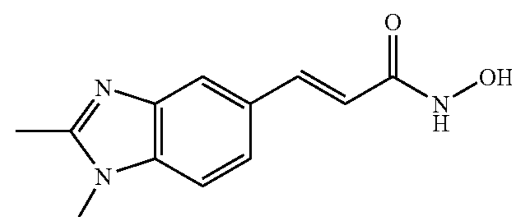
N-Hydroxy-3-(1,2-dimethyl-1H-benzimidazol-5-yl)-acrylamide
