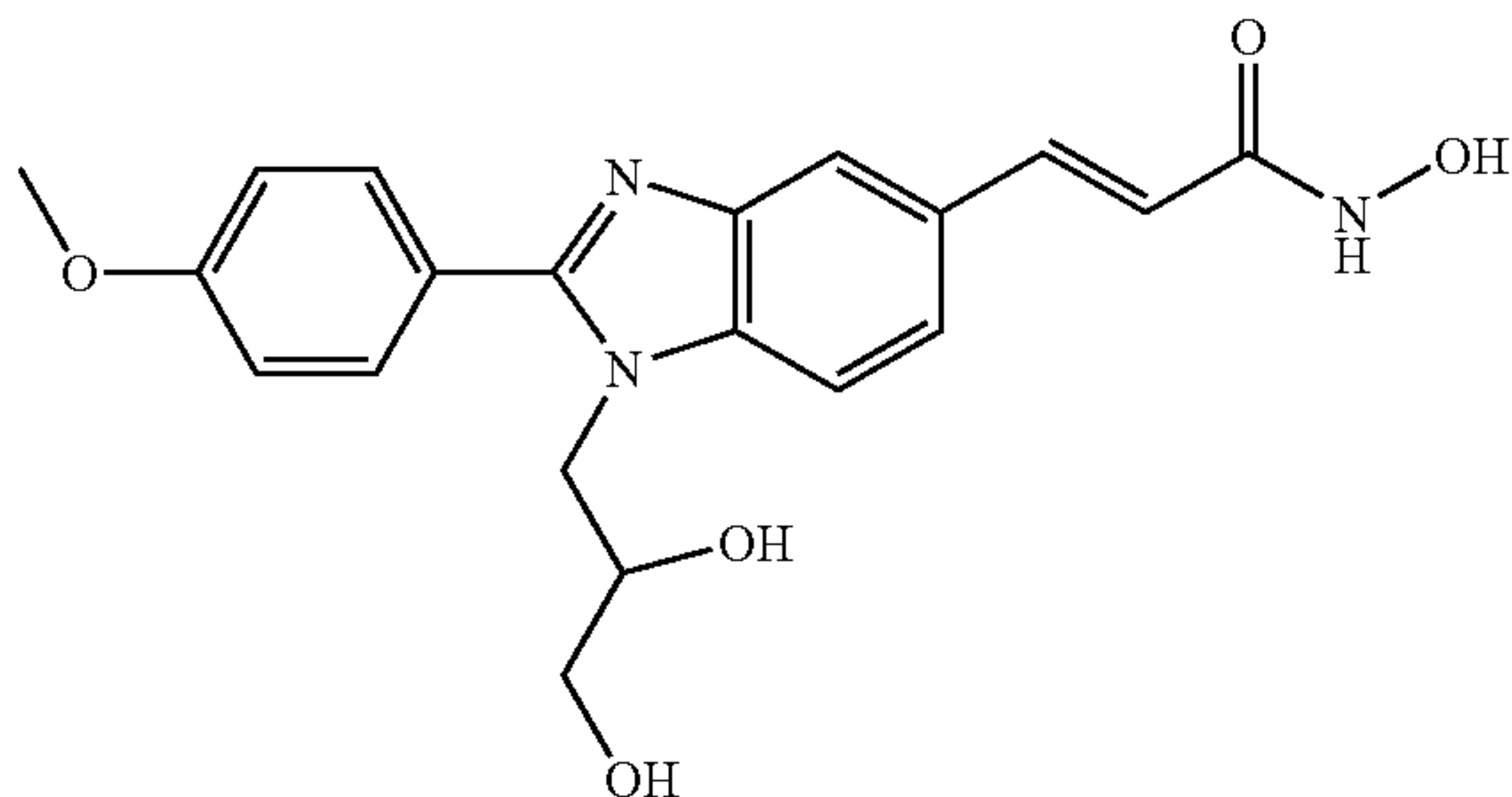
N-Hydroxy-3-[1-(2,3-hydroxy-propyl)-2-(4-methoxy-phenyl)-1H-benzimidazole-5-yl]-acrylamide
