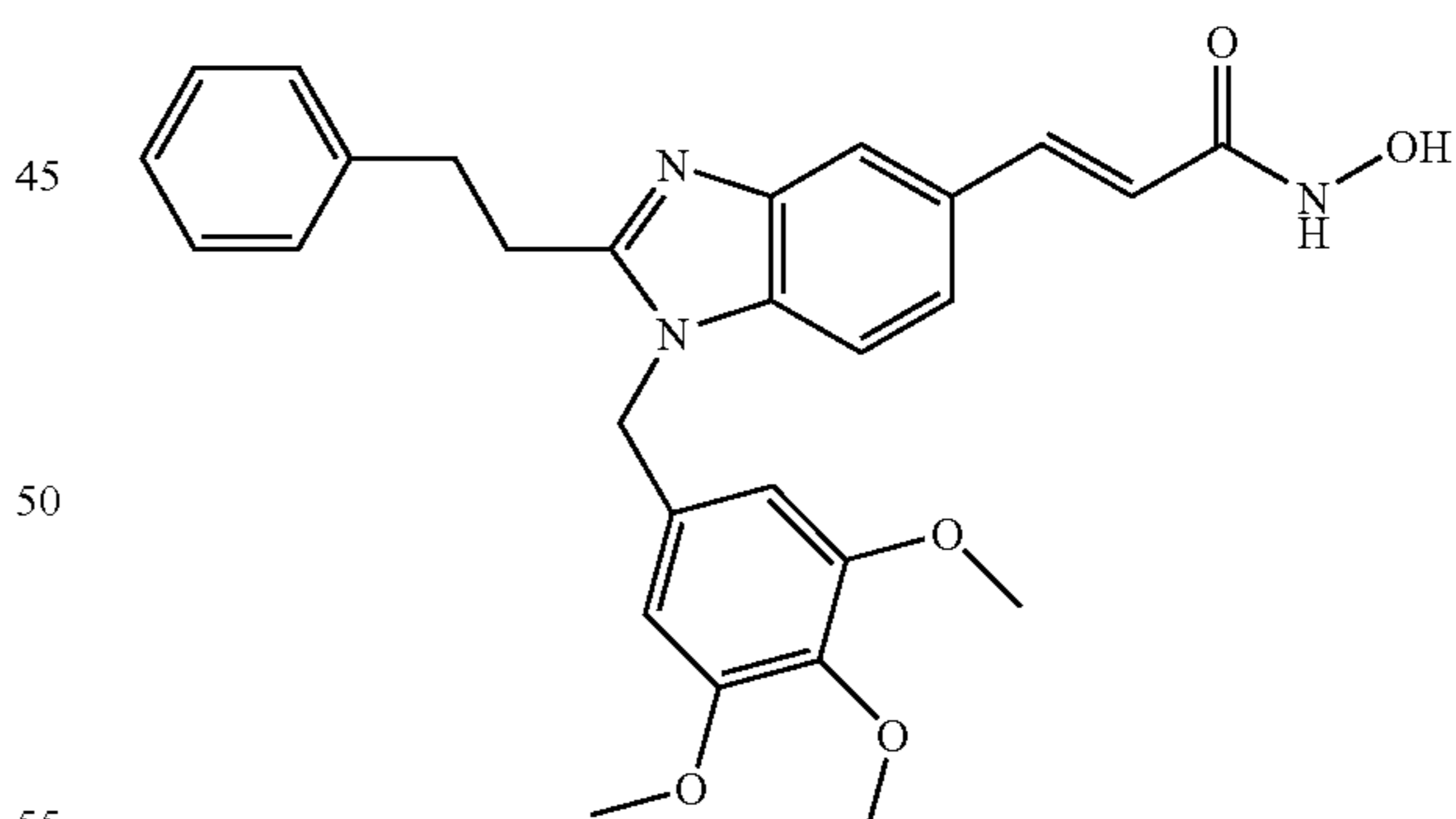
N-Hydroxy-3-[1-(3,4,5-trimethoxybenzyl)-2-(2-phenyl-ethyl)-1H-benzimidazol-5-yl]-acrylamide
