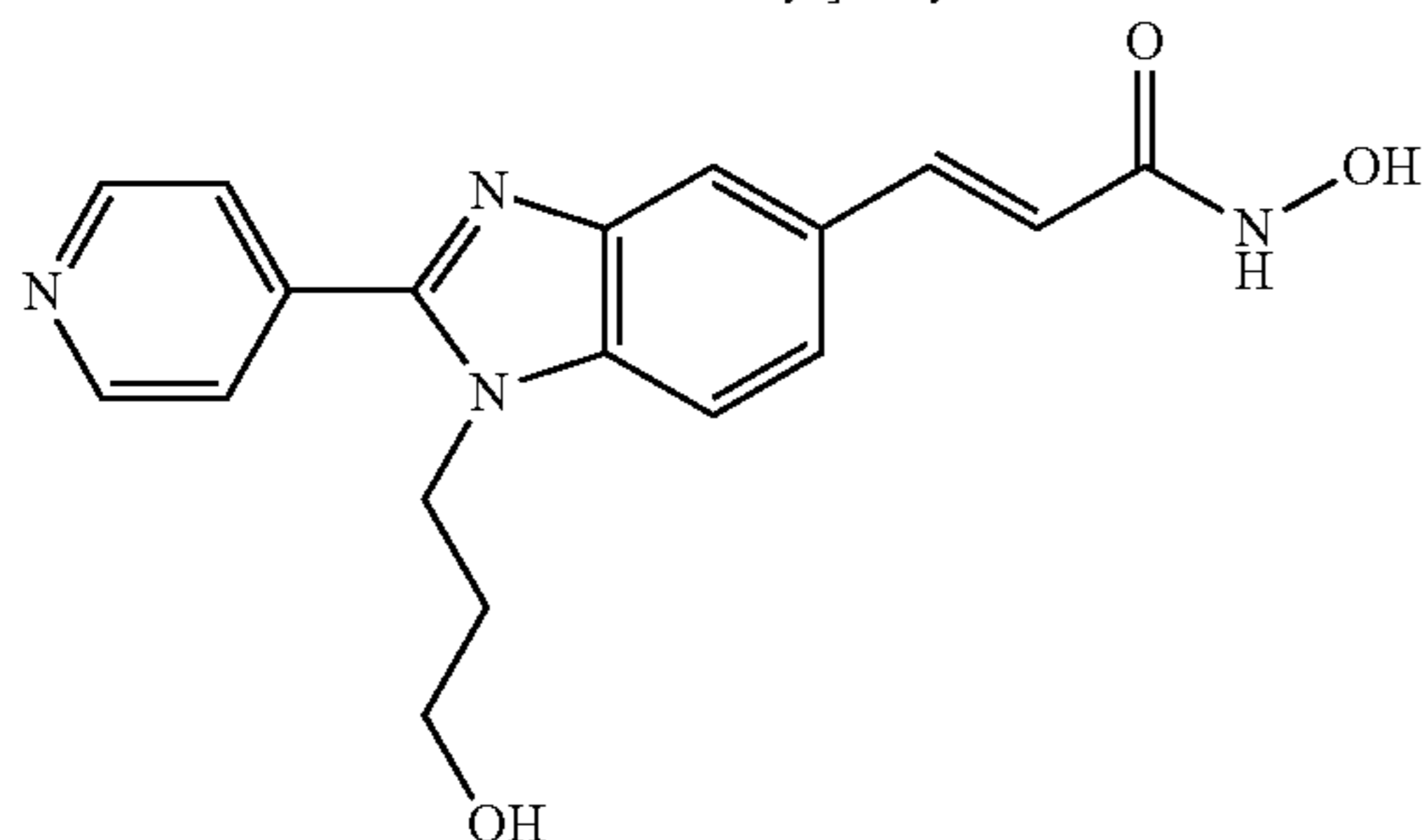
N-Hydroxy-3-[1-(3-hydroxy-propyl)-2-(4-pyridyl)-1H-benzimidazol-5-yl]-acrylamide
