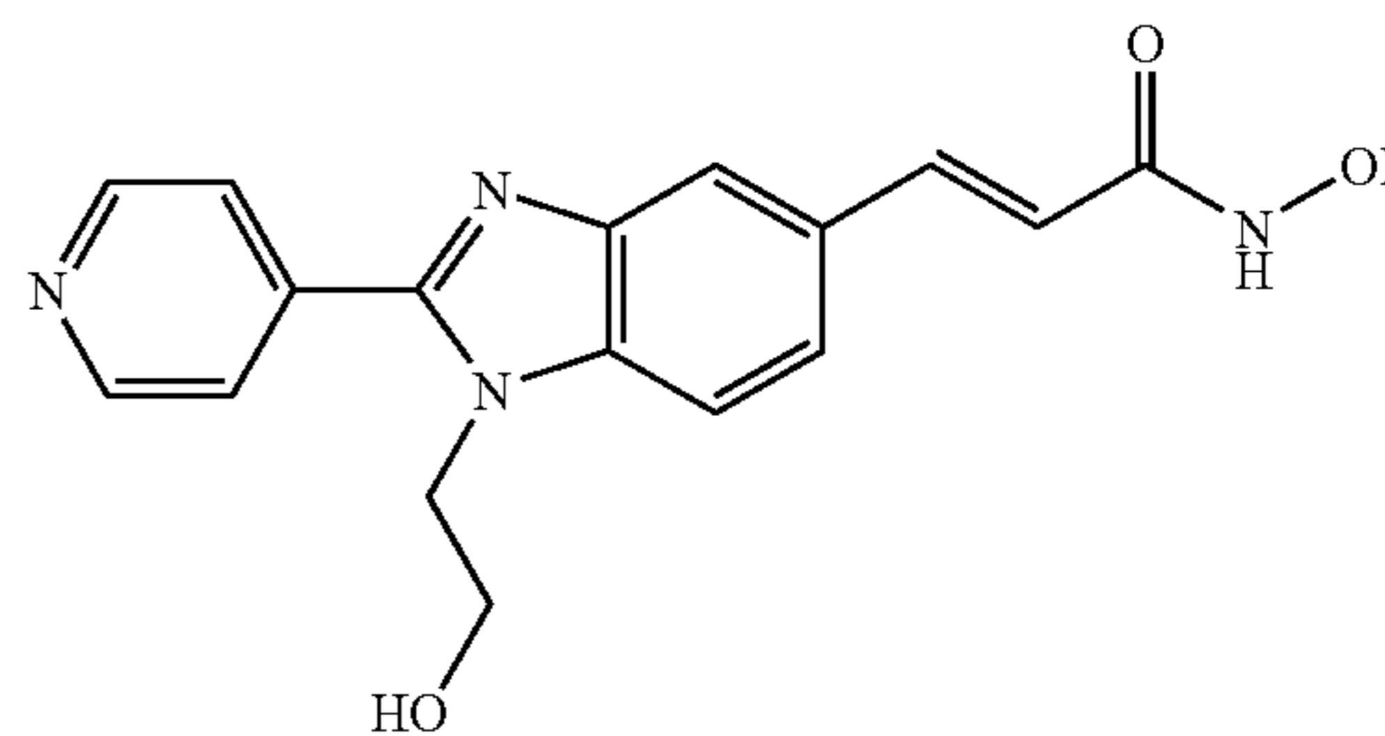
N-Hydroxy-3-[1-(2-hydroxy-ethyl)-2-(4-pyridyl)-1H-benzimidazole-5-yl]-acrylamide
