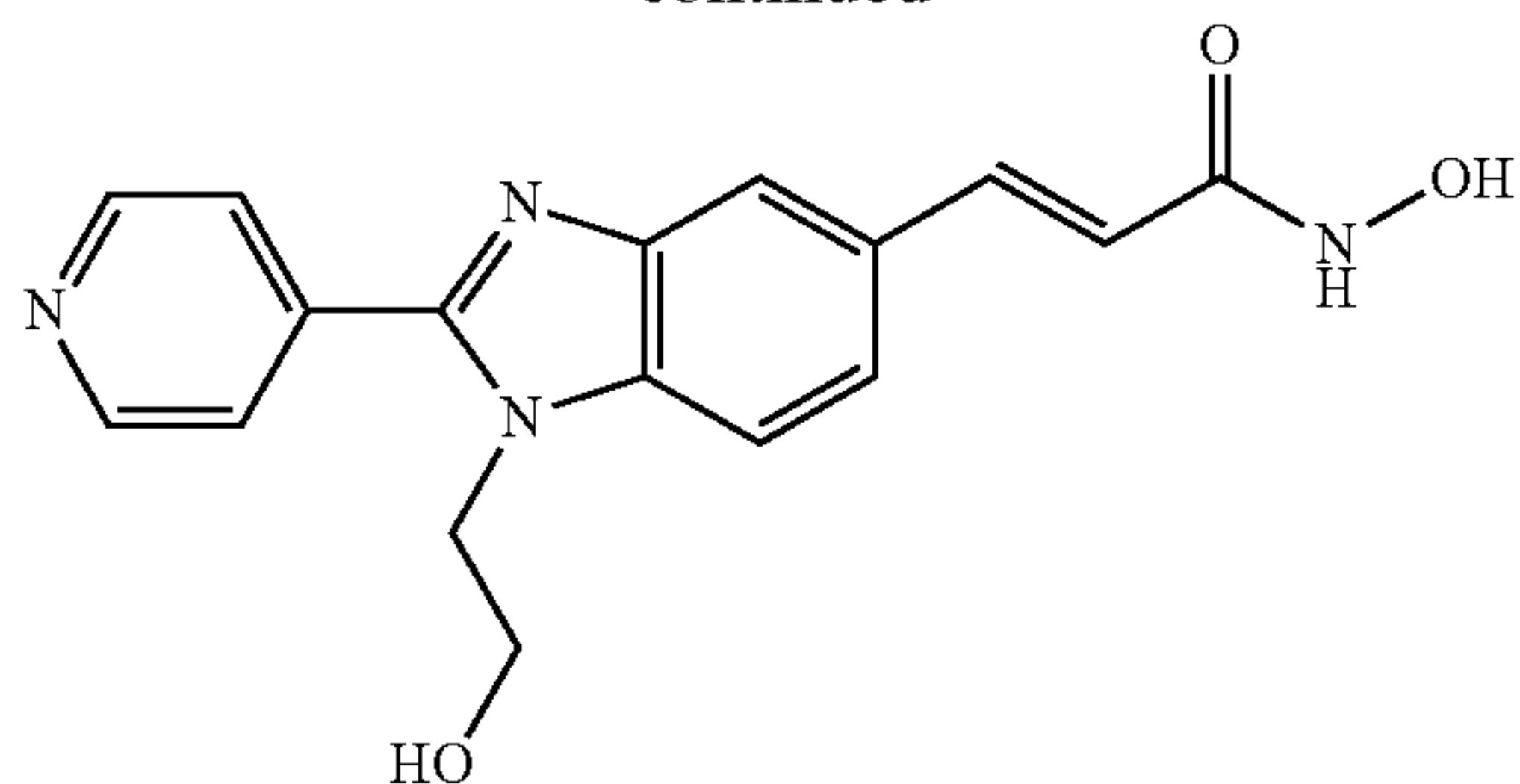
N-Hydroxy-3-[1-(2-hydroxy-ethyl)-2-(4-pyridyl)-1H-benzimidazol-5-yl]-acrylamide
