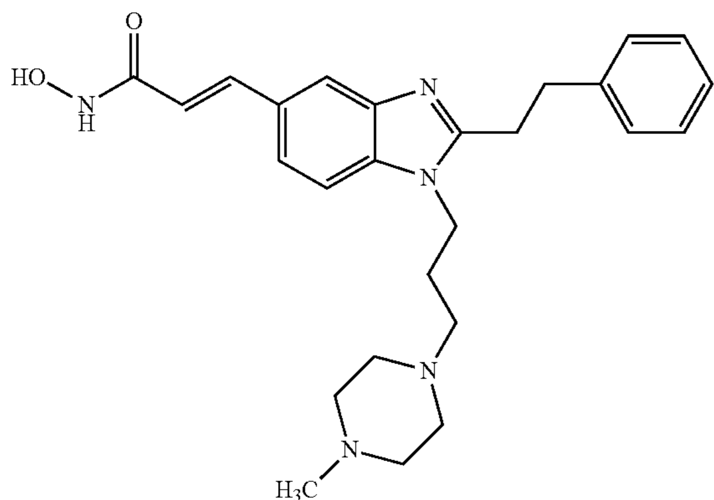
N-Hydroxy-3-(1-[3-(4-methyl-piperzin-1-yl)-2-phenethyl-1H-benzimidazol-5-yl]-acrylamide
