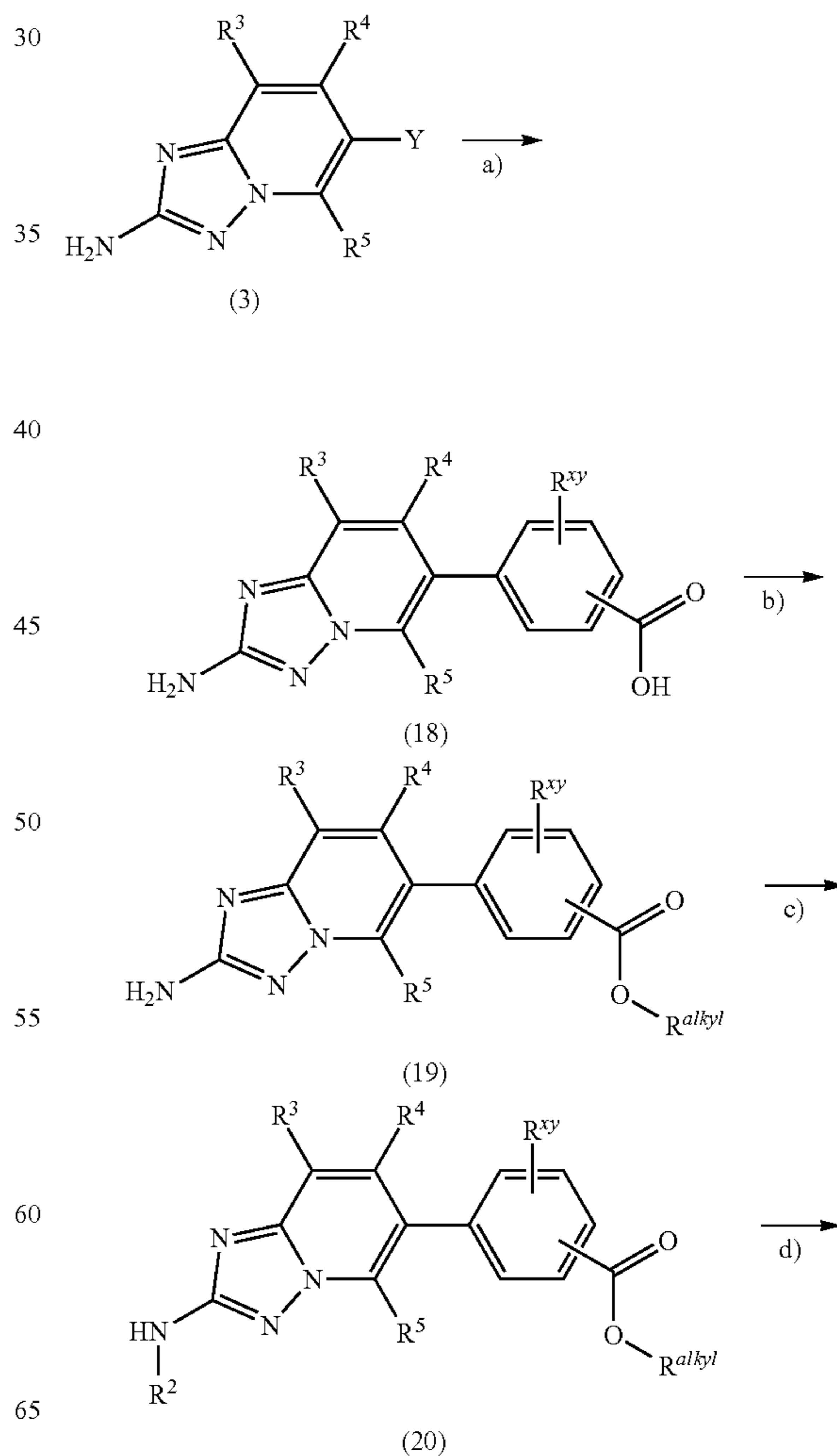
Scheme 7: Synthesis of compounds of general formula (22)
