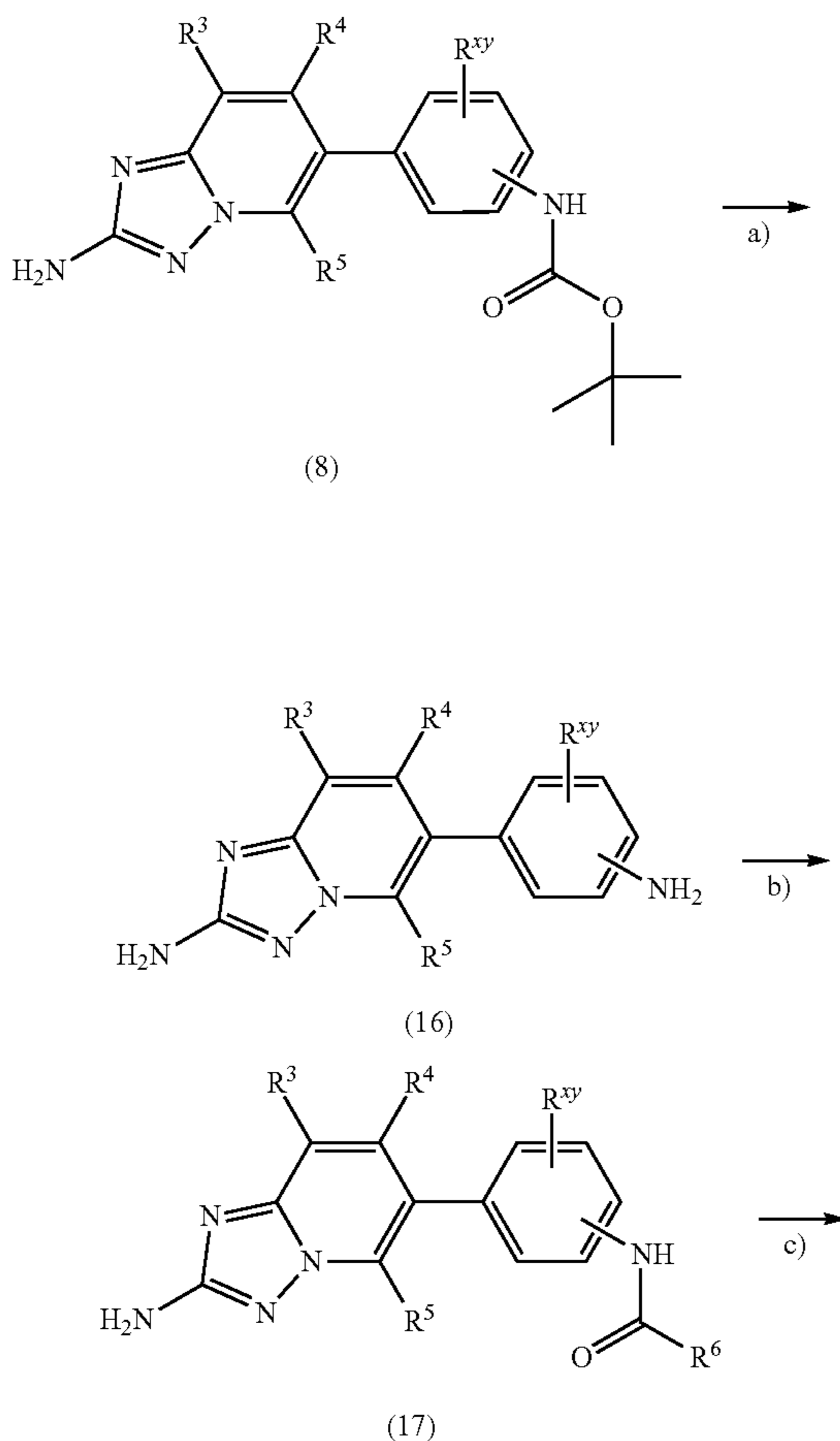
Scheme 6: Synthesis of compounds of general formula (11)
